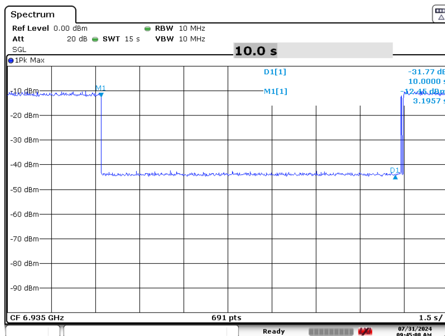
Plot 7-142. Contention Based Protocol Timing Plot (20MHz (UNII Band 8) – Ch. 197)
