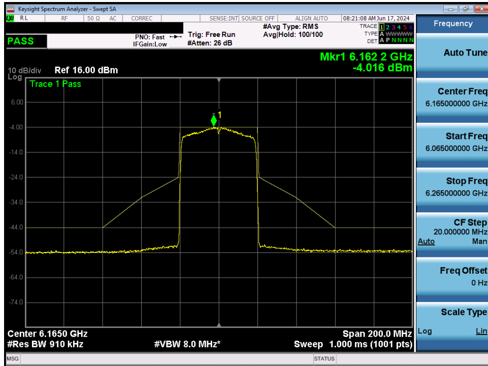
Plot 7-110. In-Band Emission MIMO ANT2 (40MHz 802.11ax (UNII Band 5) – Ch. 43)
