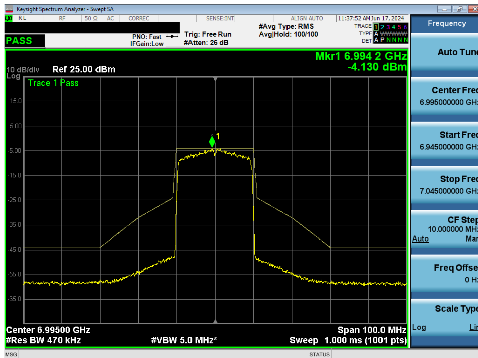
Plot 7-104. In-Band Emission MIMO ANT1 (20MHz 802.11ax (UNII Band 8) – Ch. 209)
