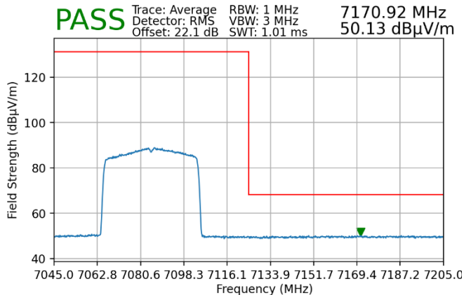
Plot 7-162. Radiated Upper Band Edge Plot SISO ANT1 (Average – UNII Band 8)
