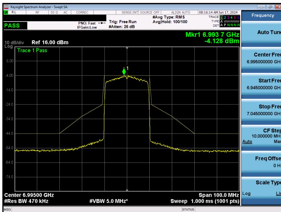
Plot 7-124. In-Band Emission MIMO ANT2 (20MHz 802.11ax (UNII Band 8) – Ch. 209)
