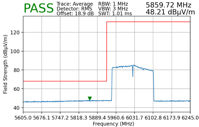
Plot 7-168. Radiated Lower Band Edge Plot SISO ANT1 (Average – UNII Band 5)
