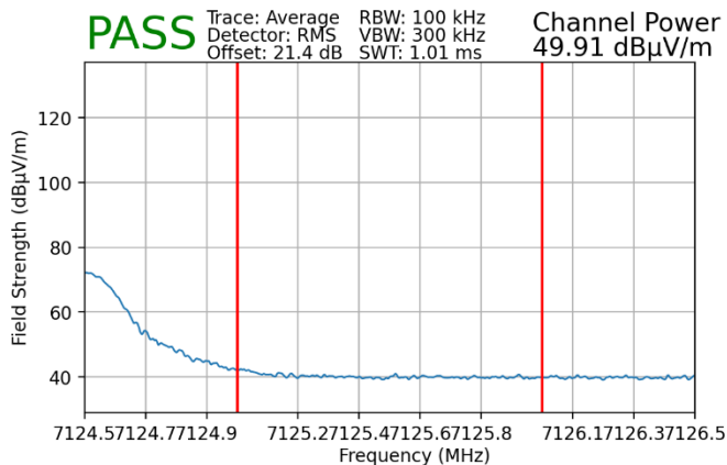
Plot 7-174. Radiated Upper Band Edge Plot SISO ANT2 (Average – UNII Band 8)
