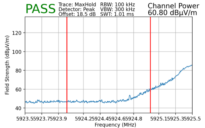
Plot 7-157. Radiated Lower Band Edge Plot SISO ANT1 (Peak – UNII Band 5)
