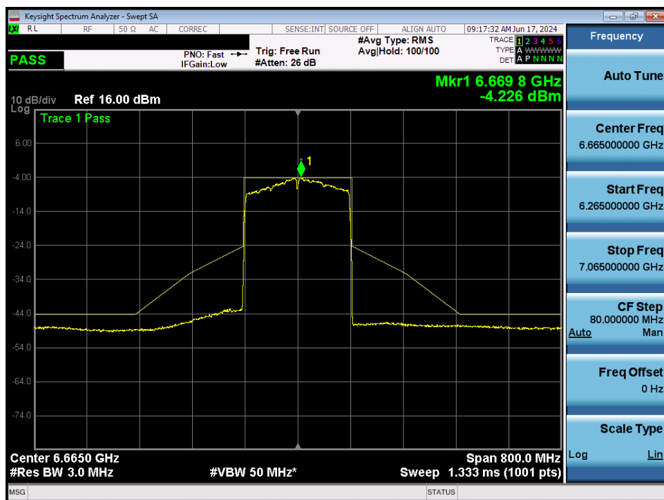
Plot 7-122. In-Band Emission MIMO ANT2 (160MHz 802.11ax (UNII Band 7) – Ch. 143)
