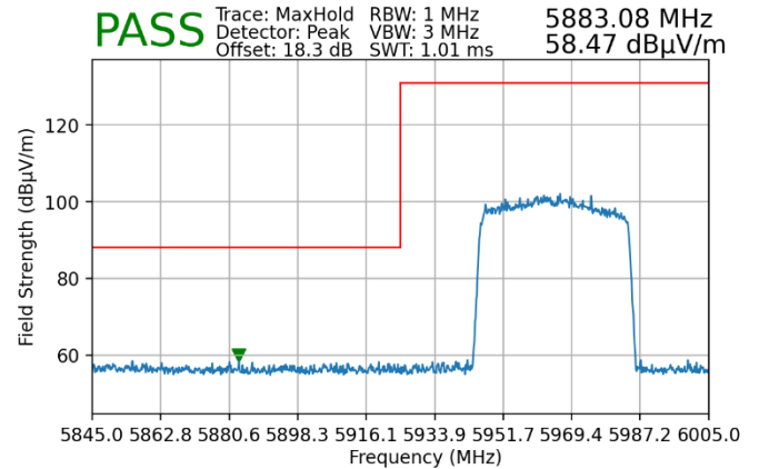
Plot 7-161. Radiated Lower Band Edge Plot SISO ANT1 (Peak – UNII Band 5)
