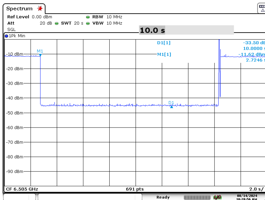
Plot 7-136. Contention Based Protocol Timing Plot (160MHz (UNII Band 6) – Ch. 111 Mid)
