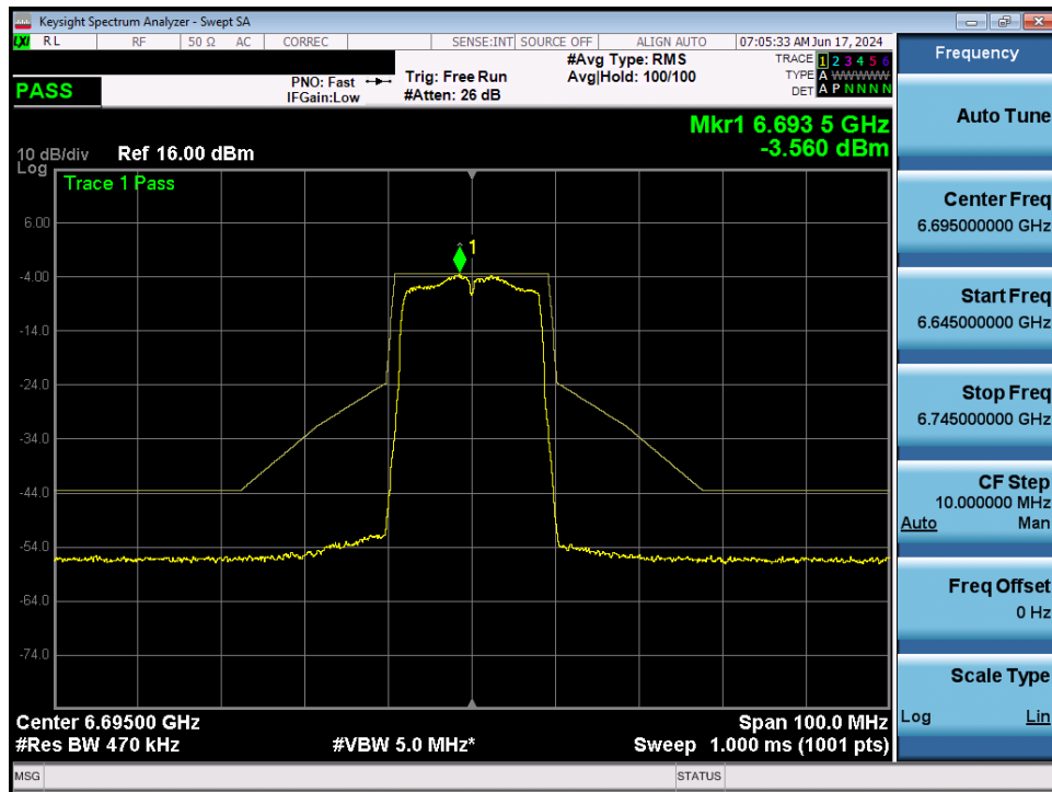
Plot 7-118. In-Band Emission MIMO ANT2 (20MHz 802.11a (UNII Band 7) – Ch. 149)
