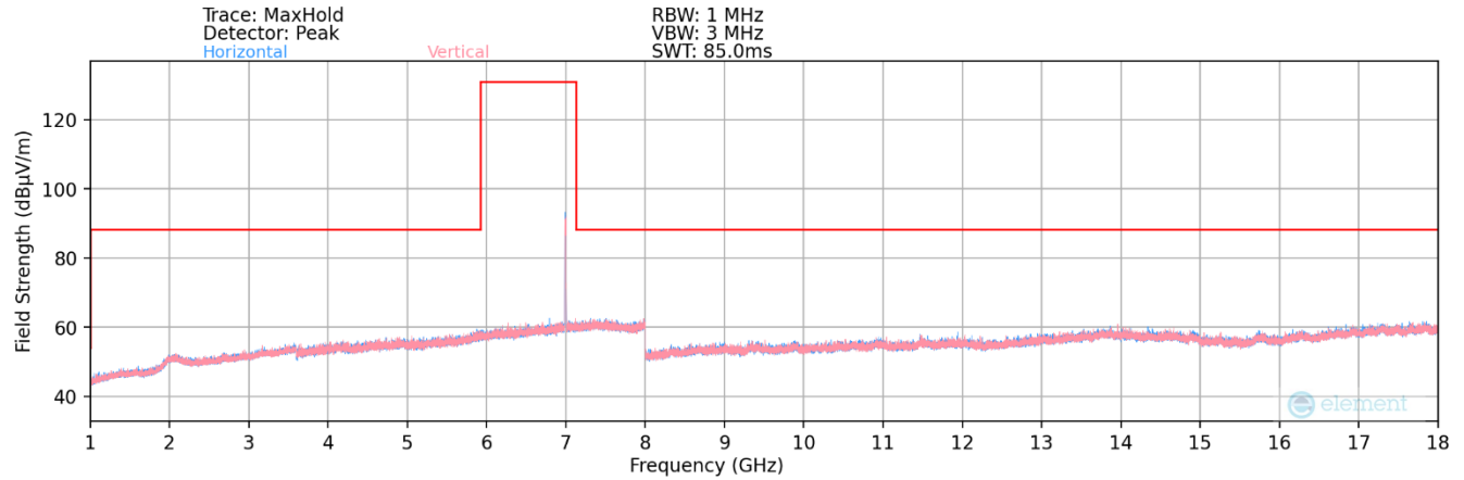
Plot 7-153. Radiated Spurious Plot 1GHz – 18GHz MIMO (802.11a – U Band 8 Ch. 209 – LPI)
