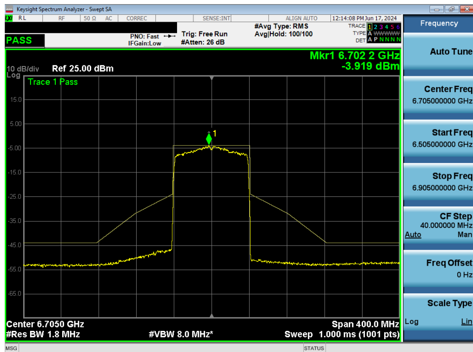
Plot 7-101. In-Band Emission MIMO ANT1 (80MHz 802.11ax (UNII Band 7) – Ch. 151)
