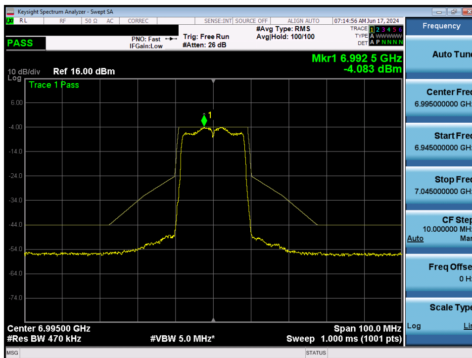
Plot 7-123. In-Band Emission MIMO ANT2 (20MHz 802.11a (UNII Band 8) – Ch. 209)
