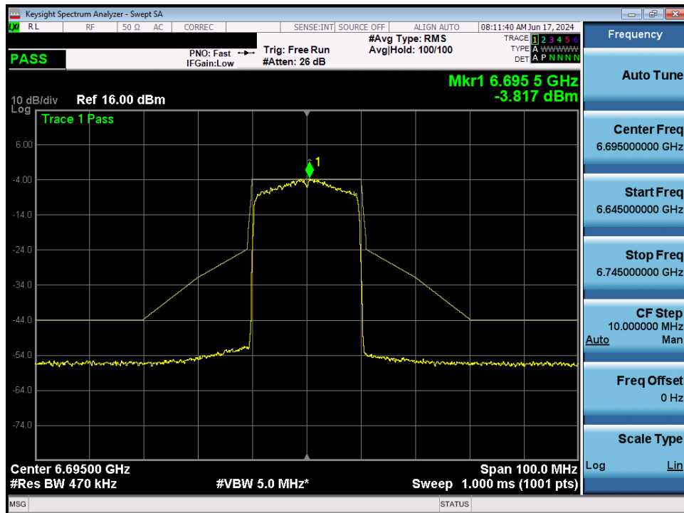
Plot 7-119. In-Band Emission MIMO ANT2 (20MHz 802.11ax (UNII Band 7) – Ch. 149)
