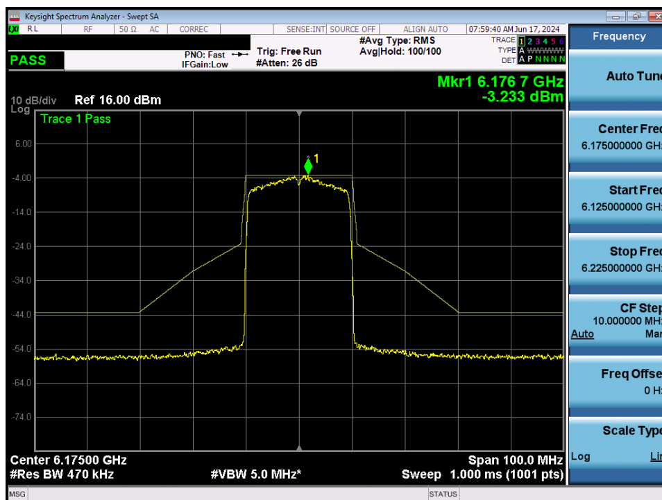
Plot 7-109. In-Band Emission MIMO ANT2 (20MHz 802.11ax (UNII Band 5) – Ch. 45)
