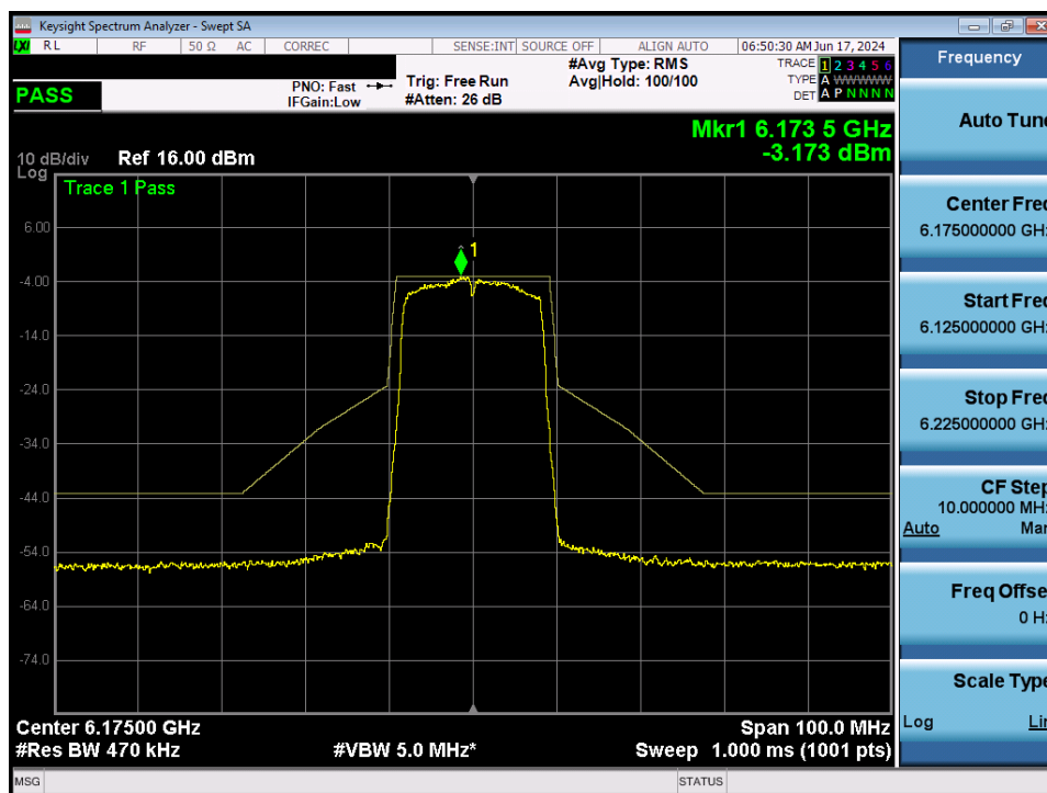
Plot 7-108. In-Band Emission MIMO ANT2 (20MHz 802.11a (UNII Band 5) – Ch. 45)
