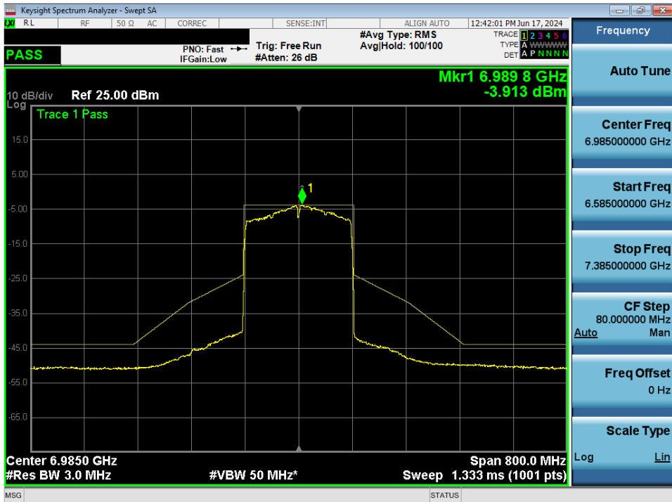
Plot 7-107. In-Band Emission MIMO ANT1 (160MHz 802.11ax (UNII Band 8) – Ch. 207)
