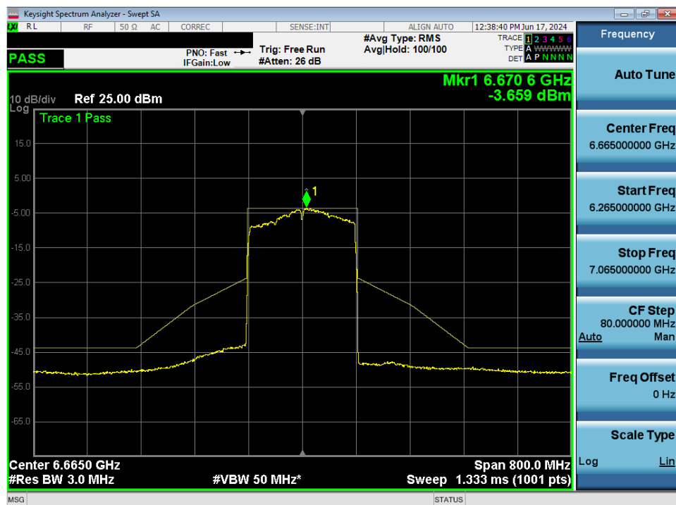
Plot 7-102. In-Band Emission MIMO ANT1 (160MHz 802.11ax (UNII Band 7) – Ch. 143)
