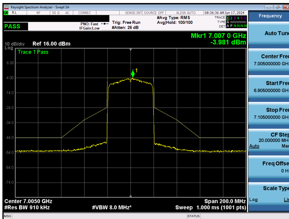
Plot 7-125. In-Band Emission MIMO ANT2 (40MHz 802.11ax (UNII Band 8) – Ch. 211)
