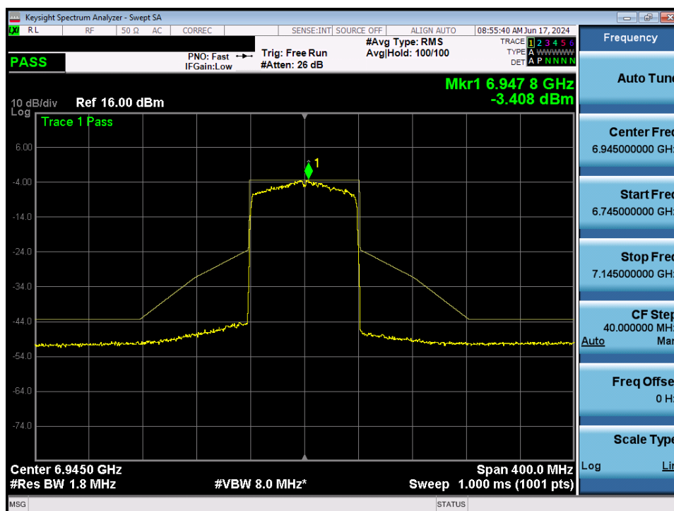
Plot 7-126. In-Band Emission MIMO ANT2 (80MHz 802.11ax (UNII Band 8) – Ch. 199)
