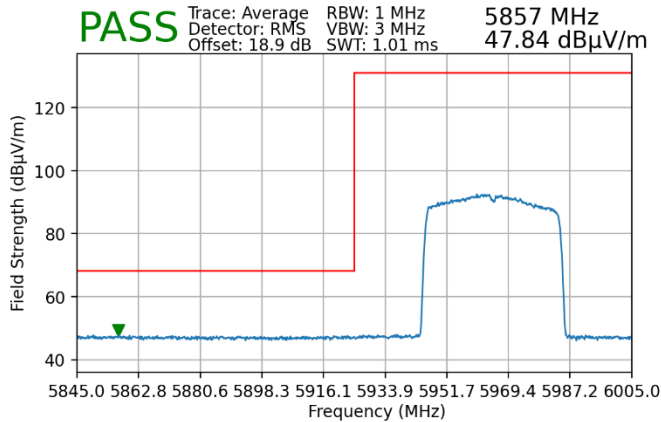
Plot 7-160. Radiated Lower Band Edge Plot SISO ANT1 (Average – UNII Band 5)
