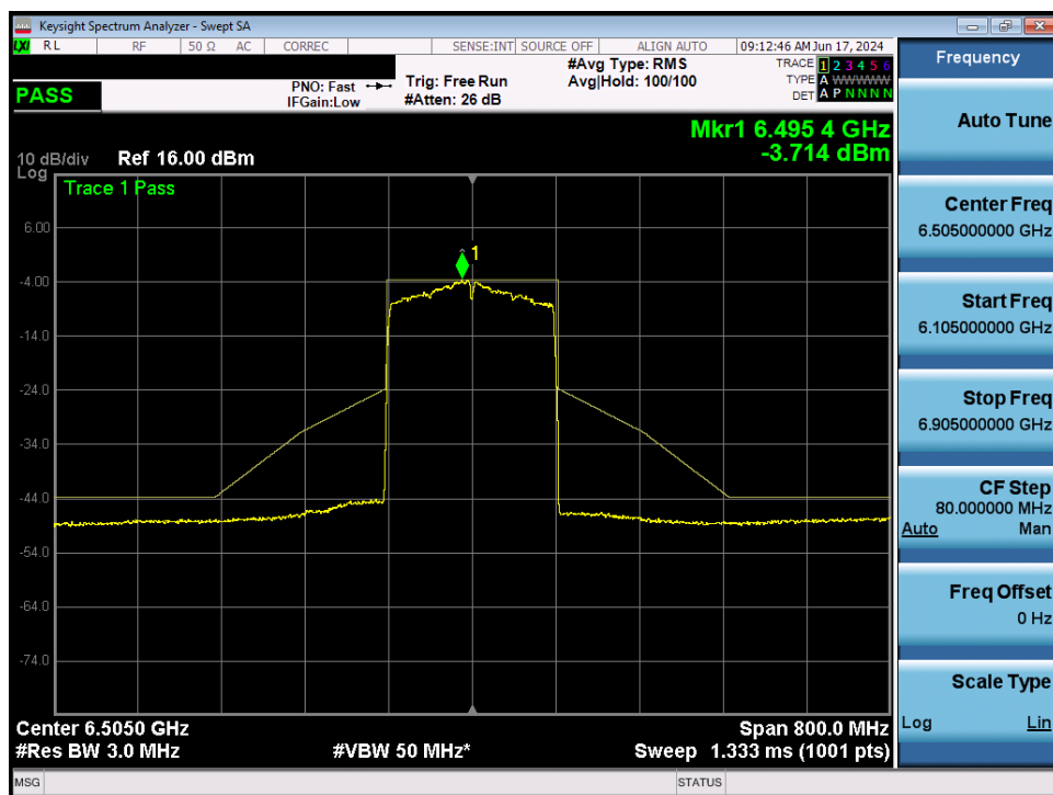
Plot 7-117. In-Band Emission MIMO ANT2 (160MHz 802.11ax (UNII Band 6) – Ch. 111)
