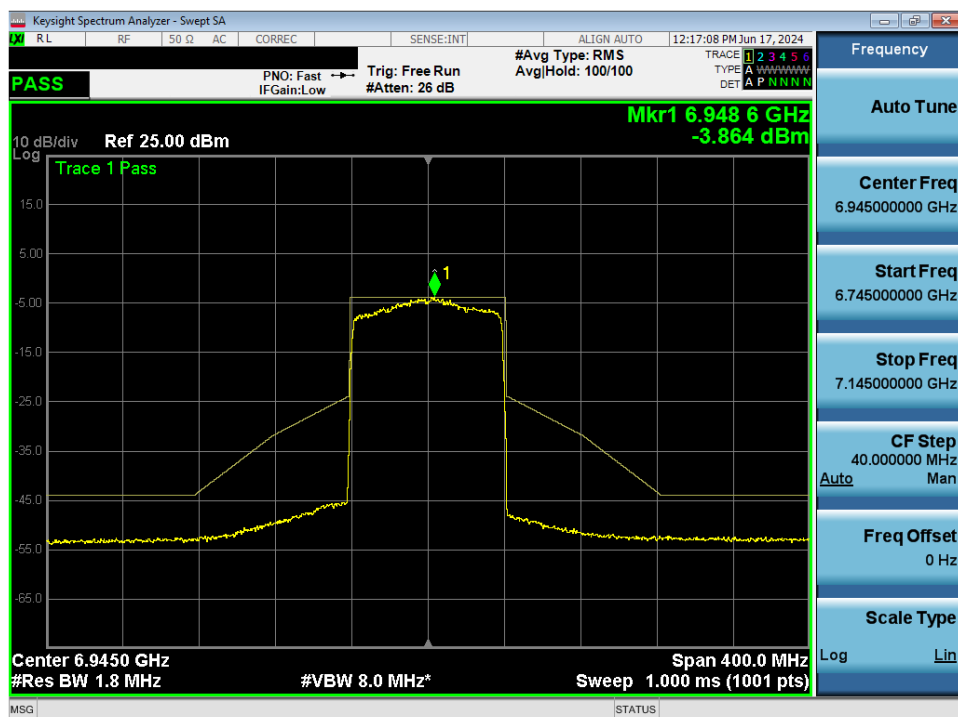
Plot 7-106. In-Band Emission MIMO ANT1 (80MHz 802.11ax (UNII Band 8) – Ch. 199)
