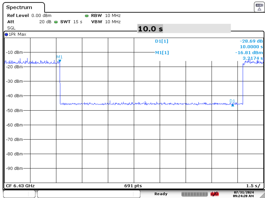
Plot 7-134. Contention Based Protocol Timing Plot (20MHz (UNII Band 6) – Ch. 101)
