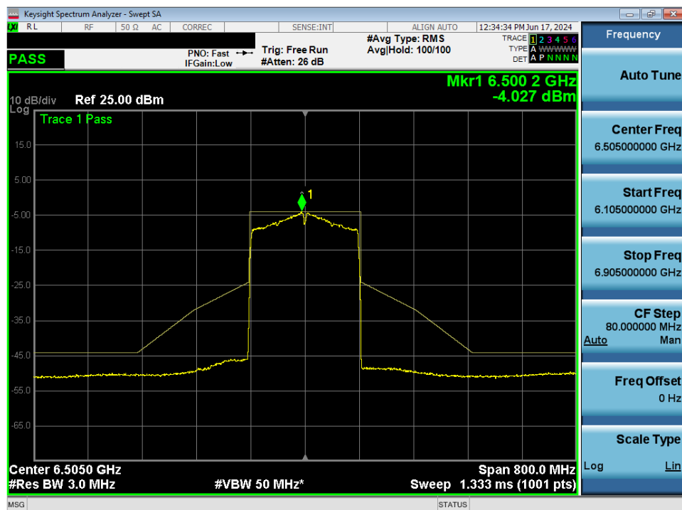
Plot 7-97. In-Band Emission MIMO ANT1 (160MHz 802.11ax (UNII Band 6) – Ch. 111)
