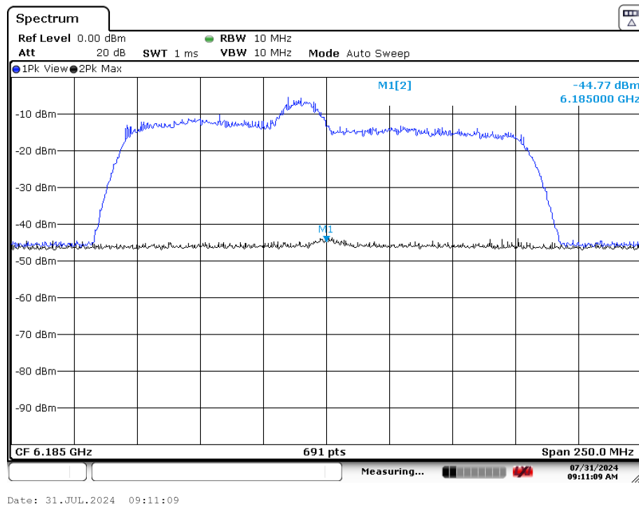
Plot 7-147. CBP 160MHz Channel - Injection Center – [6185 MHz]
