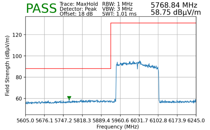
Plot 7-169. Radiated Lower Band Edge Plot SISO ANT1 (Peak – UNII Band 5)
