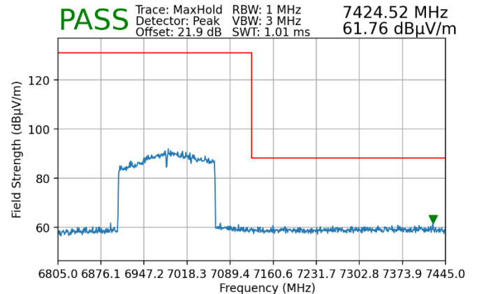
Plot 7-171. Radiated Upper Band Edge Plot SISO ANT1 (Peak – UNII Band 8)
