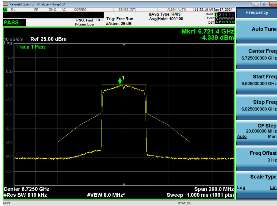
Plot 7-100. In-Band Emission MIMO ANT1 (40MHz 802.11ax (UNII Band 7) – Ch. 155)
