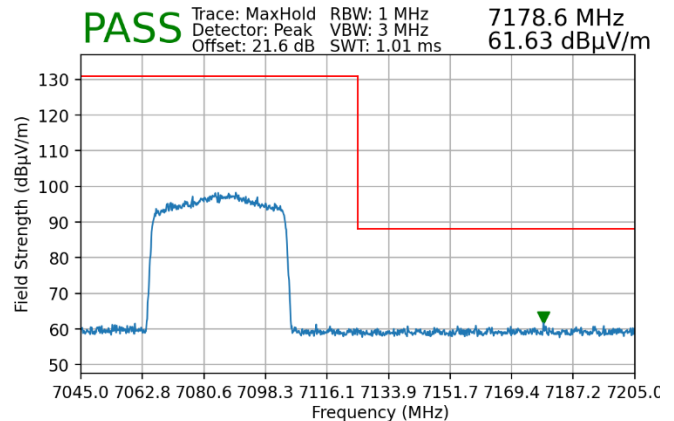
Plot 7-163. Radiated Upper Band Edge Plot SISO ANT1 (Peak – UNII Band 8)
