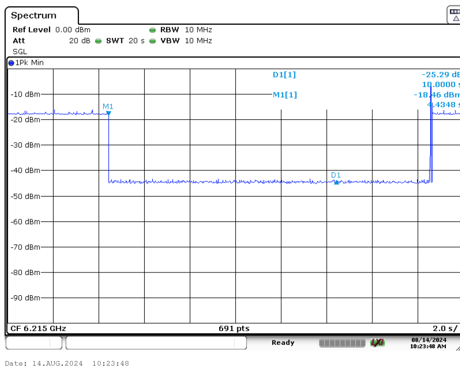
Plot 7-130. Contention Based Protocol Timing Plot (20MHz (UNII Band 5) – Ch. 53)
