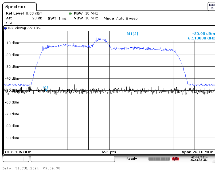
Plot 7-146. CBP 160MHz Channel - Injection Lower Edge – [6110 MHz]
