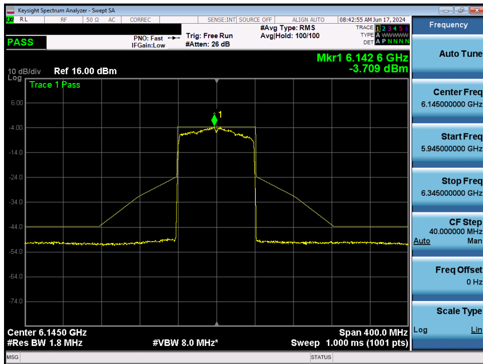
Plot 7-111. In-Band Emission MIMO ANT2 (80MHz 802.11ax (UNII Band 5) – Ch. 39)
