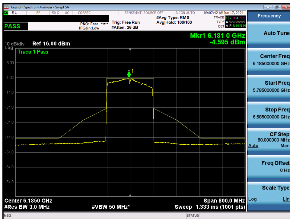
Plot 7-112. In-Band Emission MIMO ANT2 (160MHz 802.11ax (UNII Band 5) – Ch. 47)
