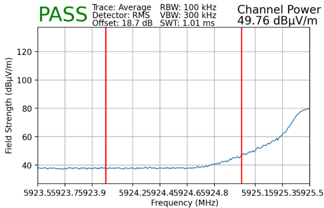
Plot 7-172. Radiated Lower Band Edge Plot SISO ANT2 (Average – UNII Band 5)
