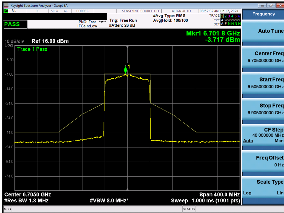
Plot 7-121. In-Band Emission MIMO ANT2 (80MHz 802.11ax (UNII Band 7) – Ch. 151)
