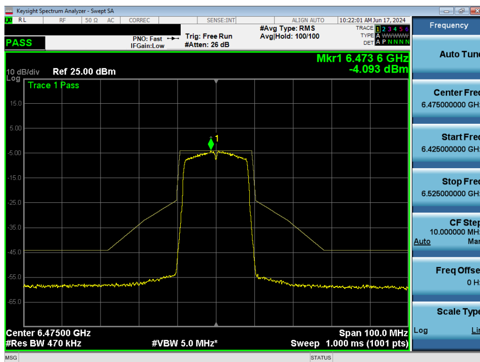
Plot 7-93. In-Band Emission MIMO ANT1 (20MHz 802.11a (UNII Band 6) – Ch. 105)
