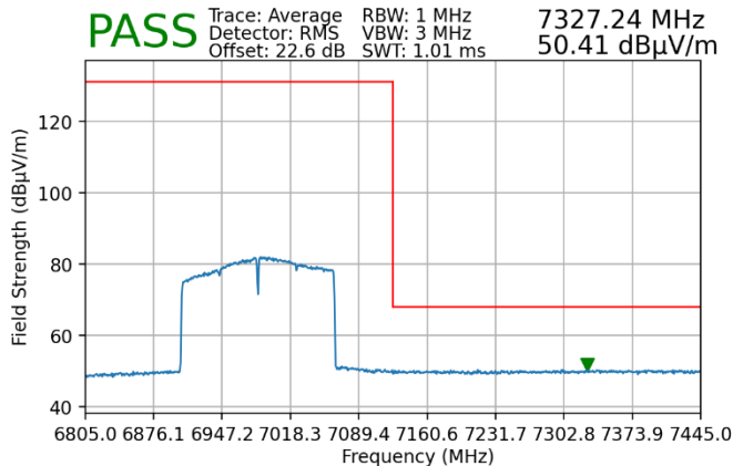
Plot 7-170. Radiated Upper Band Edge Plot SISO ANT1 (Average – UNII Band 8)
