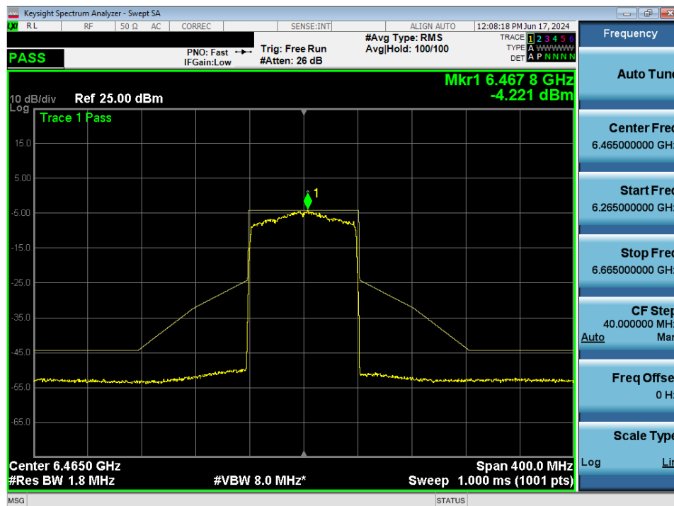
Plot 7-96. In-Band Emission MIMO ANT1 (80MHz 802.11ax (UNII Band 6) – Ch. 103)
