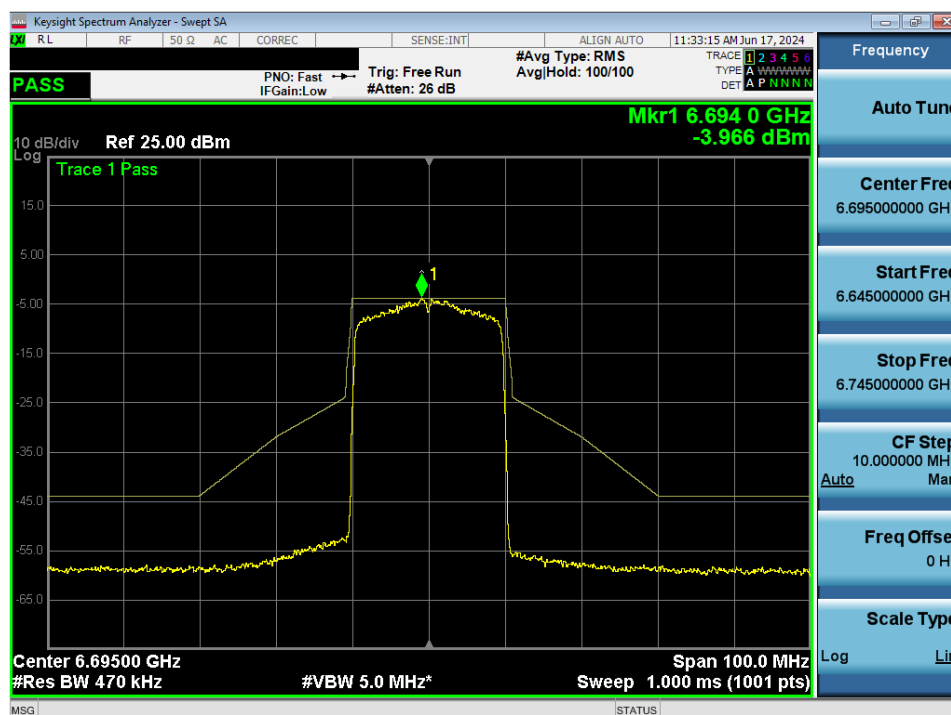
Plot 7-99. In-Band Emission MIMO ANT1 (20MHz 802.11ax (UNII Band 7) – Ch. 149)
