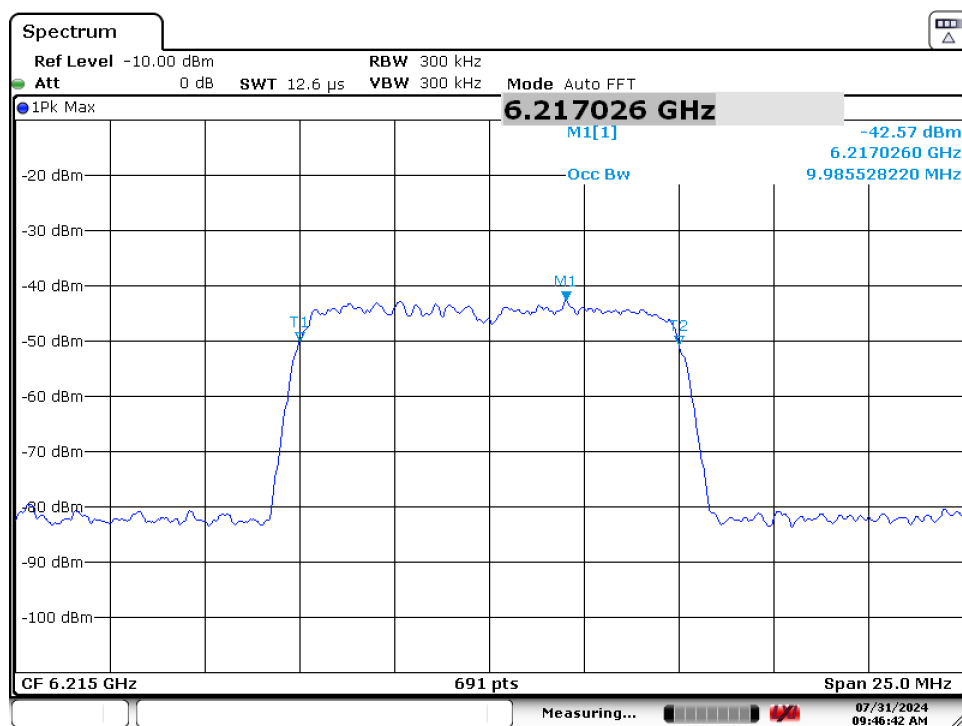
Plot 7-128. AWGN Signal (Demonstration)
