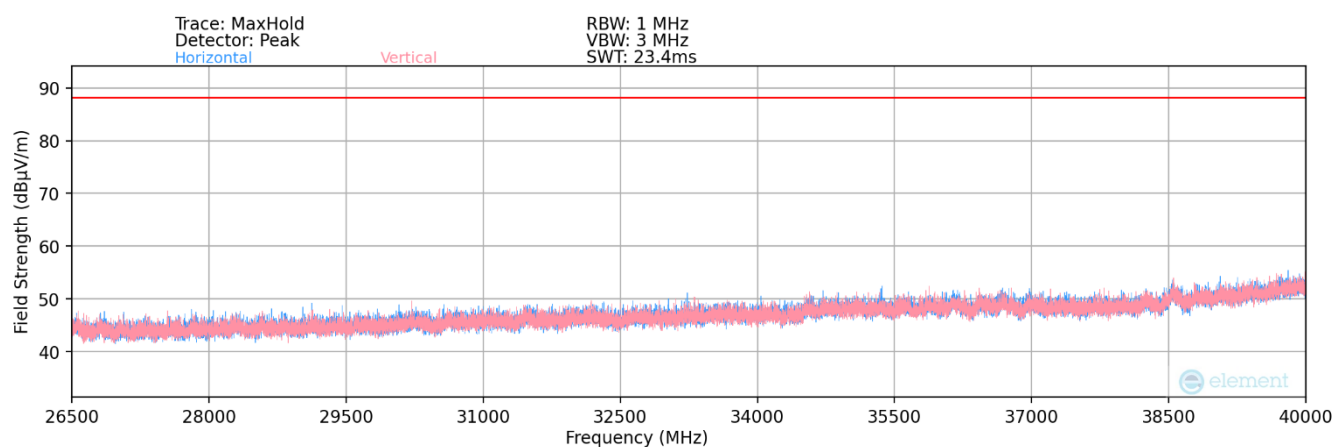
Plot 7-155. Radiated Spurious Plot 26.5GHz - 40GHz (802.11a)
