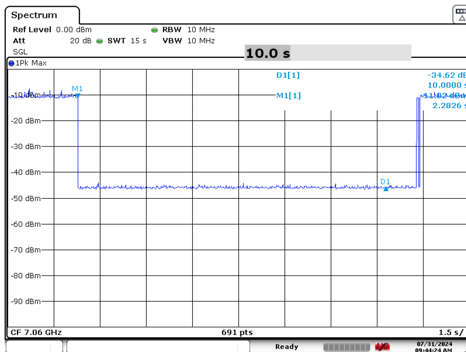
Plot 7-144. Contention Based Protocol Timing Plot (160MHz (UNII Band 8) – Ch. 207 Mid)
