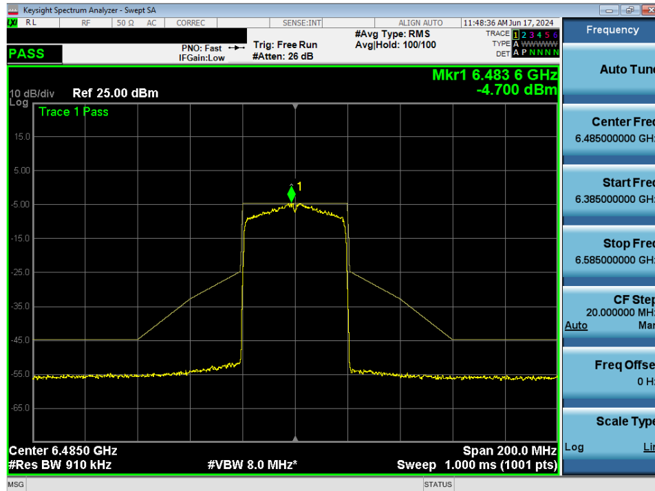
Plot 7-95. In-Band Emission MIMO ANT1 (40MHz 802.11ax (UNII Band 6) – Ch. 107)
