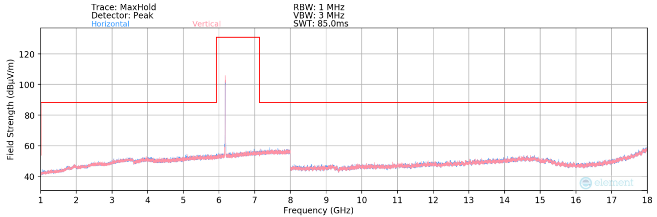
Plot 7-150. Radiated Spurious Plot 1GHz – 18GHz MIMO (802.11a – UNII Band 5 Ch. 45 – LPI/SP)
