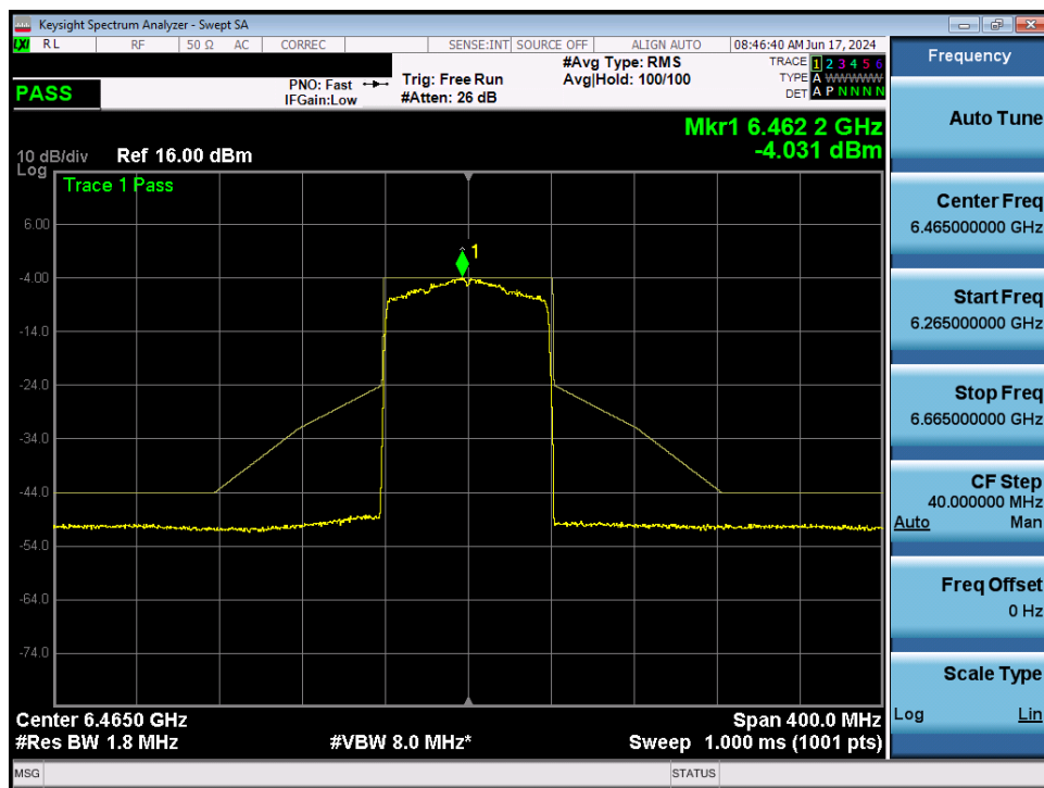
Plot 7-116. In-Band Emission MIMO ANT2 (80MHz 802.11ax (UNII Band 6) – Ch. 103)
