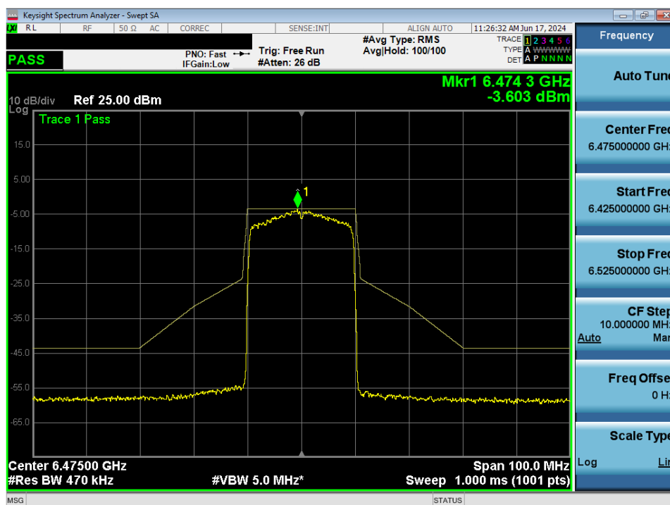
Plot 7-94. In-Band Emission MIMO ANT1 (20MHz 802.11ax (UNII Band 6) – Ch. 105)
