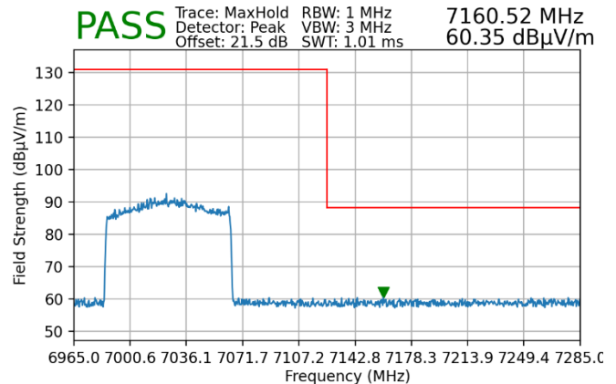
Plot 7-167. Radiated Upper Band Edge Plot SISO ANT1 (Peak – UNII Band 8)
