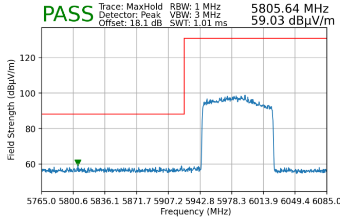
Plot 7-165. Radiated Lower Band Edge Plot SISO ANT1 (Peak – UNII Band 5)
