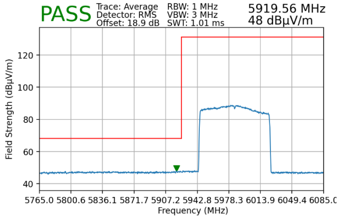
Plot 7-164. Radiated Lower Band Edge Plot SISO ANT1 (Average – UNII Band 5)
