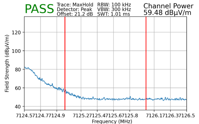
Plot 7-159. Radiated Upper Band Edge Plot SISO ANT1 (Peak – UNII Band 8)
