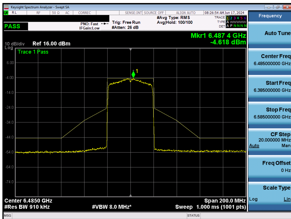
Plot 7-115. In-Band Emission MIMO ANT2 (40MHz 802.11ax (UNII Band 6) – Ch. 107)
