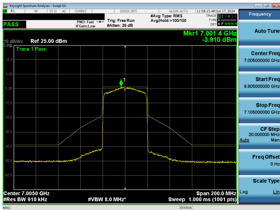
Plot 7-105. In-Band Emission MIMO ANT1 (40MHz 802.11ax (UNII Band 8) – Ch. 211)
