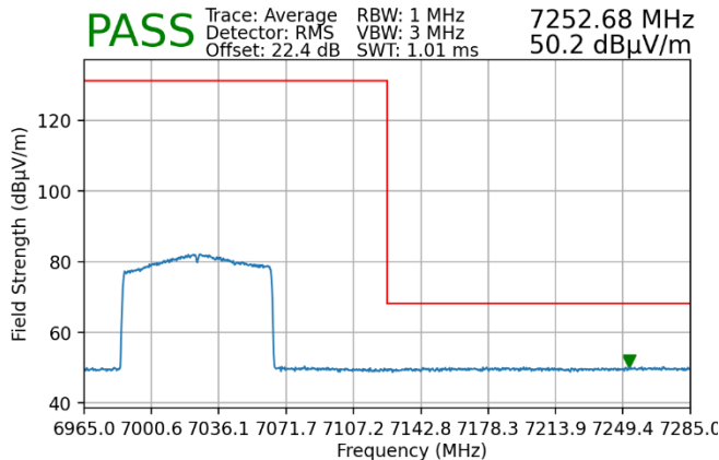
Plot 7-166. Radiated Upper Band Edge Plot SISO ANT1 (Average – UNII Band 8)
