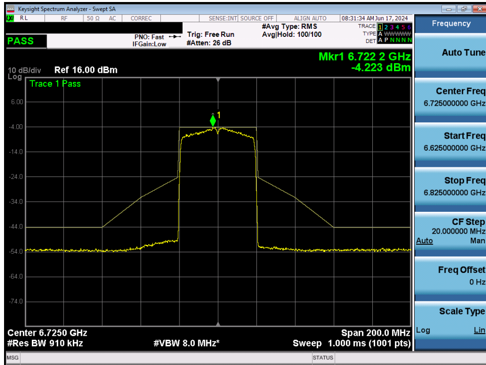
Plot 7-120. In-Band Emission MIMO ANT2 (40MHz 802.11ax (UNII Band 7) – Ch. 155)
