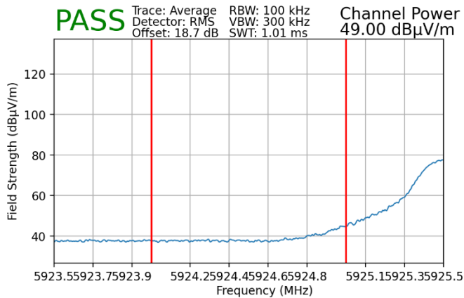
Plot 7-156. Radiated Lower Band Edge Plot SISO ANT1 (Average – UNII Band 5)
