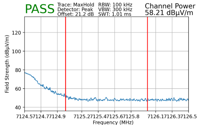
Plot 7-175. Radiated Upper Band Edge Plot SISO ANT2 (Peak – UNII Band 8)
