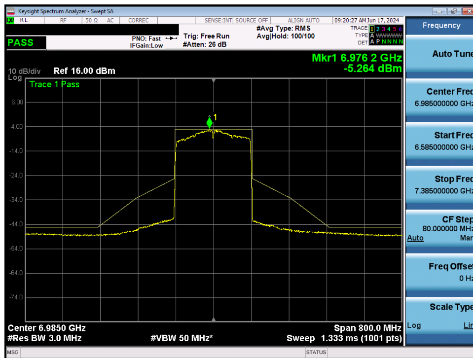
Plot 7-127. In-Band Emission MIMO ANT2 (160MHz 802.11ax (UNII Band 8) – Ch. 207)
