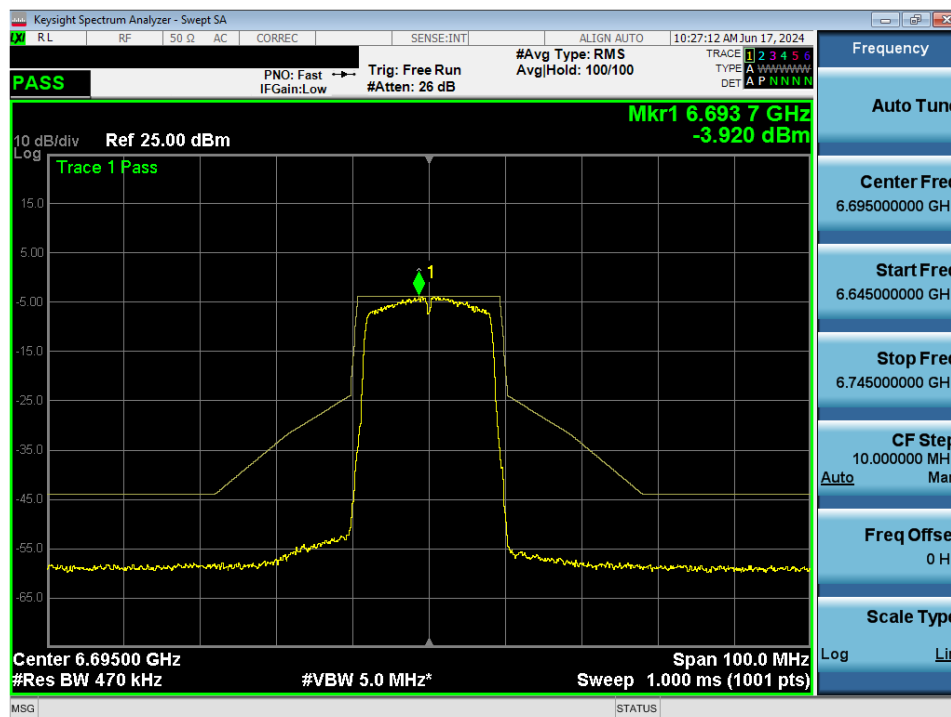
Plot 7-98. In-Band Emission MIMO ANT1 (20MHz 802.11a (UNII Band 7) – Ch. 149)
