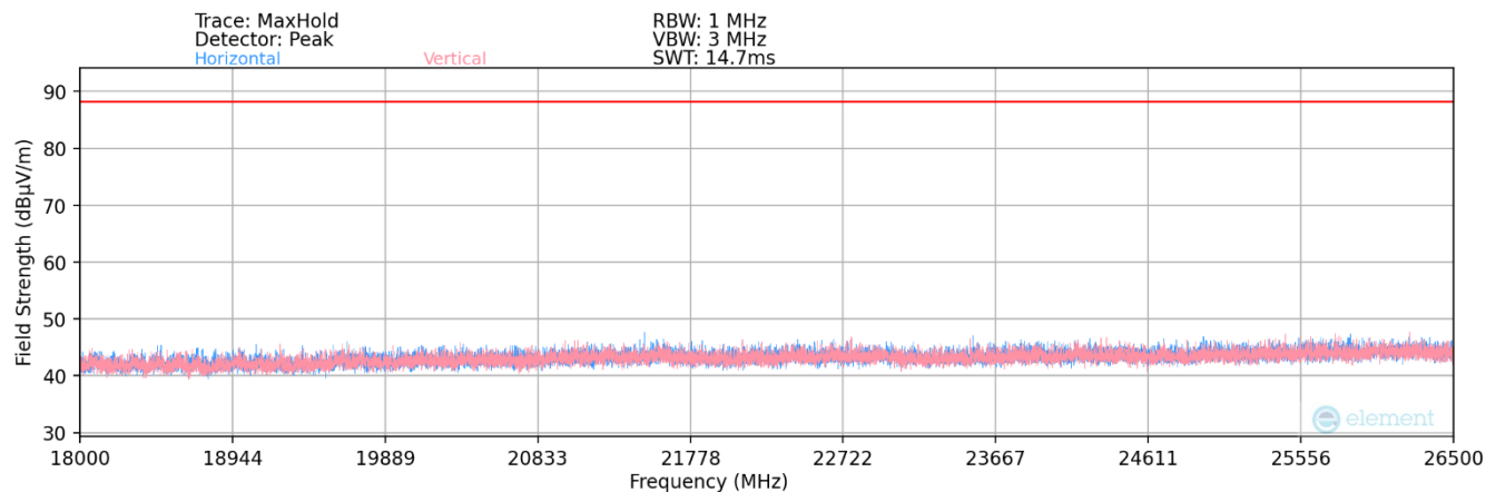
Plot 7-154. Radiated Spurious Plot 18GHz - 26.5GHz (802.11a)
