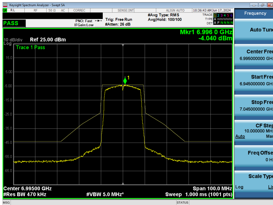
Plot 7-103. In-Band Emission MIMO ANT1 (20MHz 802.11a (UNII Band 8) – Ch. 209)
