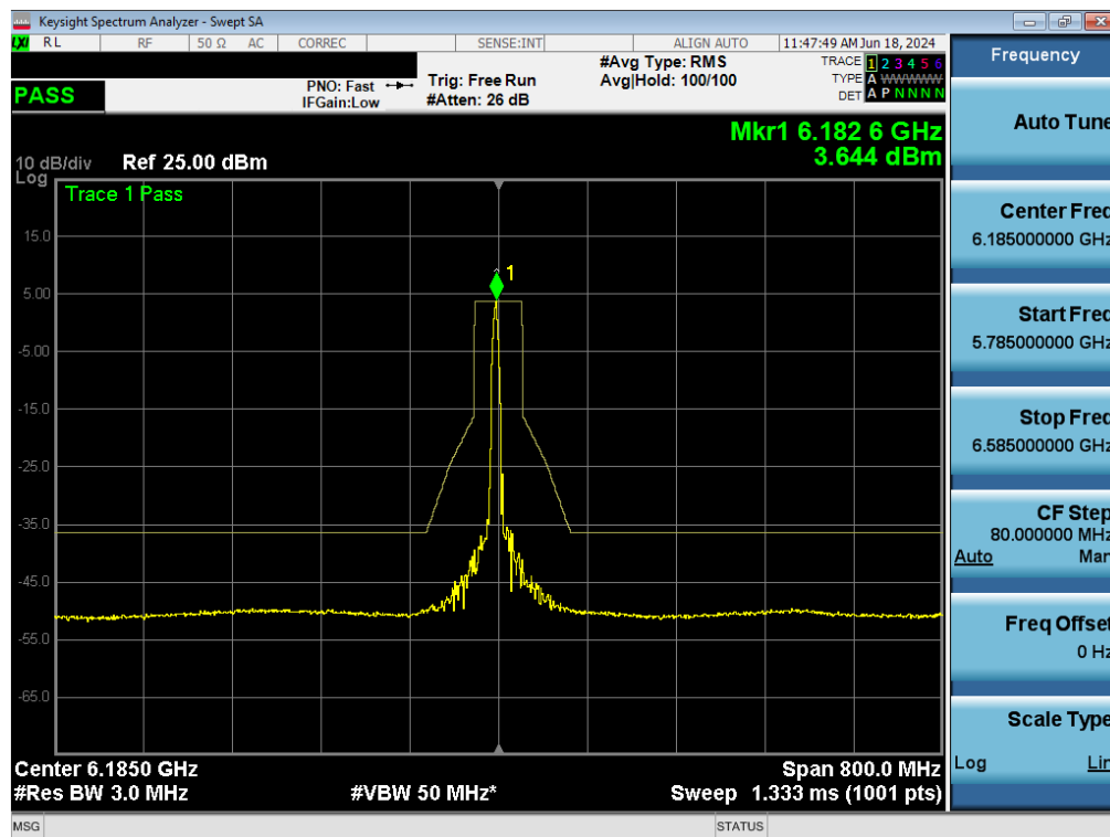
Plot 7-139. In-Band Emissions Plot MIMO ANT1 (160MHz BW 802.11ax (26 Tones) (UNII Band 5) – Ch. 47) - LPI/SP
