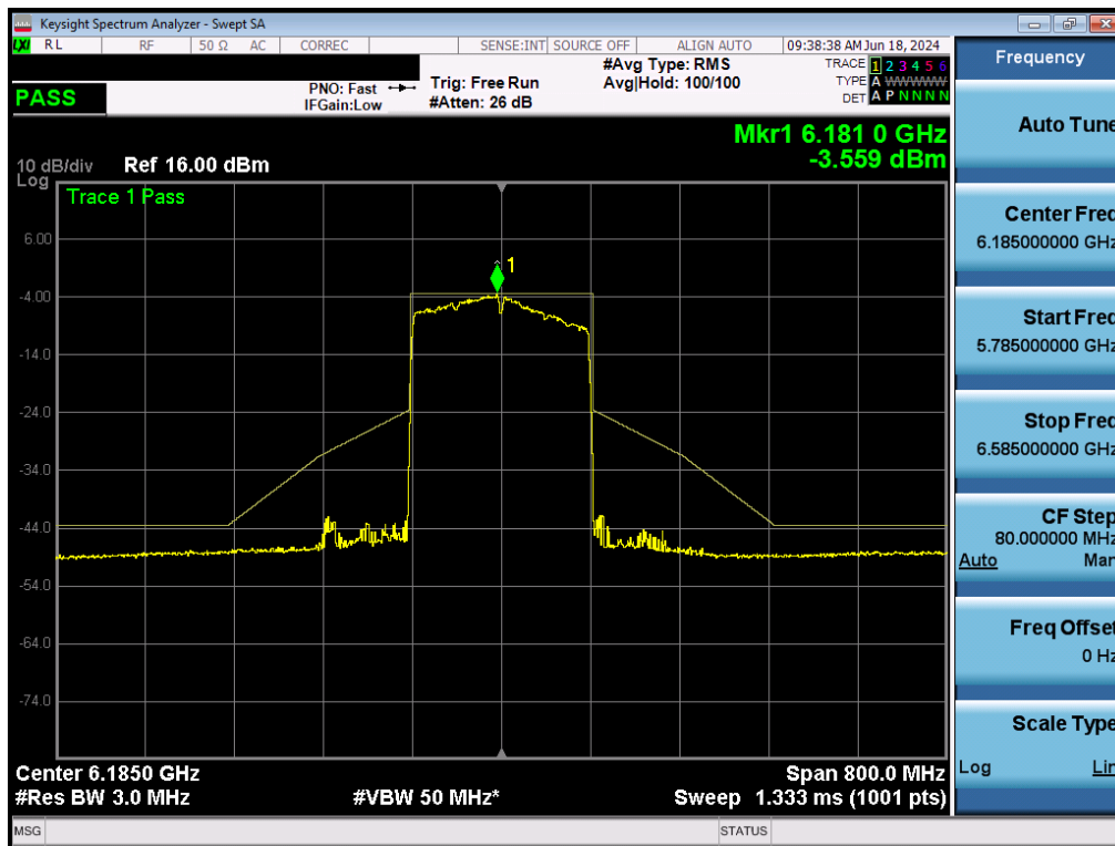
Plot 7-187. In-Band Emissions Plot MIMO ANT2 (160MHz BW 802.11ax (Full Tones) (UNII Band 5) – Ch. 47) - LPI/SP
