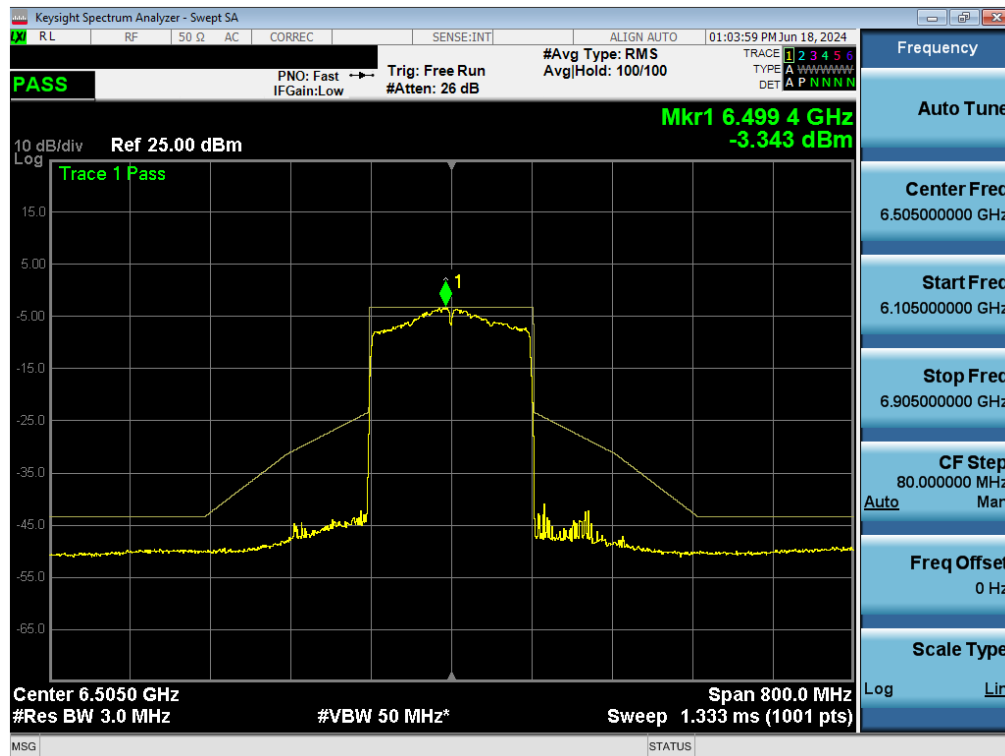
Plot 7-159. In-Band Emissions Plot MIMO ANT1 (160MHz BW 802.11ax (Full Tones) (UNII Band 6) – Ch. 111) - LPI/SP
