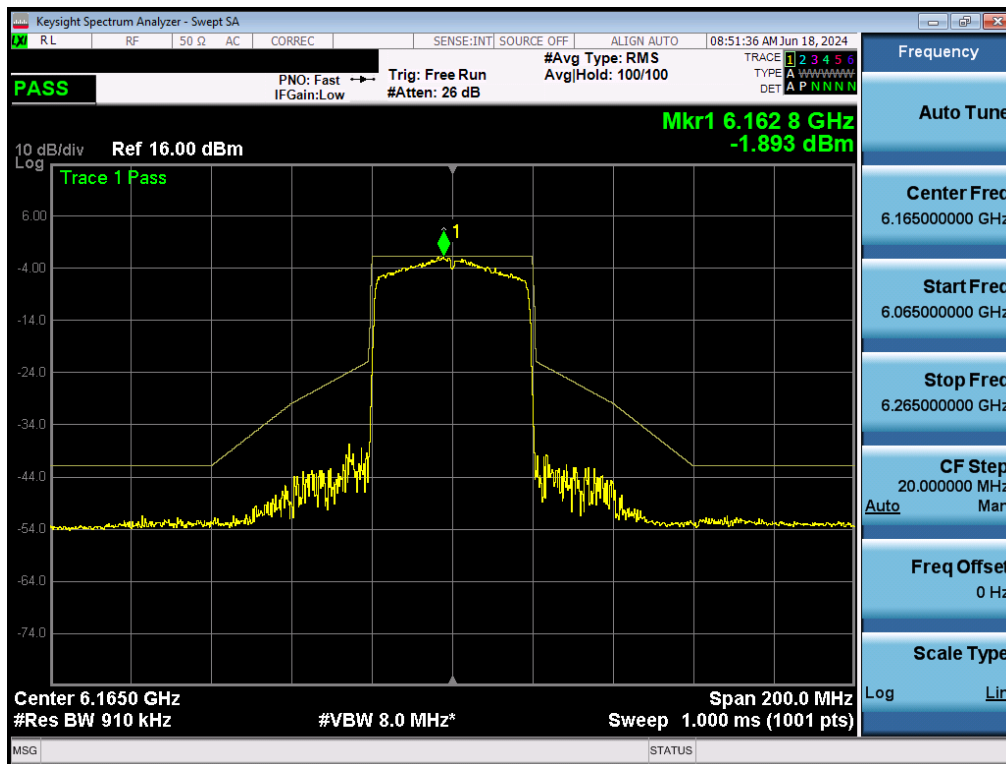
Plot 7-185. In-Band Emissions Plot MIMO ANT2 (40MHz BW 802.11ax (Full Tones) (UNII Band 5) – Ch. 43) - LPI/SP
