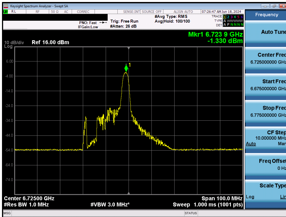
Plot 7-113. Power Spectral Density Plot MIMO ANT2 (40MHz BW 802.11ax (26 Tones) (UNII Band 7) – Ch. 155) - LPI/SP
