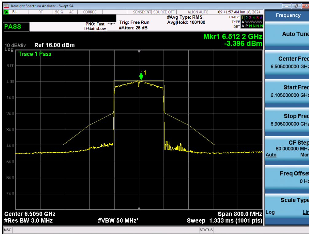
Plot 7-191. In-Band Emissions Plot MIMO ANT2 (160MHz BW 802.11ax (Full Tones) (UNII Band 6) – Ch. 111) - LPI/SP
