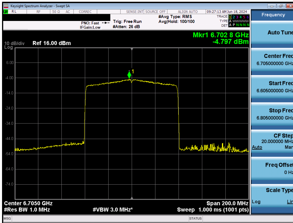
Plot 7-130. Power Spectral Density Plot MIMO ANT2 (80MHz BW 802.11ax (Full Tones) (UNII Band 7) – Ch. 151) - LPI/SP
