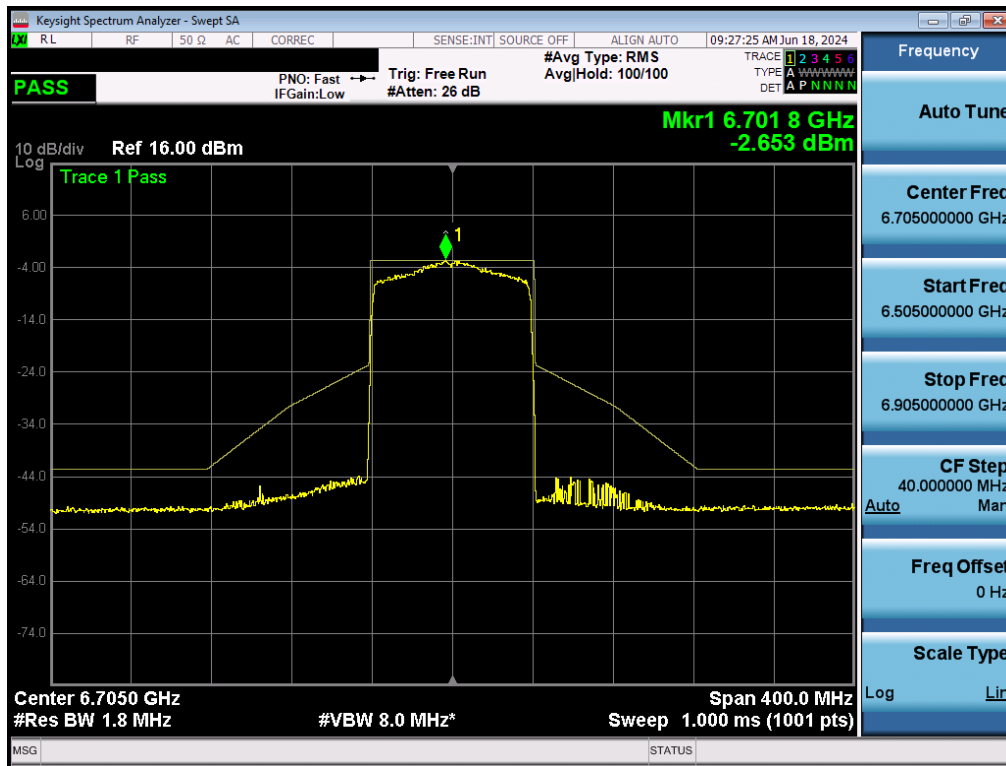
Plot 7-194. In-Band Emissions Plot MIMO ANT2 (80MHz BW 802.11ax (Full Tones) (UNII Band 7) – Ch. 151) - LPI/SP
