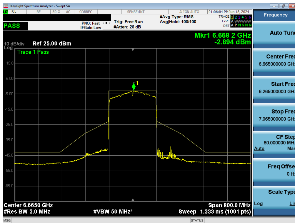
Plot 7-163. In-Band Emissions Plot MIMO ANT1 (160MHz BW 802.11ax (Full Tones) (UNII Band 7) – Ch. 143) - LPI/SP
