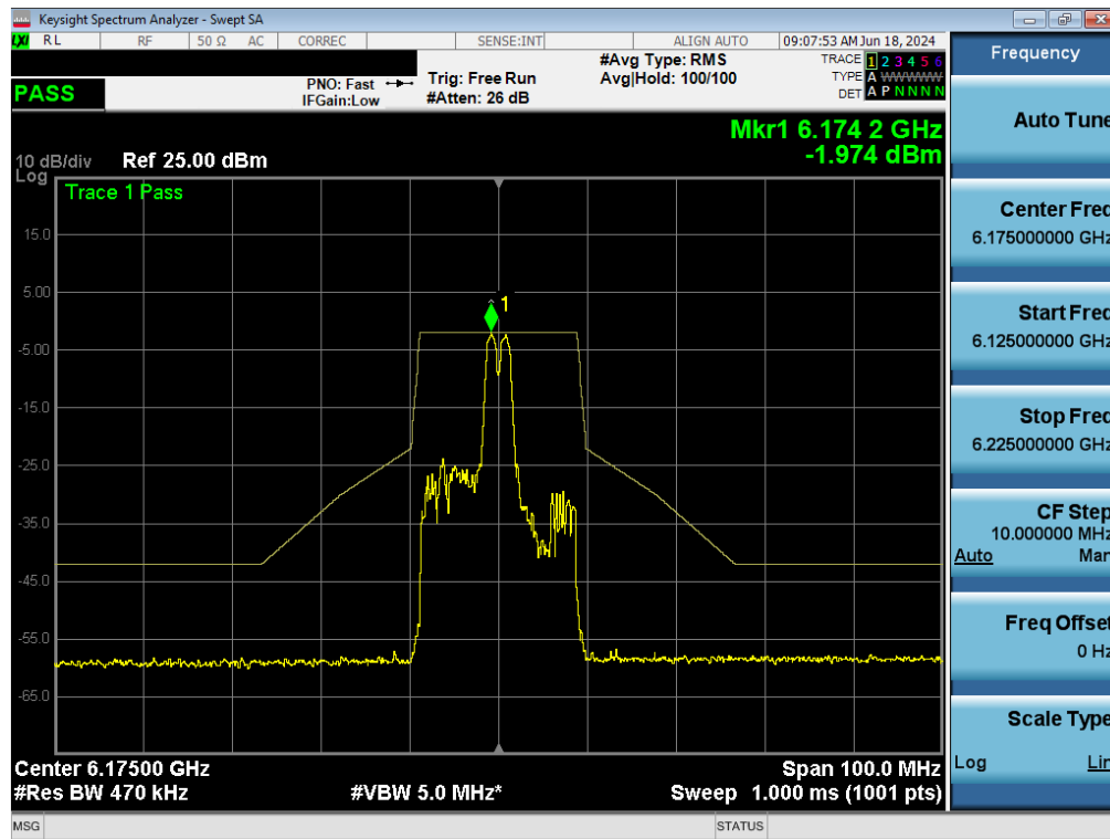
Plot 7-136. In-Band Emissions Plot MIMO ANT1 (20MHz BW 802.11ax (26 Tones) (UNII Band 5) – Ch. 45) – LPI/SP
