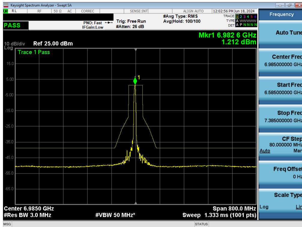
Plot 7-151. In-Band Emissions Plot MIMO ANT1 (160MHz BW 802.11ax (26 Tones) (UNII Band 8) – Ch. 207) - LPI/SP
