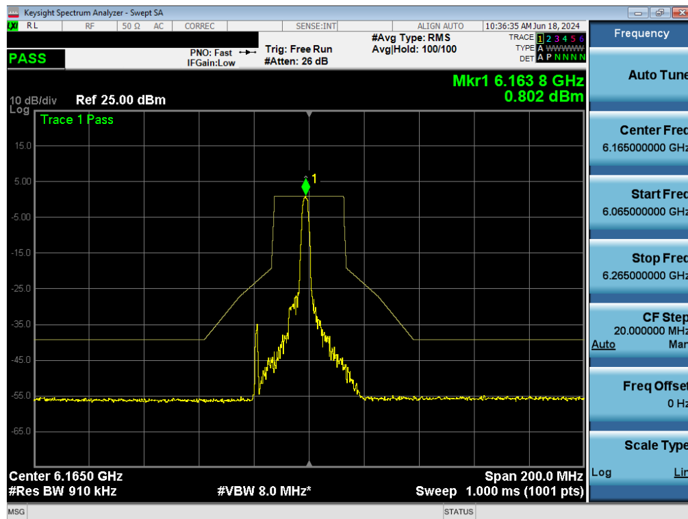
Plot 7-137. In-Band Emissions Plot MIMO ANT1 (40MHz BW 802.11ax (26 Tones) (UNII Band 5) – Ch. 43) – LPI/SP
