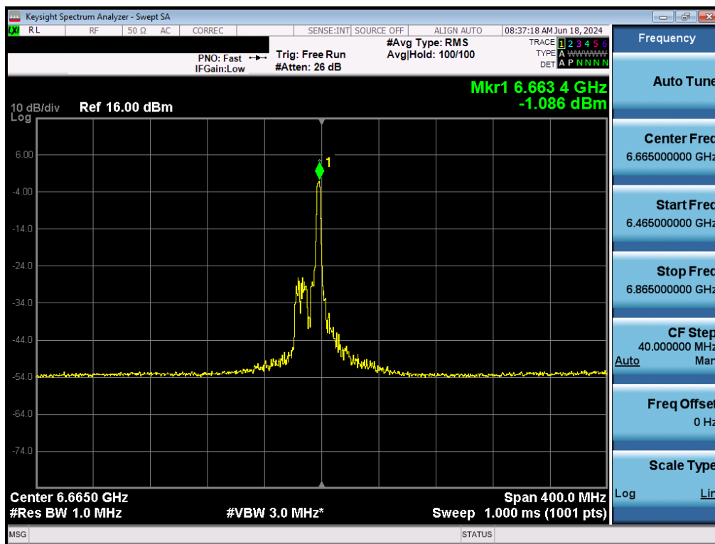
Plot 7-115. Power Spectral Density Plot MIMO ANT2 (160MHz BW 802.11ax (26 Tones) (UNII Band 7) – Ch. 143) - LPI/SP
