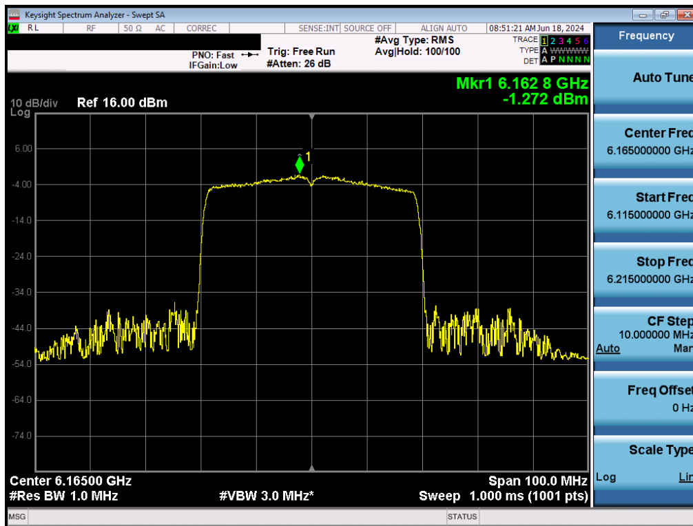
Plot 7-121. Power Spectral Density Plot MIMO ANT2 (40MHz BW 802.11ax (Full Tones) (UNII Band 5) – Ch. 43) - LPI/SP
