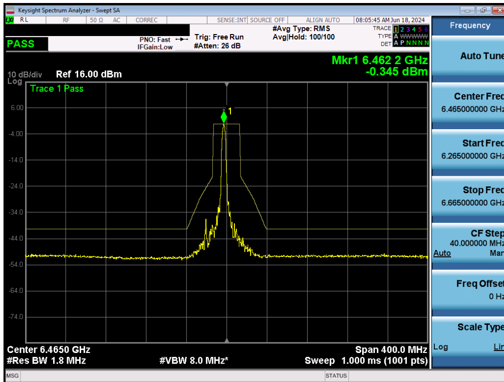
Plot 7-174. In-Band Emissions Plot MIMO ANT2 (80MHz BW 802.11ax (26 Tones) (UNII Band 6) – Ch. 103) - LPI/SP
