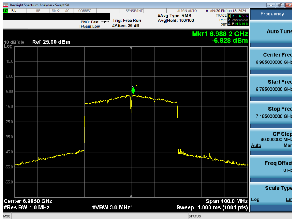
Plot 7-103. Power Spectral Density Plot MIMO ANT1 (160MHz BW 802.11ax (Full Tones) (UNII Band 8) – Ch. 207) - LPI/SP
