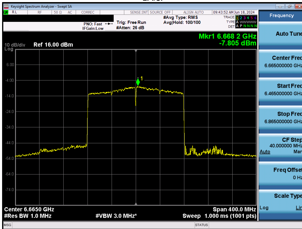
Plot 7-131. Power Spectral Density Plot MIMO ANT2 (160MHz BW 802.11ax (Full Tones) (UNII Band 7) – Ch. 143) - LPI/SP
