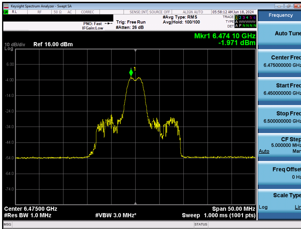
Plot 7-108. Power Spectral Density Plot MIMO ANT2 (20MHz BW 802.11ax (26 Tones) (UNII Band 6) – Ch. 105) - LPI/SP
