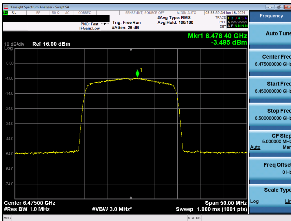
Plot 7-124. Power Spectral Density Plot MIMO ANT2 (20MHz BW 802.11ax (Full Tones) (UNII Band 6) – Ch. 105) - LPI/SP
