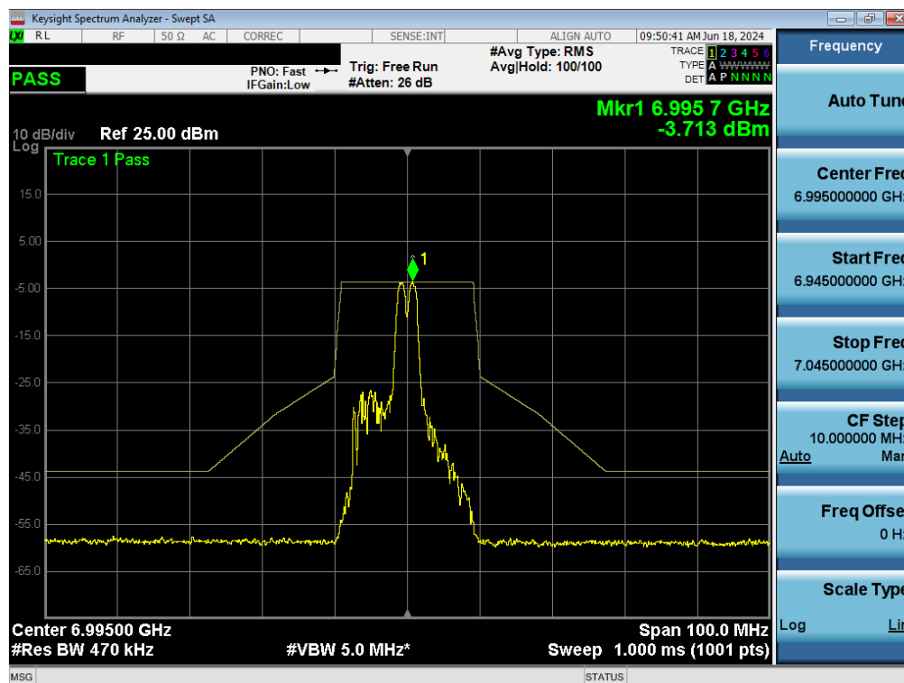
Plot 7-148. In-Band Emissions Plot MIMO ANT1 (20MHz BW 802.11ax (26 Tones) (UNII Band 8) – Ch. 209) - LPI/SP
