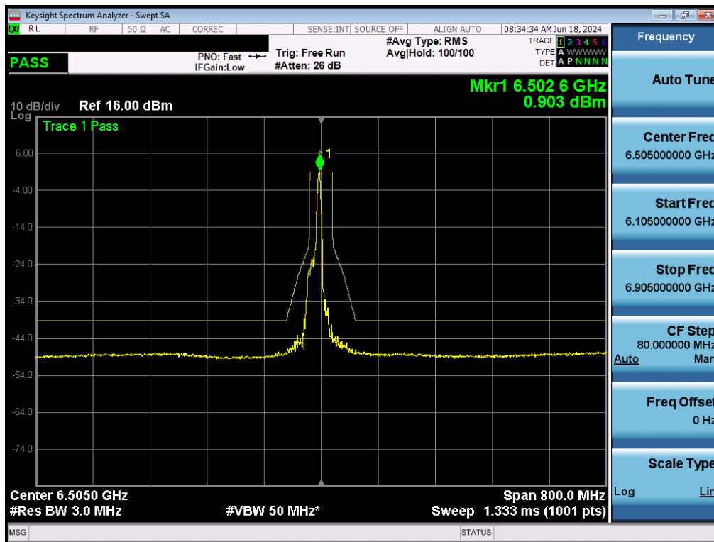
Plot 7-175. In-Band Emissions Plot MIMO ANT2 (160MHz BW 802.11ax (26 Tones) (UNII Band 6) – Ch. 111) - LPI/SP
