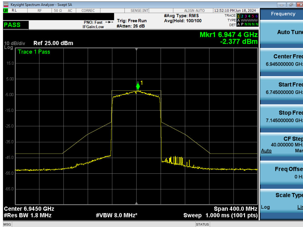
Plot 7-166. In-Band Emissions Plot MIMO ANT1 (80MHz BW 802.11ax (Full Tones) (UNII Band 8) – Ch. 199) - LPI/SP
