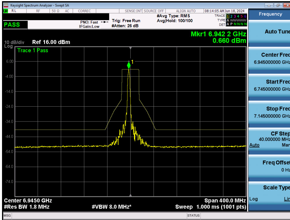
Plot 7-182. In-Band Emissions Plot MIMO ANT2 (80MHz BW 802.11ax (26 Tones) (UNII Band 8) – Ch. 199) - LPI/SP
