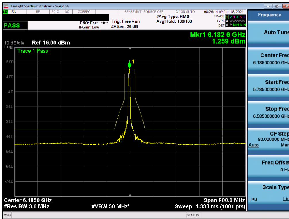
Plot 7-171. In-Band Emissions Plot MIMO ANT2 (160MHz BW 802.11ax (26 Tones) (UNII Band 5) – Ch. 47) - LPI/SP
