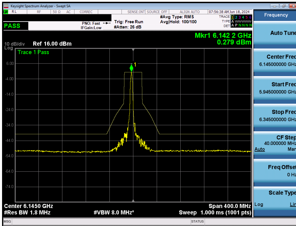
Plot 7-170. In-Band Emissions Plot MIMO ANT2 (80MHz BW 802.11ax (26 Tones) (UNII Band 5) – Ch. 39) - LPI/SP
