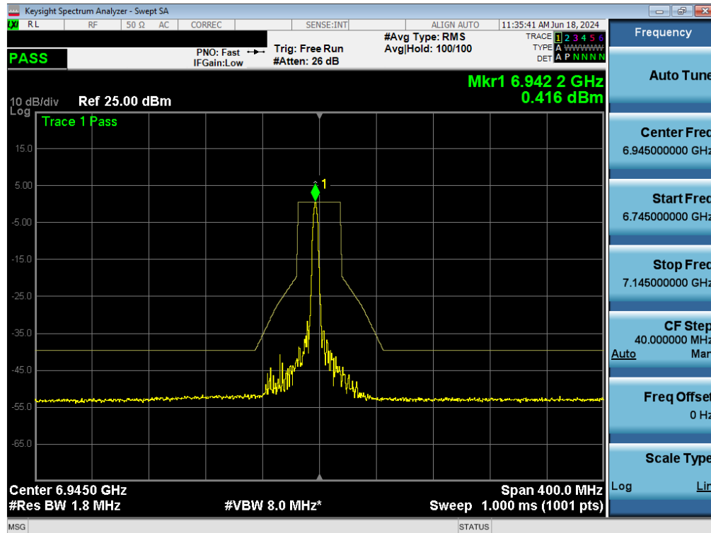
Plot 7-150. In-Band Emissions Plot MIMO ANT1 (80MHz BW 802.11ax (26 Tones) (UNII Band 8) – Ch. 199) - LPI/SP
