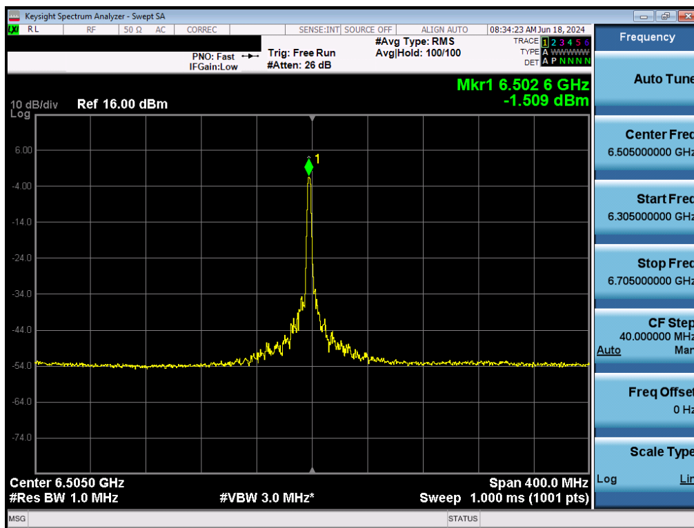
Plot 7-111. Power Spectral Density Plot MIMO ANT2 (160MHz BW 802.11ax (26 Tones) (UNII Band 6) – Ch. 111) - LPI/SP
