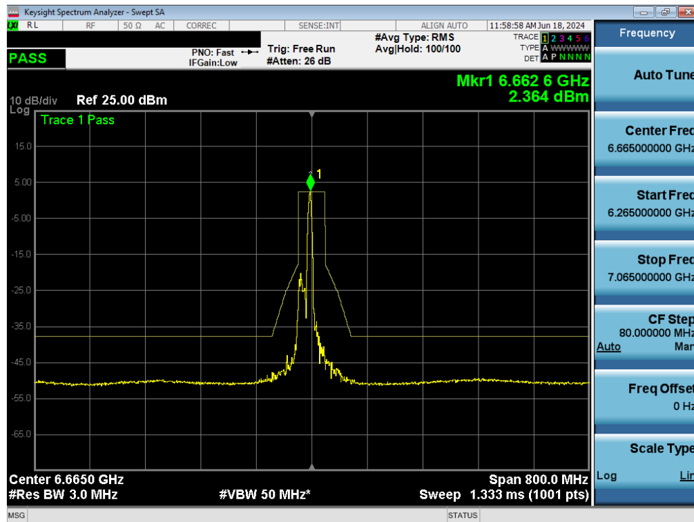
Plot 7-147. In-Band Emissions Plot MIMO ANT1 (160MHz BW 802.11ax (26 Tones) (UNII Band 7) – Ch. 143) - LPI/SP
