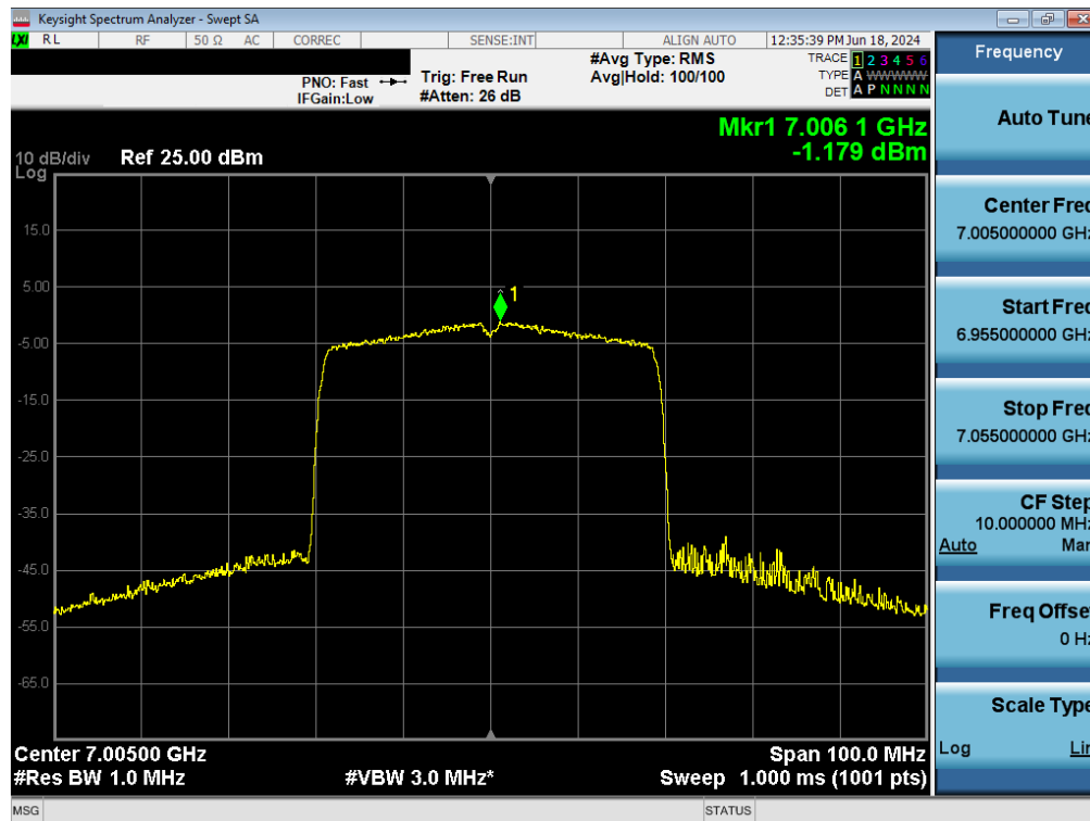
Plot 7-101. Power Spectral Density Plot MIMO ANT1 (40MHz BW 802.11ax (Full Tones) (UNII Band 8) – Ch. 211) – LPI/SP
