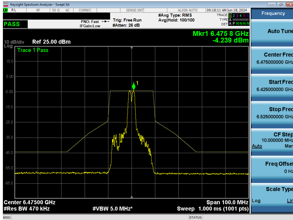
Plot 7-140. In-Band Emissions Plot MIMO ANT1 (20MHz BW 802.11ax (26 Tones) (UNII Band 6) – Ch. 105) - LPI/SP
