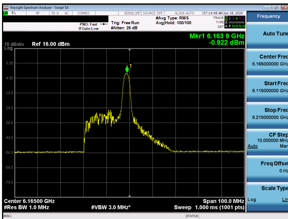
Plot 7-105. Power Spectral Density Plot MIMO ANT2 (40MHz BW 802.11ax (26 Tones) (UNII Band 5) – Ch. 43) - LPI/SP
