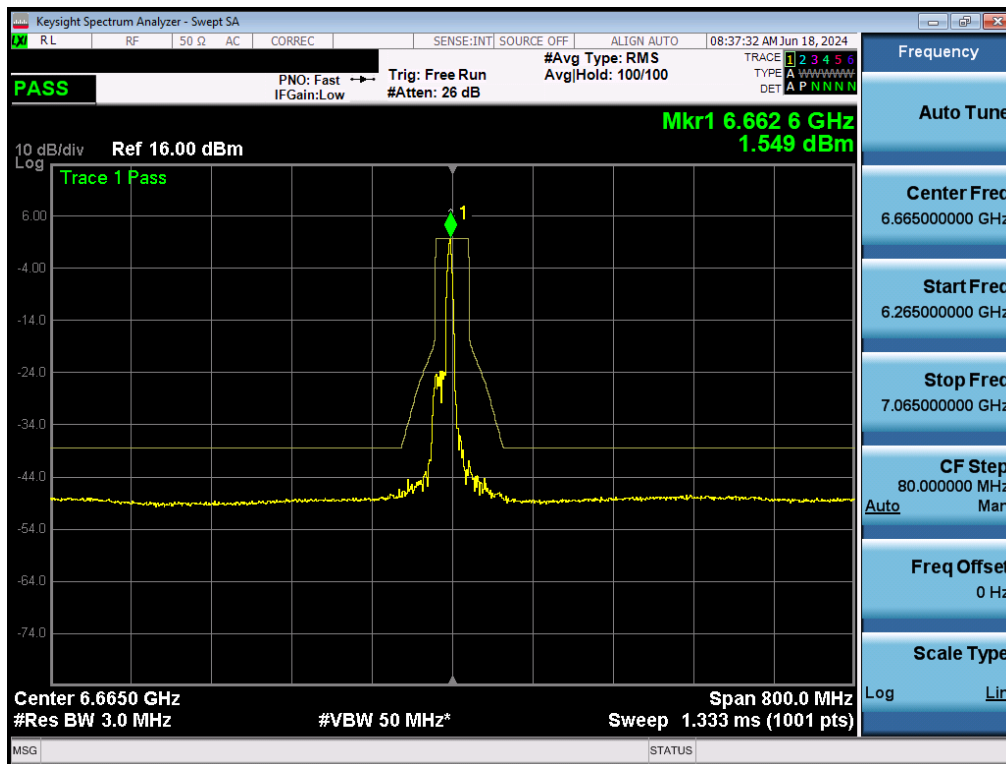
Plot 7-179. In-Band Emissions Plot MIMO ANT2 (160MHz BW 802.11ax (26 Tones) (UNII Band 7) – Ch. 143) - LPI/SP
