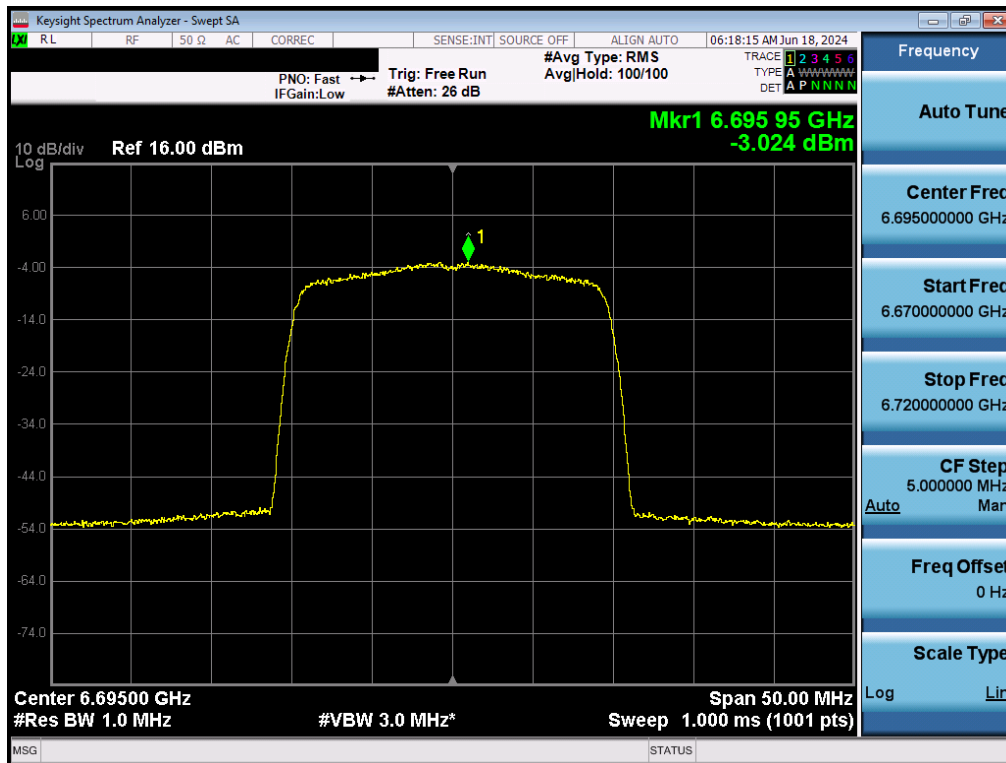
Plot 7-128. Power Spectral Density Plot MIMO ANT2 (20MHz BW 802.11ax (Full Tones) (UNII Band 7) – Ch. 149) - LPI/SP
