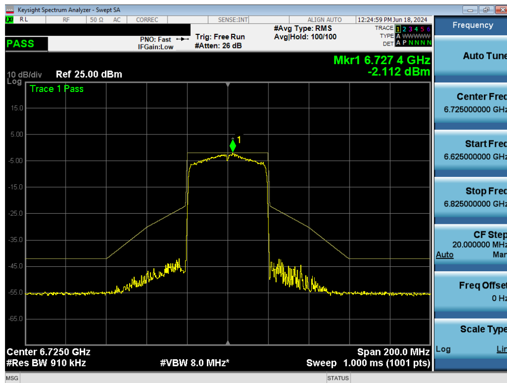
Plot 7-161. In-Band Emissions Plot MIMO ANT1 (40MHz BW 802.11ax (Full Tones) (UNII Band 7) – Ch. 155) - LPI/SP
