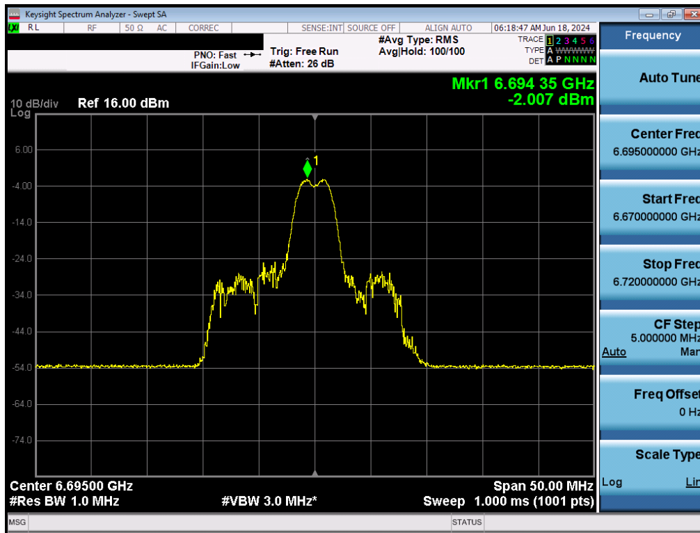
Plot 7-112. Power Spectral Density Plot MIMO ANT2 (20MHz BW 802.11ax (26 Tones) (UNII Band 7) – Ch. 149) - LPI/SP
