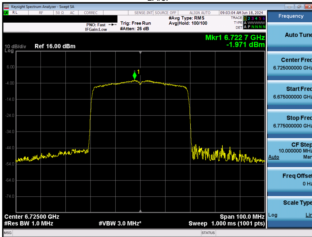
Plot 7-129. Power Spectral Density Plot MIMO ANT2 (40MHz BW 802.11ax (Full Tones) (UNII Band 7) – Ch. 155) - LPI/SP
