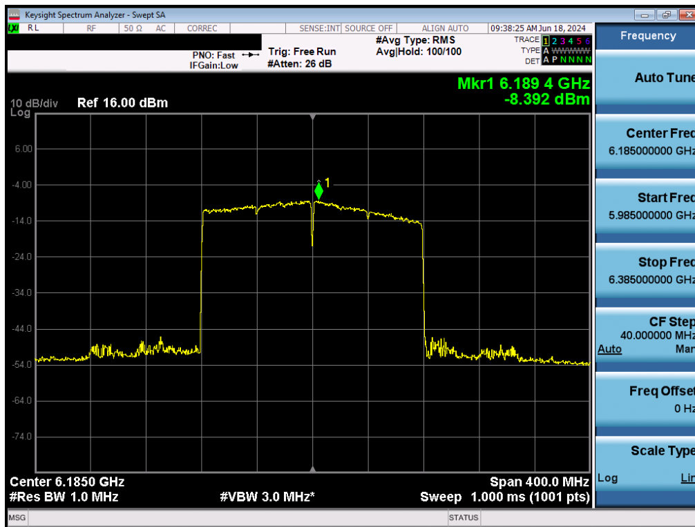
Plot 7-123. Power Spectral Density Plot MIMO ANT2 (160MHz BW 802.11ax (Full Tones) (UNII Band 5) – Ch. 47) - LPI/SP
