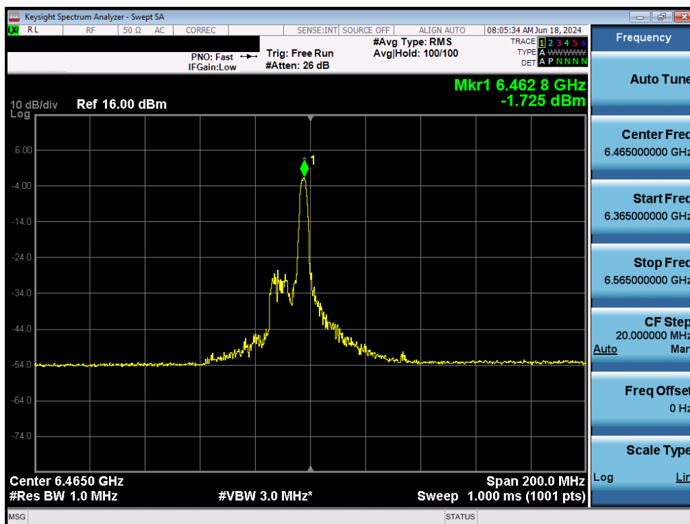
Plot 7-110. Power Spectral Density Plot MIMO ANT2 (80MHz BW 802.11ax (26 Tones) (UNII Band 6) – Ch. 103) - LPI/SP
