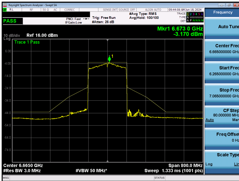
Plot 7-195. In-Band Emissions Plot MIMO ANT2 (160MHz BW 802.11ax (Full Tones) (UNII Band 7) – Ch. 143) - LPI/SP
