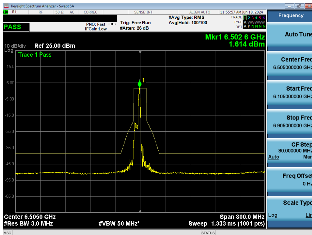
Plot 7-143. In-Band Emissions Plot MIMO ANT1 (160MHz BW 802.11ax (26 Tones) (UNII Band 6) – Ch. 111) - LPI/SP
