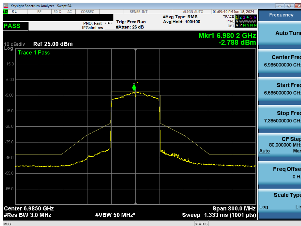
Plot 7-167. In-Band Emissions Plot MIMO ANT1 (160MHz BW 802.11ax (Full Tones) (UNII Band 8) – Ch. 207) - LPI/SP
