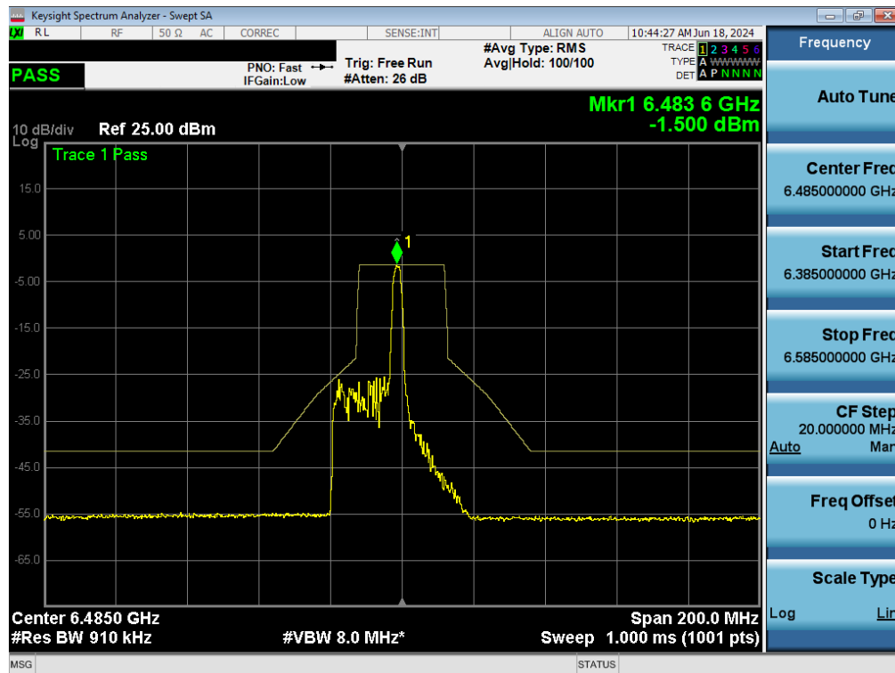
Plot 7-141. In-Band Emissions Plot MIMO ANT1 (40MHz BW 802.11ax (26 Tones) (UNII Band 6) – Ch. 107) - LPI/SP
