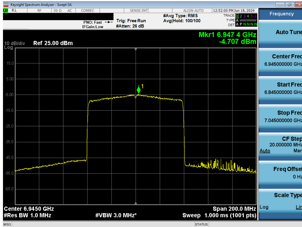
Plot 7-102. Power Spectral Density Plot MIMO ANT1 (80MHz BW 802.11ax (Full Tones) (UNII Band 8) – Ch. 199) - LPI/SP
