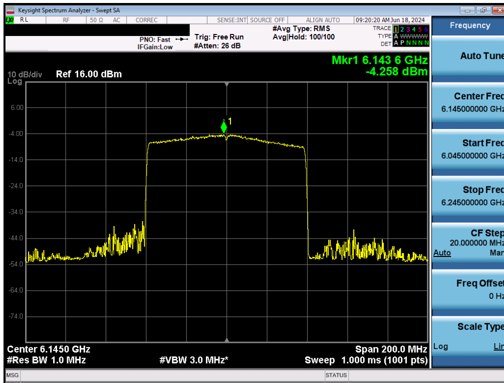
Plot 7-122. Power Spectral Density Plot MIMO ANT2 (80MHz BW 802.11ax (Full Tones) (UNII Band 5) – Ch. 39) - LPI/SP
