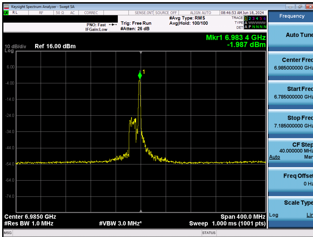
Plot 7-119. Power Spectral Density Plot MIMO ANT2 (160MHz BW 802.11ax (26 Tones) (UNII Band 8) – Ch. 207) - LPI/SP
