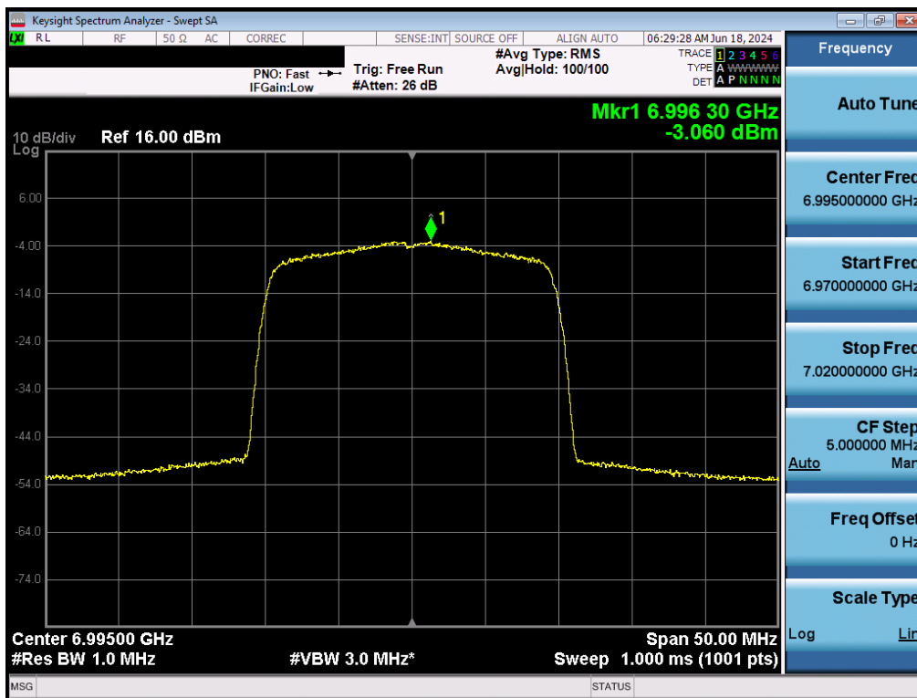
Plot 7-132. Power Spectral Density Plot MIMO ANT2 (20MHz BW 802.11ax (Full Tones) (UNII Band 8) – Ch. 209) - LPI/SP
