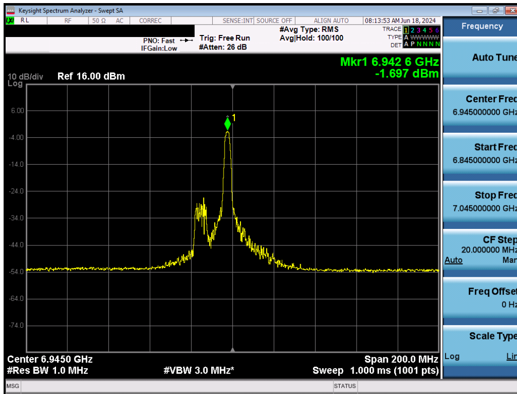
Plot 7-118. Power Spectral Density Plot MIMO ANT2 (80MHz BW 802.11ax (26 Tones) (UNII Band 8) – Ch. 199) - LPI/SP
