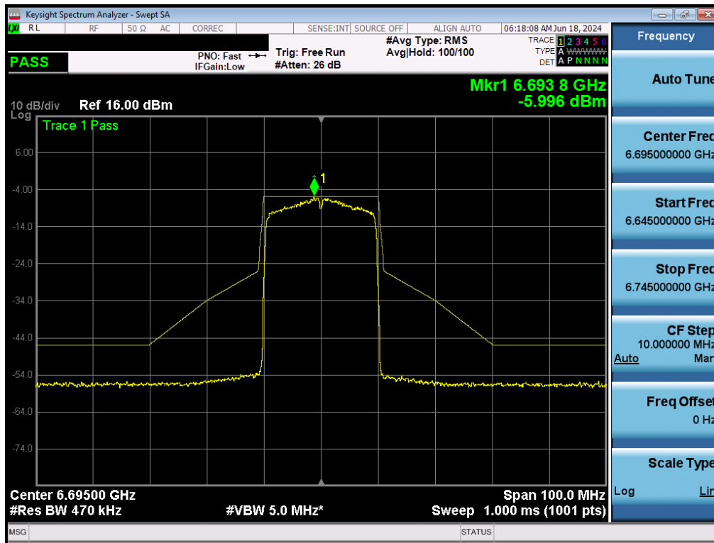
Plot 7-192. In-Band Emissions Plot MIMO ANT2 (20MHz BW 802.11ax (Full Tones) (UNII Band 7) – Ch. 149) - LPI/SP
