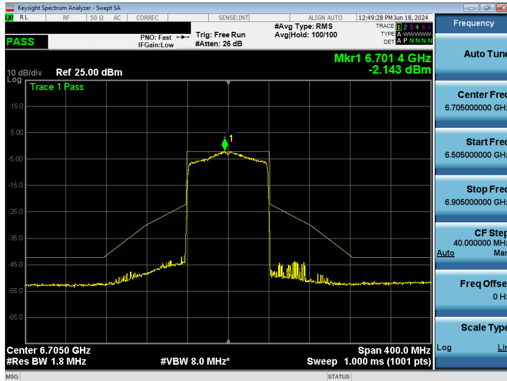
Plot 7-162. In-Band Emissions Plot MIMO ANT1 (80MHz BW 802.11ax (Full Tones) (UNII Band 7) – Ch. 151) – LPI/SP
