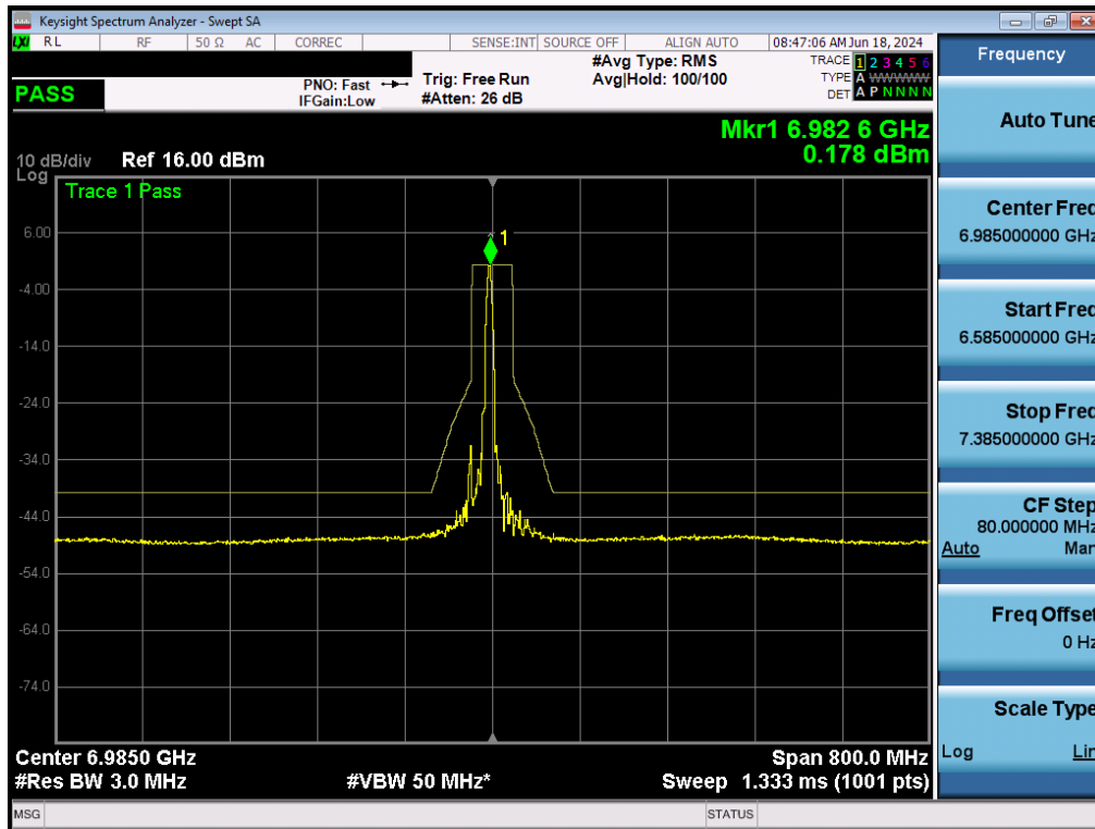
Plot 7-183. In-Band Emissions Plot MIMO ANT2 (160MHz BW 802.11ax (26 Tones) (UNII Band 8) – Ch. 207) - LPI/SP
