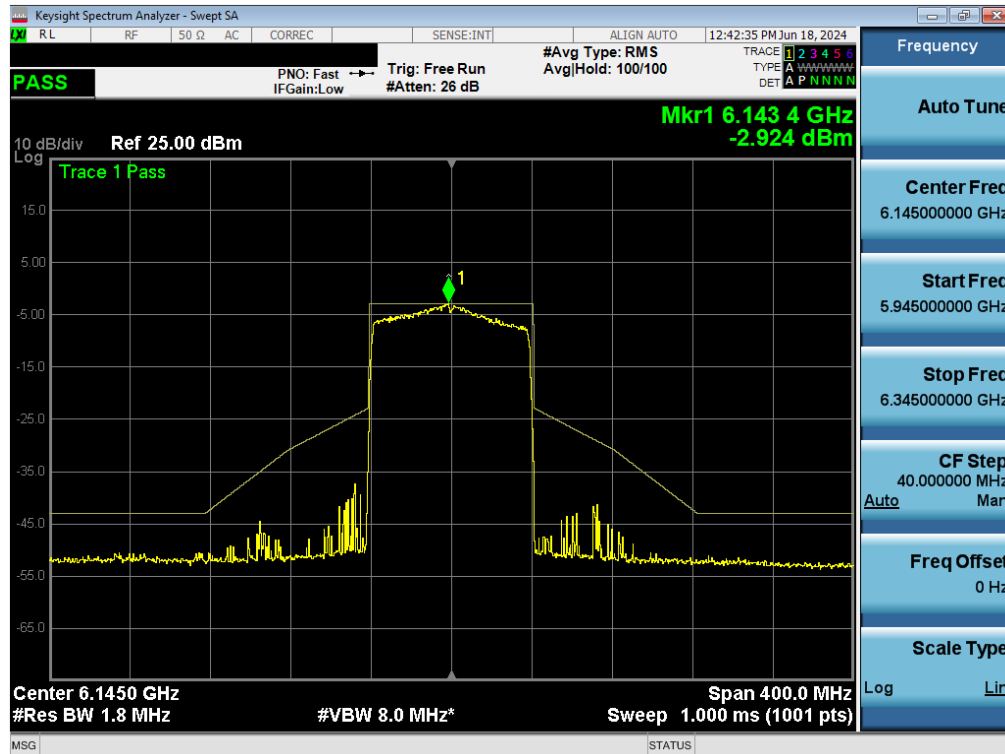
Plot 7-154. In-Band Emissions Plot MIMO ANT1 (80MHz BW 802.11ax (Full Tones) (UNII Band 5) – Ch. 39) - LPI/SP
