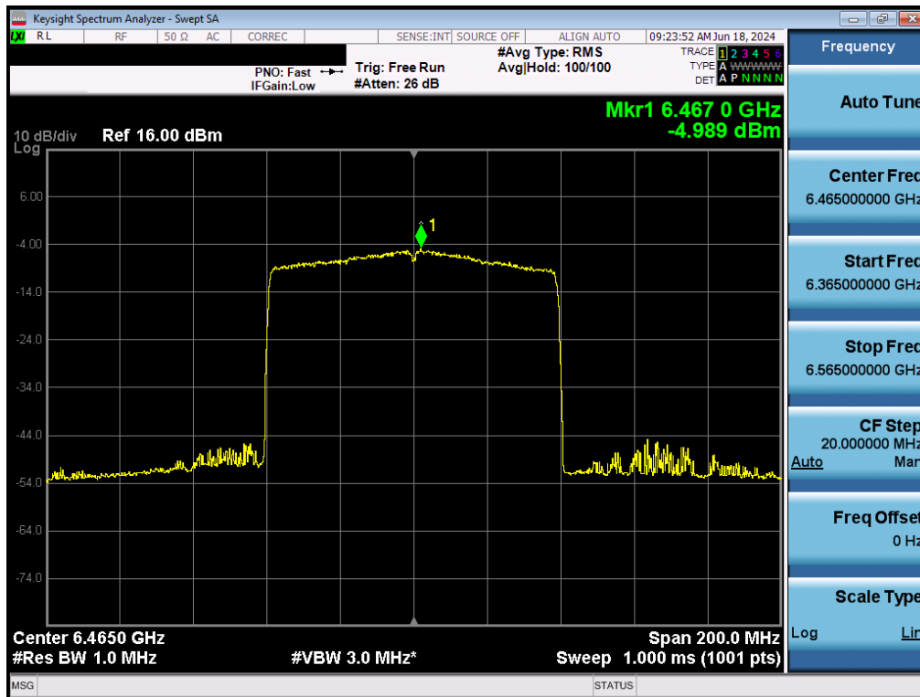
Plot 7-126. Power Spectral Density Plot MIMO ANT2 (80MHz BW 802.11ax (Full Tones) (UNII Band 6) – Ch. 103) - LPI/SP
