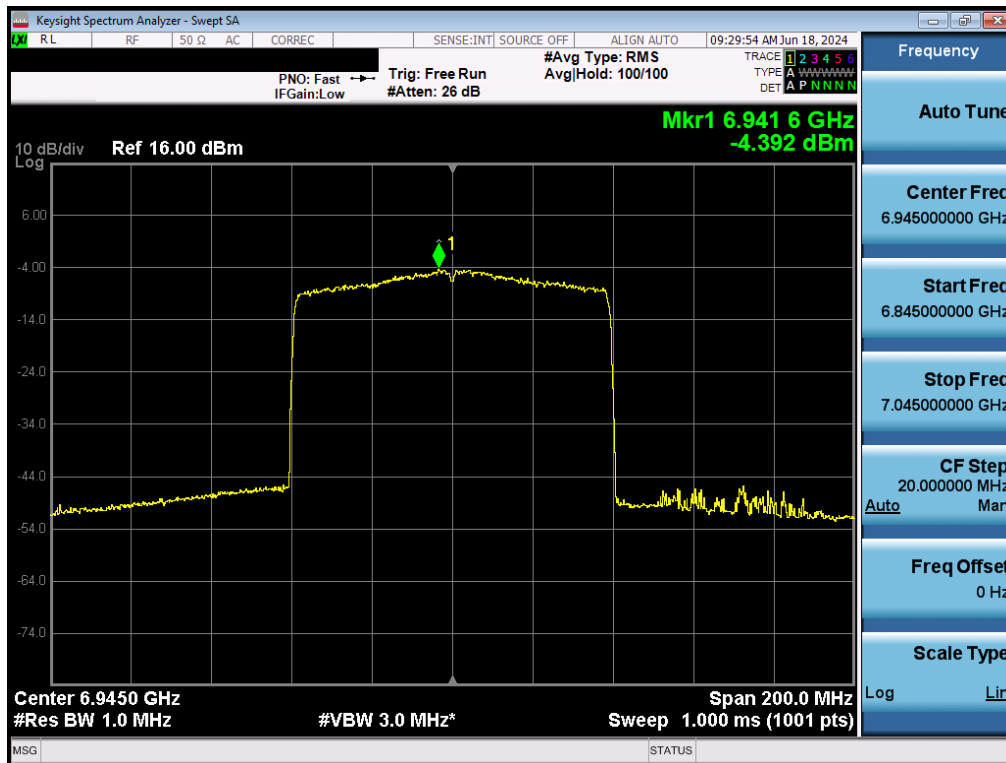
Plot 7-134. Power Spectral Density Plot MIMO ANT2 (80MHz BW 802.11ax (Full Tones) (UNII Band 8) – Ch. 199) - LPI/SP
