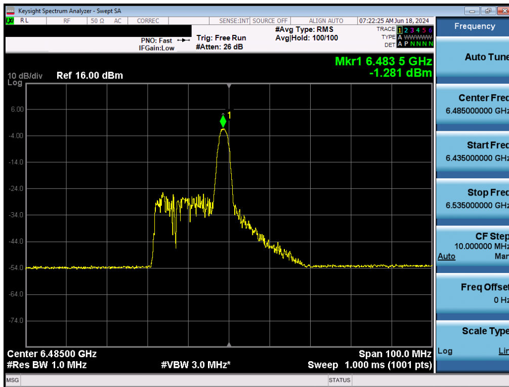
Plot 7-109. Power Spectral Density Plot MIMO ANT2 (40MHz BW 802.11ax (26 Tones) (UNII Band 6) – Ch. 107) - LPI/SP
