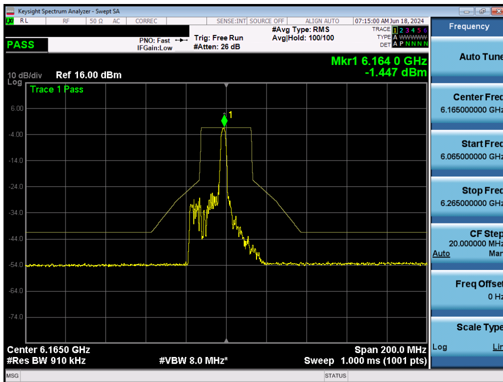
Plot 7-169. In-Band Emissions Plot MIMO ANT2 (40MHz BW 802.11ax (26 Tones) (UNII Band 5) – Ch. 43) - LPI/SP
