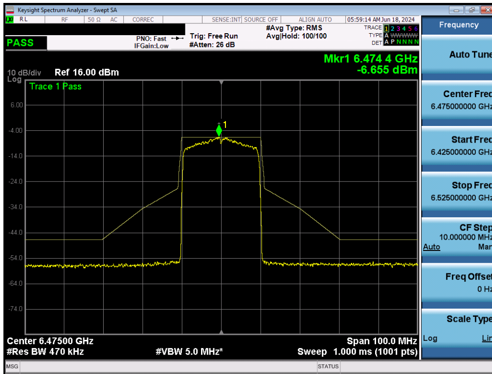
Plot 7-188. In-Band Emissions Plot MIMO ANT2 (20MHz BW 802.11ax (Full Tones) (UNII Band 6) – Ch. 105) - LPI/SP
