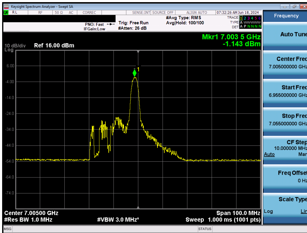
Plot 7-117. Power Spectral Density Plot MIMO ANT2 (40MHz BW 802.11ax (26 Tones) (UNII Band 8) – Ch. 211) - LPI/SP
