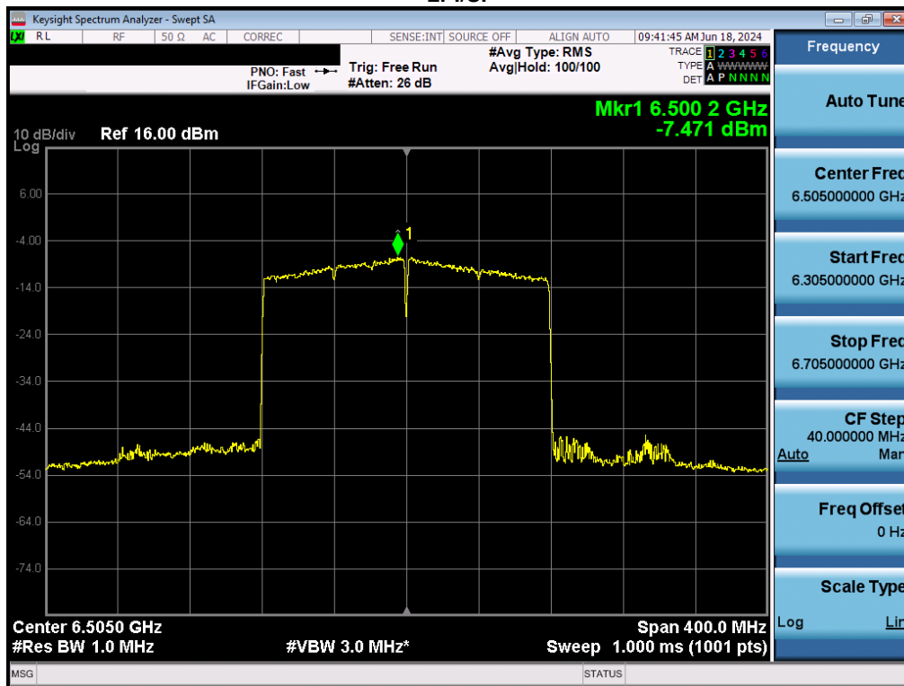
Plot 7-127. Power Spectral Density Plot MIMO ANT2 (160MHz BW 802.11ax (Full Tones) (UNII Band 6) – Ch. 111) - LPI/SP
