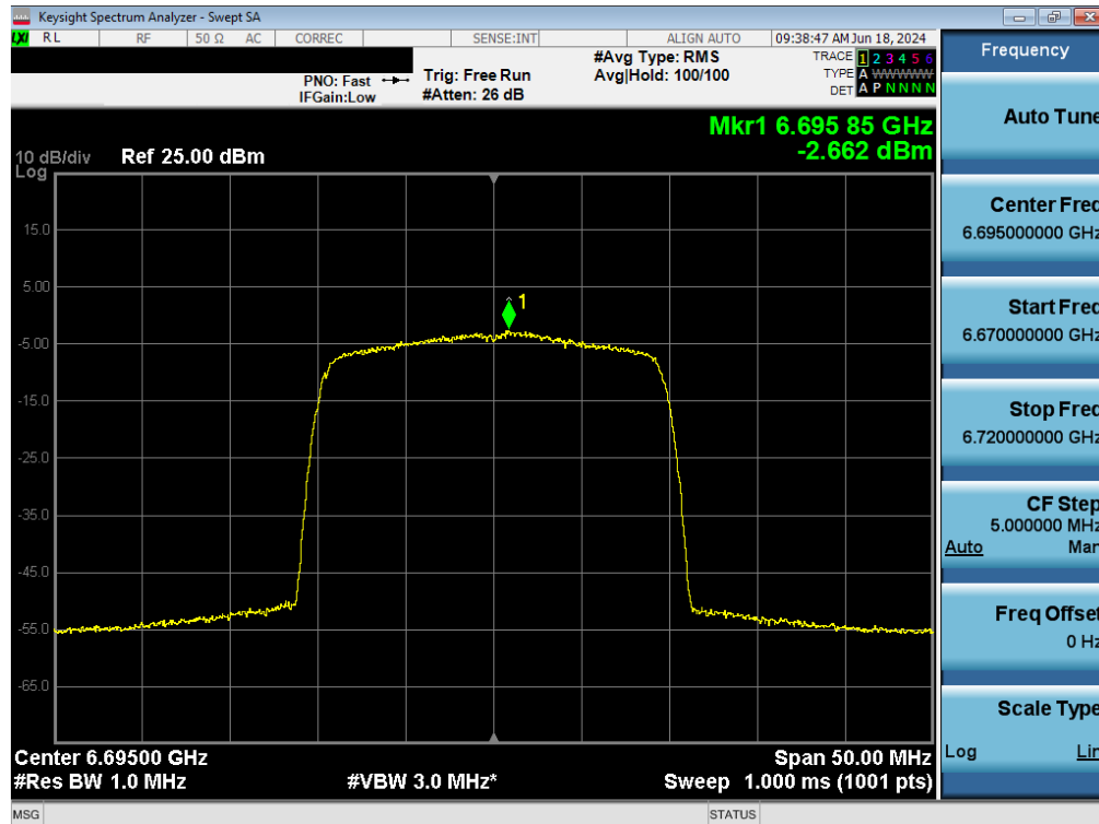
Plot 7-96. Power Spectral Density Plot MIMO ANT1 (20MHz BW 802.11ax (Full Tones) (UNII Band 7) – Ch. 149) - LPI/SP
