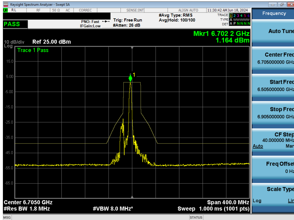
Plot 7-146. In-Band Emissions Plot MIMO ANT1 (80MHz BW 802.11ax (26 Tones) (UNII Band 7) – Ch. 151) - LPI/SP
