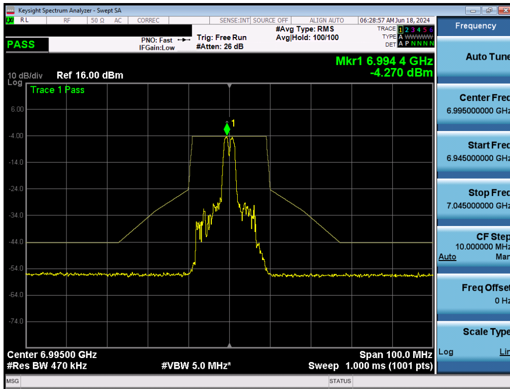
Plot 7-180. In-Band Emissions Plot MIMO ANT2 (20MHz BW 802.11ax (26 Tones) (UNII Band 8) – Ch. 209) - LPI/SP
