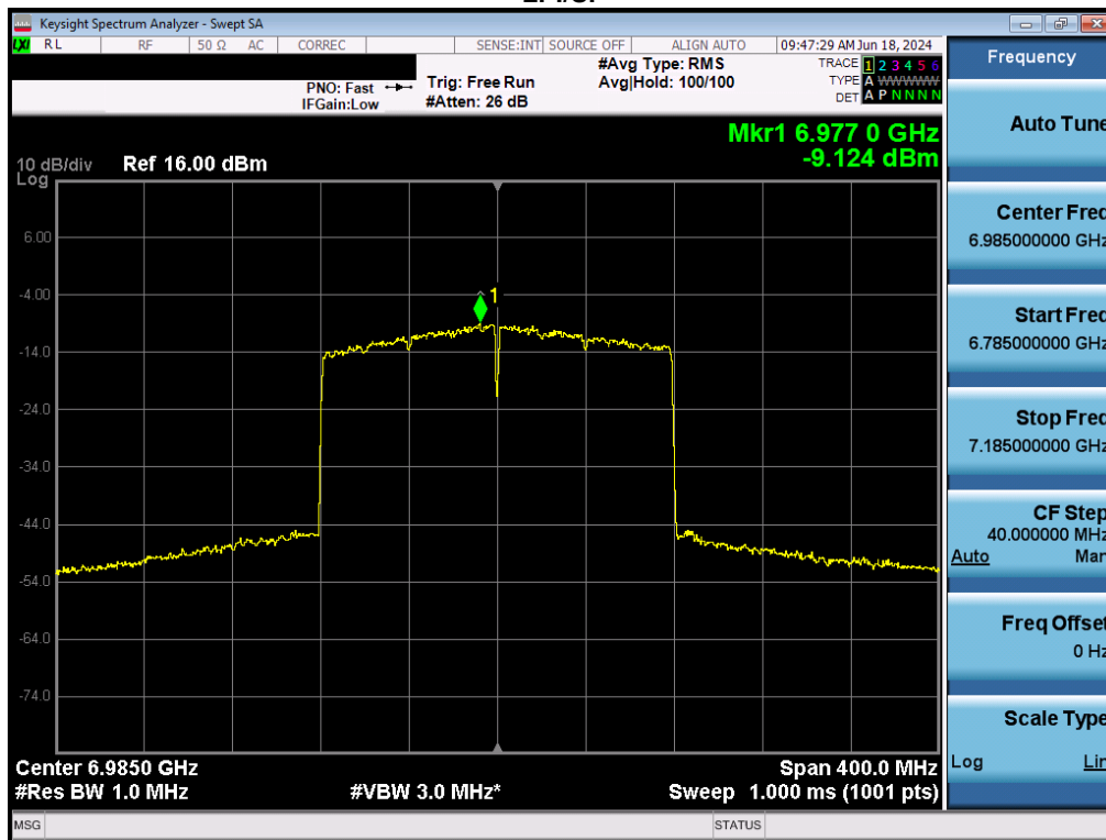
Plot 7-135. Power Spectral Density Plot MIMO ANT2 (160MHz BW 802.11ax (Full Tones) (UNII Band 8) – Ch. 207) - LPI/SP
