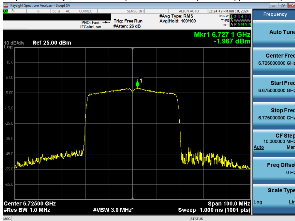
Plot 7-97. Power Spectral Density Plot MIMO ANT1 (40MHz BW 802.11ax (Full Tones) (UNII Band 7) – Ch. 155) - LPI/SP
