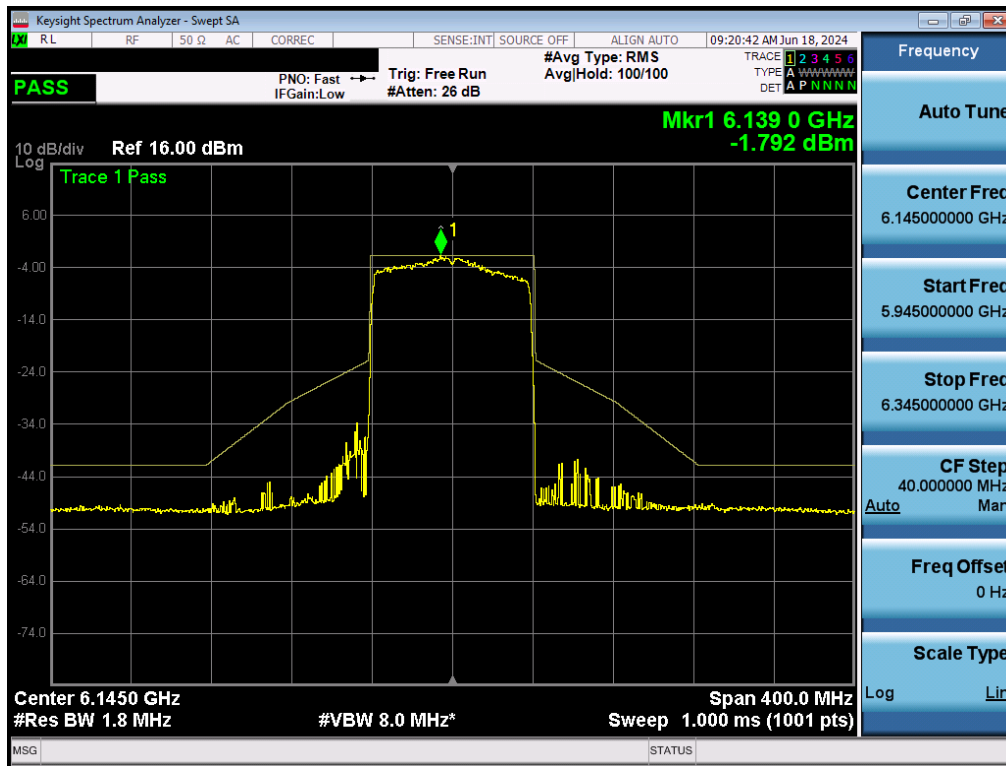
Plot 7-186. In-Band Emissions Plot MIMO ANT2 (80MHz BW 802.11ax (Full Tones) (UNII Band 5) – Ch. 39) - LPI/SP
