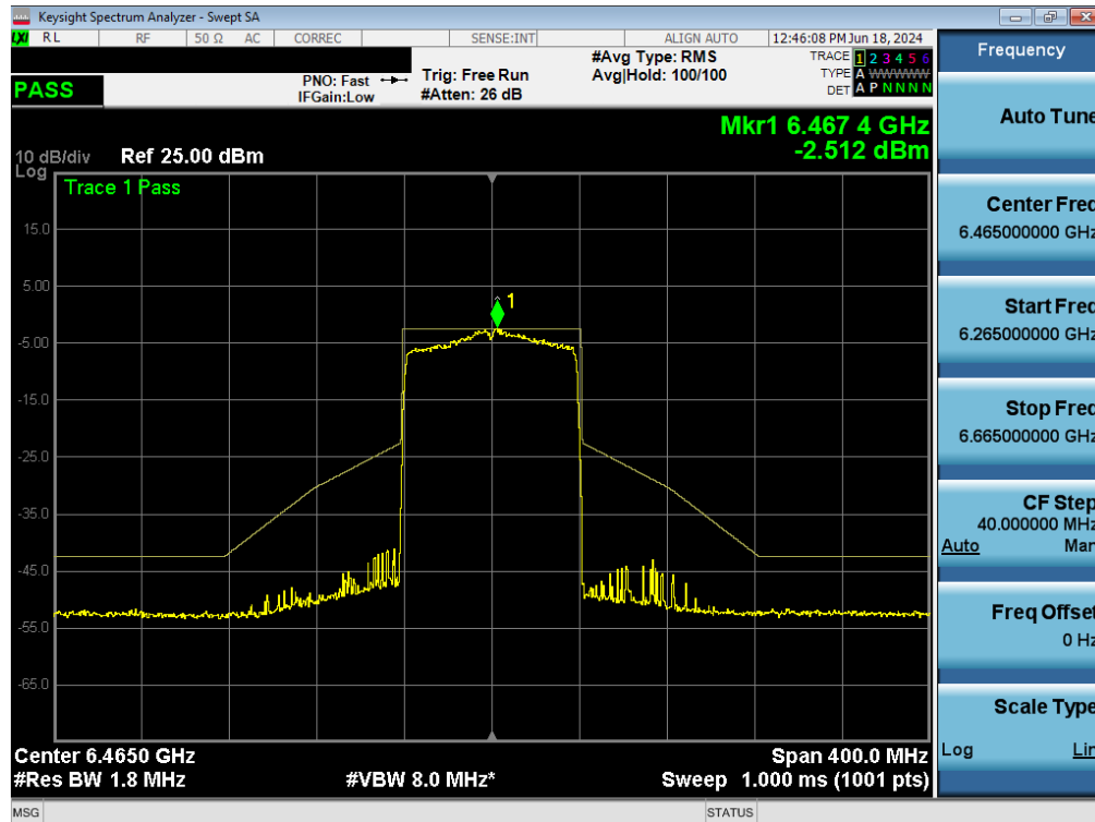
Plot 7-158. In-Band Emissions Plot MIMO ANT1 (80MHz BW 802.11ax (Full Tones) (UNII Band 6) – Ch. 103) - LPI/SP
