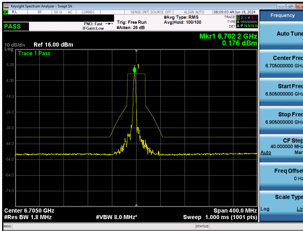
Plot 7-178. In-Band Emissions Plot MIMO ANT2 (80MHz BW 802.11ax (26 Tones) (UNII Band 7) – Ch. 151) - LPI/SP
