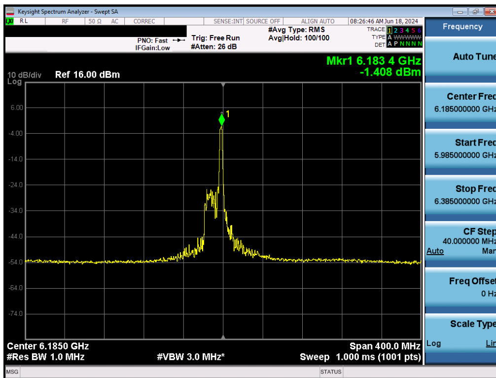
Plot 7-107. Power Spectral Density Plot MIMO ANT2 (160MHz BW 802.11ax (26 Tones) (UNII Band 5) – Ch. 47) - LPI/SP
