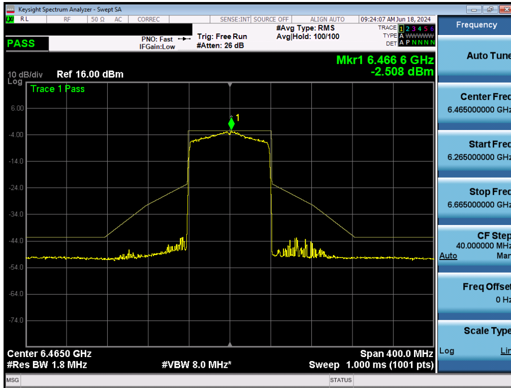
Plot 7-190. In-Band Emissions Plot MIMO ANT2 (80MHz BW 802.11ax (Full Tones) (UNII Band 6) – Ch. 103) - LPI/SP
