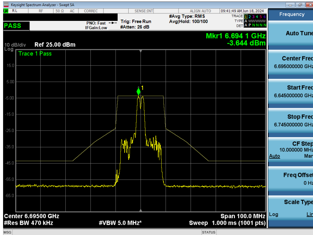
Plot 7-144. In-Band Emissions Plot MIMO ANT1 (20MHz BW 802.11ax (26 Tones) (UNII Band 7) – Ch. 149) - LPI/SP
