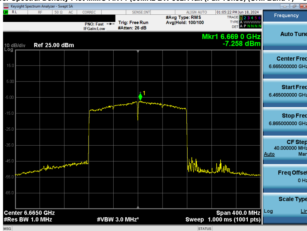
Plot 7-99. Power Spectral Density Plot MIMO ANT1 (160MHz BW 802.11ax (Full Tones) (UNII Band 7) – Ch. 143) - LPI/SP
