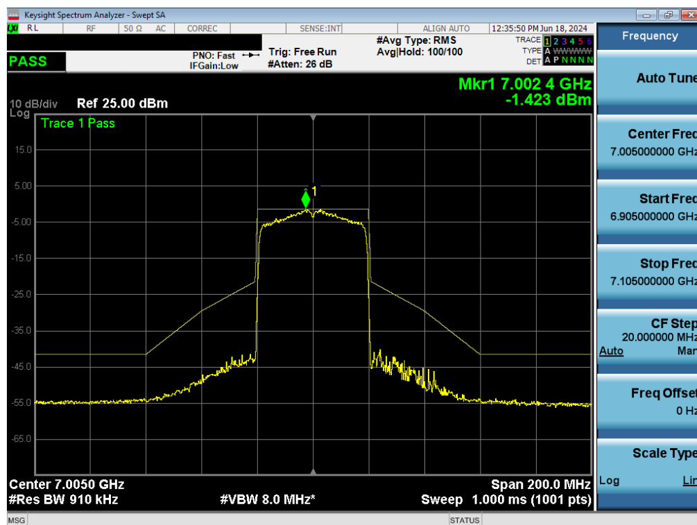
Plot 7-165. In-Band Emissions Plot MIMO ANT1 (40MHz BW 802.11ax (Full Tones) (UNII Band 8) – Ch. 211) - LPI/SP
