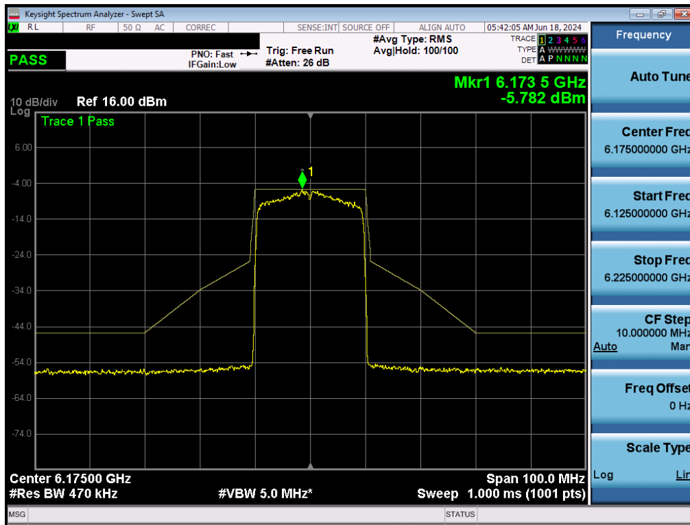
Plot 7-184. In-Band Emissions Plot MIMO ANT2 (20MHz BW 802.11ax (Full Tones) (UNII Band 5) – Ch. 45) - LPI/SP
