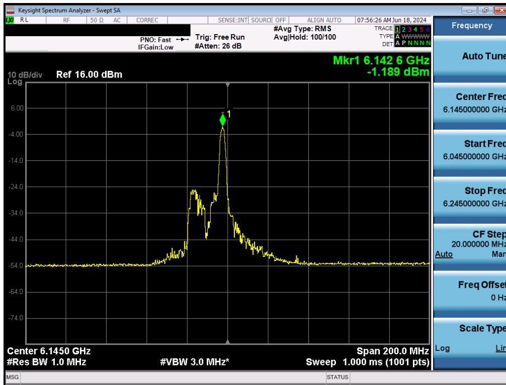
Plot 7-106. Power Spectral Density Plot MIMO ANT2 (80MHz BW 802.11ax (26 Tones) (UNII Band 5) – Ch. 39) - LPI/SP
