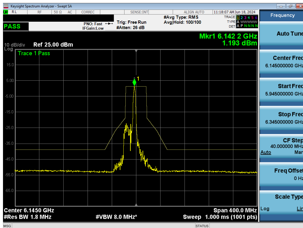
Plot 7-138. In-Band Emissions Plot MIMO ANT1 (80MHz BW 802.11ax (26 Tones) (UNII Band 5) – Ch. 39) - LPI/SP
