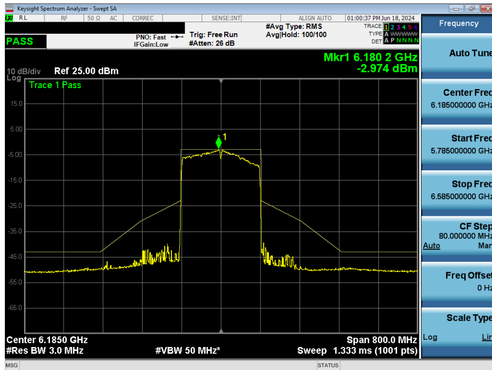
Plot 7-155. In-Band Emissions Plot MIMO ANT1 (160MHz BW 802.11ax (Full Tones) (UNII Band 5) – Ch. 47) - LPI/SP
