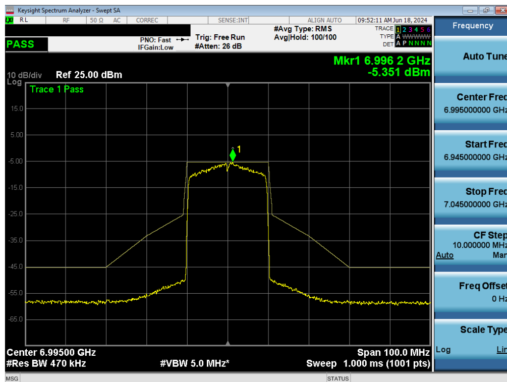
Plot 7-164. In-Band Emissions Plot MIMO ANT1 (20MHz BW 802.11ax (Full Tones) (UNII Band 8) – Ch. 209) - LPI/SP
