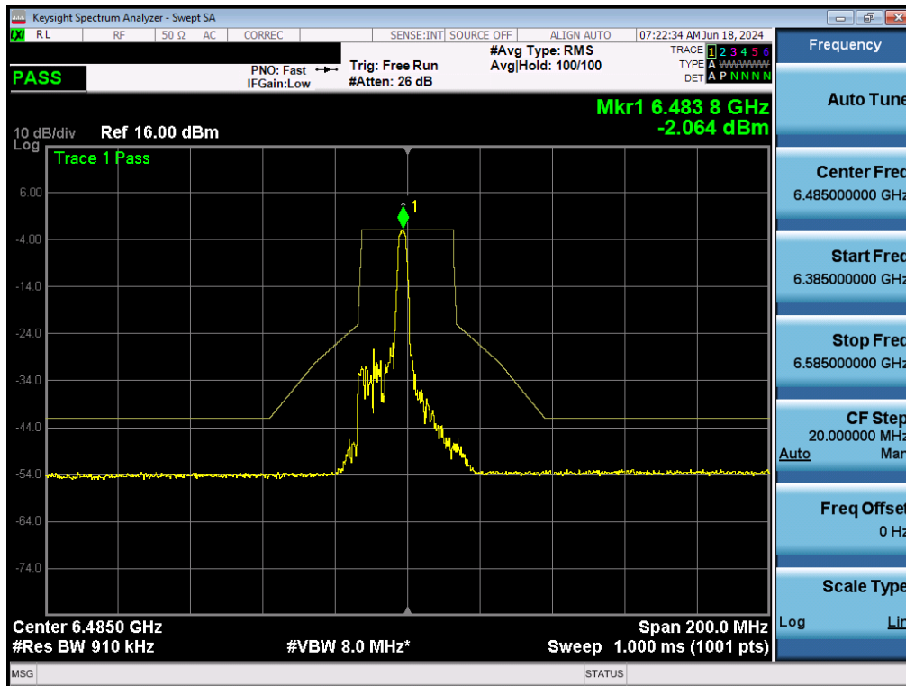
Plot 7-173. In-Band Emissions Plot MIMO ANT2 (40MHz BW 802.11ax (26 Tones) (UNII Band 6) – Ch. 107) - LPI/SP
