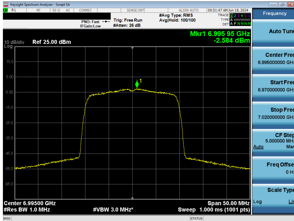
Plot 7-100. Power Spectral Density Plot MIMO ANT1 (20MHz BW 802.11ax (Full Tones) (UNII Band 8) – Ch. 209) – LPI/SP
