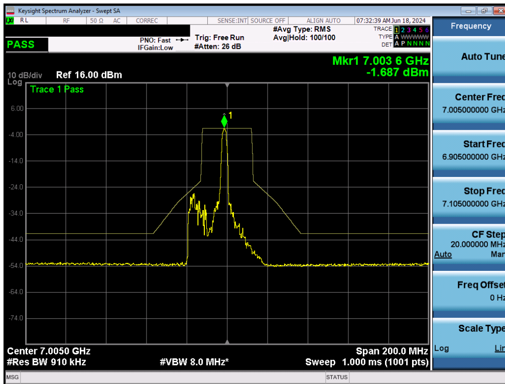
Plot 7-181. In-Band Emissions Plot MIMO ANT2 (40MHz BW 802.11ax (26 Tones) (UNII Band 8) – Ch. 211) - LPI/SP
