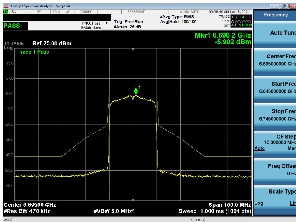
Plot 7-160. In-Band Emissions Plot MIMO ANT1 (20MHz BW 802.11ax (Full Tones) (UNII Band 7) – Ch. 149) - LPI/SP
