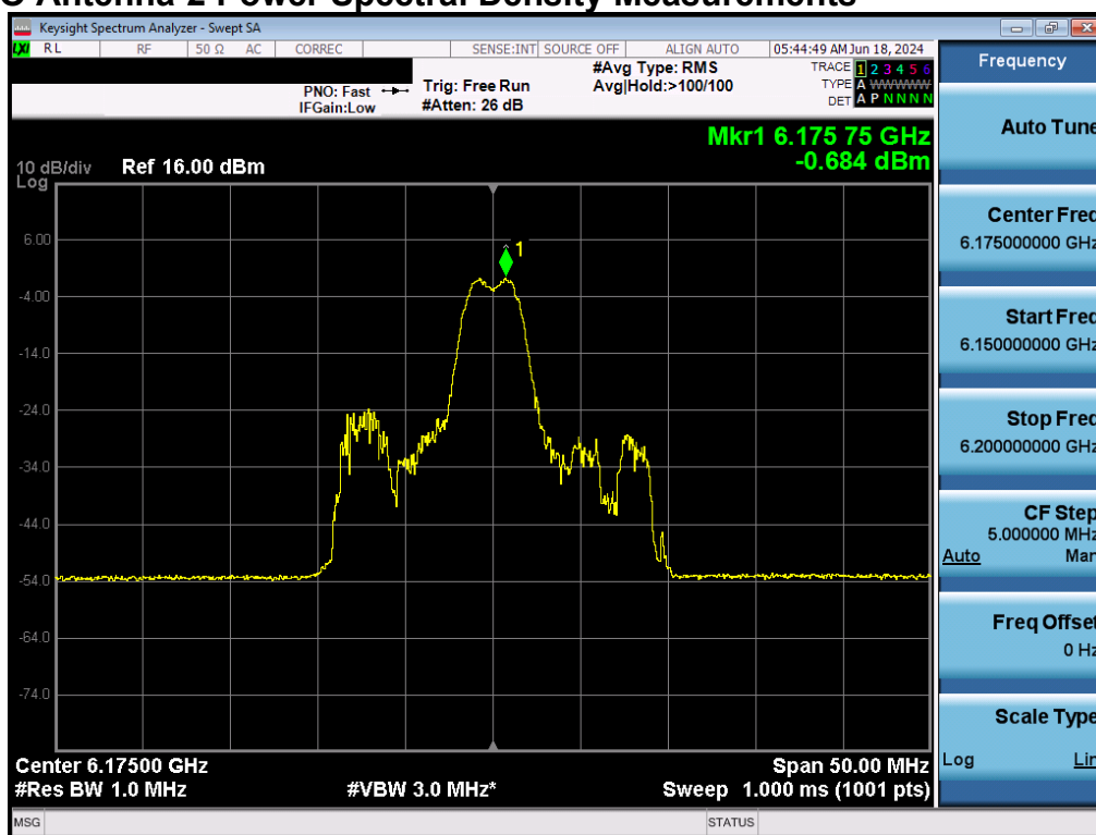
Plot 7-104. Power Spectral Density Plot MIMO ANT2 (20MHz BW 802.11ax (26 Tones) (UNII Band 5) – Ch. 45) - LPI/SP
