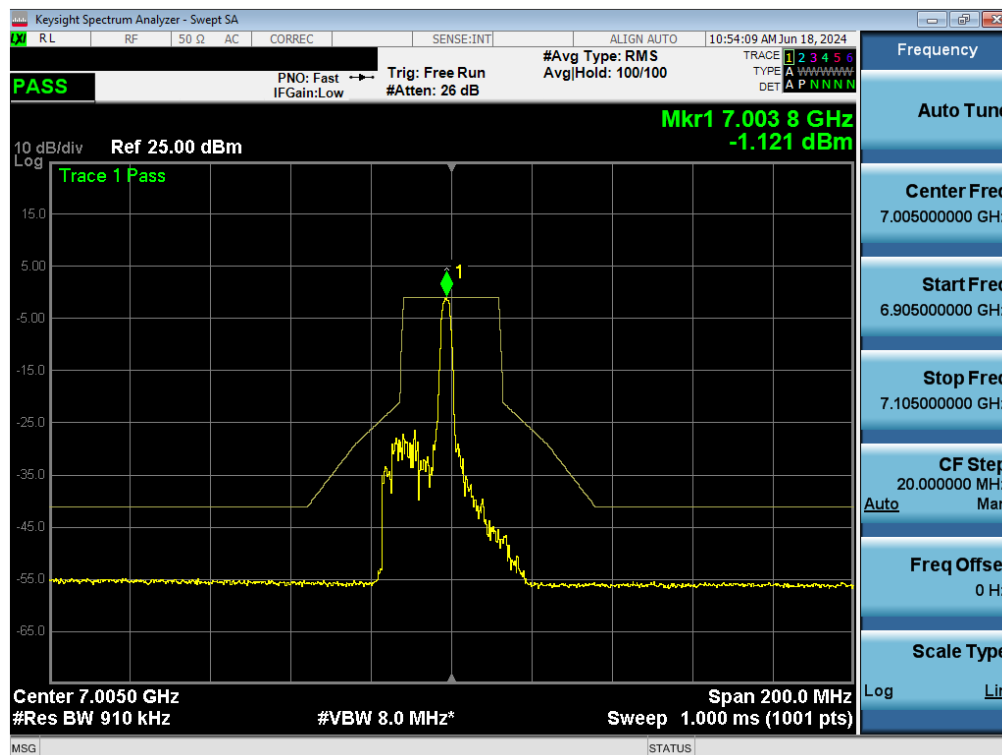
Plot 7-149. In-Band Emissions Plot MIMO ANT1 (40MHz BW 802.11ax (26 Tones) (UNII Band 8) – Ch. 211) - LPI/SP
