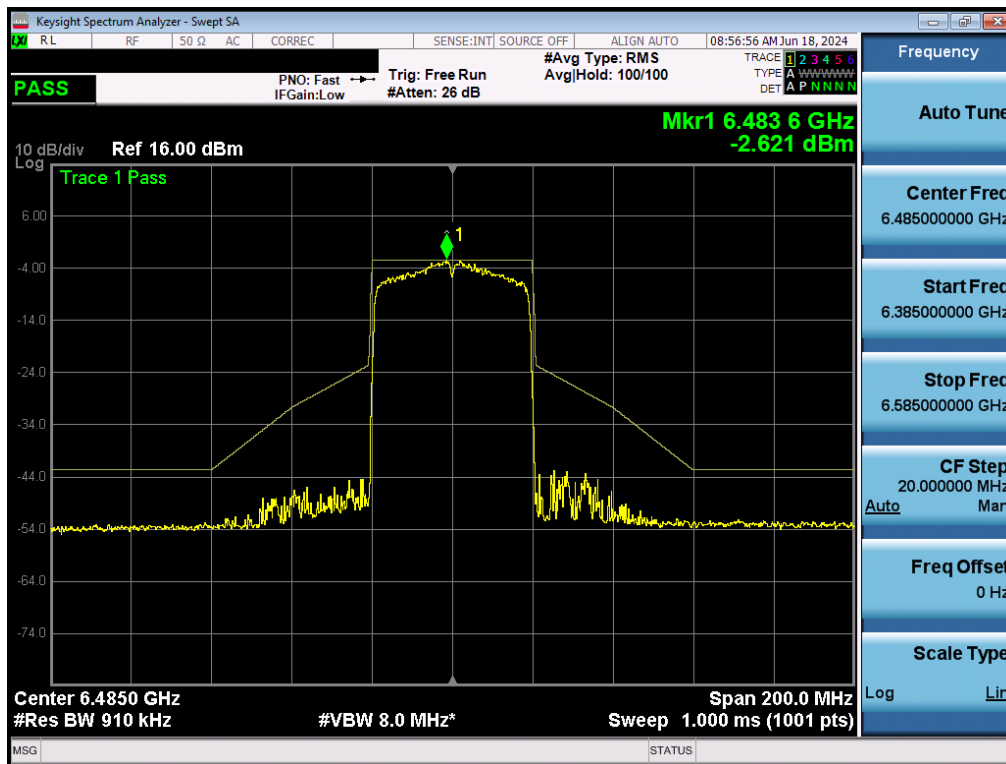
Plot 7-189. In-Band Emissions Plot MIMO ANT2 (40MHz BW 802.11ax (Full Tones) (UNII Band 6) – Ch. 107) - LPI/SP
