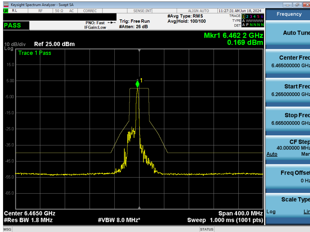
Plot 7-142. In-Band Emissions Plot MIMO ANT1 (80MHz BW 802.11ax (26 Tones) (UNII Band 6) – Ch. 103) - LPI/SP
