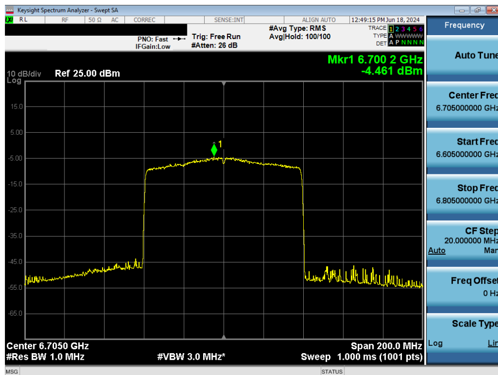
Plot 7-98. Power Spectral Density Plot MIMO ANT1 (80MHz BW 802.11ax (Full Tones) (UNII Band 7) – Ch. 151) - LPI/SP
