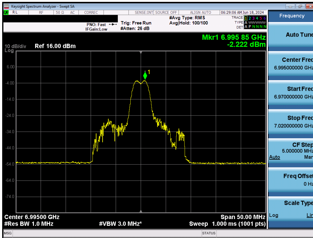
Plot 7-116. Power Spectral Density Plot MIMO ANT2 (20MHz BW 802.11ax (26 Tones) (UNII Band 8) – Ch. 209) - LPI/SP
