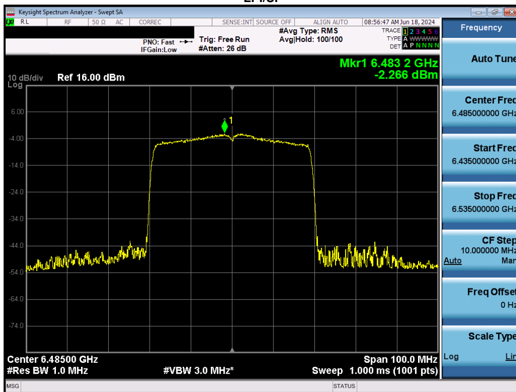
Plot 7-125. Power Spectral Density Plot MIMO ANT2 (40MHz BW 802.11ax (Full Tones) (UNII Band 6) – Ch. 107) - LPI/SP
