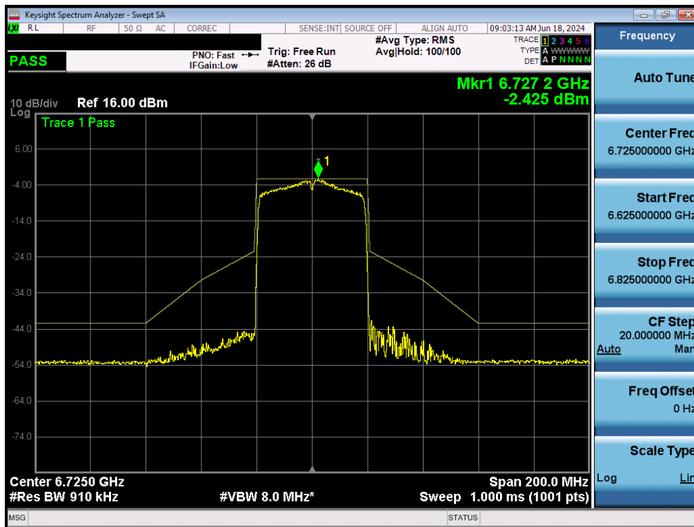
Plot 7-193. In-Band Emissions Plot MIMO ANT2 (40MHz BW 802.11ax (Full Tones) (UNII Band 7) – Ch. 155) - LPI/SP
