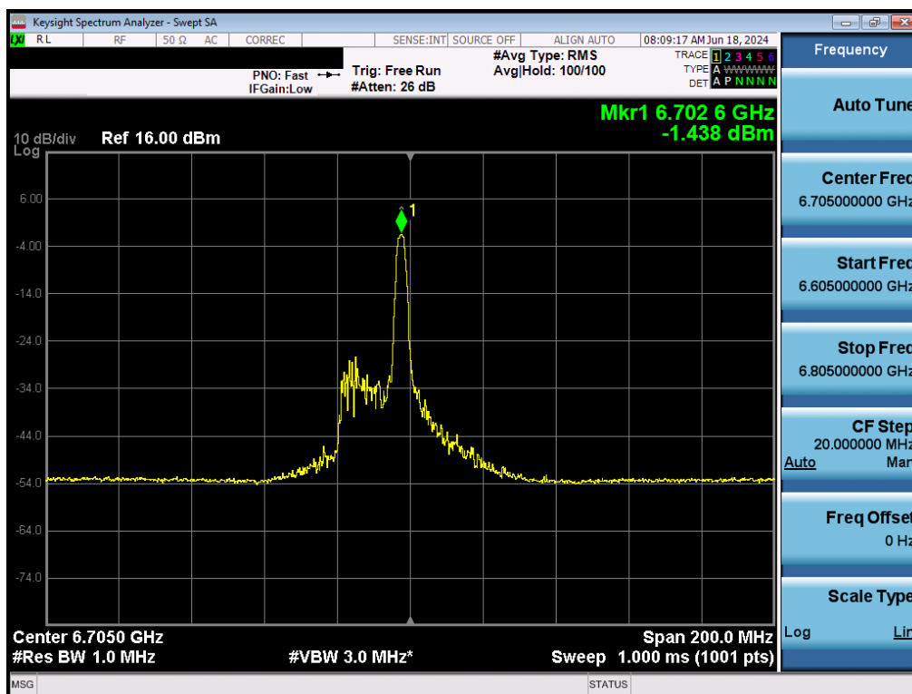
Plot 7-114. Power Spectral Density Plot MIMO ANT2 (80MHz BW 802.11ax (26 Tones) (UNII Band 7) – Ch. 151) - LPI/SP
