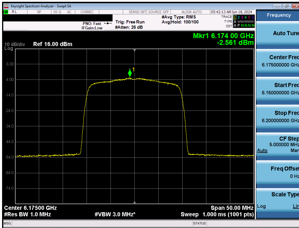
Plot 7-120. Power Spectral Density Plot MIMO ANT2 (20MHz BW 802.11ax (Full Tones) (UNII Band 5) – Ch. 45) - LPI/SP
