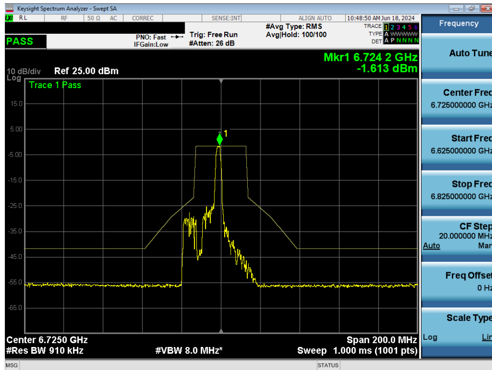
Plot 7-145. In-Band Emissions Plot MIMO ANT1 (40MHz BW 802.11ax (26 Tones) (UNII Band 7) – Ch. 155) - LPI/SP
