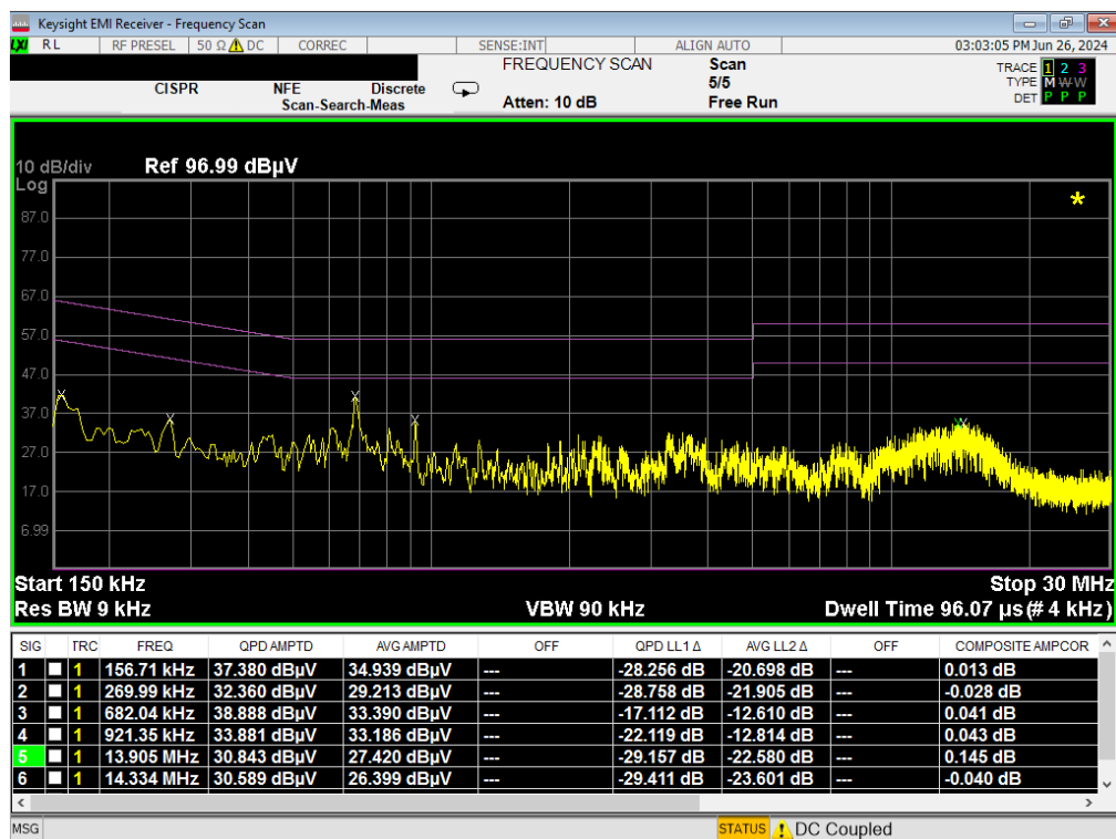
Plot 7-33. Line-Conducted Test Plot (L1) – Digitizer (Eraser)
