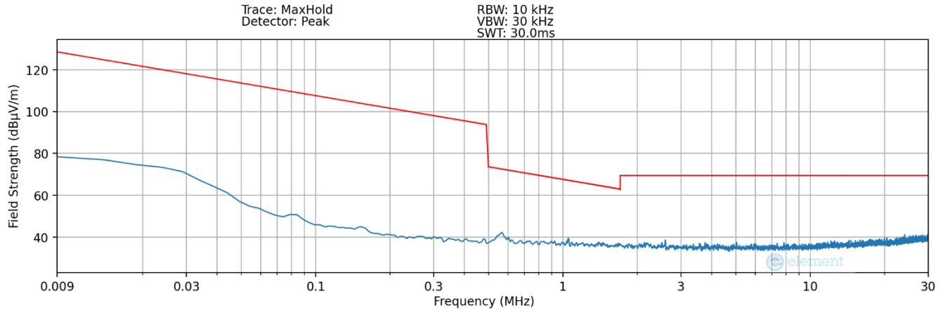
Plot 7-16. Radiated Spurious Plot 9kHz – 30MHz (Pol. X – Digitizer – Hover)
