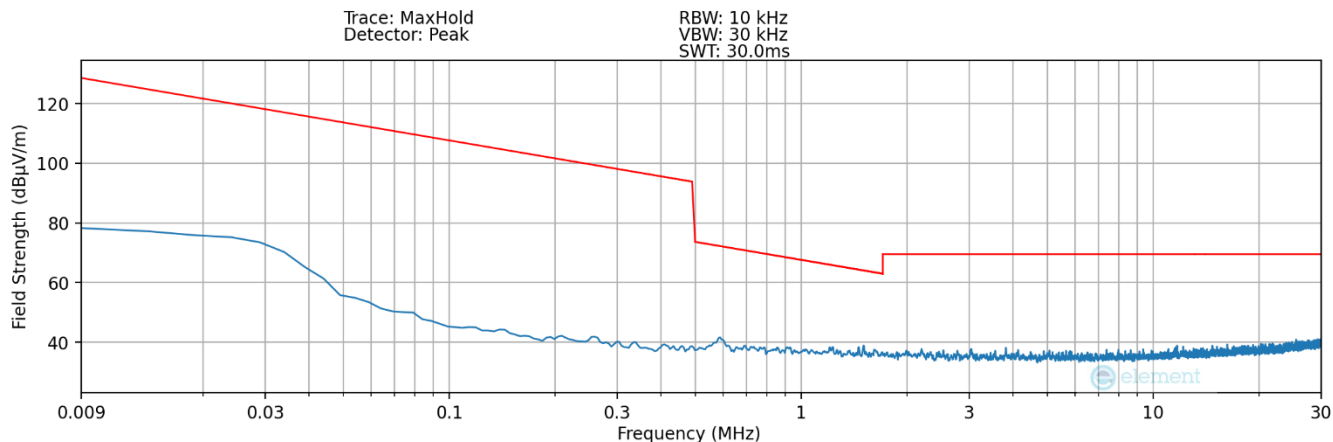
Plot 7-19. Radiated Spurious Plot 9kHz – 30MHz (Pol. X – Digitizer – Eraser)
