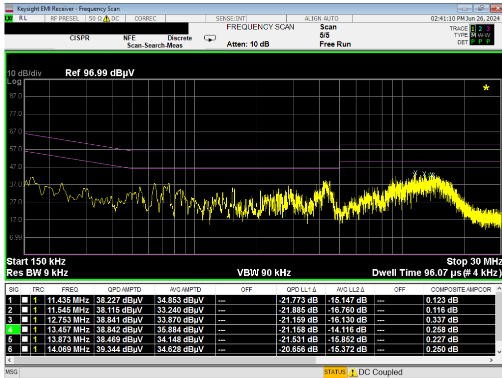
Plot 7-29. Line-Conducted Test Plot (L1) – Digitizer (Click)
