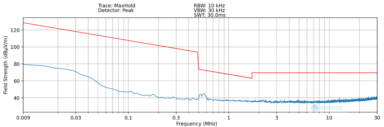
Plot 7-8 Radiated Spurious Plot 9kHz – 30MHz (Pol. Y – Device to Pen – SPEN Detection 1)
