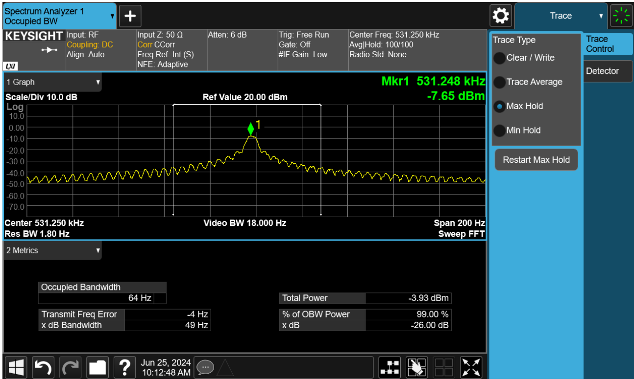
Plot 7-3. Occupied Bandwidth Measurement – Click
