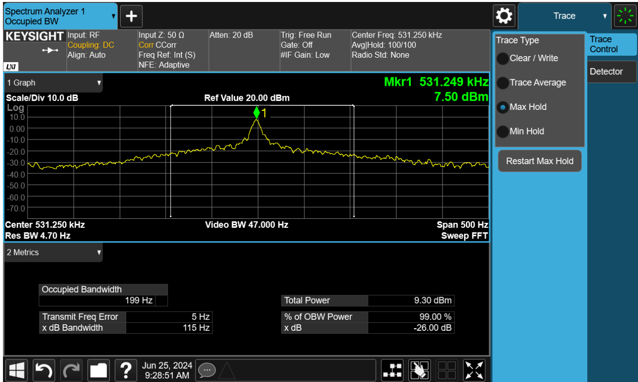
Plot 7-1. Occupied Bandwidth Measurement – Device to Pen (SPEN Detection 1)
