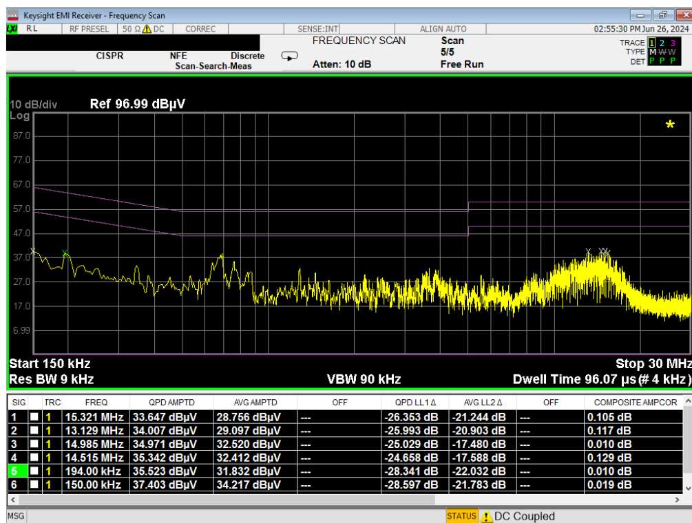
Plot 7-32. Line-Conducted Test Plot (N) – Digitizer (Hover)
