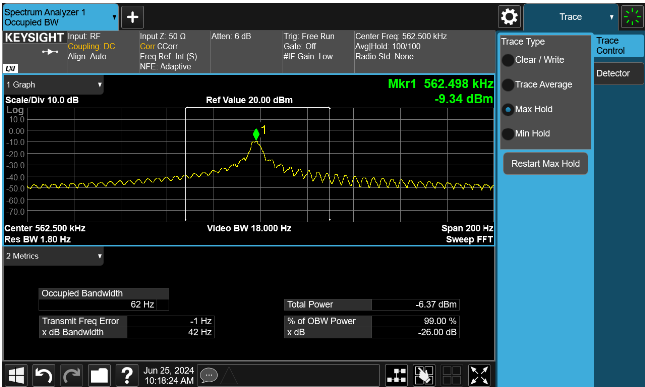
Plot 7-4. Occupied Bandwidth Measurement – Hover
