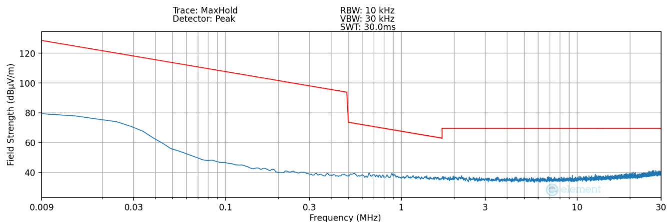
Plot 7-15. Radiated Spurious Plot 9kHz – 30MHz (Pol. Z– Digitizer – Click)
