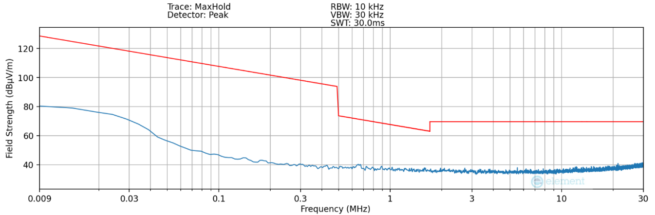
Plot 7-22. Radiated Spurious Plot 9kHz – 30MHz (Pol. X – Keyboard Detection)
