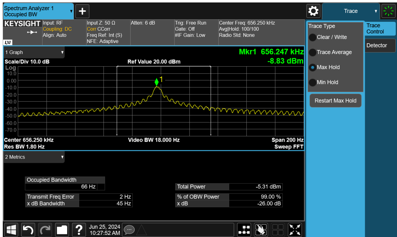
Plot 7-6. Occupied Bandwidth Measurement – Keyboard Detection
