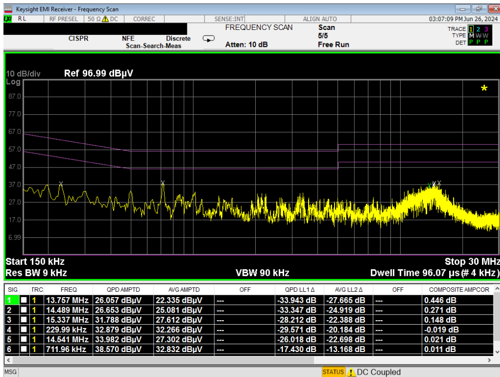
Plot 7-36. Line-Conducted Test Plot (N) – Digitizer (Keyboard Detection)
