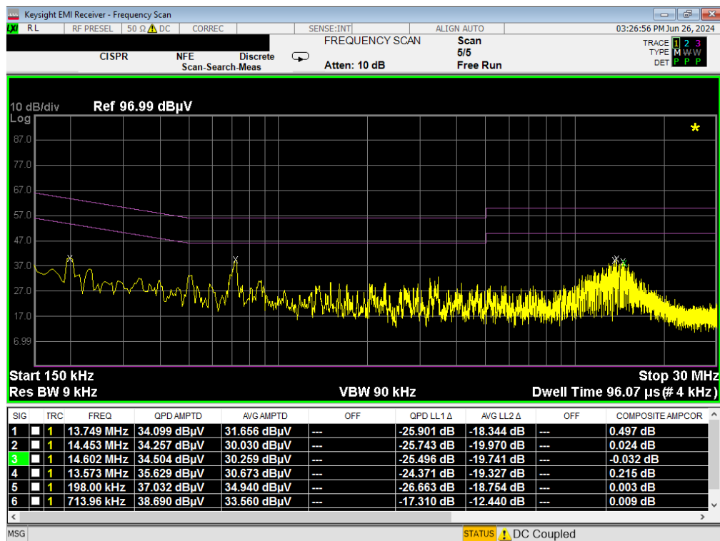
Plot 7-28. Line-Conducted Test Plot (N) – Device to Pen (SPEN Detection 2)
