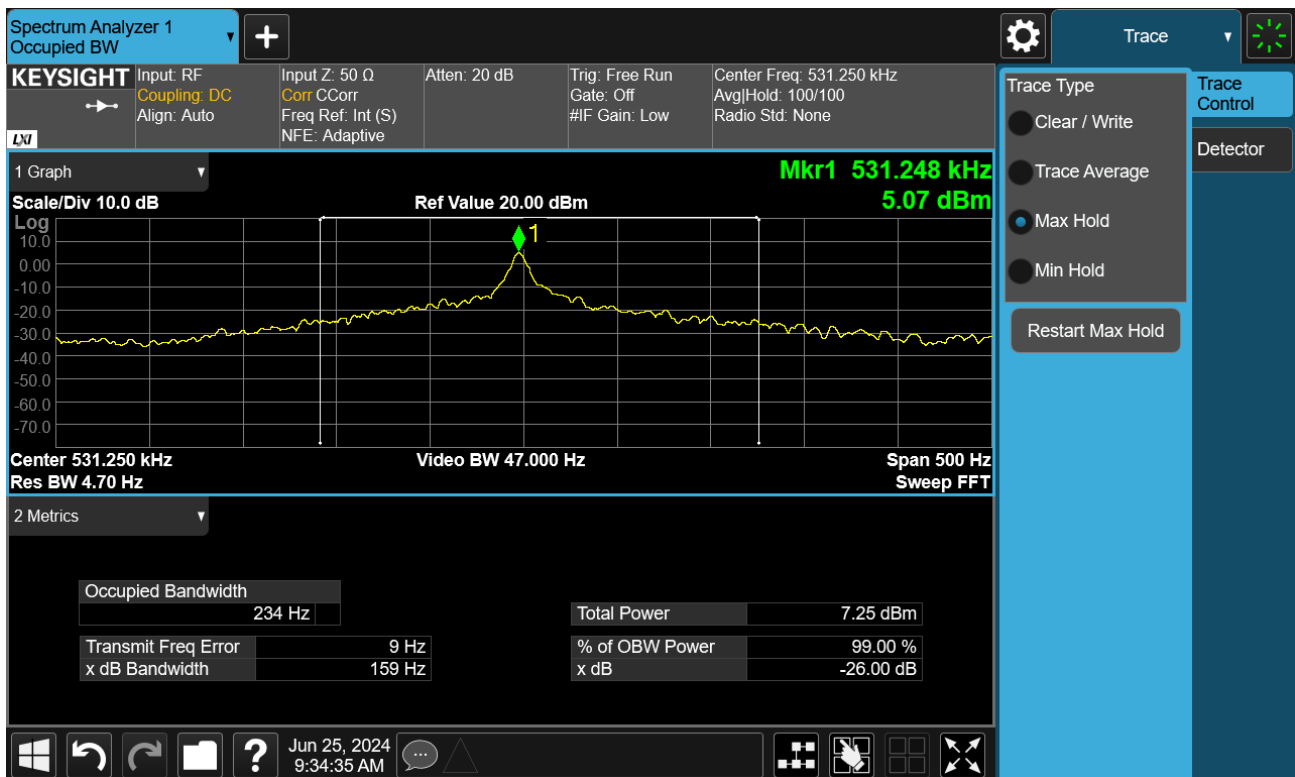
Plot 7-2. Occupied Bandwidth Measurement – Device to Pen (SPEN Detection 2)
