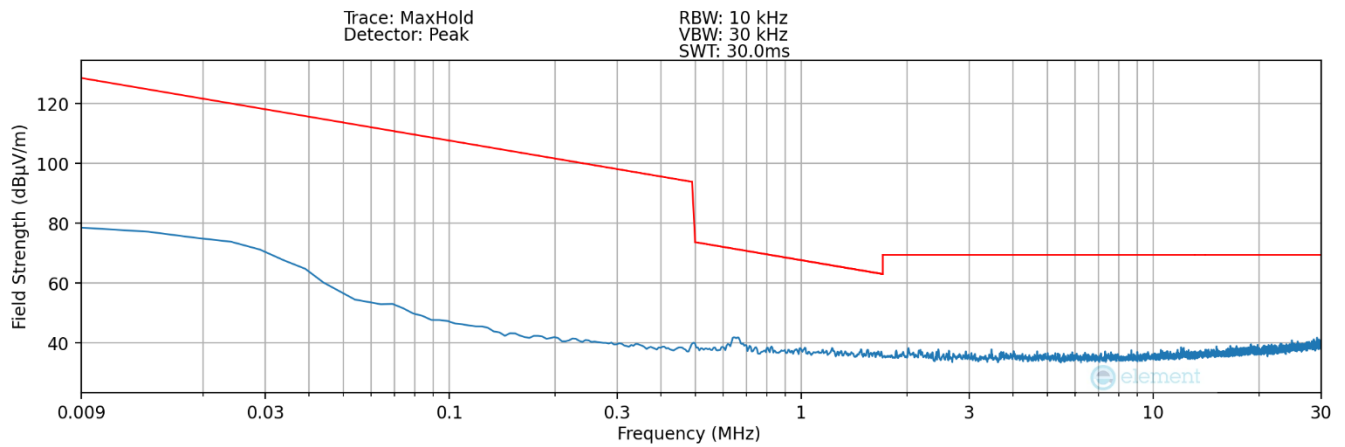
Plot 7-23Radiated Spurious Plot 9kHz – 30MHz (Pol. Y – Keyboard Detection)
