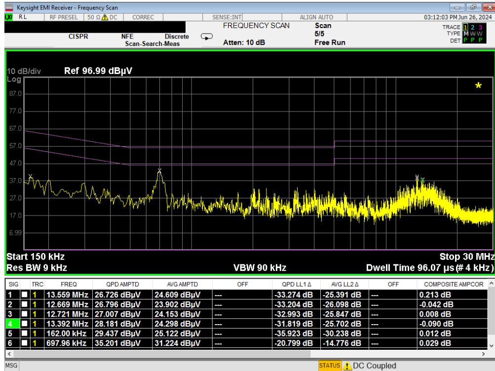
Plot 7-35. Line-Conducted Test Plot (L1) – Digitizer (Keyboard Detection)
