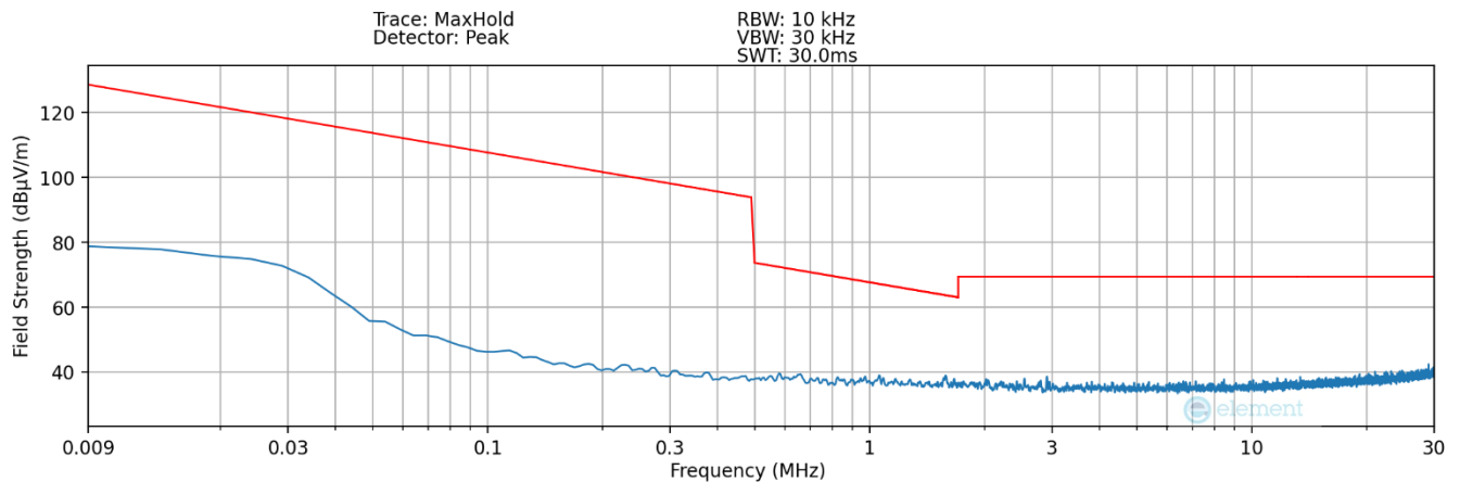
Plot 7-24. Radiated Spurious Plot 9kHz – 30MHz (Pol. Z – Keyboard Detection)
