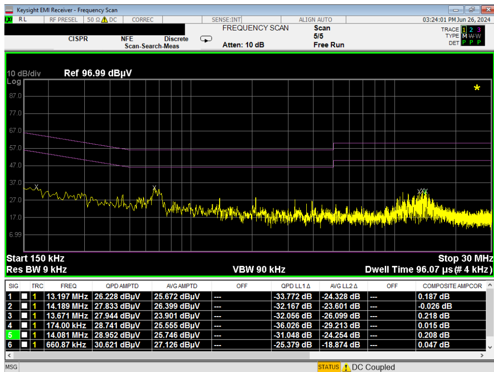
Plot 7-26. Line-Conducted Test Plot (N) – Device to Pen (SPEN Detection 1)
