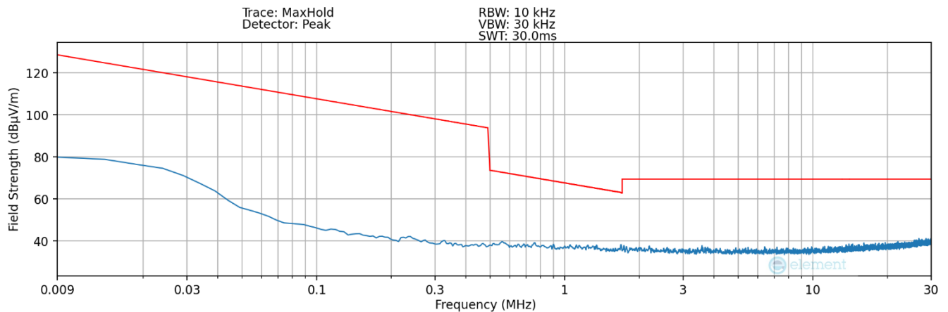
Plot 7-18. Radiated Spurious Plot 9kHz – 30MHz (Pol. Z – Digitizer – Hover)
