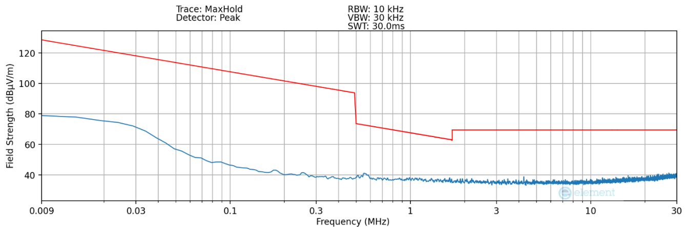
Plot 7-12. Radiated Spurious Plot 9kHz – 30MHz (Pol. Z – Device to Pen – SPEN Detection 2)
