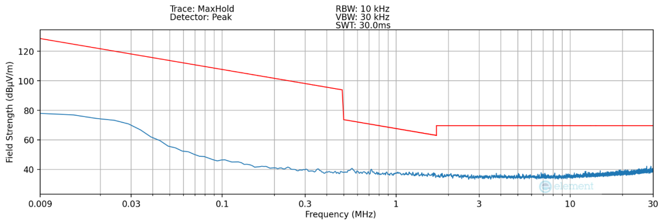
Plot 7-17Radiated Spurious Plot 9kHz – 30MHz (Pol. Y – Digitizer – Hover)
