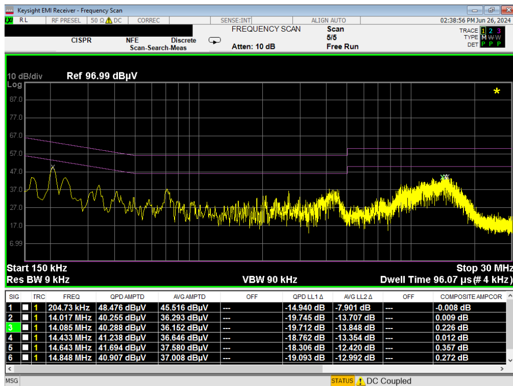
Plot 7-30. Line-Conducted Test Plot (N) – Digitizer (Click)
