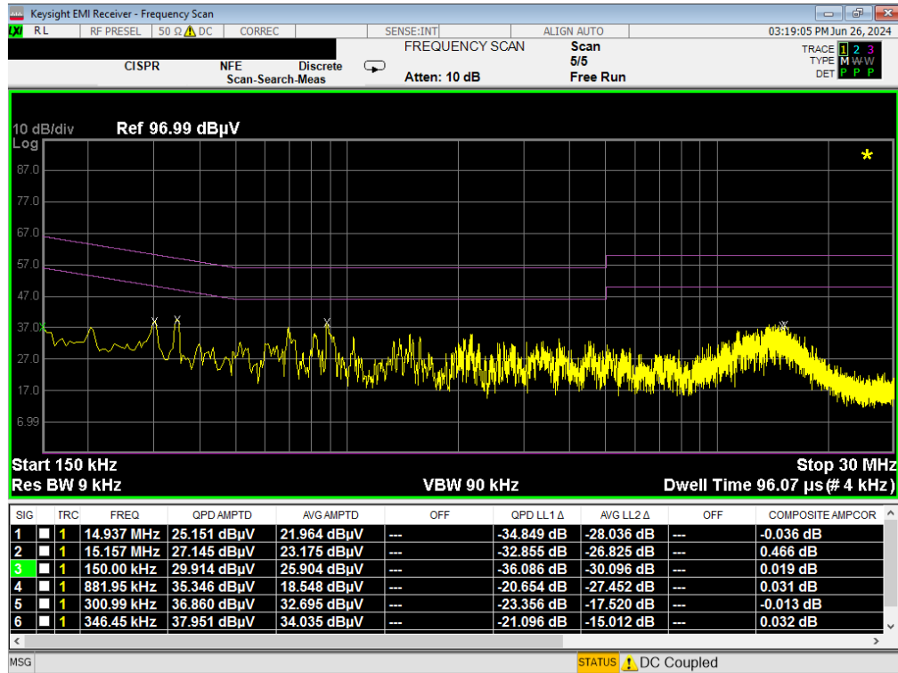
Plot 7-25. Line-Conducted Test Plot (L1) – Device to Pen (SPEN Detection 1)
