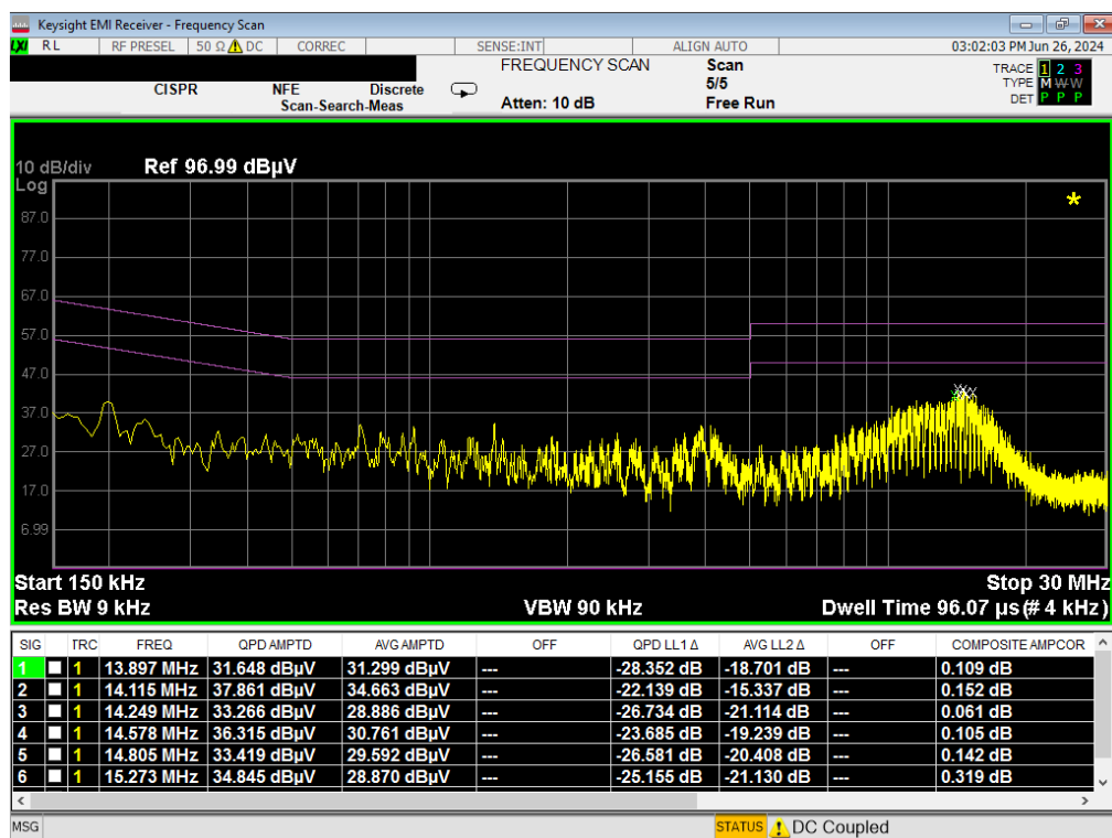
Plot 7-34. Line-Conducted Test Plot (N) – Digitizer (Eraser)
