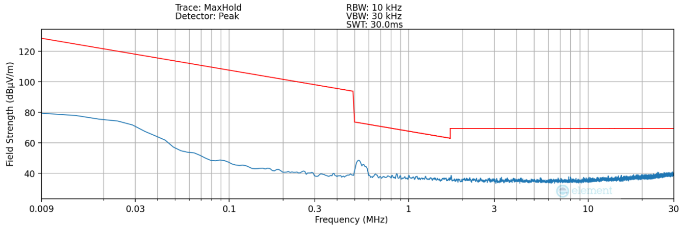
Plot 7-7. Radiated Spurious Plot 9kHz – 30MHz (Pol. X – Device to Pen – SPEN Detection 1)
