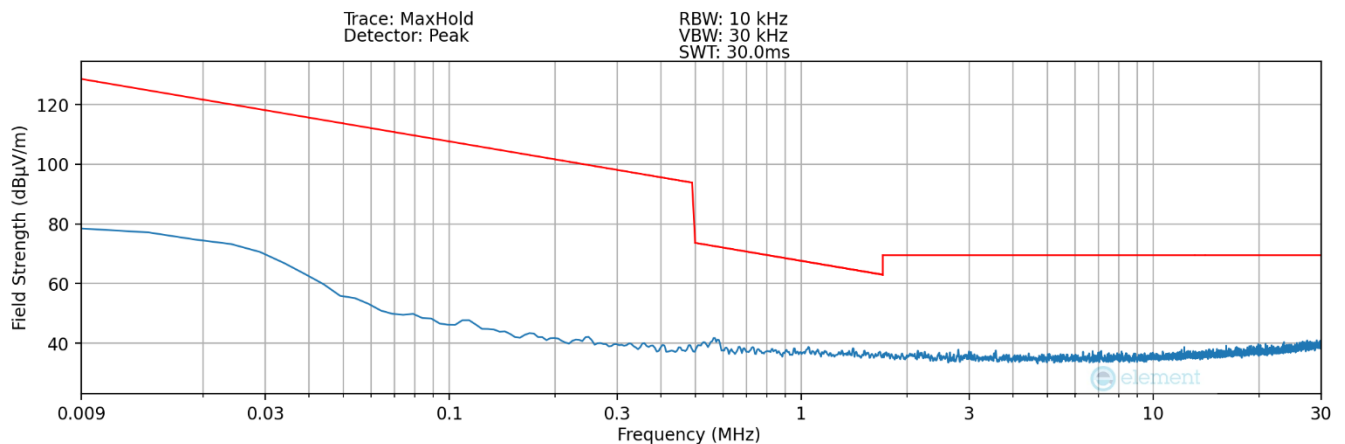
Plot 7-9. Radiated Spurious Plot 9kHz – 30MHz (Pol. Z – Device to Pen – SPEN Detection 1)
