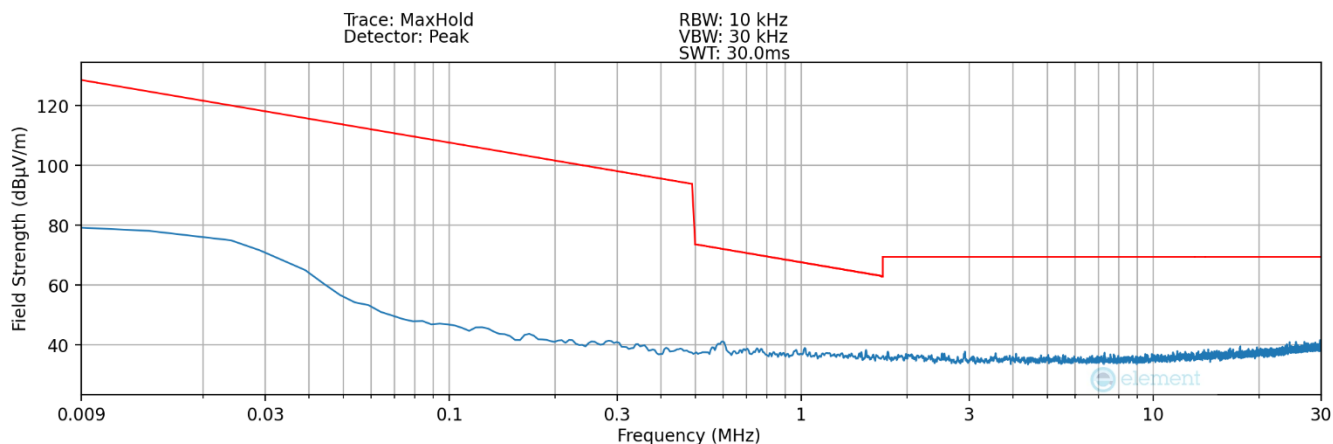
Plot 7-20Radiated Spurious Plot 9kHz – 30MHz (Pol. Y – Digitizer – Eraser)
