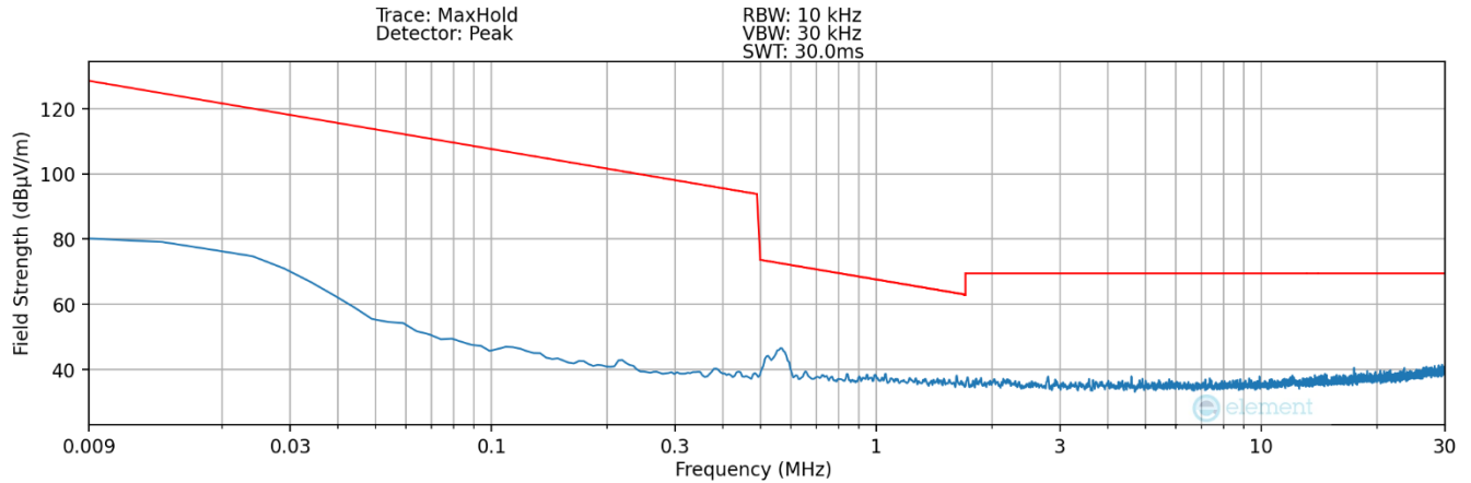
Plot 7-10. Radiated Spurious Plot 9kHz – 30MHz (Pol. X – Device to Pen – SPEN Detection 2)
