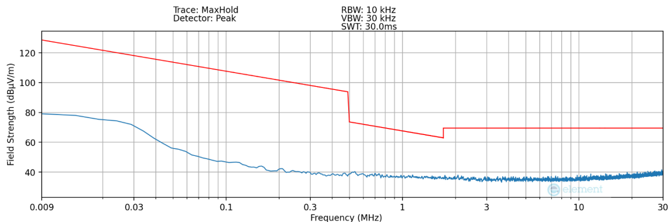
Plot 7-14Radiated Spurious Plot 9kHz – 30MHz (Pol. Y – Digitizer – Click)
