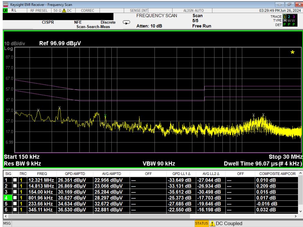
Plot 7-27. Line-Conducted Test Plot (L1) – Device to Pen (SPEN Detection 2)
