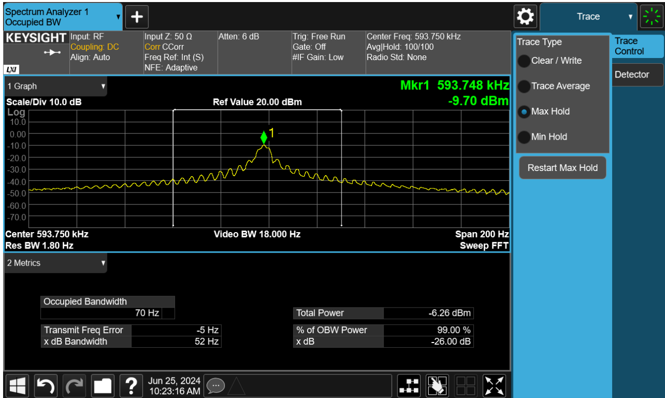
Plot 7-5. Occupied Bandwidth Measurement – Eraser
