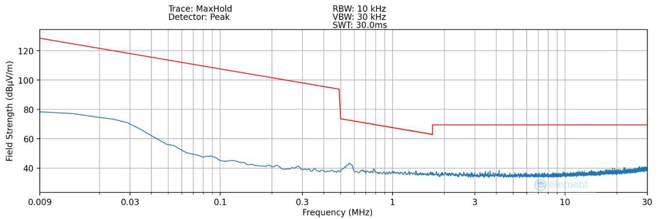
Plot 7-11Radiated Spurious Plot 9kHz – 30MHz (Pol. Y – Device to Pen – SPEN Detection 2)
