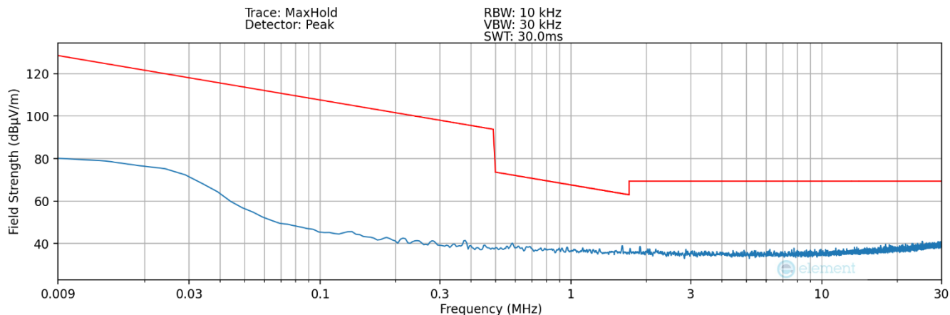
Plot 7-21. Radiated Spurious Plot 9kHz – 30MHz (Pol. Z– Digitizer – Eraser)
