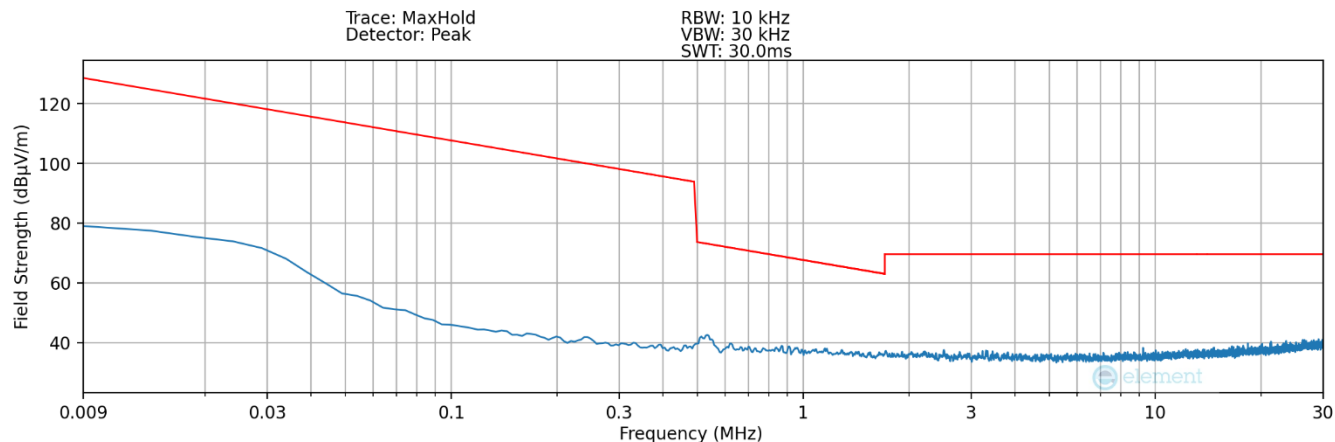
Plot 7-13. Radiated Spurious Plot 9kHz – 30MHz (Pol. X – Digitizer – Click)
