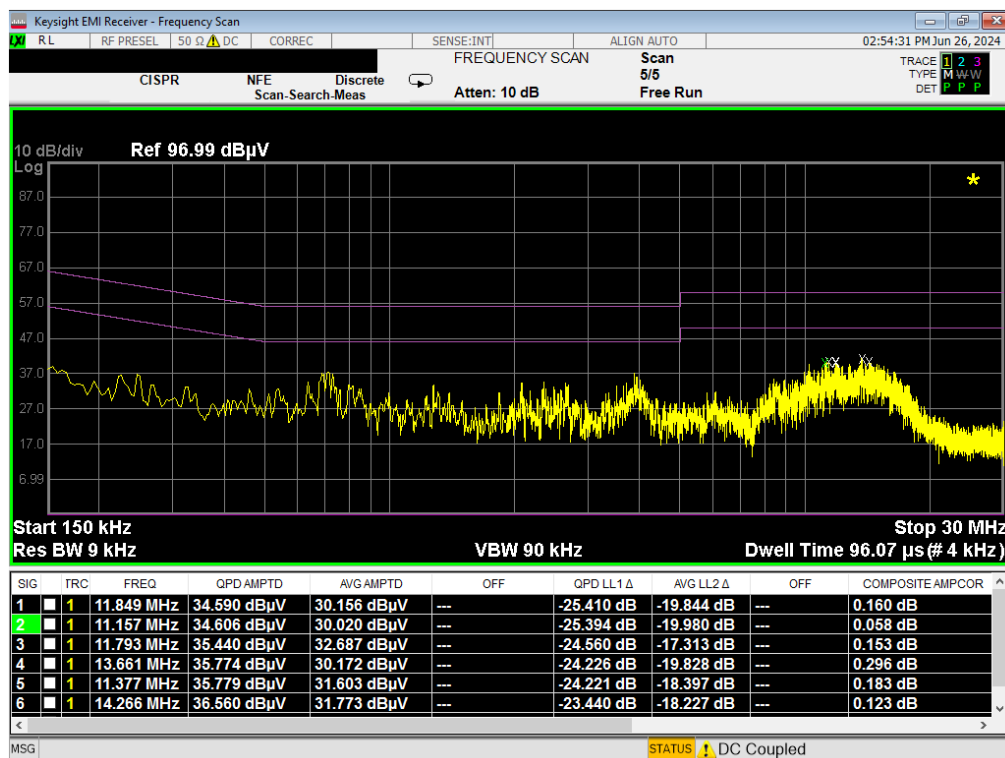
Plot 7-31. Line-Conducted Test Plot (L1) – Digitizer (Hover)
