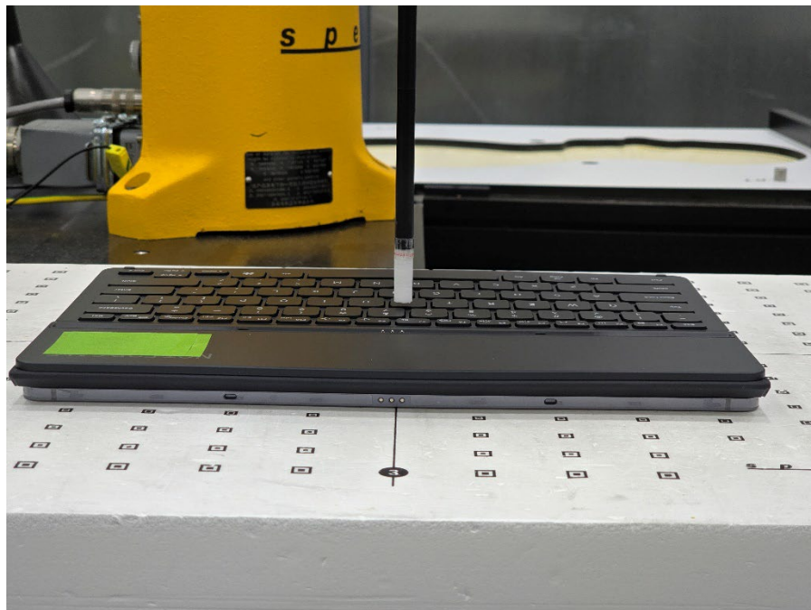
SAR Test Setup Photo 55 – Tablet with Keyboard Variant 2, Back Side at 2 mm
