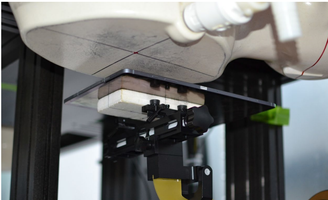
SAR Test Setup Photo 13 – Tablet, Back Side at 19 mm – Antenna WIFI 2
