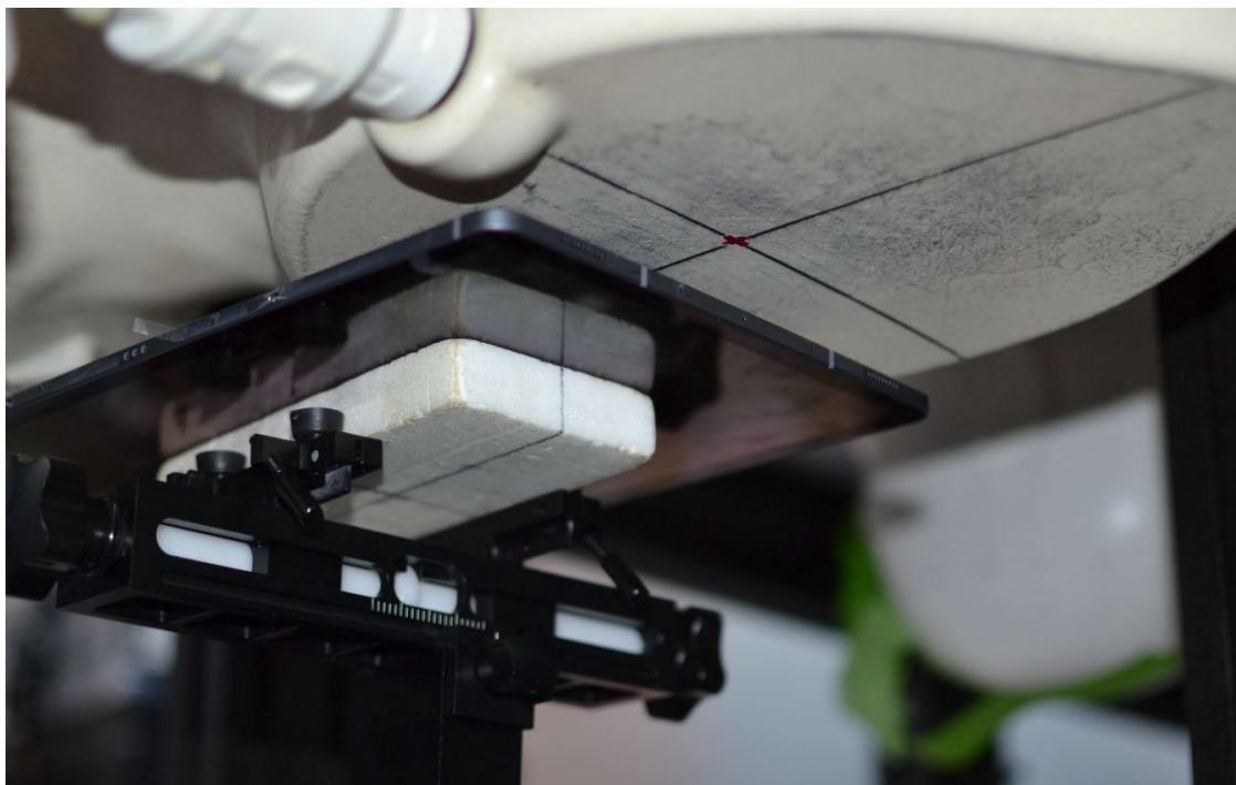
SAR Test Setup Photo 1 – Tablet, Back Side at 19 mm – Antenna M1
