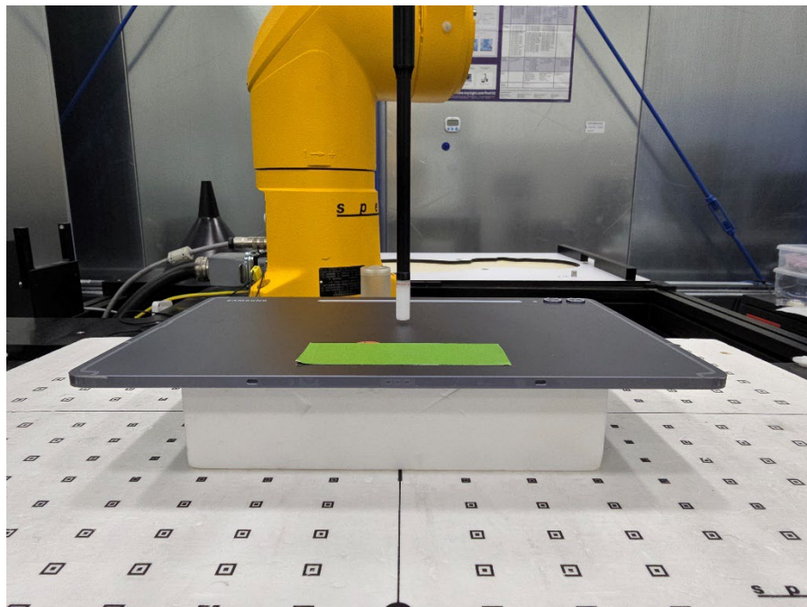
SAR Test Setup Photo 56 – Tablet, Back Side at 2 mm
