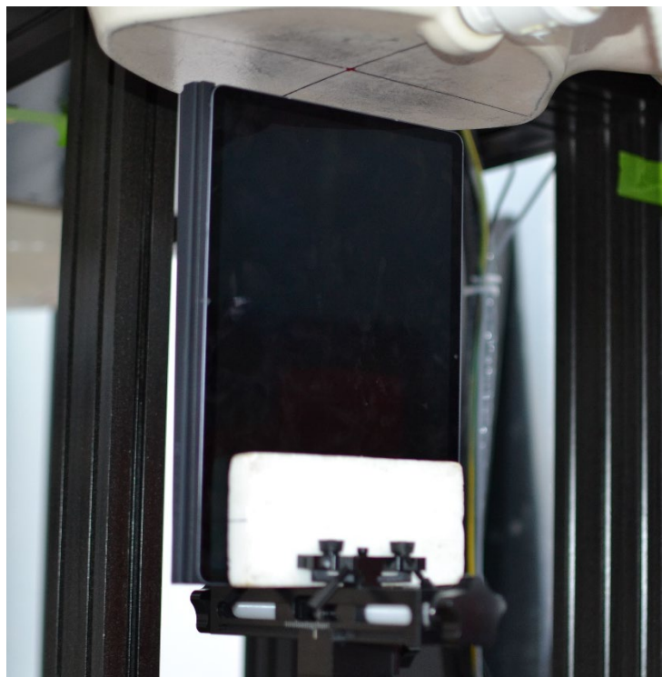
SAR Test Setup Photo 45 – Tablet with Keyboard Variant 1, Top Edge at 19 mm
