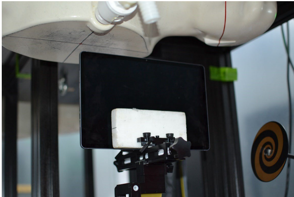
SAR Test Setup Photo 33 – Tablet, Right Edge at 15 mm – Antenna WIFI 1, 2, M1, or S3
