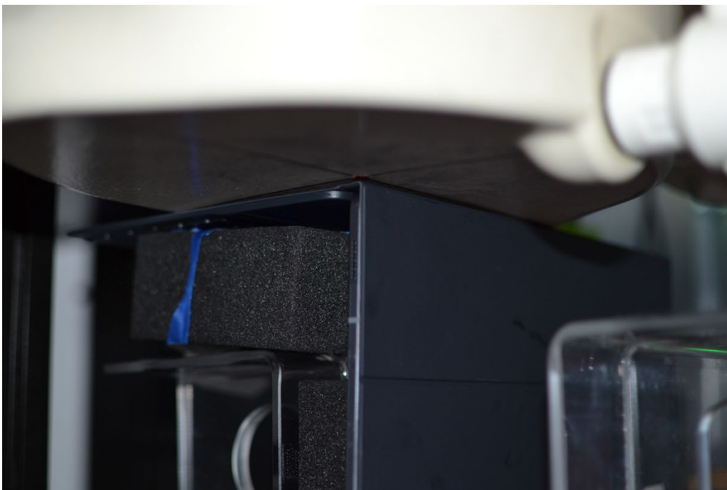
SAR Test Setup Photo 51 – Laptop with Keyboard Variant 2, Bottom Edge at 0 mm Antenna WIFI 1, 2, M1, or S3
