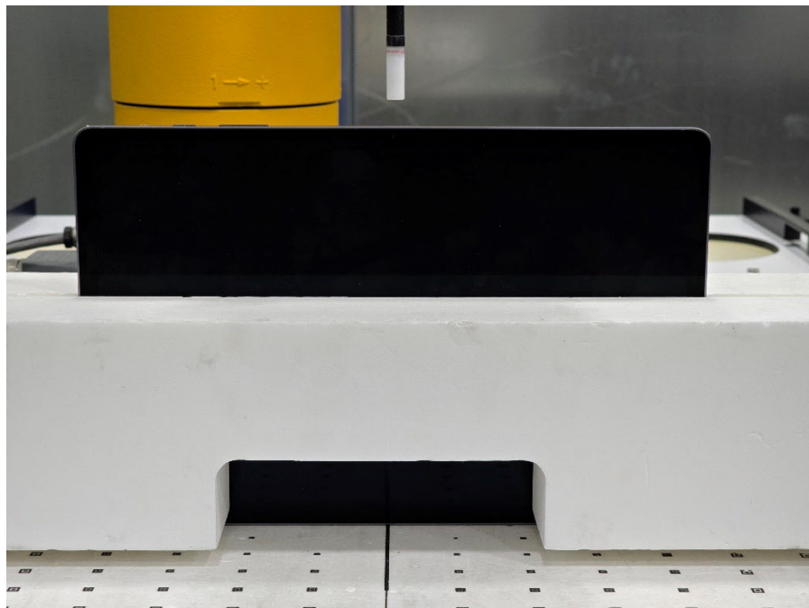
SAR Test Setup Photo 62 – Tablet, Right Edge at 8.54 mm
