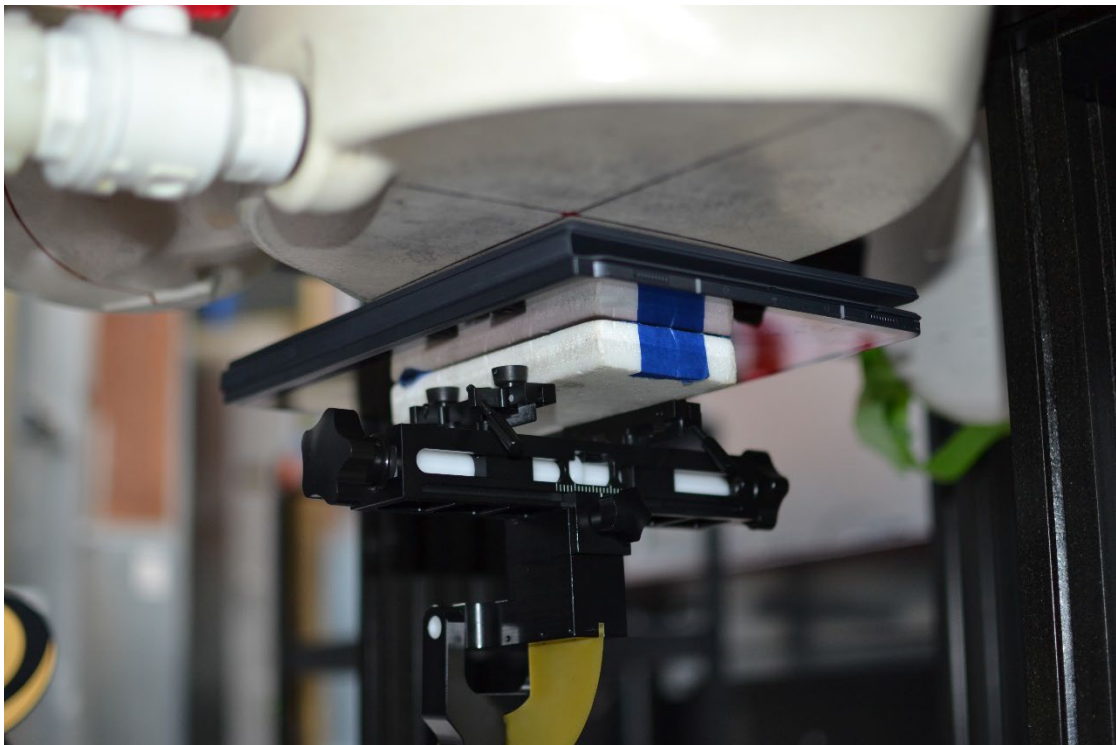
SAR Test Setup Photo 11 – Tablet with Keyboard Variant 1, Back Side at 0 mm – Antenna WIFI 1 or S3
