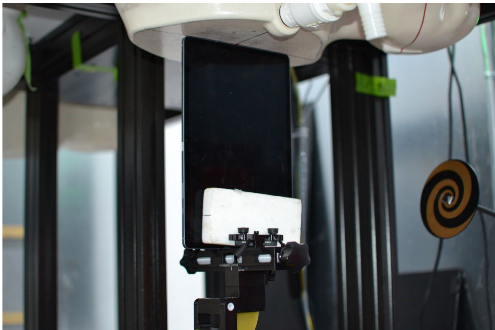
SAR Test Setup Photo 41 – Tablet, Bottom Edge at 0 mm
