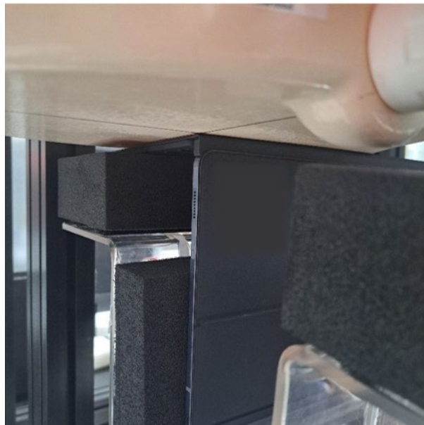
SAR Test Setup Photo 50 – Laptop with Keyboard Variant 1, Bottom Edge at 0 mm Antenna WIFI 1, 2, M1, or S3
