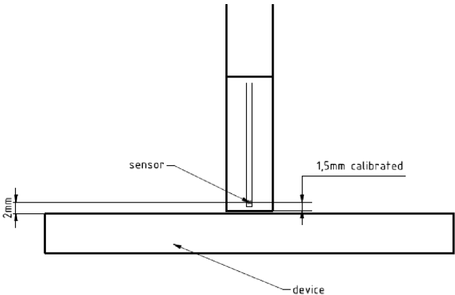
Figure K-1 EUmWVx Probe
