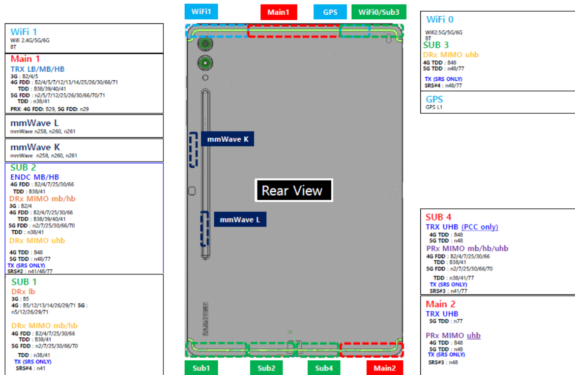
Figure K-1 DUT Antenna Locations
