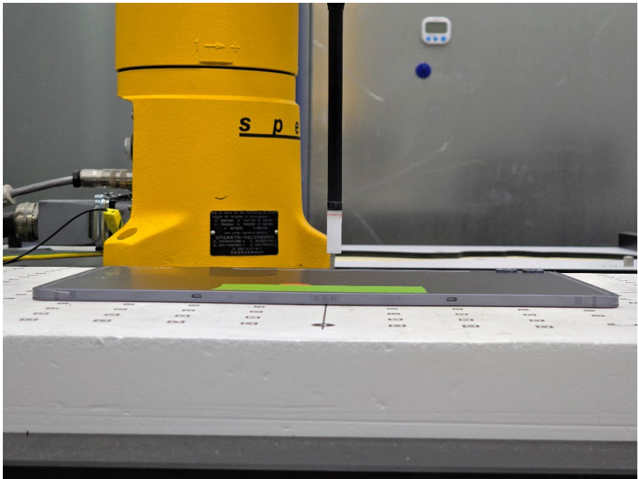
SAR Test Setup Photo 59 – Tablet, Back Side at 9.27 mm
