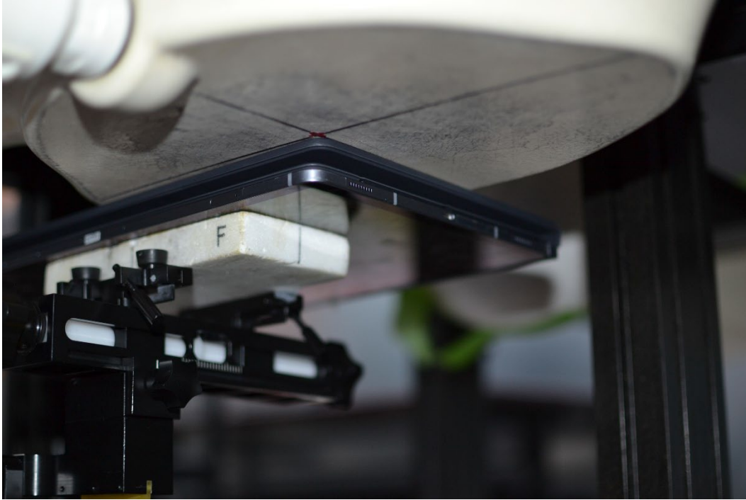
SAR Test Setup Photo 19 – Tablet with Keyboard Variant 1, Back Side at 0 mm – Antenna S1
