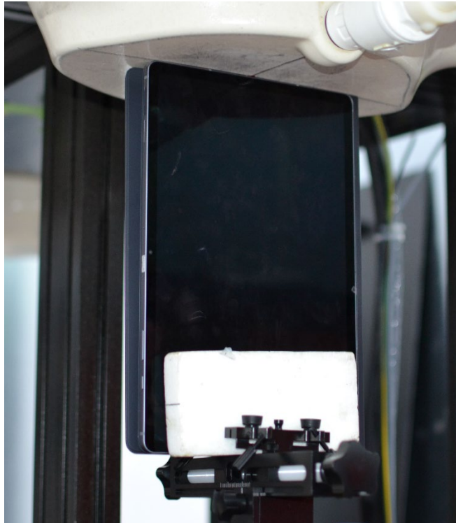
SAR Test Setup Photo 43 – Tablet with Keyboard Variant 2, Bottom Edge at 0 mm
