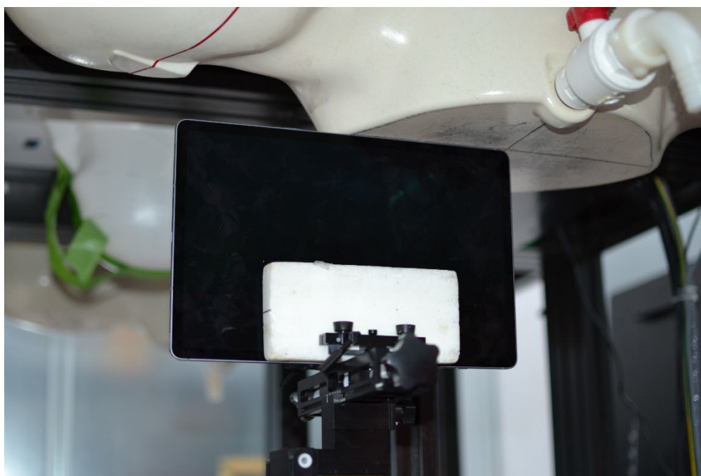
SAR Test Setup Photo 26 – Tablet, Left Edge at 0 mm – Antenna WIFI 1, 2, M1, or S3
