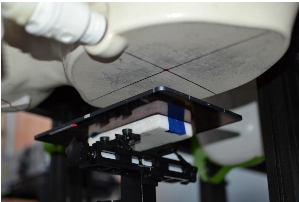
SAR Test Setup Photo 17 – Tablet, Back Side at 19 mm – Antenna S1
