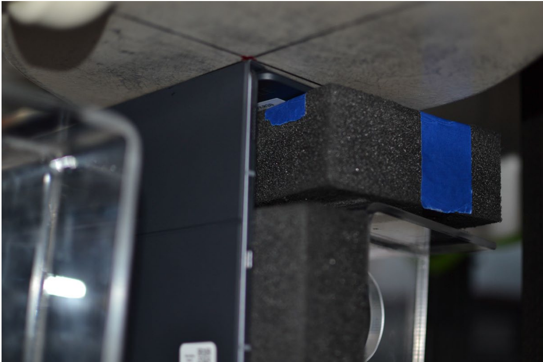
SAR Test Setup Photo 53 – Laptop with Keyboard Variant 2, Bottom Edge at 0 mm Antenna M2, S1, S2, or S4
