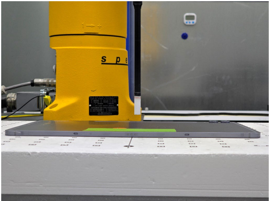
SAR Test Setup Photo 58 – Tablet, Back Side at 9.51 mm
