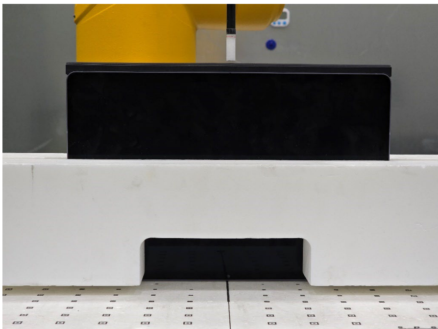
SAR Test Setup Photo 65 – Laptop with Keyboard Variant 1, Bottom Edge at 2 mm
