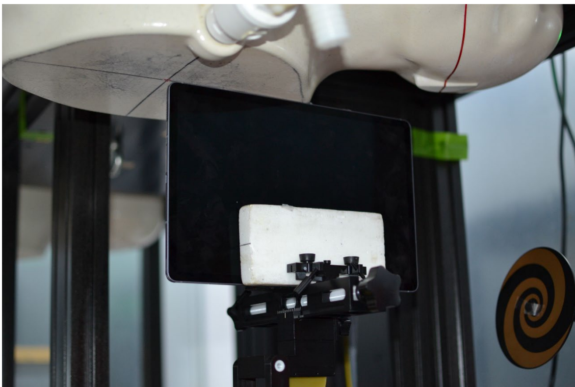
SAR Test Setup Photo 30 – Tablet, Left Edge at 0 mm – Antenna S1, S2, S4, or M2
