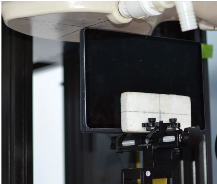
SAR Test Setup Photo 35 – Tablet with Keyboard Variant 1, Right Edge at 0 mm – Antenna WIFI 1, 2, M1, or S3
