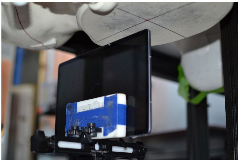
SAR Test Setup Photo 25 – Tablet, Left Edge at 15 mm – Antenna WIFI 1, 2, M1, or S3
