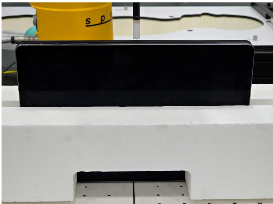
SAR Test Setup Photo 64 – Tablet with Keyboard Variant 2, Right Side at 2 mm
