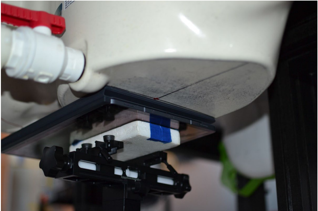
SAR Test Setup Photo 3 – Tablet with Keyboard Variant 1, Back Side at 0 mm – Antenna M1
