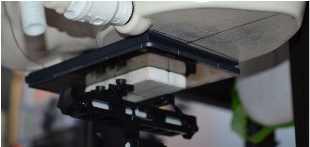
SAR Test Setup Photo 4 – Tablet with Keyboard Variant 2, Back Side at 0 mm – Antenna M1
