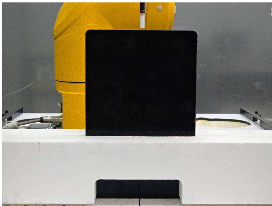
SAR Test Setup Photo 57 – Tablet, Top Edge at 2 mm
