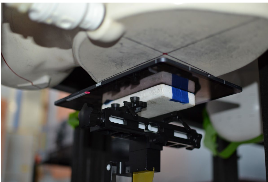
SAR Test Setup Photo 18 – Tablet, Back Side at 0 mm – Antenna S1
