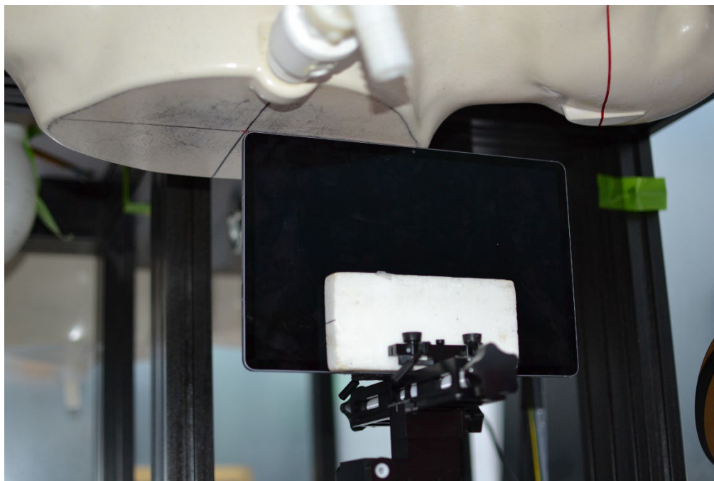
SAR Test Setup Photo 34 – Tablet, Right Edge at 0 mm – Antenna WIFI 1, 2, M1, or S3
