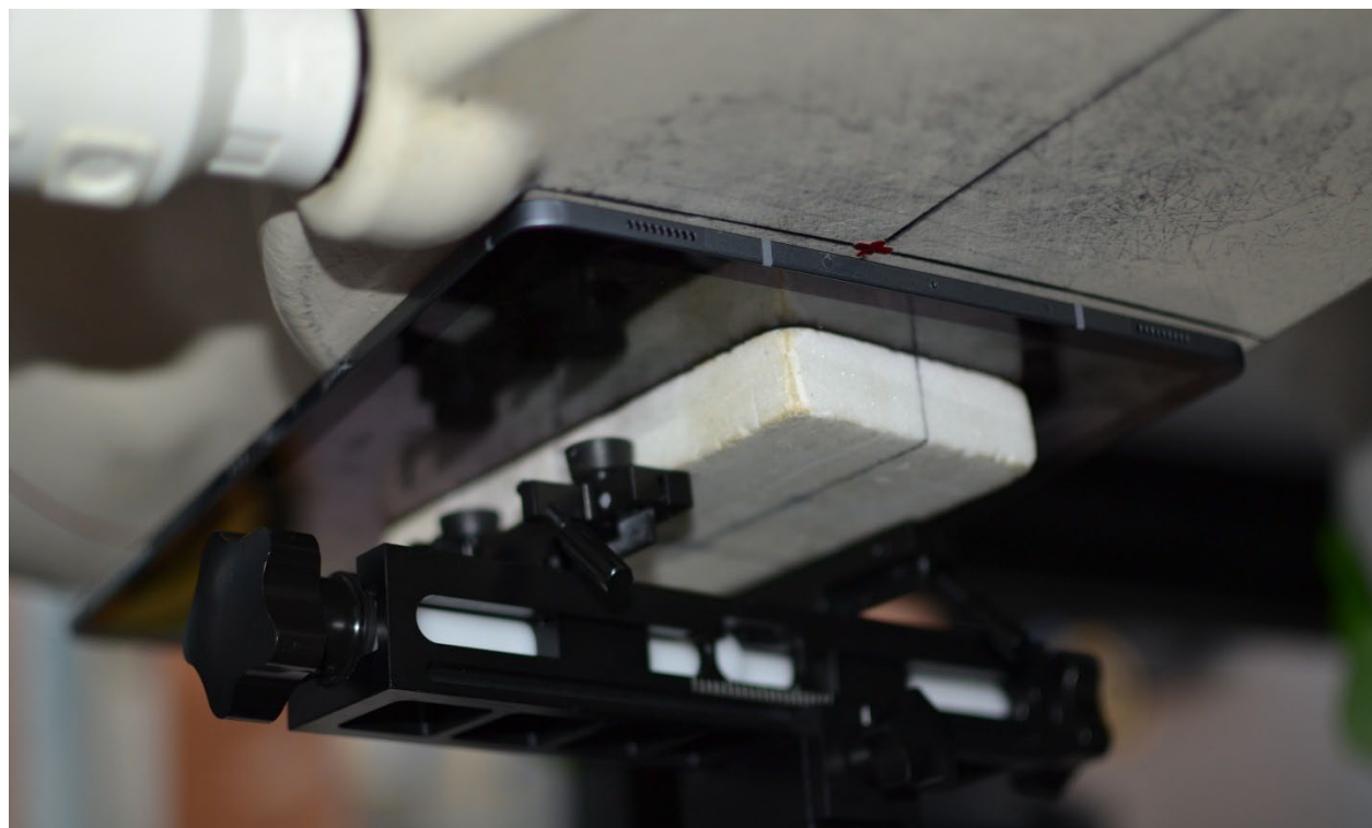
SAR Test Setup Photo 2 – Tablet, Back Side at 0 mm – Antenna M1
