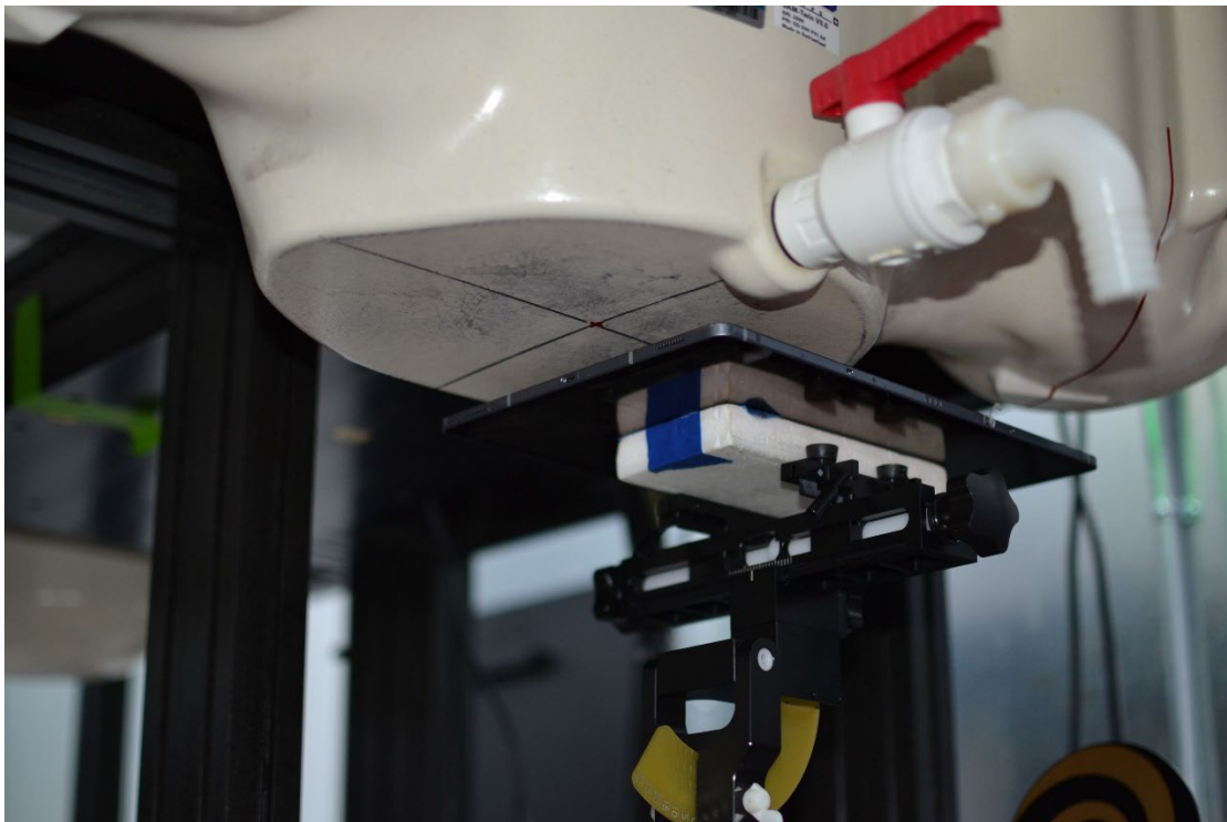
SAR Test Setup Photo 5 – Tablet, Back Side at 19 mm – Antenna M2
