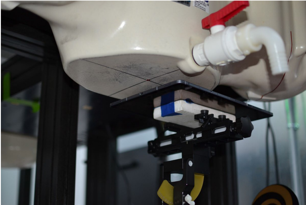
SAR Test Setup Photo 21 – Tablet, Back Side at 19 mm – Antenna S2 or S4
