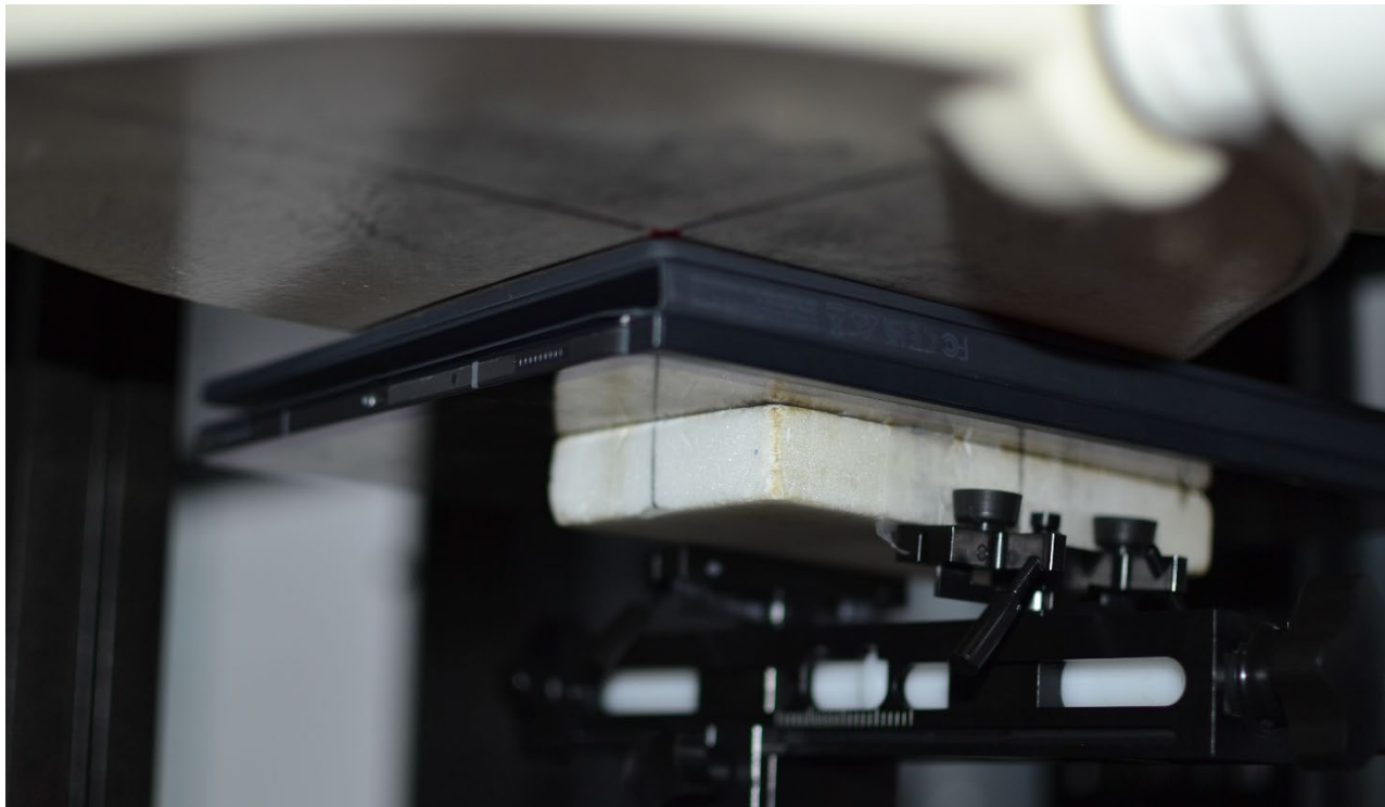
SAR Test Setup Photo 7 – Tablet with Keyboard Variant 1, Back Side at 0 mm – Antenna M2
