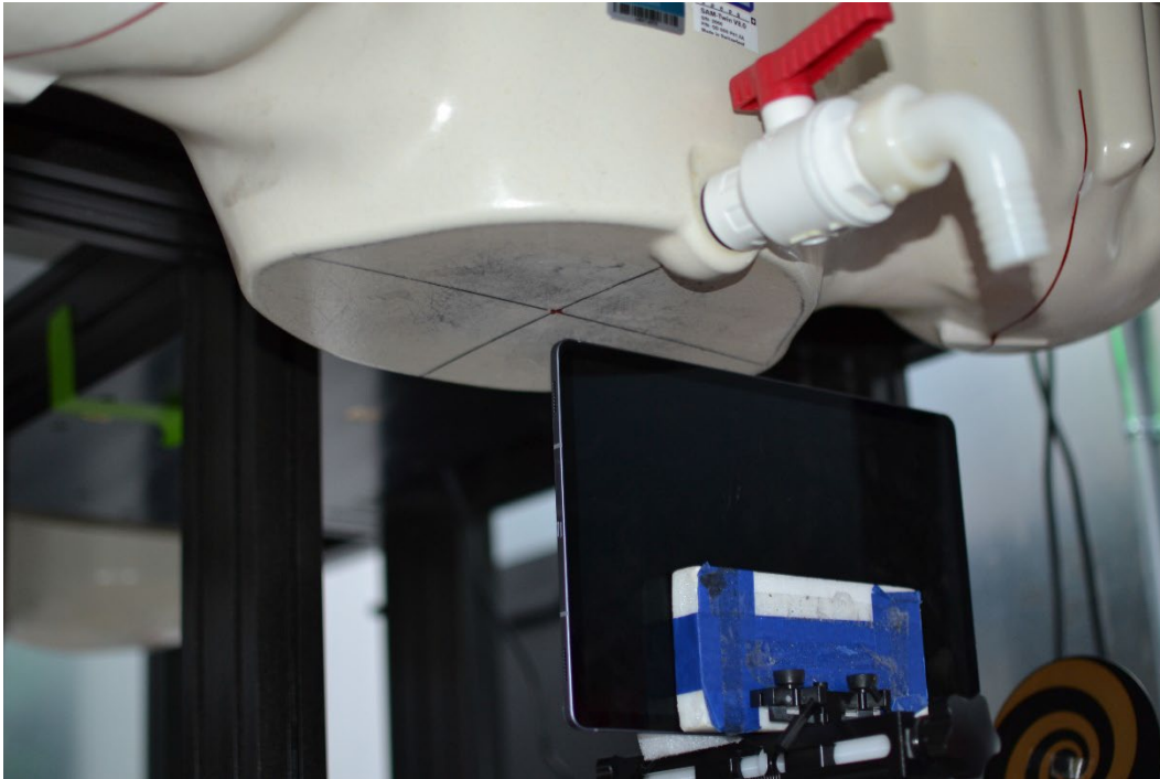
SAR Test Setup Photo 29 – Tablet, Left Edge at 15 mm – Antenna S1, S2, S4, or M2
