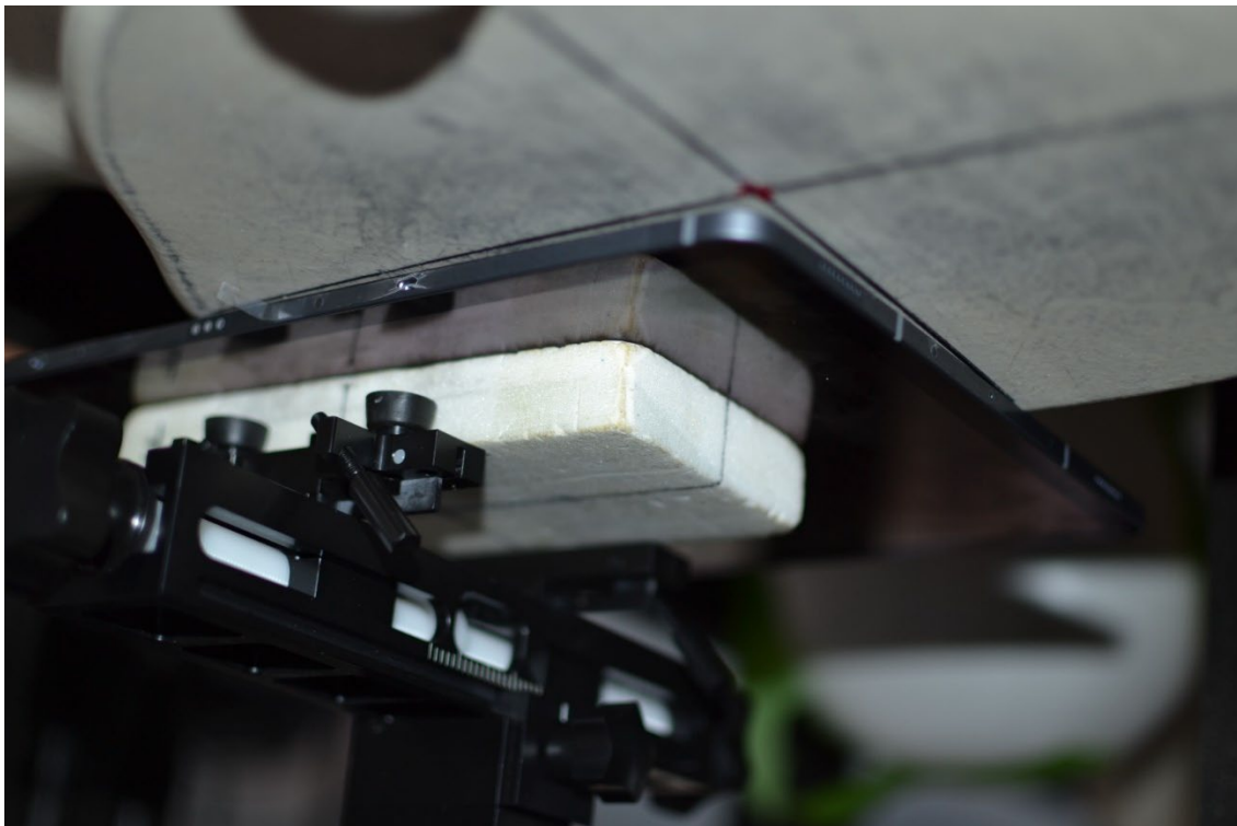
SAR Test Setup Photo 10 – Tablet, Back Side at 0 mm – Antenna WIFI 1 or S3
