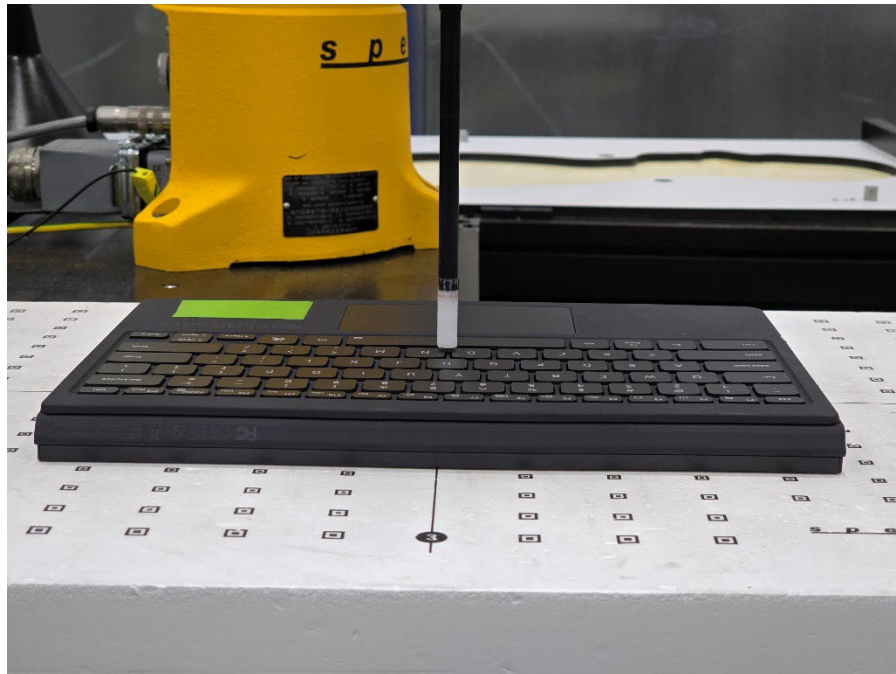
SAR Test Setup Photo 54 – Tablet with Keyboard Variant 1, Back Side at 2 mm
