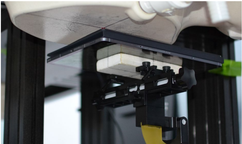
SAR Test Setup Photo 8 – Tablet with Keyboard Variant 2, Back Side at 0 mm – Antenna M2
