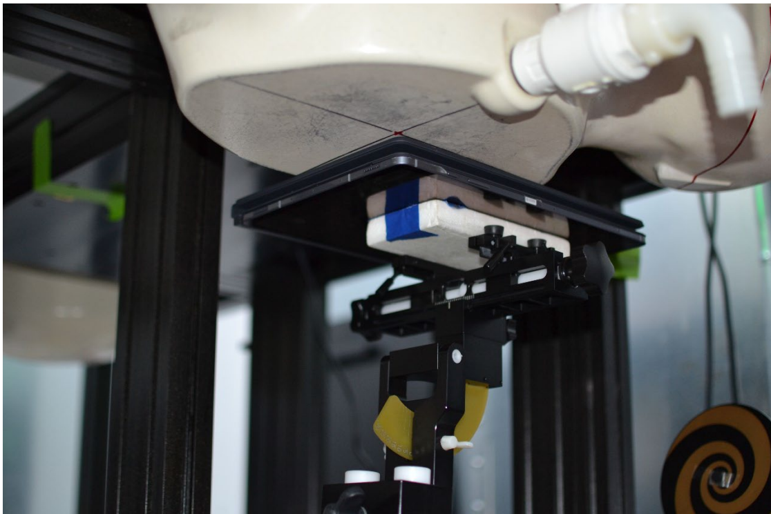
SAR Test Setup Photo 15 – Tablet with Keyboard Variant 1, Back Side at 0 mm – Antenna WIFI 2
