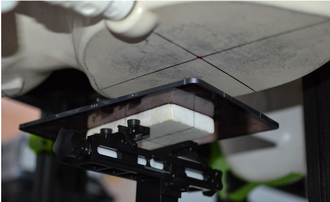
SAR Test Setup Photo 9 – Tablet, Back Side at 19 mm – Antenna WIFI 1 or S3
