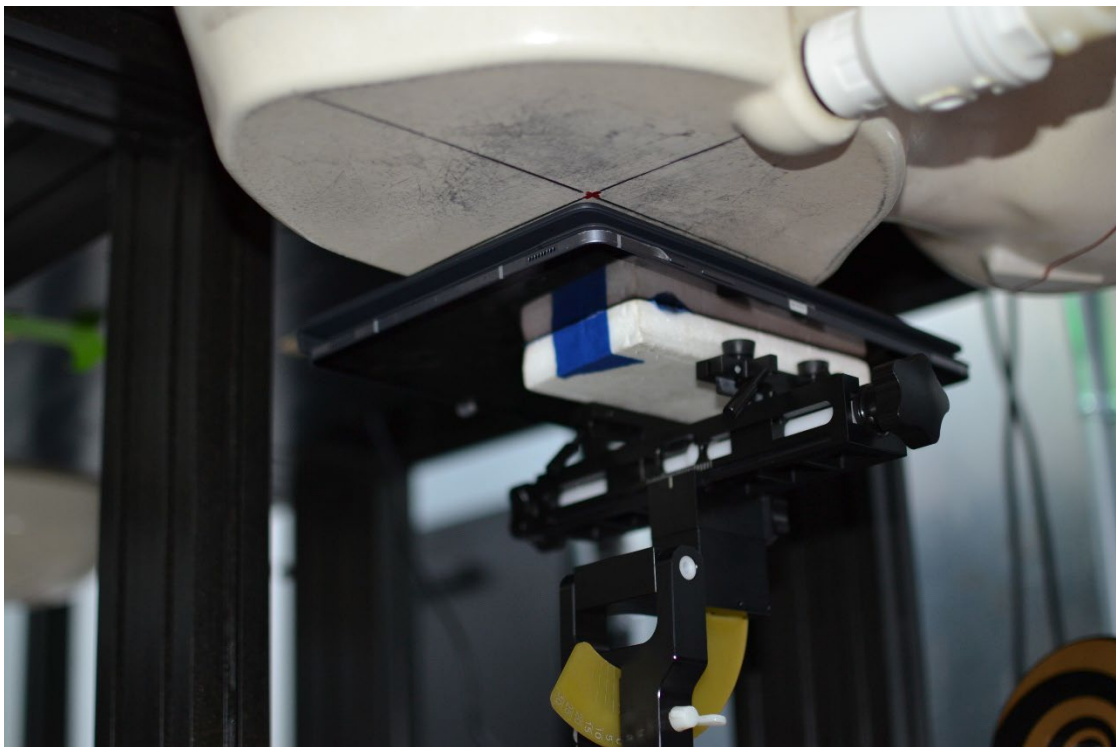
SAR Test Setup Photo 16 – Tablet with Keyboard Variant 2, Back Side at 0 mm – Antenna WIFI 2
