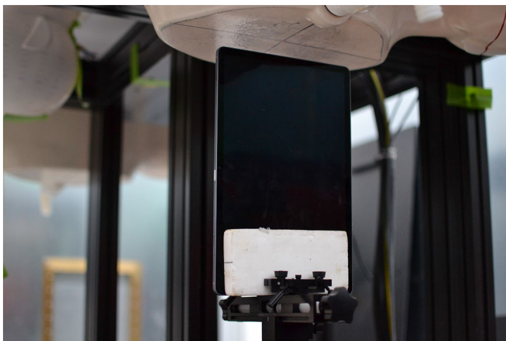
SAR Test Setup Photo 40 – Tablet, Bottom Edge at 19 mm
