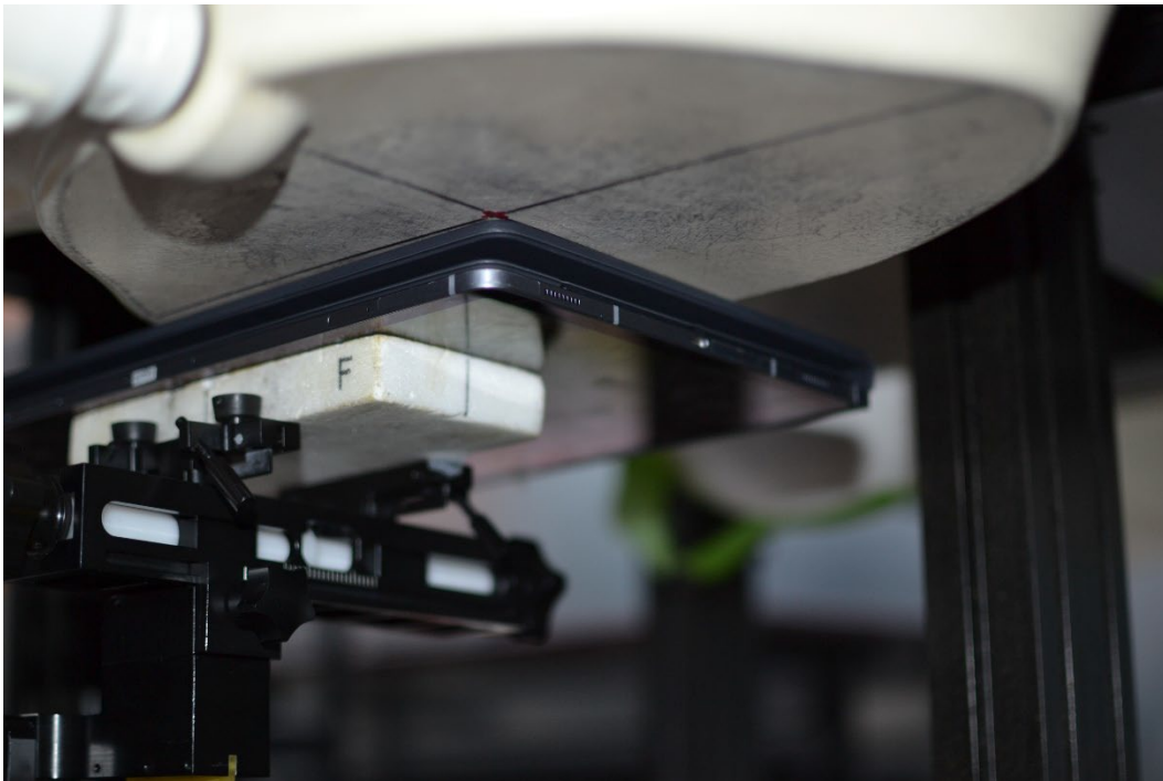
SAR Test Setup Photo 20 – Tablet with Keyboard Variant 2, Back Side at 0 mm – Antenna S1
