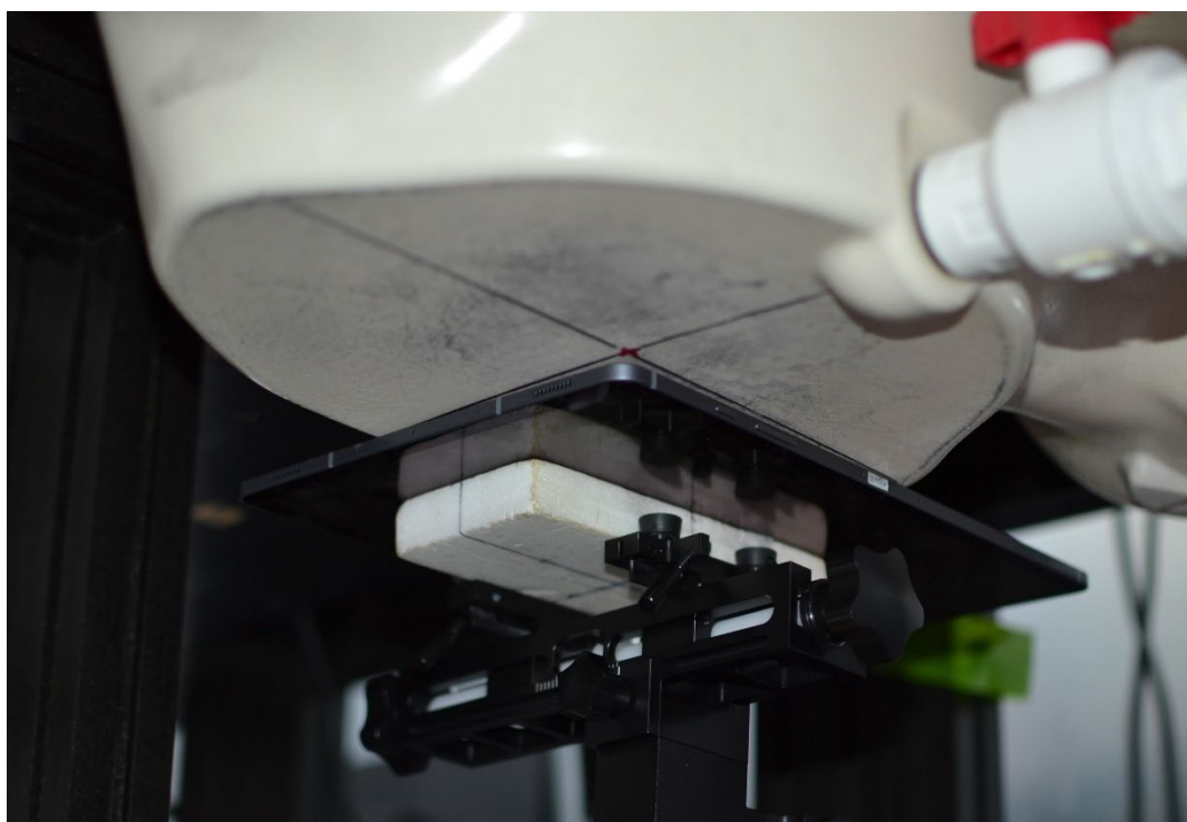
SAR Test Setup Photo 14 – Tablet, Back Side at 0 mm – Antenna WIFI 2
