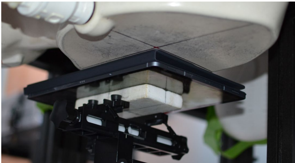
SAR Test Setup Photo 12 – Tablet with Keyboard Variant 2, Back Side at 0 mm – Antenna WIFI 1 or S3
