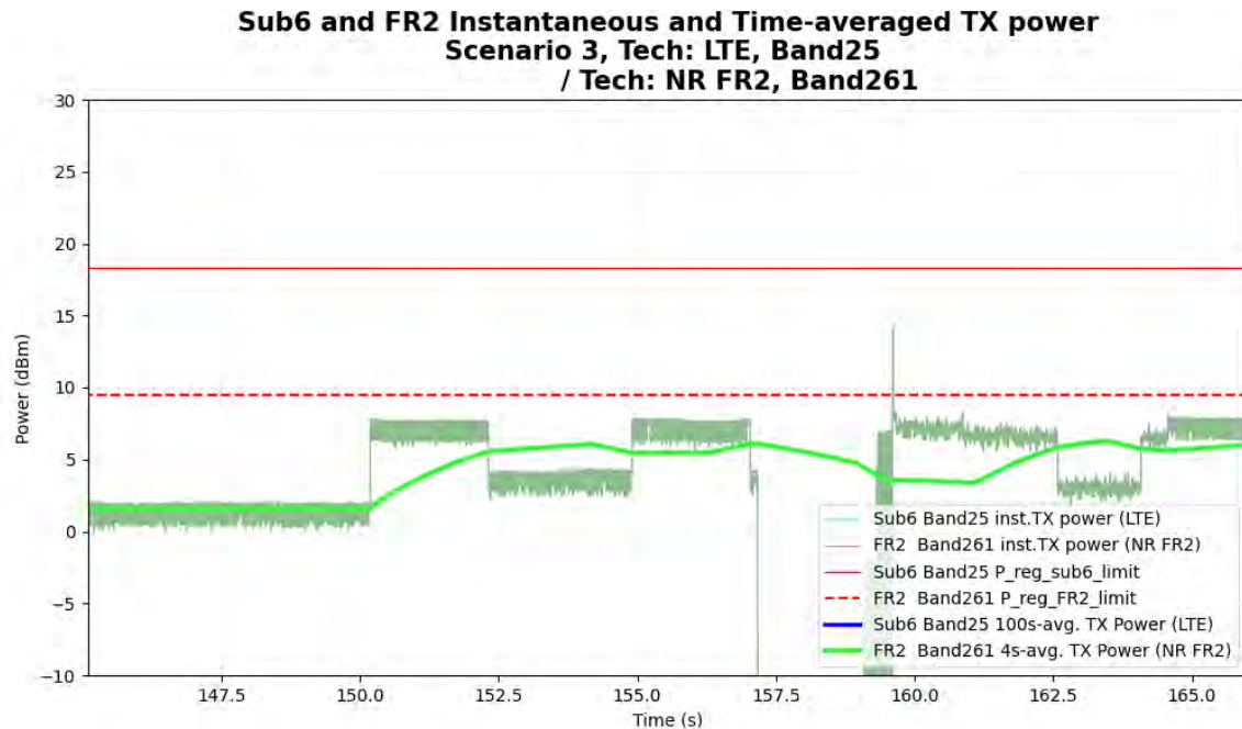
Figure 6-12 LTE, mmW inst. Pwr and Time-averaged Tx Pwr (case 3.1)
