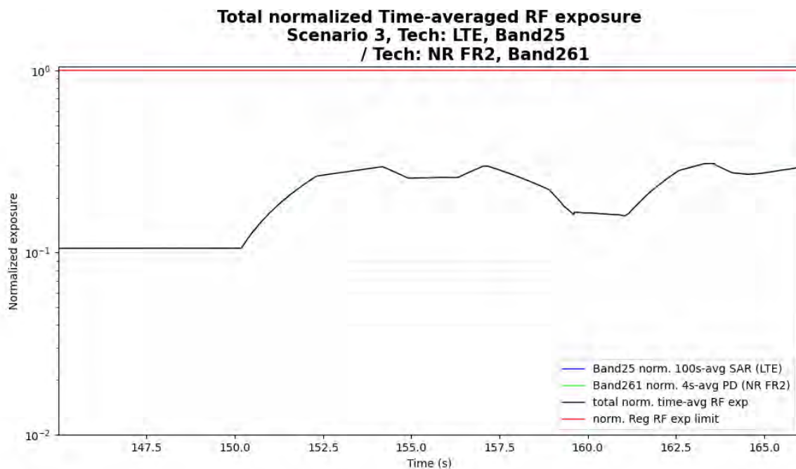
Figure 6-13 Total Normalized Time-averaged RF exposure (case 3.1)
