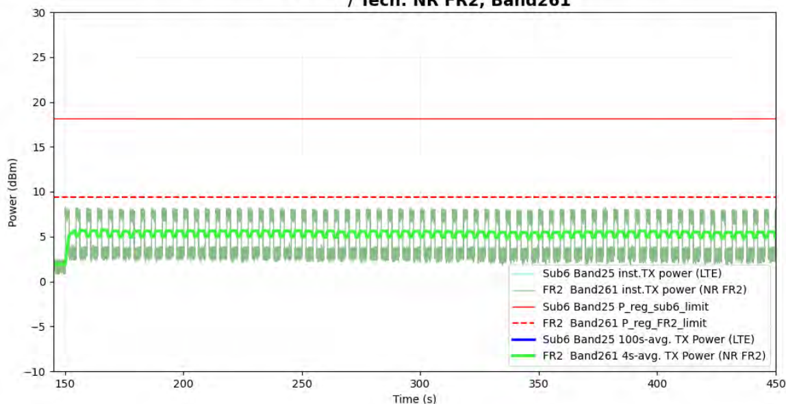
Figure 6-4 LTE, mmW inst. Pwr and Time-averaged Tx Pwr (case 1.1) Total normalized Time-averaged RF exposure Scenario 1, Tech: LTE, Band25 / Tech: NR FR2, Band261
