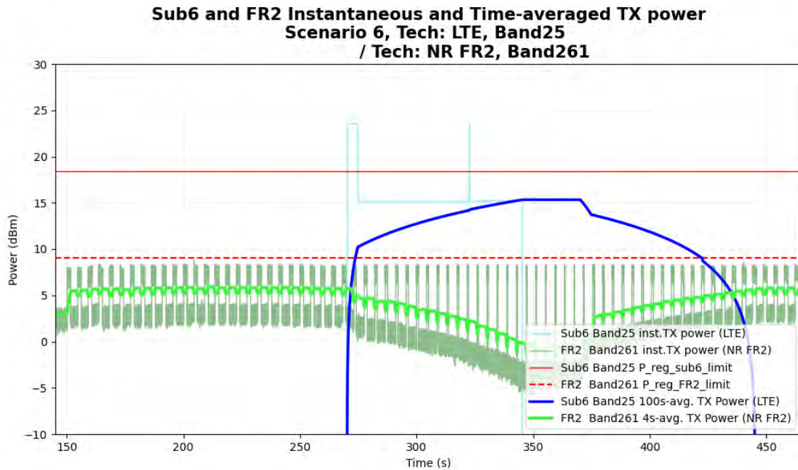
Figure 6-18 LTE, mmW inst. Pwr and Time-averaged Tx Pwr (case 6.1)
