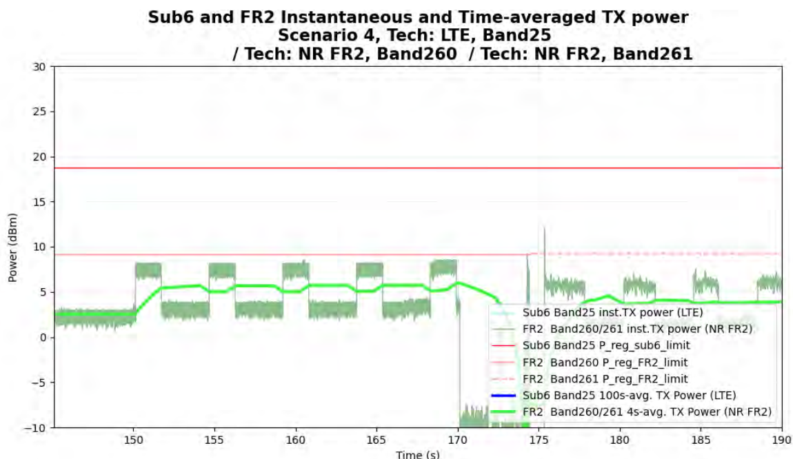
Figure 6-14 LTE, mmW inst. Pwr and Time-averaged Tx Pwr (case 4.1)
