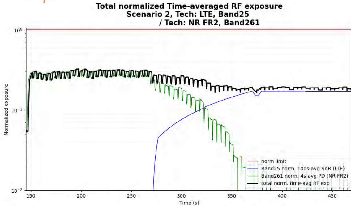
Figure 7-4 The Total Normalized Time-averaged RF exposure (n261)
