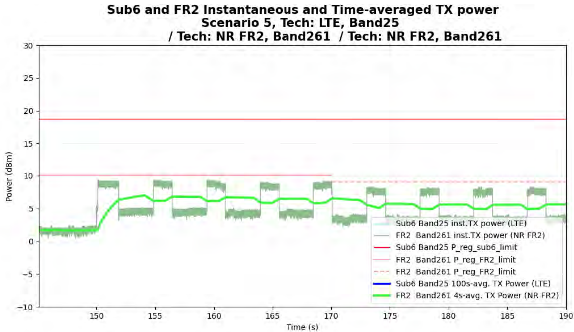
Figure 6-16 LTE, mmW inst. Pwr and Time-averaged Tx Pwr (case 5.1)
