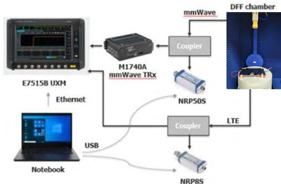
Figure 6-2 TA-PD radiated power measurement setup
