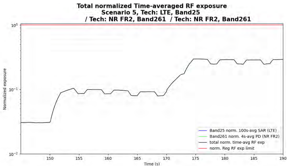
Figure 6-17 Total Normalized Time-averaged RF exposure (case 5.1)
