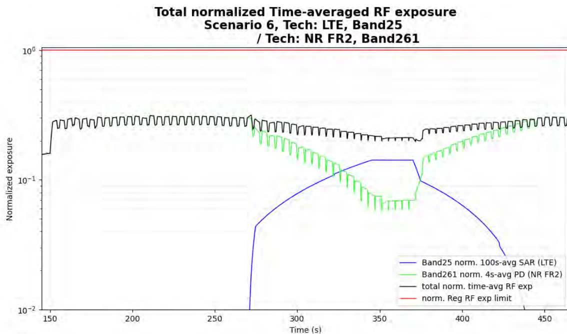
Figure 6-19 Total Normalized Time-averaged RF exposure (case 6.1)
