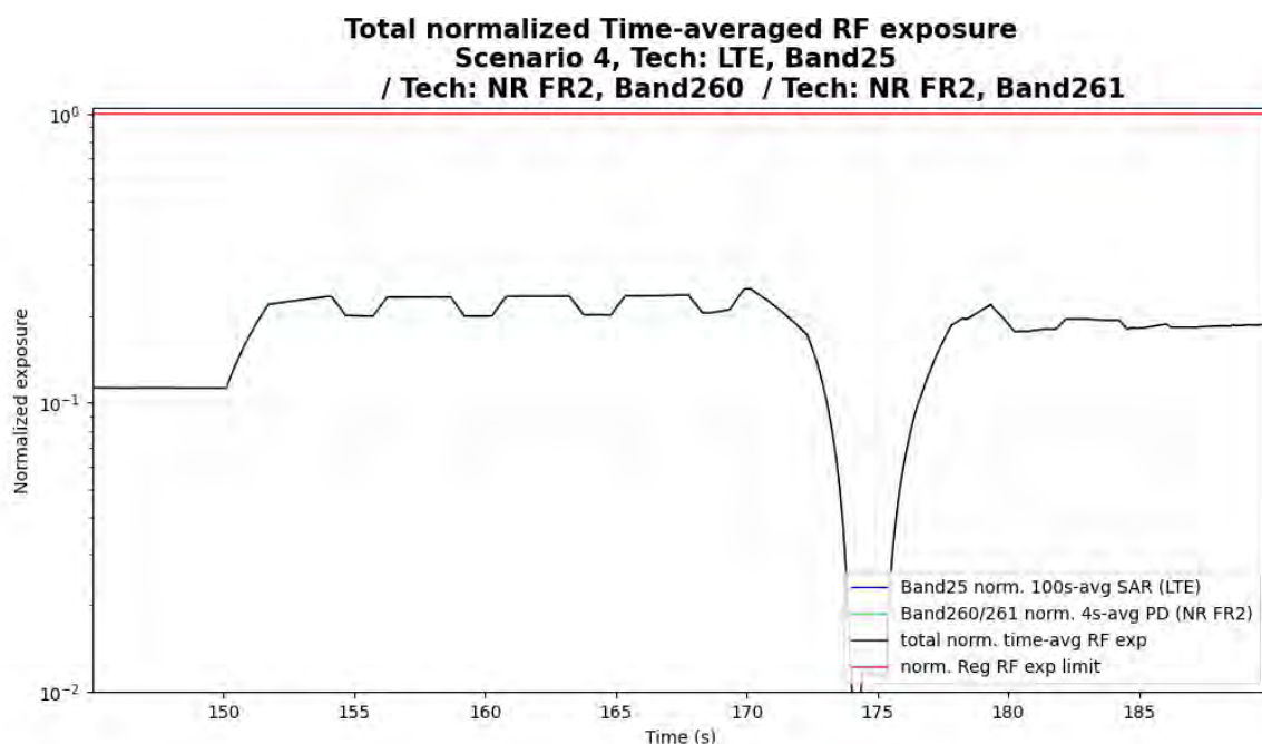
Figure 6-15 Total Normalized Time-averaged RF exposure (case 4.1)
