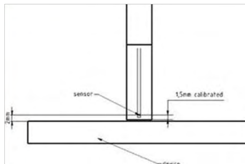
Figure C-1 EUmmWV3 Probe
