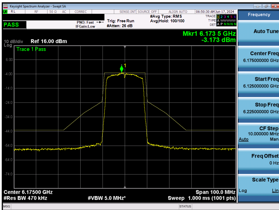
Plot 7-101. In-Band Emission MIMO ANT2 (20MHz 802.11a (UNII Band 5) – Ch. 45)
