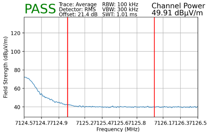
Plot 7-166. Radiated Upper Band Edge Plot SISO ANT2 (Average – UNII Band 8)
