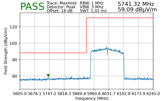
Plot 7-177. Radiated Lower Band Edge Plot SISO ANT2 (Peak – UNII Band 5)
