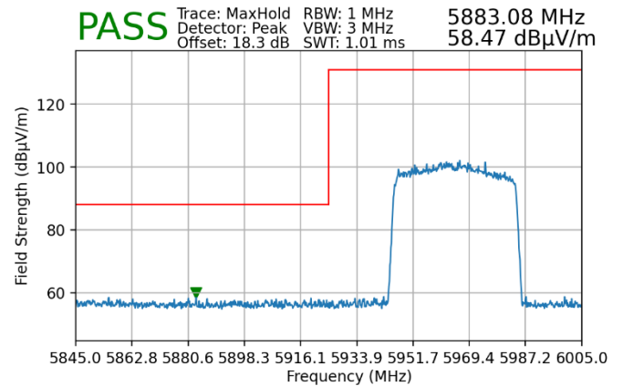
Plot 7-153. Radiated Lower Band Edge Plot SISO ANT1 (Peak – UNII Band 5)
