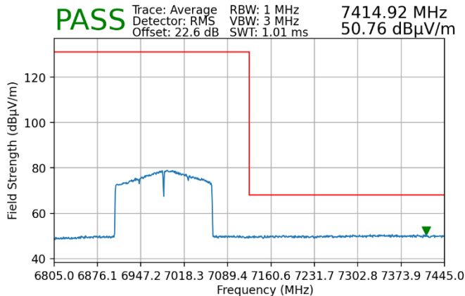
Plot 7-178. Radiated Upper Band Edge Plot SISO ANT2 (Average – UNII Band 8)
