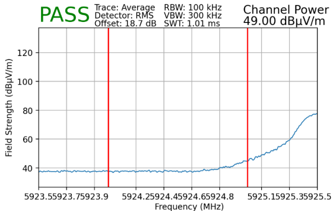
Plot 7-148. Radiated Lower Band Edge Plot SISO ANT1 (Average – UNII Band 5)
