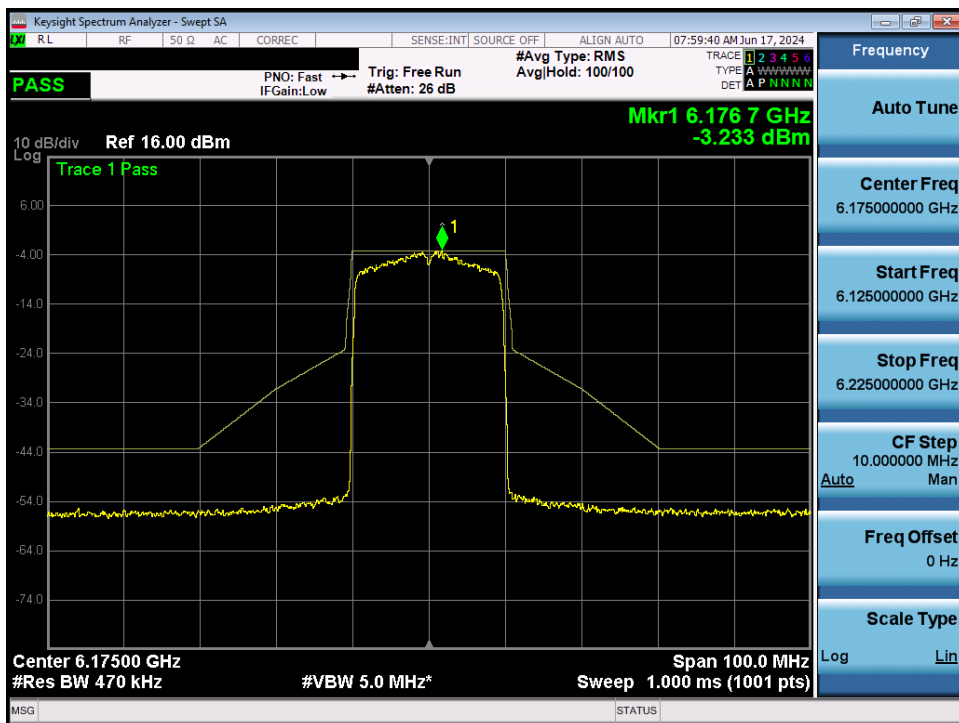
Plot 7-102. In-Band Emission MIMO ANT2 (20MHz 802.11ax (UNII Band 5) – Ch. 45)
