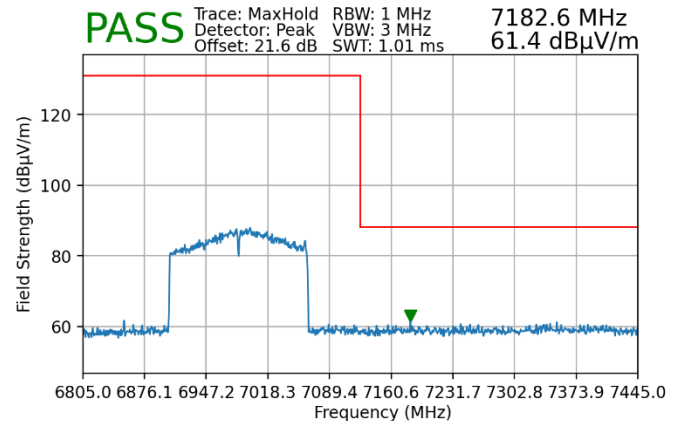
Plot 7-179. Radiated Upper Band Edge Plot SISO ANT2 (Peak – UNII Band 8)
