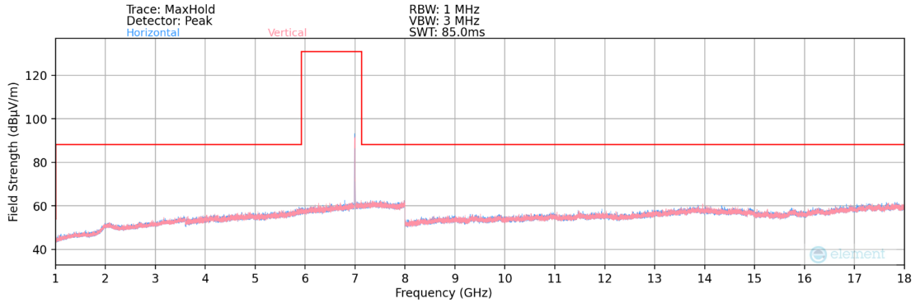
Plot 7-145. Radiated Spurious Plot 1GHz – 18GHz MIMO (802.11a – U Band 8 Ch. 209 – LPI)
