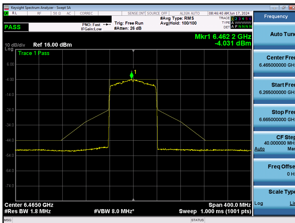
Plot 7-109. In-Band Emission MIMO ANT2 (80MHz 802.11ax (UNII Band 6) – Ch. 103)
