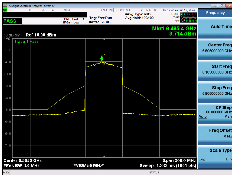
Plot 7-110. In-Band Emission MIMO ANT2 (160MHz 802.11ax (UNII Band 6) – Ch. 111)
