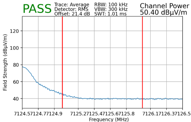
Plot 7-150. Radiated Upper Band Edge Plot SISO ANT1 (Average – UNII Band 8)
