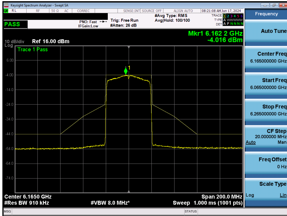
Plot 7-103. In-Band Emission MIMO ANT2 (40MHz 802.11ax (UNII Band 5) – Ch. 43)
