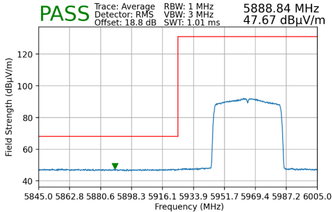
Plot 7-168. Radiated Lower Band Edge Plot SISO ANT2 (Average – UNII Band 5)
