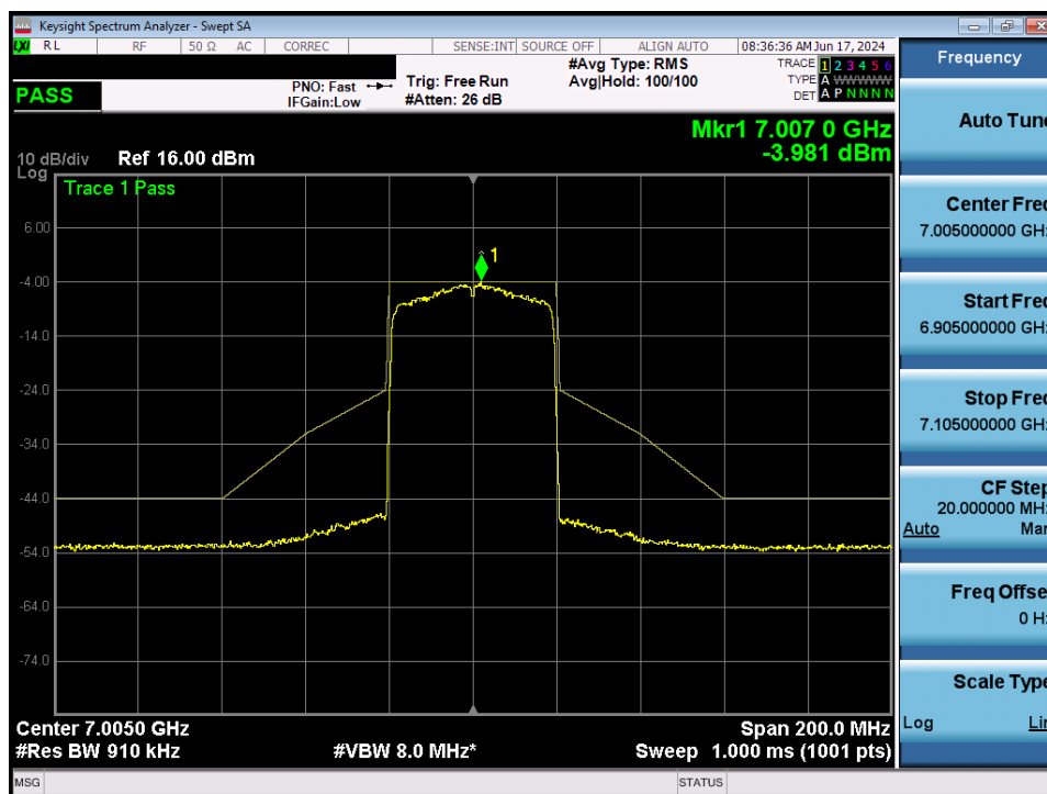
Plot 7-118. In-Band Emission MIMO ANT2 (40MHz 802.11ax (UNII Band 8) – Ch. 211)
