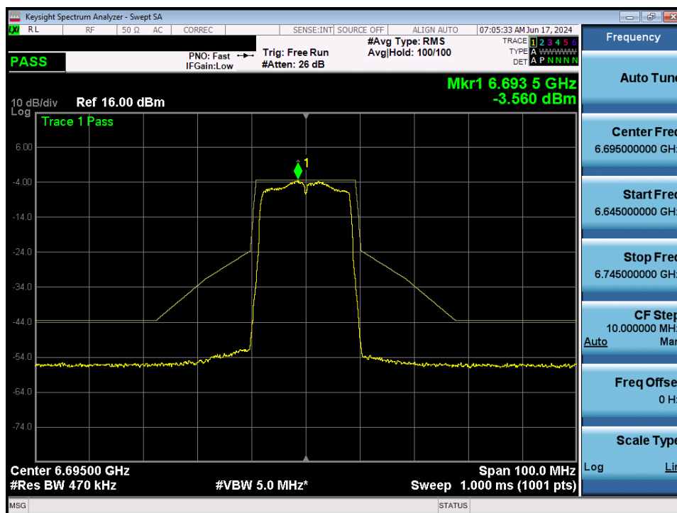
Plot 7-111. In-Band Emission MIMO ANT2 (20MHz 802.11a (UNII Band 7) – Ch. 149)
