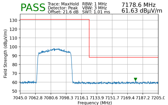
Plot 7-155. Radiated Upper Band Edge Plot SISO ANT1 (Peak – UNII Band 8)
