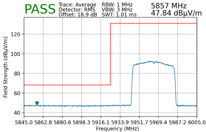
Plot 7-152. Radiated Lower Band Edge Plot SISO ANT1 (Average – UNII Band 5)
