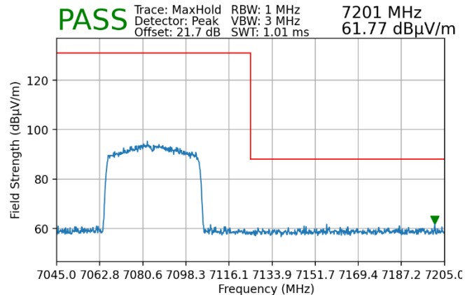
Plot 7-171. Radiated Upper Band Edge Plot SISO ANT2 (Peak – UNII Band 8)
