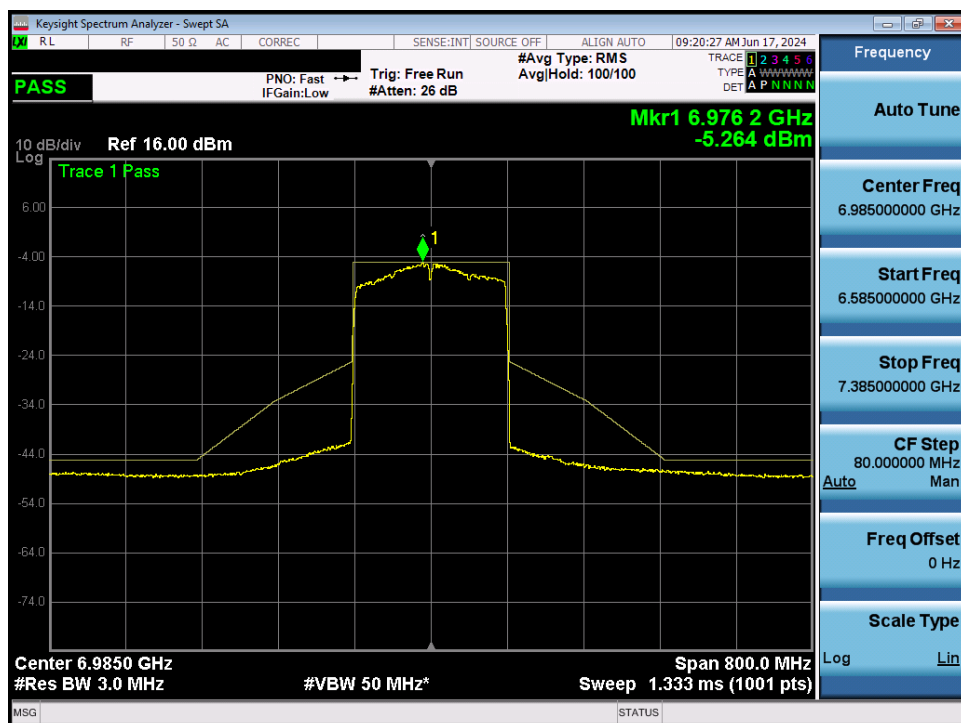
Plot 7-120. In-Band Emission MIMO ANT2 (160MHz 802.11ax (UNII Band 8) – Ch. 207)
