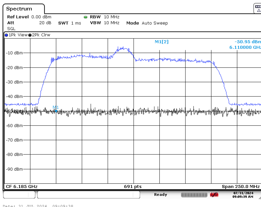
Plot 7-138. CBP 160MHz Channel - Injection Lower Edge – [6110 MHz]
