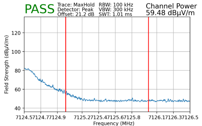
Plot 7-151. Radiated Upper Band Edge Plot SISO ANT1 (Peak – UNII Band 8)
