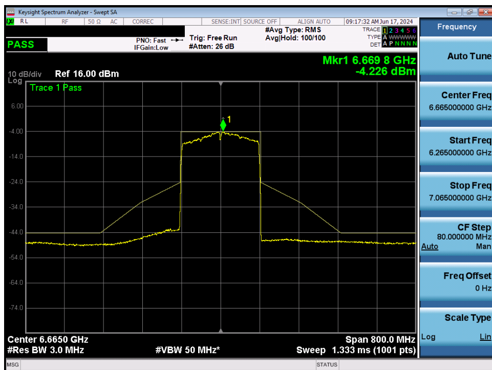
Plot 7-115. In-Band Emission MIMO ANT2 (160MHz 802.11ax (UNII Band 7) – Ch. 143)
