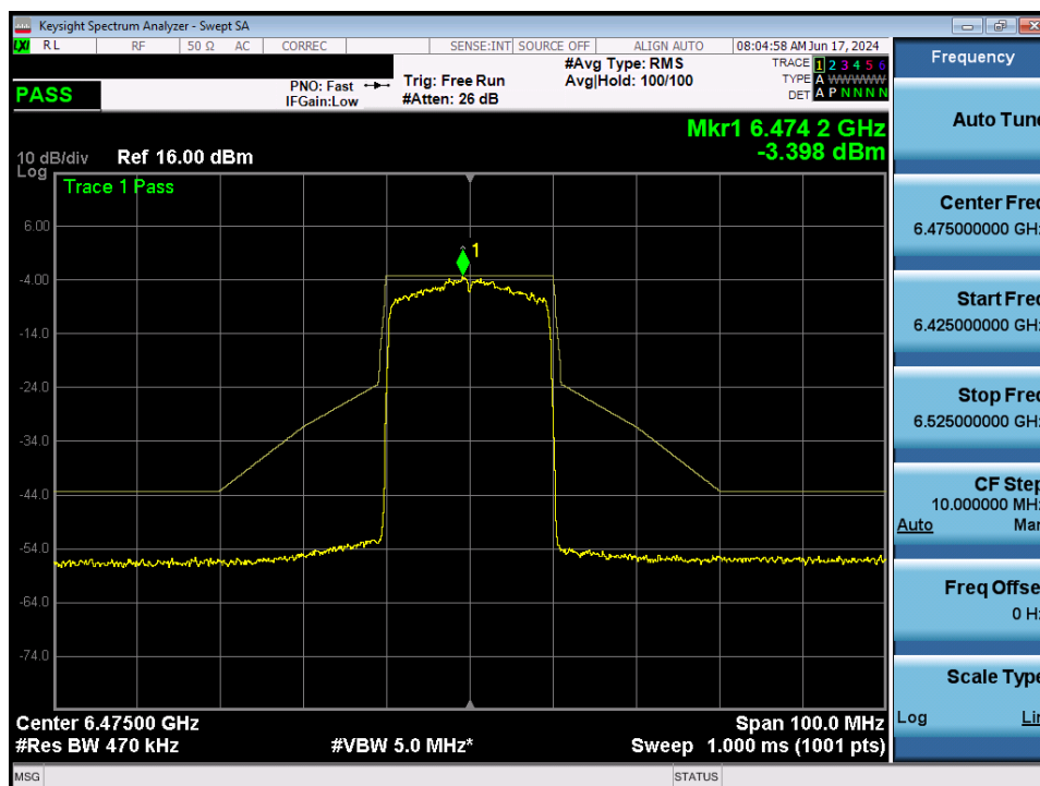
Plot 7-107. In-Band Emission MIMO ANT2 (20MHz 802.11ax (UNII Band 6) – Ch. 105)
