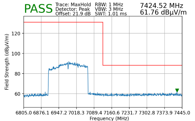
Plot 7-163. Radiated Upper Band Edge Plot SISO ANT1 (Peak – UNII Band 8)
