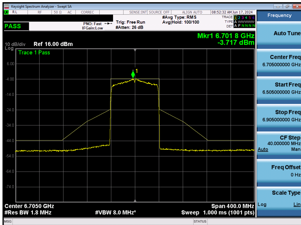
Plot 7-114. In-Band Emission MIMO ANT2 (80MHz 802.11ax (UNII Band 7) – Ch. 151)
