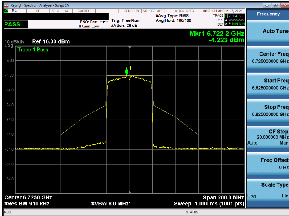
Plot 7-113. In-Band Emission MIMO ANT2 (40MHz 802.11ax (UNII Band 7) – Ch. 155)
