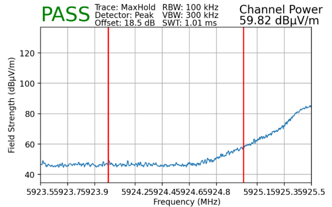
Plot 7-165. Radiated Lower Band Edge Plot SISO ANT2 (Peak – UNII Band 5)
