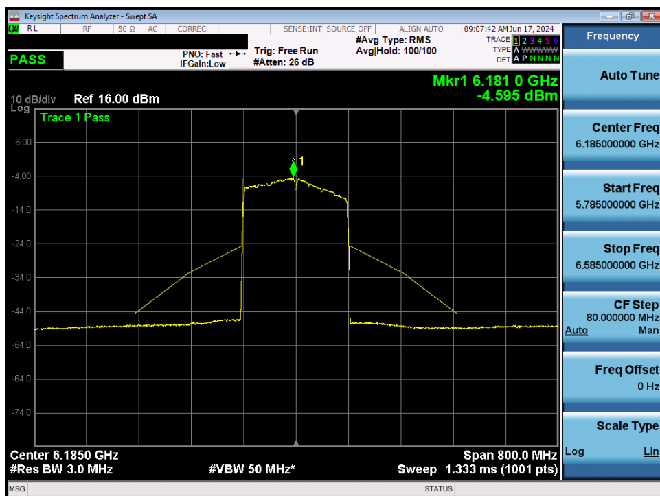
Plot 7-105. In-Band Emission MIMO ANT2 (160MHz 802.11ax (UNII Band 5) – Ch. 47)
