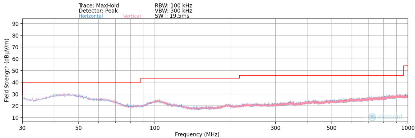
Plot 7-141. Radiated Spurious Plot below 1GHz MIMO (802.11a)
