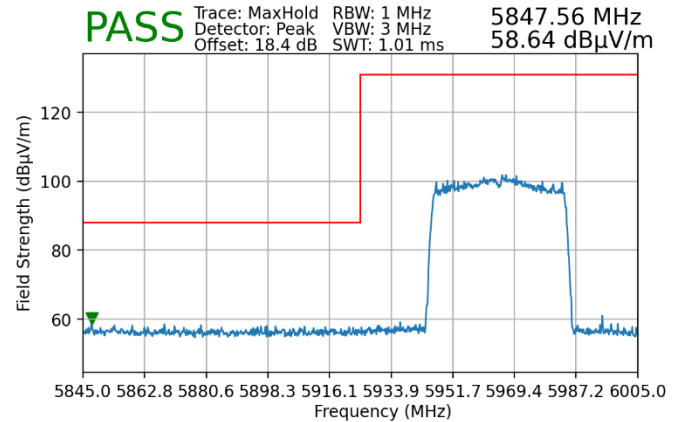
Plot 7-169. Radiated Lower Band Edge Plot SISO ANT2 (Peak – UNII Band 5)
