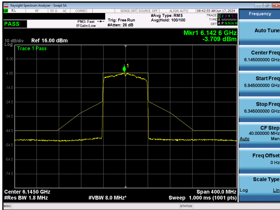
Plot 7-104. In-Band Emission MIMO ANT2 (80MHz 802.11ax (UNII Band 5) – Ch. 39)
