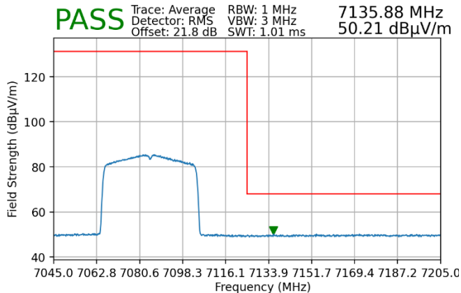
Plot 7-170. Radiated Upper Band Edge Plot SISO ANT2 (Average – UNII Band 8)
