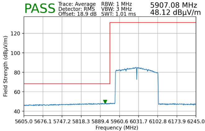
Plot 7-176. Radiated Lower Band Edge Plot SISO ANT2 (Average – UNII Band 5)
