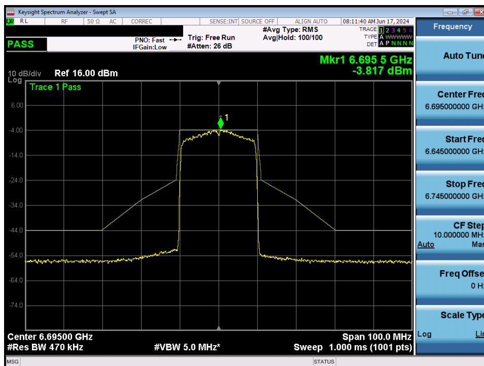
Plot 7-112. In-Band Emission MIMO ANT2 (20MHz 802.11ax (UNII Band 7) – Ch. 149)
