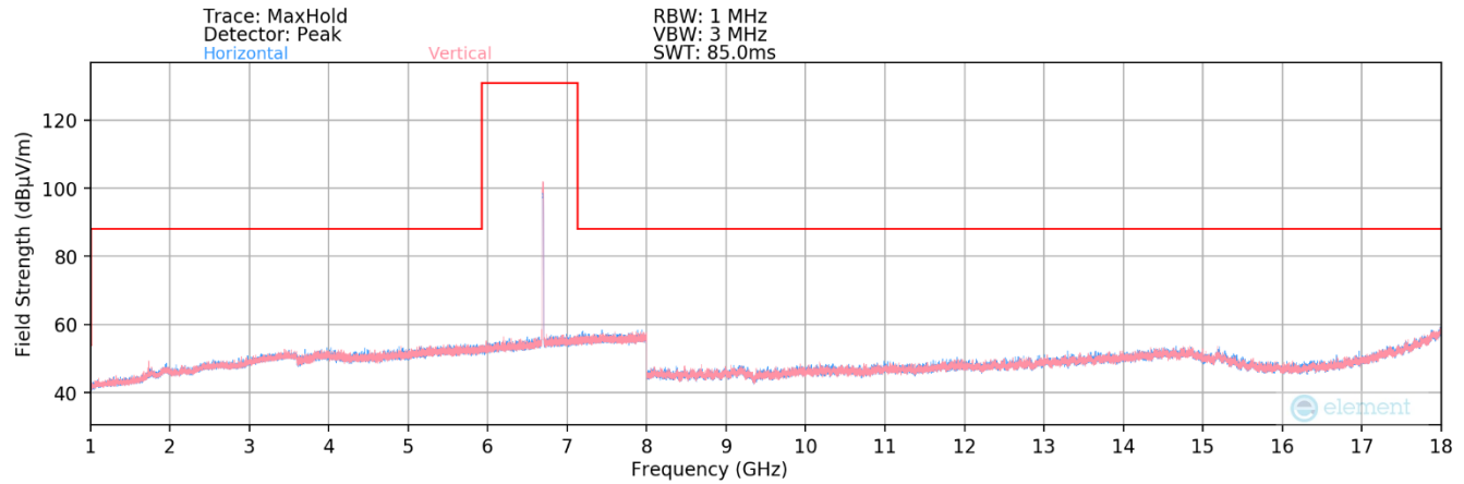
Plot 7-143. Radiated Spurious Plot 1GHz – 18GHz MIMO (802.11a – UNII Band 6 Ch. 105 – LPI)
