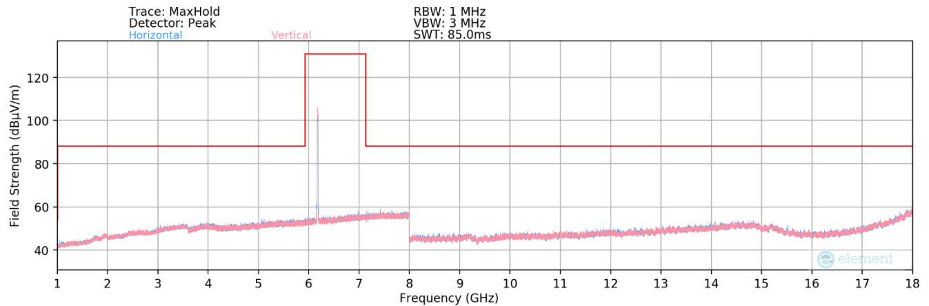
Plot 7-142. Radiated Spurious Plot 1GHz – 18GHz MIMO (802.11a – UNII Band 5 Ch. 45 – LPI/SP)
