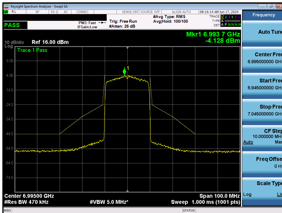
Plot 7-117. In-Band Emission MIMO ANT2 (20MHz 802.11ax (UNII Band 8) – Ch. 209)
