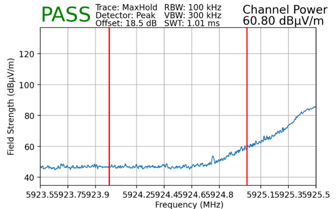
Plot 7-149. Radiated Lower Band Edge Plot SISO ANT1 (Peak – UNII Band 5)
