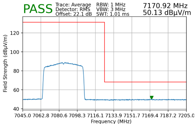
Plot 7-154. Radiated Upper Band Edge Plot SISO ANT1 (Average – UNII Band 8)
