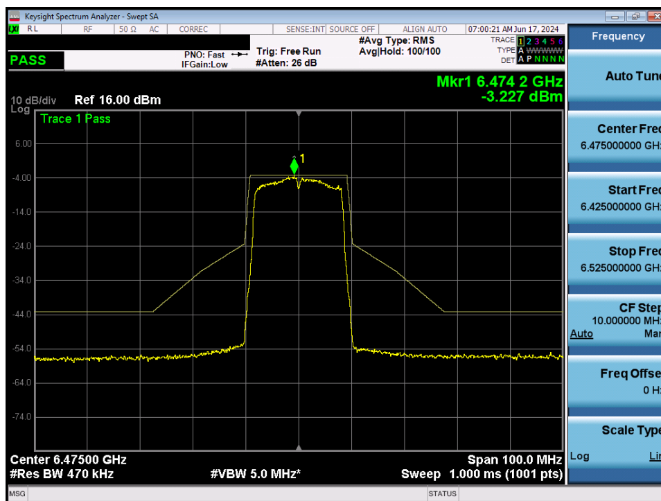
Plot 7-106. In-Band Emission MIMO ANT2 (20MHz 802.11a (UNII Band 6) – Ch. 105)
