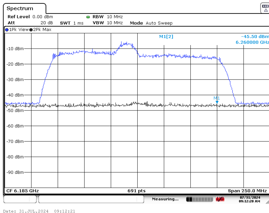
Plot 7-140. CBP 160MHz Channel - Injection Upper Edge – [6260 MHz]
