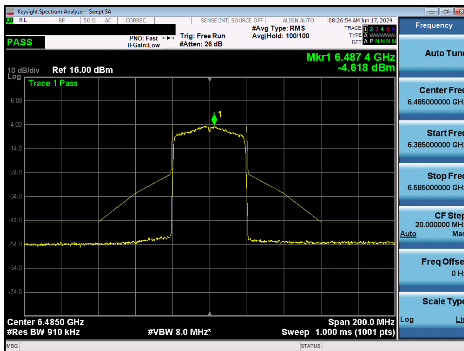
Plot 7-108. In-Band Emission MIMO ANT2 (40MHz 802.11ax (UNII Band 6) – Ch. 107)
