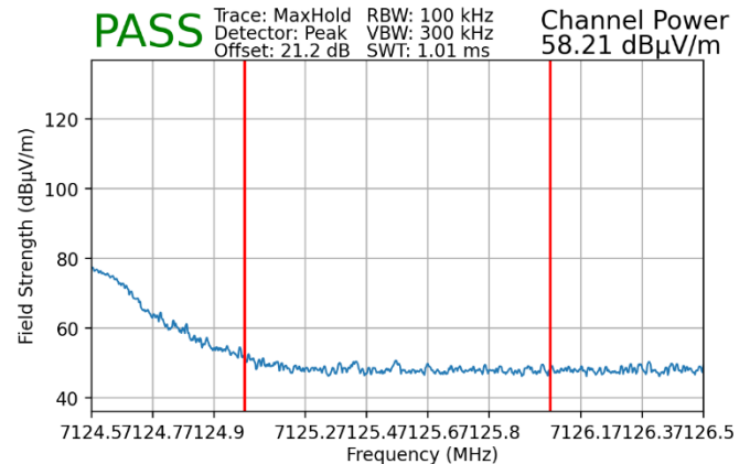
Plot 7-167. Radiated Upper Band Edge Plot SISO ANT2 (Peak – UNII Band 8)
