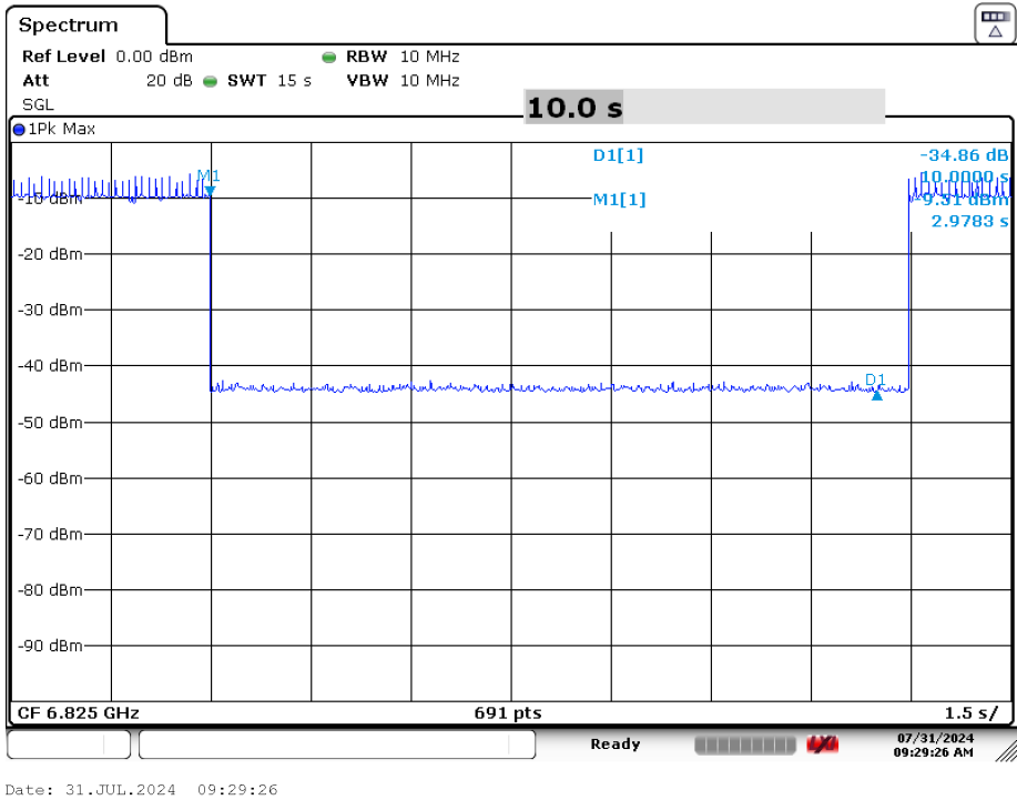
Plot 7-132. Contention Based Protocol Timing Plot (160MHz (UNII Band 7) – Ch. 175 Mid)
