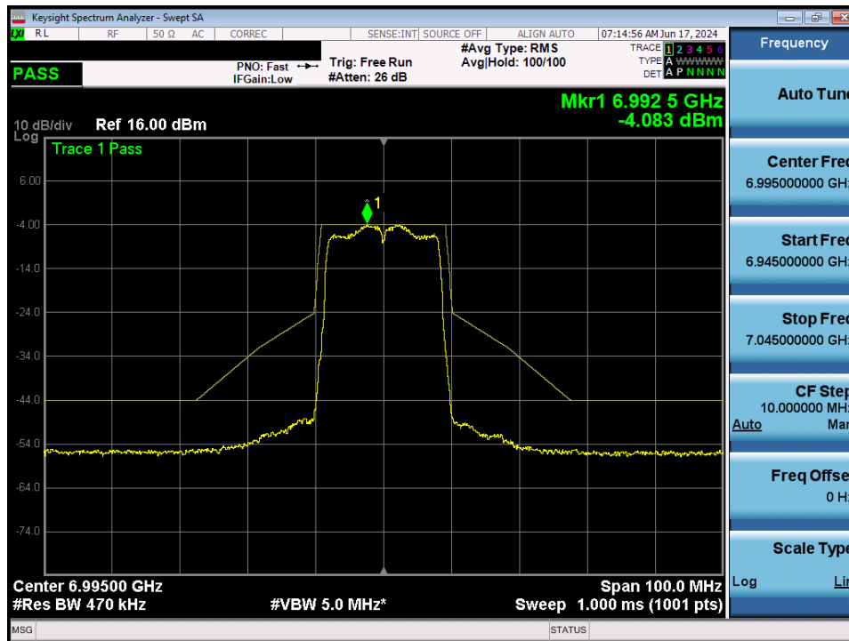
Plot 7-116. In-Band Emission MIMO ANT2 (20MHz 802.11a (UNII Band 8) – Ch. 209)
