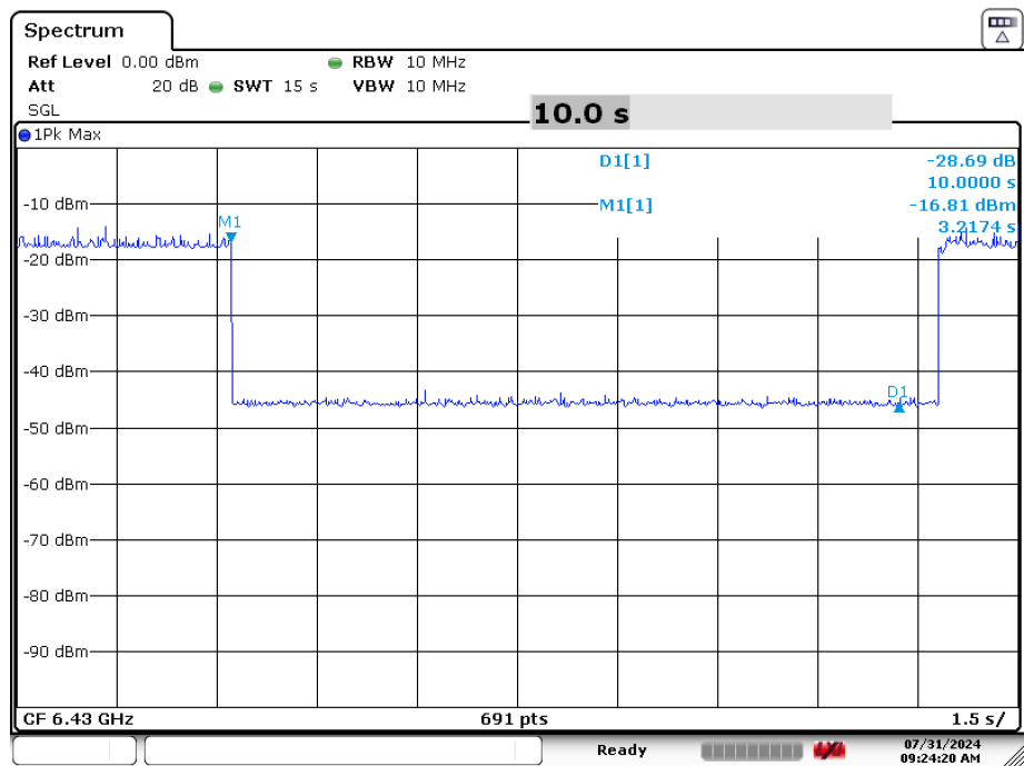
Plot 7-127. Contention Based Protocol Timing Plot (160MHz (UNII Band 6) – Ch. 111 Low)
