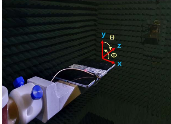
Figure 1: Geometry for SM-X828U for Radiation patterns.
