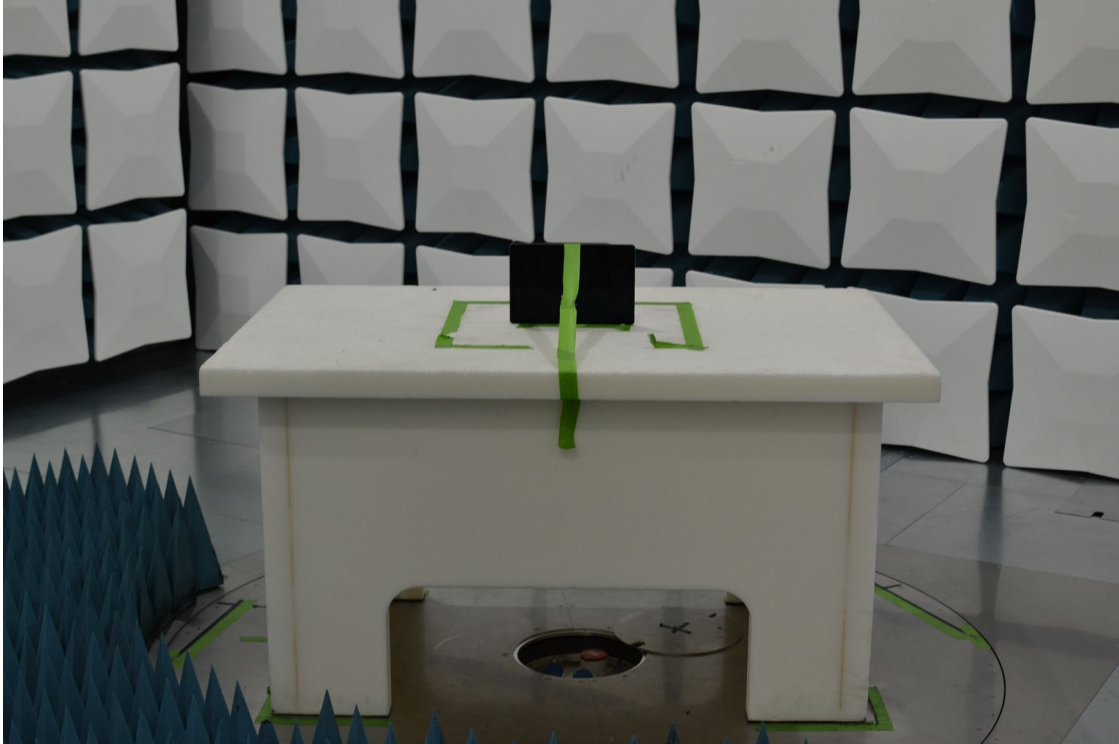
Figure 5. Test Setup – Y Position – 30MHz-1GHz
