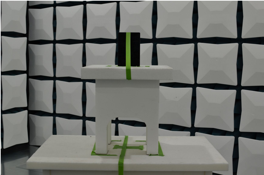
Figure 3. Test Setup – Z Position – 1GHz-40GHz
