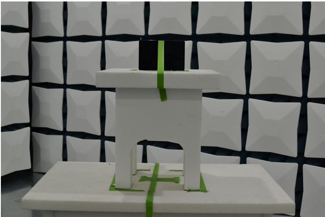
Figure 2. Test Setup – Y Position – 1GHz-40GHz
