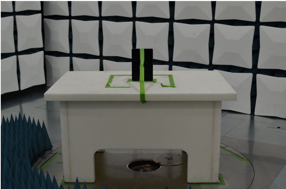
Figure 6. Test Setup – Z Position – 30MHz-1GHz
