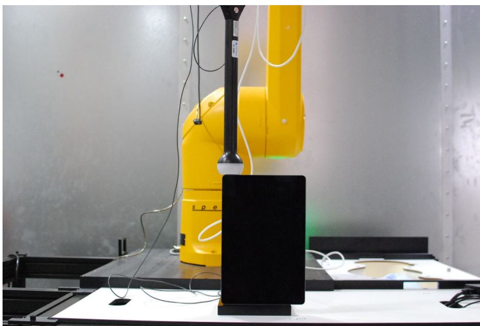
Test Setup Photo 4 H-field, Bottom edge, 0mm
