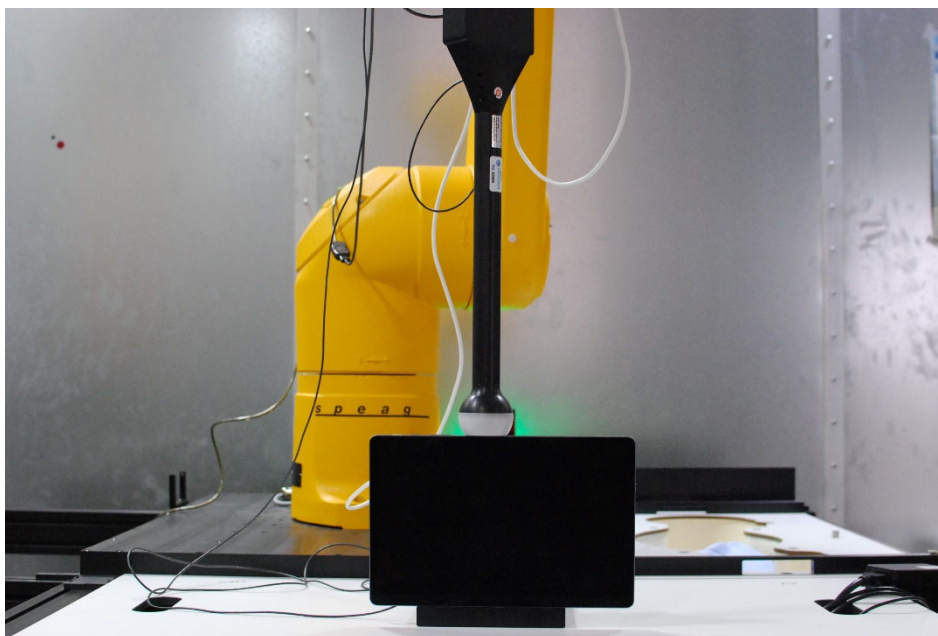
Test Setup Photo 5 H-field, Right edge, 0mm
