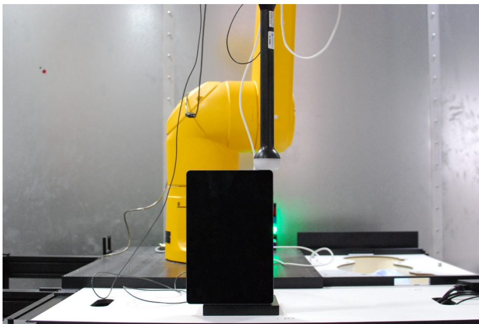
Test Setup Photo 3 H-field, Top edge, 0mm
