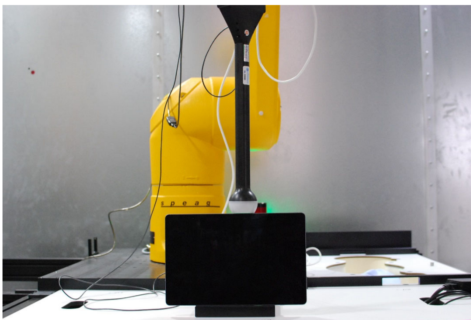
Test Setup Photo 6 H-field, Left edge, 0mm
