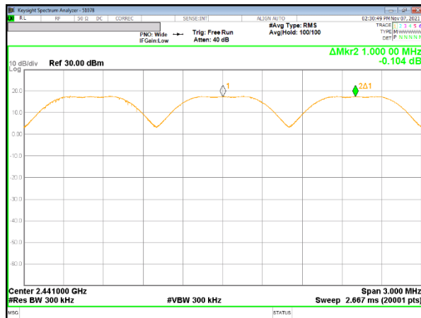
ANT1 SEPARATION
