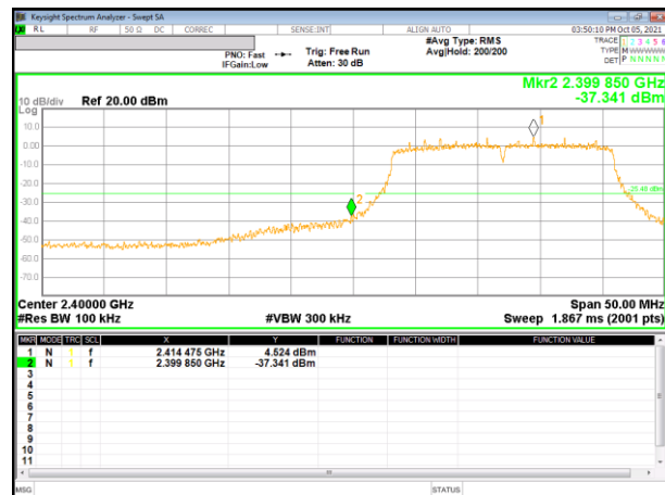
1 Channel Band-edge
