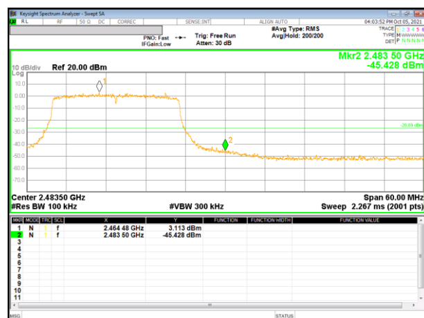
12 Channel Band-edge_SISO
