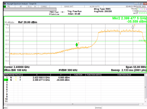
2 Channel Band-edge
