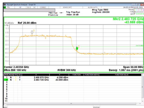
13 Channel Band-edge_SISO
