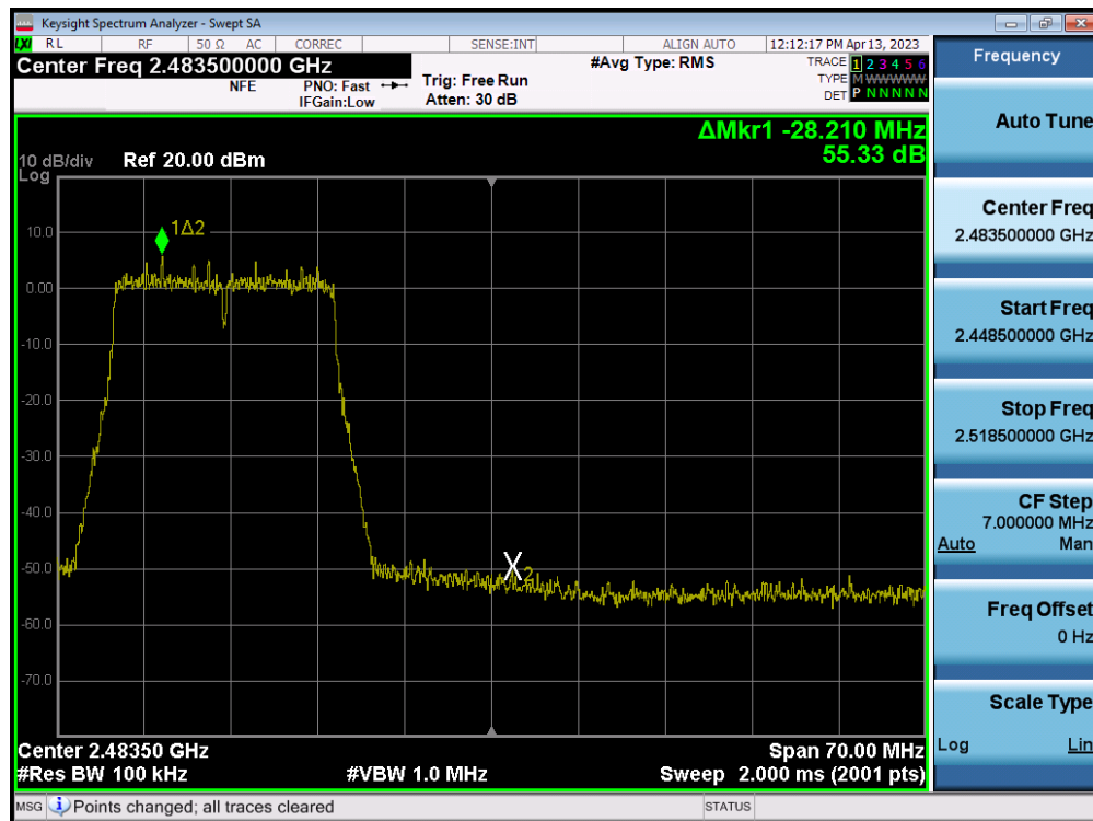
Plot 7-91. Band Edge Plot SISO ANT2 (802.11ax (2.4GHz) – Ch. 11)
