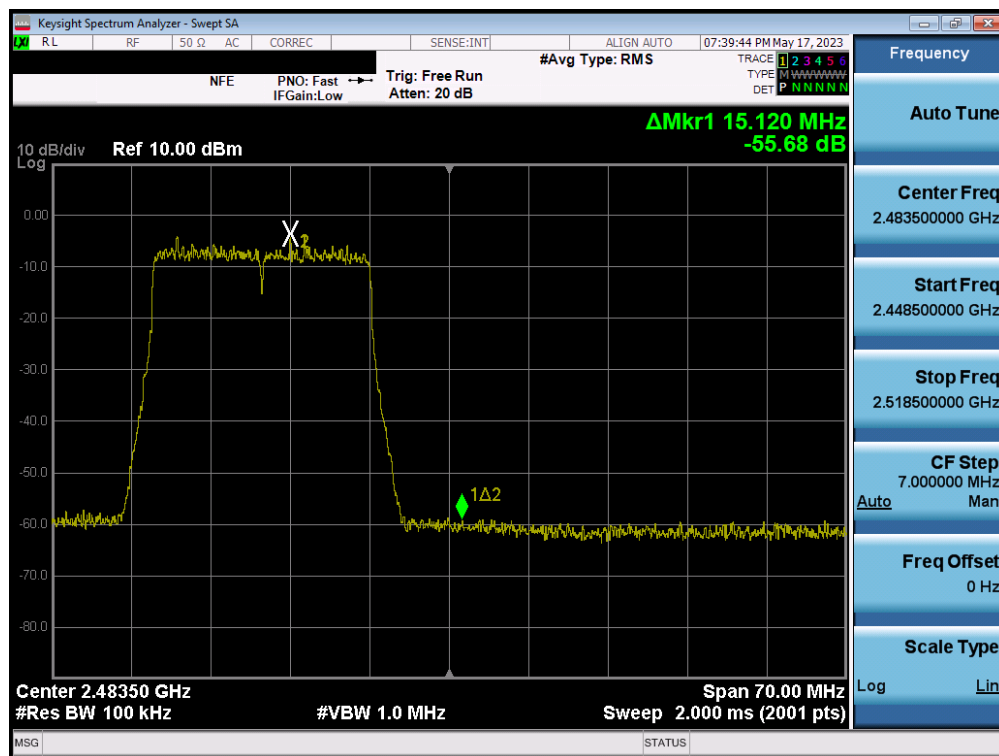
Plot 7-92. Band Edge Plot SISO ANT2 (802.11ax (2.4GHz) – Ch. 12)
