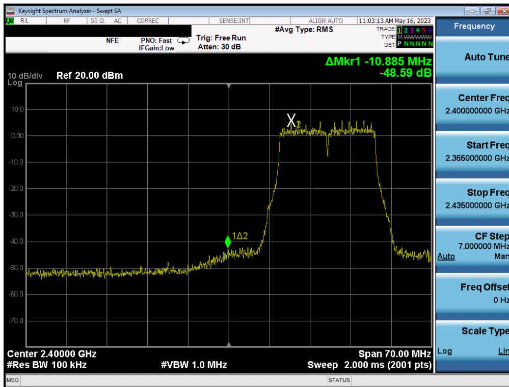
Plot 7-78. Band Edge Plot SISO ANT2 (802.11g- Ch. 2)
