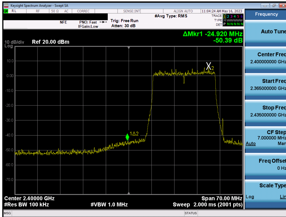
Plot 7-89. Band Edge Plot SISO ANT2 (802.11ax (2.4GHz) – Ch. 2)
