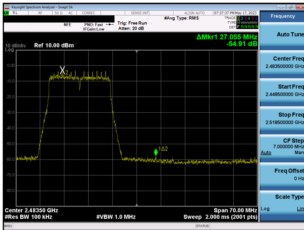
Plot 7-86. Band Edge Plot SISO ANT2 (802.11n (2.4GHz) – Ch. 12)
