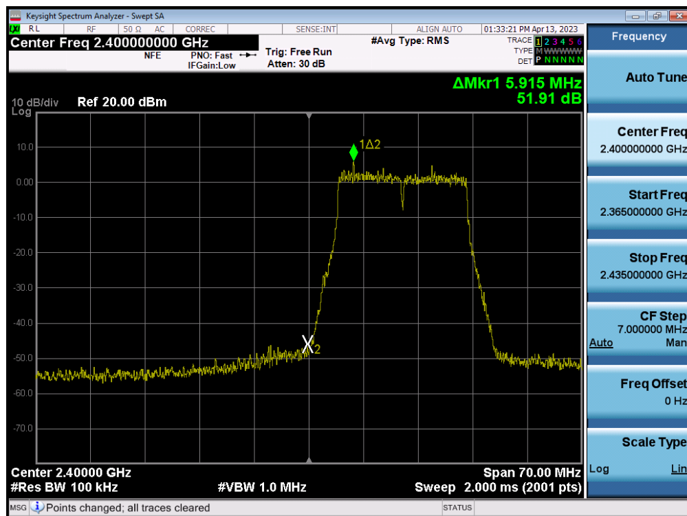
Plot 7-98. Band Edge Plot MIMO ANT1 (802.11g- Ch. 1)
