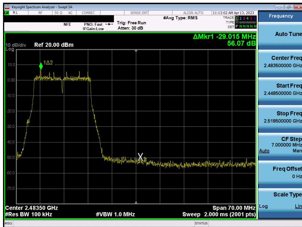
Plot 7-80. Band Edge Plot SISO ANT2 (802.11g – Ch. 11)
