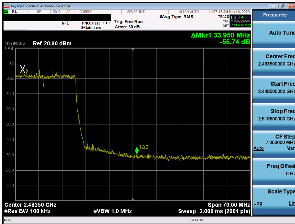
Plot 7-90. Band Edge Plot SISO ANT2 (802.11ax (2.4GHz) – Ch. 10)
