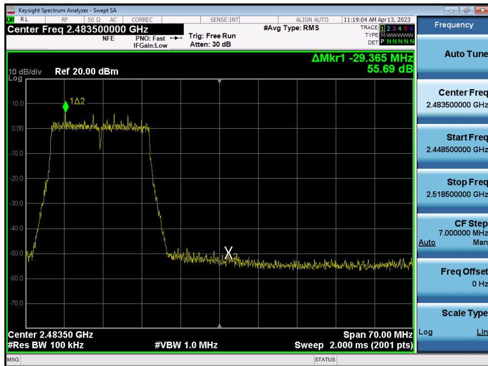
Plot 7-85. Band Edge Plot SISO ANT2 (802.11n (2.4GHz) – Ch. 11)
