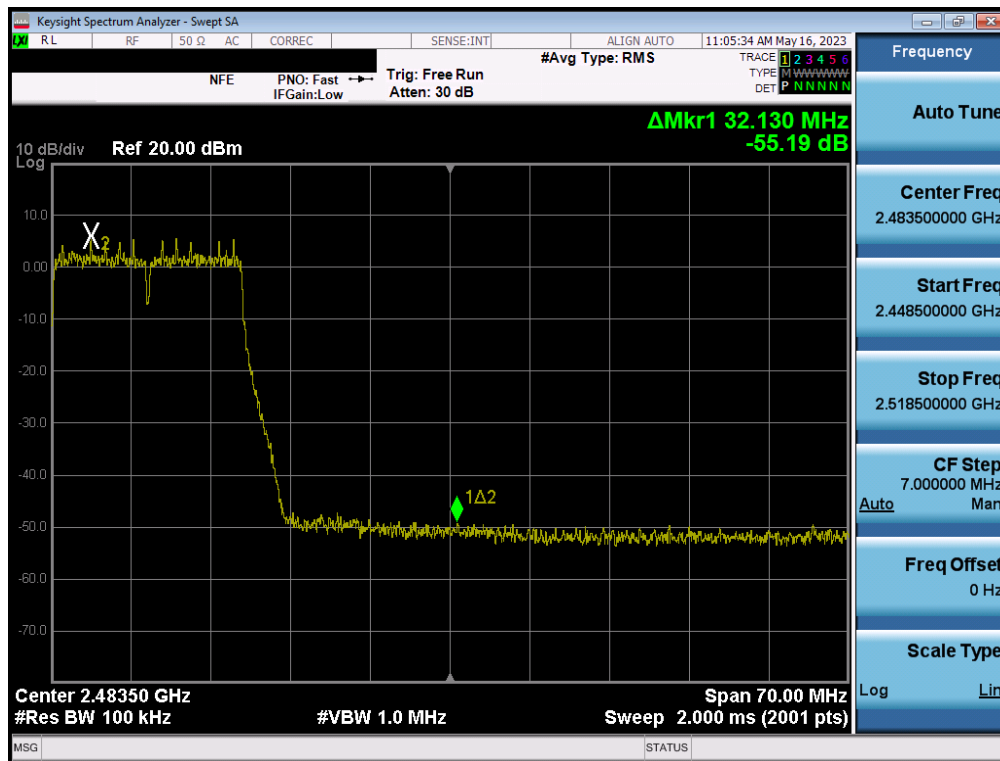
Plot 7-79. Band Edge Plot SISO ANT2 (802.11g – Ch. 10)
