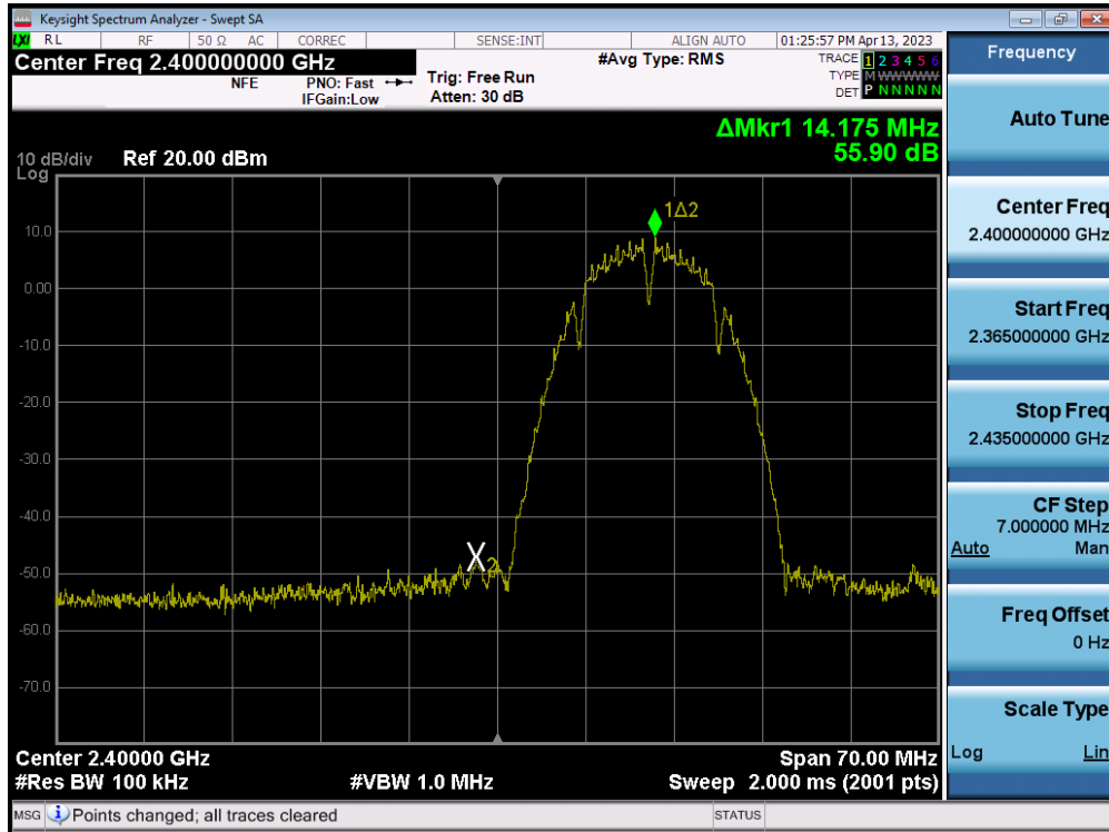
Plot 7-94. Band Edge Plot MIMO ANT1 (802.11b – Ch. 1)
