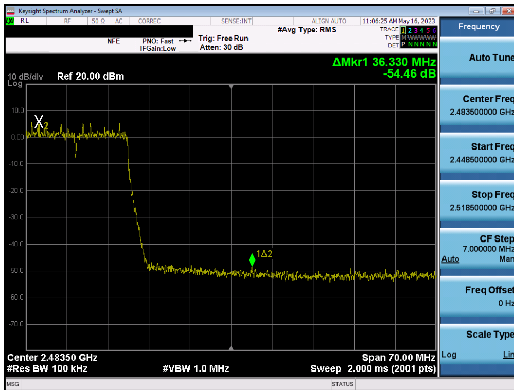
Plot 7-84. Band Edge Plot SISO ANT2 (802.11n (2.4GHz) – Ch. 10)
