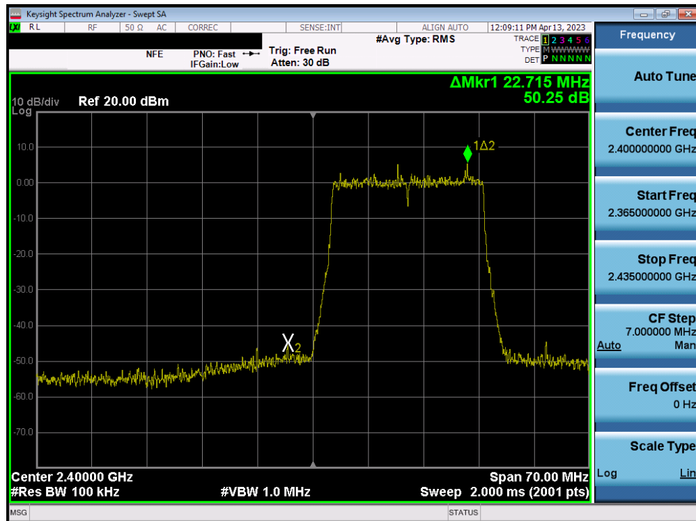
Plot 7-88. Band Edge Plot SISO ANT2 (802.11ax (2.4GHz) – Ch. 1)
