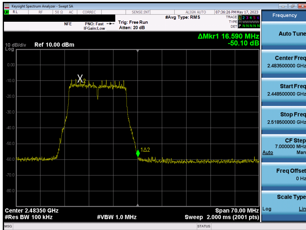
Plot 7-82. Band Edge Plot SISO ANT2 (802.11g – Ch. 13)
