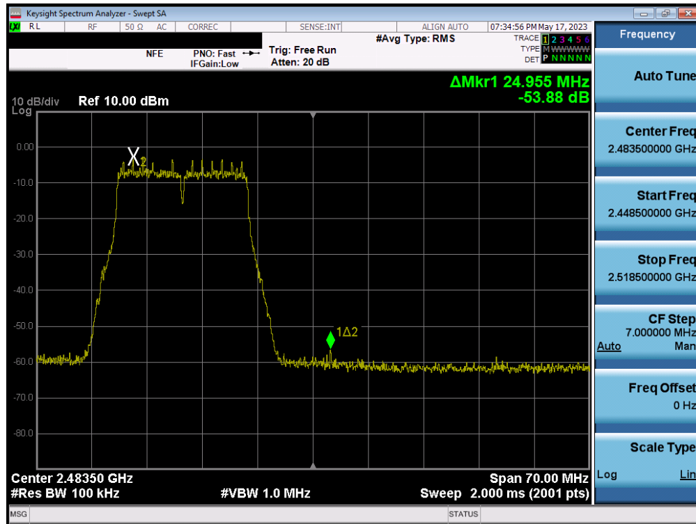
Plot 7-81. Band Edge Plot SISO ANT2 (802.11g – Ch. 12)
