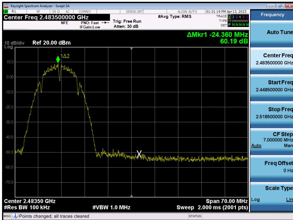
Plot 7-95. Band Edge Plot MIMO ANT1 (802.11b – Ch. 11)
