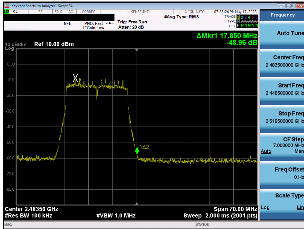
Plot 7-87. Band Edge Plot SISO ANT2 (802.11n (2.4GHz) – Ch. 13)
