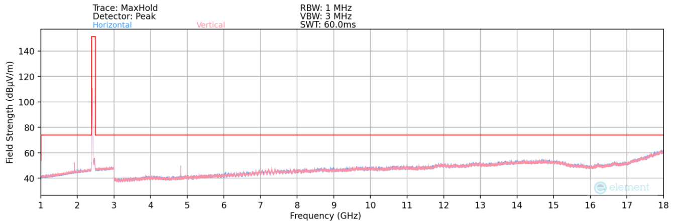
Plot 7-158. Radiated Spurious Plot above 1GHz MIMO (802.11b – Ch. 1)
