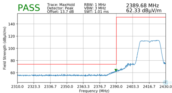
Plot 7-165. Radiated Restricted Lower Band Edge Measurement SISO ANT2 (Peak)
