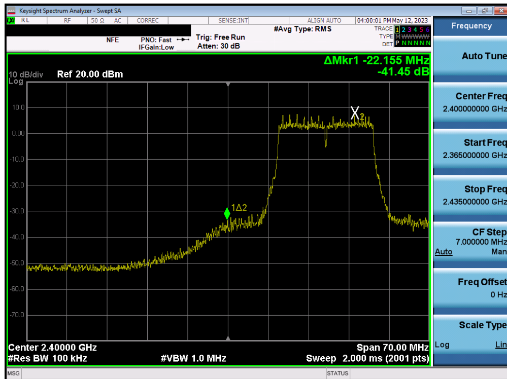
Plot 7-120. Band Edge Plot MIMO ANT2 (802.11g- Ch. 2)
