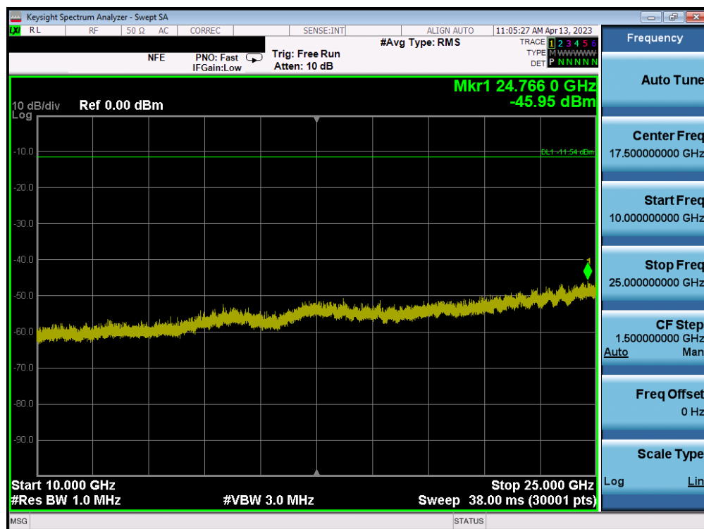
Plot 7-141. Conducted Spurious Plot SISO ANT2 (802.11b – Ch. 11)
