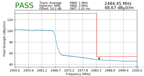
Plot 7-166. Radiated Restricted Upper Band Edge Measurement SISO ANT2 (Average)
