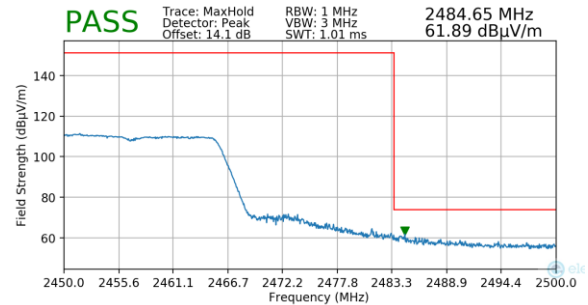
Plot 7-167. Radiated Restricted Upper Band Edge Measurement SISO ANT2 (Peak)
