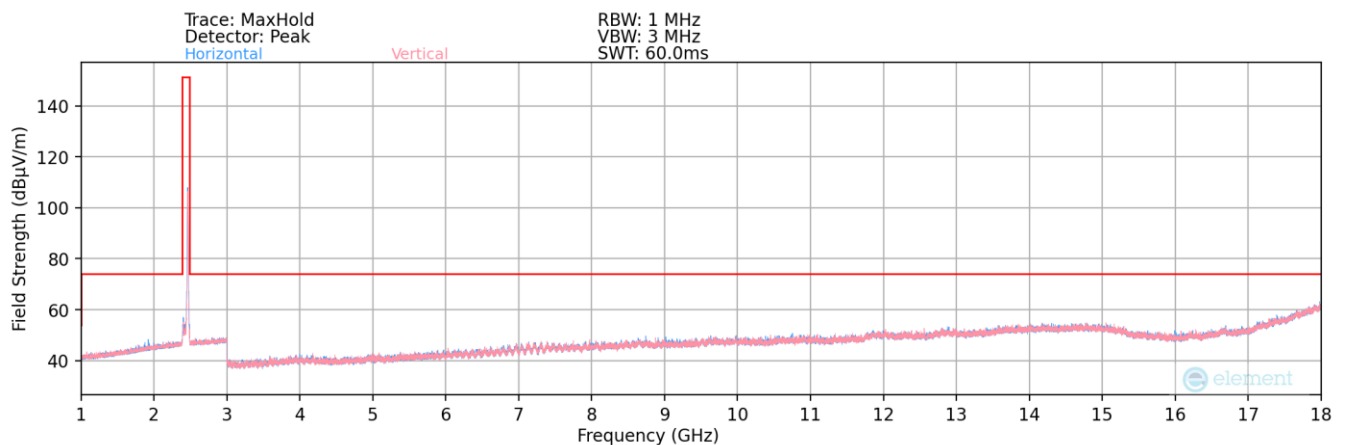
Plot 7-156. Radiated Spurious Plot above 1GHz SISO ANT2 (802.11b – Ch. 11)
