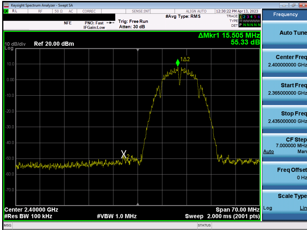
Plot 7-115. Band Edge Plot MIMO ANT2 (802.11b – Ch. 1)
