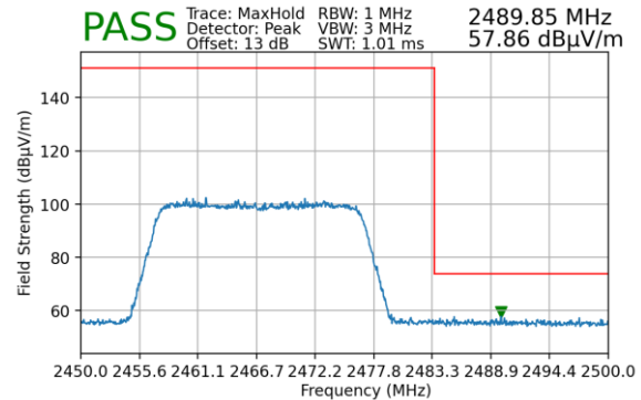
Plot 7-183. Radiated Restricted Upper Band Edge Measurement MIMO (Peak)
