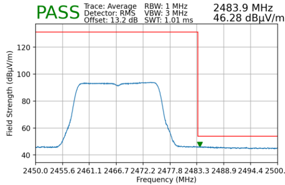
Plot 7-170. Radiated Restricted Upper Band Edge Measurement SISO ANT2 (Average)
