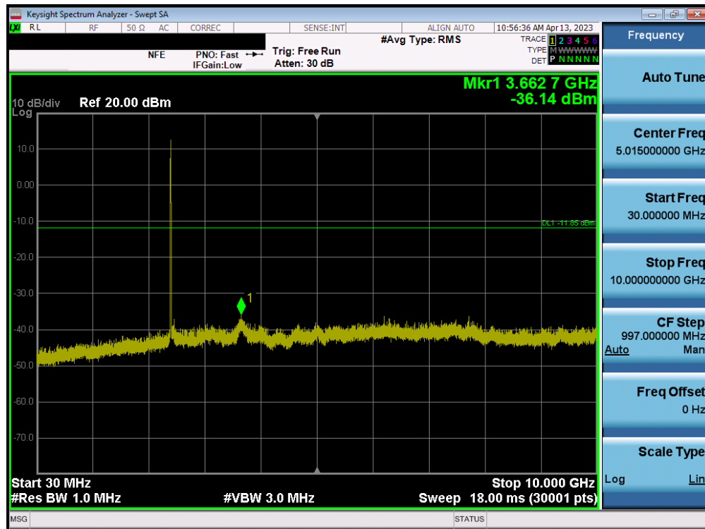
Plot 7-136. Conducted Spurious Plot SISO ANT2 (802.11b – Ch. 1)
