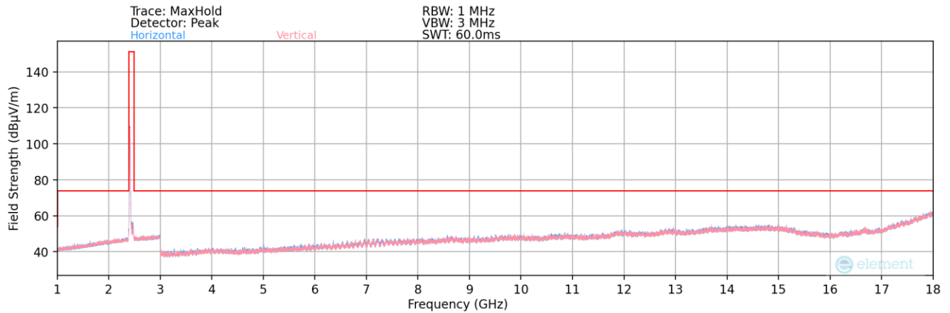
Plot 7-154. Radiated Spurious Plot above 1GHz SISO ANT2 (802.11b – Ch. 1)
