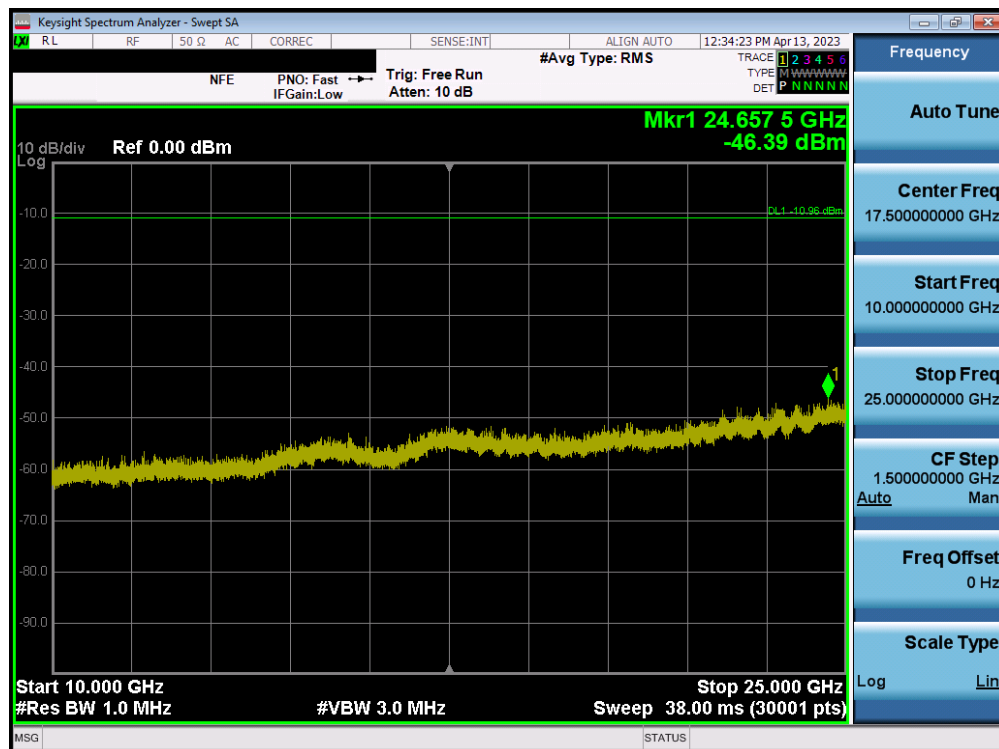
Plot 7-153. Conducted Spurious Plot MIMO ANT2 (802.11b – Ch. 11)
