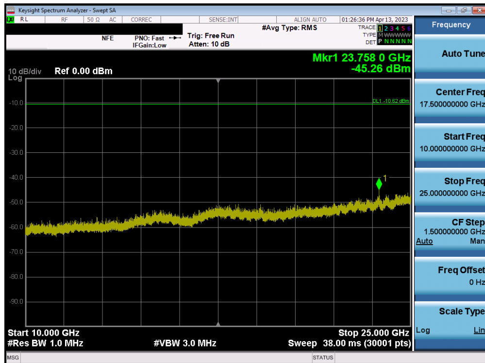
Plot 7-143. Conducted Spurious Plot MIMO ANT1 (802.11b – Ch. 1)
