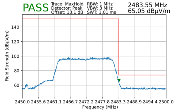
Plot 7-173. Radiated Restricted Upper Band Edge Measurement SISO ANT2 (Peak)
