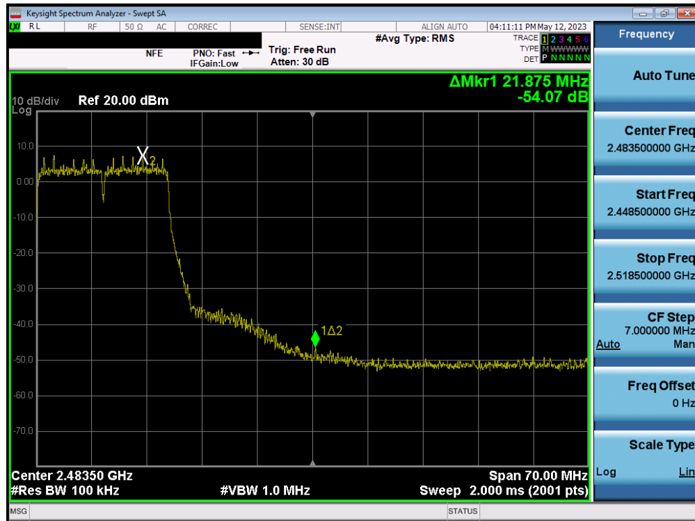
Plot 7-100. Band Edge Plot MIMO ANT1 (802.11g - Ch. 10)
