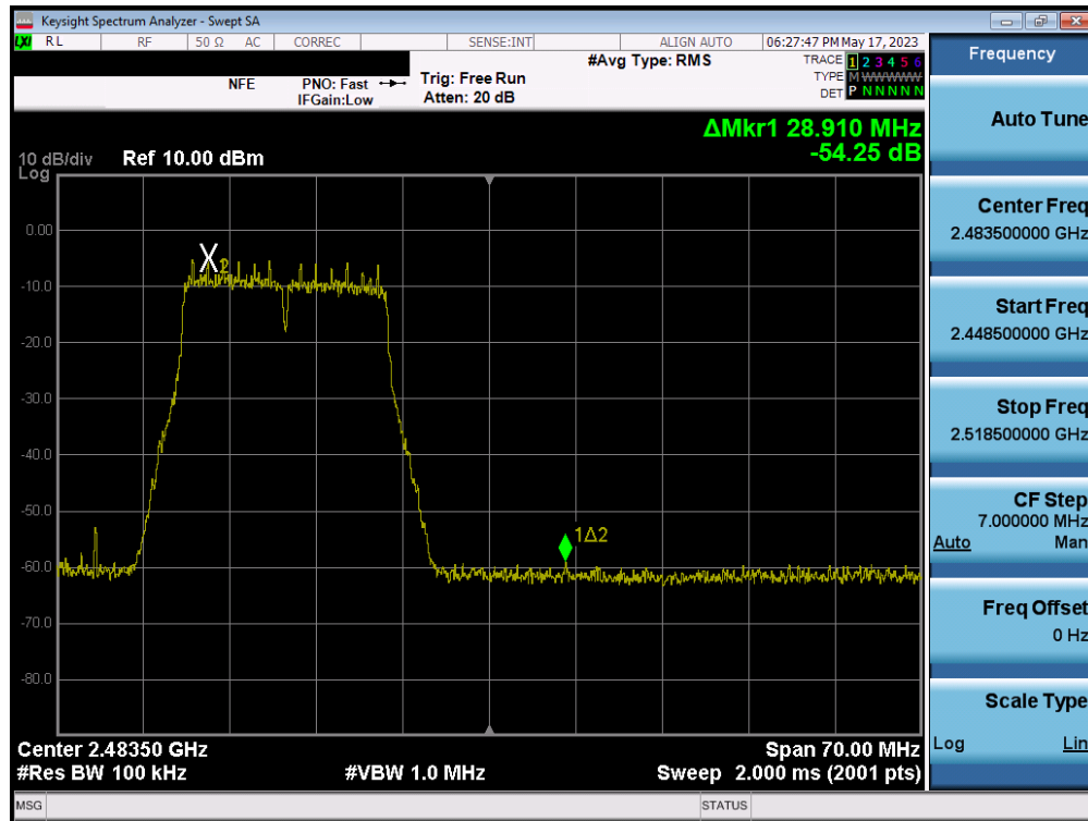
Plot 7-102. Band Edge Plot MIMO ANT1 (802.11g – Ch. 12)
