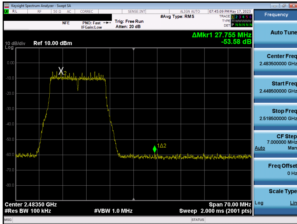
Plot 7-123. Band Edge Plot MIMO ANT2 (802.11g – Ch. 12)
