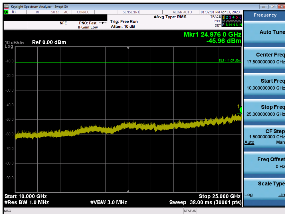
Plot 7-147. Conducted Spurious Plot MIMO ANT1 (802.11b – Ch. 11)
