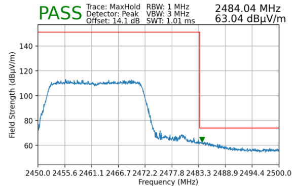
Plot 7-169. Radiated Restricted Upper Band Edge Measurement SISO ANT2 (Peak)
