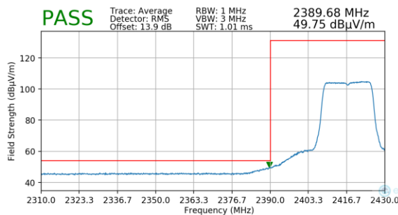
Plot 7-164. Radiated Restricted Lower Band Edge Measurement SISO ANT2 (Average)
