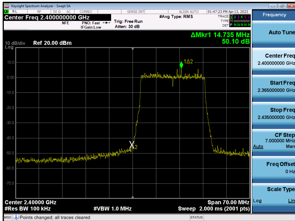
Plot 7-109. Band Edge Plot MIMO ANT1 (802.11ax (2.4GHz) – Ch. 1)
