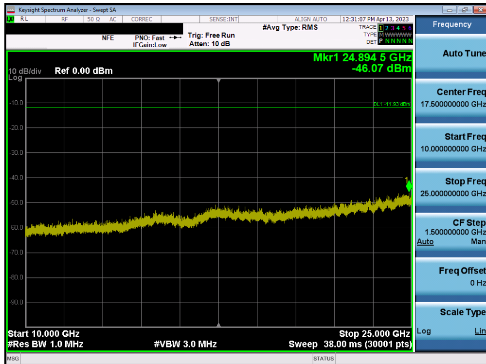
Plot 7-149. Conducted Spurious Plot MIMO ANT2 (802.11b – Ch. 1)
