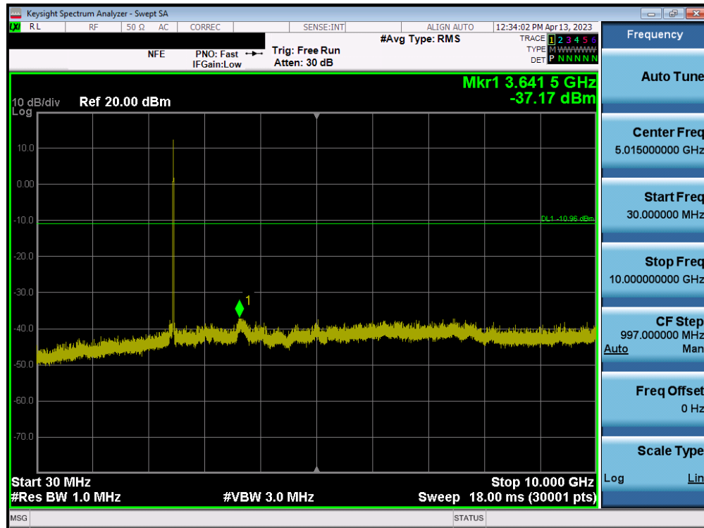
Plot 7-152. Conducted Spurious Plot MIMO ANT2 (802.11b – Ch. 11)
