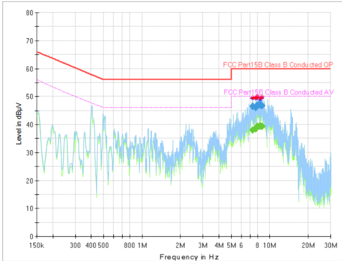
Plot 7-188. Line Conducted Plot with 802.11b (N)
