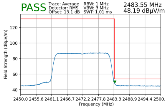
Plot 7-172. Radiated Restricted Upper Band Edge Measurement SISO ANT2 (Average)
