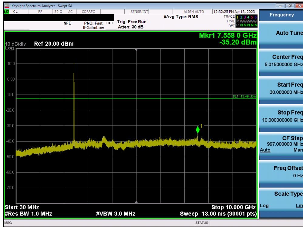
Plot 7-150. Conducted Spurious Plot MIMO ANT2 (802.11b – Ch. 6)
