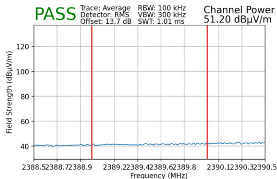
Plot 7-162. Radiated Restricted Lower Band Edge Measurement SISO ANT2 (Average)
