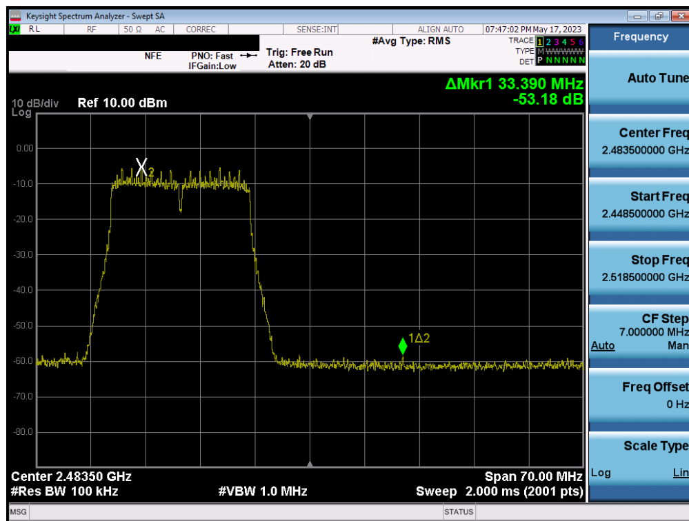
Plot 7-128. Band Edge Plot MIMO ANT2 (802.11n (2.4GHz) – Ch. 12)
