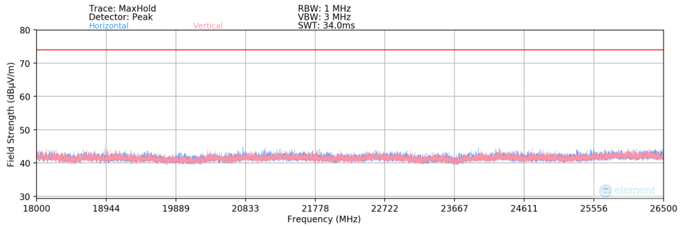
Plot 7-161. Radiated Spurious Plot above 18GHz MIMO
