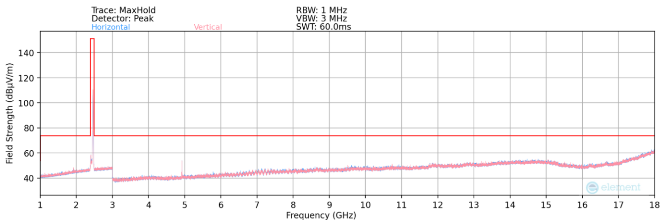
Plot 7-160. Radiated Spurious Plot above 1GHz MIMO (802.11b – Ch. 11)
