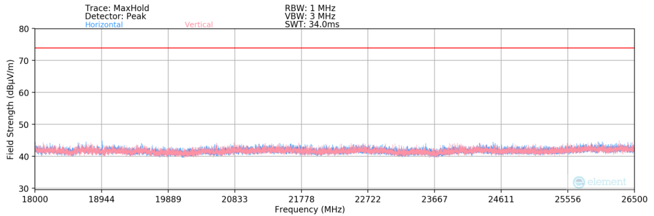
Plot 7-157. Radiated Spurious Plot above 18GHz SISO ANT2
