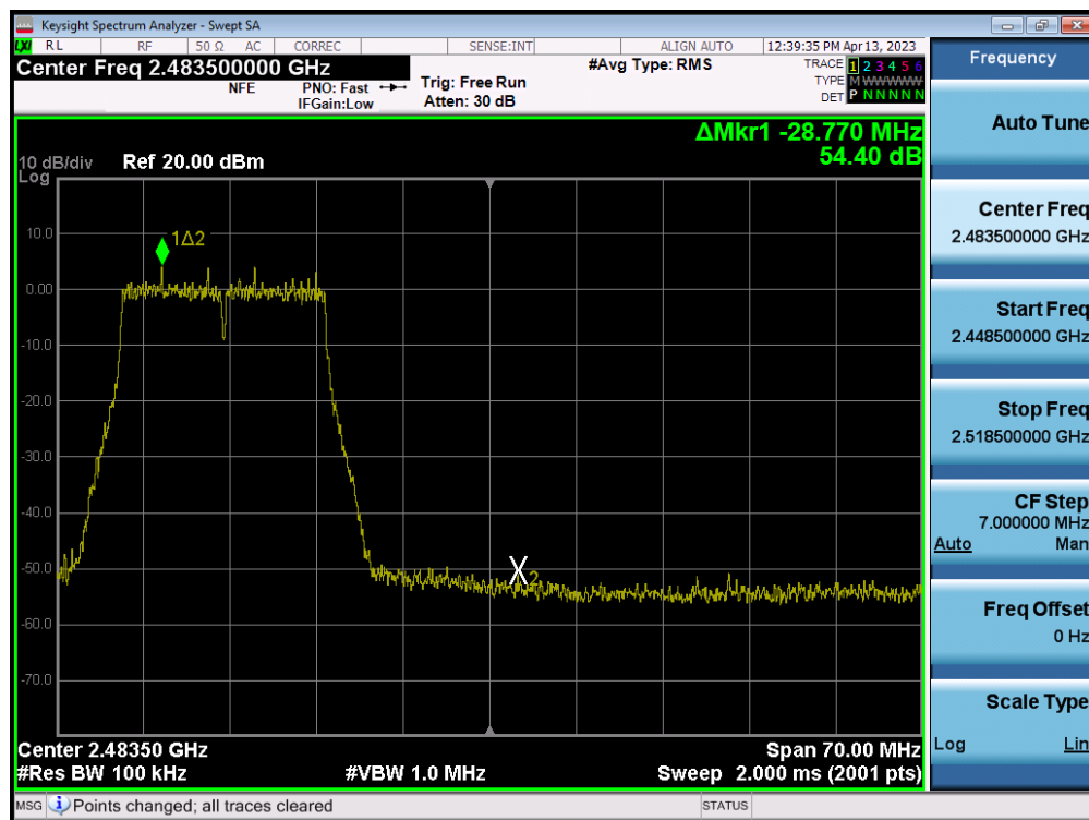
Plot 7-122. Band Edge Plot MIMO ANT2 (802.11g – Ch. 11)
