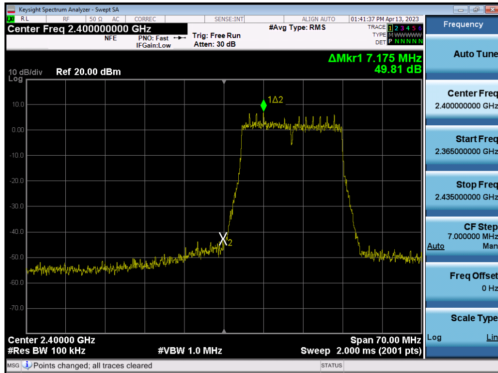
Plot 7-104. Band Edge Plot MIMO ANT1 (802.11n (2.4GHz) – Ch. 1)
