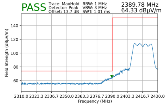
Plot 7-177. Radiated Restricted Lower Band Edge Measurement MIMO (Peak)
