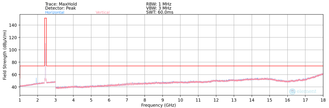
Plot 7-155. Radiated Spurious Plot above 1GHz SISO ANT2 (802.11b – Ch. 6)
