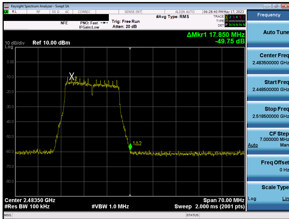
Plot 7-103. Band Edge Plot MIMO ANT1 (802.11g – Ch. 13)
