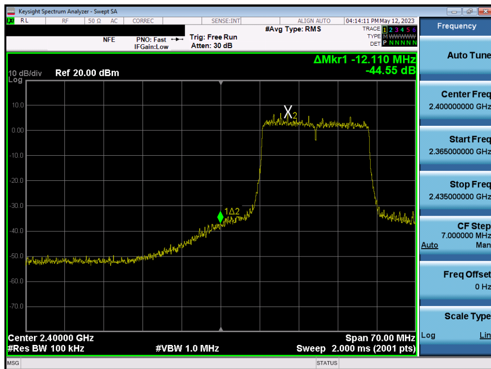
Plot 7-110. Band Edge Plot MIMO ANT1 (802.11ax (2.4GHz) – Ch. 2)
