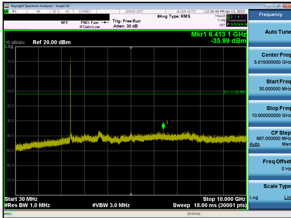
Plot 7-148. Conducted Spurious Plot MIMO ANT2 (802.11b – Ch. 1)
