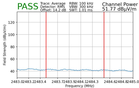
Plot 7-180. Radiated Restricted Upper Band Edge Measurement MIMO (Average)
