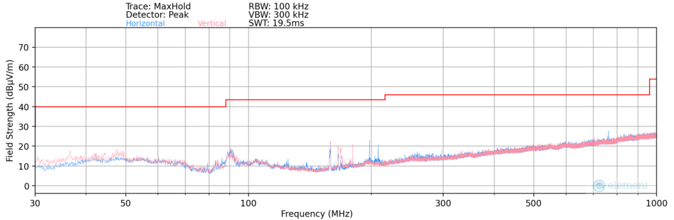
Plot 7-186. Radiated Spurious Plot below 1GHz MIMO
