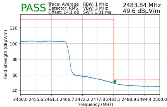
Plot 7-178. Radiated Restricted Upper Band Edge Measurement MIMO (Average)
