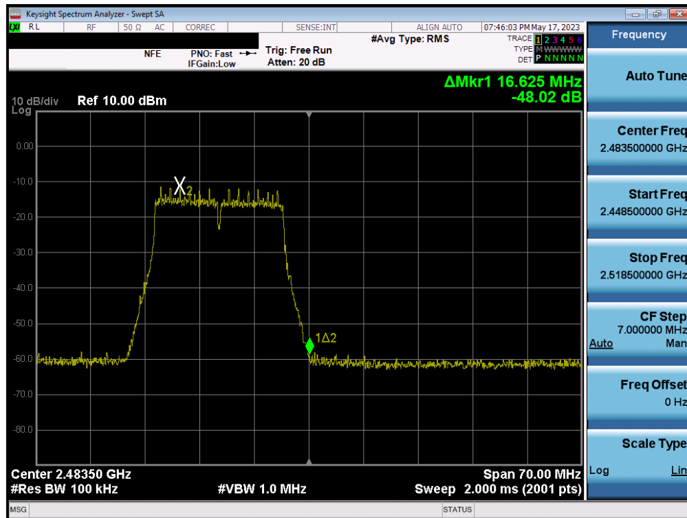
Plot 7-124. Band Edge Plot MIMO ANT2 (802.11g – Ch. 13)
