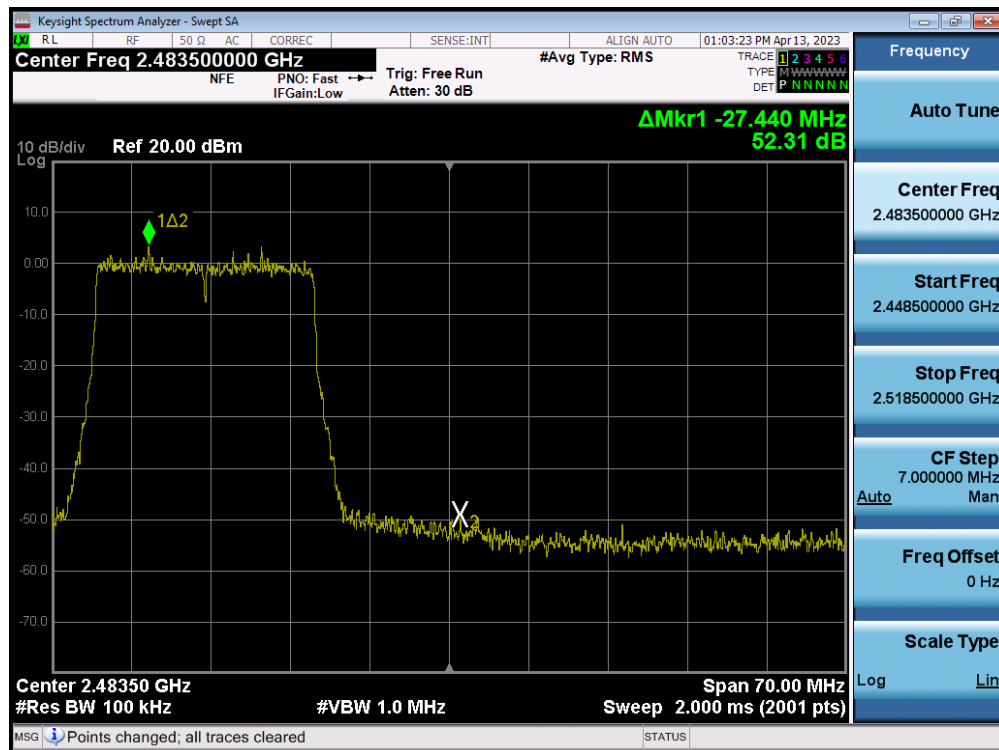
Plot 7-133. Band Edge Plot MIMO ANT2 (802.11ax (2.4GHz) – Ch. 11)
