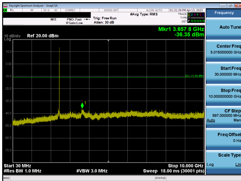
Plot 7-146. Conducted Spurious Plot MIMO ANT1 (802.11b – Ch. 11)
