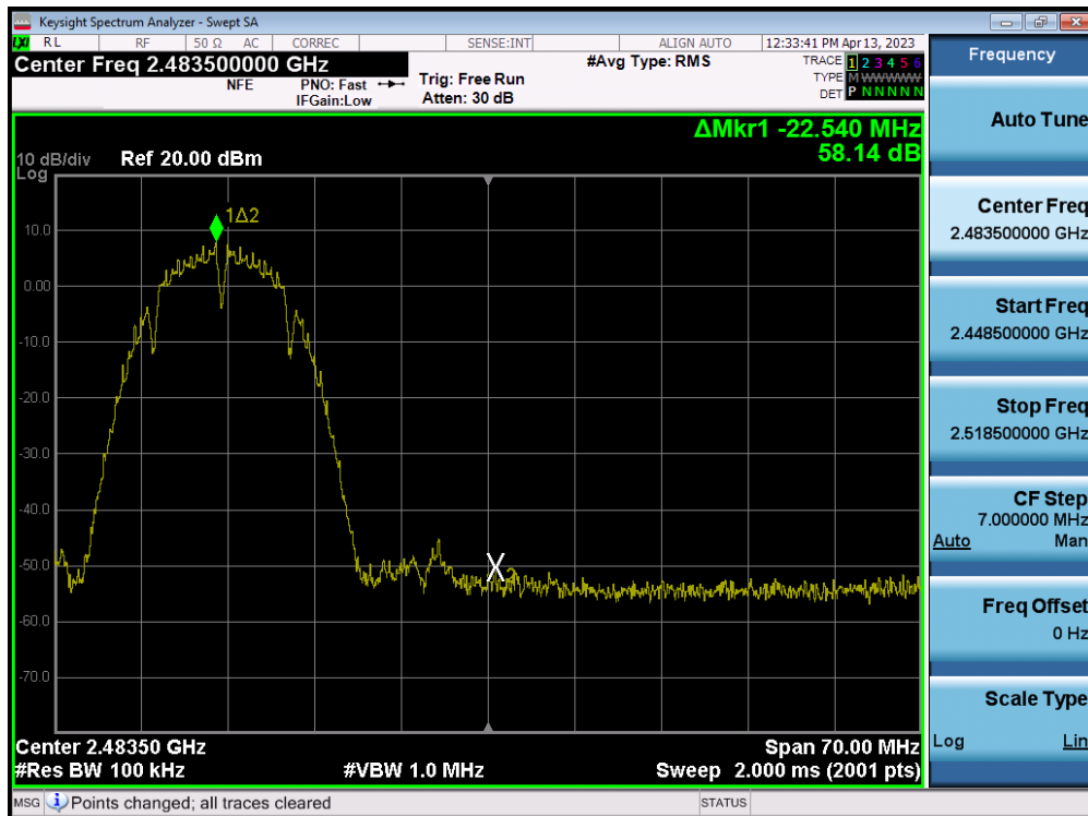
Plot 7-116. Band Edge Plot MIMO ANT2 (802.11b – Ch. 11)
