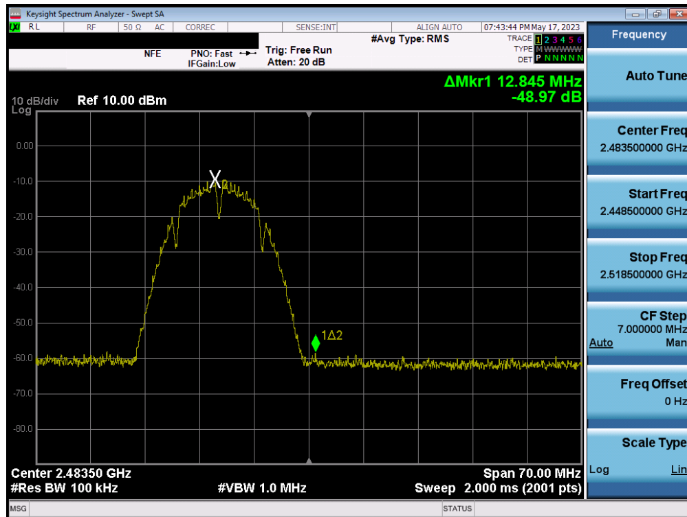
Plot 7-118. Band Edge Plot MIMO ANT2 (802.11b – Ch. 13)
