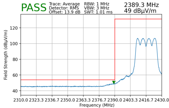
Plot 7-176. Radiated Restricted Lower Band Edge Measurement MIMO (Average)
