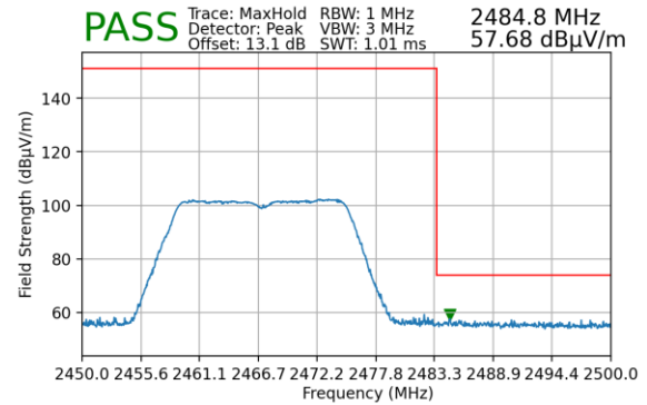
Plot 7-171. Radiated Restricted Upper Band Edge Measurement SISO ANT2 (Peak)
