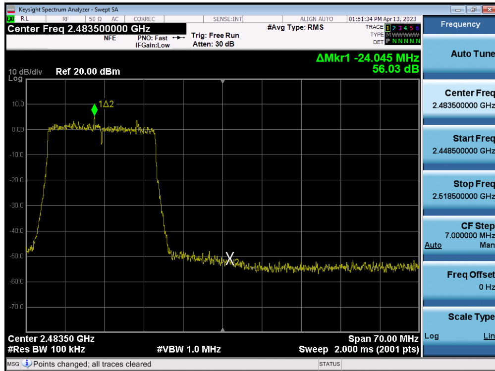
Plot 7-112. Band Edge Plot MIMO ANT1 (802.11ax (2.4GHz) – Ch. 11)
