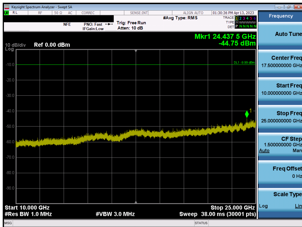
Plot 7-145. Conducted Spurious Plot MIMO ANT1 (802.11b – Ch. 6)
