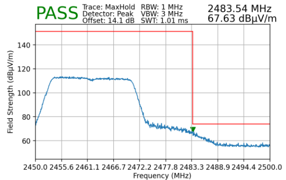
Plot 7-181. Radiated Restricted Upper Band Edge Measurement MIMO (Peak)
