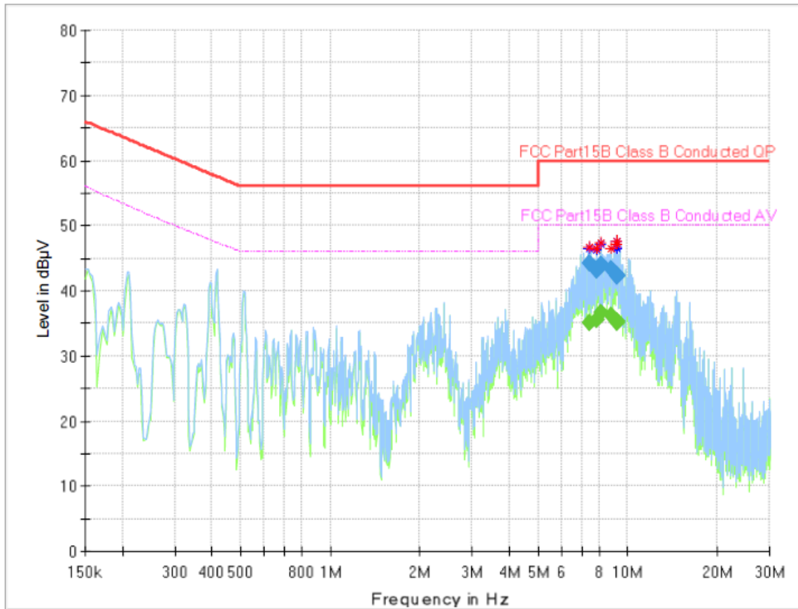
Plot 7-187. Line Conducted Plot with 802.11b (L1)
