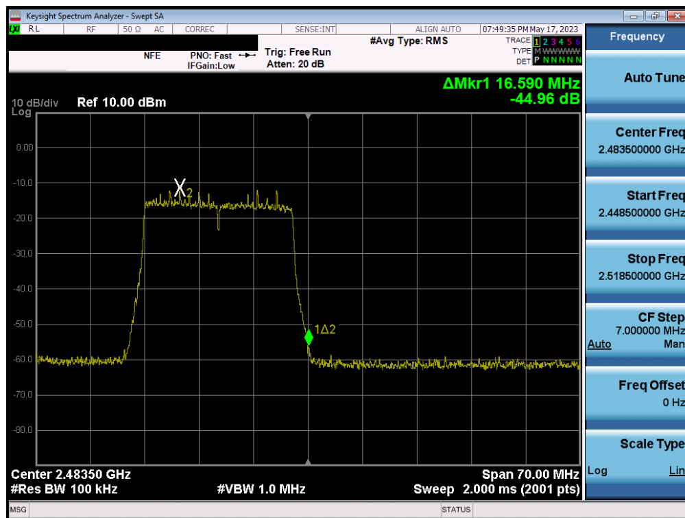
Plot 7-135. Band Edge Plot MIMO ANT2 (802.11ax (2.4GHz) – Ch. 13)
