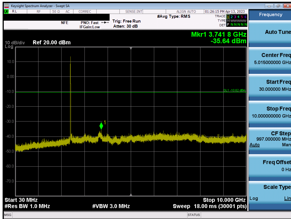
Plot 7-142. Conducted Spurious Plot MIMO ANT1 (802.11b – Ch. 1)
