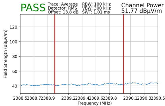
Plot 7-174. Radiated Restricted Lower Band Edge Measurement MIMO (Average)
