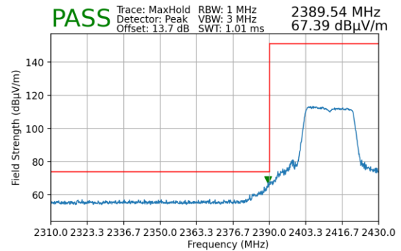
Plot 7-175. Radiated Restricted Lower Band Edge Measurement MIMO (Peak)
