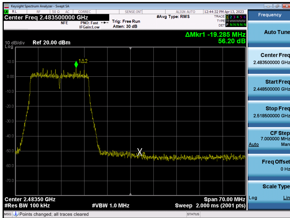
Plot 7-127. Band Edge Plot MIMO ANT2 (802.11n (2.4GHz) – Ch. 11)
