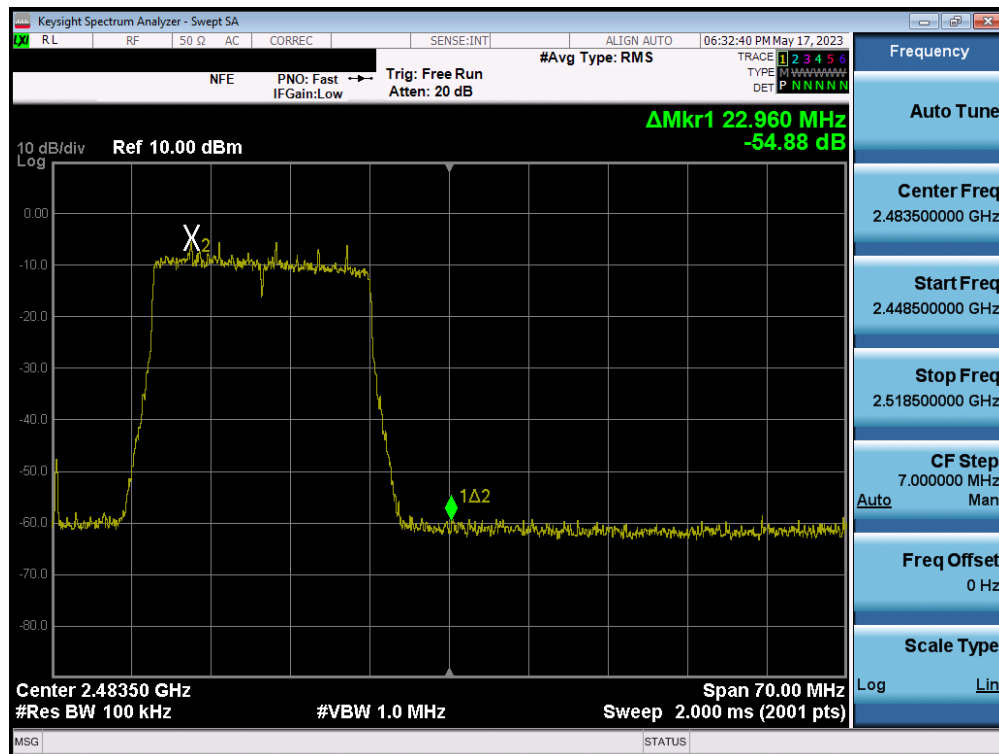
Plot 7-113. Band Edge Plot MIMO ANT1 (802.11ax (2.4GHz) – Ch. 12)
