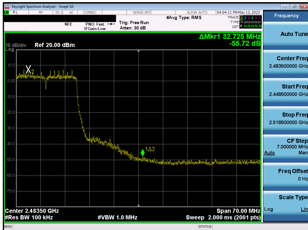
Plot 7-132. Band Edge Plot MIMO ANT2 (802.11ax (2.4GHz) – Ch. 10)
