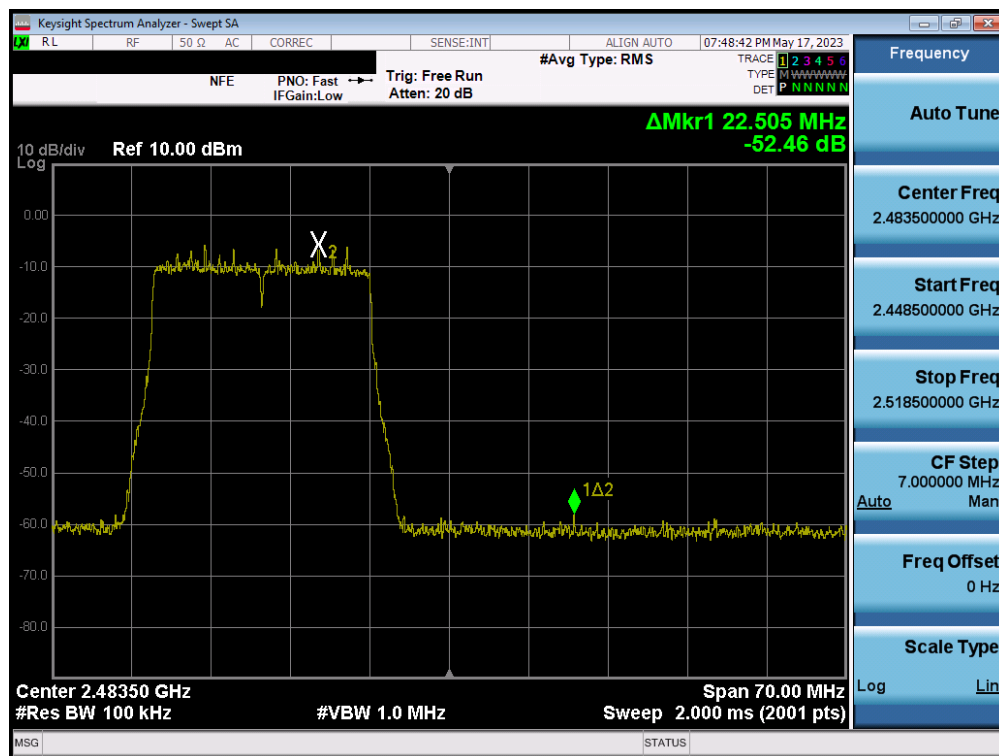
Plot 7-134. Band Edge Plot MIMO ANT2 (802.11ax (2.4GHz) – Ch. 12)
