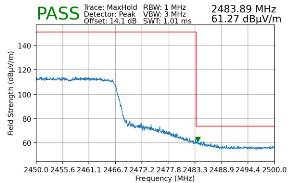
Plot 7-179. Radiated Restricted Upper Band Edge Measurement MIMO (Peak)
