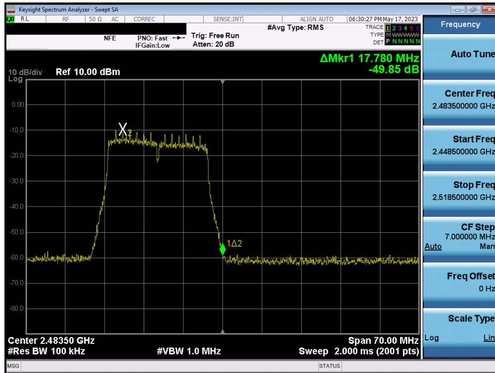
Plot 7-108. Band Edge Plot MIMO ANT1 (802.11n (2.4GHz) – Ch. 13)
