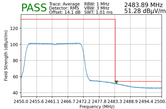
Plot 7-168. Radiated Restricted Upper Band Edge Measurement SISO ANT2 (Average)
