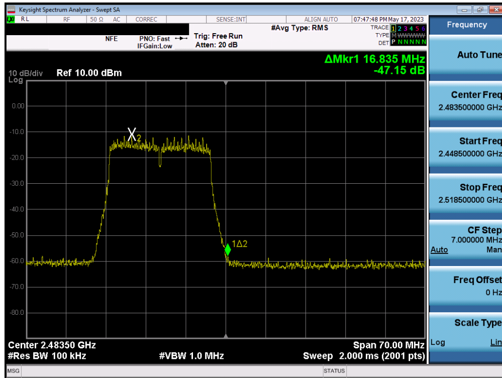
Plot 7-129. Band Edge Plot MIMO ANT2 (802.11n (2.4GHz) – Ch. 13)
