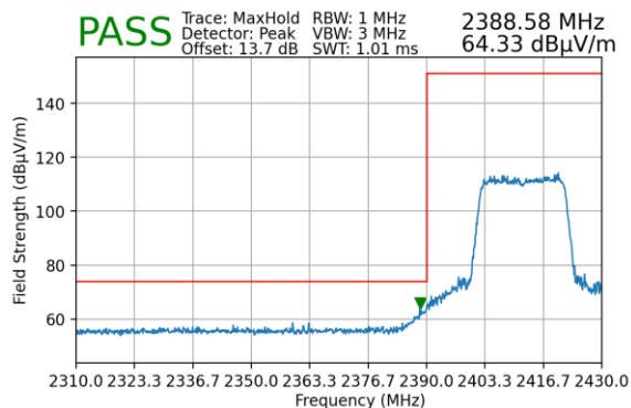
Plot 7-163. Radiated Restricted Lower Band Edge Measurement SISO ANT2 (Peak)
