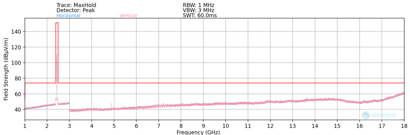
Plot 7-159. Radiated Spurious Plot above 1GHz MIMO (802.11b – Ch. 6)
