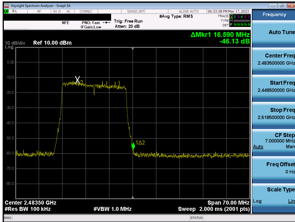
Plot 7-114. Band Edge Plot MIMO ANT1 (802.11ax (2.4GHz) – Ch. 13)
