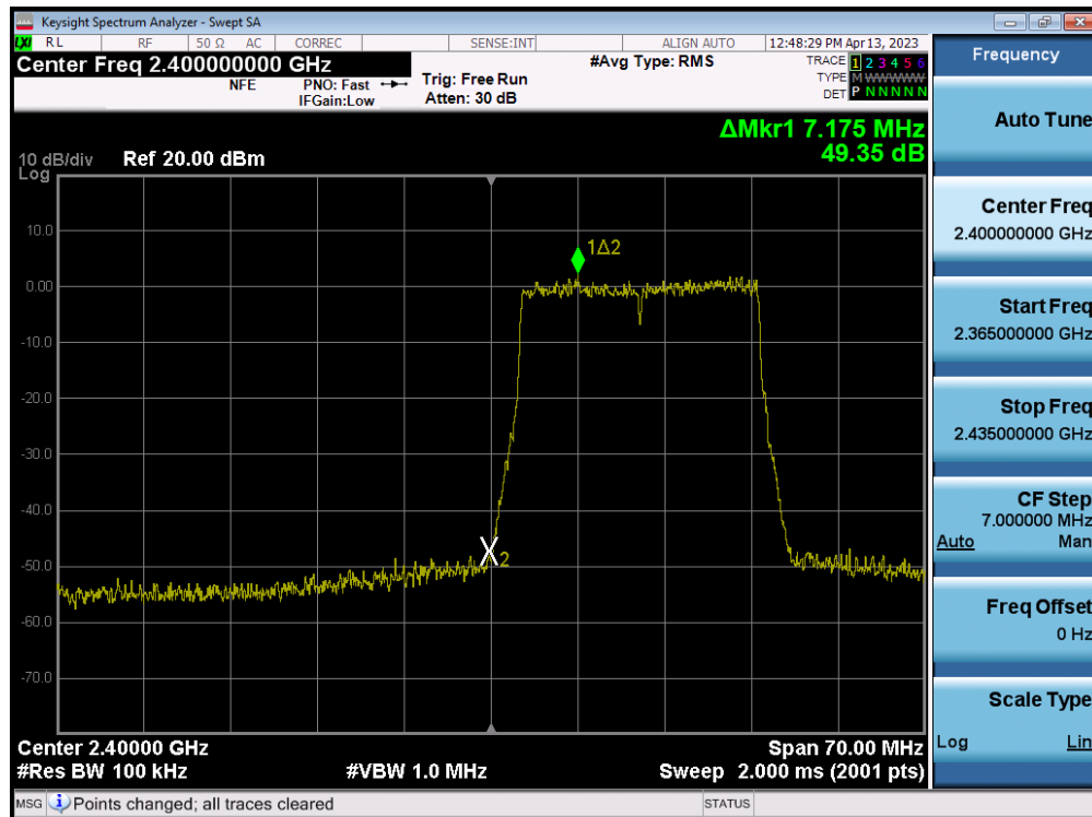
Plot 7-130. Band Edge Plot MIMO ANT2 (802.11ax (2.4GHz) – Ch. 1)
