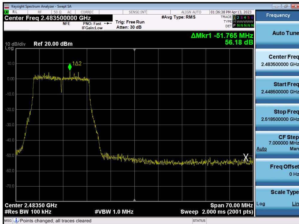
Plot 7-101. Band Edge Plot MIMO ANT1 (802.11g - Ch. 11)
