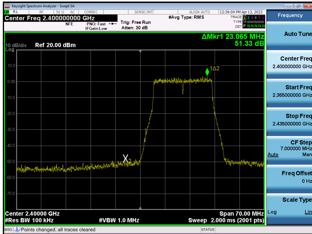
Plot 7-119. Band Edge Plot MIMO ANT2 (802.11g- Ch. 1)
