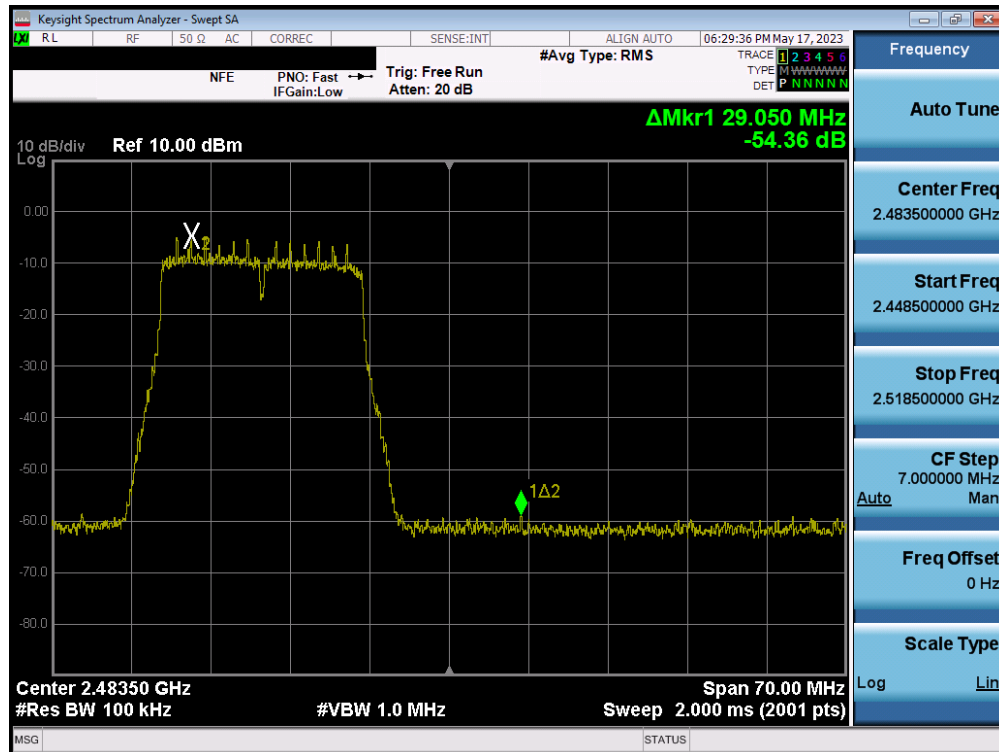
Plot 7-107. Band Edge Plot MIMO ANT1 (802.11n (2.4GHz) – Ch. 12)
