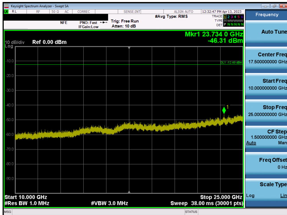
Plot 7-151. Conducted Spurious Plot MIMO ANT2 (802.11b – Ch. 6)
