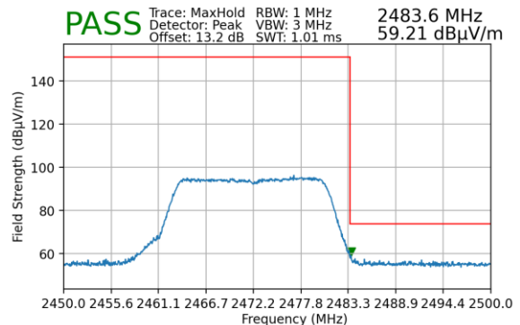
Plot 7-185. Radiated Restricted Upper Band Edge Measurement MIMO (Peak)
