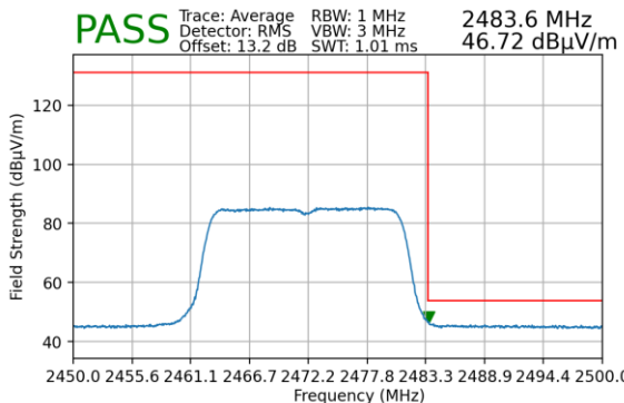
Plot 7-184. Radiated Restricted Upper Band Edge Measurement MIMO (Average)
