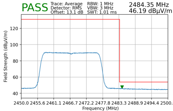
Plot 7-182. Radiated Restricted Upper Band Edge Measurement MIMO (Average)
