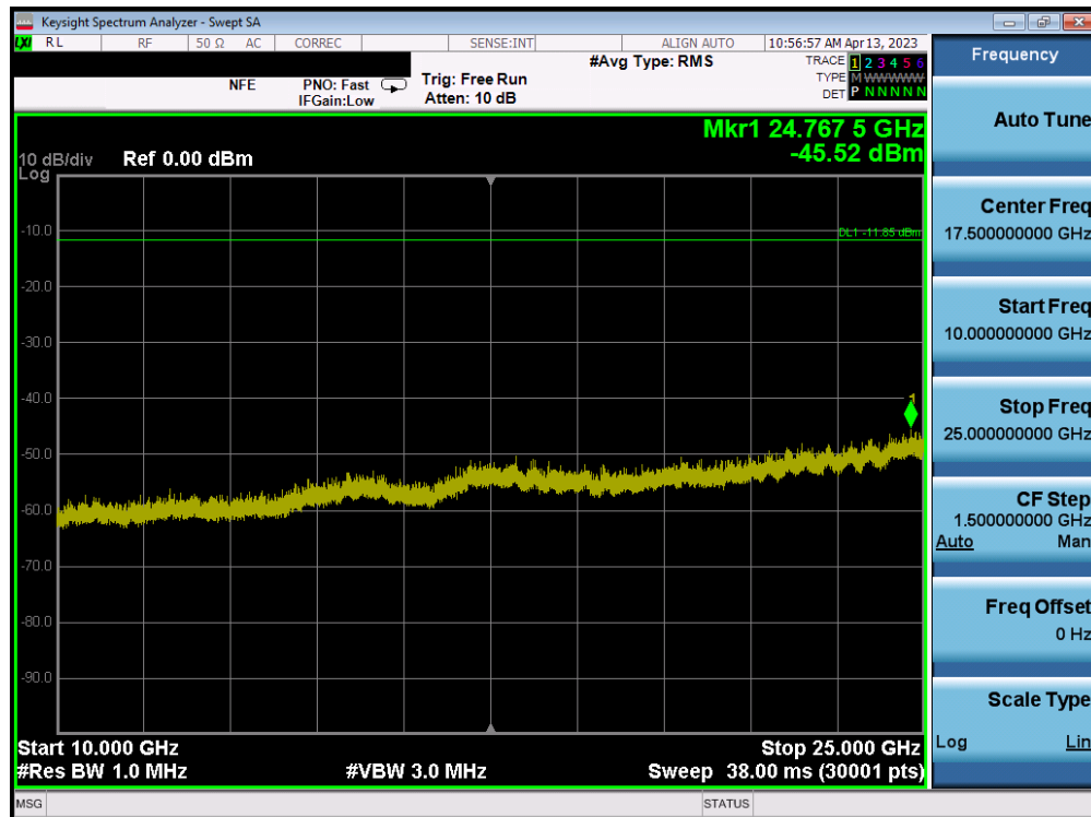
Plot 7-137. Conducted Spurious Plot SISO ANT2 (802.11b – Ch. 1)
