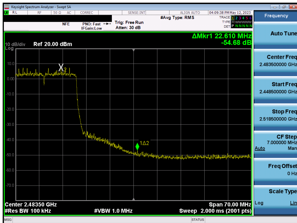
Plot 7-111. Band Edge Plot MIMO ANT1 (802.11ax (2.4GHz) – Ch. 10)
