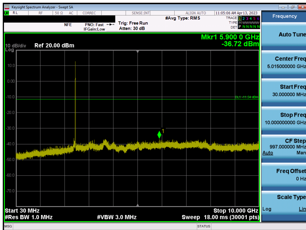
Plot 7-140. Conducted Spurious Plot SISO ANT2 (802.11b – Ch. 11)
