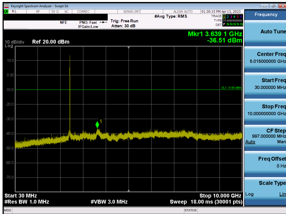
Plot 7-144. Conducted Spurious Plot MIMO ANT1 (802.11b – Ch. 6)
