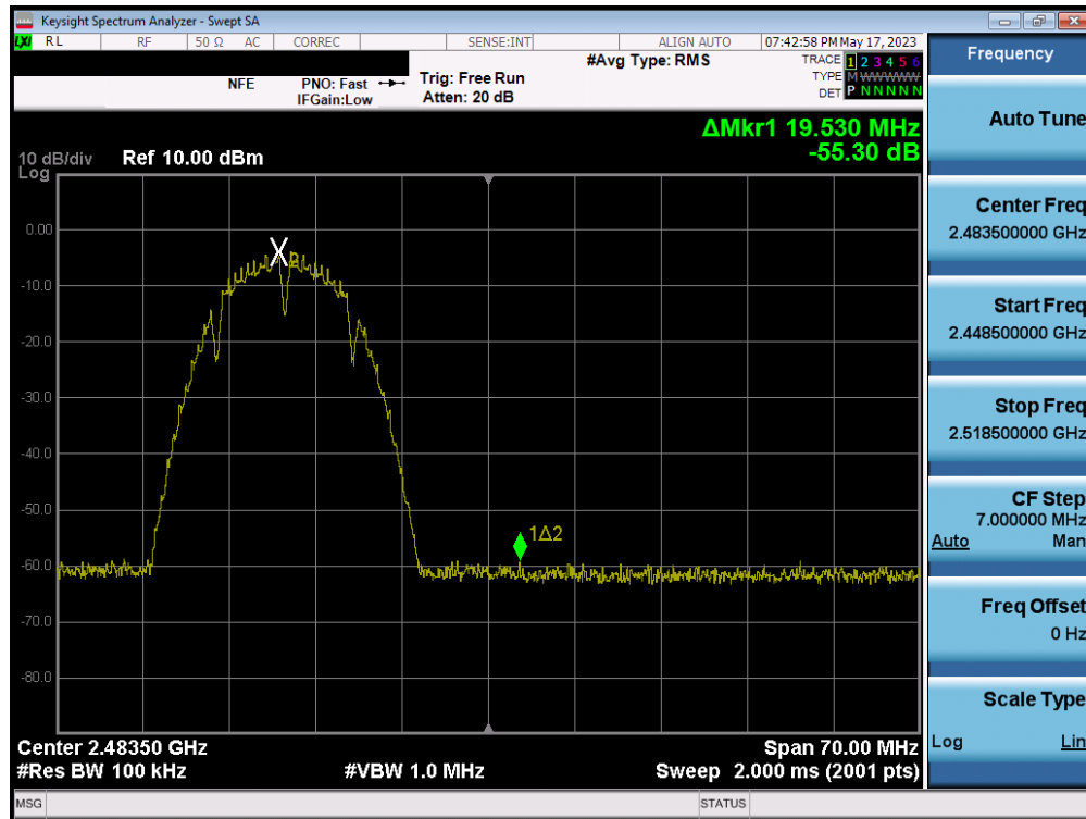
Plot 7-117. Band Edge Plot MIMO ANT2 (802.11b – Ch. 12)
