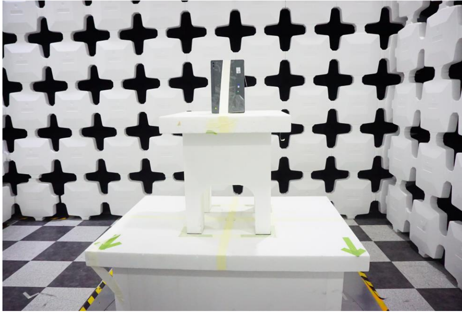
Figure 7. Test Setup – Z Position – 1GHz-18GHz
