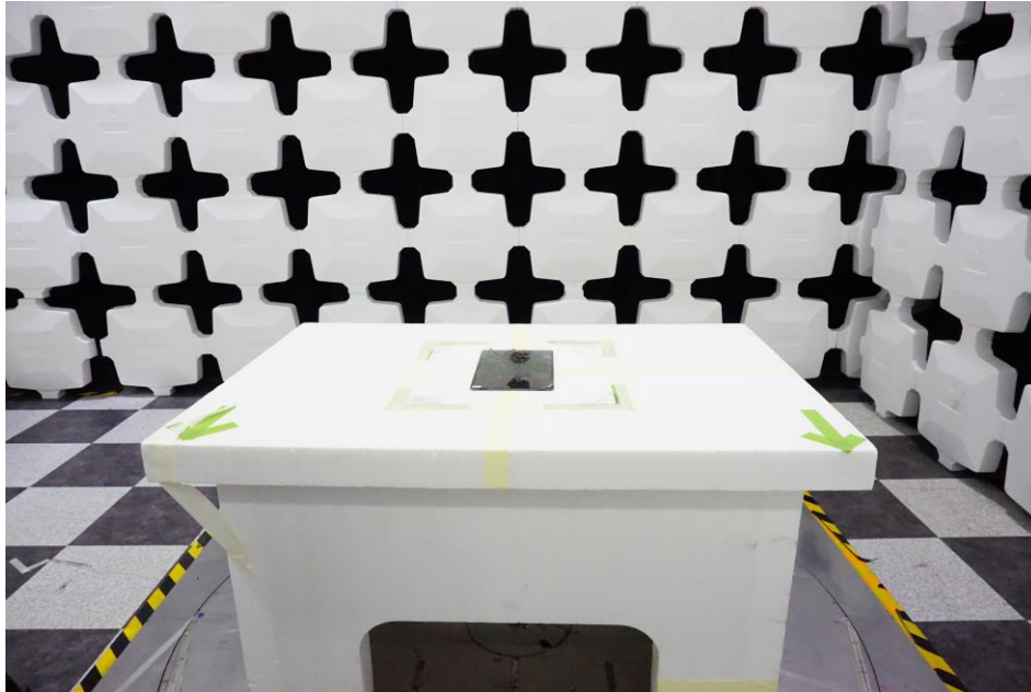
Figure 9. Test Setup – X Position – 30MHz-1GHz
