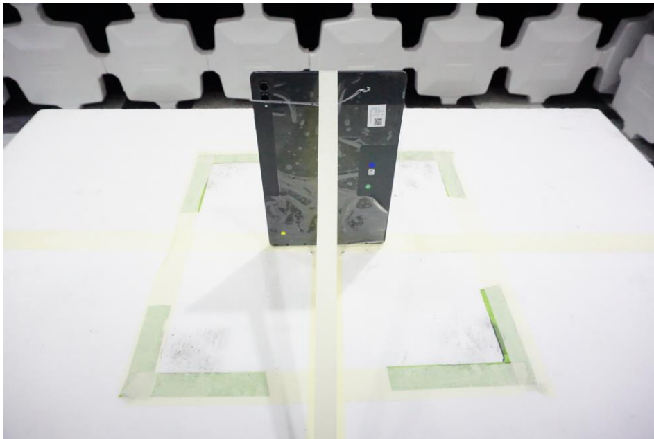
Figure 8. Test Setup – Z Position – 1GHz-18GHz
