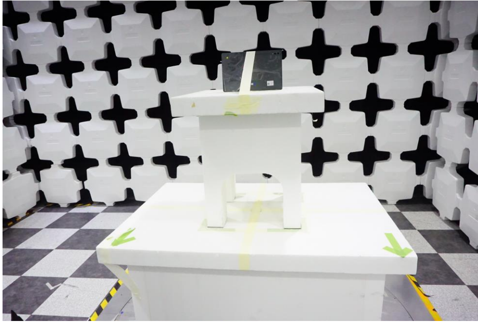
Figure 5. Test Setup – Y Position – 1GHz-18GHz
