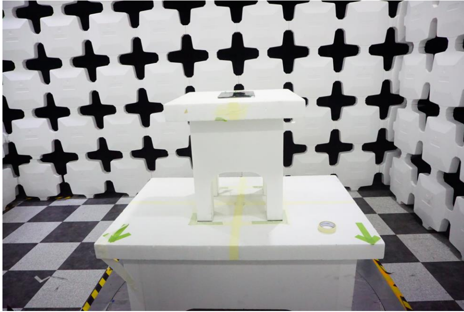
Figure 3. Test Setup – X Position – 1GHz-18GHz
