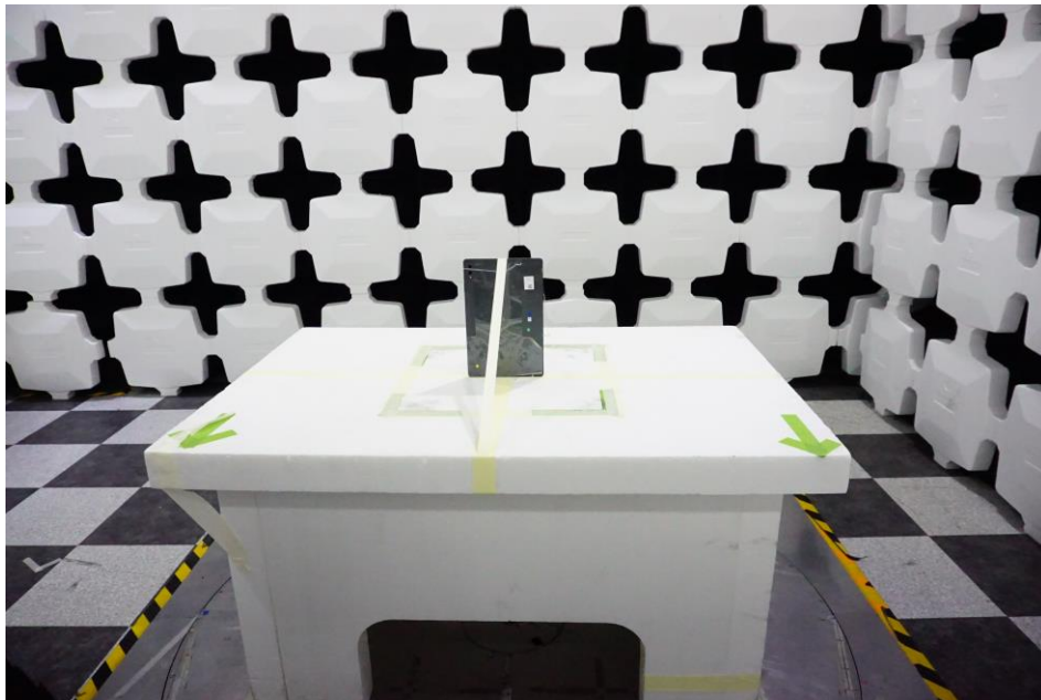
Figure 11. Test Setup – Z Position – 30MHz-1GHz
