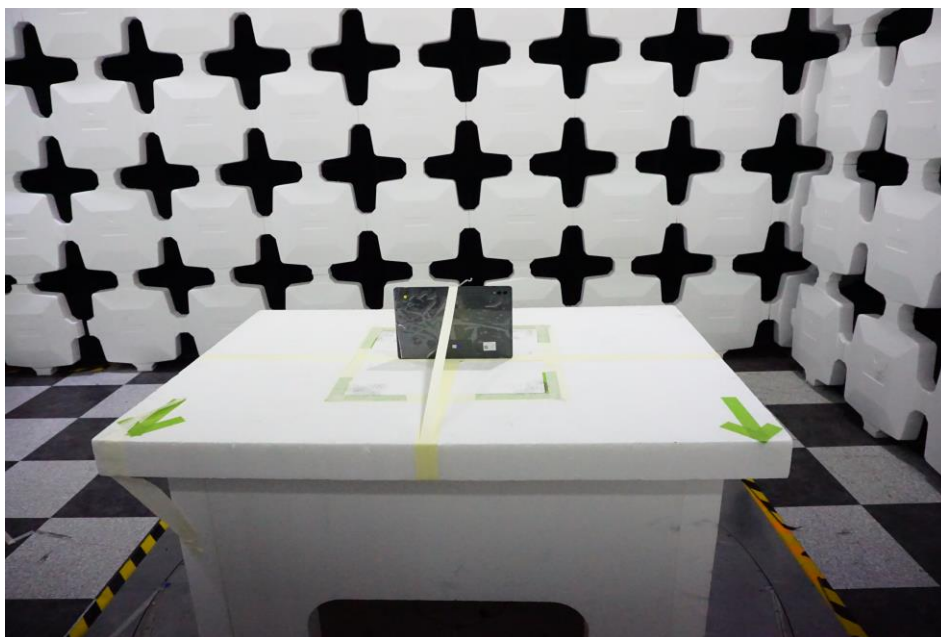
Figure 10. Test Setup – Y Position – 30MHz-1GHz
