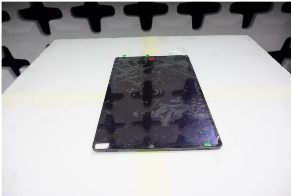
Figure 4. Test Setup – X Position – 1GHz-18GHz
