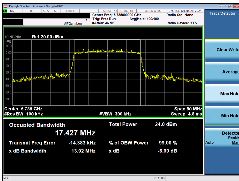
Plot 7-62. 6dB Bandwidth Plot MIMO ANT1 (20MHz BW 802.11n (UNII Band 3) – Ch. 157)
