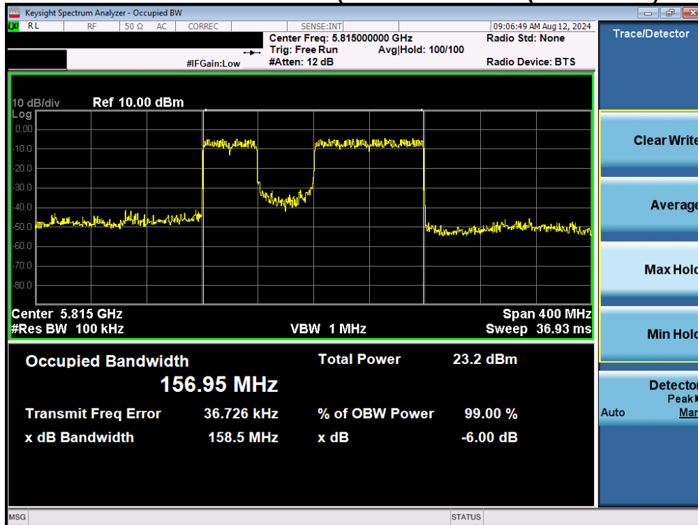
Plot 7-95. 6dB Bandwidth Plot MIMO ANT1 (160MHz BW 802.11be (UNII Band 3/4) – Ch. 163)
