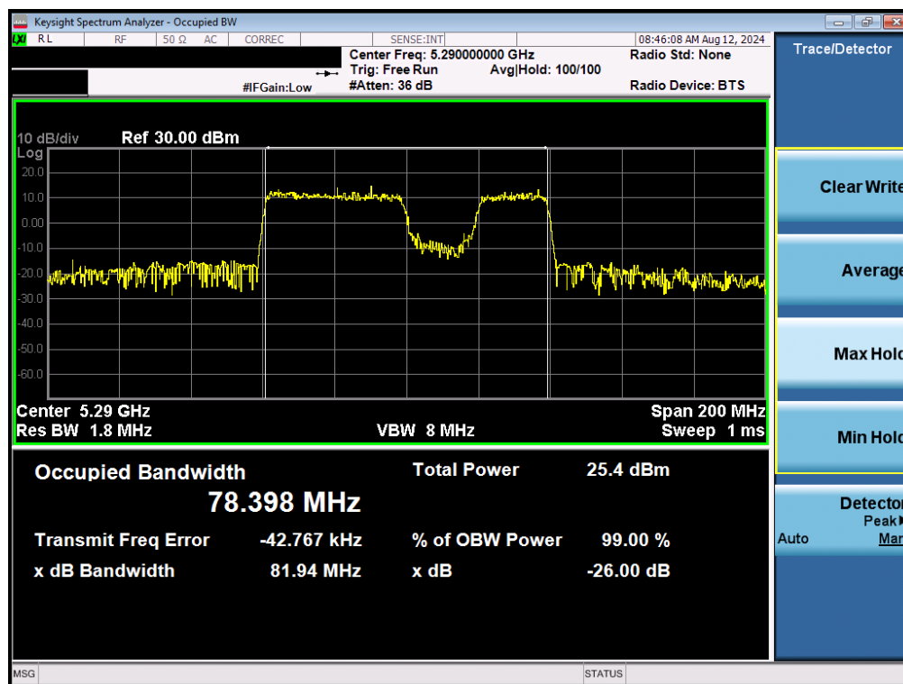
Plot 7-53. 26dB Bandwidth Plot MIMO ANT1 (80MHz BW 802.11be (UNII Band 2A) – Ch. 58)
