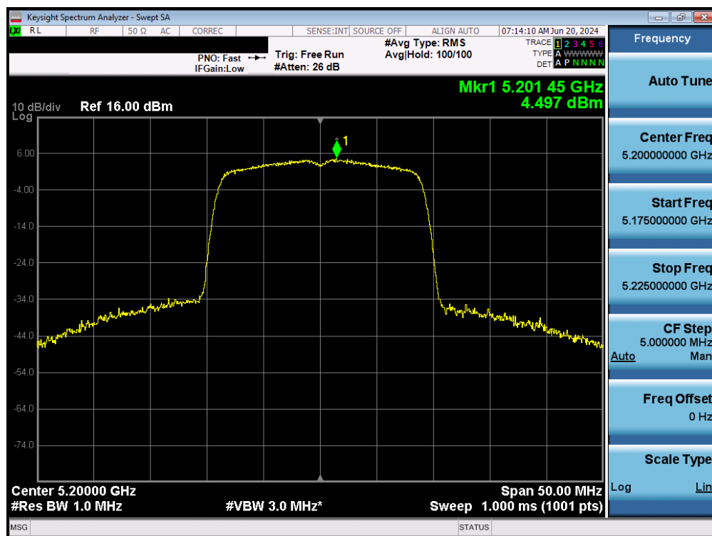
Plot 7-100. Power Spectral Density Plot MIMO ANT1 (20MHz BW 802.11n (UNII Band 1) – Ch. 40)
