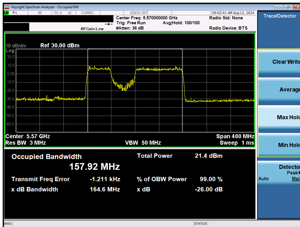
Plot 7-55 26dB Bandwidth Plot MIMO ANT1 (160MHz BW 802.11be (UNII Band 2C) – Ch. 114)
