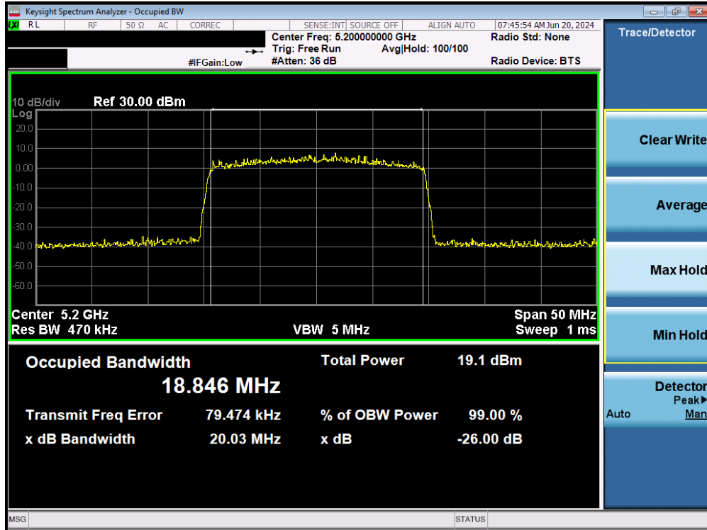
Plot 7-3. 26dB Bandwidth Plot MIMO ANT1 (20MHz BW 802.11be) - Ch. 40)
