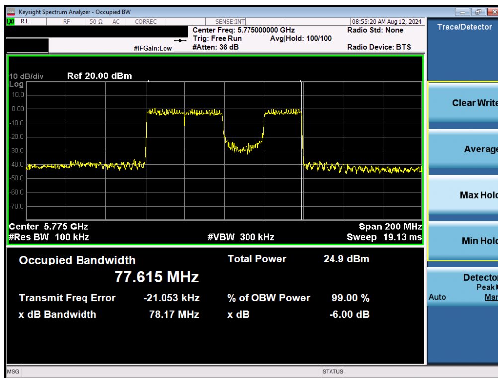
Plot 7-93. 6dB Bandwidth Plot MIMO ANT1 (80MHz BW 802.11be (UNII Band 3) – Ch. 155)
