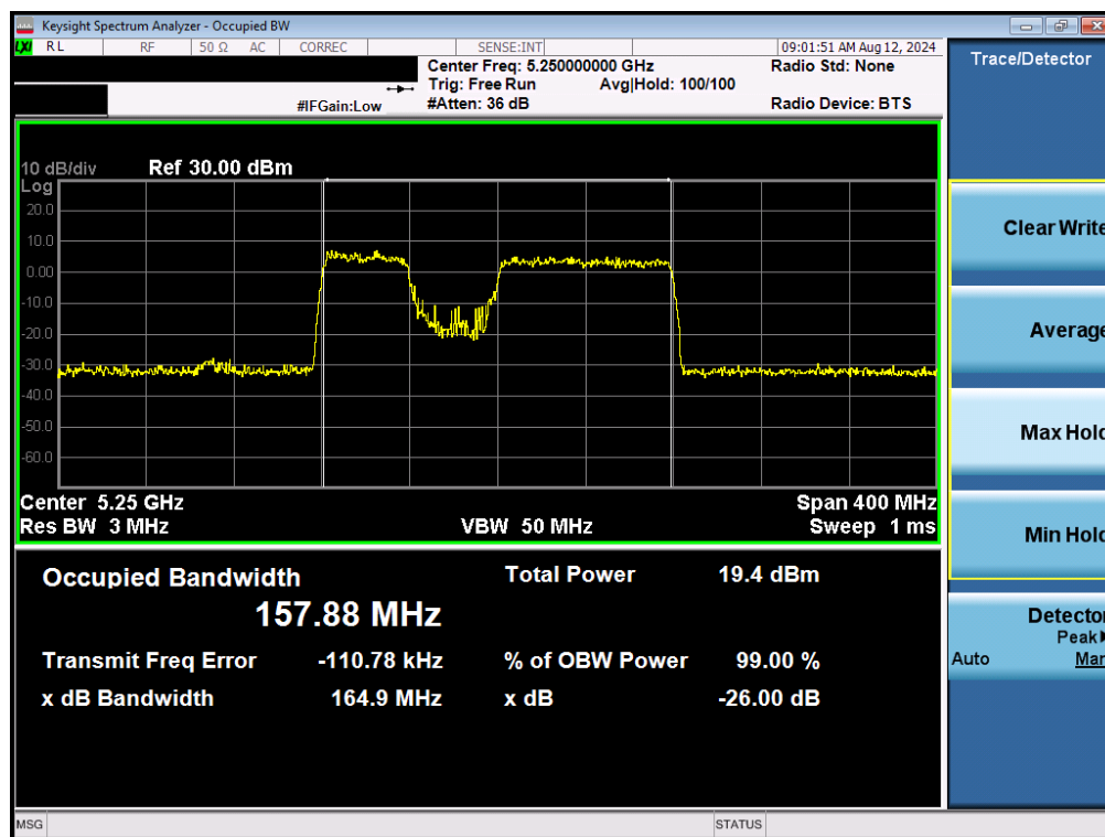
Plot 7-52. 26dB Bandwidth Plot MIMO ANT1 (160MHz BW 802.11be (UNII Band 1/2A) – Ch. 50)
