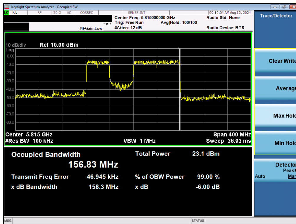
Plot 7-98. 6dB Bandwidth Plot MIMO ANT2 (160MHz BW 802.11be (UNII Band 3/4) – Ch. 163)
