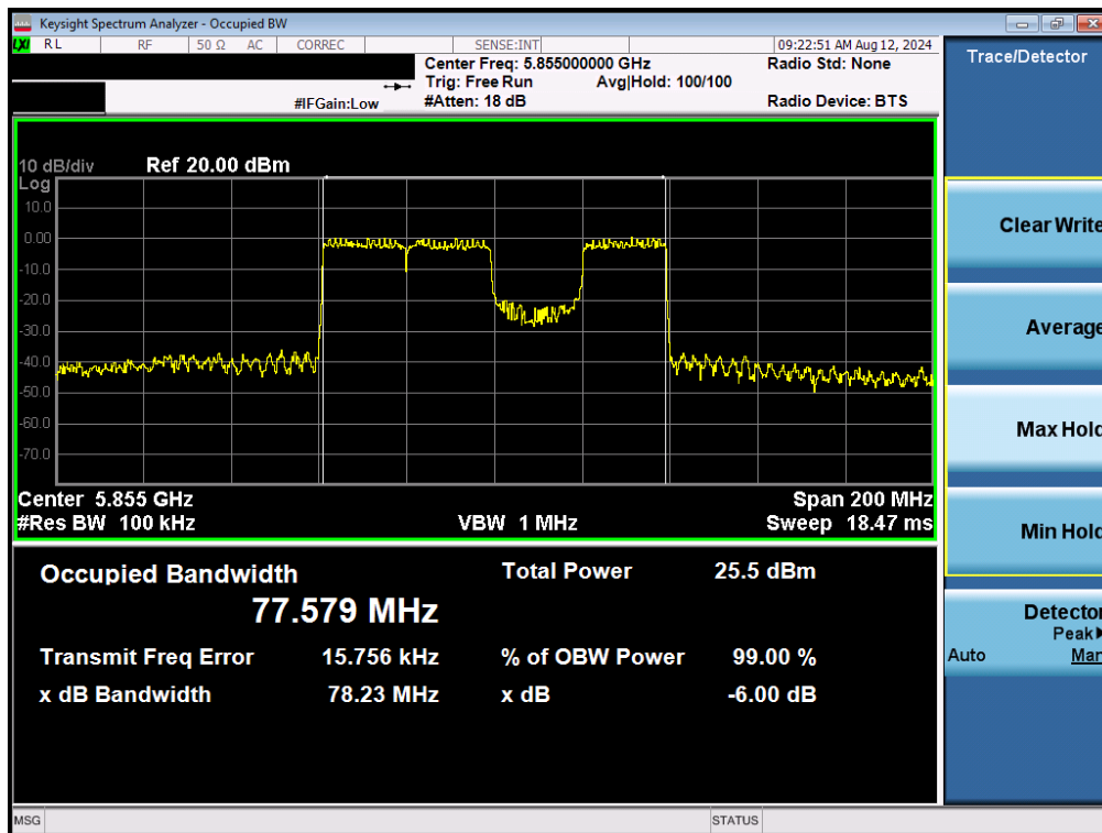
Plot 7-97. 6dB Bandwidth Plot MIMO ANT2 (80MHz BW 802.11be (UNII Band 3/4) – Ch. 171)
