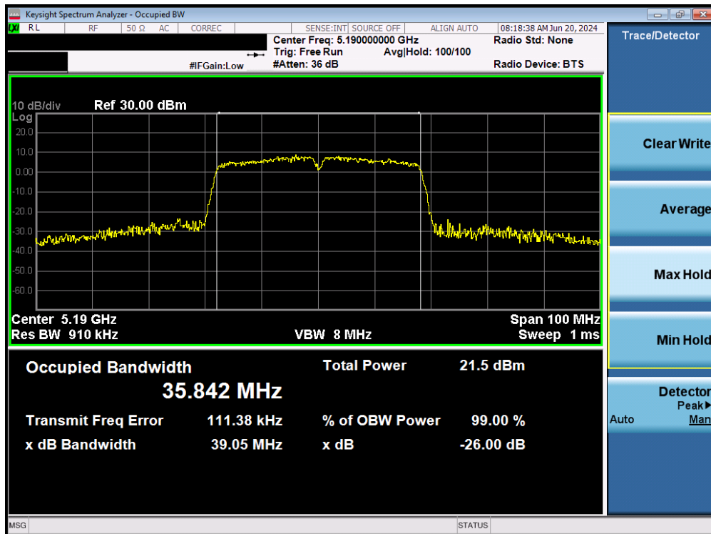
Plot 7-4. 26dB Bandwidth Plot MIMO ANT1 (40MHz BW 802.11n) - Ch. 38)
