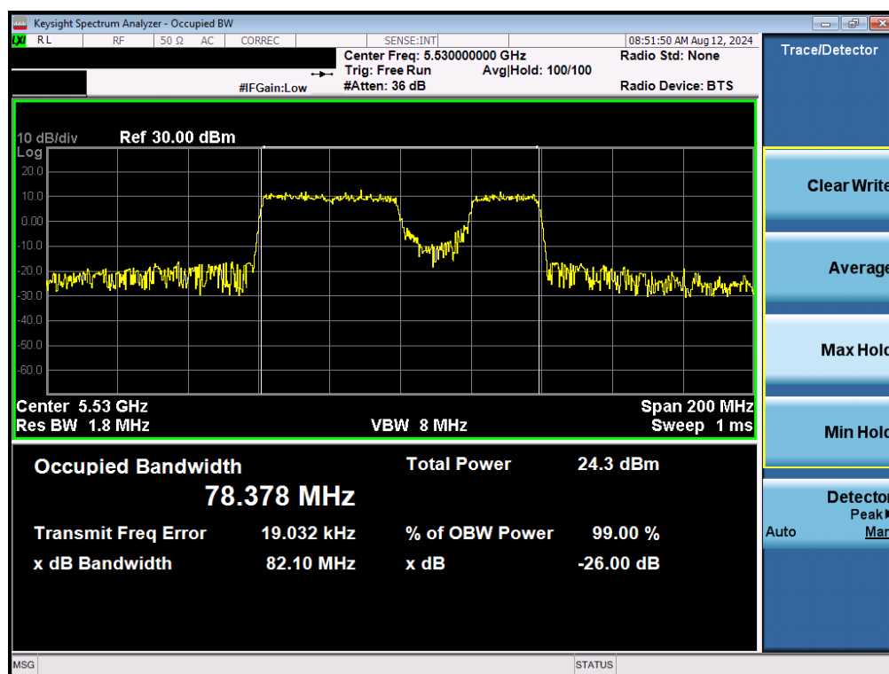
Plot 7-59. 26dB Bandwidth Plot MIMO ANT2 (80MHz BW 802.11be (UNII Band 2C) – Ch. 106)
