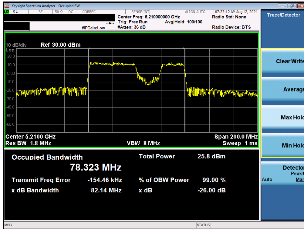
Plot 7-56. 26dB Bandwidth Plot MIMO ANT2 (80MHz BW 802.11be (UNII Band 1) – Ch. 42)
