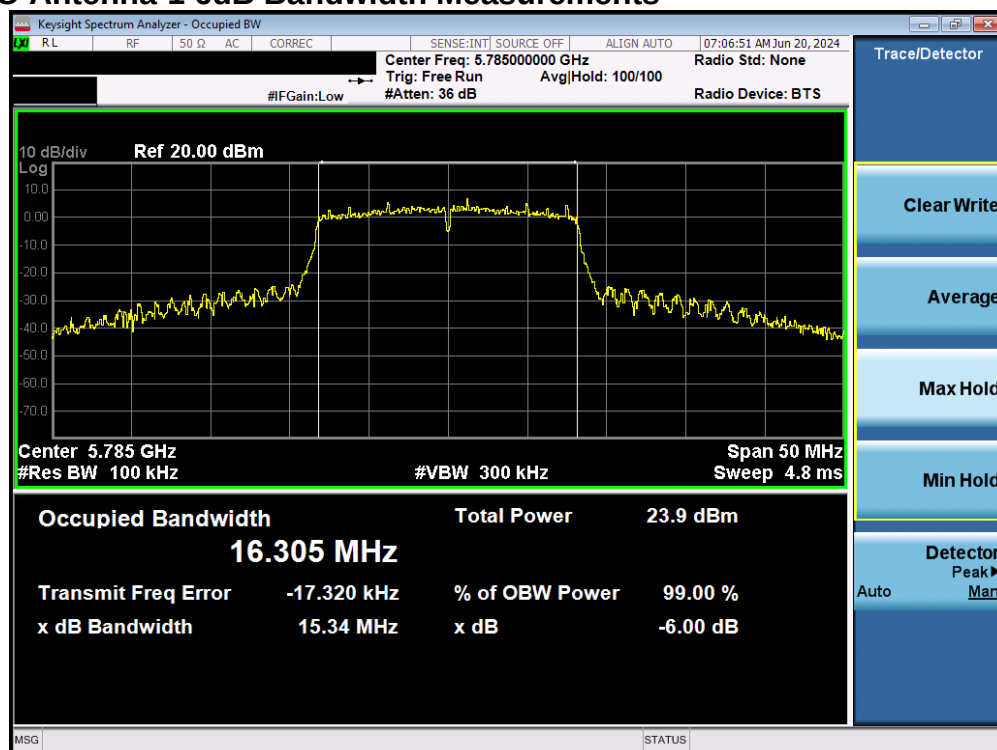
Plot 7-61. 6dB Bandwidth Plot MIMO ANT1 (802.11a (UNII Band 3) – Ch. 157)
