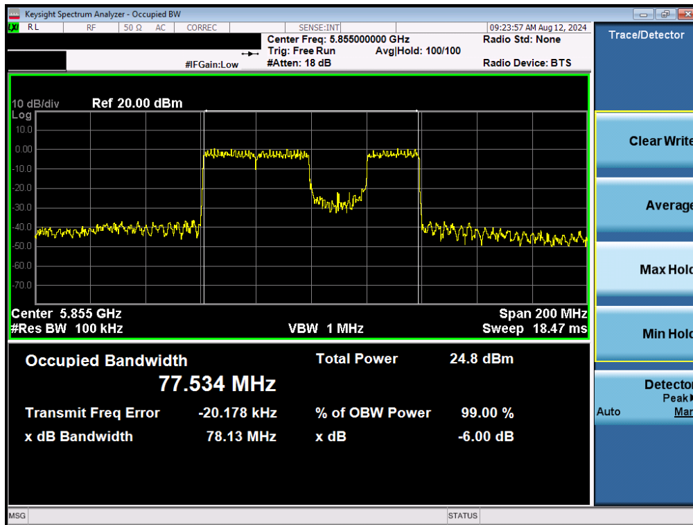
Plot 7-94. 6dB Bandwidth Plot MIMO ANT1 (80MHz BW 802.11be (UNII Band 3/4) – Ch. 171)
