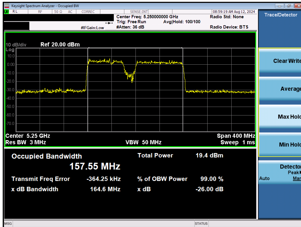
Plot 7-57. 26dB Bandwidth Plot MIMO ANT2 (160MHz BW 802.11be (UNII Band 1/2A) – Ch. 50)
