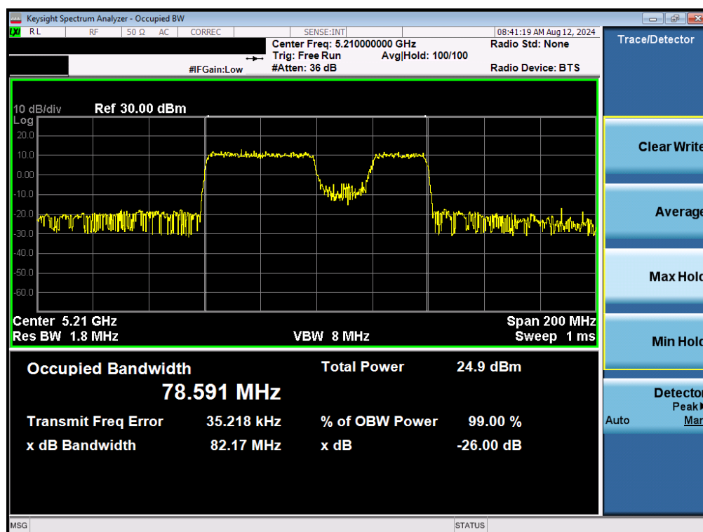
Plot 7-51. 26dB Bandwidth Plot MIMO ANT1 (80MHz BW 802.11be (UNII Band 1) – Ch. 42)
