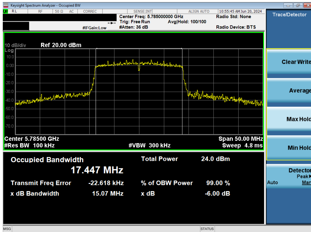
Plot 7-78. 6dB Bandwidth Plot MIMO ANT2 (20MHz BW 802.11n (UNII Band 3) – Ch. 157)
