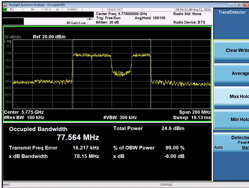
Plot 7-96. 6dB Bandwidth Plot MIMO ANT2 (80MHz BW 802.11be (UNII Band 3) – Ch. 155)
