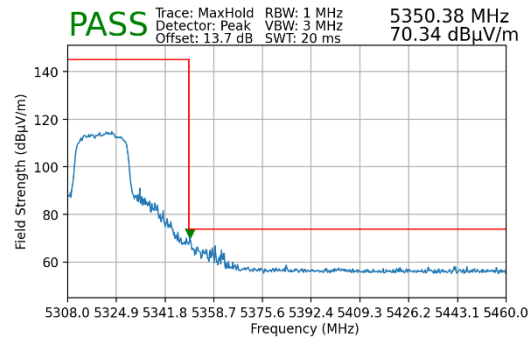
Plot 7-208. Radiated Upper Band Edge Plot MIMO (Peak – UNII Band 2A)
