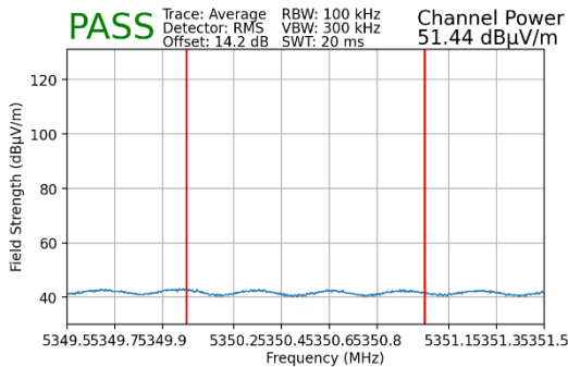
Plot 7-227. Radiated Upper Band Edge Plot MIMO (Average – UNII Band 2A)
