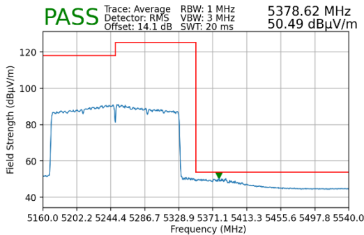
Plot 7-237. Radiated Upper Band Edge Plot MIMO (Average – UNII Band 2A)
