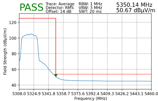
Plot 7-207. Radiated Upper Band Edge Plot MIMO (Average – UNII Band 2A)
