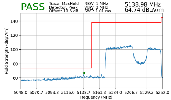
Plot 7-226. Radiated Lower Band Edge Plot MIMO (Peak – UNII Band 1)
