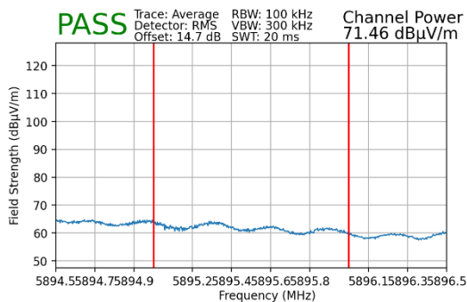
Plot 7-213. Radiated Upper Band Edge Plot MIMO (Average – UNII Band 4)
