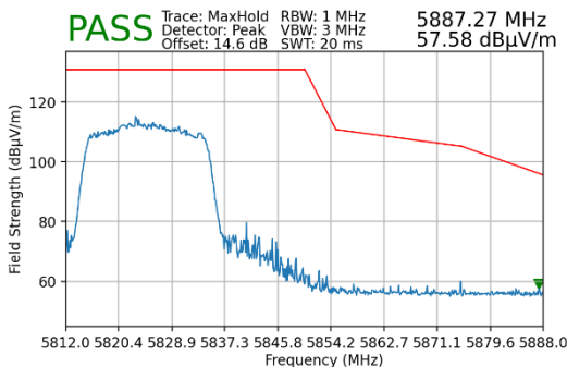
Plot 7-211. Radiated Upper Band Edge Plot MIMO (Peak – UNII Band 3)
