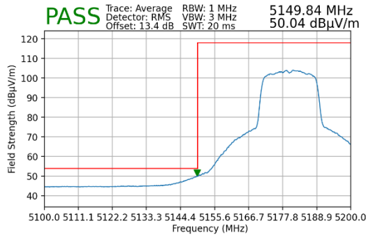
Plot 7-205. Radiated Lower Band Edge Plot MIMO (Average – UNII Band 1)
