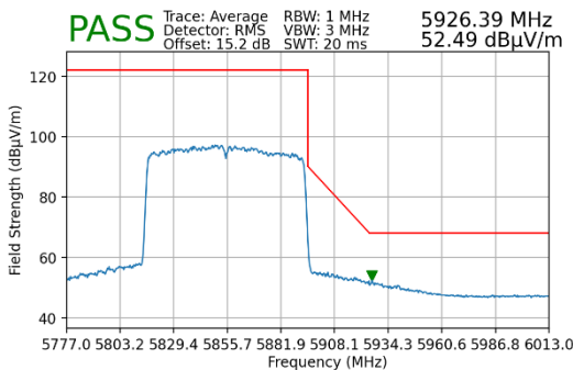
Plot 7-233. Radiated Upper Band Edge Plot MIMO (Average – UNII Band 4)
