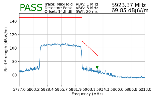
Plot 7-234. Radiated Upper Band Edge Plot MIMO (Peak – UNII Band 4)
