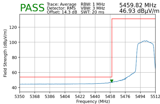
Plot 7-209. Radiated Lower Band Edge Plot MIMO (Average – UNII Band 2C)
