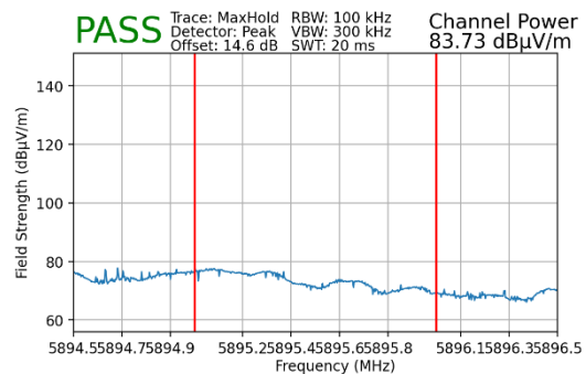
Plot 7-214. Radiated Upper Band Edge Plot MIMO (Peak – UNII Band 4)
