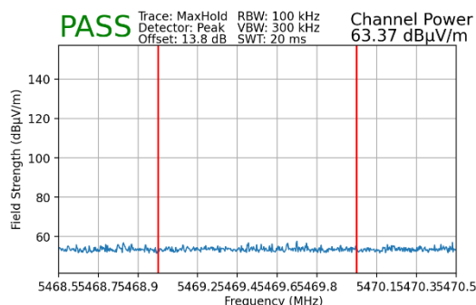
Plot 7-230. Radiated Lower Band Edge Plot MIMO (Peak – UNII Band 2C)
