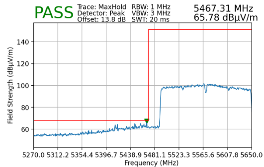
Plot 7-240. Radiated Lower Band Edge Plot MIMO (Peak – UNII Band 2C)
