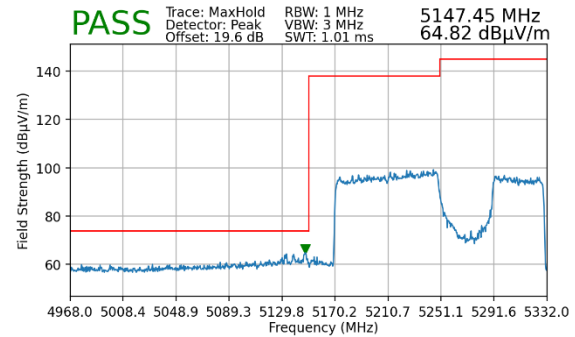
Plot 7-236. Radiated Lower Band Edge Plot MIMO (Peak – UNII Band 1)
