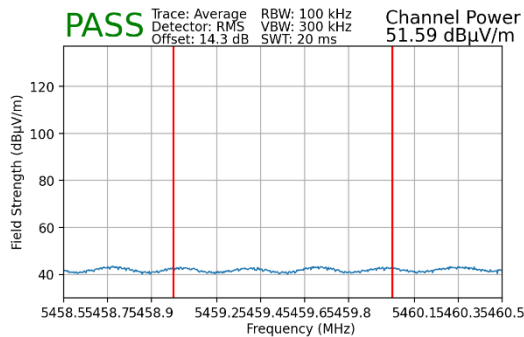
Plot 7-239. Radiated Lower Band Edge Plot MIMO (Average – UNII Band 2C)
