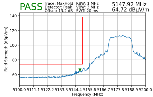
Plot 7-206. Radiated Lower Band Edge Plot MIMO (Peak – UNII Band 1)
