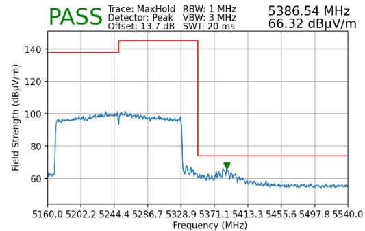
Plot 7-238. Radiated Upper Band Edge Plot MIMO (Peak – UNII Band 2A)
