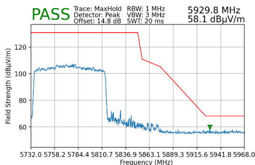
Plot 7-231. Radiated Upper Band Edge Plot MIMO (Peak – UNII Band 3)
