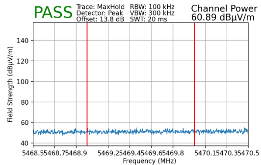
Plot 7-210. Radiated Lower Band Edge Plot MIMO (Peak – UNII Band 2C)
