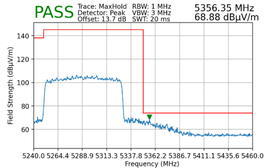
Plot 7-228. Radiated Upper Band Edge Plot MIMO (Peak – UNII Band 2A)
