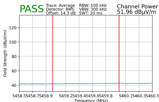
Plot 7-229. Radiated Lower Band Edge Plot MIMO (Average – UNII Band 2C)
