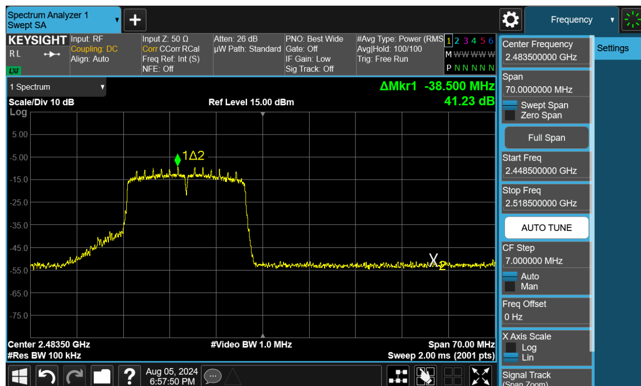
Plot 7-140. Band Edge Plot MIMO ANT1 (802.11n (2.4GHz) – Ch. 13)
