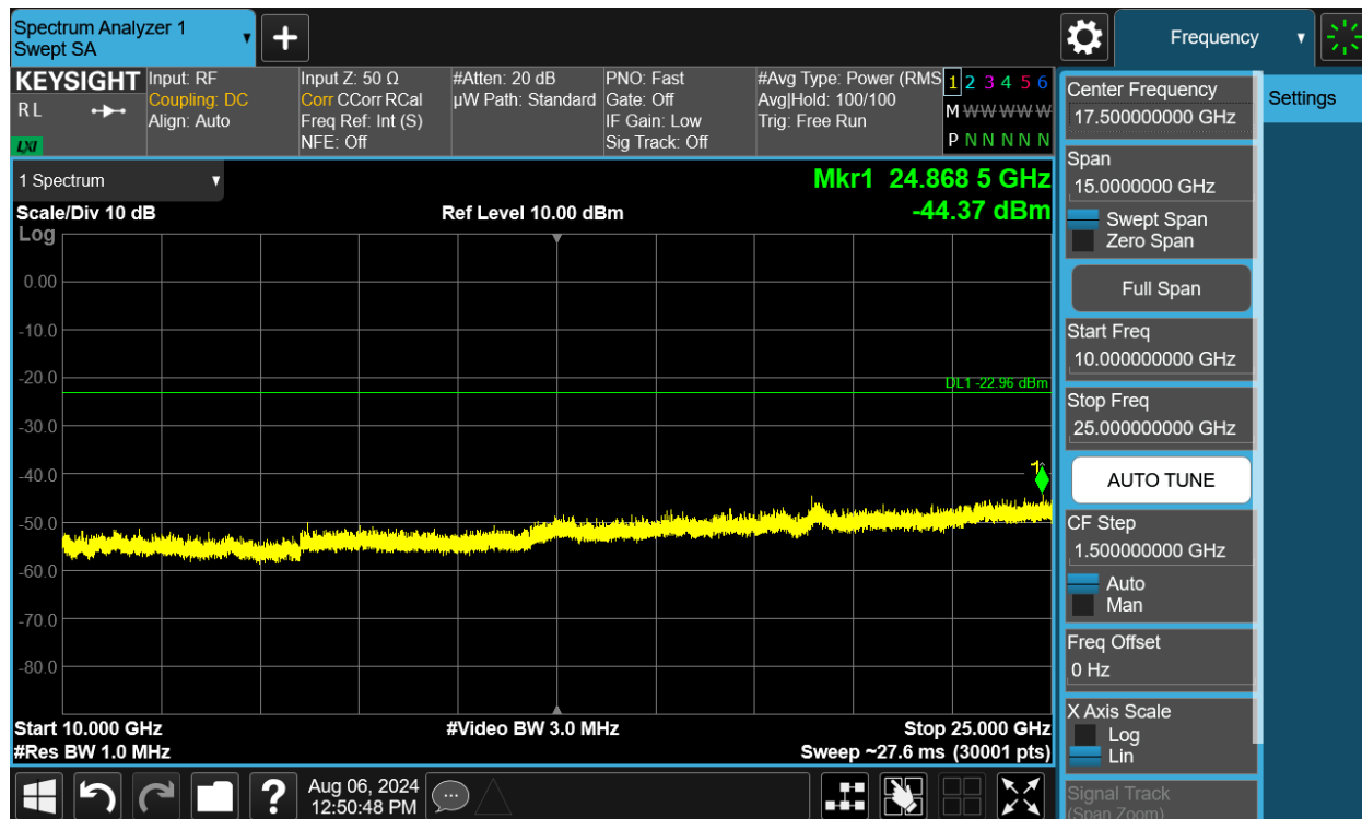
Plot 7-168. Conducted Spurious Plot SISO ANT2 (802.11b – Ch. 1)
