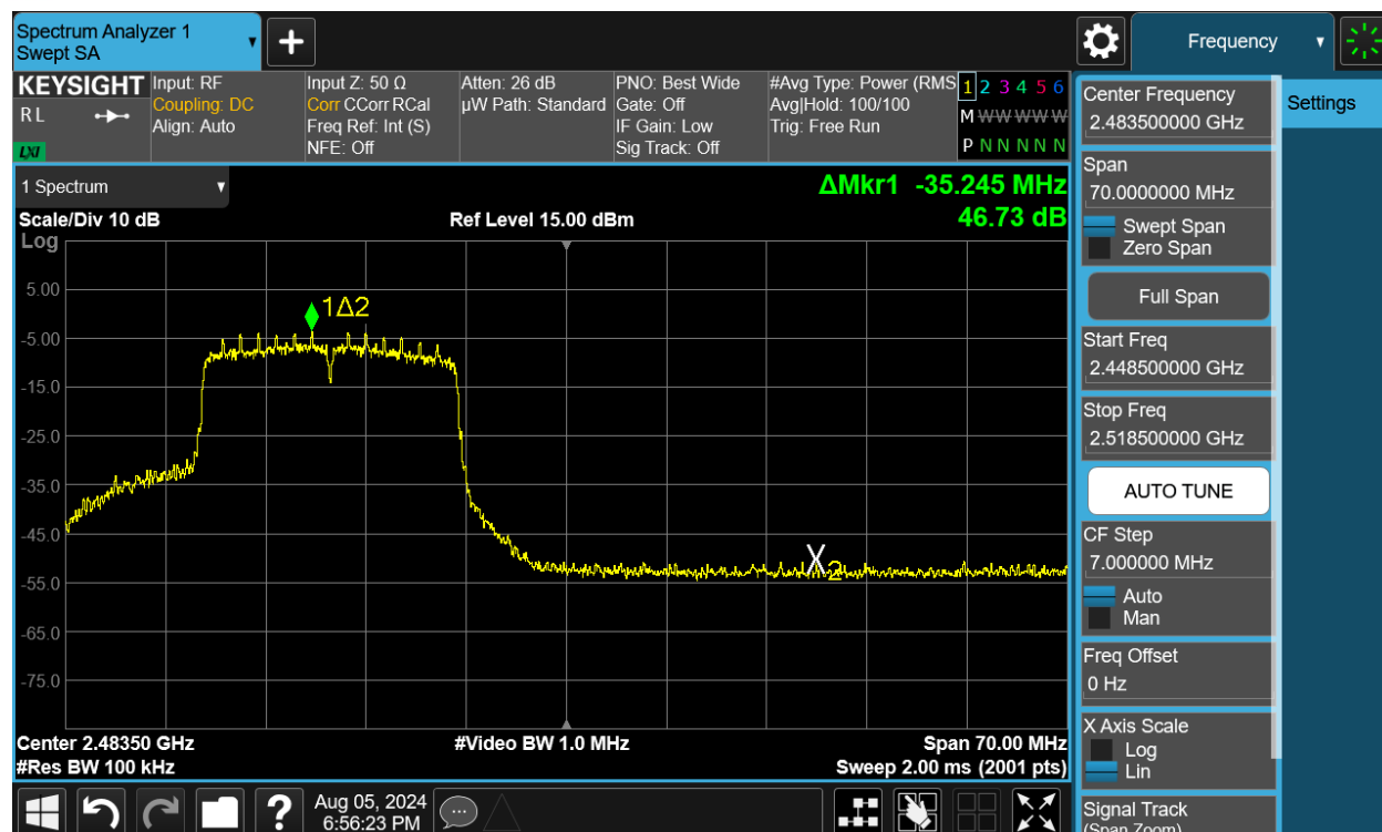
Plot 7-139. Band Edge Plot MIMO ANT1 (802.11n (2.4GHz) – Ch. 12)
