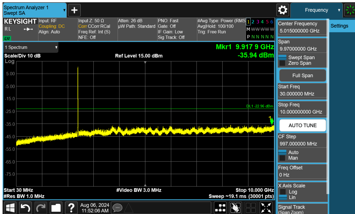
Plot 7-167. Conducted Spurious Plot SISO ANT2 (802.11b – Ch. 1)
