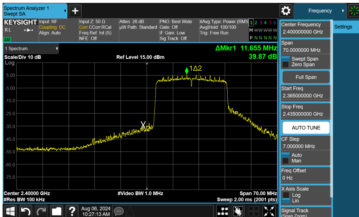
Plot 7-157. Band Edge Plot MIMO ANT2 (802.11be (2.4GHz) – Ch. 1)
