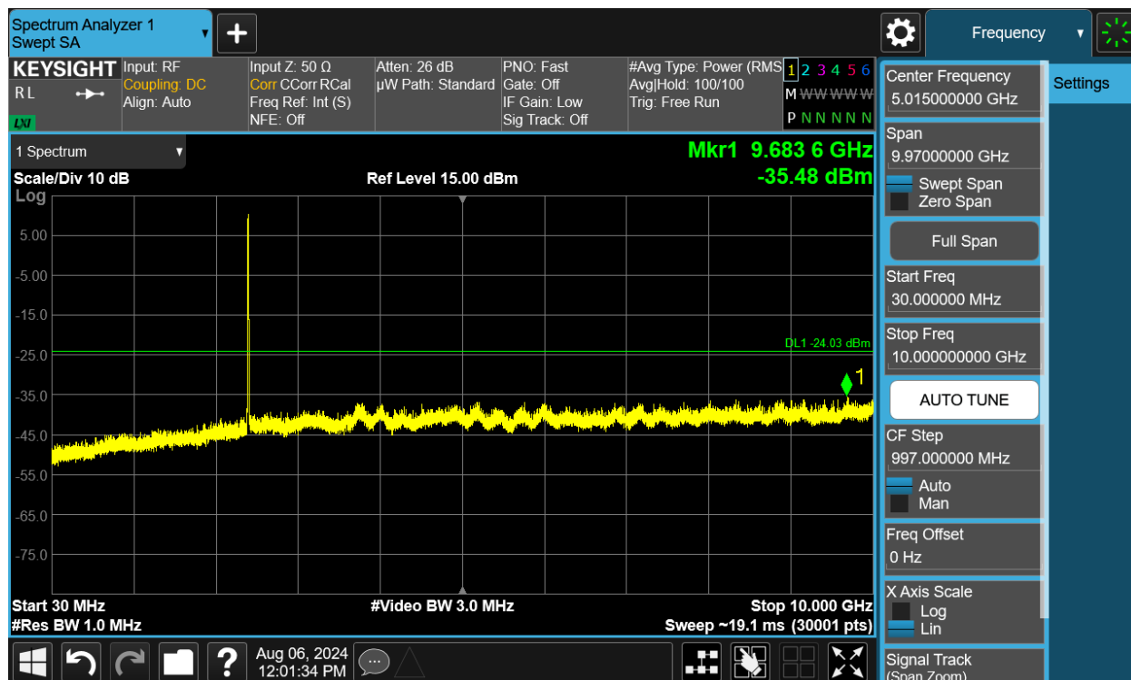
Plot 7-161. Conducted Spurious Plot SISO ANT1 (802.11b – Ch. 1)
