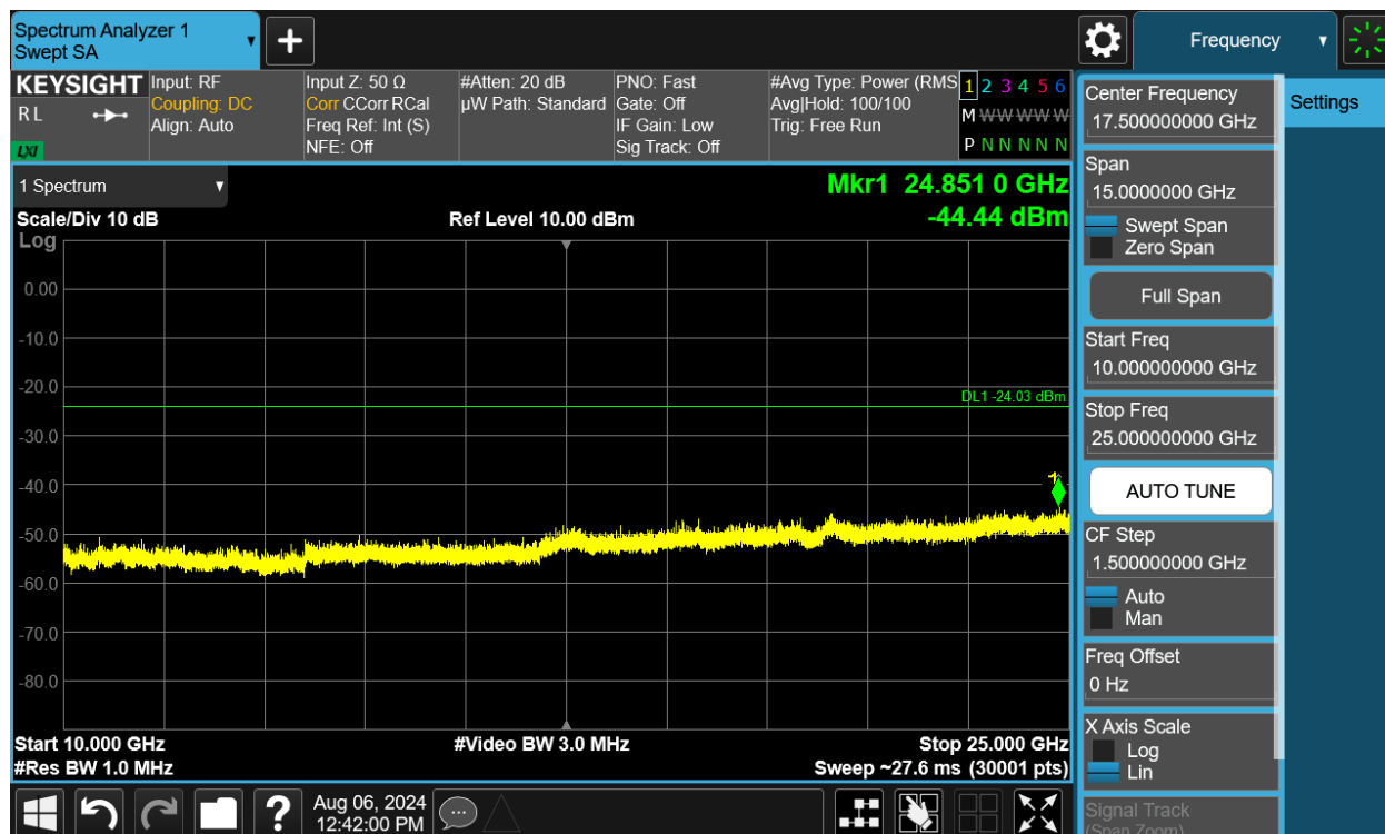
Plot 7-162. Conducted Spurious Plot SISO ANT1 (802.11b – Ch. 1)
