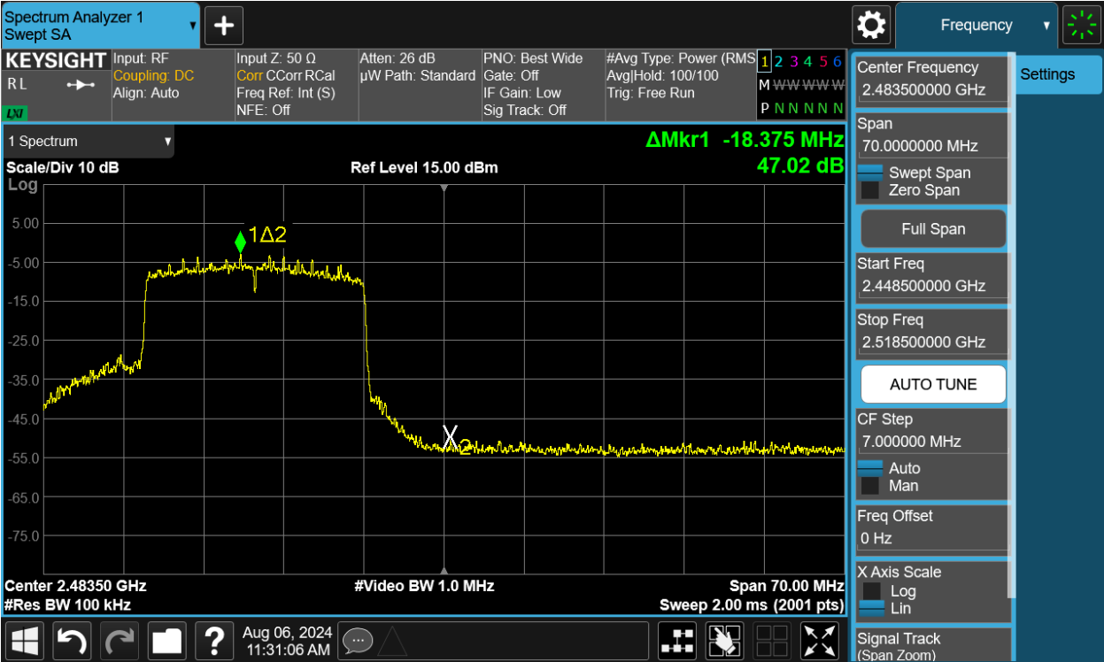
Plot 7-143. Band Edge Plot MIMO ANT1 (802.11be (2.4GHz) – Ch. 12)
