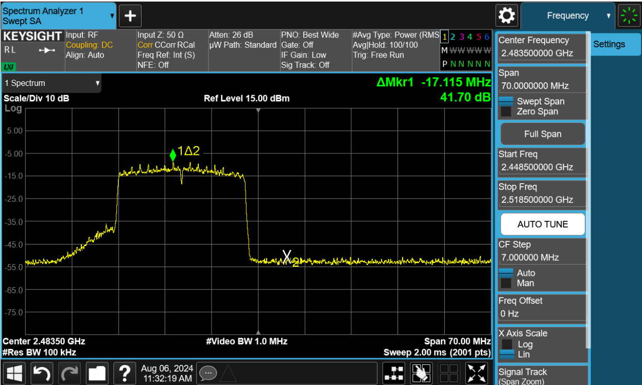
Plot 7-144. Band Edge Plot MIMO ANT1 (802.11be (2.4GHz) – Ch. 13)
