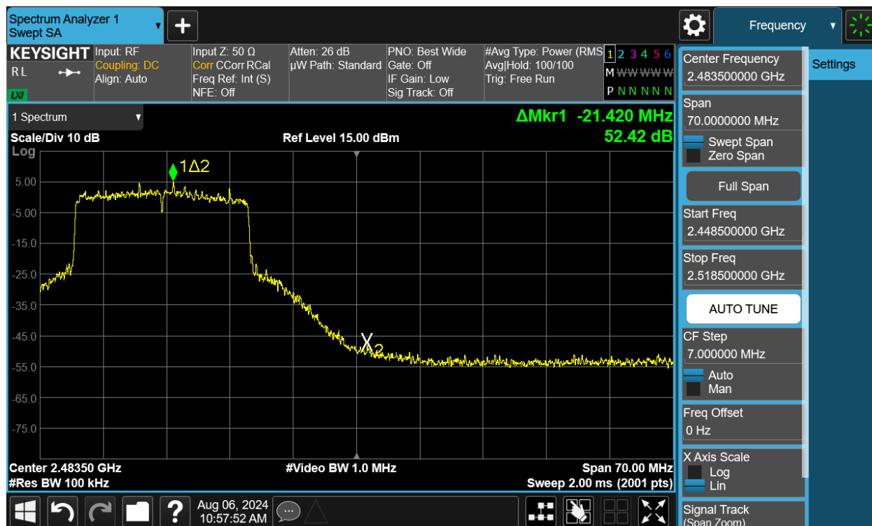
Plot 7-158. Band Edge Plot MIMO ANT2 (802.11be (2.4GHz) – Ch. 11)
