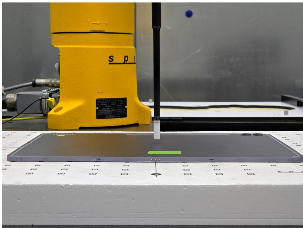
SAR Test Setup Photo 26 – Tablet, Back Side at 2 mm
