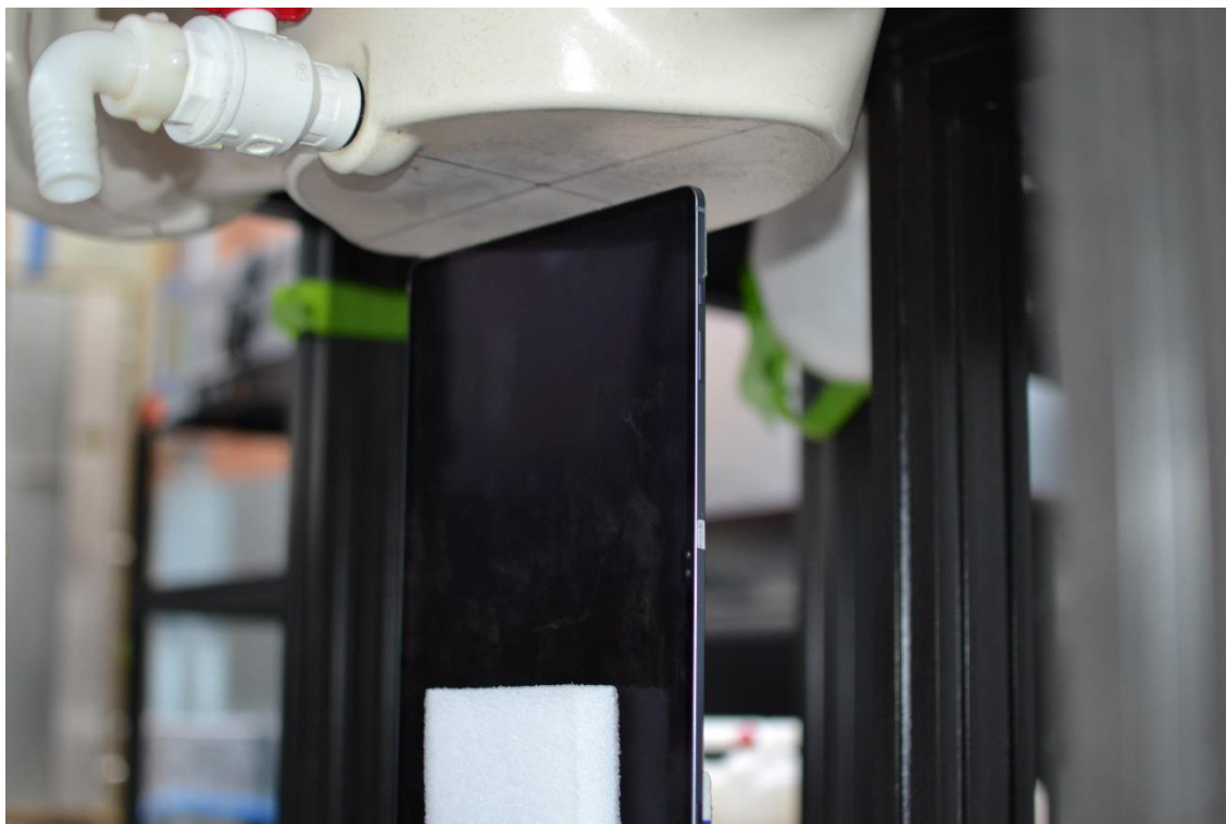
SAR Test Setup Photo 17 – Tablet, Top Edge at 19 mm – Antenna WIFI 1
