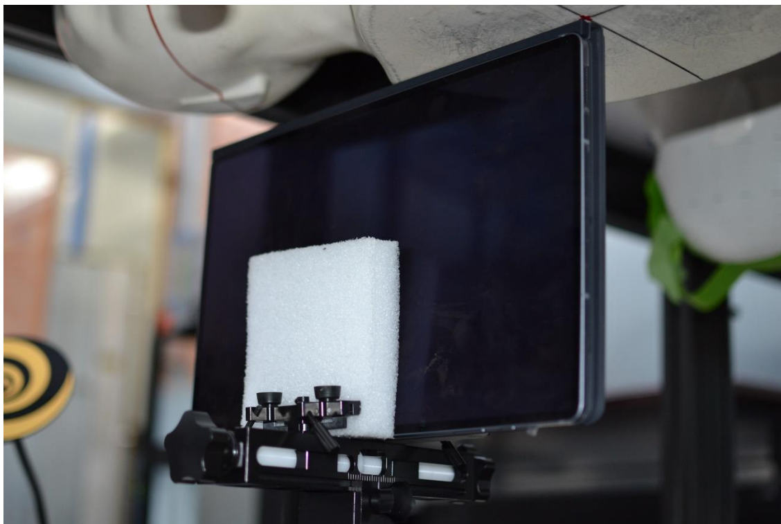
SAR Test Setup Photo 11 – Tablet with Keyboard Variant 1, Left Edge at 0 mm – Antenna WIFI 1, 2
