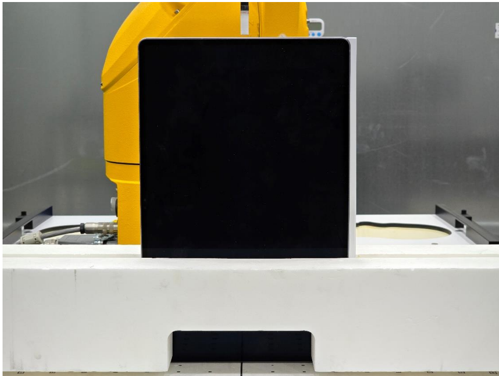
SAR Test Setup Photo 24 – Tablet with Keyboard Variant 1, Bottom Edge at 2 mm
