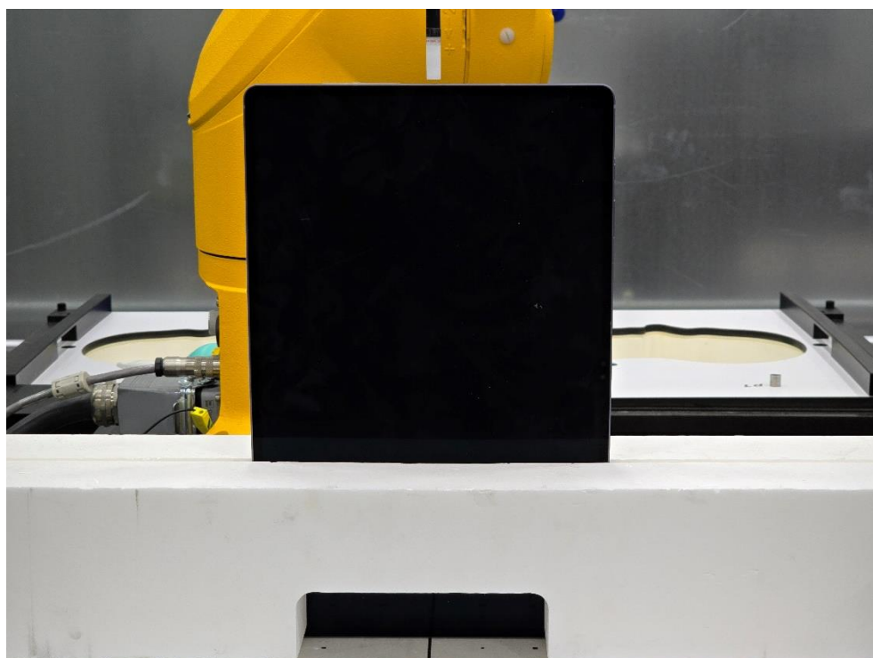
SAR Test Setup Photo 27 – Tablet, Top Edge at 2 mm
