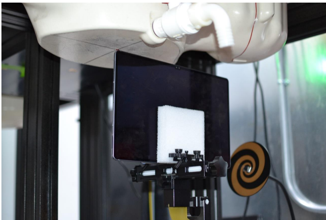
SAR Test Setup Photo 14 – Tablet, Right Edge at 0 mm – Antenna WIFI 1, 2
