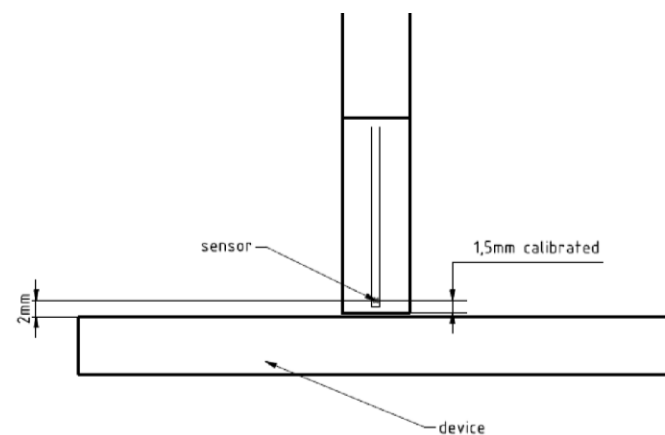
Figure I-4 EUmWVx Probe
