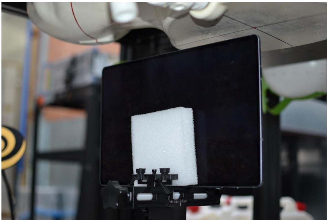
SAR Test Setup Photo 9 – Tablet, Left Edge at 9 mm – Antenna WIFI 1, 2
