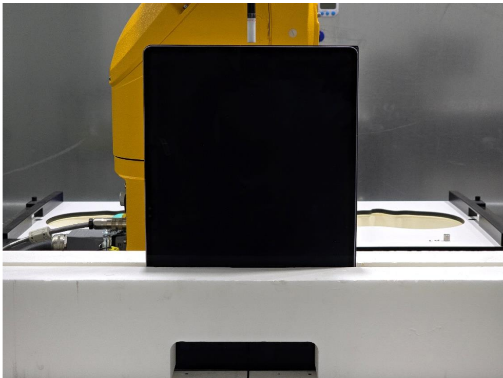
SAR Test Setup Photo 25 – Tablet with Keyboard Variant 2, Bottom Edge at 2 mm
