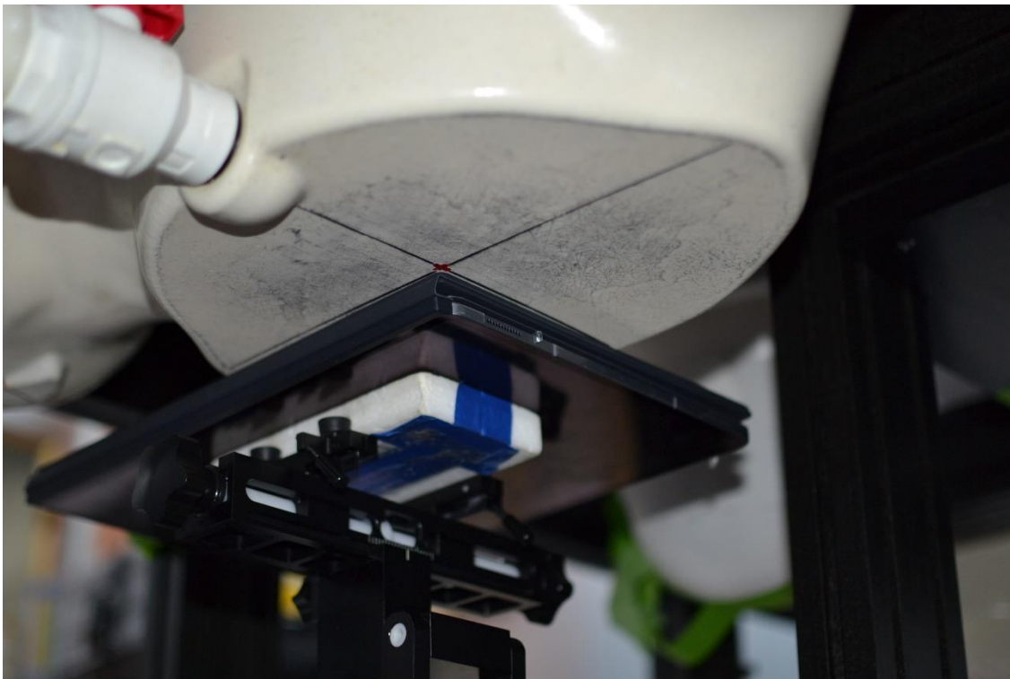
SAR Test Setup Photo 3 – Tablet with Keyboard Variant 1, Back Side at 0 mm – Antenna WIFI 1
