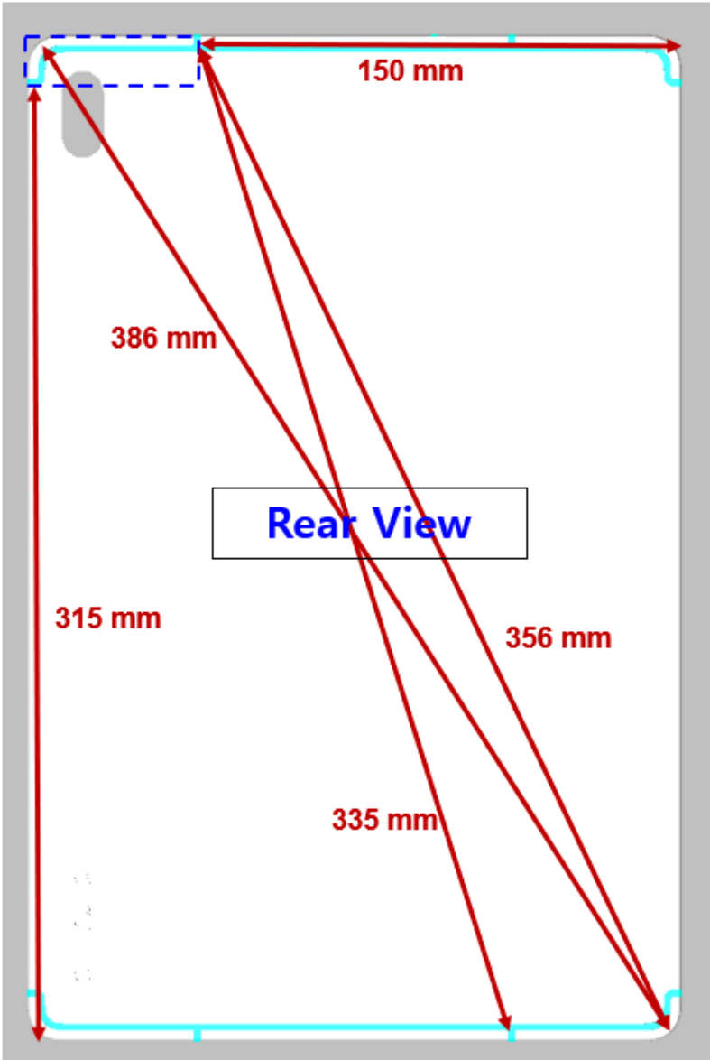
Figure I-2 DUT Dimensions
