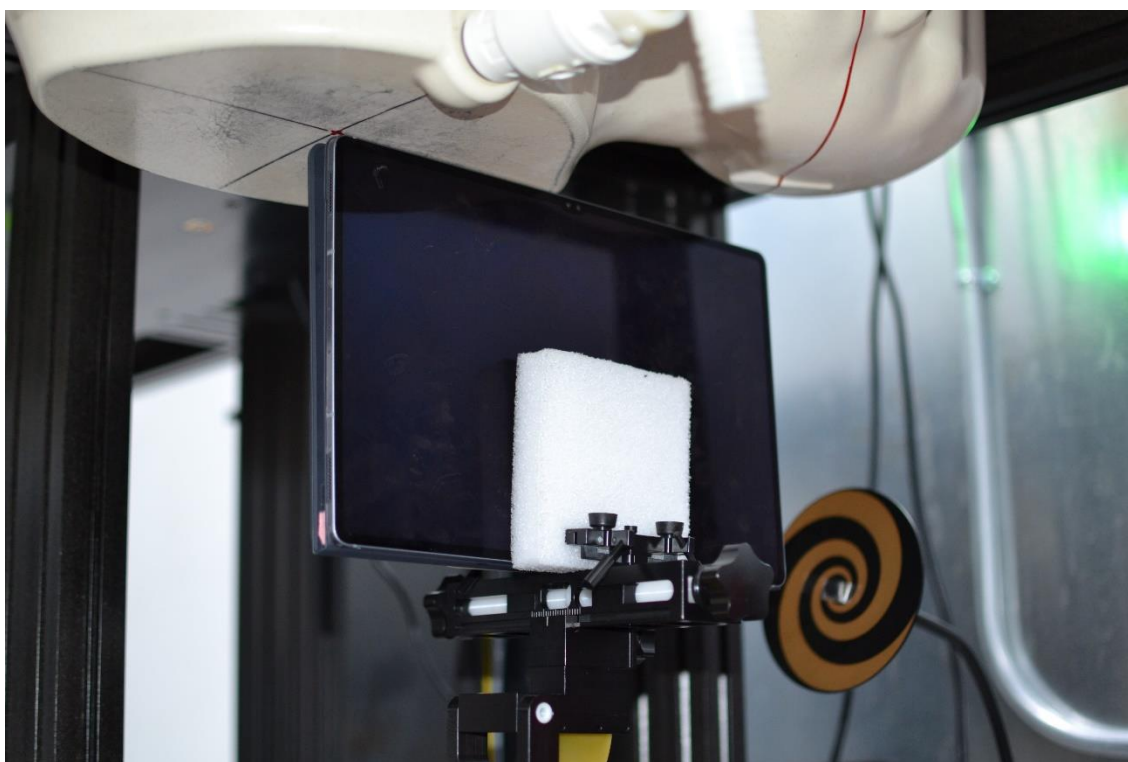
SAR Test Setup Photo 163 – Tablet with Keyboard Variant 2, Right Edge at 0 mm – Antenna WIFI 1, 2
