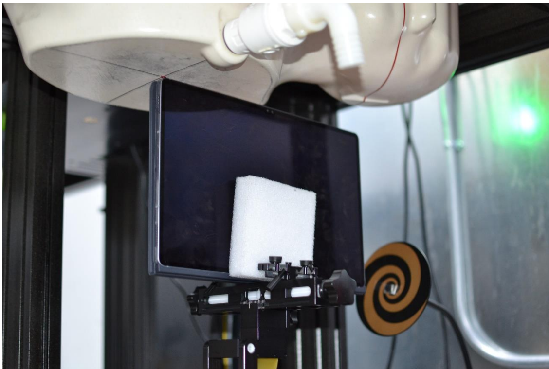
SAR Test Setup Photo 15 – Tablet with Keyboard Variant 1, Right Edge at 0 mm – Antenna WIFI 1, 2
