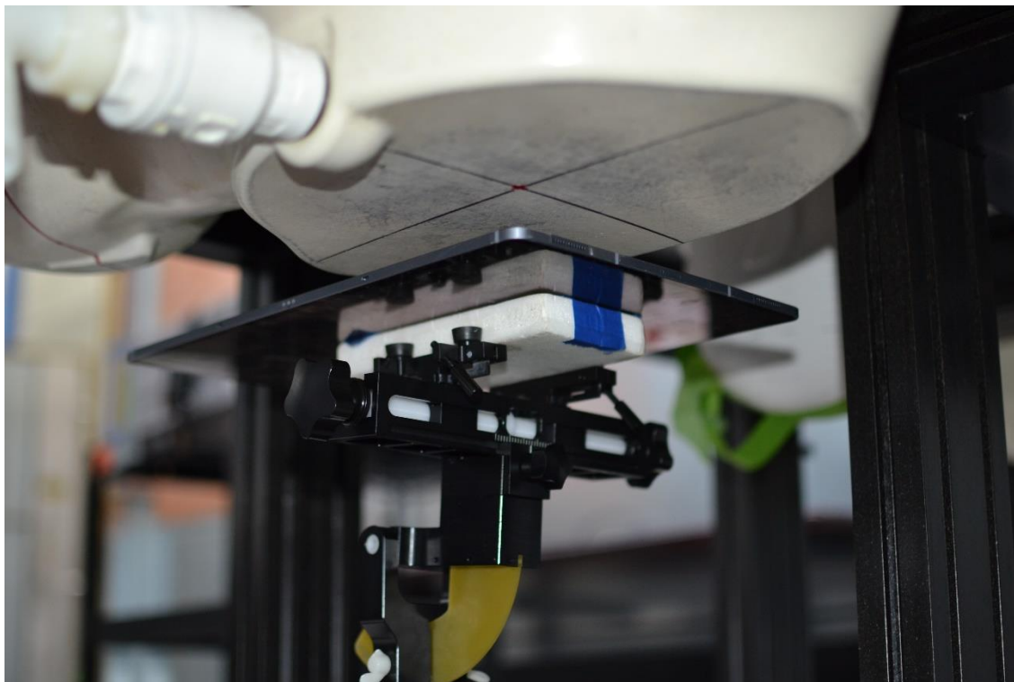
SAR Test Setup Photo 1 – Tablet, Back Side at 15 mm – Antenna WIFI 1
