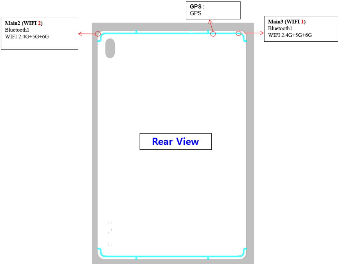
Figure I-1 DUT Antenna Locations
