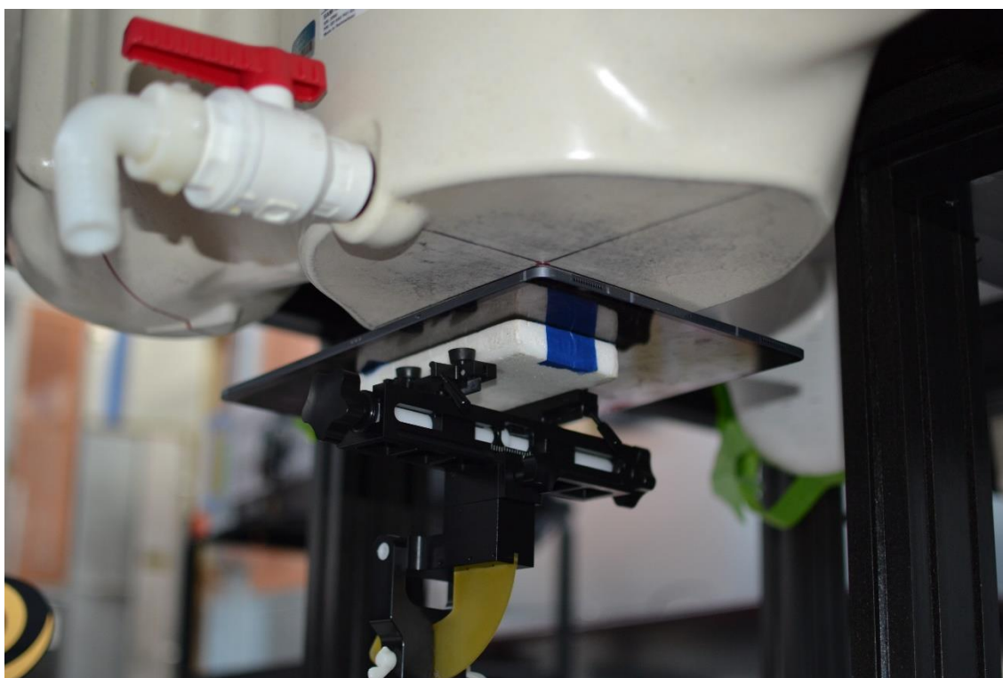
SAR Test Setup Photo 2 – Tablet, Back Side at 0 mm – Antenna WIFI 1
