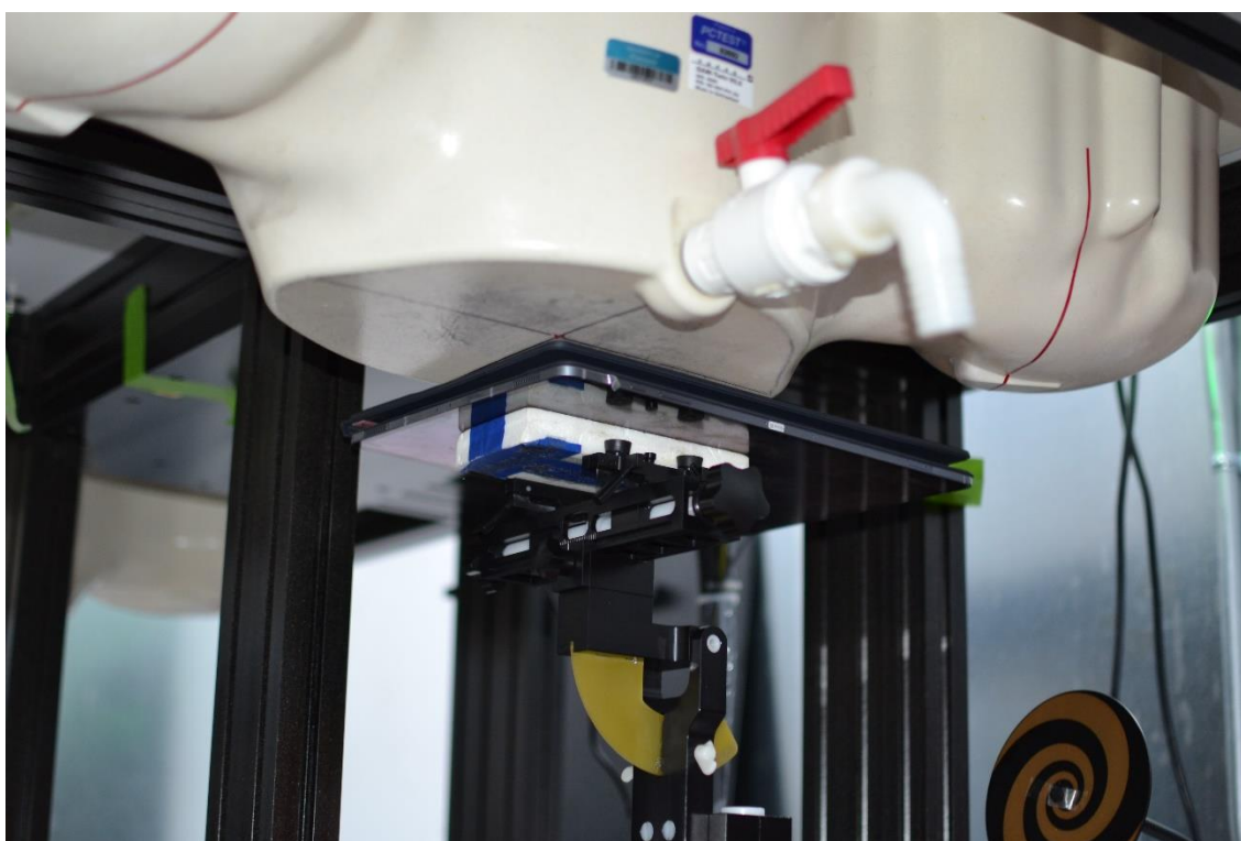
SAR Test Setup Photo 8 – Tablet with Keyboard Variant 2, Back Side at 0 mm – Antenna WIFI 2
