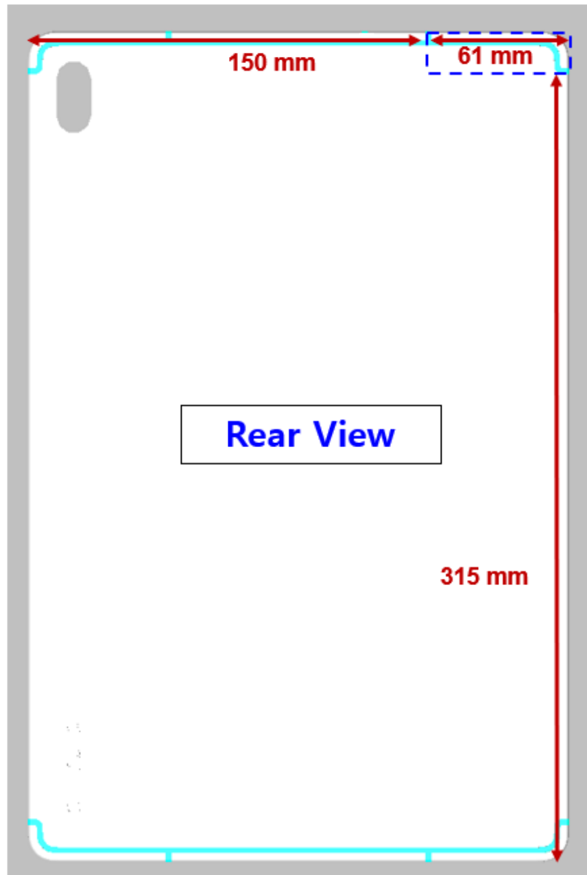
Figure I-3 DUT Dimensions
