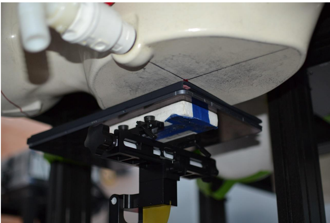
SAR Test Setup Photo 4 – Tablet with Keyboard Variant 2, Back Side at 0 mm – Antenna WIFI 1
