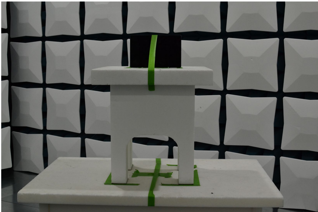
Figure 4. Test Setup – Y Position – 1GHz-40GHz
