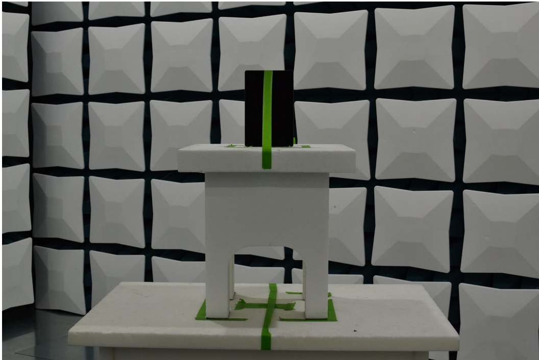
Figure 5. Test Setup – Z Position – 1GHz-40GHz
