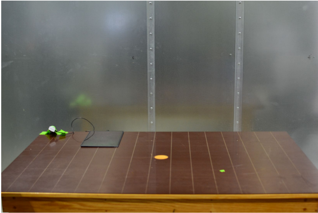
Figure 1. Test Setup – ACLC– <30MHz
