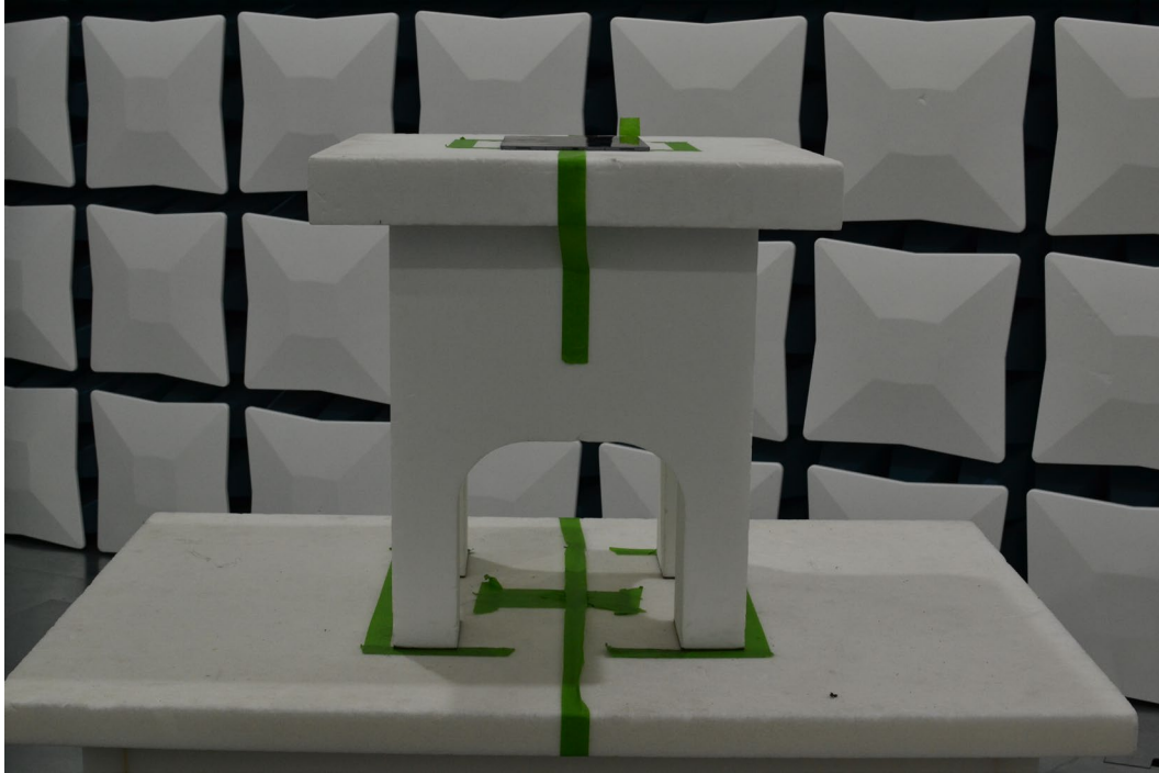
Figure 3. Test Setup – X Position – 1GHz-40GHz
