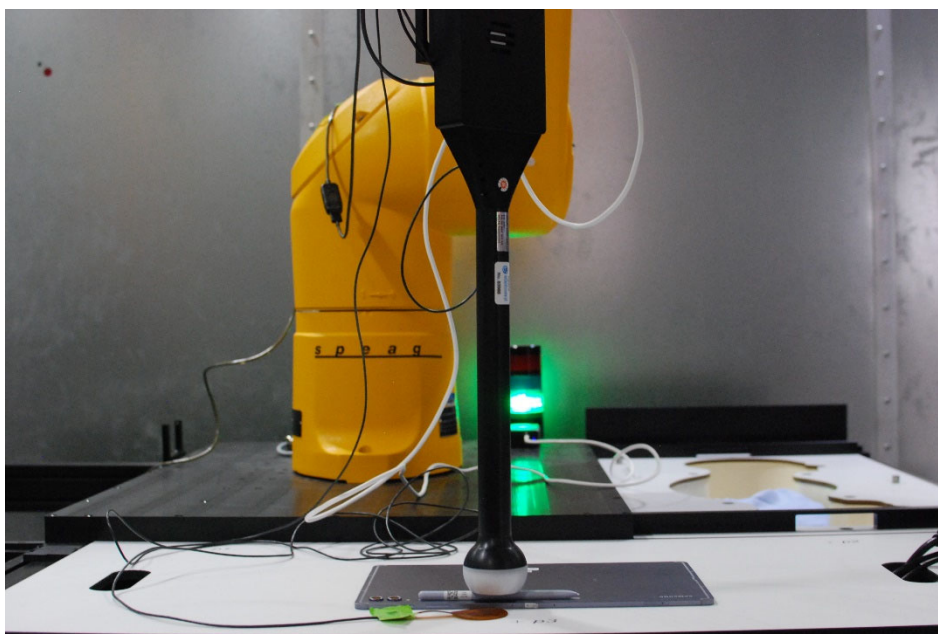
Test Setup Photo 2 H-field, Back side, Garage 2, 0mm
