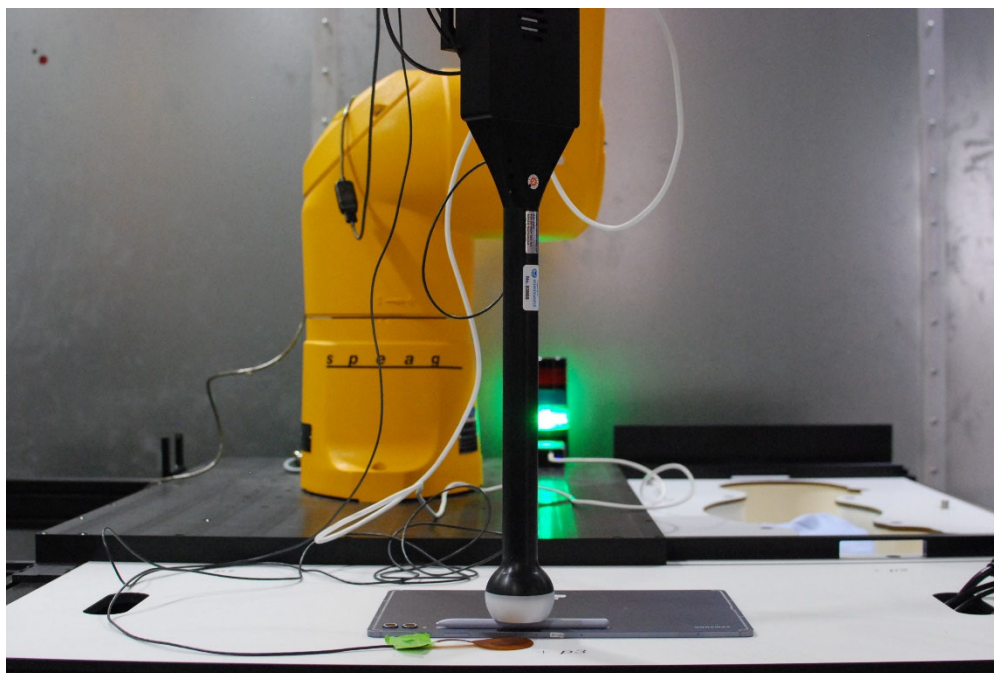
Test Setup Photo 1 H-field, Back side, Garage 1, 0mm
