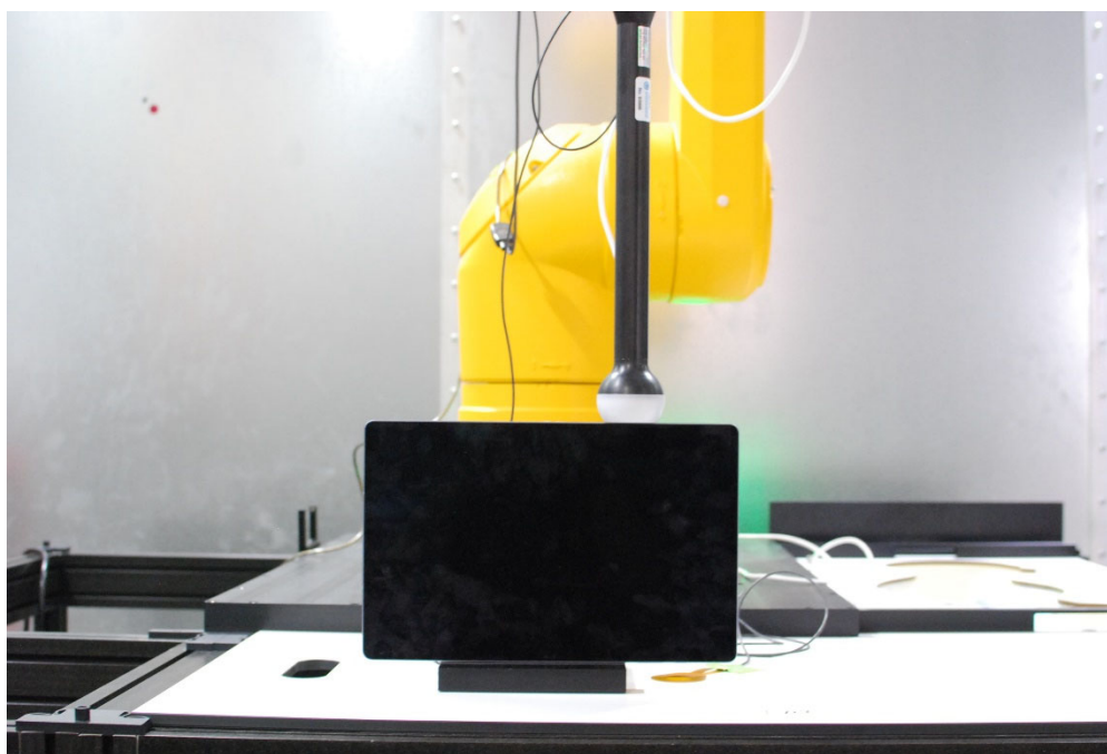
Test Setup Photo 8 H-field, Left edge, 0mm
