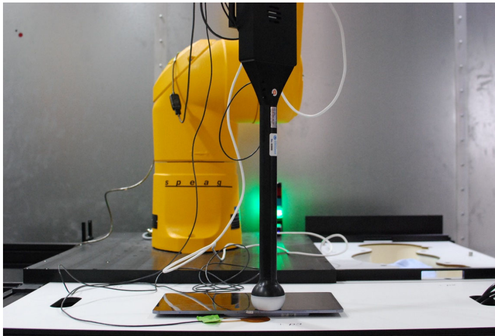
Test Setup Photo 4 H-field, Front side, Garage 2, 0mm
