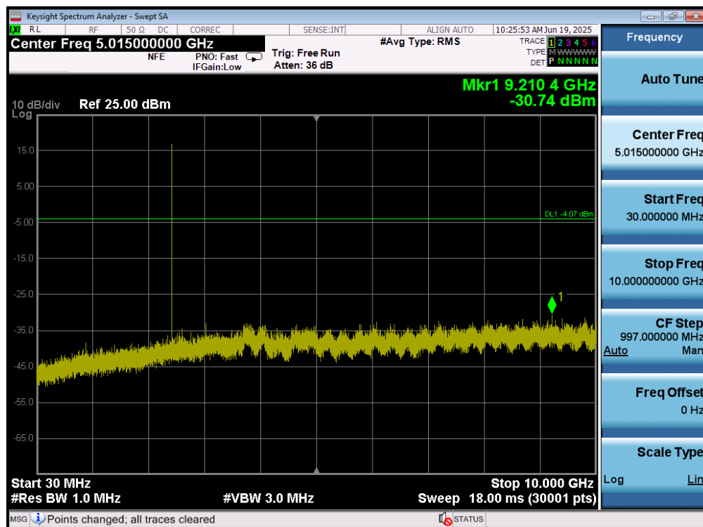
Plot 7-73. Conducted Spurious Plot (Bluetooth, 3Mbps – Ch. 39) – ANT1
