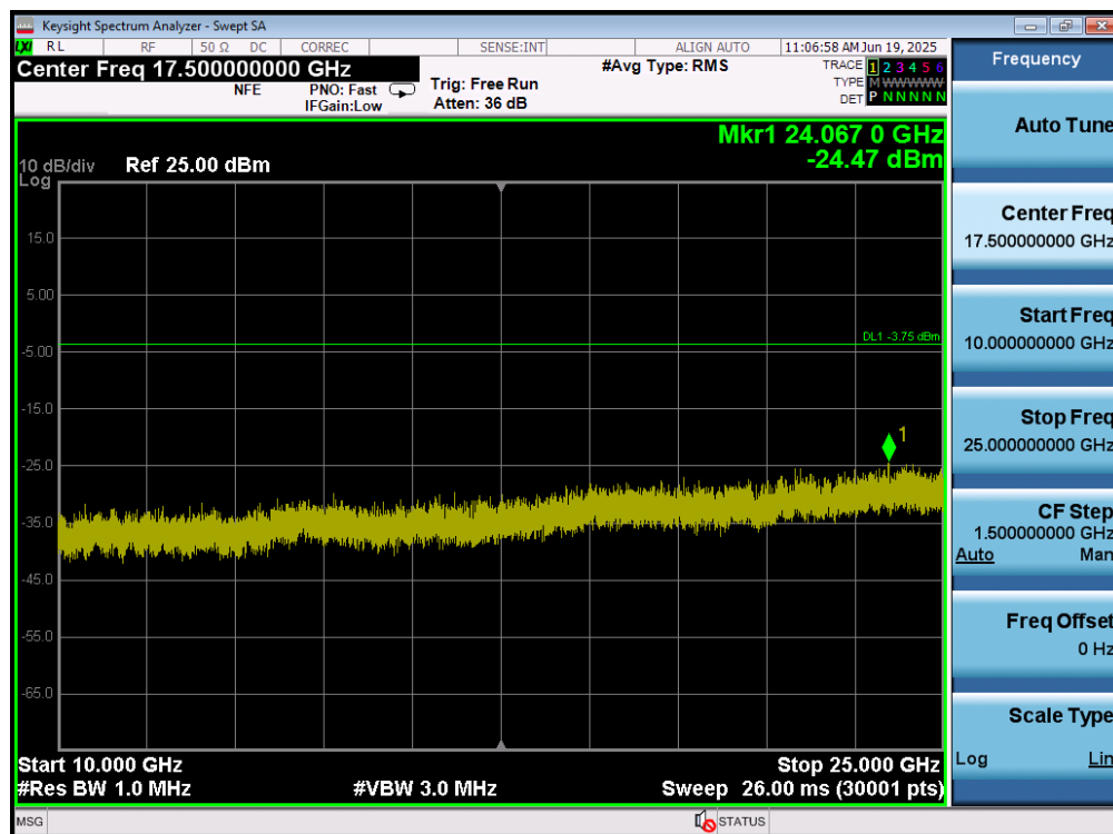
Plot 7-80. Conducted Spurious Plot (Bluetooth, 3Mbps – Ch. 39) – ANT2
