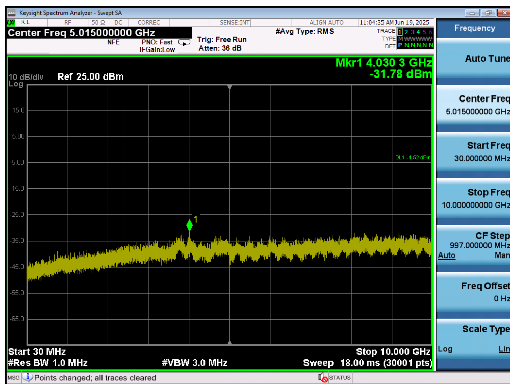
Plot 7-77. Conducted Spurious Plot (Bluetooth, 3Mbps – Ch. 0) – ANT2
