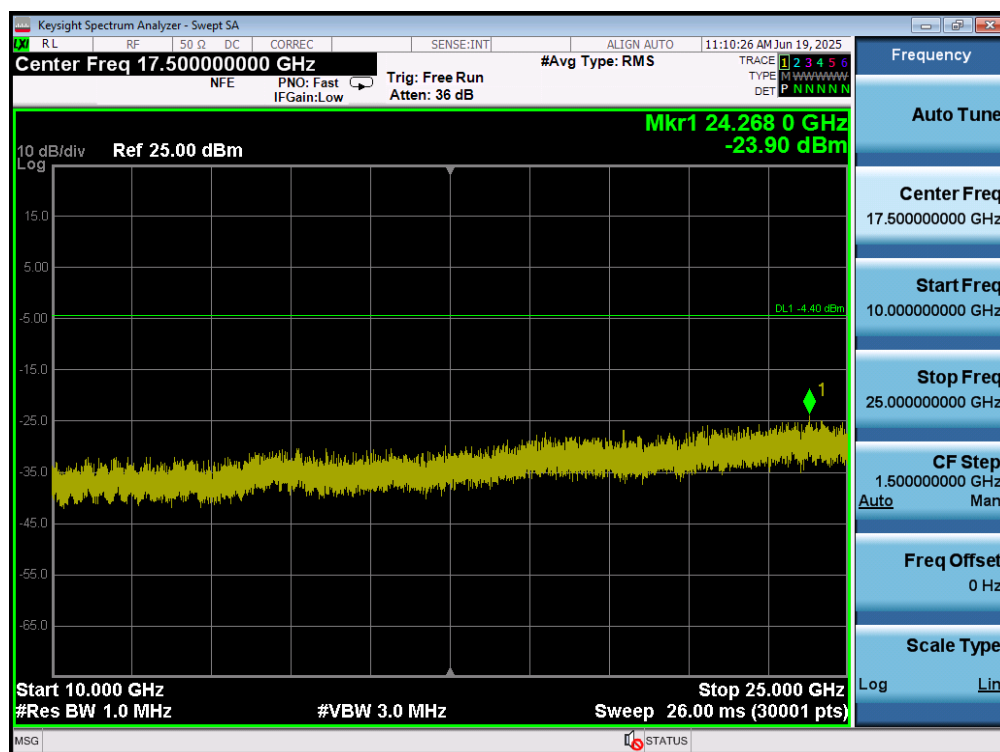
Plot 7-82. Conducted Spurious Plot (Bluetooth, 3Mbps – Ch. 78) – ANT2
