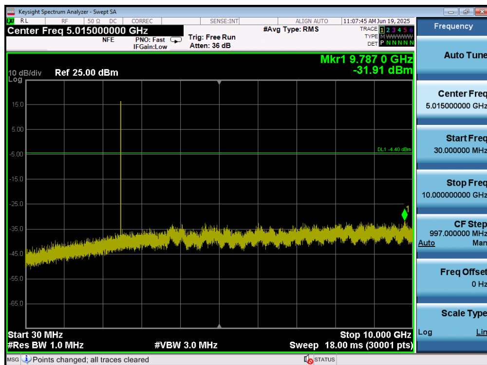
Plot 7-81. Conducted Spurious Plot (Bluetooth, 3Mbps – Ch. 78) – ANT2
