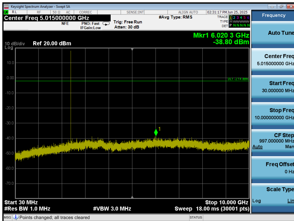
Plot 7-71. Conducted Spurious Plot (Bluetooth, 3Mbps – Ch. 0) – ANT1
