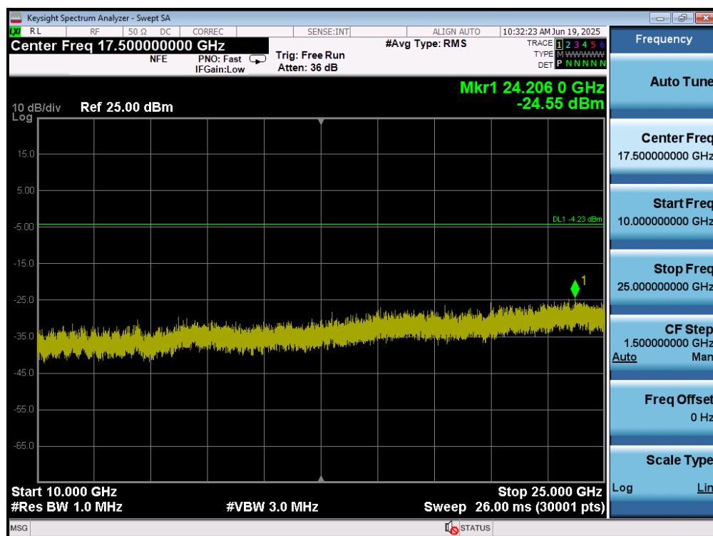
Plot 7-76. Conducted Spurious Plot (Bluetooth, 3Mbps - Ch. 78) - ANT1
