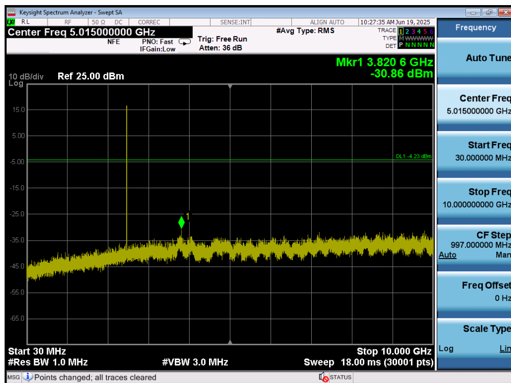
Plot 7-75. Conducted Spurious Plot (Bluetooth, 3Mbps - Ch. 78) - ANT1
