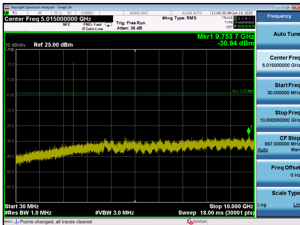
Plot 7-79. Conducted Spurious Plot (Bluetooth, 3Mbps – Ch. 39) – ANT2
