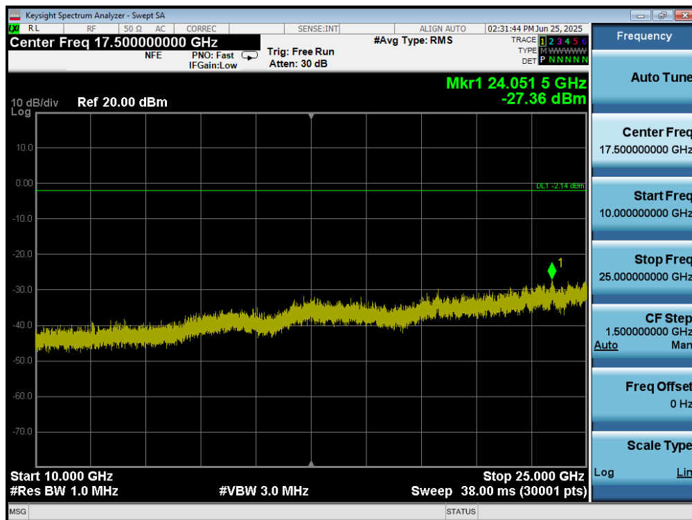
Plot 7-72. Conducted Spurious Plot (Bluetooth, 3Mbps – Ch. 0) – ANT1
