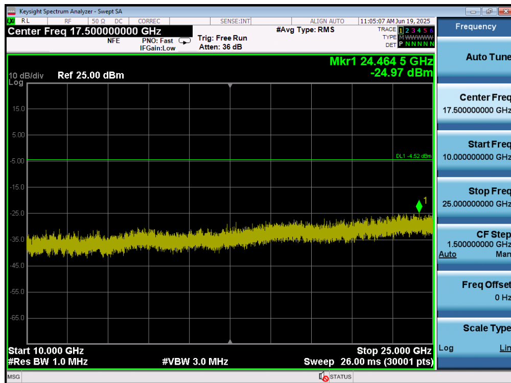
Plot 7-78. Conducted Spurious Plot (Bluetooth, 3Mbps – Ch. 0) – ANT2
