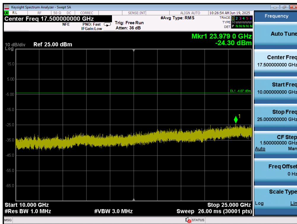
Plot 7-74. Conducted Spurious Plot (Bluetooth, 3Mbps – Ch. 39) – ANT1
