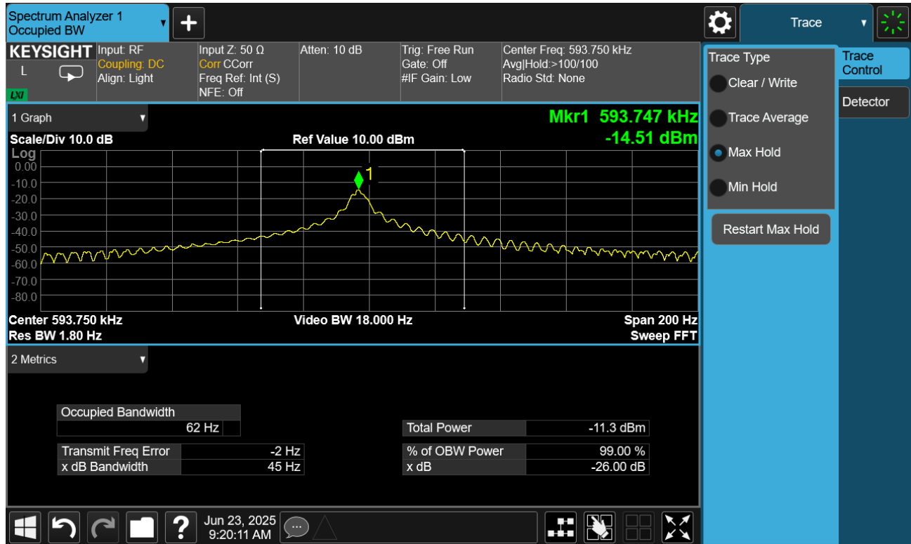
Plot 7-3. Occupied Bandwidth Measurement – Eraser
