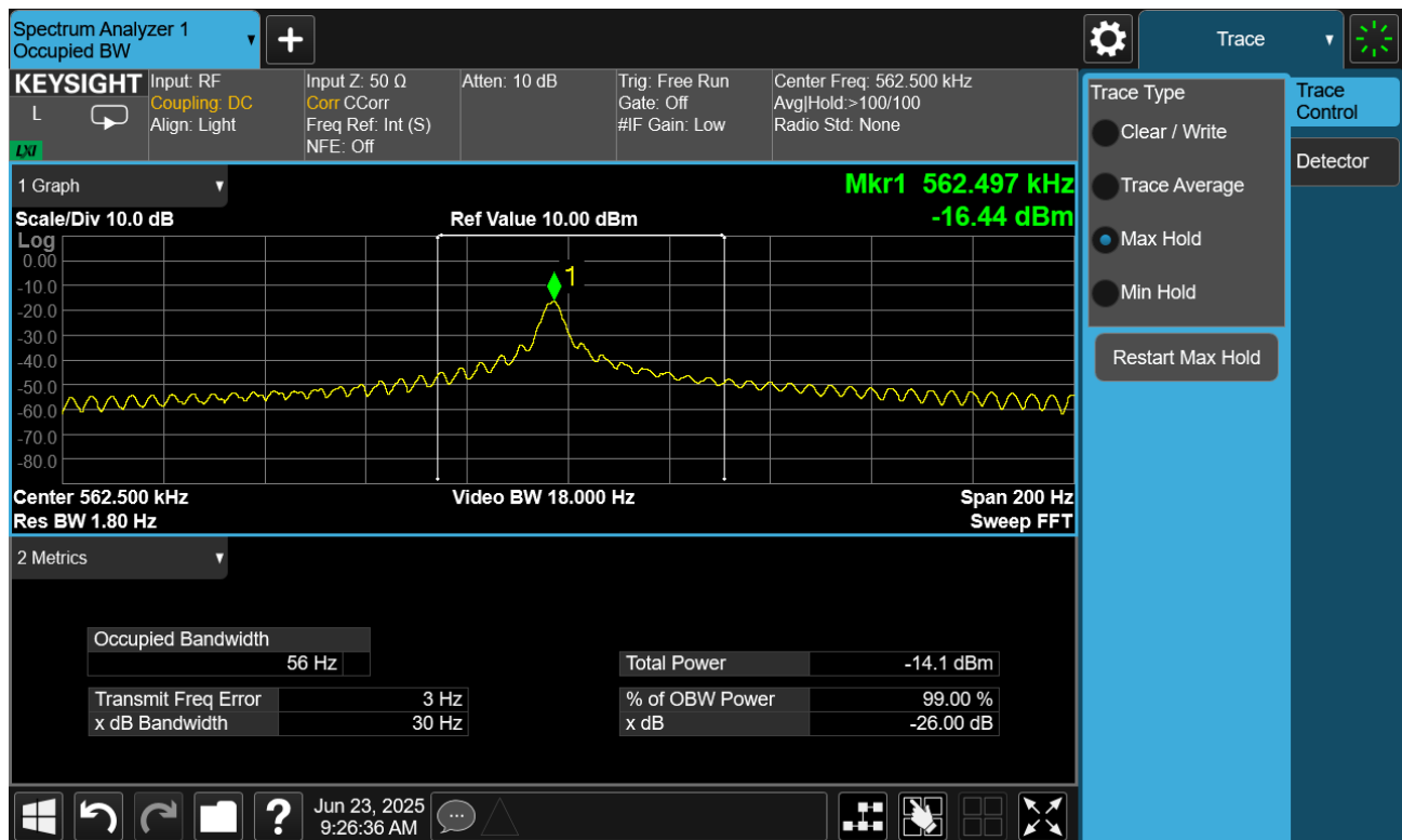
Plot 7-2. Occupied Bandwidth Measurement – Hover
