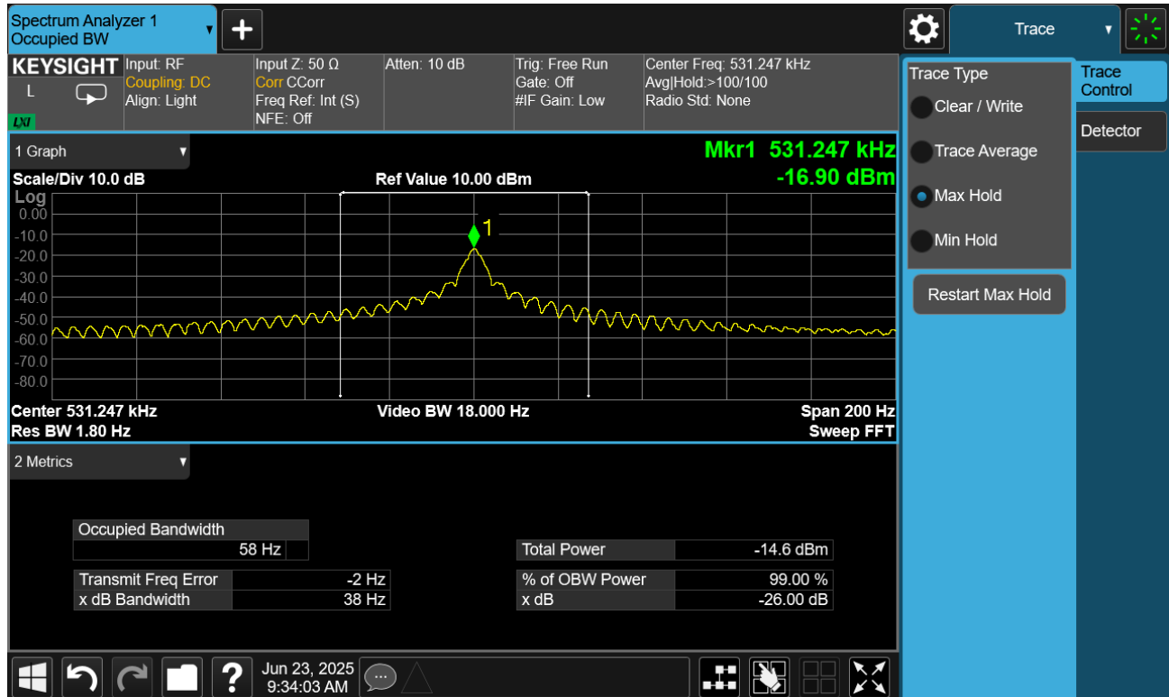
Plot 7-1. Occupied Bandwidth Measurement – Click
