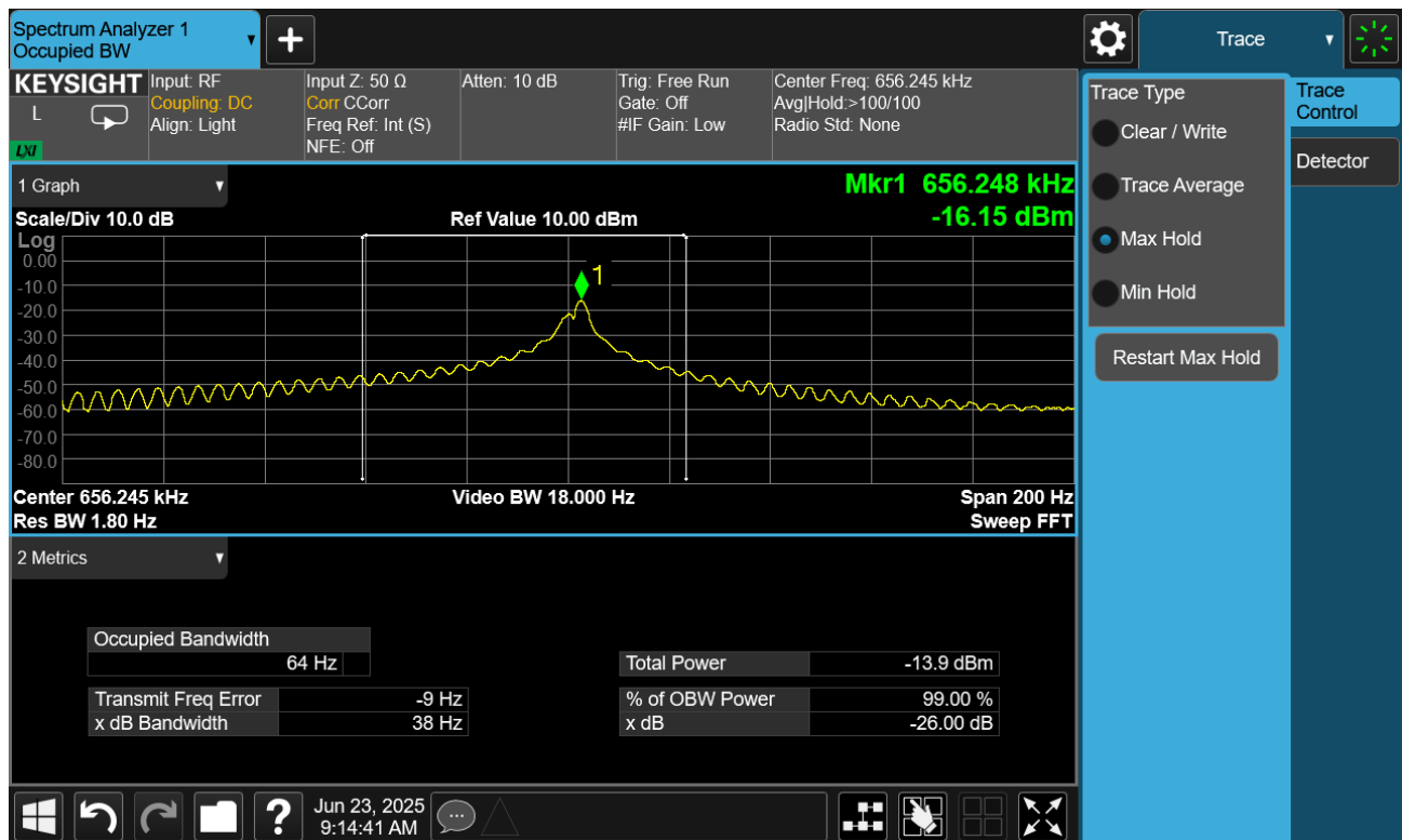
Plot 7-4. Occupied Bandwidth Measurement – Keyboard Detection
