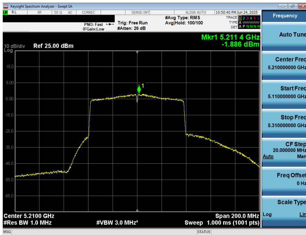
Plot 7-96. Power Spectral Density Plot MIMO ANT2 (80MHz BW 802.11ac (UNII Band 1) – Ch. 42)
