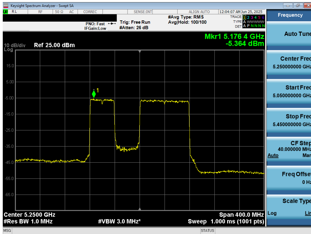
Plot 7-101. Power Spectral Density Plot MIMO ANT2 (160MHz BW 802.11b (40MHz Puncture) (UNII Band 1/2A) – Ch. 50)
