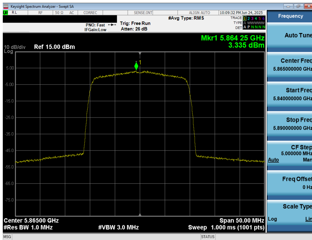
Plot 7-112. Power Spectral Density Plot MIMO ANT2 (20MHz BW 802.11be (UNII Band 4) – Ch. 173)
