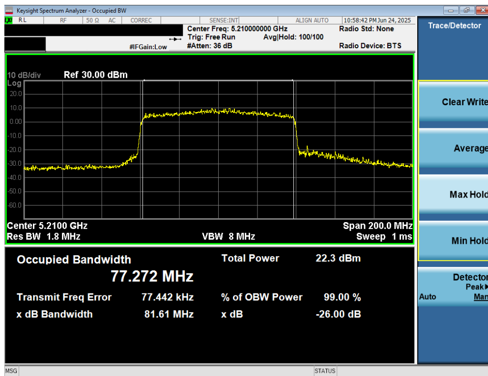
Plot 7-18. 26dB Bandwidth Plot MIMO ANT2 (80MHz BW 802.11be (UNII Band 1) – Ch. 42)
