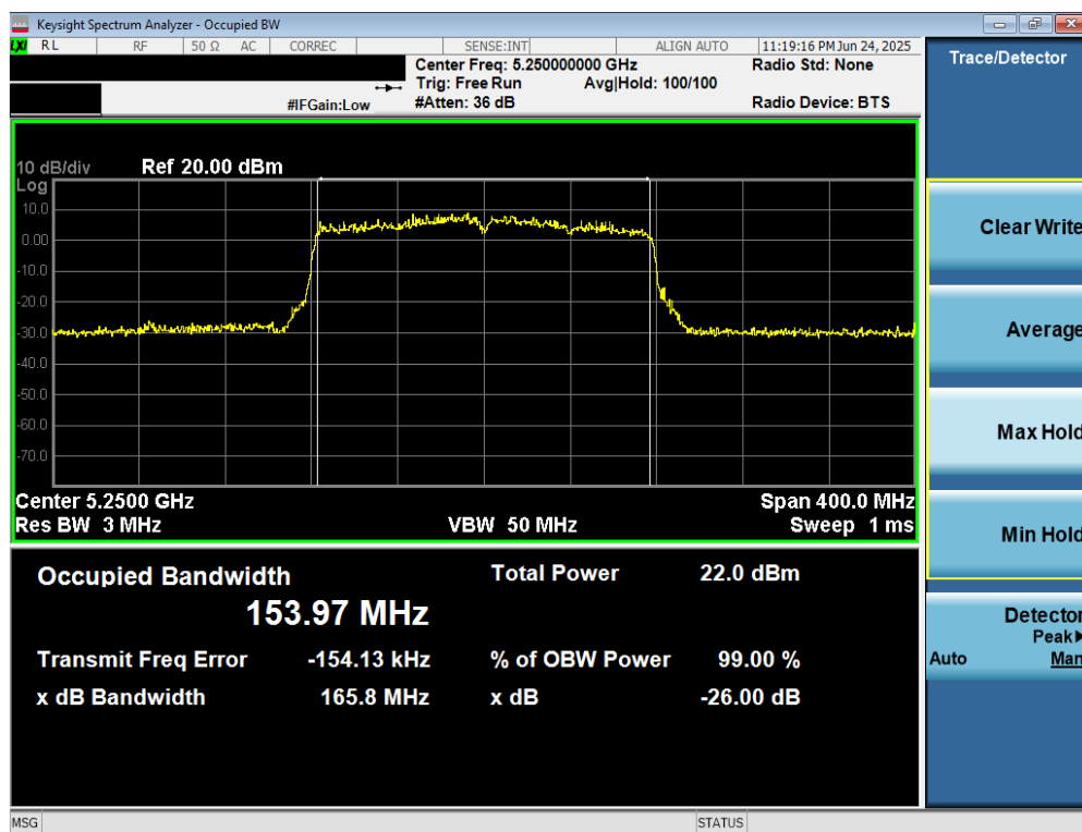
Plot 7-19. 26dB Bandwidth Plot MIMO ANT2 (160MHz BW 802.11ac (UNII Band 1/2A) – Ch. 50)
