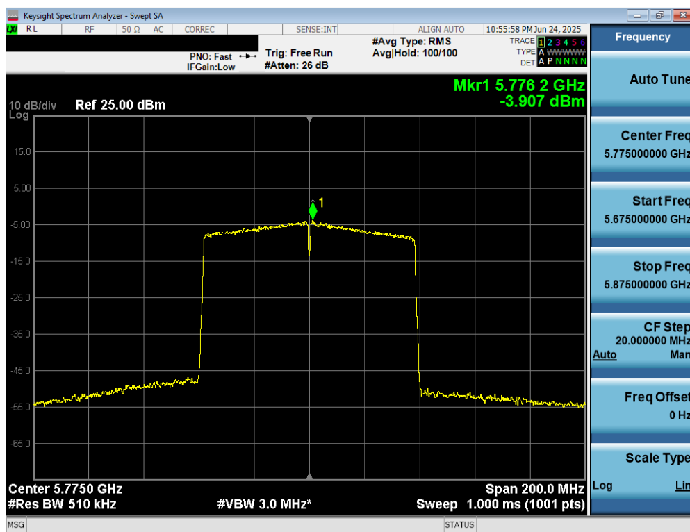
Plot 7-107. Power Spectral Density Plot MIMO ANT2 (80MHz BW 802.11ac (UNII Band 3) – Ch. 155)
