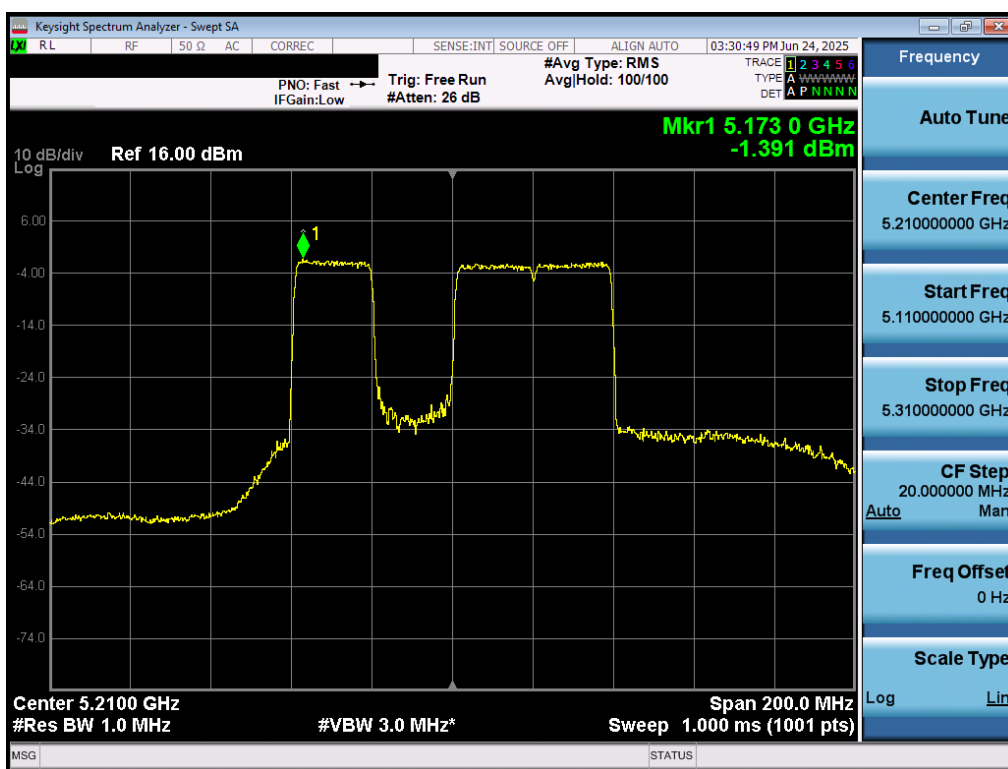
Plot 7-70. Power Spectral Density Plot MIMO ANT1 (80MHz BW 802.11be (20MHz Puncture (UNII Band 1) – Ch. 42)
