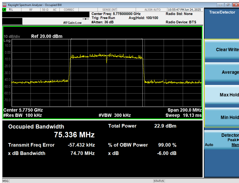
Plot 7-47. 6dB Bandwidth Plot MIMO ANT2 (80MHz BW 802.11ac (UNII Band 3) – Ch. 155)
