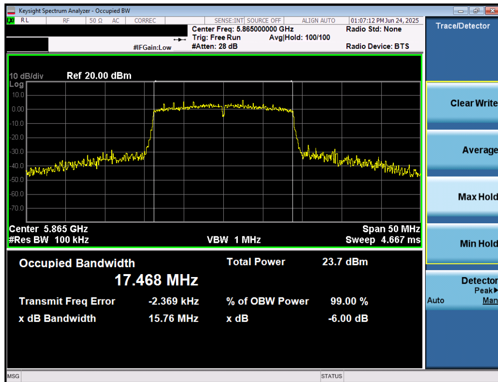
Plot 7-32. 6dB Bandwidth Plot MIMO ANT1 (20MHz BW 802.11n (UNII Band 4) – Ch. 173)
