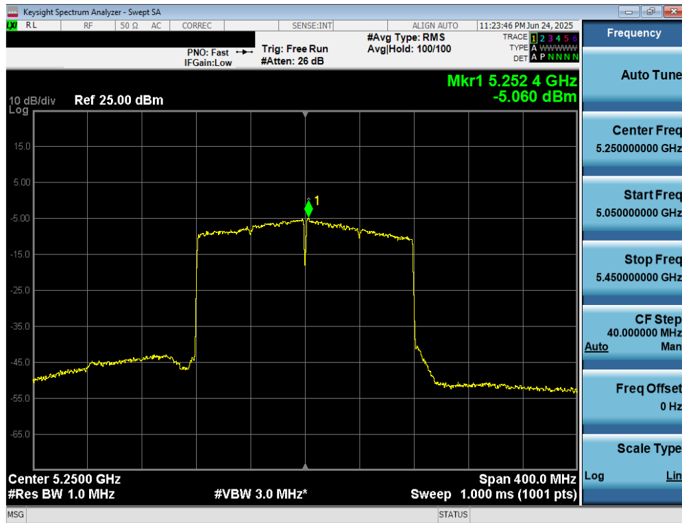
Plot 7-99. Power Spectral Density Plot MIMO ANT2 (160MHz BW 802.11be (UNII Band 1/2A) – Ch. 50)
