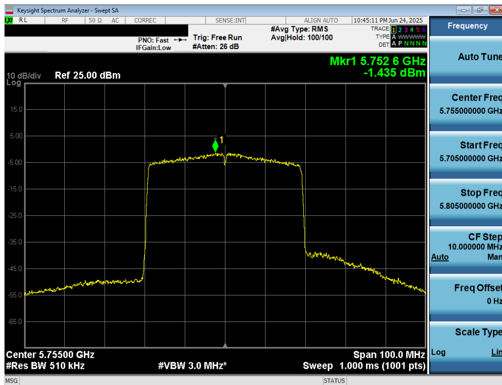
Plot 7-106. Power Spectral Density Plot MIMO ANT2 (40MHz BW 802.11be (UNII Band 3) – Ch. 151)
