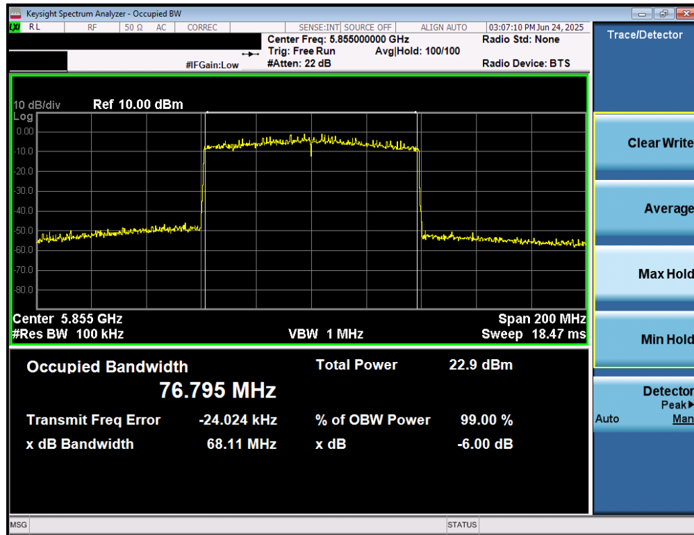
Plot 7-37. 6dB Bandwidth Plot MIMO ANT1 (80MHz BW 802.11be (UNII Band 3/4) – Ch. 171)
