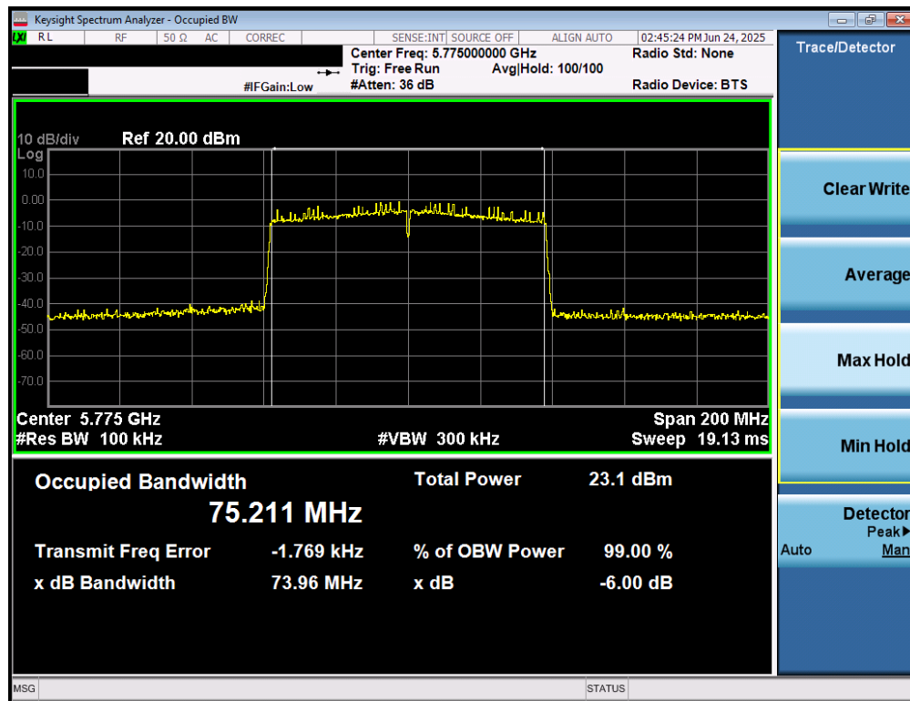
Plot 7-28. 6dB Bandwidth Plot MIMO ANT1 (80MHz BW 802.11ac (UNII Band 3) – Ch. 155)
