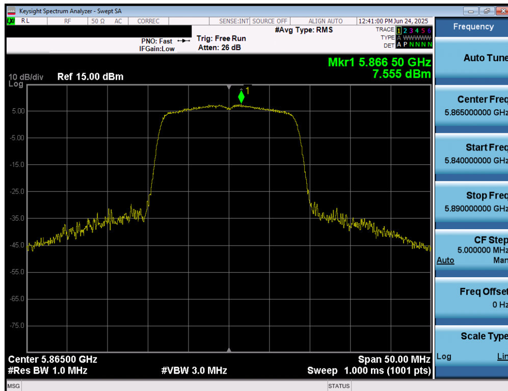
Plot 7-80. Power Spectral Density Plot MIMO ANT1 (802.11a (UNII Band 4) – Ch. 173)
