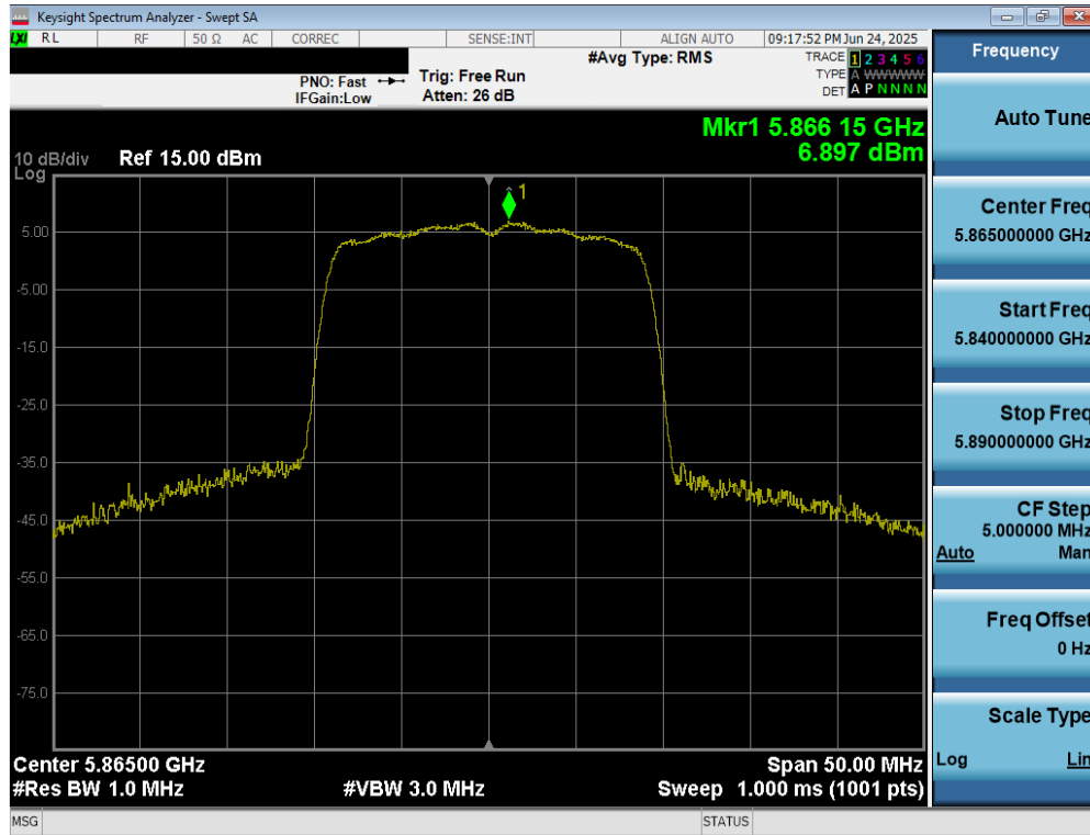
Plot 7-111. Power Spectral Density Plot MIMO ANT2 (20MHz BW 802.11n (UNII Band 4) – Ch. 173)
