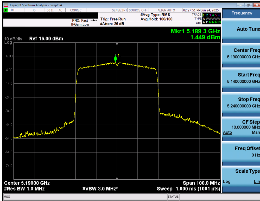
Plot 7-65. Power Spectral Density Plot MIMO ANT1 (40MHz BW 802.11be (UNII Band 1) – Ch. 38)
