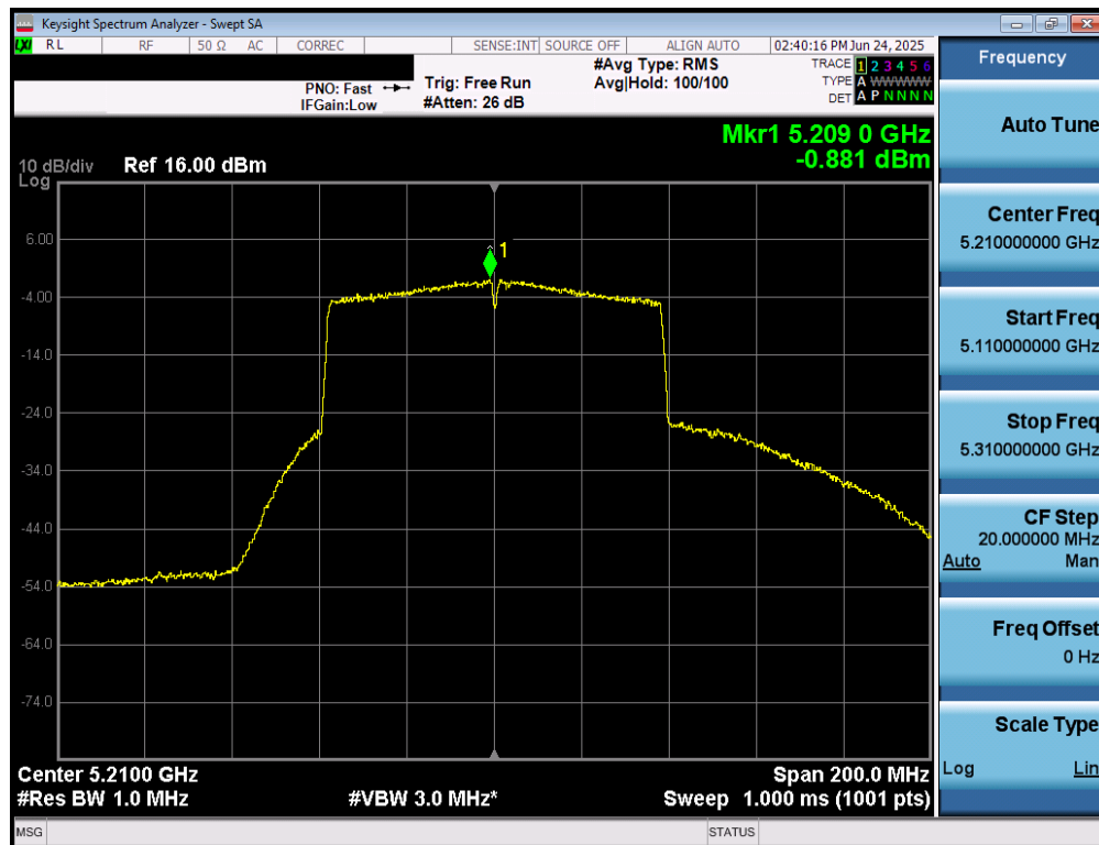
Plot 7-66. Power Spectral Density Plot MIMO ANT1 (80MHz BW 802.11ac (UNII Band 1) – Ch. 42)
