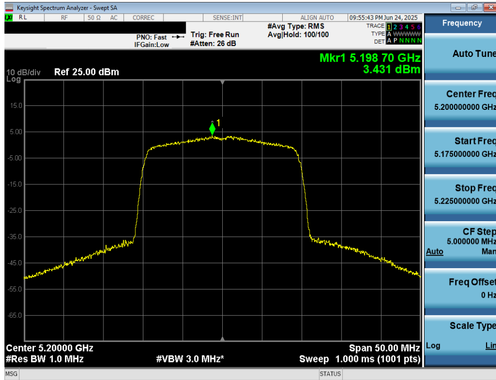
Plot 7-93. Power Spectral Density Plot MIMO ANT2 (20MHz BW 802.11be (UNII Band 1) – Ch. 40)
