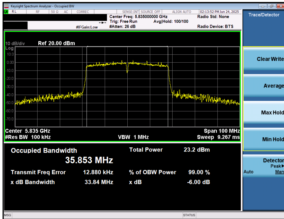
Plot 7-34. 6dB Bandwidth Plot MIMO ANT1 (40MHz BW 802.11n (UNII Band 3/4) – Ch. 167)
