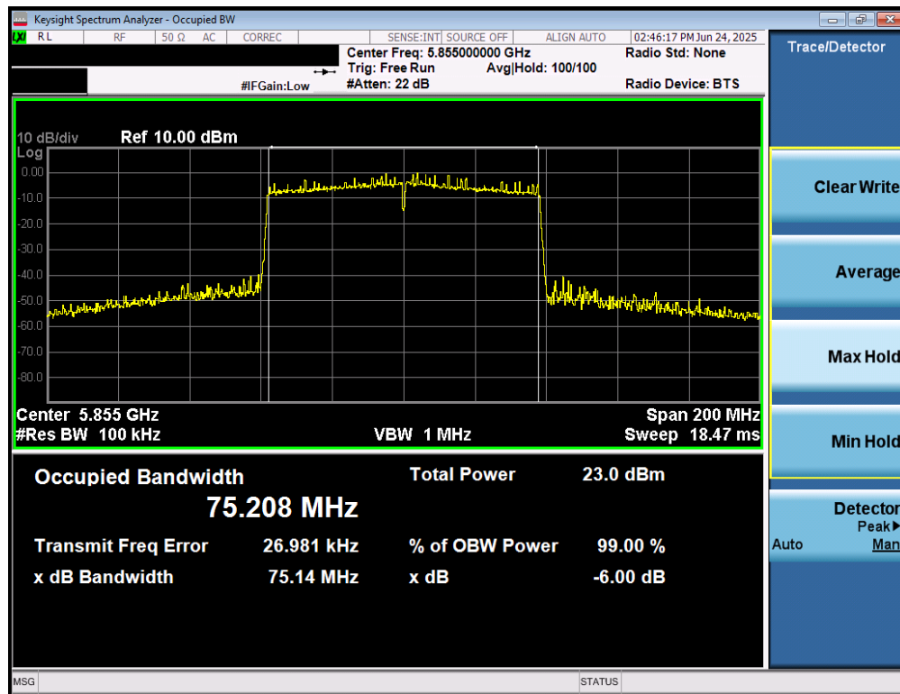
Plot 7-36. 6dB Bandwidth Plot MIMO ANT1 (80MHz BW 802.11ac (UNII Band 3/4) – Ch. 171)
