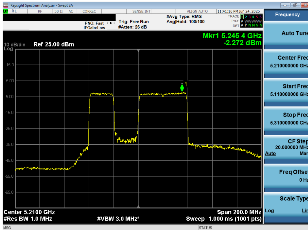
Plot 7-100. Power Spectral Density Plot MIMO ANT2 (80MHz BW 802.11be (20MHz Puncture) (UNII Band 1/2A) – Ch. 42)
