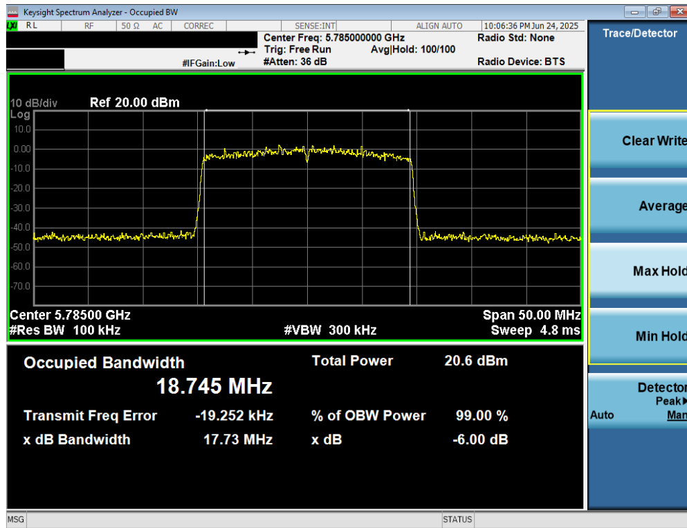
Plot 7-44. 6dB Bandwidth Plot MIMO ANT2 (20MHz BW 802.11be (UNII Band 3) – Ch. 157)
