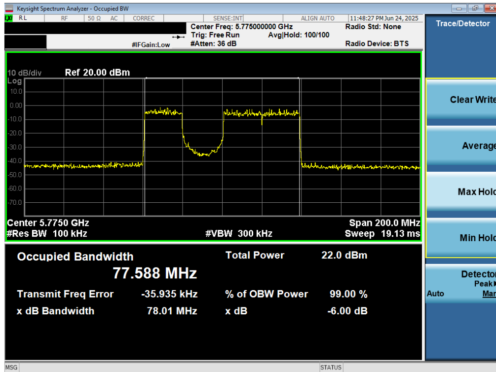
Plot 7-49. 6dB Bandwidth Plot MIMO ANT2 (80MHz BW 802.11be (20MHz Puncture) (UNII Band 3) – Ch. 155)
