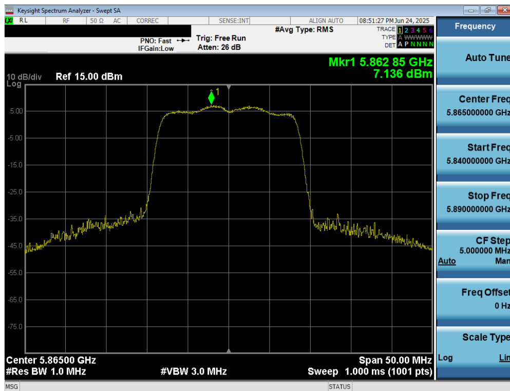
Plot 7-110. Power Spectral Density Plot MIMO ANT2 (802.11a (UNII Band 4) – Ch. 173)
