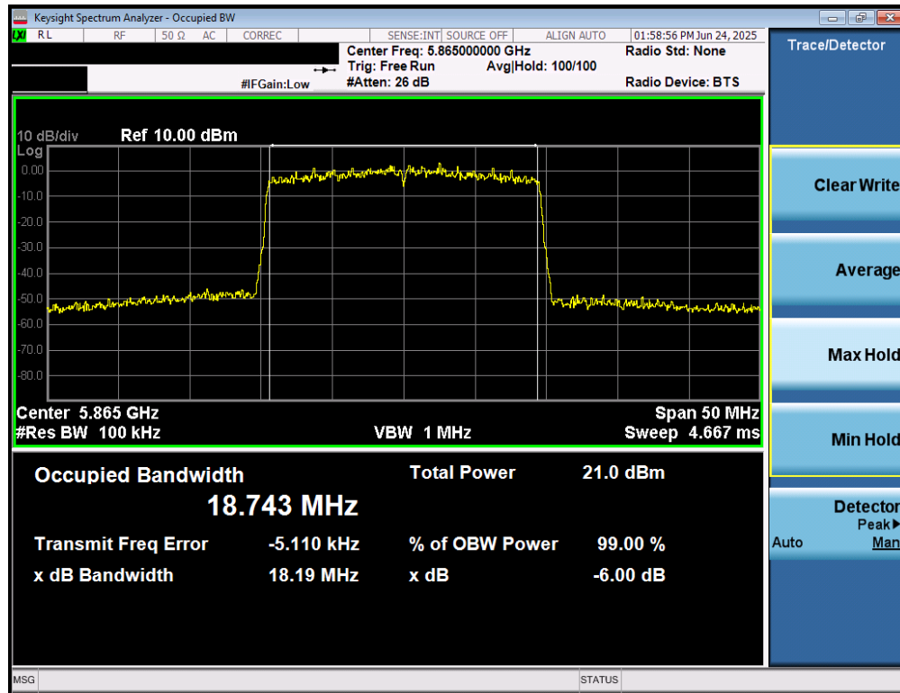
Plot 7-33. 6dB Bandwidth Plot MIMO ANT1 (20MHz BW 802.11be (UNII Band 4) – Ch. 173)
