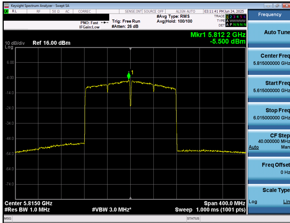
Plot 7-87. Power Spectral Density Plot MIMO ANT1 (160MHz BW 802.11ac (UNII Band 3/4) – Ch. 163)
