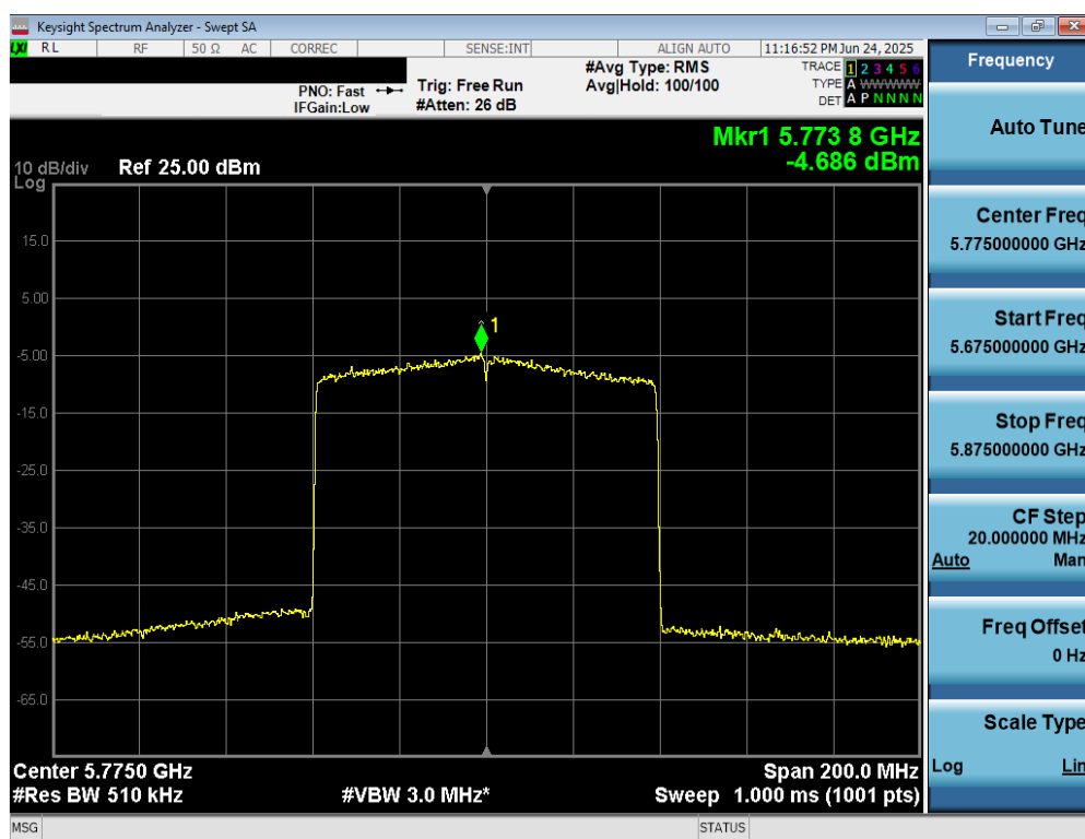
Plot 7-108. Power Spectral Density Plot MIMO ANT2 (80MHz BW 802.11be (UNII Band 3) – Ch. 155)
