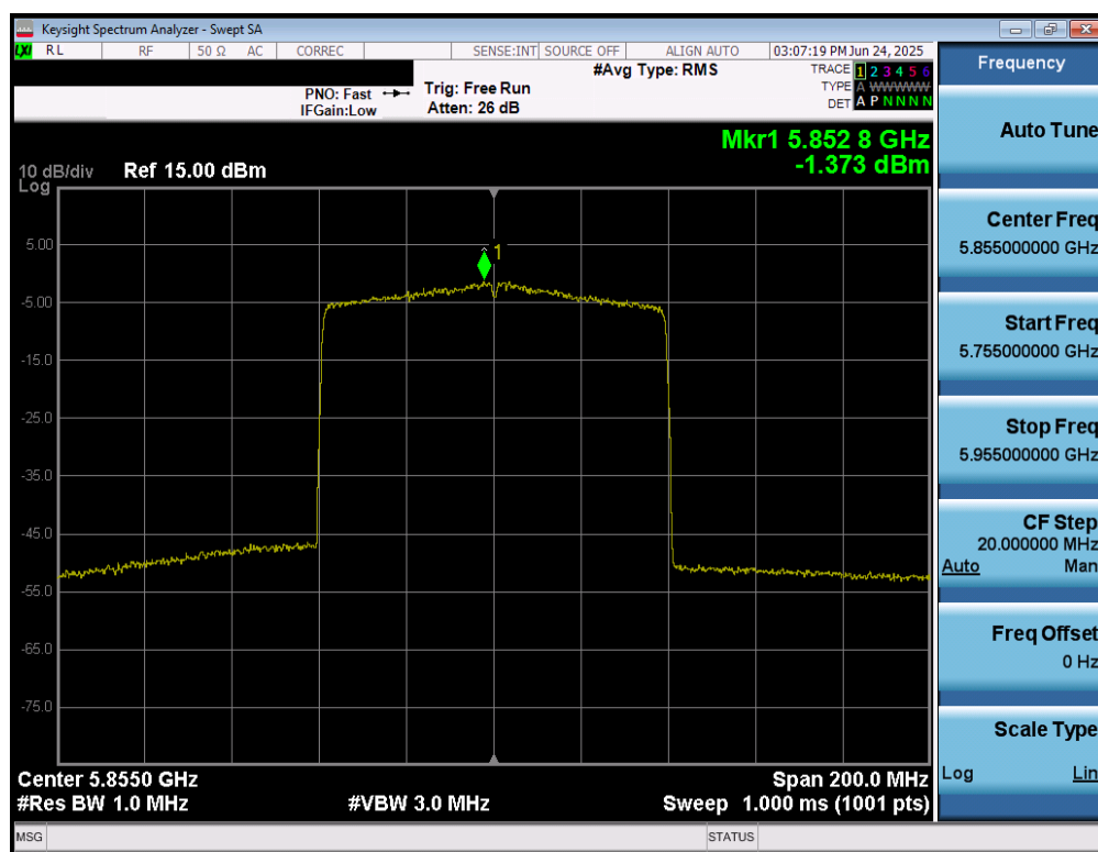
Plot 7-86. Power Spectral Density Plot MIMO ANT1 (80MHz BW 802.11be (UNII Band 3/4) – Ch. 171)
