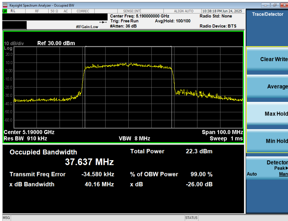
Plot 7-16. 26dB Bandwidth Plot MIMO ANT2 (40MHz BW 802.11be (UNII Band 1) – Ch. 38)
