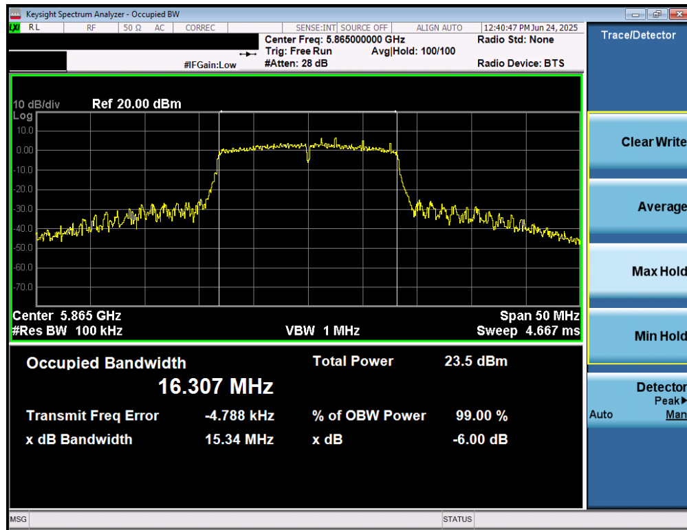
Plot 7-31. 6dB Bandwidth Plot MIMO ANT1 (802.11a (UNII Band 4) – Ch. 173)
