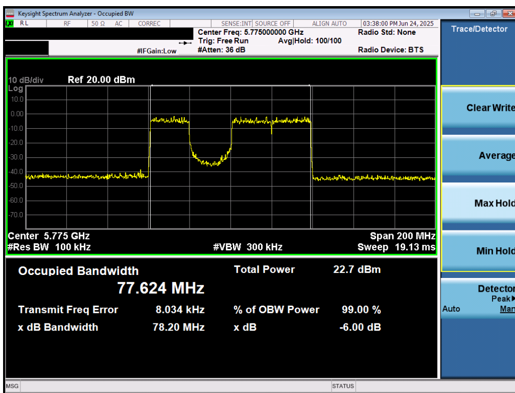
Plot 7-30. 6dB Bandwidth Plot MIMO ANT1 (80MHz BW 802.11be (20MHz Puncture) (UNII Band 3) – Ch. 155)
