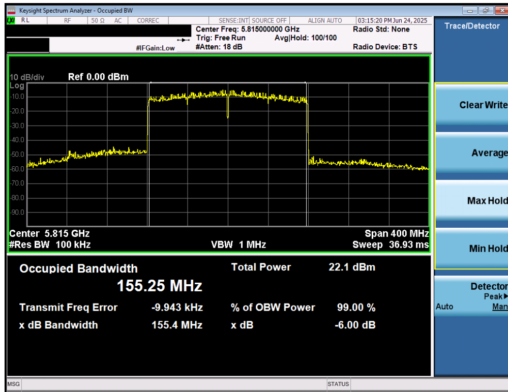
Plot 7-39. 6dB Bandwidth Plot MIMO ANT1 (160MHz BW 802.11be (UNII Band 3/4) – Ch. 163)
