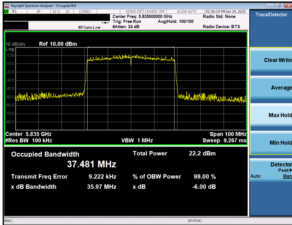
Plot 7-35. 6dB Bandwidth Plot MIMO ANT1 (40MHz BW 802.11be (UNII Band 3/4) – Ch. 167)
