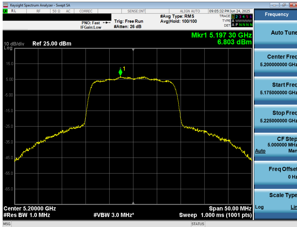
Plot 7-92. Power Spectral Density Plot MIMO ANT2 (20MHz BW 802.11n (UNII Band 1) – Ch. 40)
