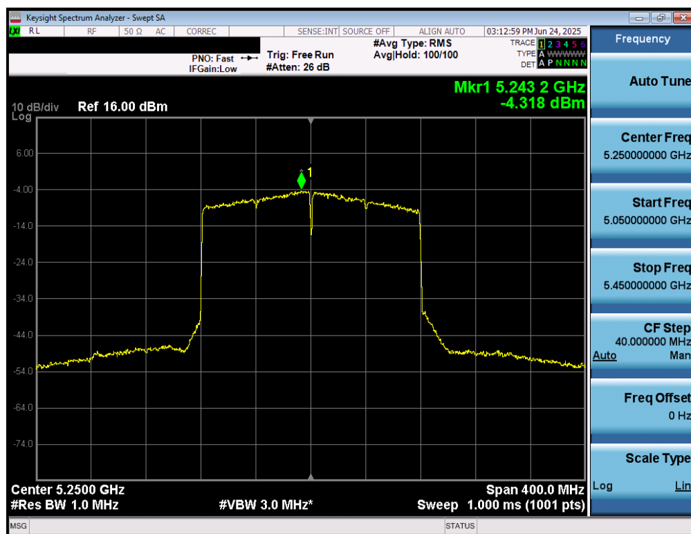
Plot 7-69. Power Spectral Density Plot MIMO ANT1 (160MHz BW 802.11be (UNII Band 1/2A) – Ch. 50)
