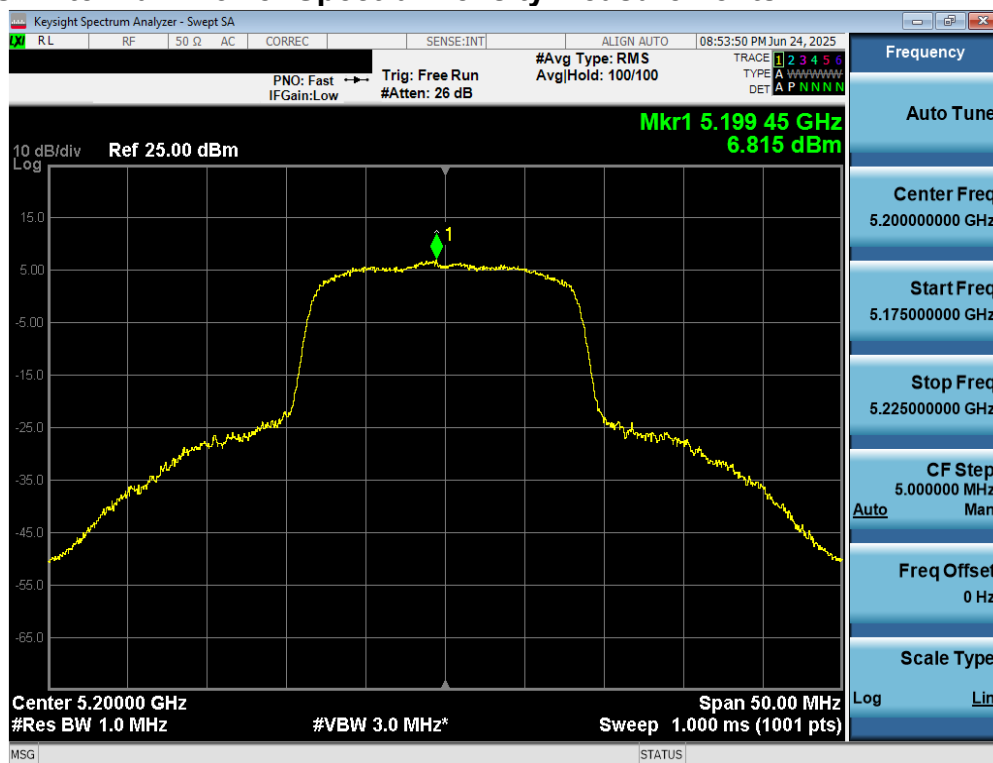
Plot 7-91. Power Spectral Density Plot MIMO ANT2 (802.11a (UNII Band 1) – Ch. 40)
