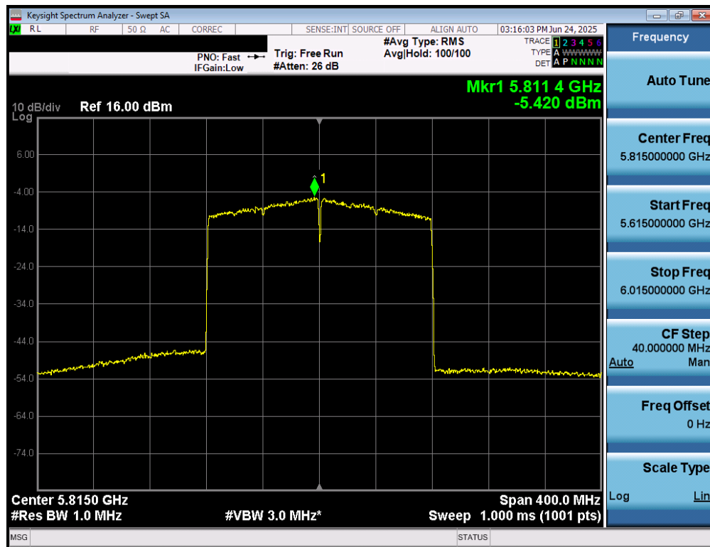
Plot 7-88. Power Spectral Density Plot MIMO ANT1 (160MHz BW 802.11be (UNII Band 3/4) – Ch. 163)
