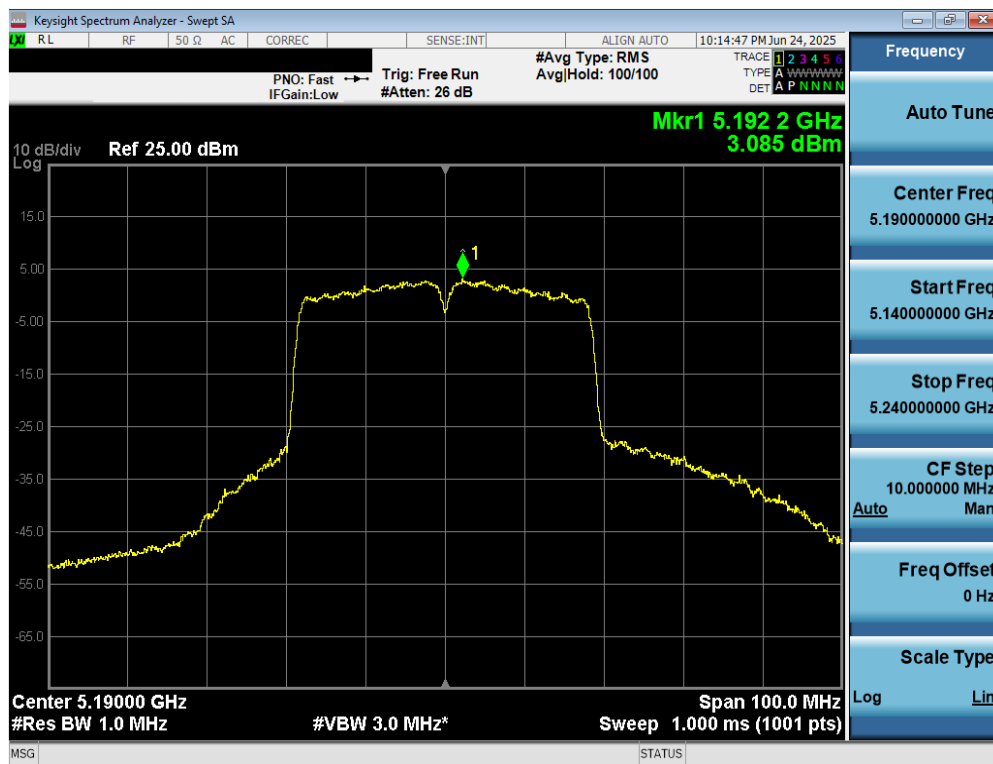
Plot 7-94. Power Spectral Density Plot MIMO ANT2 (40MHz BW 802.11n (UNII Band 1) – Ch. 38)
