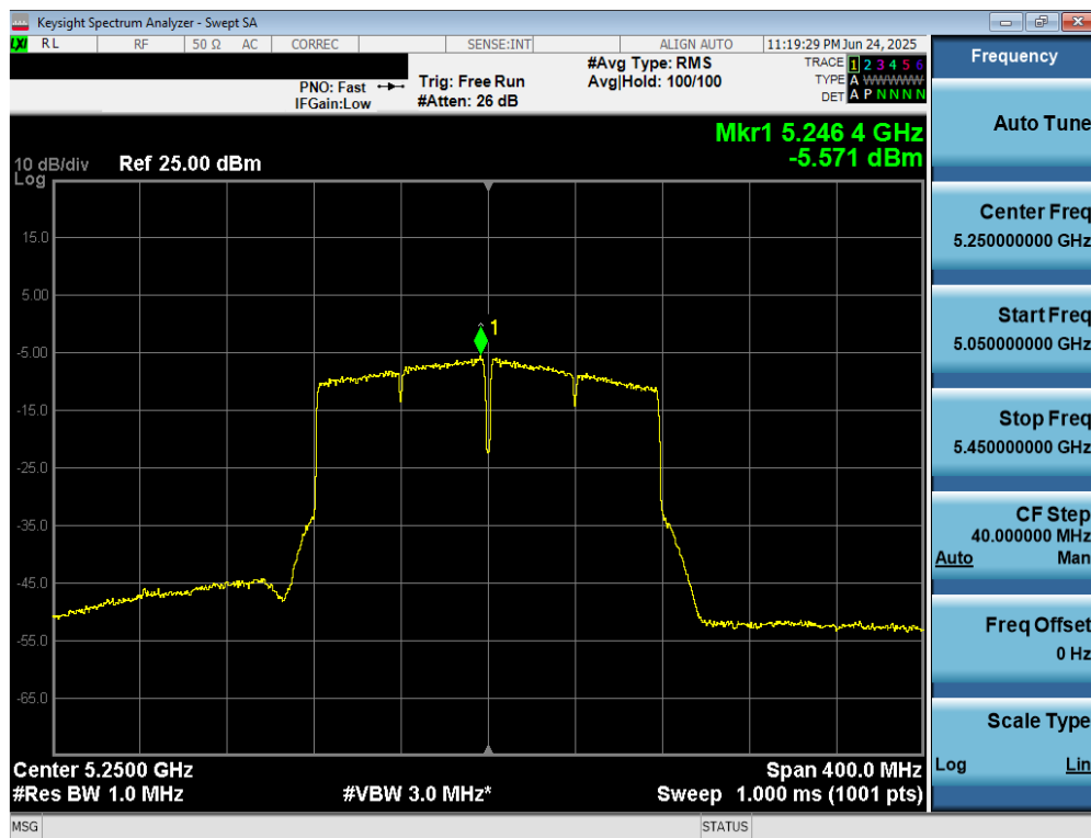
Plot 7-98. Power Spectral Density Plot MIMO ANT2 (160MHz BW 802.11ac (UNII Band 1/2A) – Ch. 50)
