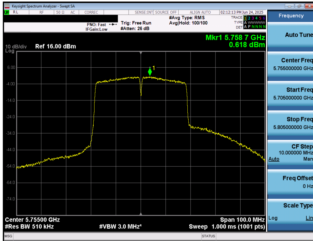
Plot 7-75. Power Spectral Density Plot MIMO ANT1 (40MHz BW 802.11n (UNII Band 3) – Ch. 151)
