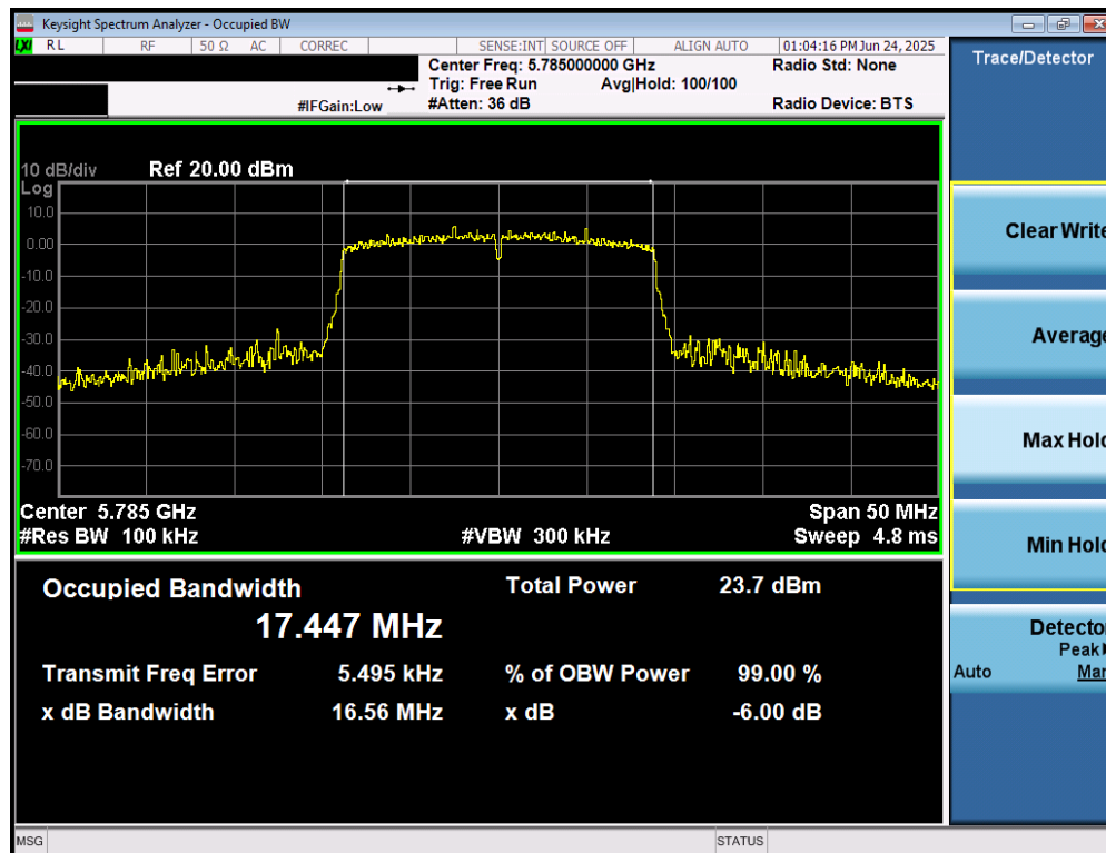
Plot 7-24. 6dB Bandwidth Plot MIMO ANT1 (20MHz BW 802.11n (UNII Band 3) – Ch. 157)
