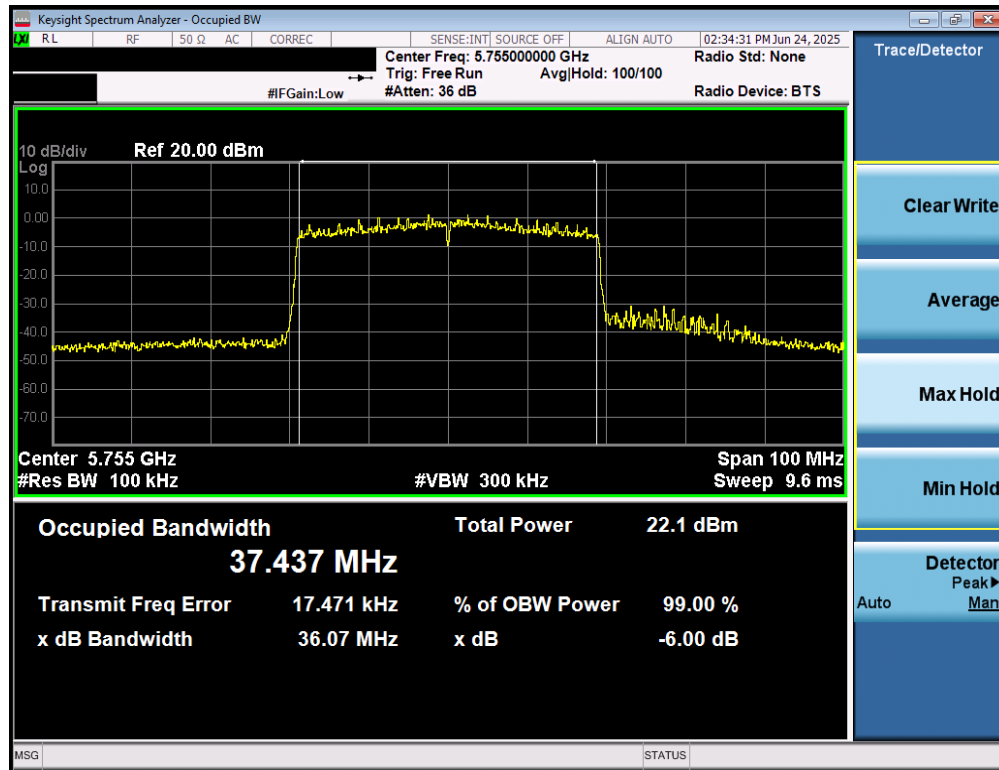
Plot 7-27. 6dB Bandwidth Plot MIMO ANT1 (40MHz BW 802.11be (UNII Band 3) – Ch. 151)
