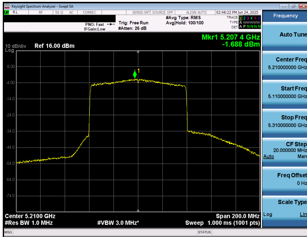
Plot 7-67. Power Spectral Density Plot MIMO ANT1 (80MHz BW 802.11be (UNII Band 1) – Ch. 42)
