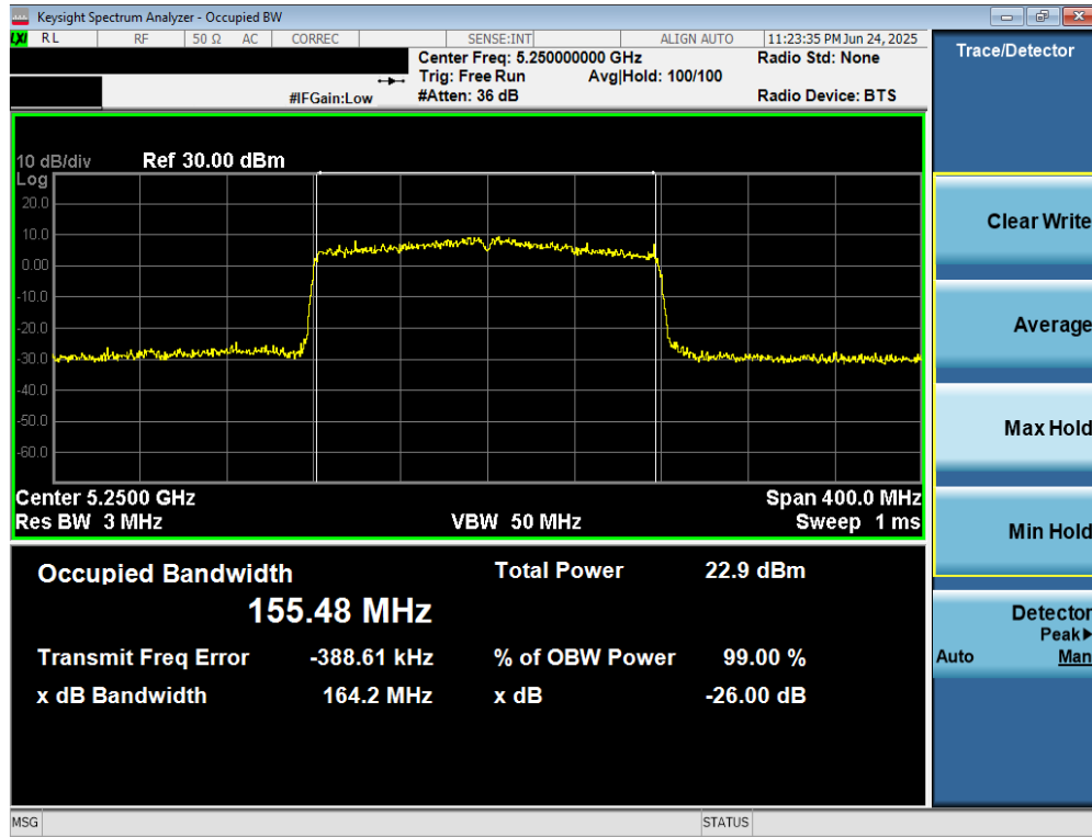
Plot 7-20. 26dB Bandwidth Plot MIMO ANT2 (160MHz BW 802.11be (UNII Band 1/2A) – Ch. 50)
