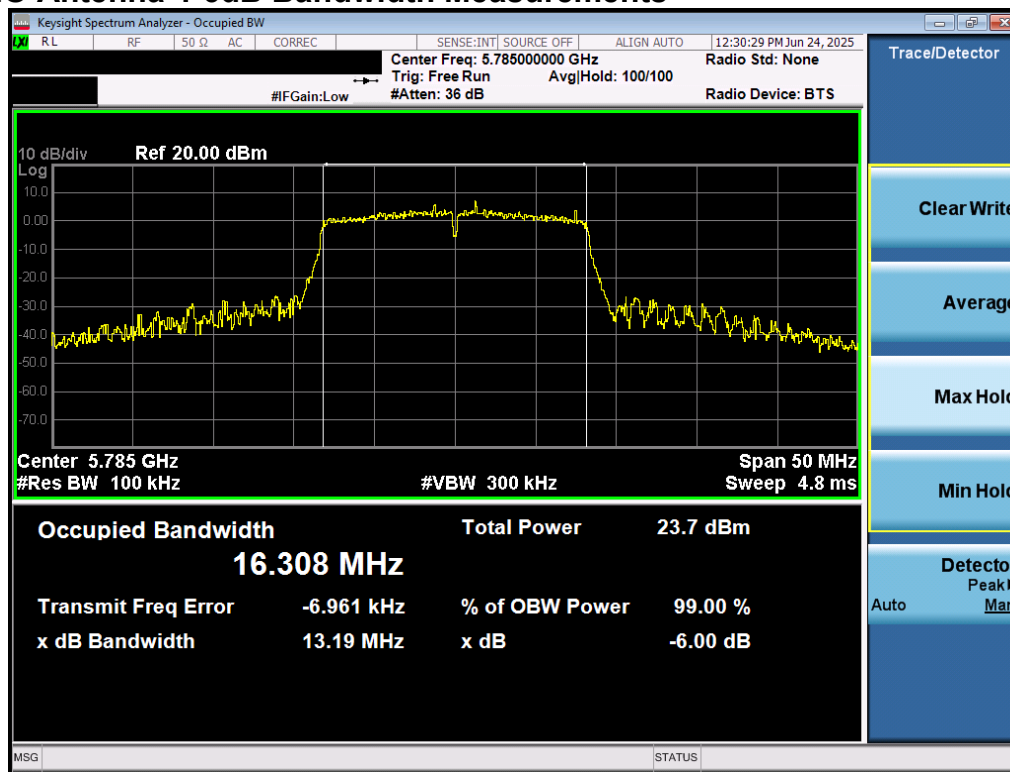
Plot 7-23. 6dB Bandwidth Plot MIMO ANT1 (802.11a (UNII Band 3) – Ch. 157)
