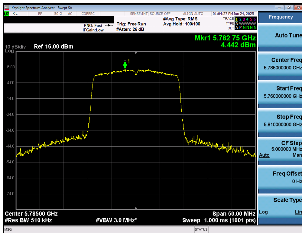
Plot 7-73. Power Spectral Density Plot MIMO ANT1 (20MHz BW 802.11n (UNII Band 3) – Ch. 157)
