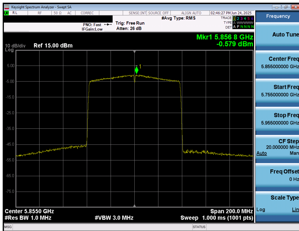
Plot 7-85. Power Spectral Density Plot MIMO ANT1 (80MHz BW 802.11ac (UNII Band 3/4) – Ch. 171)
