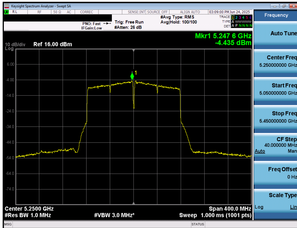
Plot 7-68. Power Spectral Density Plot MIMO ANT1 (160MHz BW 802.11ac (UNII Band 1/2A) – Ch. 50)
