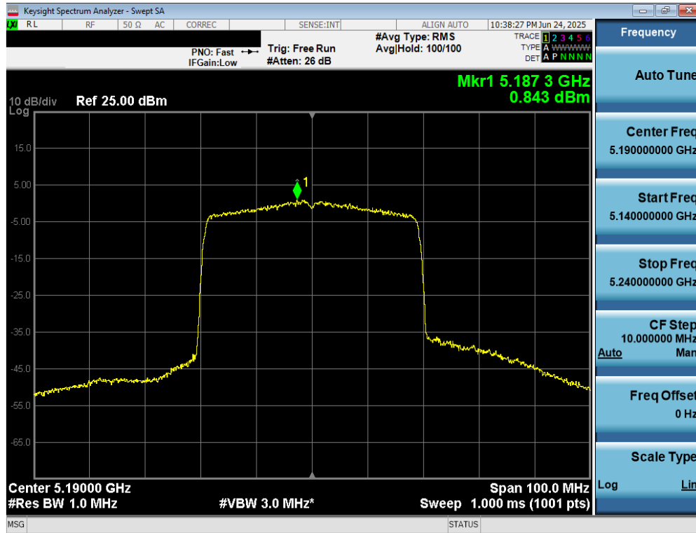
Plot 7-95. Power Spectral Density Plot MIMO ANT2 (40MHz BW 802.11be (UNII Band 1) – Ch. 38)
