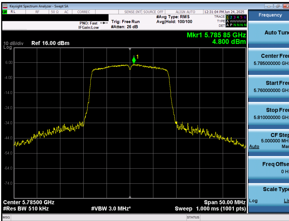
Plot 7-72. Power Spectral Density Plot MIMO ANT1 (802.11a (UNII Band 3) – Ch. 157)
