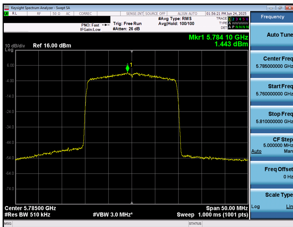
Plot 7-74. Power Spectral Density Plot MIMO ANT1 (20MHz BW 802.11be (UNII Band 3) – Ch. 157)
