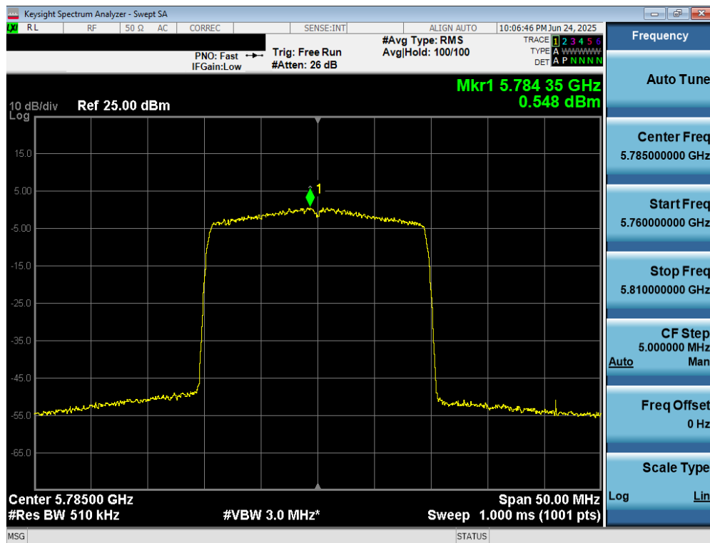
Plot 7-104. Power Spectral Density Plot MIMO ANT2 (20MHz BW 802.11be (UNII Band 3) – Ch. 157)
