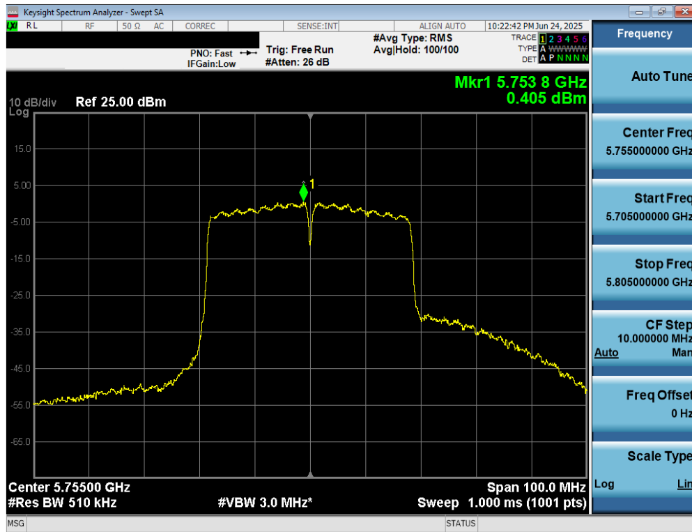
Plot 7-105. Power Spectral Density Plot MIMO ANT2 (40MHz BW 802.11n (UNII Band 3) – Ch. 151)
