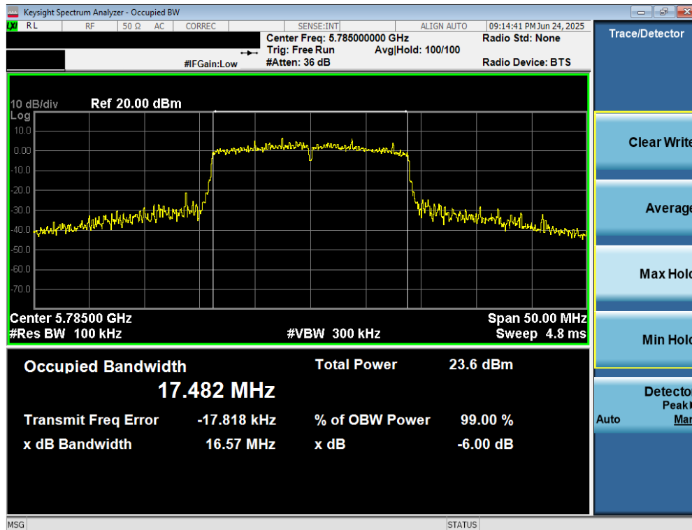
Plot 7-43. 6dB Bandwidth Plot MIMO ANT2 (20MHz BW 802.11n (UNII Band 3) – Ch. 157)
