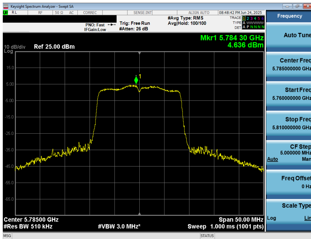
Plot 7-102. Power Spectral Density Plot MIMO ANT2 (802.11a (UNII Band 3) – Ch. 157)
