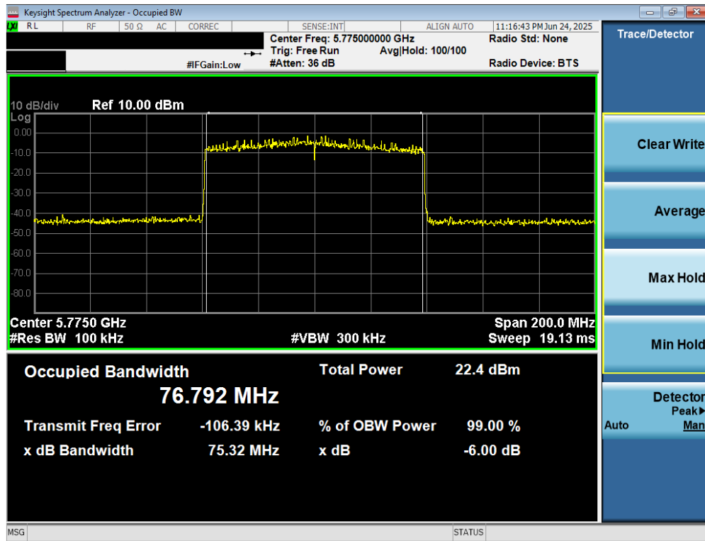
Plot 7-48. 6dB Bandwidth Plot MIMO ANT2 (80MHz BW 802.11be (UNII Band 3) – Ch. 155)
