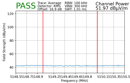
Plot 7-182. Radiated Lower Band Edge Plot MIMO (Average – UNII Band 1)
