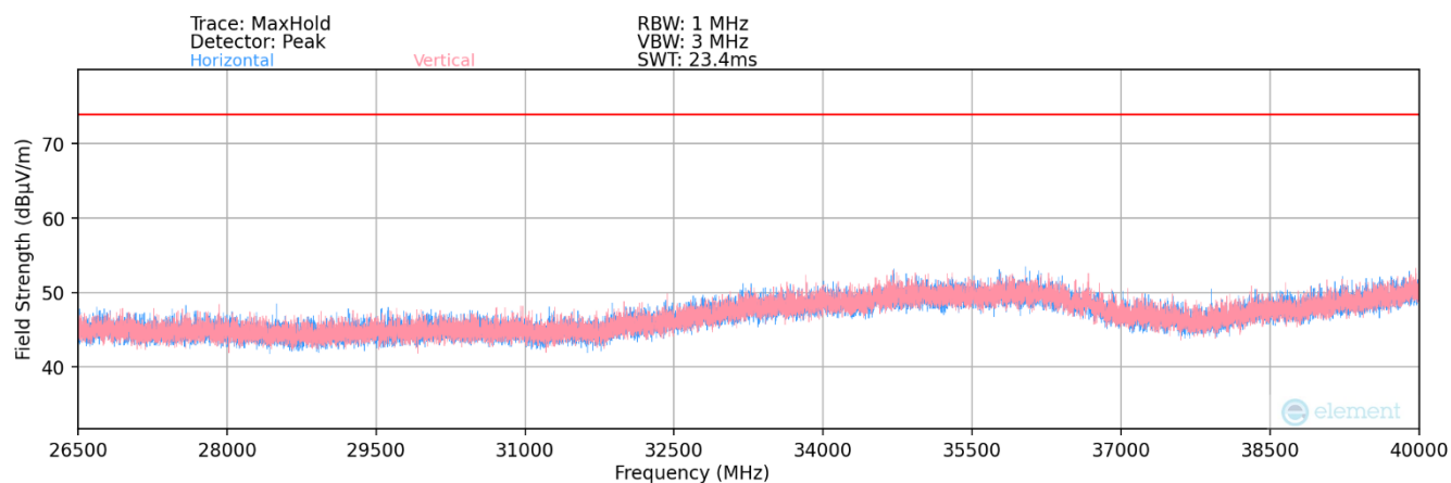
Plot 7-128. Radiated Spurious Plot 26.5GHz – 40GHz MIMO (802.11a)
