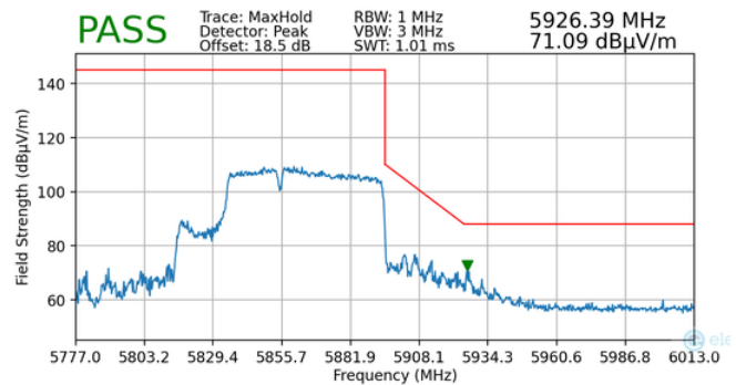
Plot 7-172. Radiated Upper Band Edge Plot MIMO (Peak – UNII Band 4)
