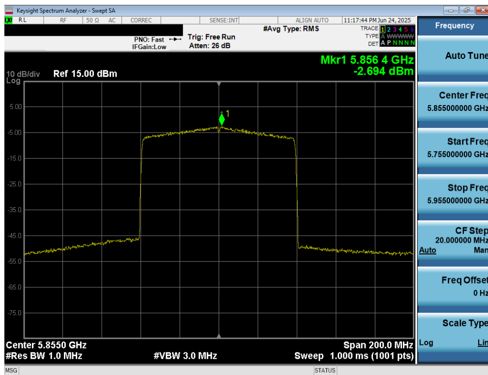
Plot 7-116. Power Spectral Density Plot MIMO ANT2 (80MHz BW 802.11be (UNII Band 3/4) – Ch. 171)
