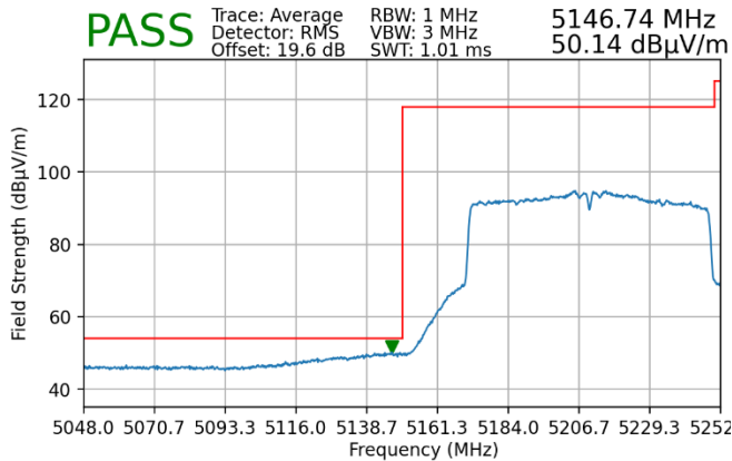
Plot 7-153. Radiated Lower Band Edge Plot MIMO (Average – UNII Band 1)
