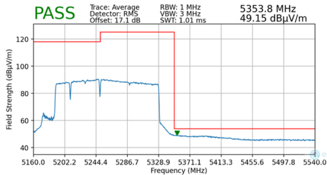
Plot 7-184. Radiated Upper Band Edge Plot MIMO (Average – UNII Band 2A)
