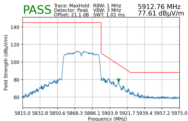
Plot 7-152. Radiated Upper Band Edge Plot MIMO (Peak – UNII Band 4)
