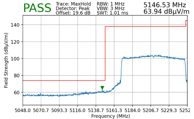
Plot 7-154. Radiated Lower Band Edge Plot MIMO (Peak – UNII Band 1)
