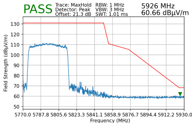
Plot 7-149. Radiated Upper Band Edge Plot MIMO (Peak – UNII Band 3)
