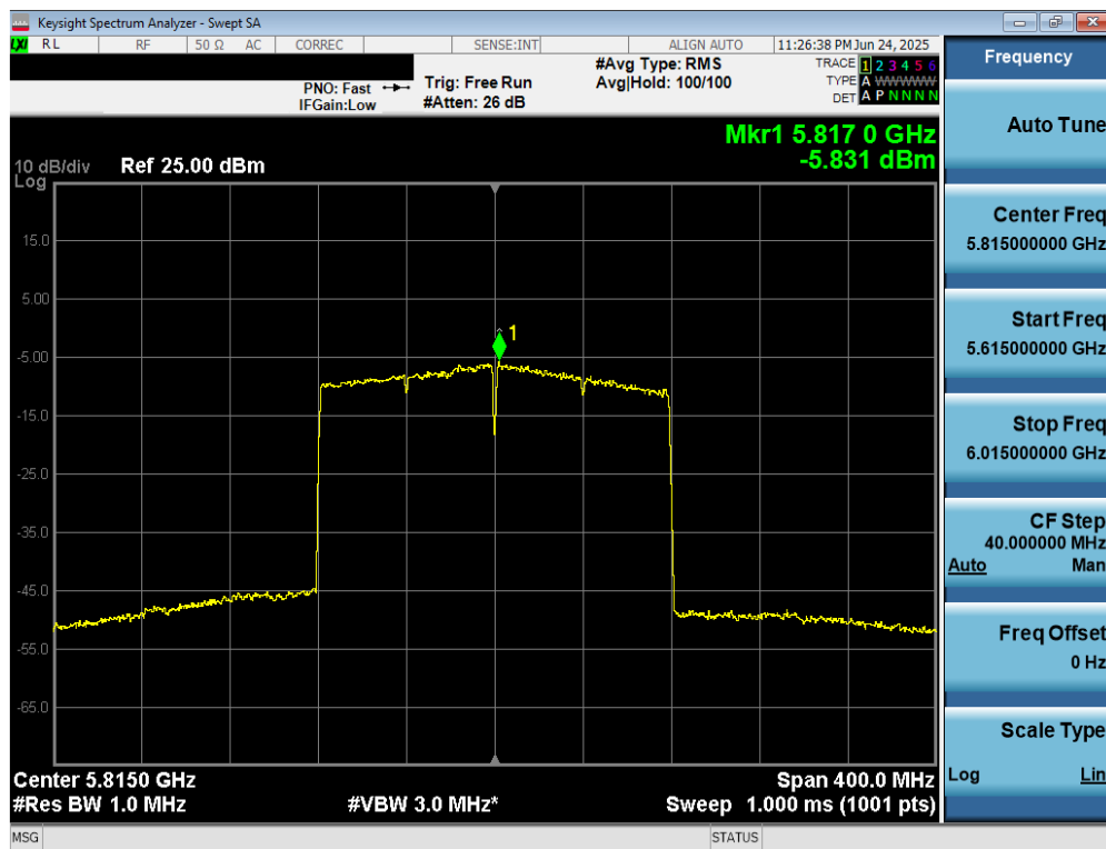
Plot 7-118. Power Spectral Density Plot MIMO ANT2 (160MHz BW 802.11be (UNII Band 3/4) – Ch. 163)
