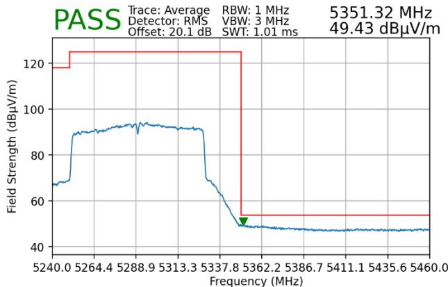
Plot 7-155. Radiated Upper Band Edge Plot MIMO (Average – UNII Band 2A)
