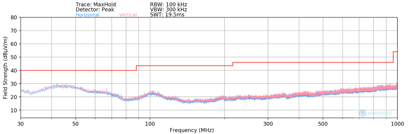
Plot 7-129. Radiated Spurious Plot below 1GHz MIMO 802.11b (2.4GHz – Ch. 6) + MIMO 802.11a (5GHz – Ch. 120)
