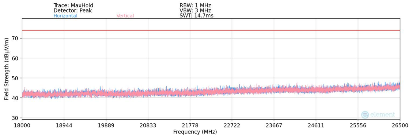
Plot 7-127. Radiated Spurious Plot 18GHz – 26.5GHz MIMO (802.11a)
