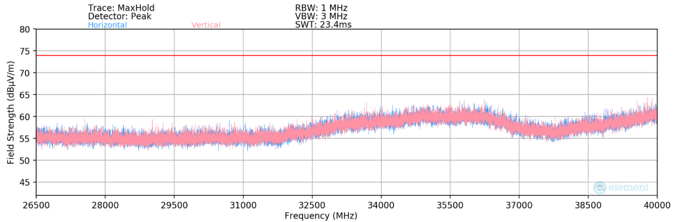
Plot 7-132. Radiated Spurious Plot below 26.5-40GHz MIMO 802.11b (2.4GHz – Ch.6) + MIMO 802.11a (5GHz – Ch. 120)
