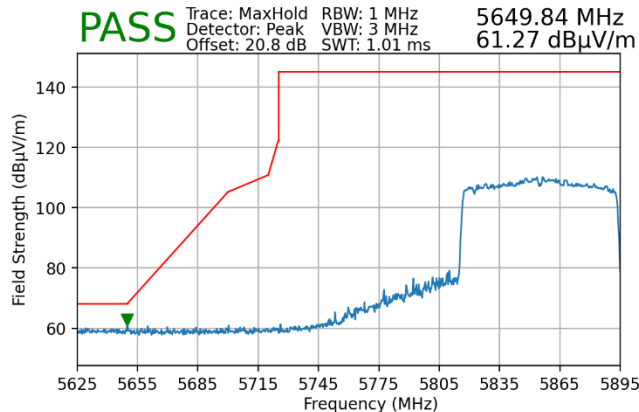
Plot 7-160. Radiated Lower Band Edge Plot MIMO (Peak – UNII Band 4)
