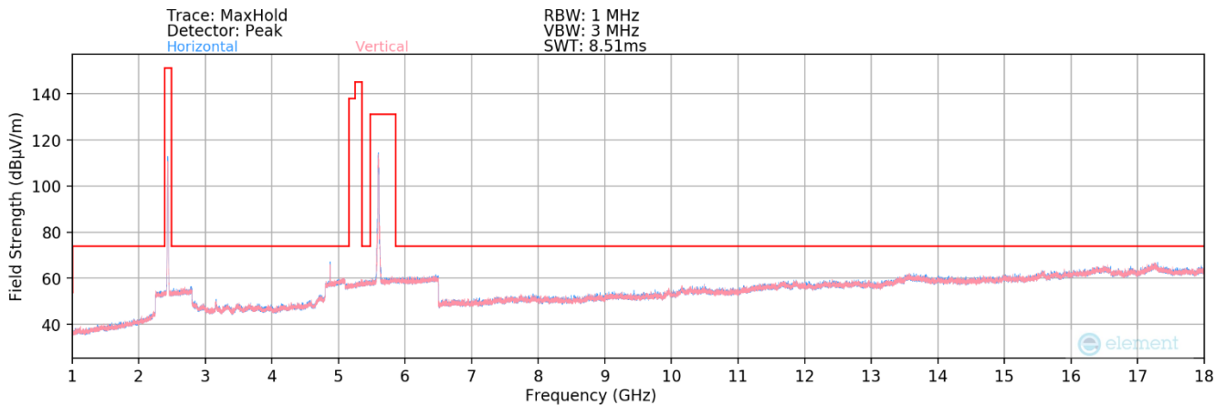
Plot 7-130. Radiated Spurious Plot below 1-18GHz MIMO 802.11b (2.4GHz – Ch.6) + MIMO 802.11a (5GHz – Ch. 120)
