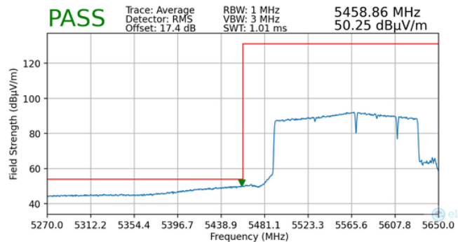
Plot 7-186. Radiated Lower Band Edge Plot MIMO (Average – UNII Band 2C)
