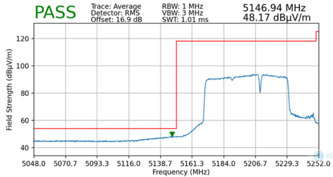
Plot 7-163. Radiated Lower Band Edge Plot MIMO (Average – UNII Band 1)
