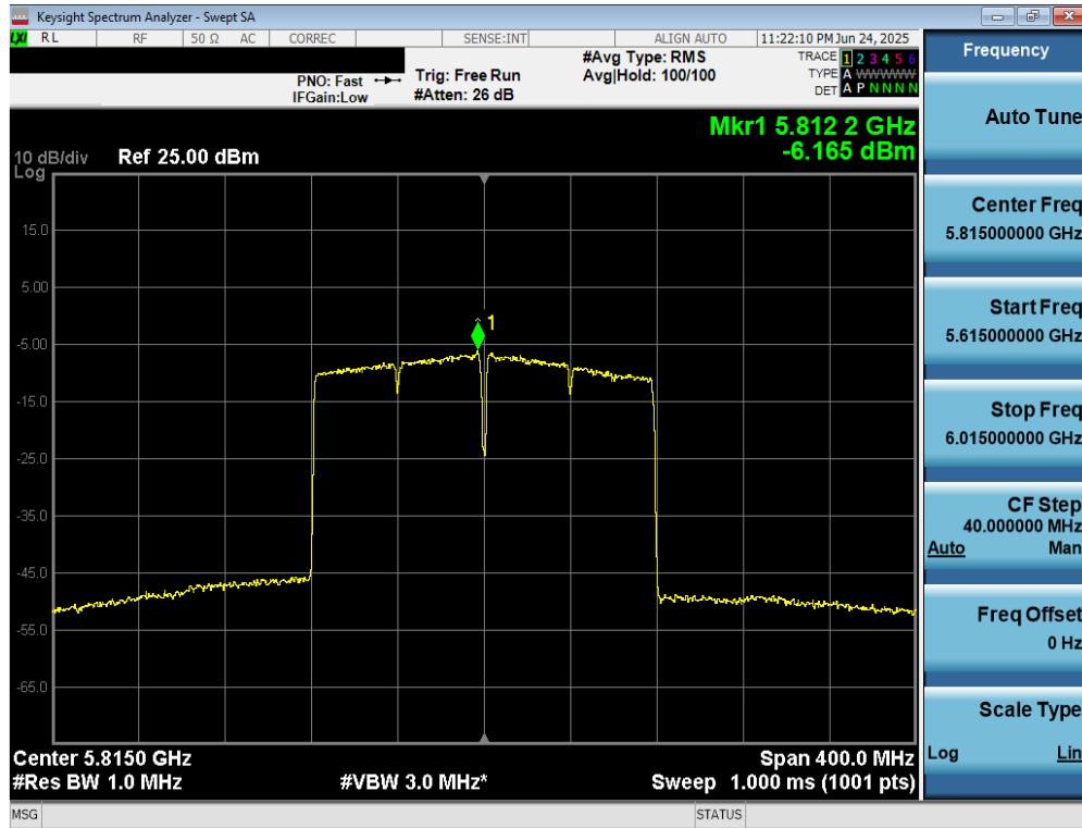
Plot 7-117. Power Spectral Density Plot MIMO ANT2 (160MHz BW 802.11ac (UNII Band 3/4) – Ch. 163)
