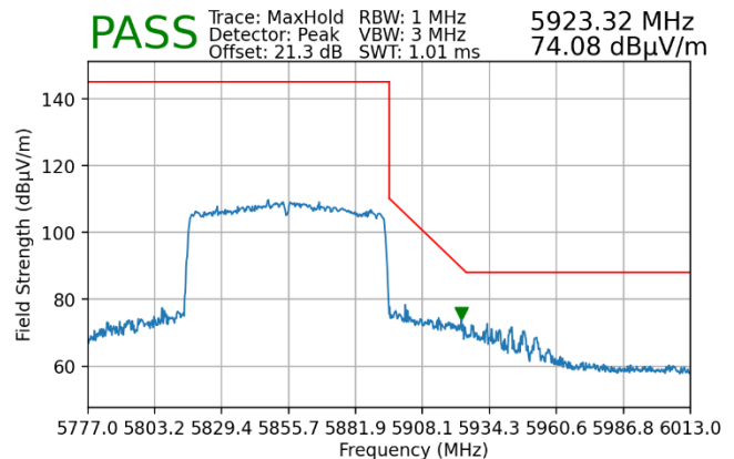
Plot 7-162. Radiated Upper Band Edge Plot MIMO (Peak – UNII Band 4)
