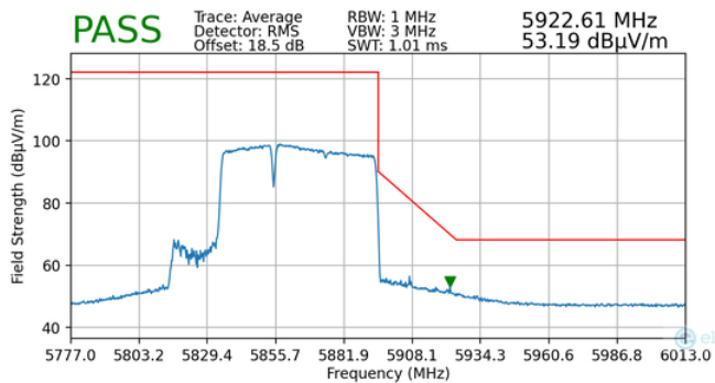
Plot 7-171. Radiated Upper Band Edge Plot MIMO (Average – UNII Band 4)
