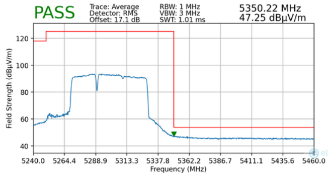
Plot 7-165. Radiated Upper Band Edge Plot MIMO (Average – UNII Band 2A)
