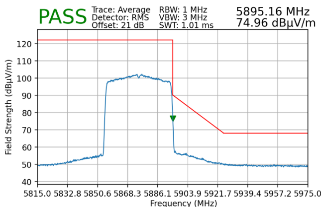
Plot 7-151. Radiated Upper Band Edge Plot MIMO (Average – UNII Band 4)
