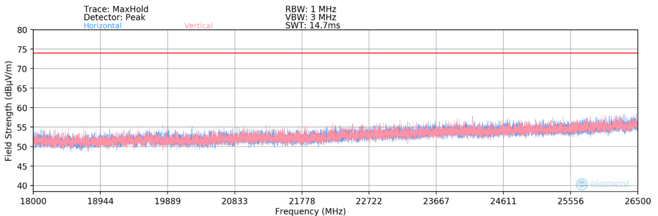
Plot 7-131. Radiated Spurious Plot below 18-26.5GHz MIMO 802.11b (2.4GHz – Ch.6) + MIMO 802.11a (5GHz – Ch. 120)
