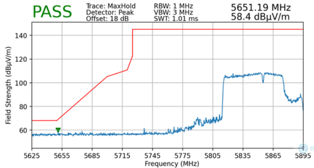
Plot 7-170. Radiated Lower Band Edge Plot MIMO (Peak – UNII Band 4)
