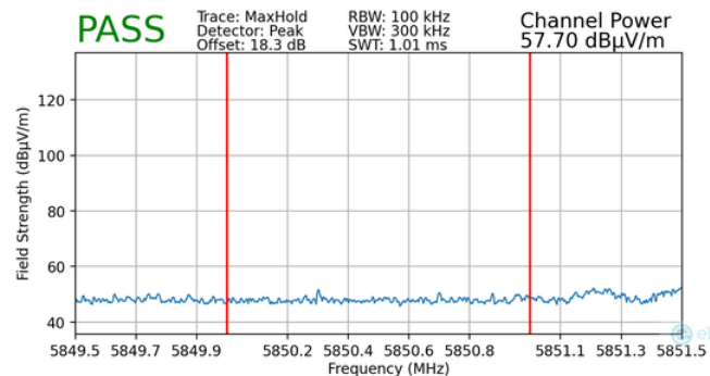
Plot 7-169. Radiated Upper Band Edge Plot MIMO (Peak – UNII Band 3)
