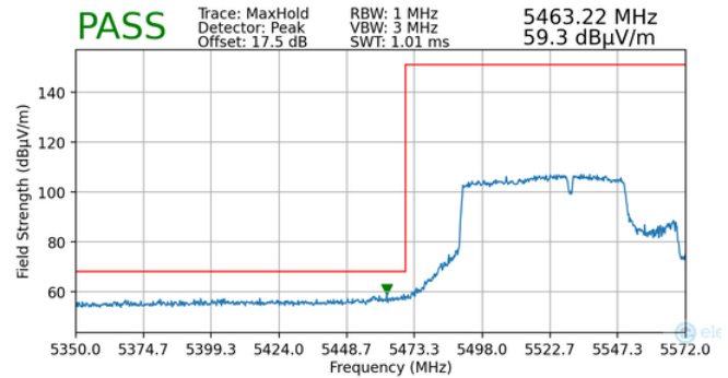
Plot 7-168. Radiated Lower Band Edge Plot MIMO (Peak – UNII Band 2C)
