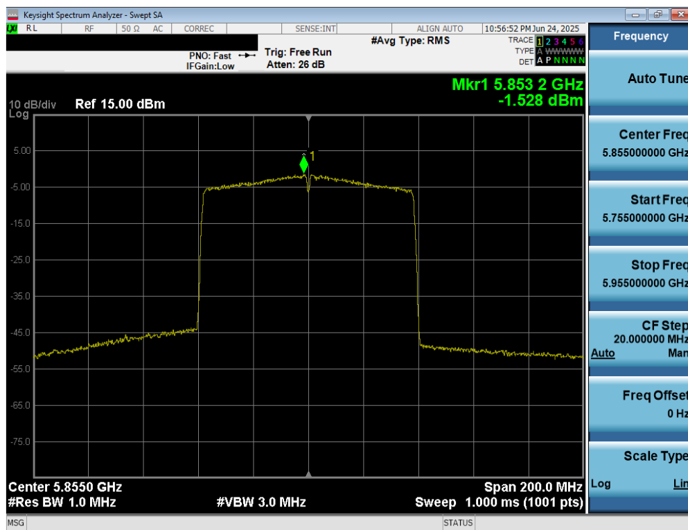
Plot 7-115. Power Spectral Density Plot MIMO ANT2 (80MHz BW 802.11ac (UNII Band 3/4) – Ch. 171)
