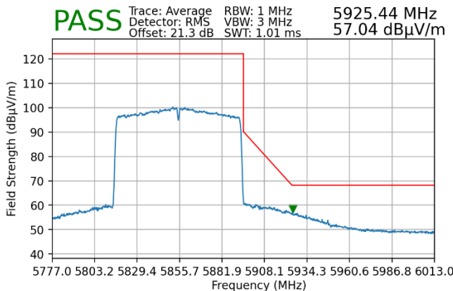
Plot 7-161. Radiated Upper Band Edge Plot MIMO (Average – UNII Band 4)
