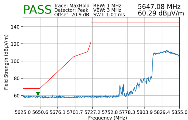
Plot 7-150. Radiated Lower Band Edge Plot MIMO (Peak – UNII Band 4)
