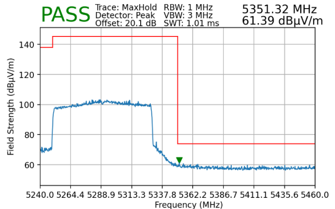
Plot 7-156. Radiated Upper Band Edge Plot MIMO (Peak – UNII Band 2A)
