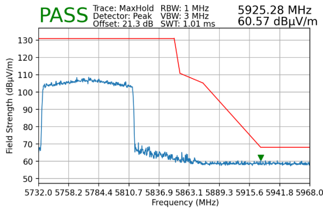
Plot 7-159. Radiated Upper Band Edge Plot MIMO (Peak – UNII Band 3)
