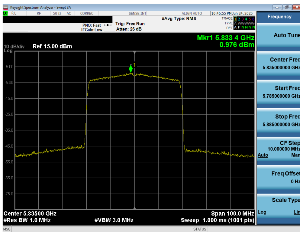
Plot 7-114. Power Spectral Density Plot MIMO ANT2 (40MHz BW 802.11be (UNII Band 3/4) – Ch. 167)
