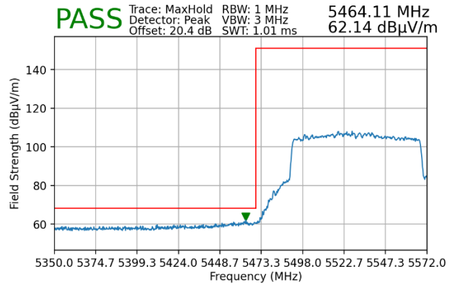
Plot 7-158. Radiated Lower Band Edge Plot MIMO (Peak – UNII Band 2C)
