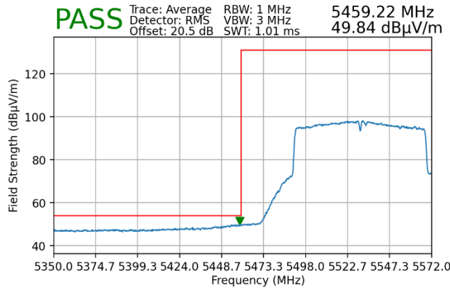
Plot 7-157. Radiated Lower Band Edge Plot MIMO (Average – UNII Band 2C)
