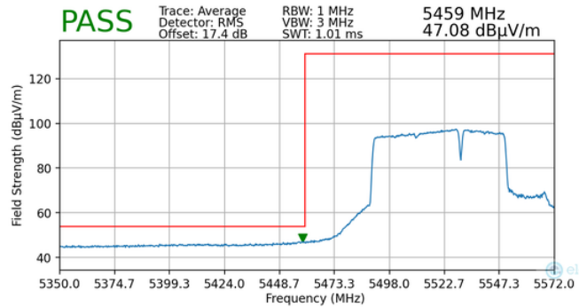
Plot 7-167. Radiated Lower Band Edge Plot MIMO (Average – UNII Band 2C)
