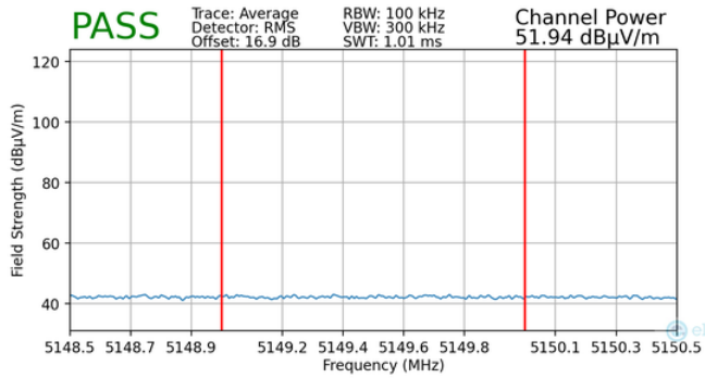
Plot 7-173. Radiated Lower Band Edge Plot MIMO (Average – UNII Band 1)
