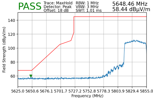
Plot 7-163. Radiated Lower Band Edge Plot MIMO (Peak - UNII Band 4 - 484 Tones)
