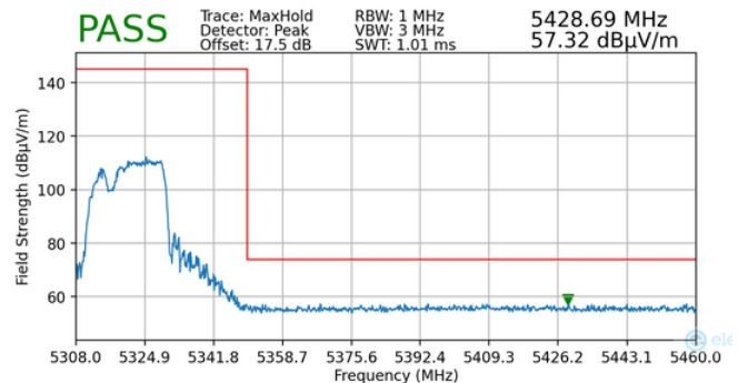
Plot 7-139. Radiated Upper Band Edge Plot MIMO (Peak – UNII Band 2A – 106+26 Tones)
