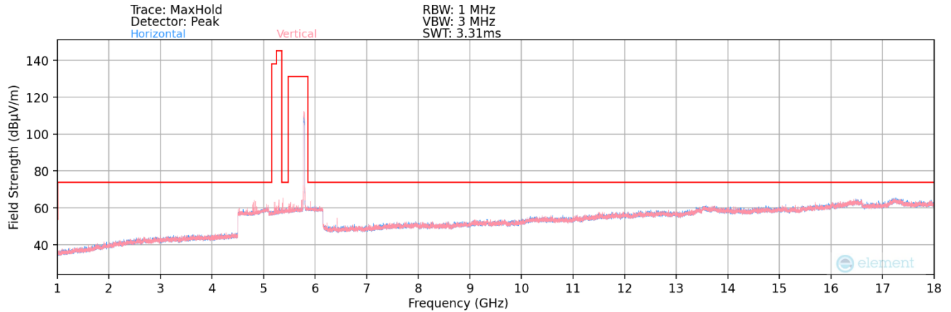
Plot 7-132. Radiated Spurious Plot above 1GHz MIMO (802.11ax –UNII 3 Ch. 157)
