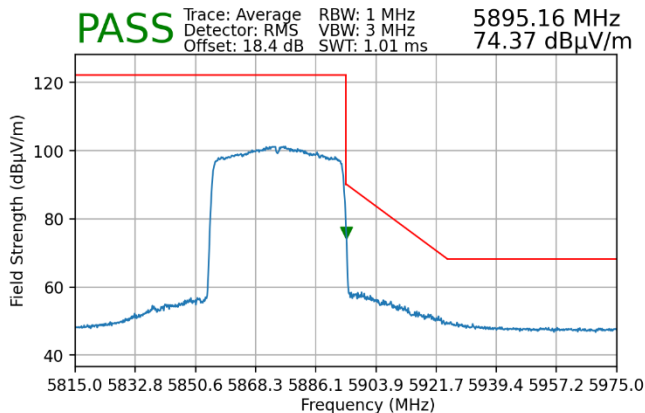
Plot 7-164. Radiated Upper Band Edge Plot MIMO (Average - UNII Band 4 - 484 Tones)
