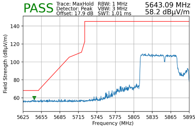
Plot 7-183. Radiated Lower Band Edge Plot MIMO (Peak – UNII Band 4 – 484+242 Tones)
