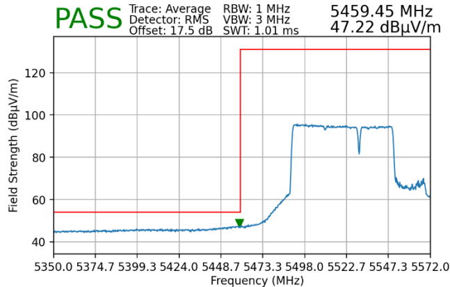
Plot 7-180. Radiated Lower Band Edge Plot MIMO (Average – UNII Band 2C – 484+242 Tones)
