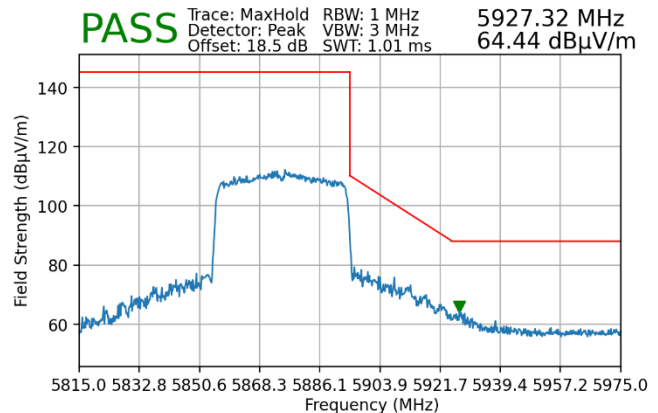
Plot 7-165. Radiated Upper Band Edge Plot MIMO (Peak - UNII Band 4 - 484 Tones)
