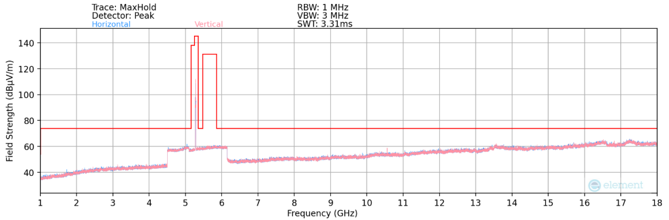
Plot 7-123. Radiated Spurious Plot above 1GHz MIMO (802.11ax – UNII 2A Ch. 56)
