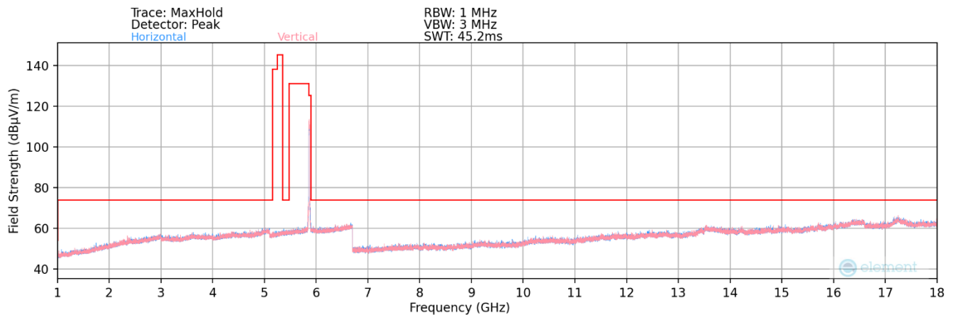
Plot 7-133. Radiated Spurious Plot above 1GHz MIMO (802.11ax –UNII 4 Ch. 173)
