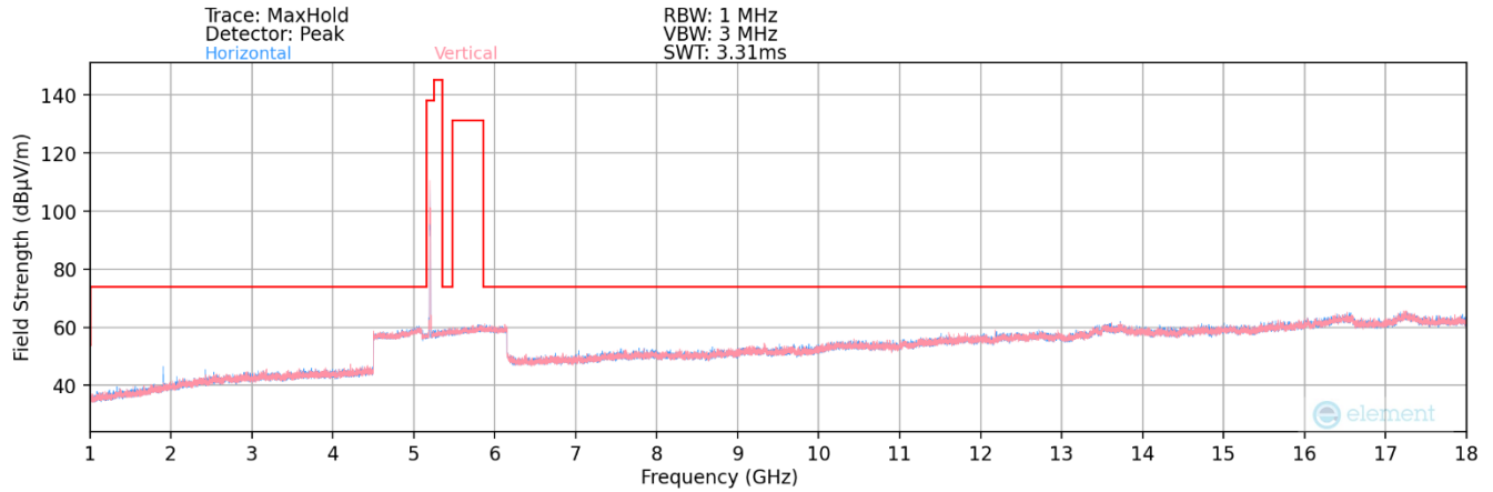
Plot 7-122. Radiated Spurious Plot above 1GHz MIMO (802.11ax – UNII 1 Ch. 40)
