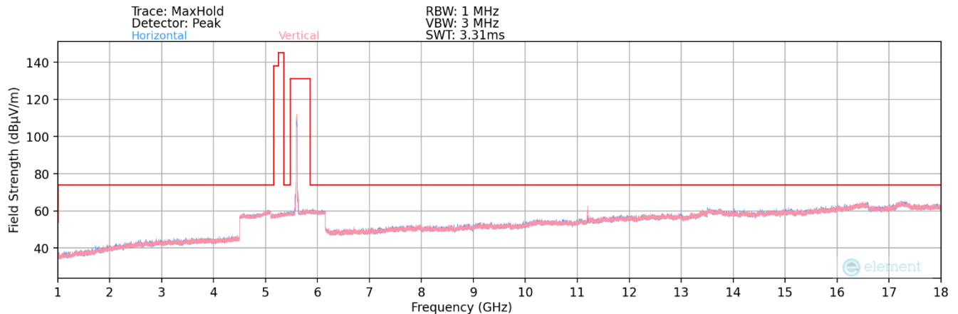
Plot 7-131. Radiated Spurious Plot above 1GHz MIMO (802.11ax – UNII 2C Ch. 120)
