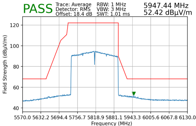
Plot 7-193. Radiated Upper Band Edge Plot MIMO (Average - UNII Band 4 - 2x996 Tones)
