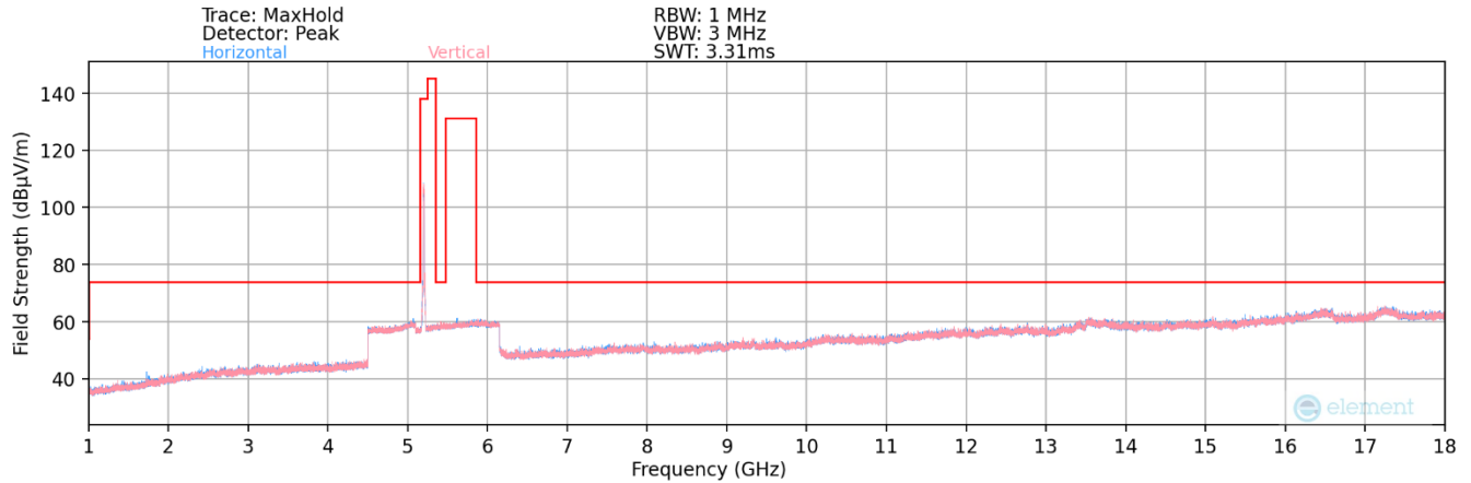
Plot 7-129. Radiated Spurious Plot above 1GHz MIMO (802.11ax – UNII 1 Ch. 40)
