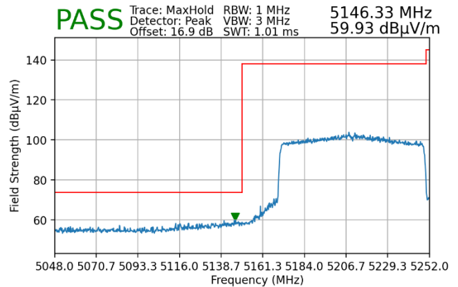
Plot 7-167. Radiated Lower Band Edge Plot MIMO (Peak – UNII Band 1 – 996 Tones)
