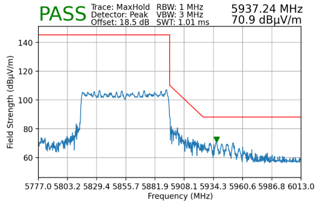
Plot 7-175. Radiated Upper Band Edge Plot MIMO (Peak - UNII Band 4 - 996 Tones)
