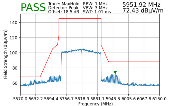
Plot 7-194. Radiated Upper Band Edge Plot MIMO (Peak - UNII Band 4 - 2x996 Tones)
