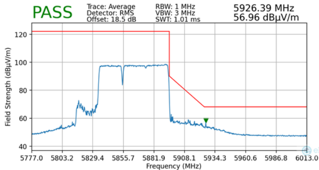
Plot 7-184. Radiated Upper Band Edge Plot MIMO (Average – UNII Band 4 – 484+242 Tones)
