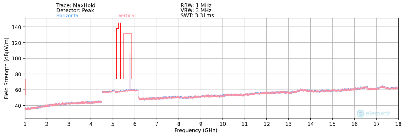
Plot 7-125. Radiated Spurious Plot above 1GHz MIMO (802.11ax –UNII 3 Ch. 157)
