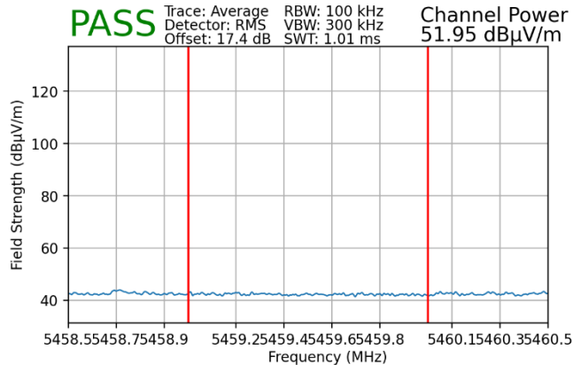
Plot 7-190. Radiated Lower Band Edge Plot MIMO (Average – UNII Band 2C – 2x996 Tones)
