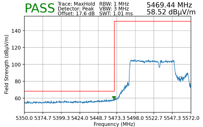
Plot 7-181. Radiated Lower Band Edge Plot MIMO (Peak – UNII Band 2C – 484+242 Tones)
