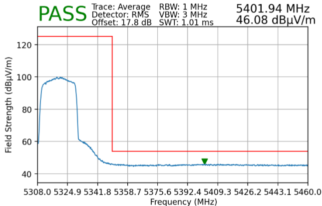
Plot 7-148. Radiated Upper Band Edge Plot MIMO (Average – UNII Band 2A – 242 Tones)
