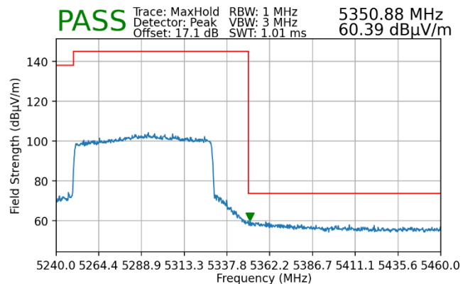
Plot 7-169. Radiated Upper Band Edge Plot MIMO (Peak – UNII Band 2A – 996 Tones)
