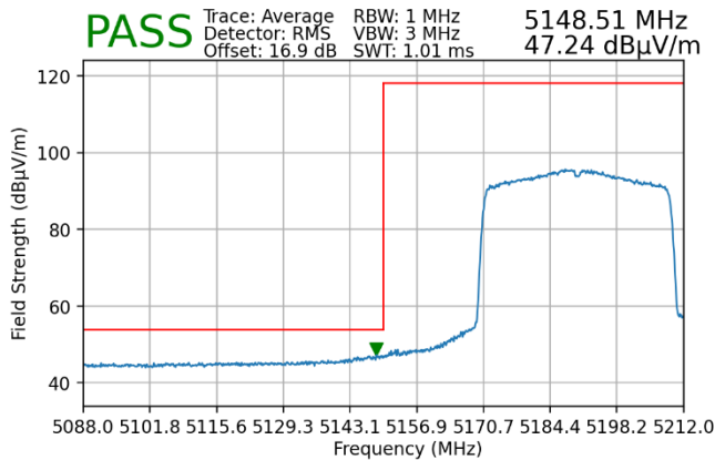
Plot 7-156. Radiated Lower Band Edge Plot MIMO (Average – UNII Band 1 – 484 Tones)
