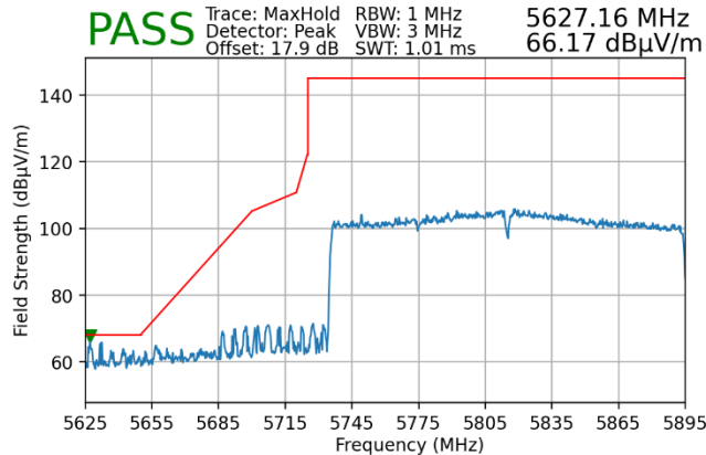
Plot 7-192. Radiated Lower Band Edge Plot MIMO (Peak - UNII Band 4 - 2x996 Tones)
