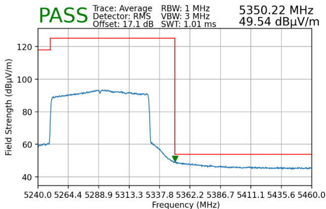
Plot 7-168. Radiated Upper Band Edge Plot MIMO (Average – UNII Band 2A – 996 Tones)
