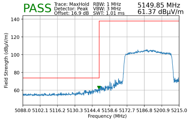
Plot 7-157. Radiated Lower Band Edge Plot MIMO (Peak – UNII Band 1 – 484 Tones)
