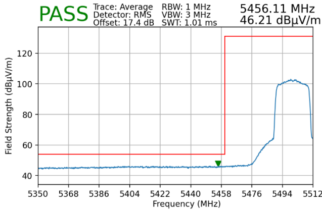
Plot 7-150. Radiated Lower Band Edge Plot MIMO (Average – UNII Band 2C – 242 Tones)
