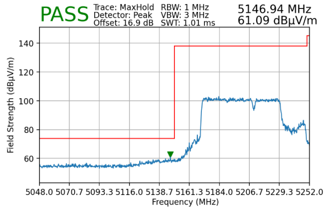
Plot 7-177. Radiated Lower Band Edge Plot MIMO (Peak – UNII Band 1 – 484+242 Tones)
