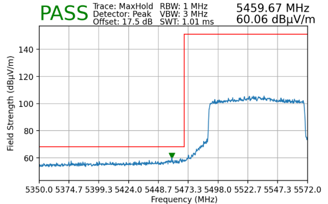
Plot 7-171. Radiated Lower Band Edge Plot MIMO (Peak - UNII Band 2C - 996 Tones)
