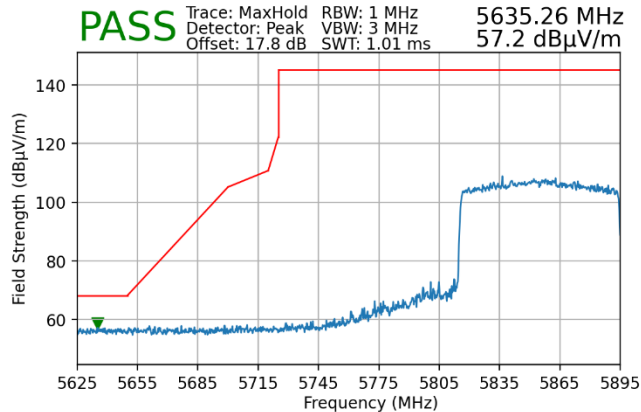
Plot 7-173. Radiated Lower Band Edge Plot MIMO (Peak - UNII Band 4 - 996 Tones)
