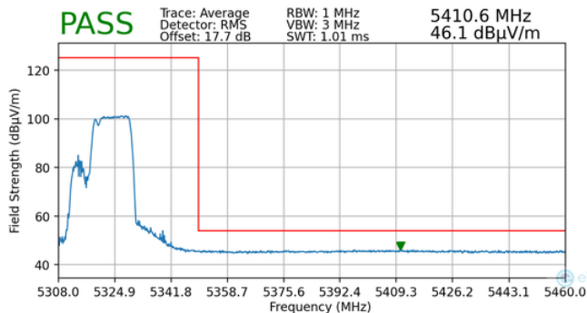
Plot 7-138. Radiated Upper Band Edge Plot MIMO (Average – UNII Band 2A – 106+26 Tones)
