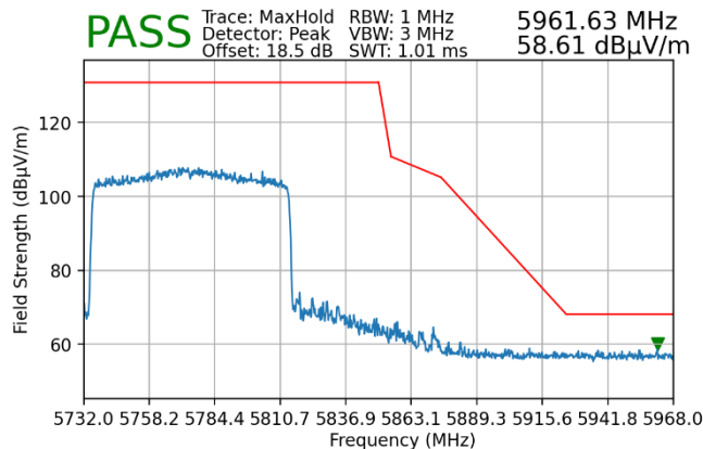
Plot 7-172. Radiated Upper Band Edge Plot MIMO (Peak - UNII Band 3 - 996 Tones)
