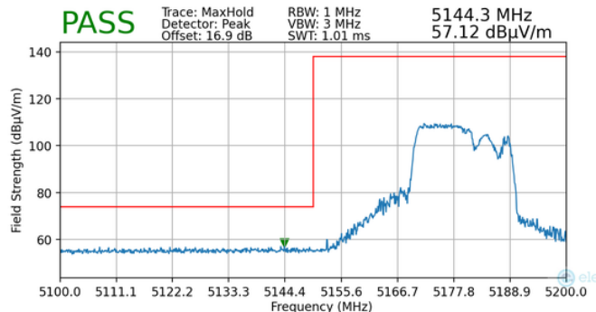
Plot 7-137. Radiated Lower Band Edge Plot MIMO (Peak – UNII Band 1 – 106+26 Tones)
