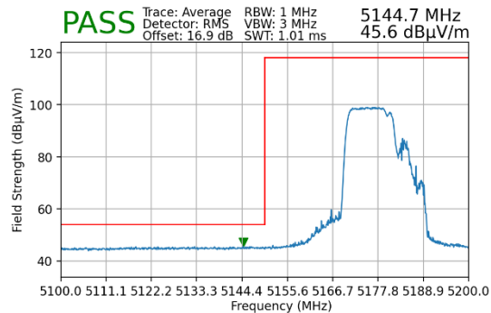
Plot 7-136. Radiated Lower Band Edge Plot MIMO (Average – UNII Band 1 – 106+26 Tones)
