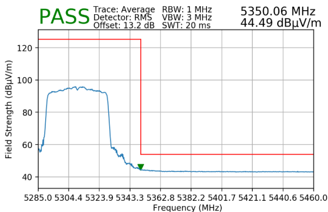
Plot 7-158. Radiated Upper Band Edge Plot MIMO (Average – UNII Band 2A – 484 Tones)
