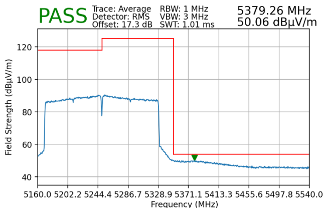
Plot 7-188. Radiated Upper Band Edge Plot MIMO (Average – UNII Band 2A – 2x996 Tones)
