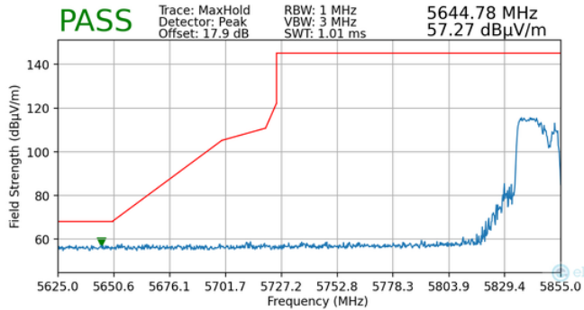
Plot 7-143. Radiated Lower Band Edge Plot MIMO (Peak – UNII Band 4 – 106+26 Tones)
