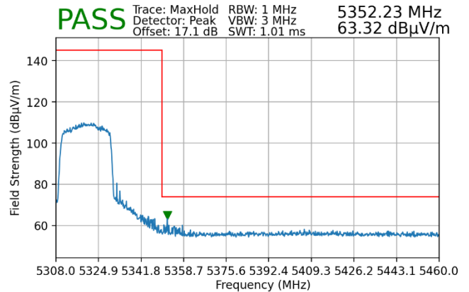
Plot 7-149. Radiated Upper Band Edge Plot MIMO (Peak – UNII Band 2A – 242 Tones)
