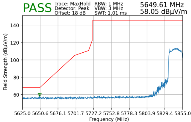
Plot 7-153. Radiated Lower Band Edge Plot MIMO (Peak - UNII Band 4 - 242 Tones)
