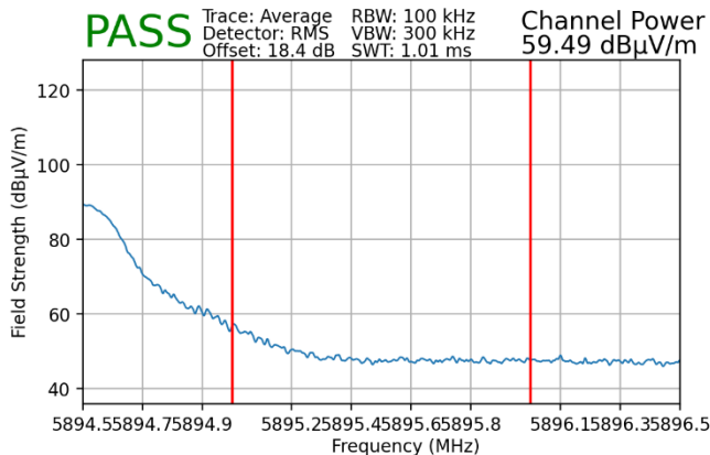
Plot 7-154. Radiated Upper Band Edge Plot MIMO (Average - UNII Band 4 - 242 Tones)
