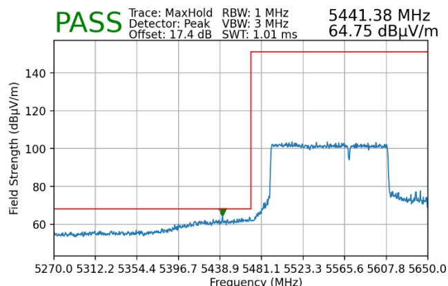
Plot 7-200. Radiated Lower Band Edge Plot MIMO (Peak – UNII Band 2C – 996+484 Tones)
