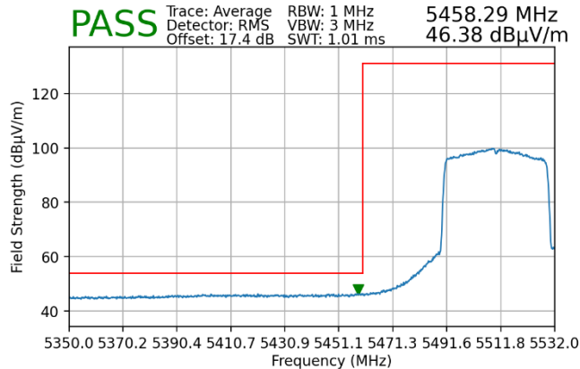
Plot 7-160. Radiated Lower Band Edge Plot MIMO (Average – UNII Band 2C – 484 Tones)
