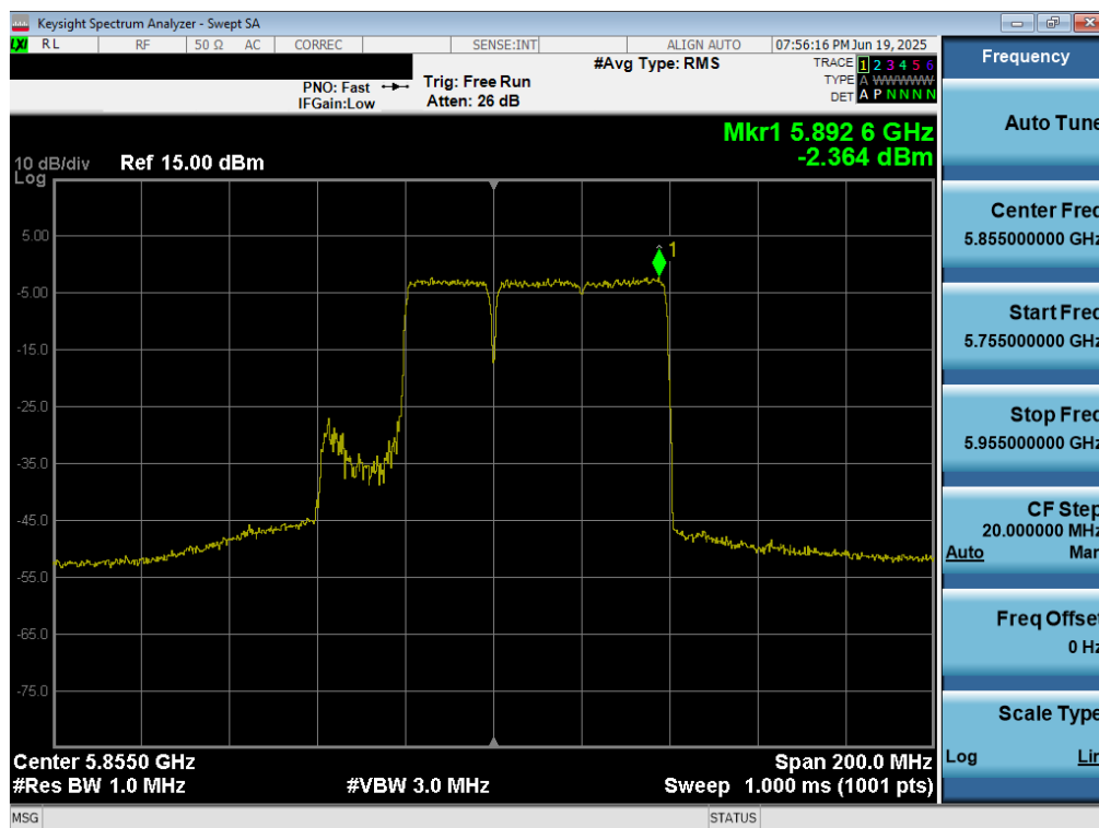
Plot 7-120. Power Spectral Density Plot MIMO ANT2 (80MHz BW 802.11be – 484+242 Tones (UNII Band 3/4) – Ch. 171)
