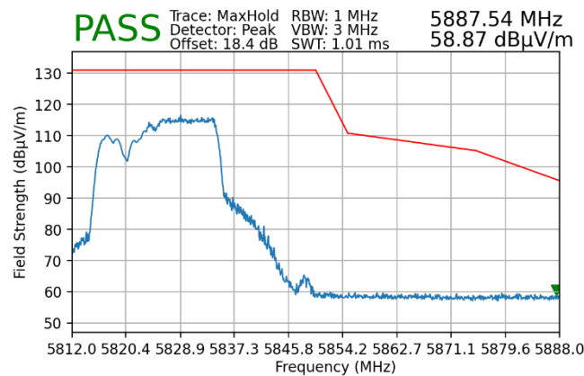
Plot 7-142. Radiated Upper Band Edge Plot MIMO (Peak – UNII Band 3 – 106+26 Tones)
