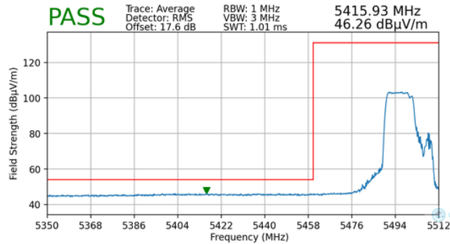
Plot 7-140. Radiated Lower Band Edge Plot MIMO (Average – UNII Band 2C – 106+26 Tones)
