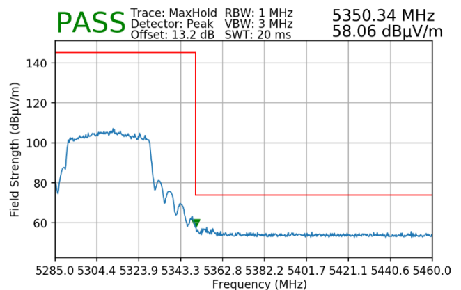
Plot 7-159. Radiated Upper Band Edge Plot MIMO (Peak – UNII Band 2A – 484 Tones)
