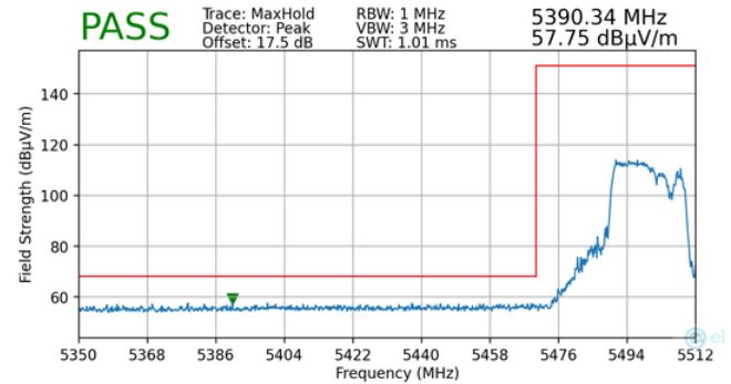
Plot 7-141. Radiated Lower Band Edge Plot MIMO (Peak – UNII Band 2C – 106+26 Tones)
