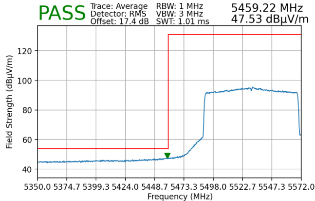
Plot 7-170. Radiated Lower Band Edge Plot MIMO (Average - UNII Band 2C - 996 Tones)
