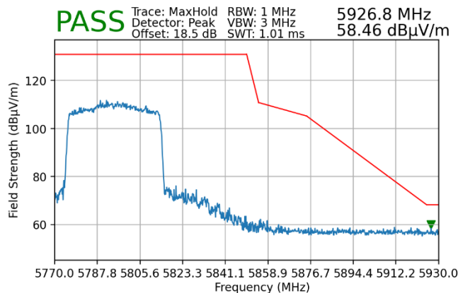
Plot 7-162. Radiated Upper Band Edge Plot MIMO (Peak – UNII Band 3 – 484 Tones)
