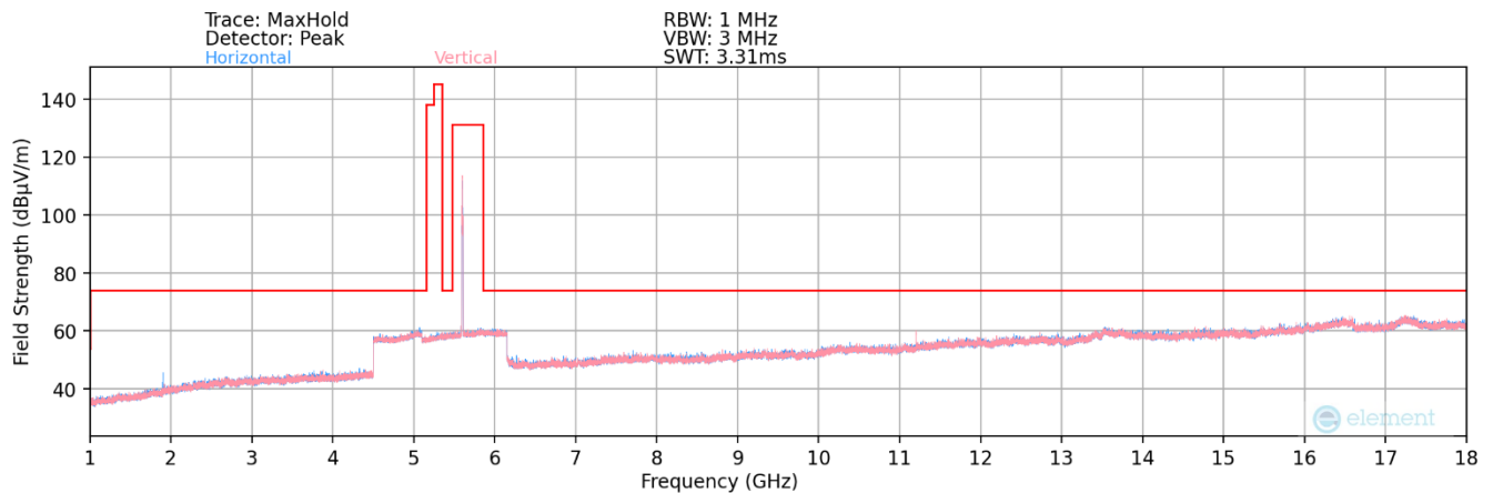
Plot 7-124. Radiated Spurious Plot above 1GHz MIMO (802.11ax – UNII 2C Ch. 120)
