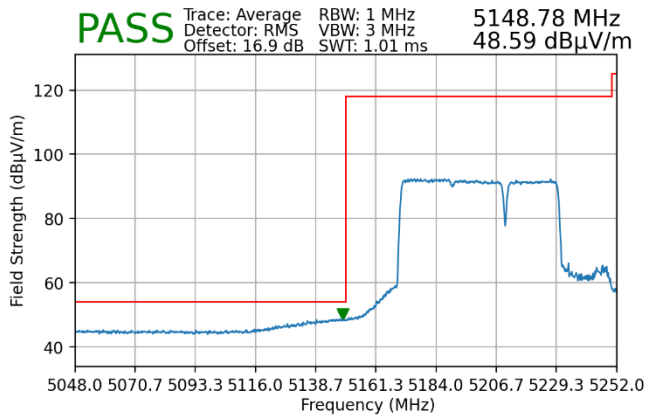
Plot 7-176. Radiated Lower Band Edge Plot MIMO (Average – UNII Band 1 – 484+242 Tones)
