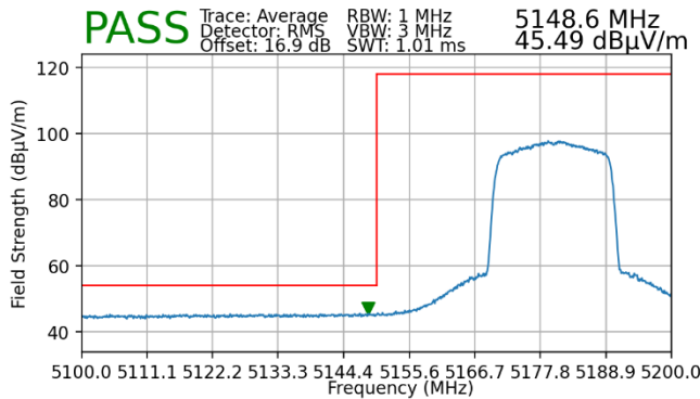
Plot 7-146. Radiated Lower Band Edge Plot MIMO (Average – UNII Band 1 – 242 Tones)
