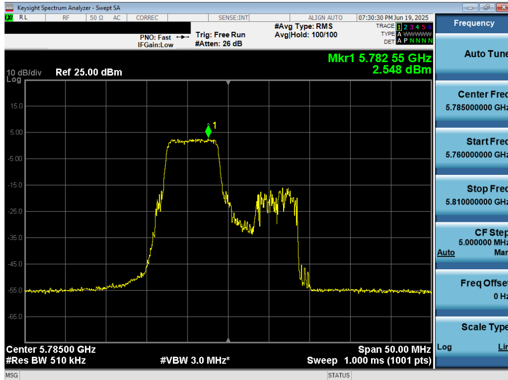
Plot 7-117. Power Spectral Density Plot MIMO ANT2 (20MHz BW 802.11be – 106+26 Tones (UNII Band 3) – Ch. 157)
