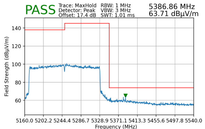
Plot 7-189. Radiated Upper Band Edge Plot MIMO (Peak – UNII Band 2A – 2x996 Tones)
