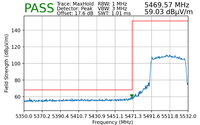
Plot 7-161. Radiated Lower Band Edge Plot MIMO (Peak – UNII Band 2C – 484 Tones)
