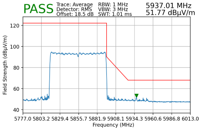
Plot 7-174. Radiated Upper Band Edge Plot MIMO (Average - UNII Band 4 - 996 Tones)
