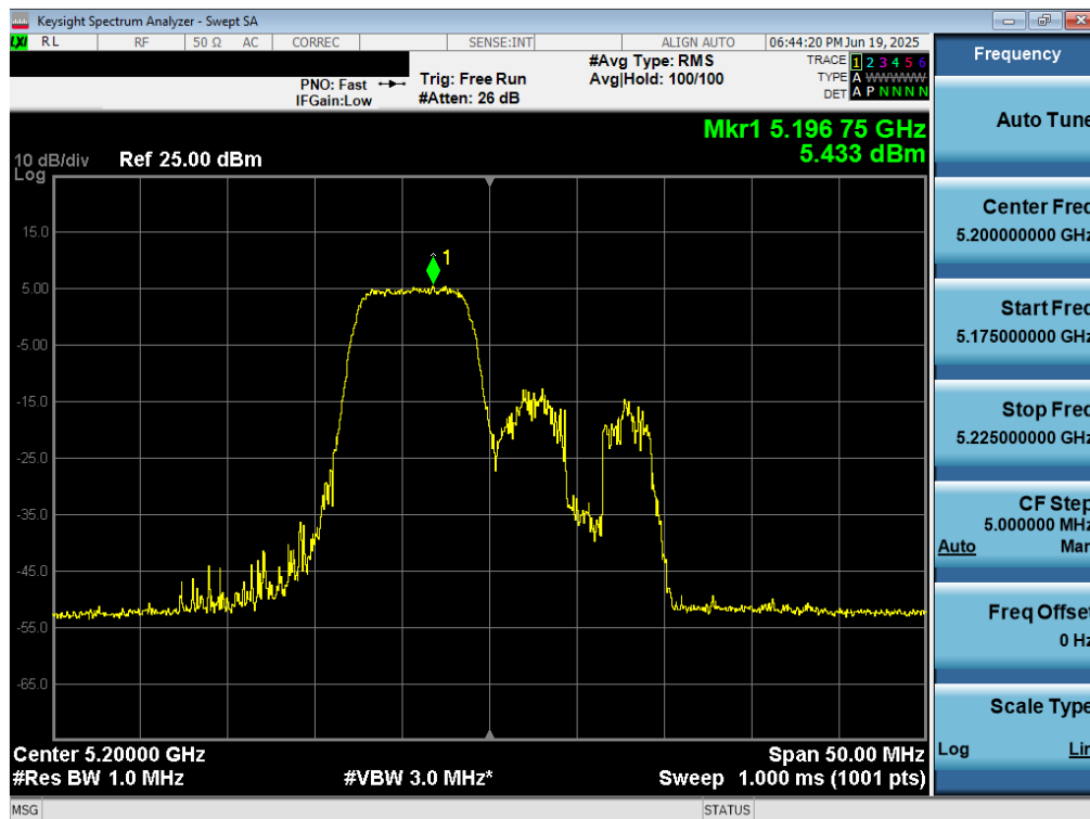
Plot 7-114. Power Spectral Density Plot MIMO ANT2 (20MHz BW 802.11be – 106+26 Tones (UNII Band 1) – Ch. 40)
