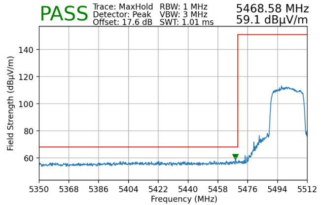
Plot 7-151. Radiated Lower Band Edge Plot MIMO (Peak – UNII Band 2C – 242 Tones)
