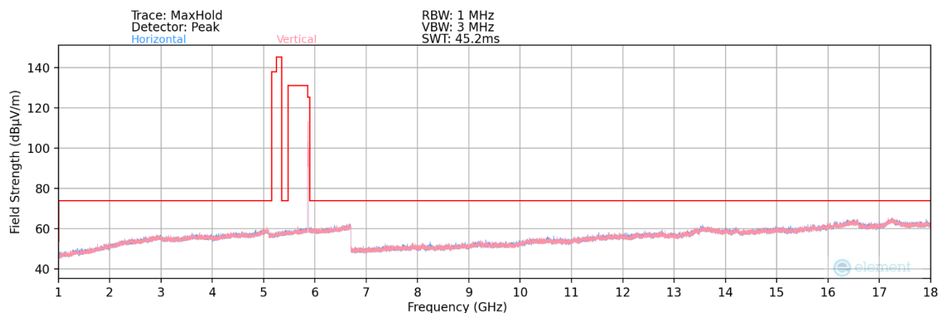
Plot 7-126. Radiated Spurious Plot above 1GHz MIMO (802.11ax –UNII 4 Ch. 173)
