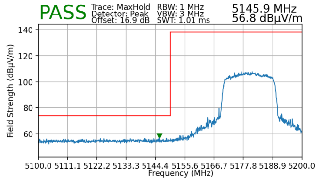
Plot 7-147. Radiated Lower Band Edge Plot MIMO (Peak – UNII Band 1 – 242 Tones)
