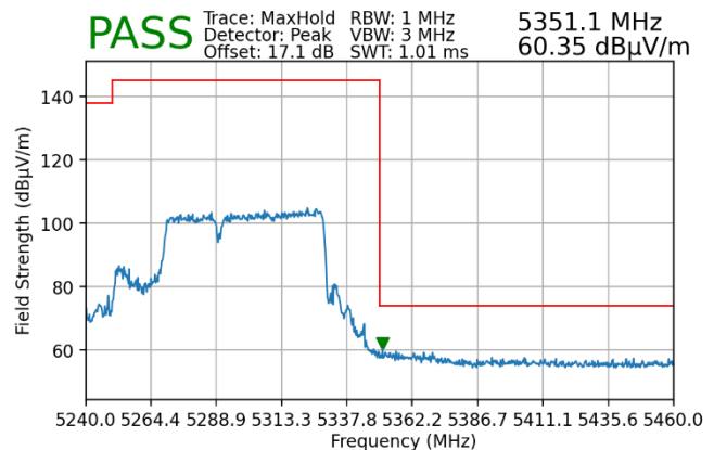
Plot 7-179. Radiated Upper Band Edge Plot MIMO (Peak – UNII Band 2A – 484+242 Tones)
