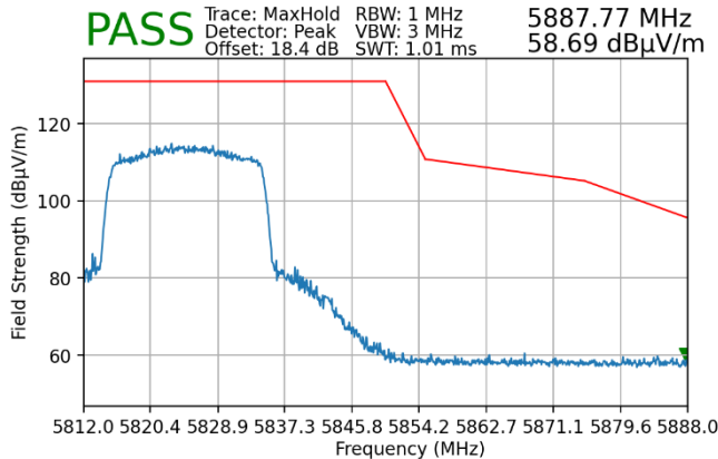
Plot 7-152. Radiated Upper Band Edge Plot MIMO (Peak – UNII Band 3 – 242 Tones)
