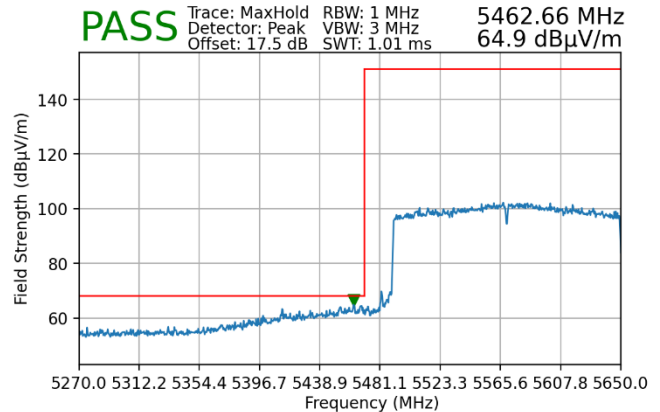
Plot 7-191. Radiated Lower Band Edge Plot MIMO (Peak – UNII Band 2C – 2x996 Tones)
