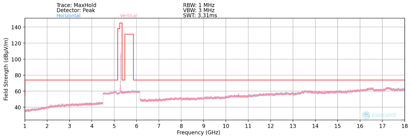
Plot 7-130. Radiated Spurious Plot above 1GHz MIMO (802.11ax – UNII 2A Ch. 56)
