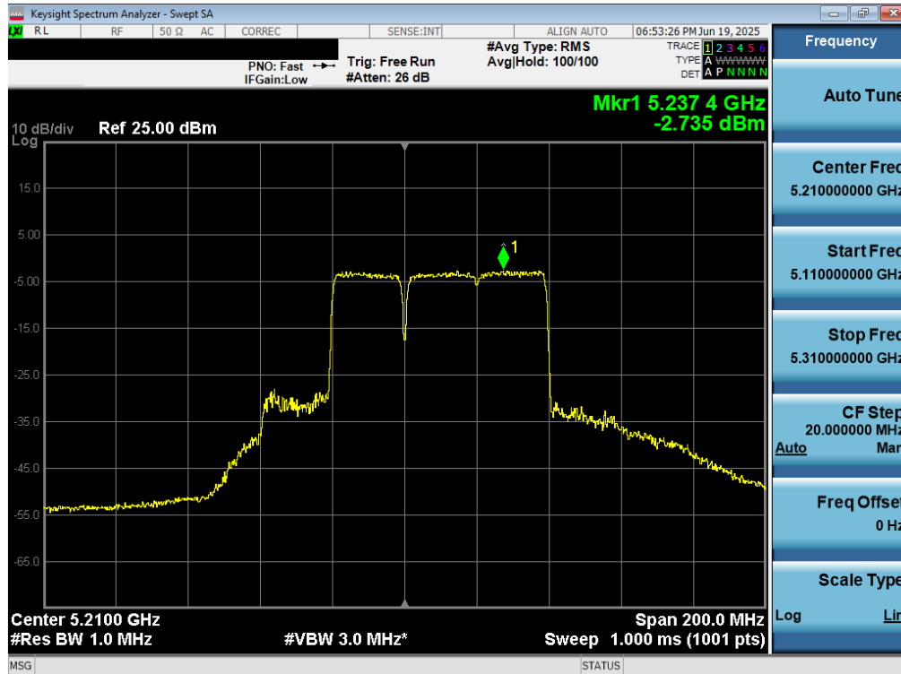
Plot 7-115. Power Spectral Density Plot MIMO ANT2 (80MHz BW 802.11be – 484+242 Tones (UNII Band 1) – Ch. 42)
