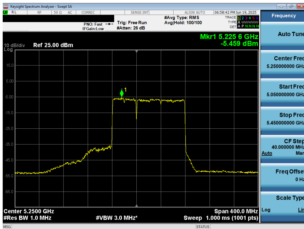
Plot 7-116. Power Spectral Density Plot MIMO ANT2 (160MHz BW 802.11be – 996+484 Tones (UNII Band 1/2A) – Ch. 50)
