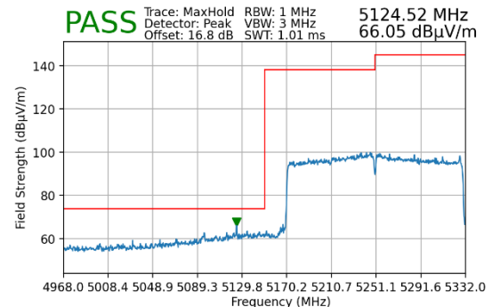
Plot 7-187. Radiated Lower Band Edge Plot MIMO (Peak – UNII Band 1 – 2x996 Tones)
