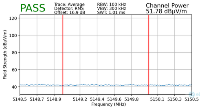
Plot 7-195. Radiated Lower Band Edge Plot MIMO (Average – UNII Band 1 – 996+484 Tones)
