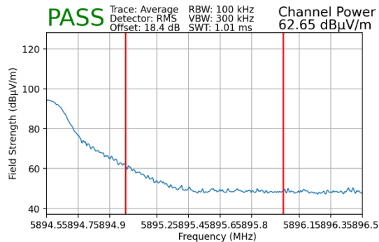
Plot 7-144. Radiated Upper Band Edge Plot MIMO (Average – UNII Band 4 – 106+26 Tones)
