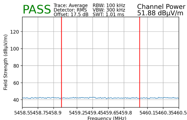
Plot 7-199. Radiated Lower Band Edge Plot MIMO (Average – UNII Band 2C – 996+484 Tones)
