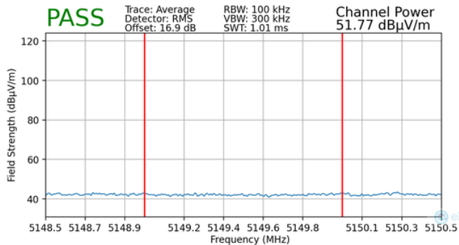
Plot 7-186. Radiated Lower Band Edge Plot MIMO (Average – UNII Band 1 – 2x996 Tones)
