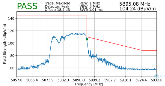
Plot 7-145. Radiated Upper Band Edge Plot MIMO (Peak – UNII Band 4 – 106+26 Tones)
