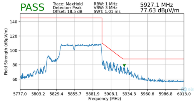
Plot 7-185. Radiated Upper Band Edge Plot MIMO (Peak – UNII Band 4 – 484+242 Tones)
