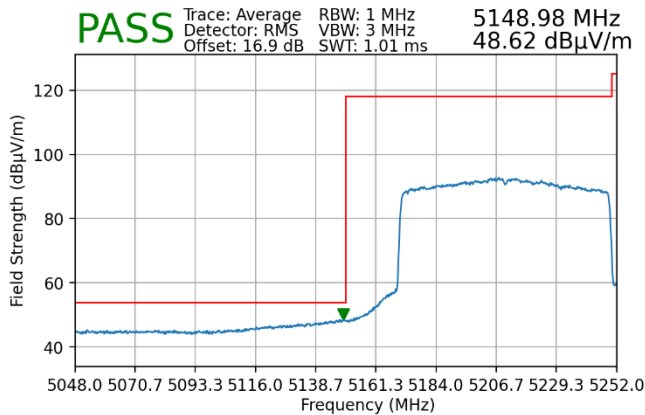
Plot 7-166. Radiated Lower Band Edge Plot MIMO (Average – UNII Band 1 – 996 Tones)
