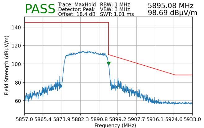
Plot 7-155. Radiated Upper Band Edge Plot MIMO (Peak - UNII Band 4 - 242 Tones)
