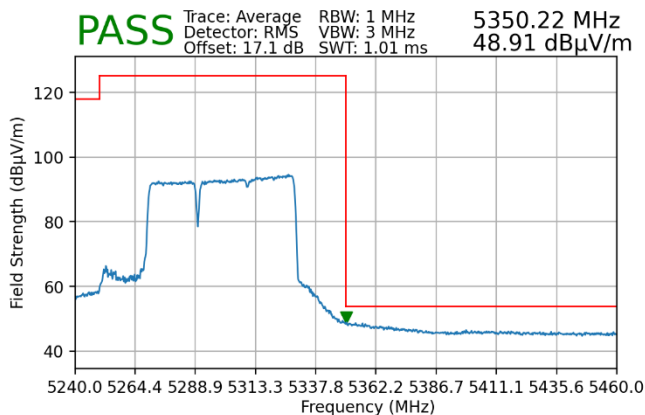
Plot 7-178. Radiated Upper Band Edge Plot MIMO (Average – UNII Band 2A – 484+242 Tones)
