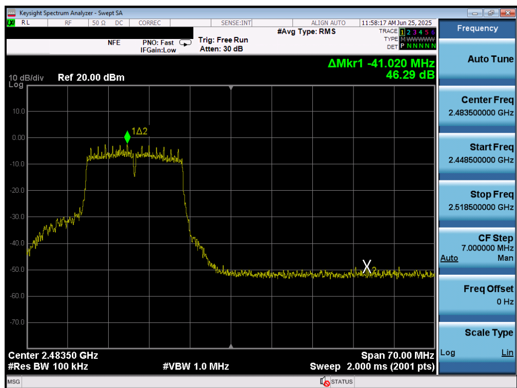
Plot 7-71. Band Edge Plot MIMO ANT2 (802.11g – Ch. 12)
