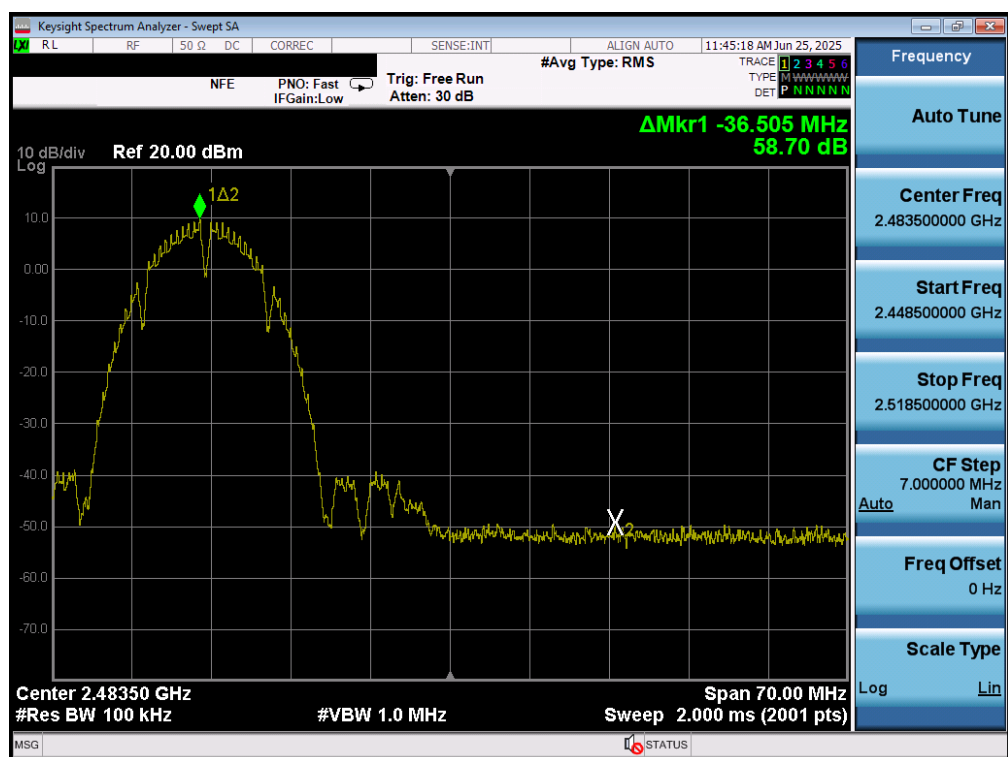
Plot 7-66. Band Edge Plot MIMO ANT2 (802.11b – Ch. 11)
