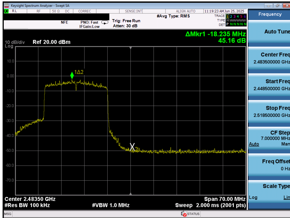
Plot 7-63. Band Edge Plot MIMO ANT1 (802.11ax/be (2.4GHz) – Ch. 12)
