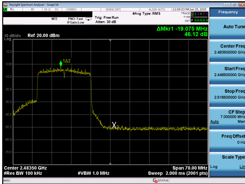
Plot 7-79. Band Edge Plot MIMO ANT2 (802.11ax/be (2.4GHz) – Ch. 12)
