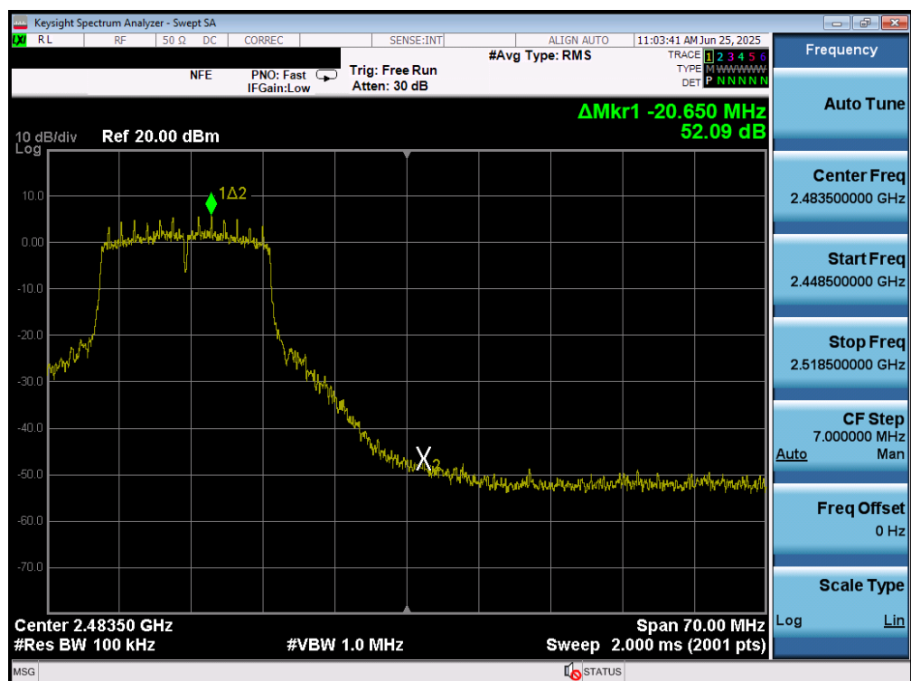
Plot 7-54. Band Edge Plot MIMO ANT1 (802.11g - Ch. 11)
