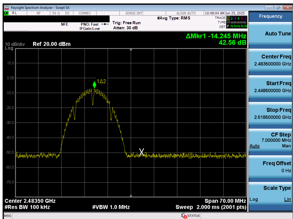
Plot 7-52. Band Edge Plot MIMO ANT1 (802.11b – Ch. 13)
