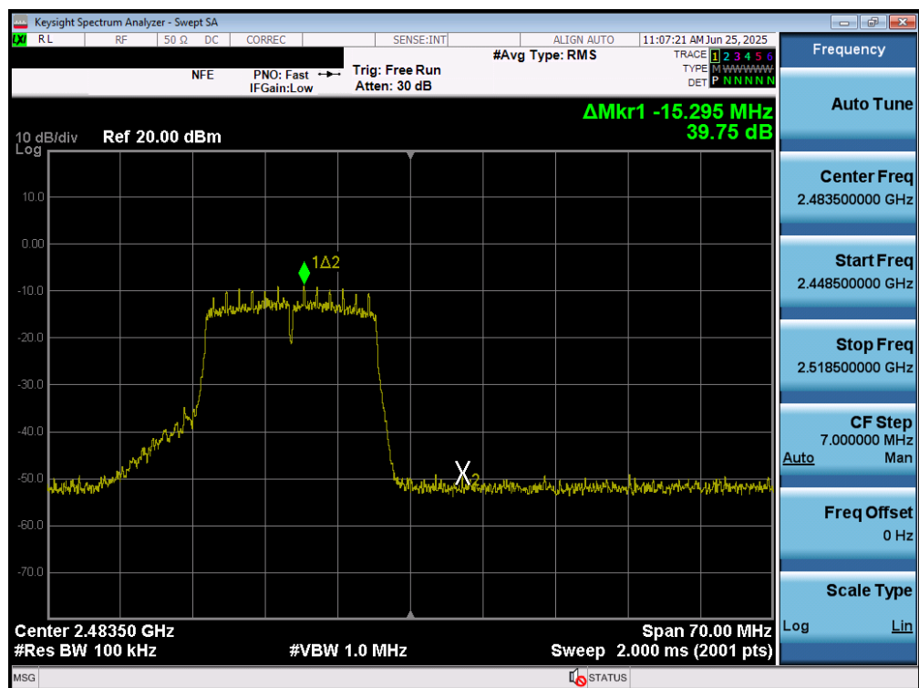
Plot 7-56. Band Edge Plot MIMO ANT1 (802.11g - Ch. 13)
