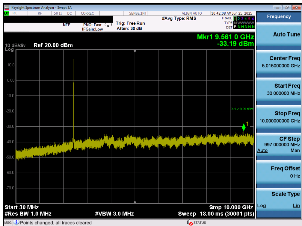
Plot 7-83. Conducted Spurious Plot MIMO ANT1 (802.11b – Ch. 6)
