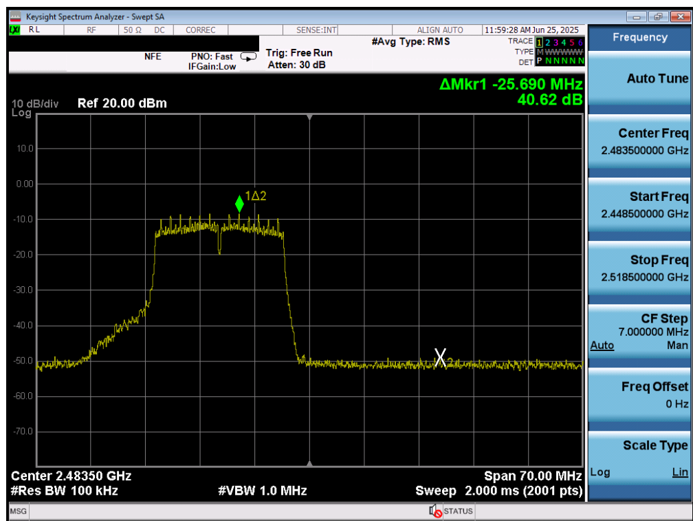
Plot 7-72. Band Edge Plot MIMO ANT2 (802.11g – Ch. 13)
