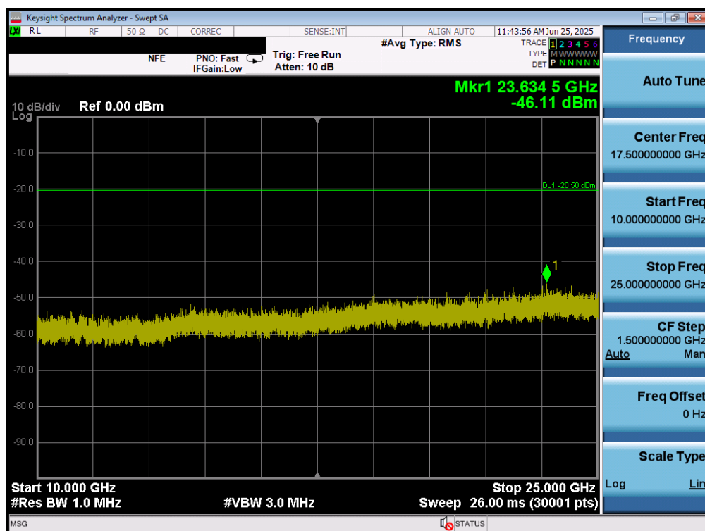
Plot 7-90. Conducted Spurious Plot MIMO ANT2 (802.11b – Ch. 6)
