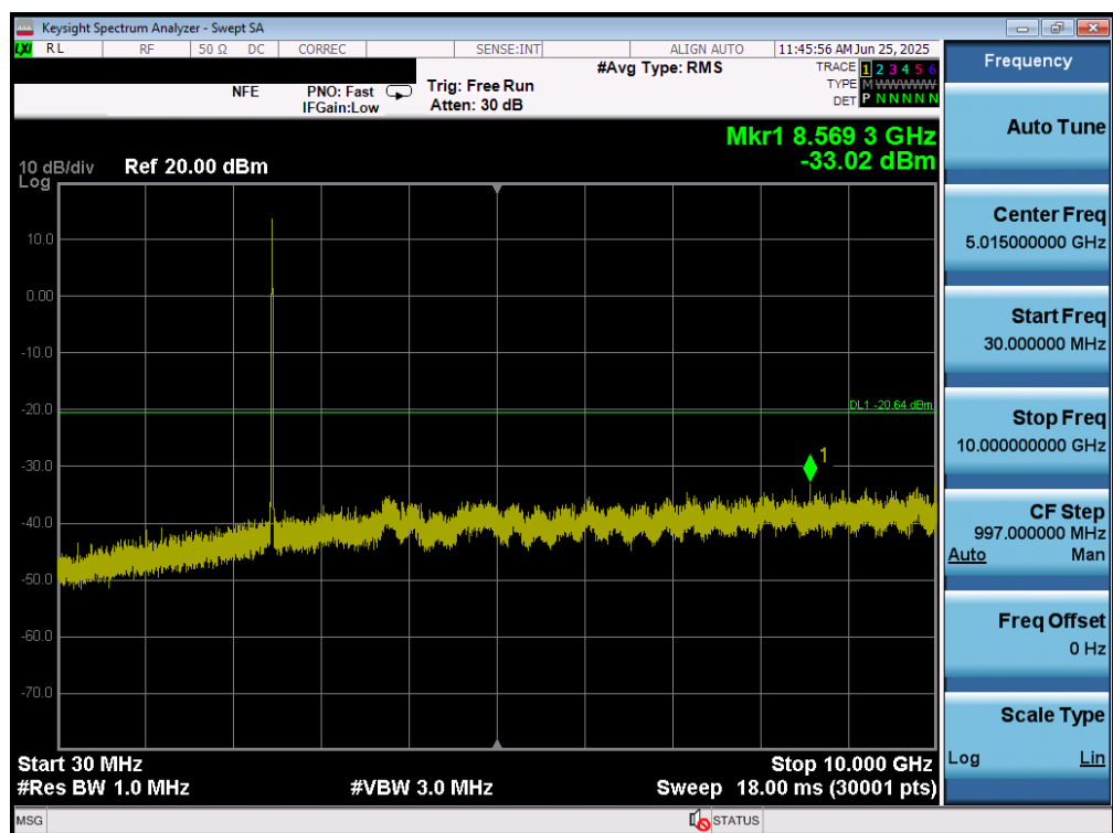
Plot 7-91. Conducted Spurious Plot MIMO ANT2 (802.11b – Ch. 11)
