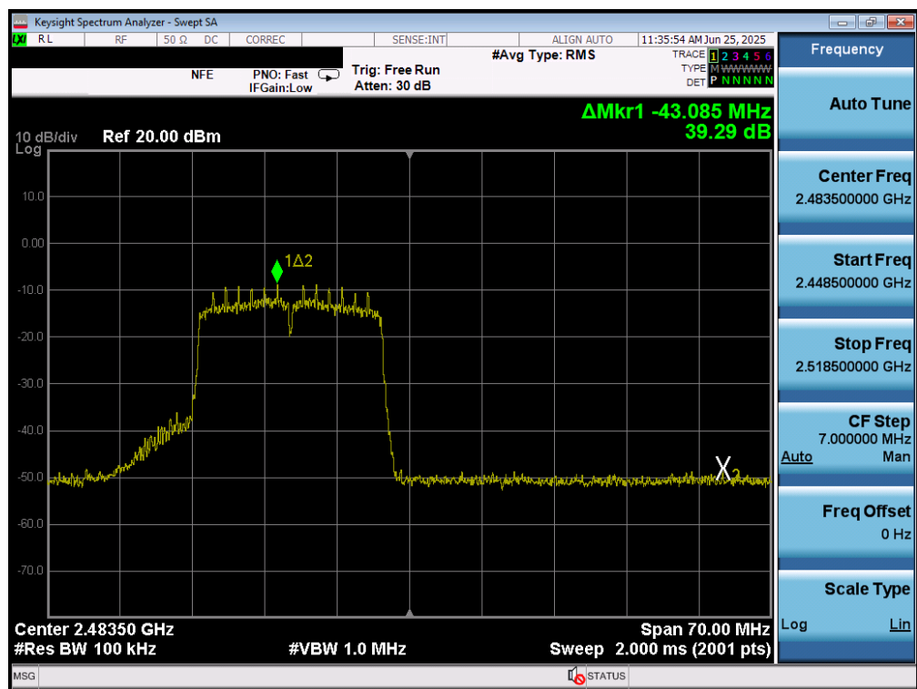
Plot 7-60. Band Edge Plot MIMO ANT1 (802.11n/ac (2.4GHz) – Ch. 13)
