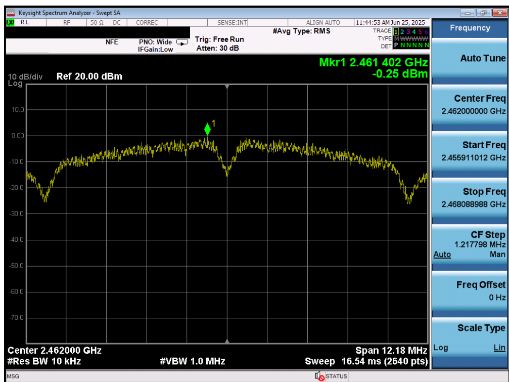
Plot 7-39. Power Spectral Density Plot MIMO ANT2 (802.11b – Ch. 11)
