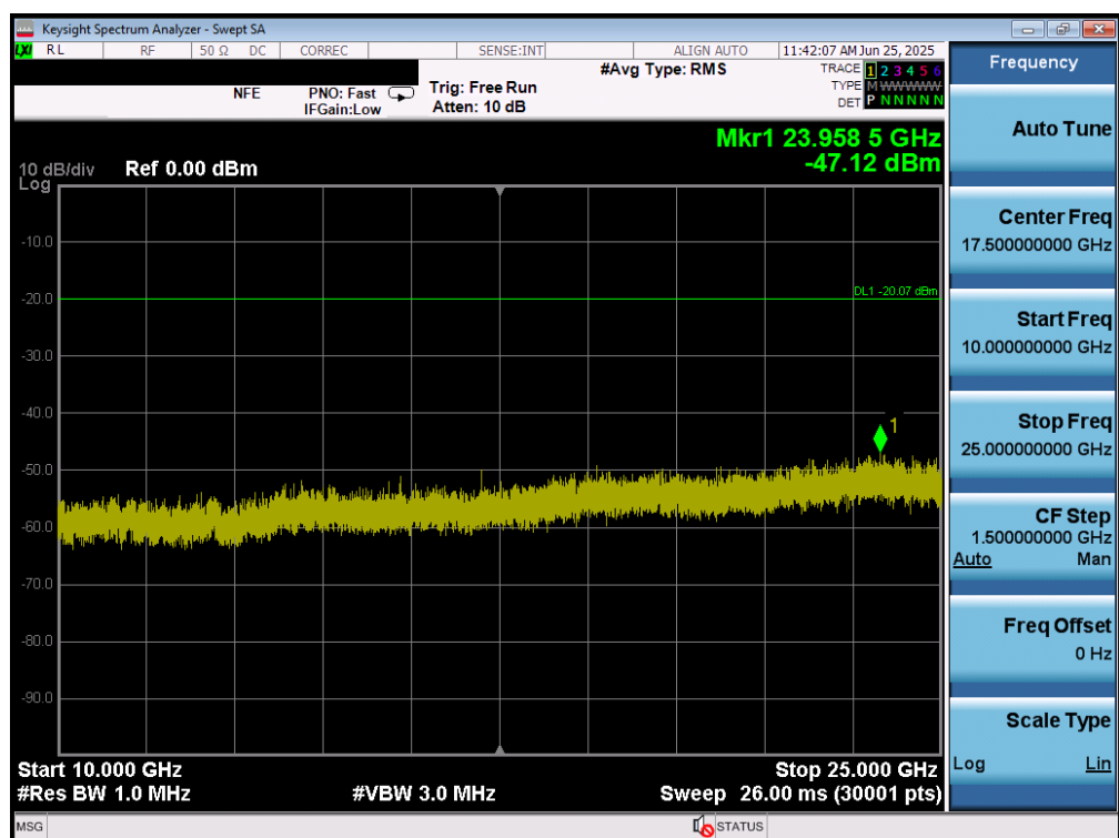
Plot 7-88. Conducted Spurious Plot MIMO ANT2 (802.11b – Ch. 1)
