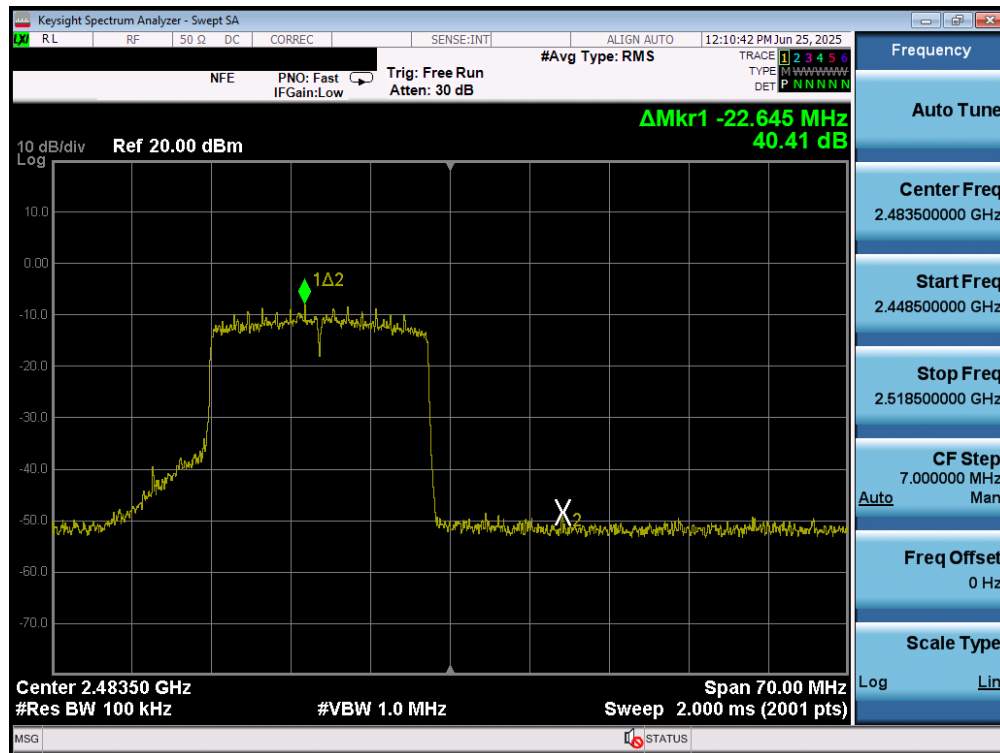
Plot 7-80. Band Edge Plot MIMO ANT2 (802.11ax/be (2.4GHz) – Ch. 13)
