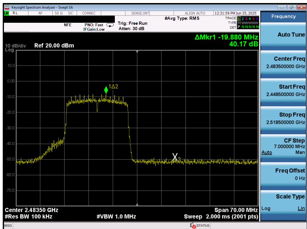
Plot 7-76. Band Edge Plot MIMO ANT2 (802.11n/ac (2.4GHz) – Ch. 13)
