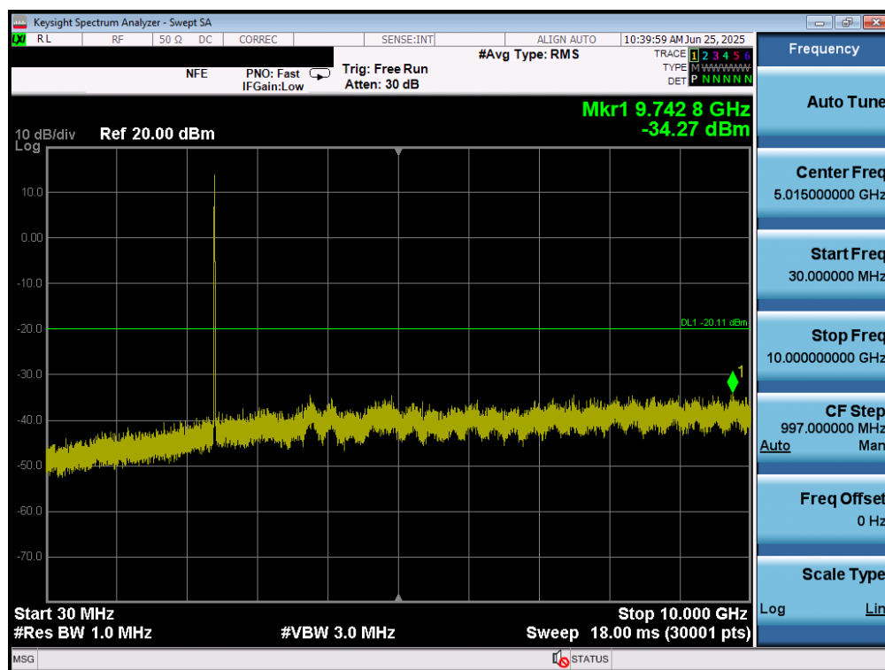
Plot 7-81. Conducted Spurious Plot MIMO ANT1 (802.11b – Ch. 1)
