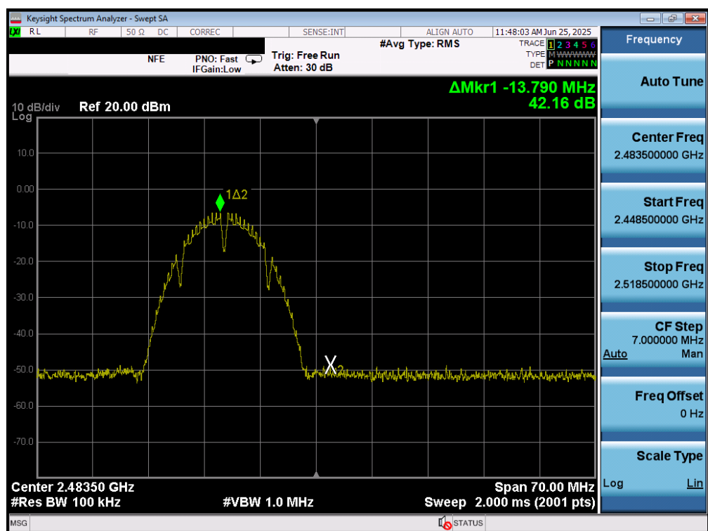
Plot 7-68. Band Edge Plot MIMO ANT2 (802.11b – Ch. 13)
