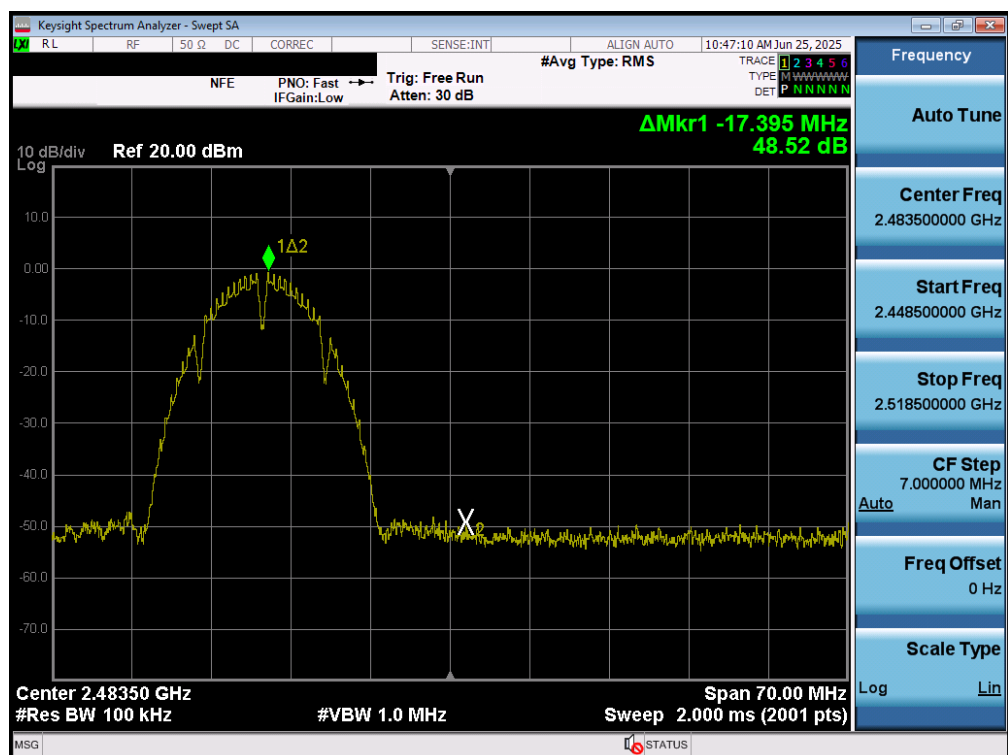
Plot 7-51. Band Edge Plot MIMO ANT1 (802.11b – Ch. 12)
