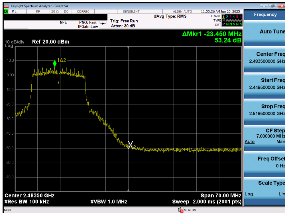
Plot 7-70. Band Edge Plot MIMO ANT2 (802.11g - Ch. 11)
