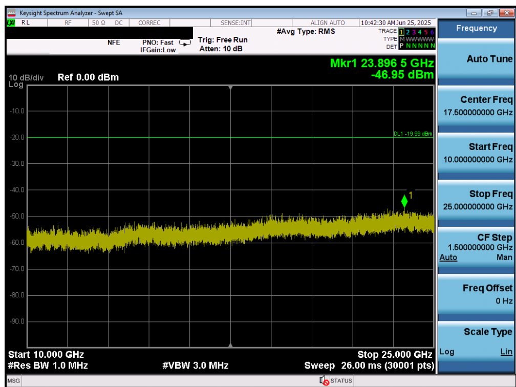
Plot 7-84. Conducted Spurious Plot MIMO ANT1 (802.11b – Ch. 6)
