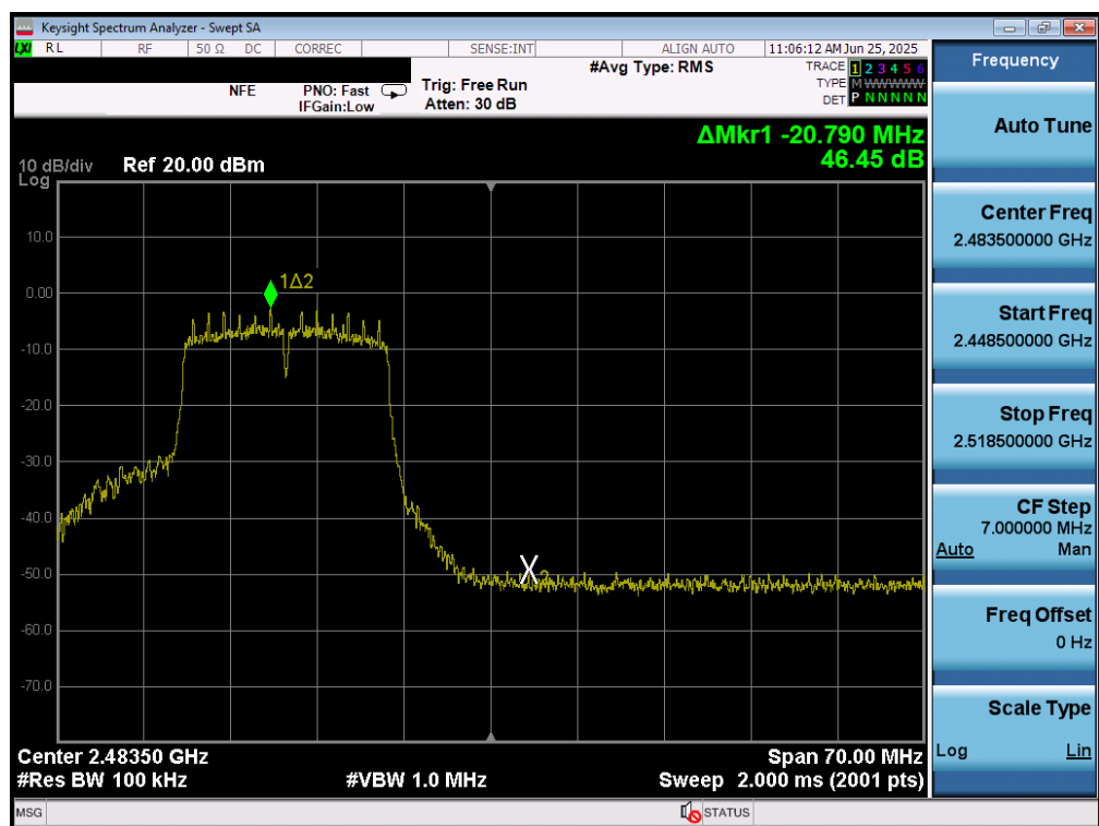
Plot 7-55. Band Edge Plot MIMO ANT1 (802.11g - Ch. 12)
