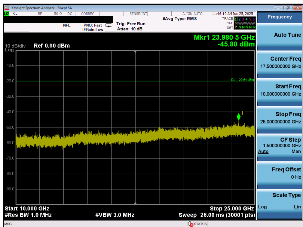
Plot 7-92. Conducted Spurious Plot MIMO ANT2 (802.11b – Ch. 11)
