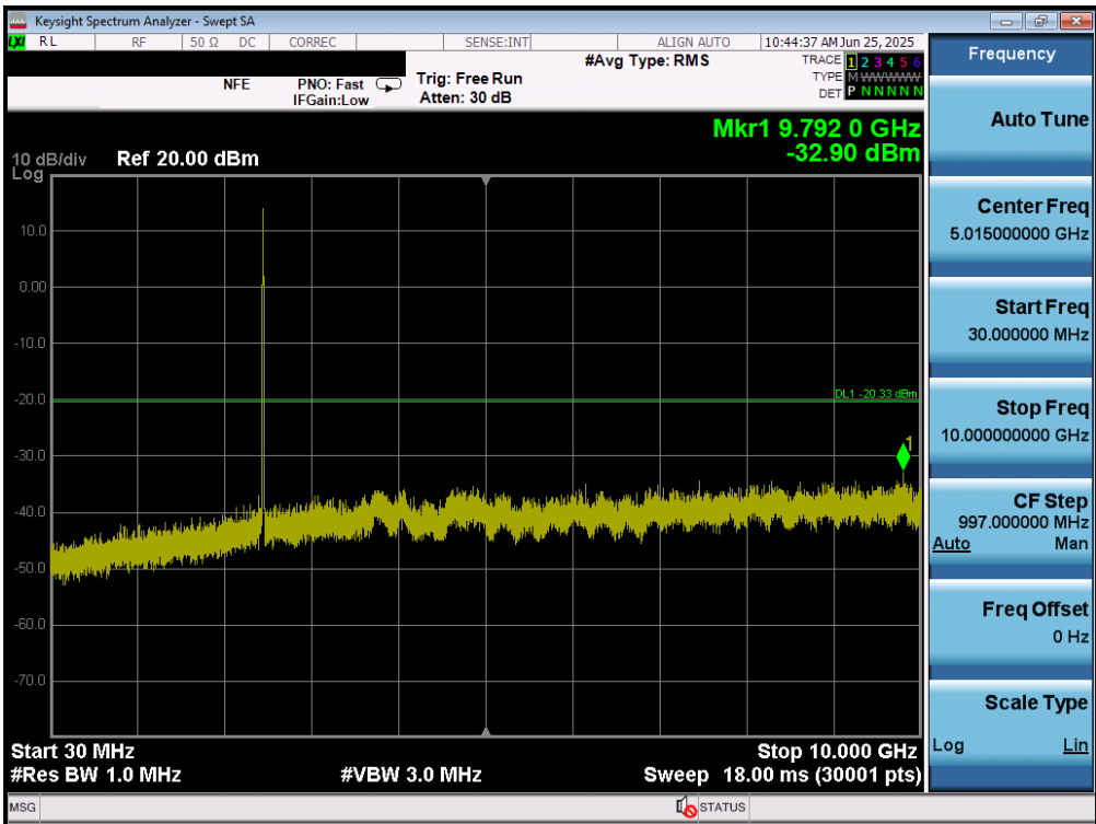
Plot 7-85. Conducted Spurious Plot MIMO ANT1 (802.11b – Ch. 11)
