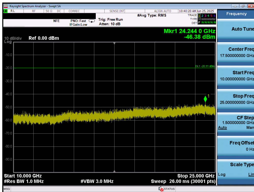
Plot 7-82. Conducted Spurious Plot MIMO ANT1 (802.11b – Ch. 1)
