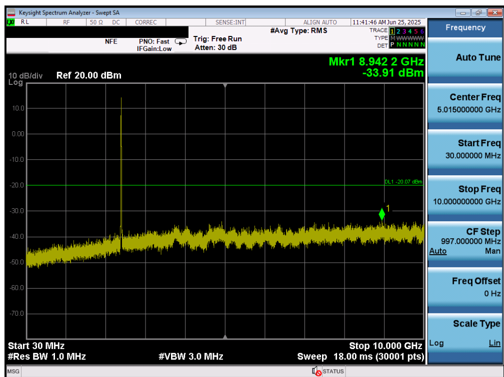
Plot 7-87. Conducted Spurious Plot MIMO ANT2 (802.11b – Ch. 1)
