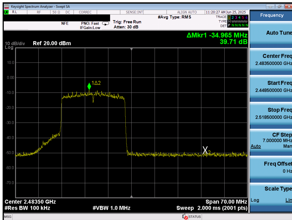
Plot 7-64. Band Edge Plot MIMO ANT1 (802.11ax/be (2.4GHz) – Ch. 13)
