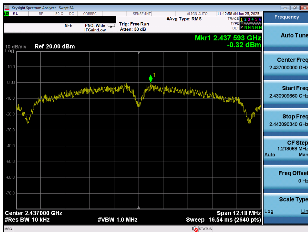
Plot 7-38. Power Spectral Density Plot MIMO ANT2 (802.11b – Ch. 6)
