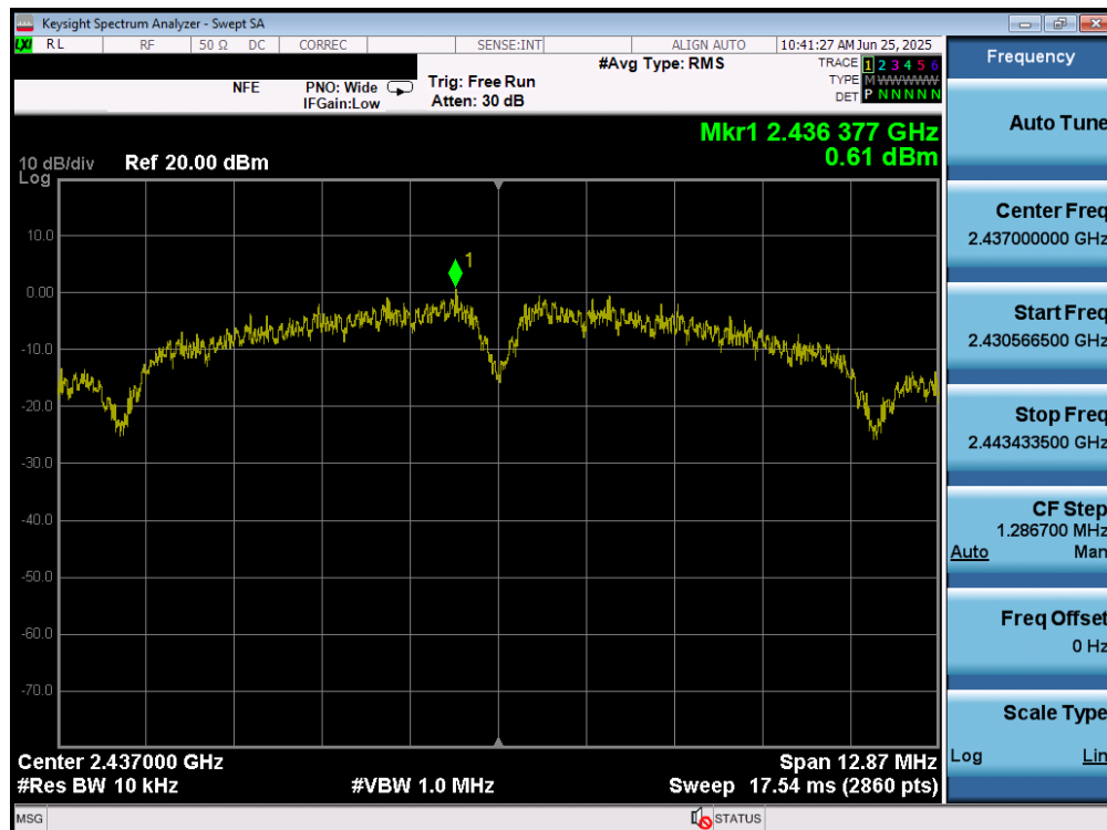
Plot 7-26. Power Spectral Density Plot MIMO ANT1 (802.11b – Ch. 6)
