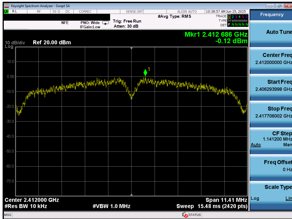
Plot 7-25. Power Spectral Density Plot MIMO ANT1 (802.11b – Ch. 1)
