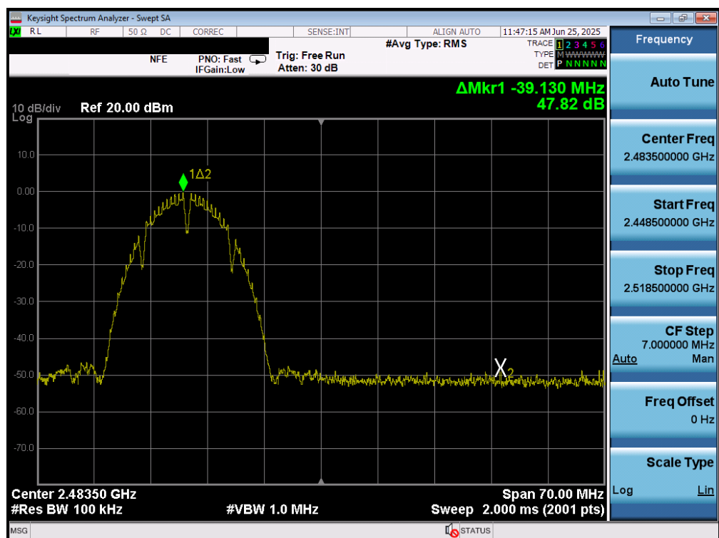
Plot 7-67. Band Edge Plot MIMO ANT2 (802.11b – Ch. 12)
