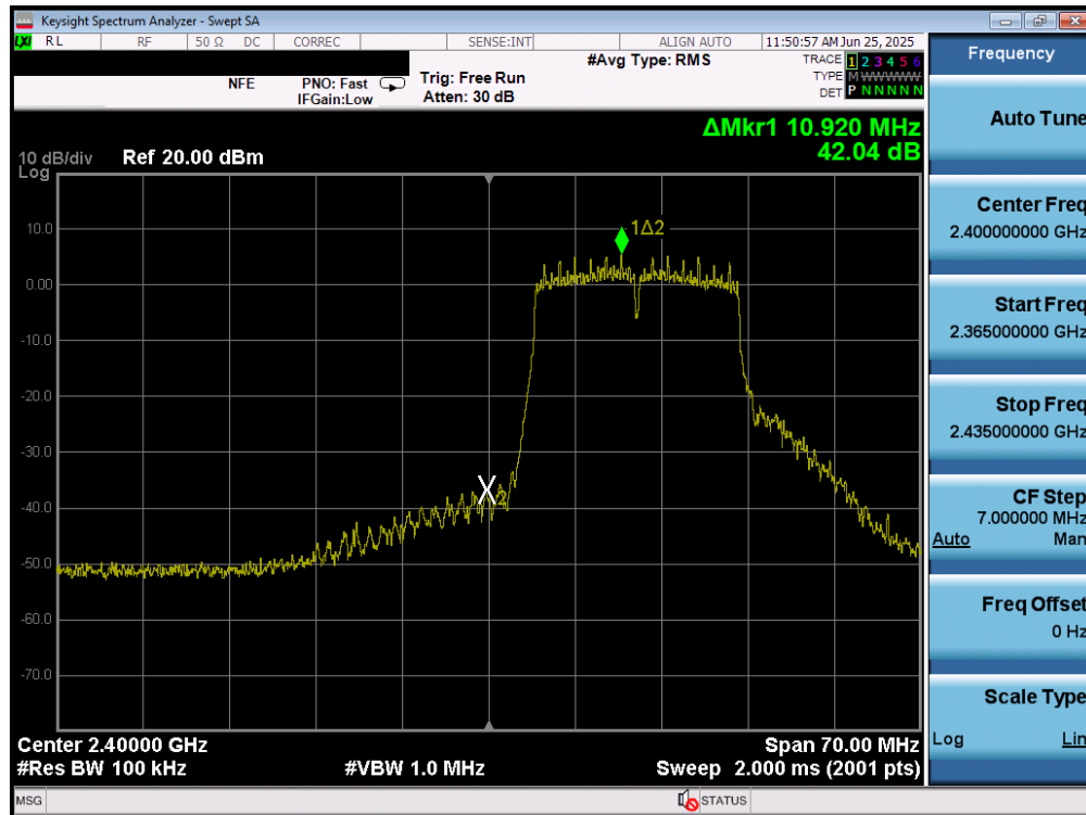
Plot 7-69. Band Edge Plot MIMO ANT2 (802.11g- Ch. 1)
