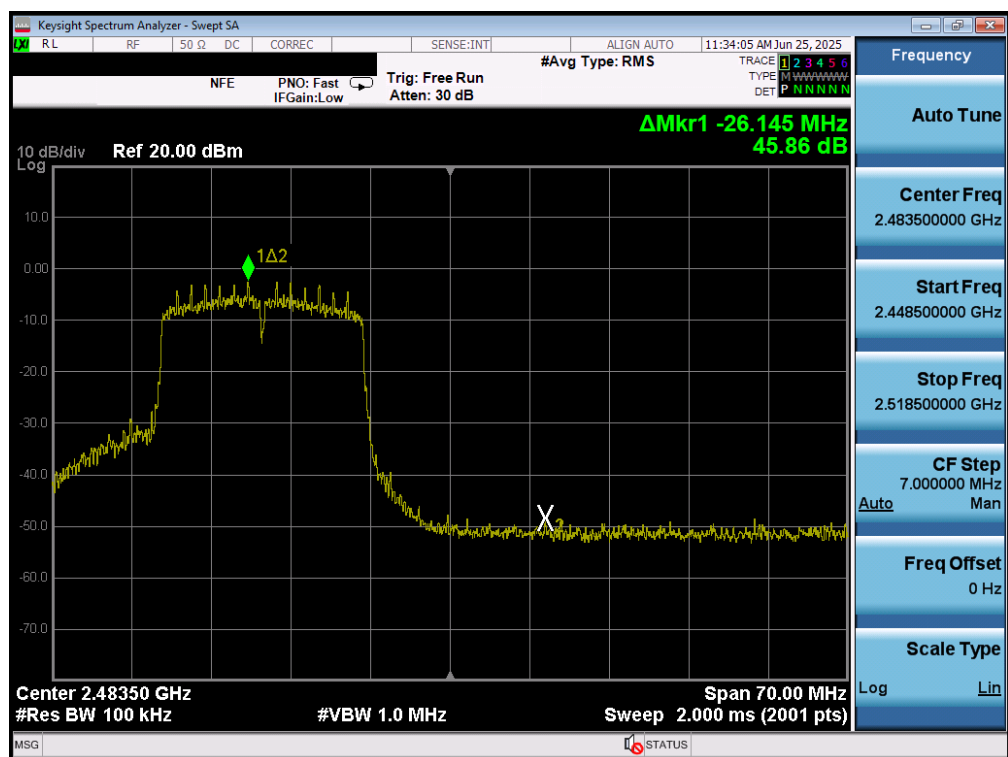
Plot 7-59. Band Edge Plot MIMO ANT1 (802.11n/ac (2.4GHz) – Ch. 12)
