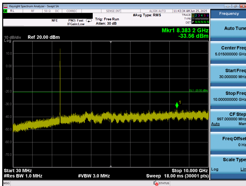
Plot 7-89. Conducted Spurious Plot MIMO ANT2 (802.11b – Ch. 6)
