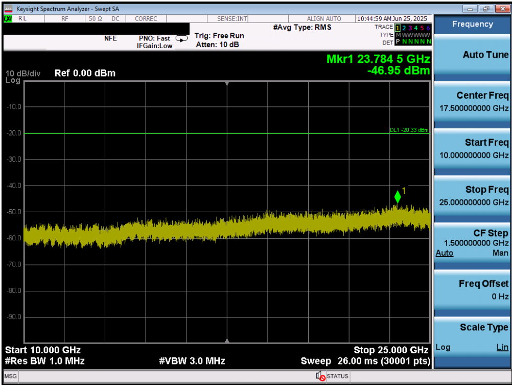
Plot 7-86. Conducted Spurious Plot MIMO ANT1 (802.11b – Ch. 11)
