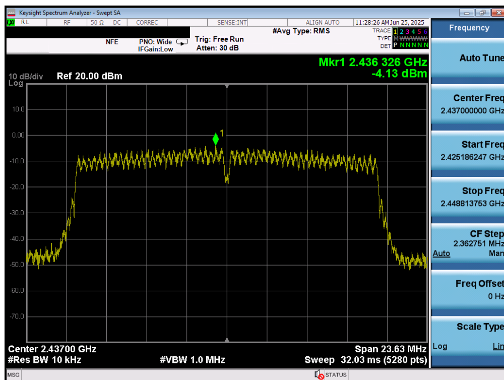
Plot 7-32. Power Spectral Density Plot MIMO ANT1 (802.11n/ac (2.4GHz) – Ch. 6)
