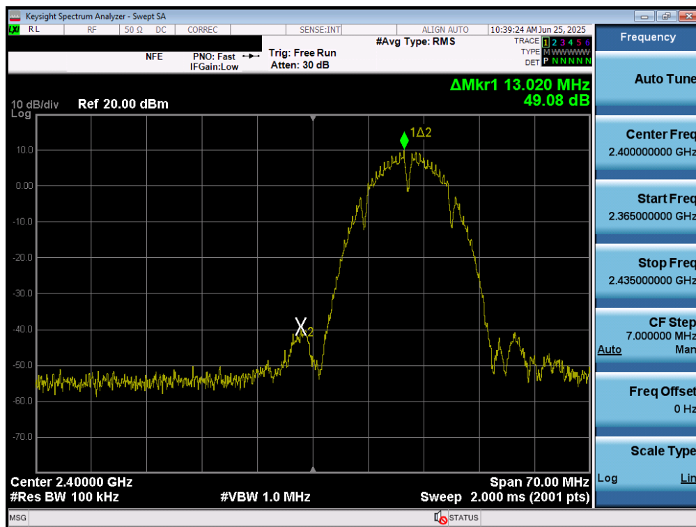
Plot 7-49. Band Edge Plot MIMO ANT1 (802.11b – Ch. 1)
