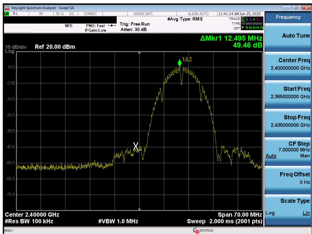
Plot 7-65. Band Edge Plot MIMO ANT2 (802.11b – Ch. 1)
