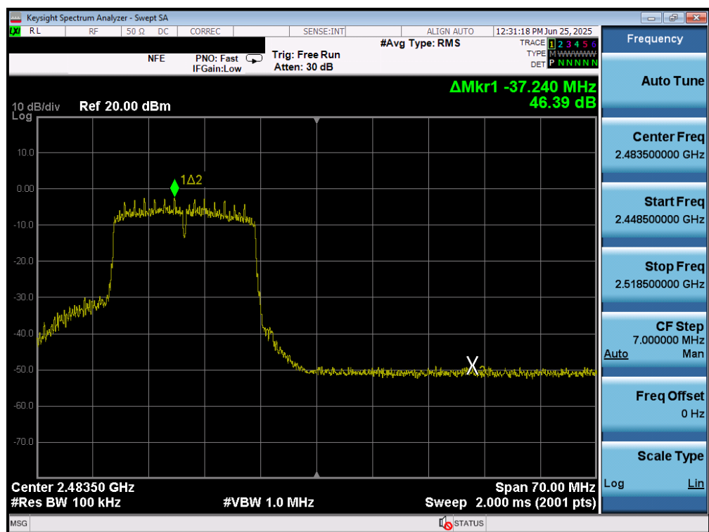
Plot 7-75. Band Edge Plot MIMO ANT2 (802.11n/ac (2.4GHz) – Ch. 12)
