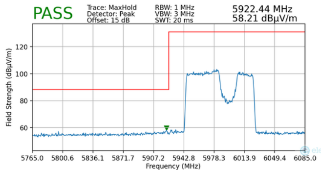
Plot 7-78. Radiated Lower Band Edge Plot MIMO (Peak – UNII Band 5)
