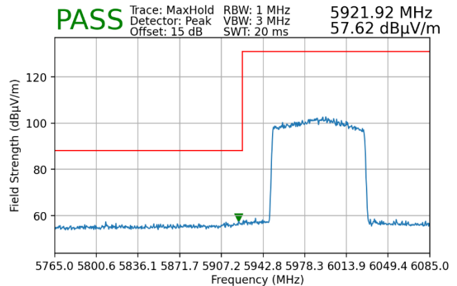
Plot 7-74. Radiated Lower Band Edge Plot MIMO (Peak – UNII Band 5)
