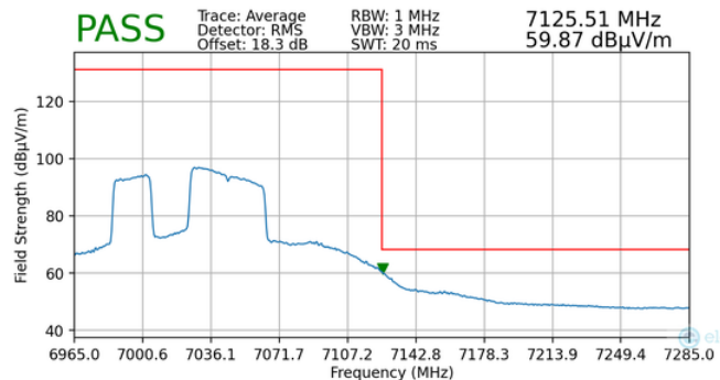
Plot 7-79. Radiated Upper Band Edge Plot MIMO (Average – UNII Band 8)
