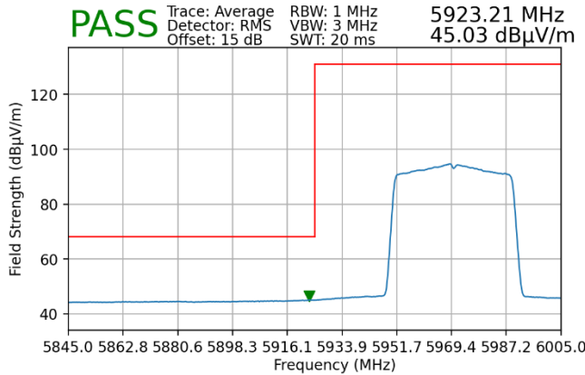
Plot 7-69. Radiated Lower Band Edge Plot MIMO (Average – UNII Band 5)
