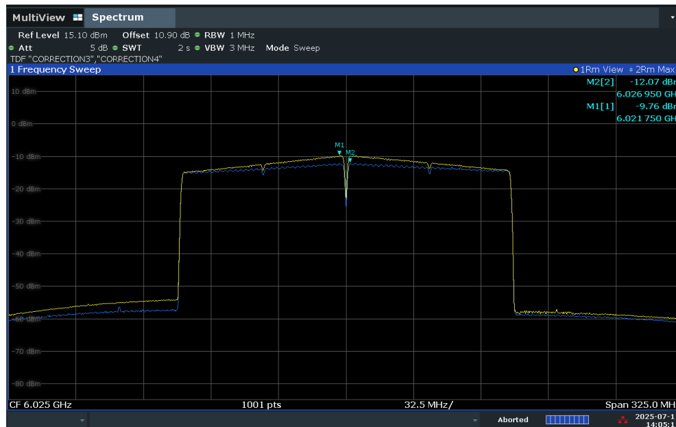
Plot 7-56. Power Spectral Density Plot – ANT2 (160MHz Bandwidth, RSSI level at -49dBm (yellow) and -31dBm (blue))
