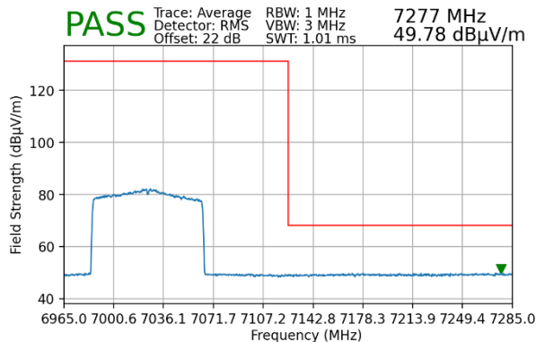
Plot 7-75. Radiated Upper Band Edge Plot MIMO (Average – UNII Band 8)
