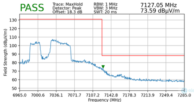
Plot 7-80. Radiated Upper Band Edge Plot MIMO (Peak – UNII Band 8)
