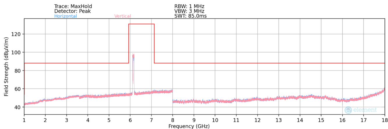
Plot 7-64. Radiated Spurious Plot 1GHz – 18GHz MIMO (802.11be – UNII Band 5 Ch. 39) - Punctured
