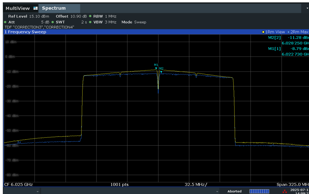
Plot 7-55. Power Spectral Density Plot – ANT1 (160MHz Bandwidth, RSSI level at -49dBm (yellow) and -31dBm (blue))
