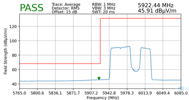
Plot 7-77. Radiated Lower Band Edge Plot MIMO (Average – UNII Band 5)
