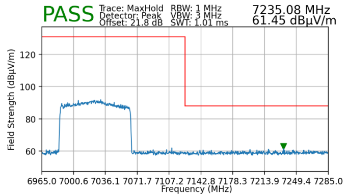
Plot 7-76. Radiated Upper Band Edge Plot MIMO (Peak – UNII Band 8)
