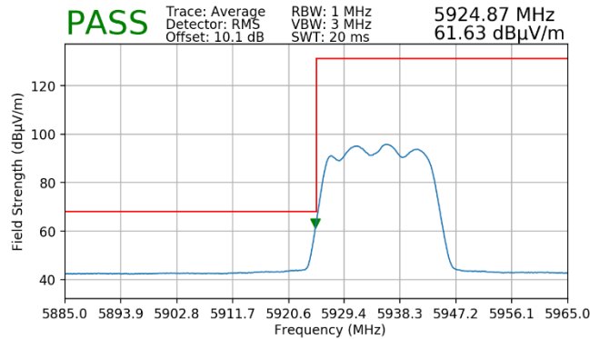
Plot 7-65. Radiated Lower Band Edge Plot MIMO (Average – UNII Band 5)
