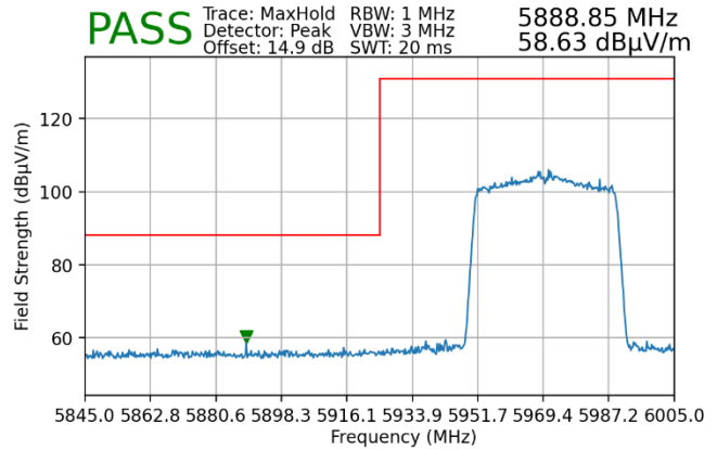
Plot 7-70. Radiated Lower Band Edge Plot MIMO (Peak – UNII Band 5)
