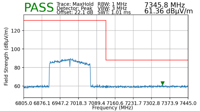
Plot 7-84. Radiated Upper Band Edge Plot MIMO (Peak – UNII Band 8)
