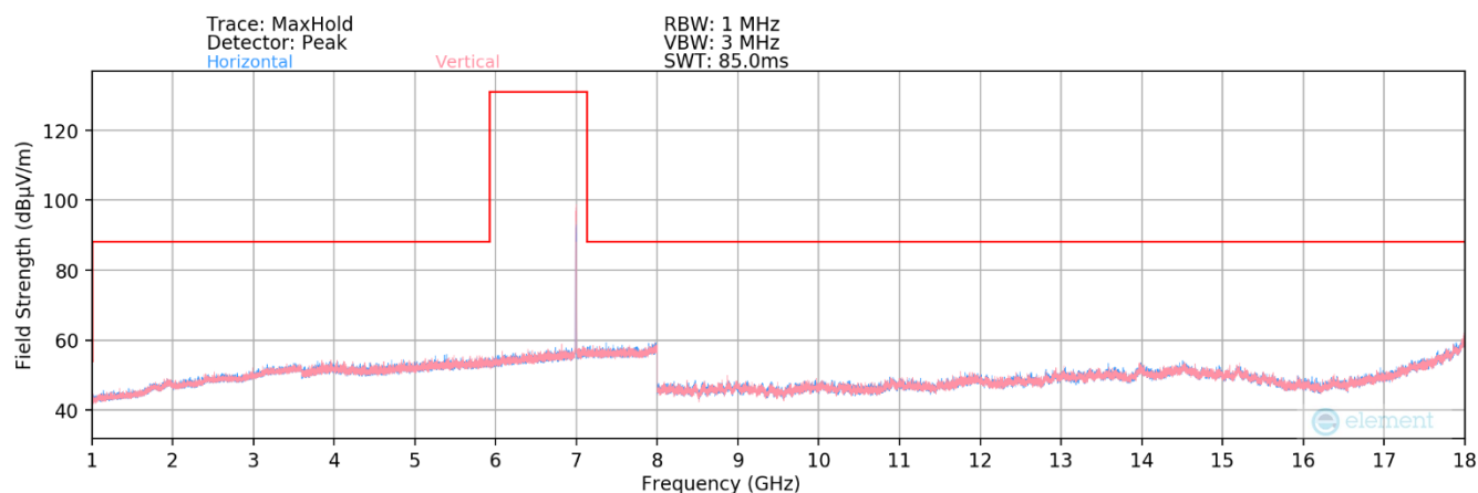
Plot 7-61. Radiated Spurious Plot 1GHz – 18GHz MIMO (802.11a – U Band 8 Ch. 209)
