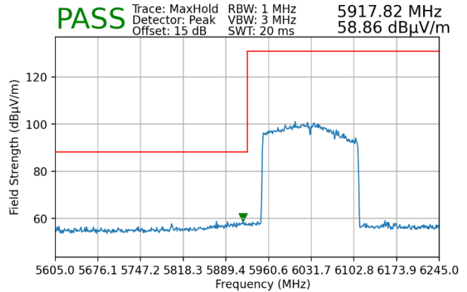
Plot 7-82. Radiated Lower Band Edge Plot MIMO (Peak – UNII Band 5)
