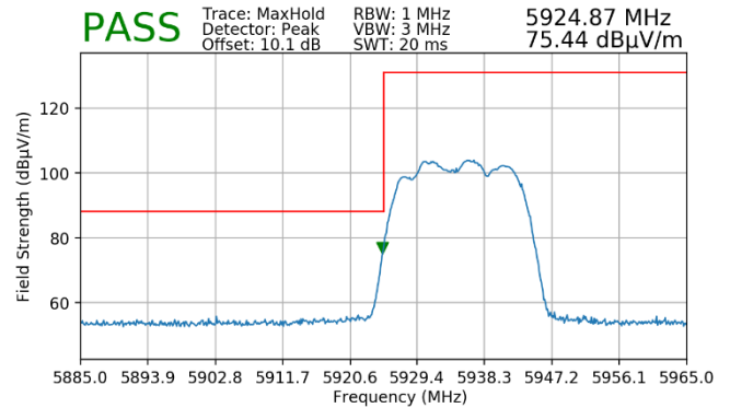
Plot 7-66. Radiated Lower Band Edge Plot MIMO (Peak – UNII Band 5)
