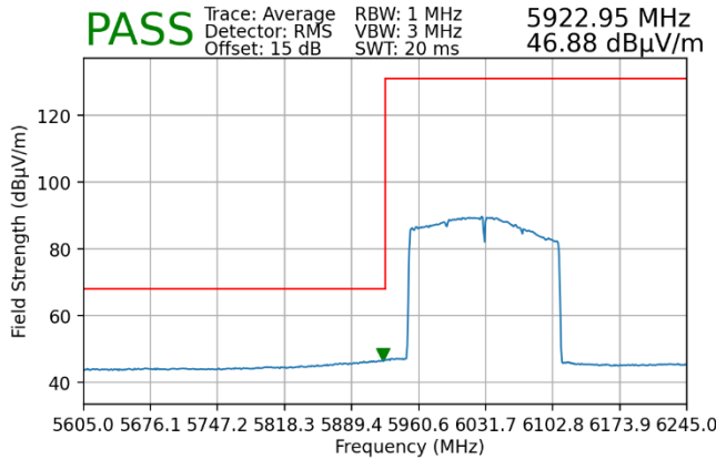
Plot 7-81. Radiated Lower Band Edge Plot MIMO (Average – UNII Band 5)
