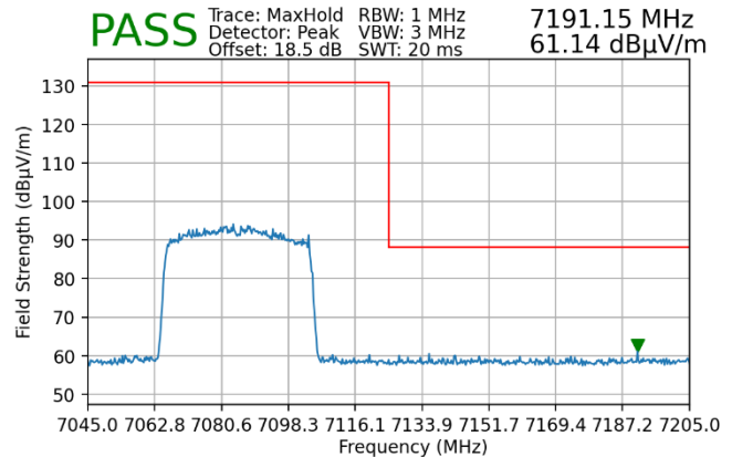
Plot 7-72. Radiated Upper Band Edge Plot MIMO (Peak – UNII Band 8)
