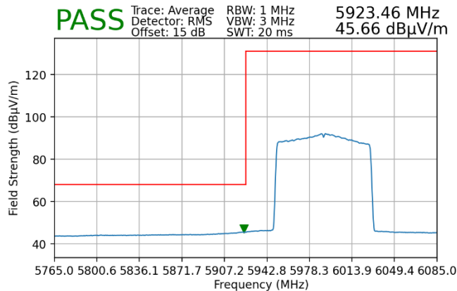
Plot 7-73. Radiated Lower Band Edge Plot MIMO (Average – UNII Band 5)
