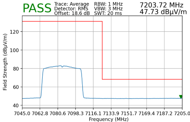
Plot 7-71. Radiated Upper Band Edge Plot MIMO (Average – UNII Band 8)
