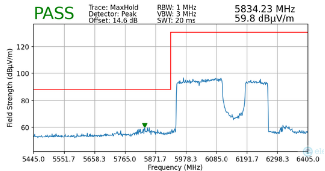
Plot 7-94. Radiated Lower Band Edge Plot MIMO (Peak – UNII Band 5)
