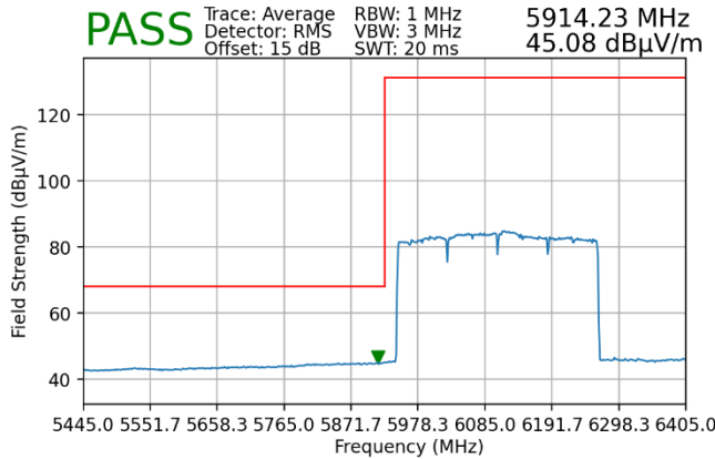
Plot 7-89. Radiated Lower Band Edge Plot MIMO (Average – UNII Band 5)
