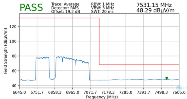
Plot 7-95. Radiated Upper Band Edge Plot MIMO (Average – UNII Band 8)
