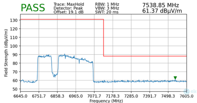
Plot 7-96. Radiated Upper Band Edge Plot MIMO (Peak – UNII Band 8)
