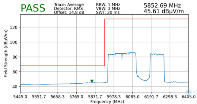
Plot 7-93. Radiated Lower Band Edge Plot MIMO (Average – UNII Band 5)
