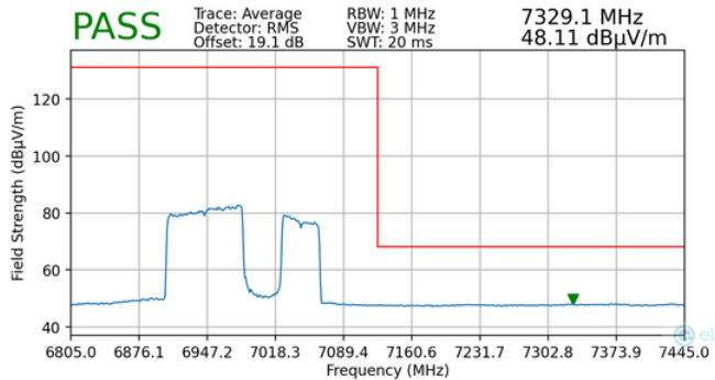
Plot 7-87. Radiated Upper Band Edge Plot MIMO (Average – UNII Band 8)
