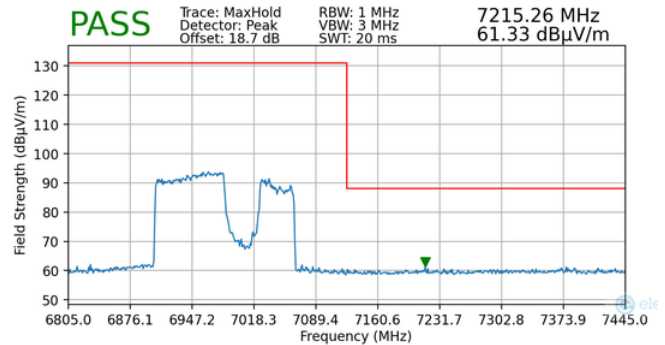
Plot 7-88. Radiated Upper Band Edge Plot MIMO (Peak – UNII Band 8)
