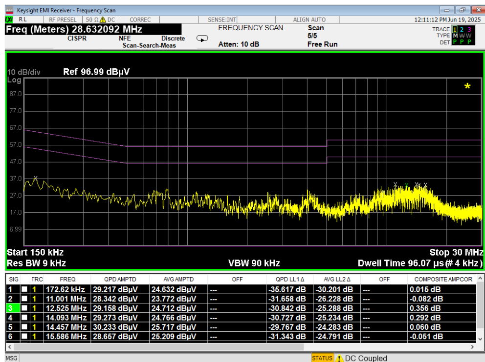
Plot 7-99. Line Conducted Plot with 802.11a UNII Band 6 (L1)
