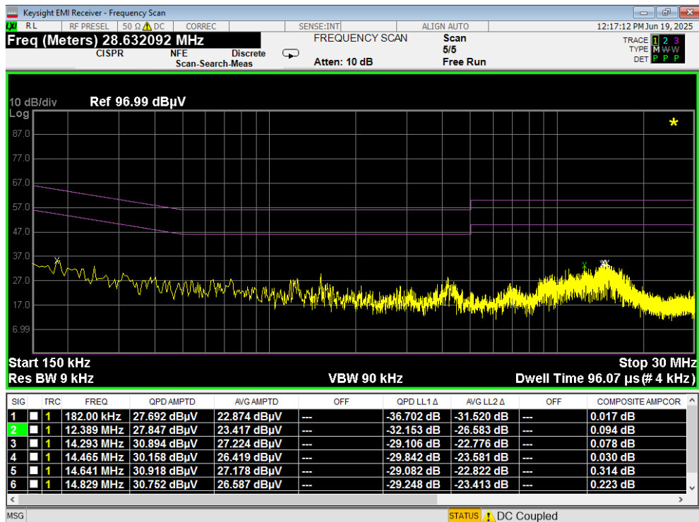
Plot 7-104. Line Conducted Plot with 802.11a UNII Band 8 (N)
