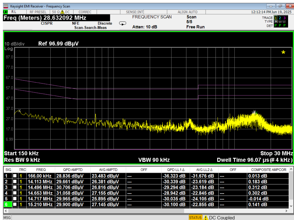
Plot 7-100. Line Conducted Plot with 802.11a UNII Band 6 (N)
