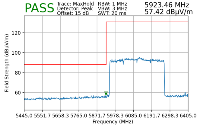
Plot 7-90. Radiated Lower Band Edge Plot MIMO (Peak – UNII Band 5)
