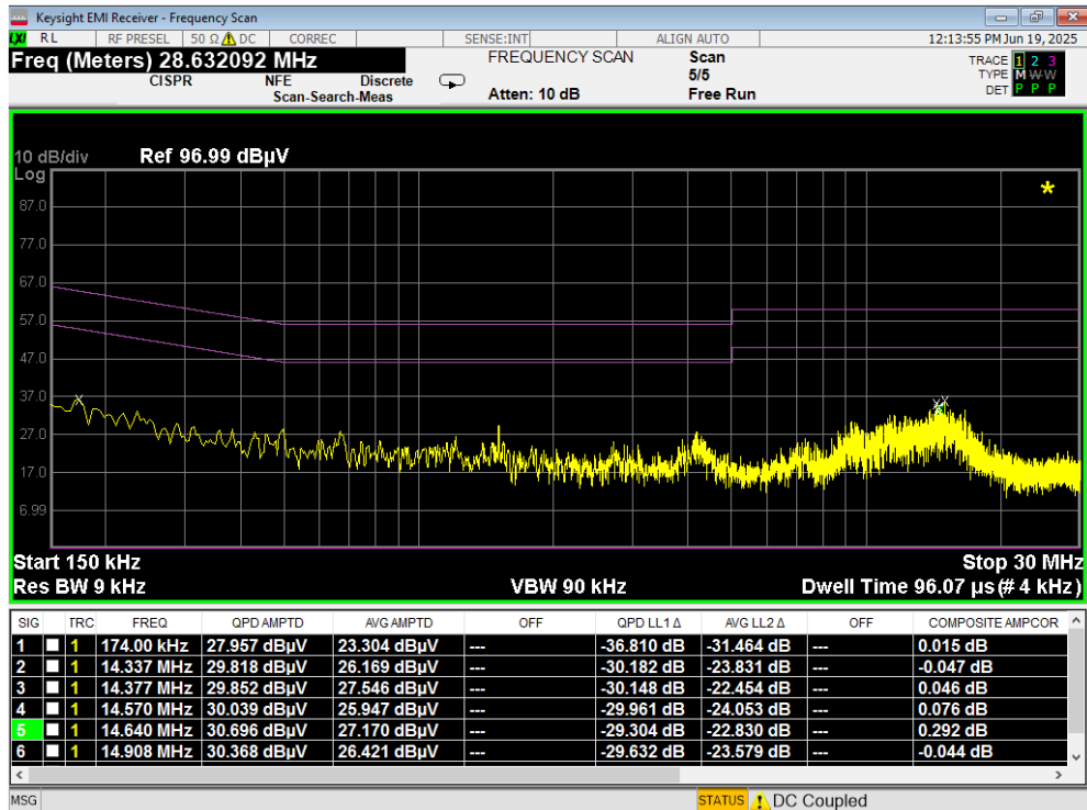
Plot 7-102. Line Conducted Plot with 802.11a UNII Band 7 (N)
