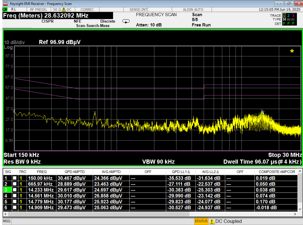
Plot 7-101. Line Conducted Plot with 802.11a UNII Band 7 (L1)
