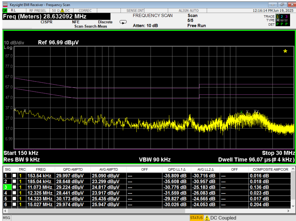
Plot 7-103. Line Conducted Plot with 802.11a UNII Band 8 (L1)
