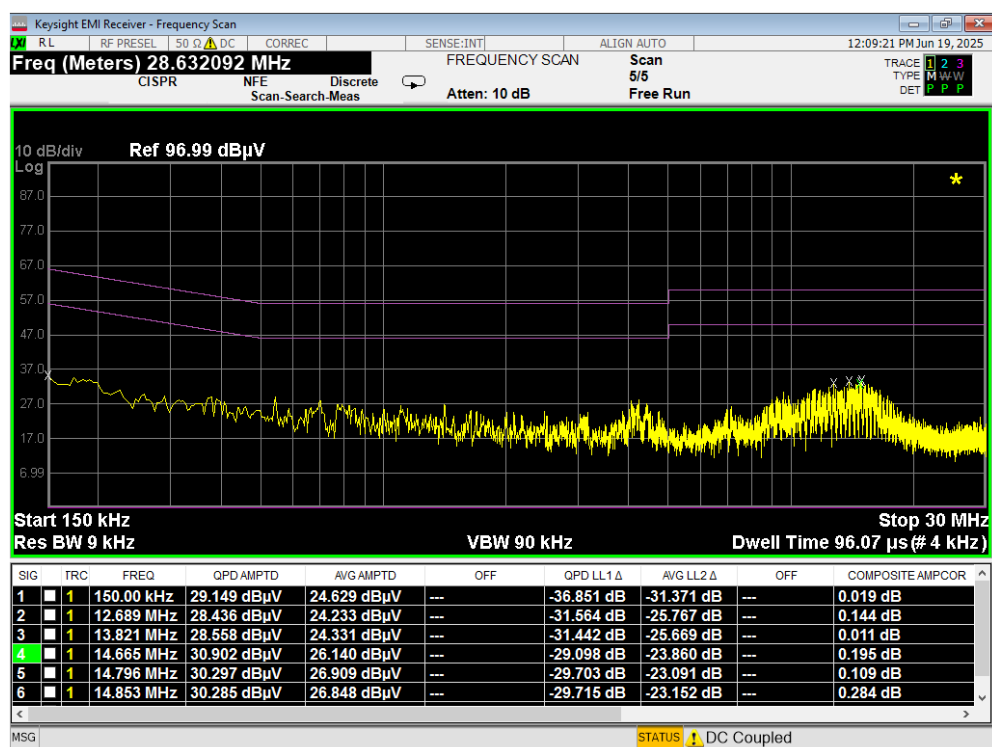
Plot 7-98. Line Conducted Plot with 802.11a UNII Band 5 (N)
