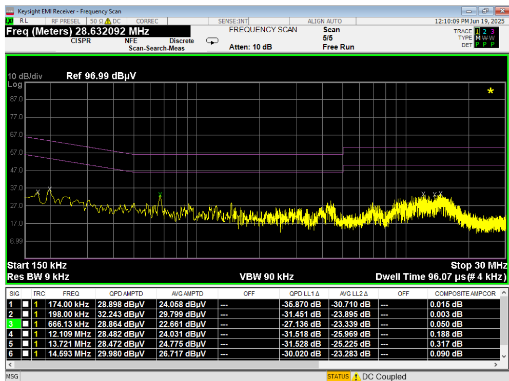
Plot 7-97. Line Conducted Plot with 802.11a UNII Band 5 (L1)
