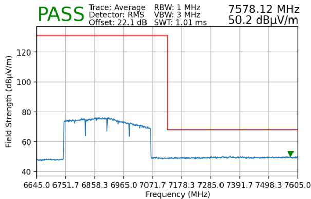
Plot 7-91. Radiated Upper Band Edge Plot MIMO (Average – UNII Band 8)
