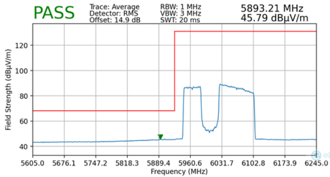
Plot 7-87. Radiated Lower Band Edge Plot MIMO (Average – UNII Band 5)
