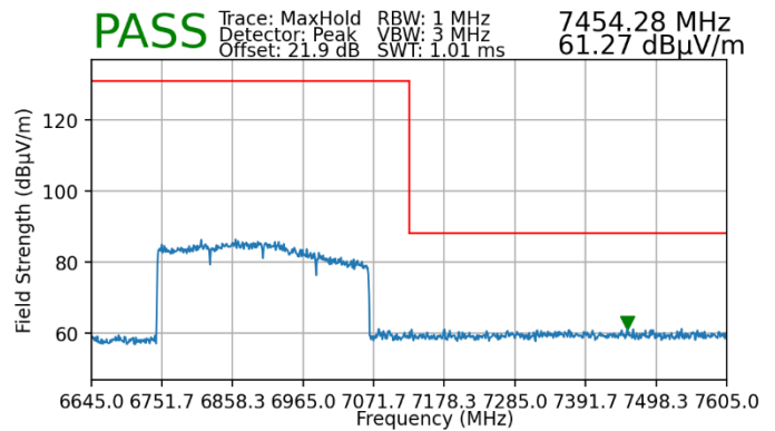
Plot 7-94. Radiated Upper Band Edge Plot MIMO (Peak – UNII Band 8)
