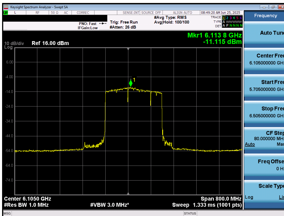
Plot 7-37. Power Spectral Density Plot MIMO ANT1 (320MHz 802.11be (UNII Band 5) – Ch. 31) LPI/SP
