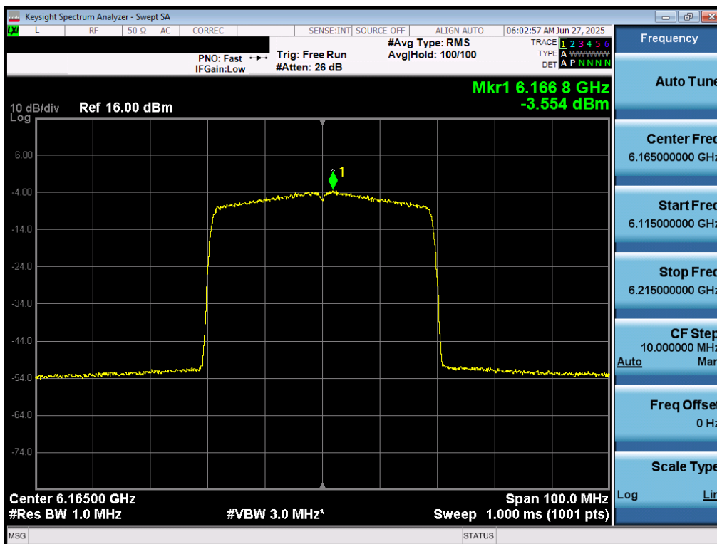
Plot 7-44. Power Spectral Density Plot MIMO ANT1 (40MHz 802.11ax/be (Full Tones) (UNII Band 5) – Ch. 43) – LPI/SP
