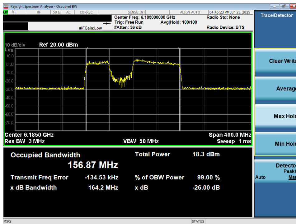
Plot 7-22. 26dB Bandwidth Plot MIMO ANT2 (160MHz 802.11be (996+484 Tones) (UNII Band 5) – Ch. 47) LPI/SP
