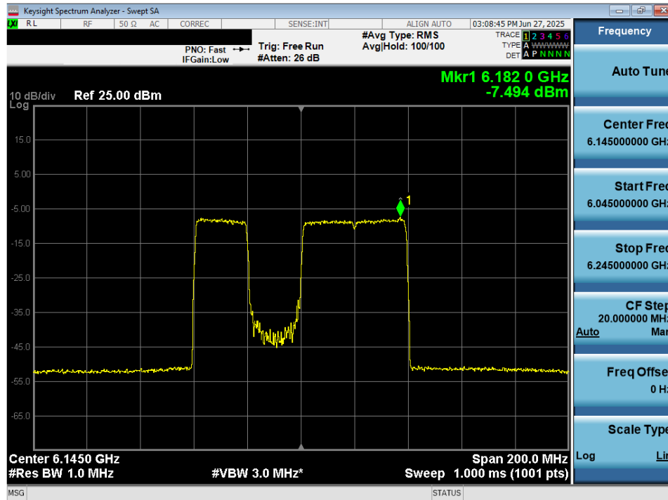
Plot 7-51. Power Spectral Density Plot MIMO ANT2 (80MHz 802.11be (484+242 Tones) (UNII Band 5) – Ch. 39) LPI/SP
