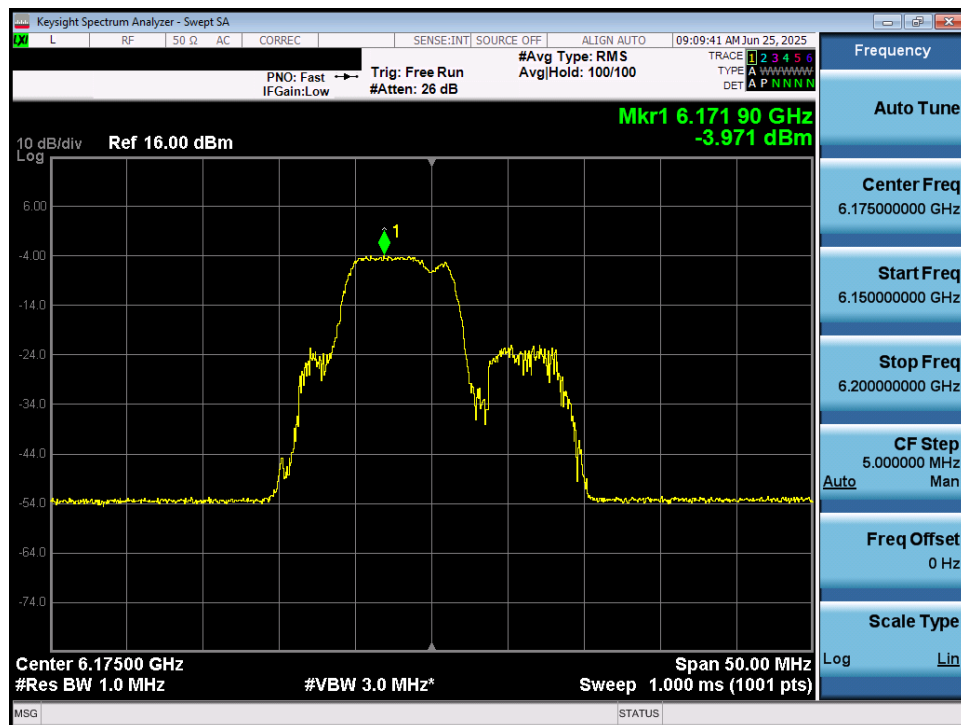
Plot 7-34. Power Spectral Density Plot MIMO ANT1 (20MHz 802.11be (52+26 Tones) (UNII Band 5) – Ch. 45) – LPI/SP
