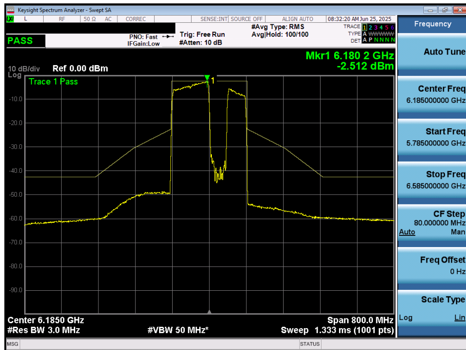
Plot 7-66. In Band Emissions Plot MIMO ANT1 (160MHz 802.11be (996+484 Tones) (UNII Band 5) – Ch. 47) LPI/SP
