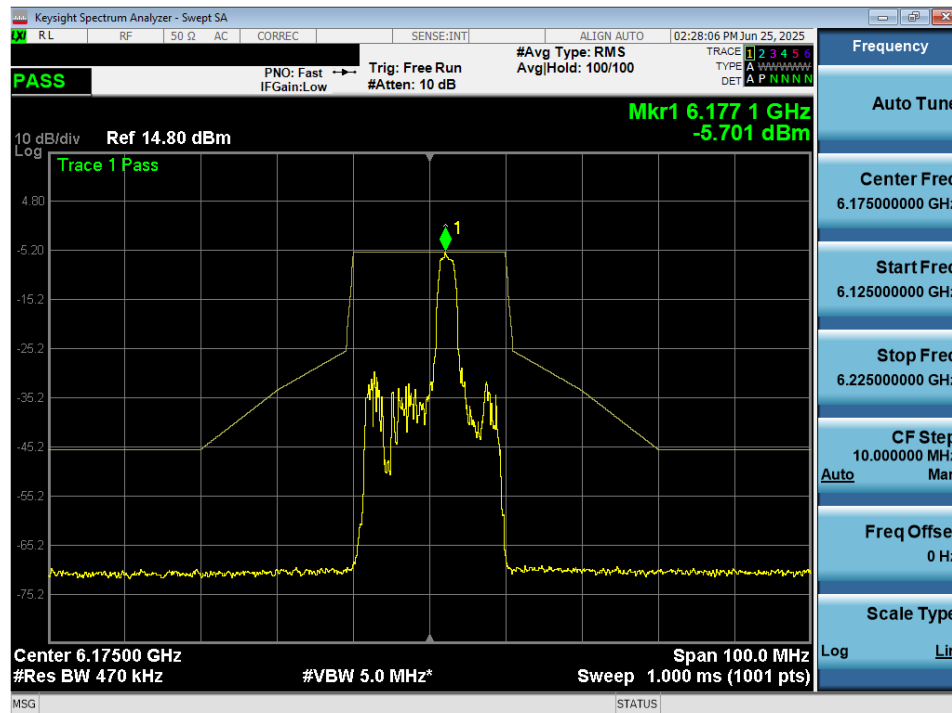
Plot 7-73. In Band Emissions Plot MIMO ANT2 (20MHz 802.11ax/be (26 Tones) (UNII Band 5) – Ch. 45) – LPI/SP
