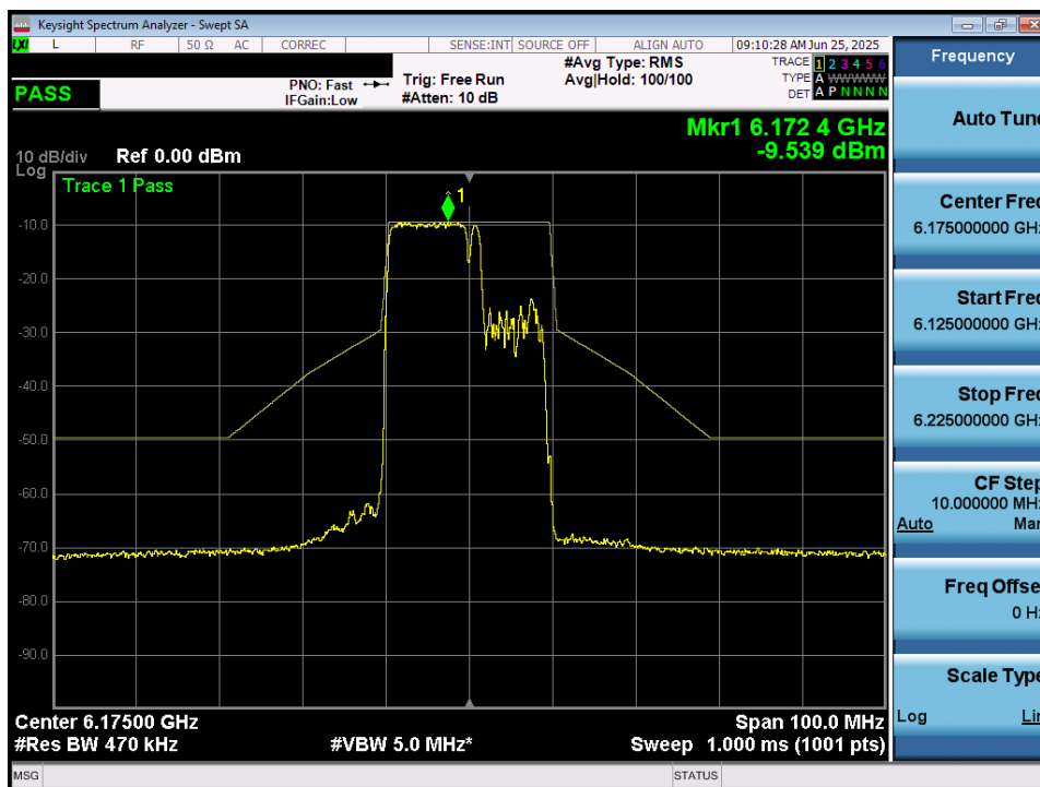
Plot 7-64. In Band Emissions Plot MIMO ANT1 (20MHz 802.11be (106+26 Tones) (UNII Band 5) – Ch. 45) – LPI/SP
