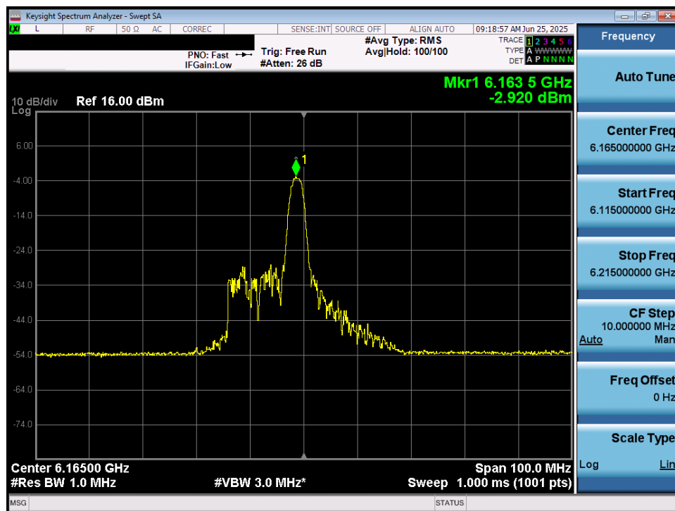
Plot 7-30. Power Spectral Density Plot MIMO ANT1 (40MHz 802.11ax/be (26 Tones) (UNII Band 5) – Ch. 43) – LPI/SP
