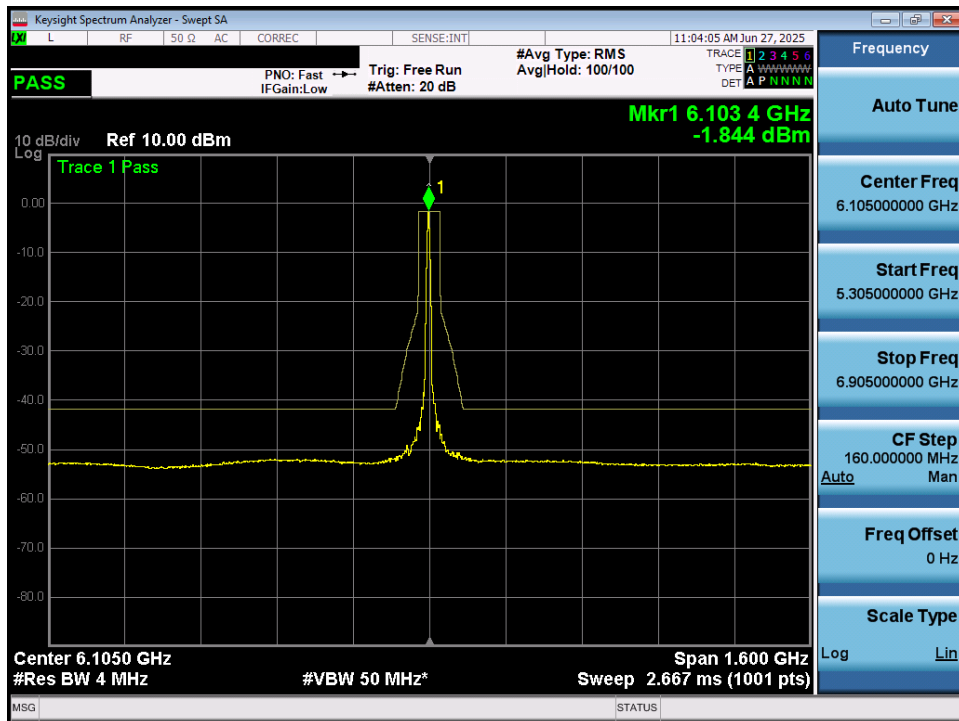
Plot 7-77. In Band Emissions Plot MIMO ANT2 (320MHz 802.11ax/be (26 Tones) (UNII Band 5) – Ch. 31) – LPI/SP
