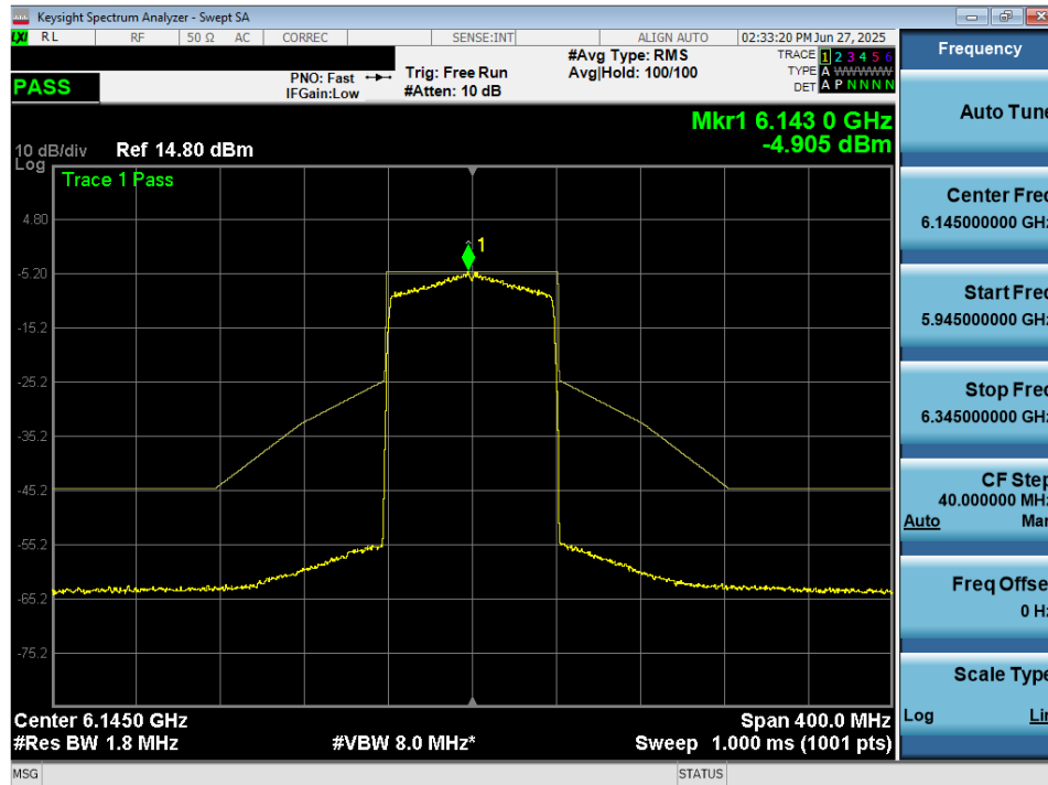
Plot 7-84. In Band Emissions Plot MIMO ANT2 (80MHz 802.11ax/be (Full Tones) (UNII Band 5) – Ch. 39) - LPI/SP
