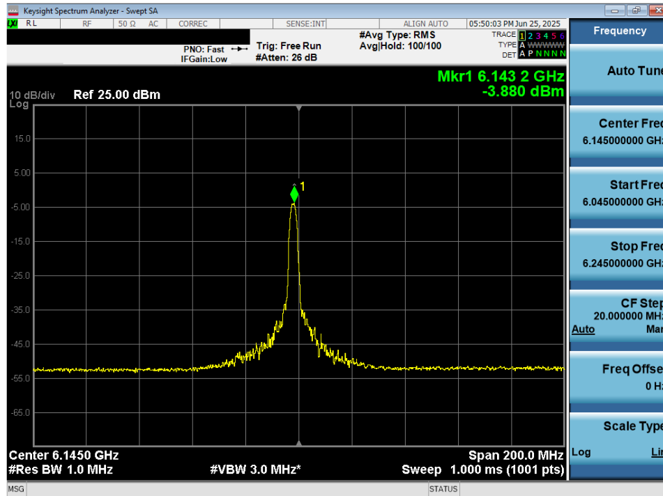
Plot 7-47. Power Spectral Density Plot MIMO ANT2 (80MHz 802.11ax/be (26 Tones) (UNII Band 5) – Ch. 39) – LPI/SP
