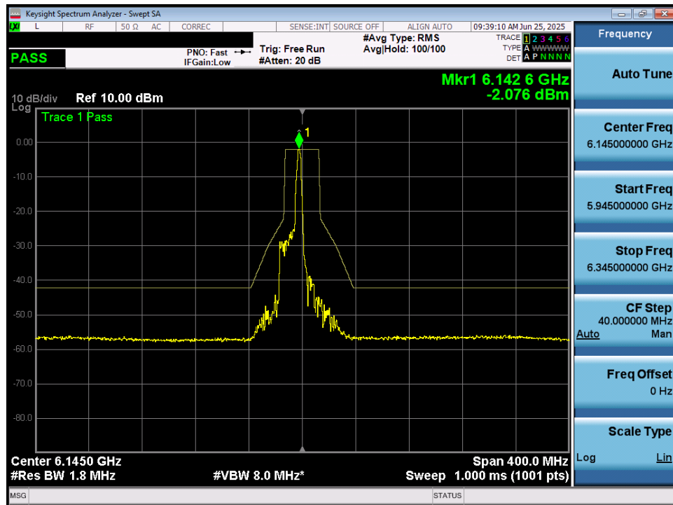
Plot 7-61. In Band Emissions Plot MIMO ANT1 (80MHz 802.11ax/be (26 Tones) (UNII Band 5) – Ch. 39) – LPI/SP
