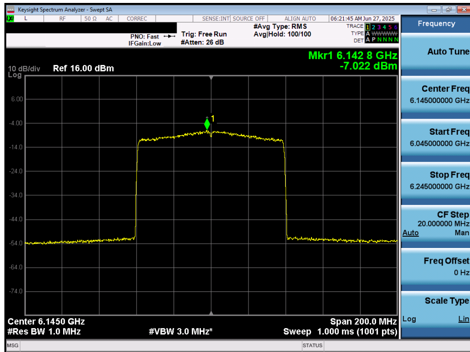
Plot 7-40. Power Spectral Density Plot MIMO ANT1 (80MHz 802.11ax/be (Full Tones) (UNII Band 5) – Ch. 39) - LPI/SP
