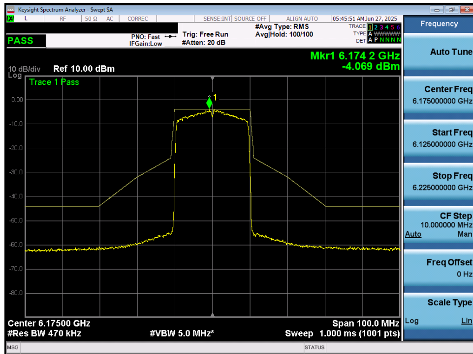
Plot 7-68. In Band Emissions Plot MIMO ANT1 (20MHz 802.11ax/be (Full Tones) (UNII Band 5) – Ch. 45) – LPI/SP
