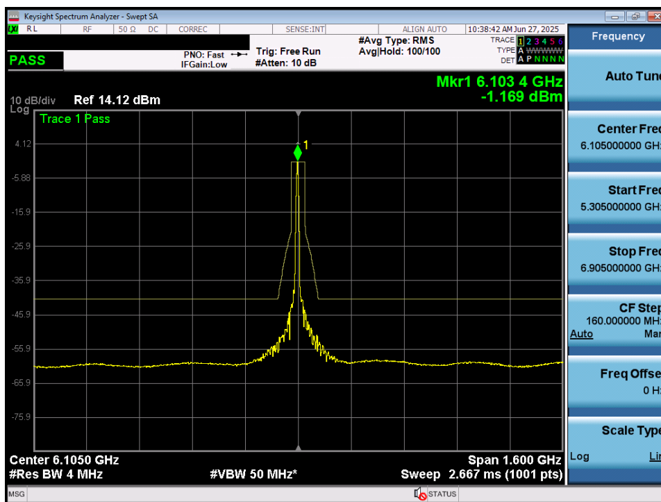
Plot 7-63. In Band Emissions Plot MIMO ANT1 (320MHz 802.11ax/be (26 Tones) (UNII Band 5) – Ch. 31) – LPI/SP
