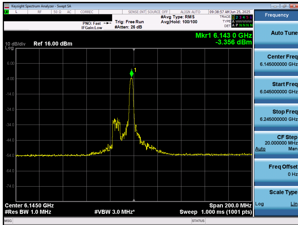
Plot 7-31. Power Spectral Density Plot MIMO ANT1 (80MHz 802.11ax/be (26 Tones) (UNII Band 5) – Ch. 39) – LPI/SP
