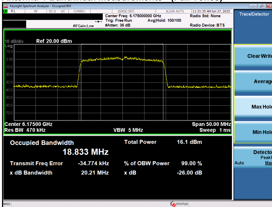
Plot 7-10. 26dB Bandwidth Plot MIMO ANT1 (20MHz 802.11ax/be (Full Tones) (UNII Band 5) – Ch. 45) – LPI/SP
