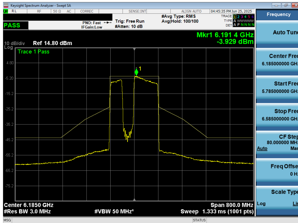
Plot 7-80. In Band Emissions Plot MIMO ANT2 (160MHz 802.11be (996+484 Tones) (UNII Band 5) – Ch. 47) LPI/SP
