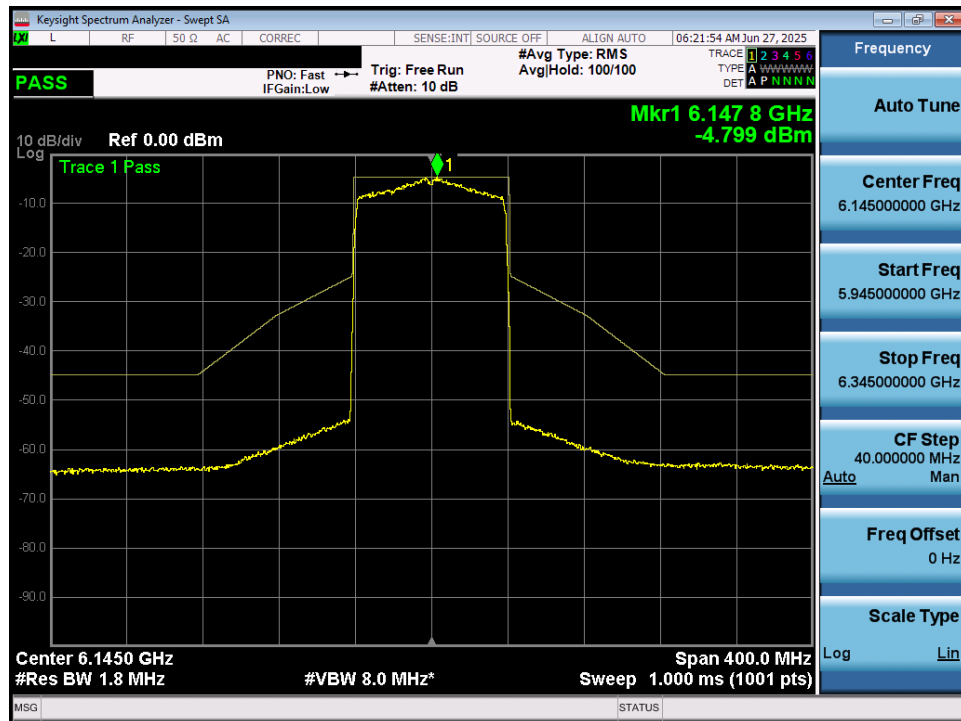
Plot 7-70. In Band Emissions Plot MIMO ANT1 (80MHz 802.11ax/be (Full Tones) (UNII Band 5) – Ch. 39) - LPI/SP
