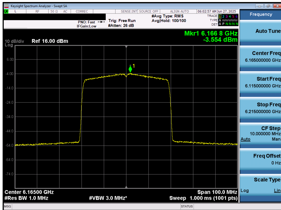
Plot 7-39. Power Spectral Density Plot MIMO ANT1 (40MHz 802.11ax/be (Full Tones) (UNII Band 5) – Ch. 43) – LPI/SP
