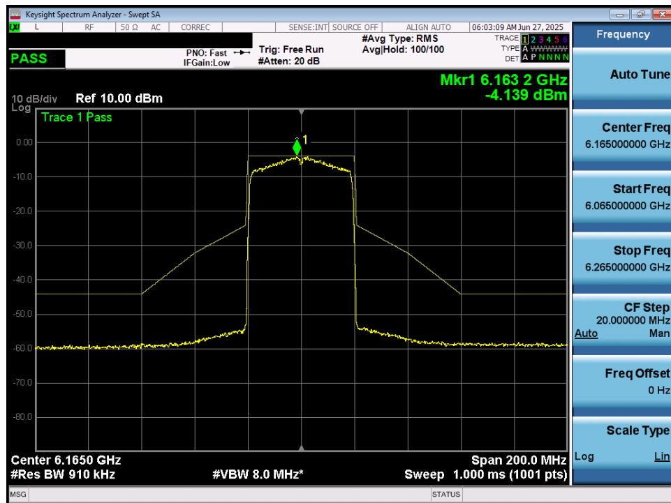
Plot 7-69. In Band Emissions Plot MIMO ANT1 (40MHz 802.11ax/be (Full Tones) (UNII Band 5) – Ch. 43) – LPI/SP
