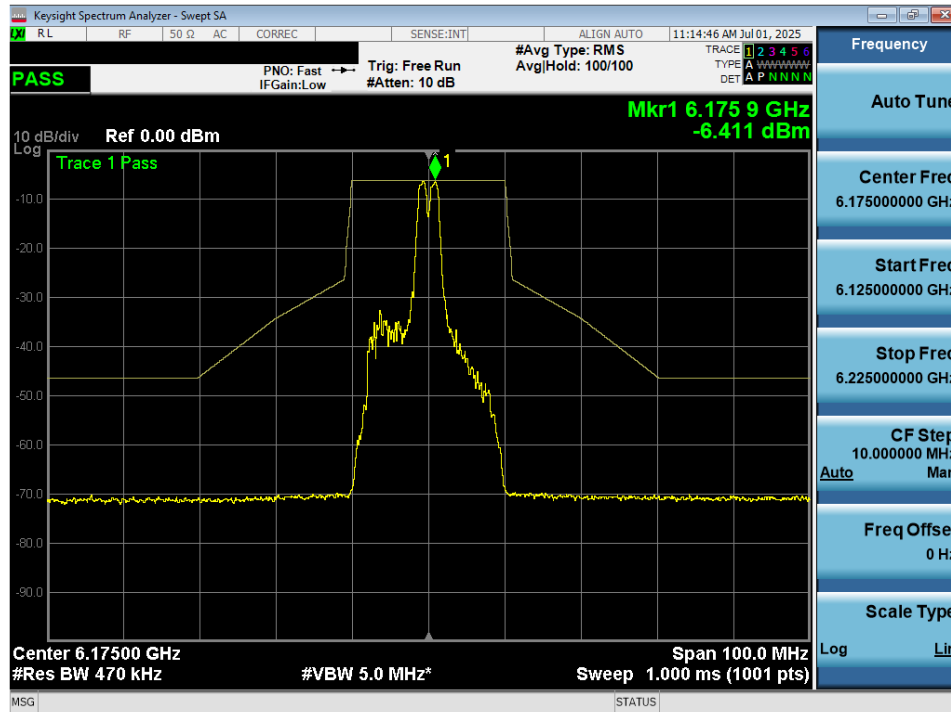
Plot 7-82. In Band Emissions Plot MIMO ANT2 (20MHz 802.11ax/be (Full Tones) (UNII Band 5) – Ch. 45) – LPI/SP
