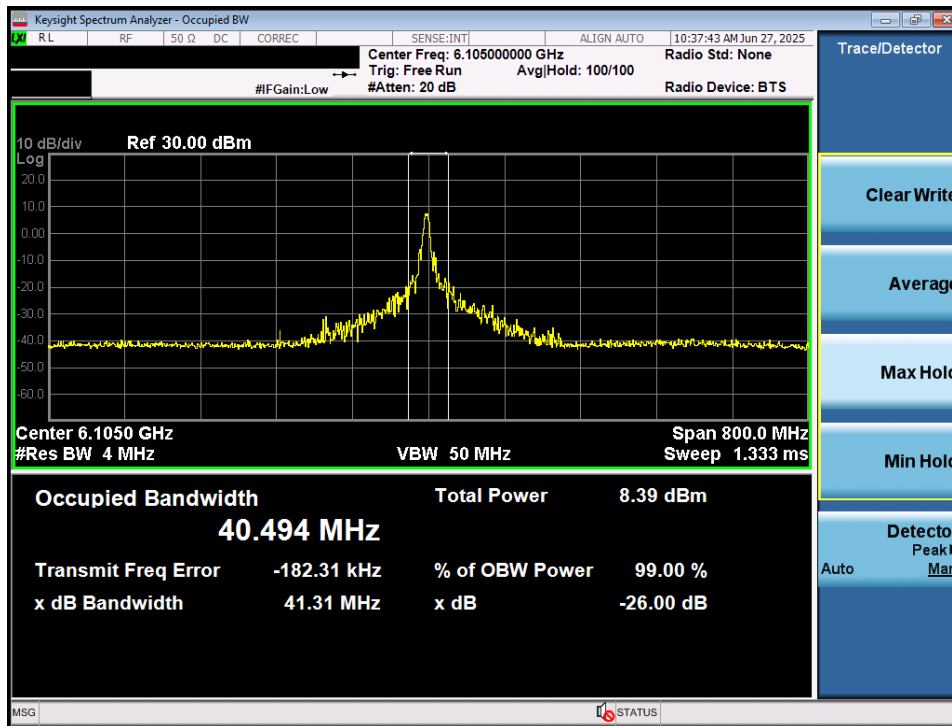
Plot 7-5. 26dB Bandwidth Plot MIMO ANT1 (320MHz 802.11ax/be (26 Tones) (UNII Band 5) – Ch. 31) – LPI/SP
