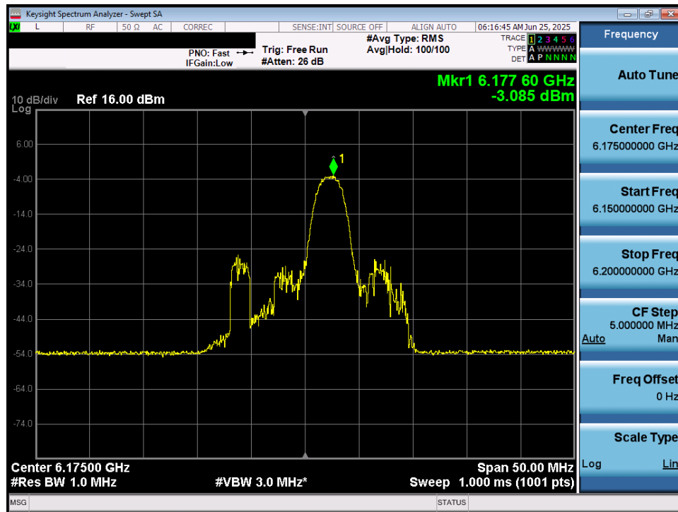
Plot 7-29. Power Spectral Density Plot MIMO ANT1 (20MHz 802.11ax/be (26 Tones) (UNII Band 5) – Ch. 45) – LPI/SP
