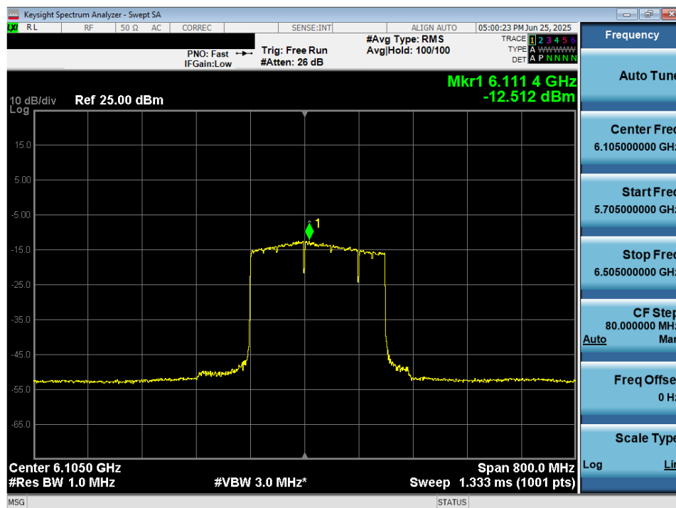
Plot 7-53. Power Spectral Density Plot MIMO ANT2 (320MHz 802.11be (UNII Band 5) – Ch. 31) LPI/SP
