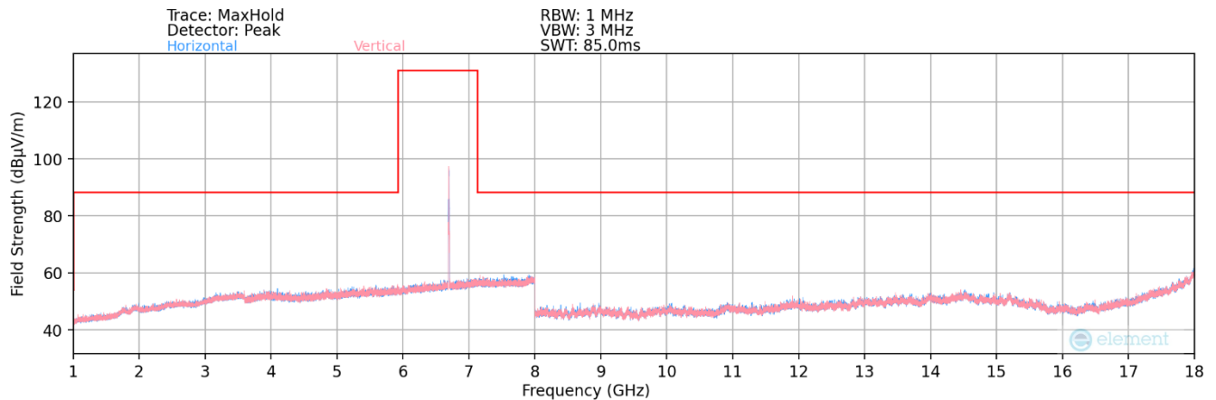
Plot 7-89. Radiated Spurious Plot 1GHz – 18GHz MIMO (802.11ax – UNII Band 7 Ch. 149)
