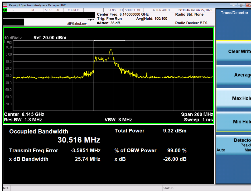
Plot 7-3. 26dB Bandwidth Plot MIMO ANT1 (80MHz 802.11ax/be (26 Tones) (UNII Band 5) – Ch. 39) – LPI/SP
