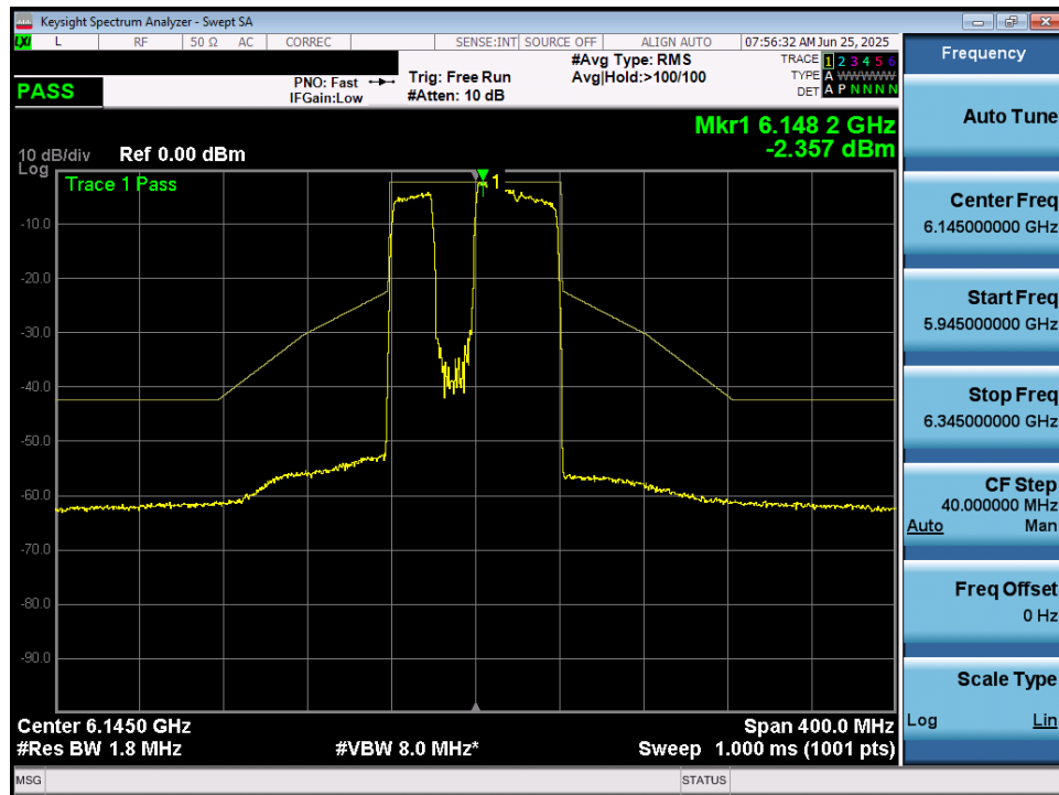
Plot 7-65. In Band Emissions Plot MIMO ANT1 (80MHz 802.11be (484+242 Tones) (UNII Band 5) – Ch. 39) LPI/SP
