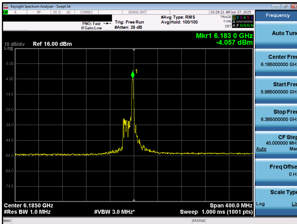
Plot 7-48. Power Spectral Density Plot MIMO ANT2 (160MHz 802.11ax/be (26 Tones) (UNII Band 5) – Ch. 47) – LPI/SP
