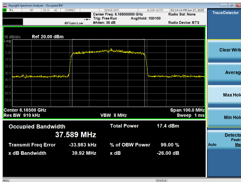
Plot 7-25. 26dB Bandwidth Plot MIMO ANT2 (40MHz 802.11ax/be (Full Tones) (UNII Band 5) – Ch. 43) – LPI/SP
