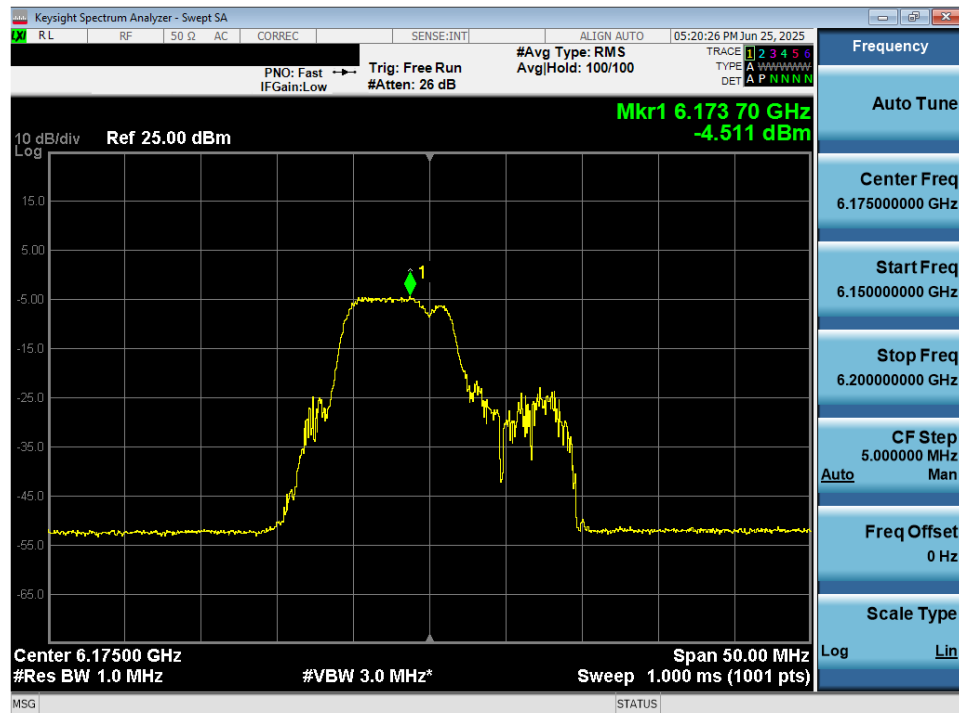
Plot 7-50. Power Spectral Density Plot MIMO ANT2 (20MHz 802.11be (52+26 Tones) (UNII Band 5) – Ch. 45) – LPI/SP
