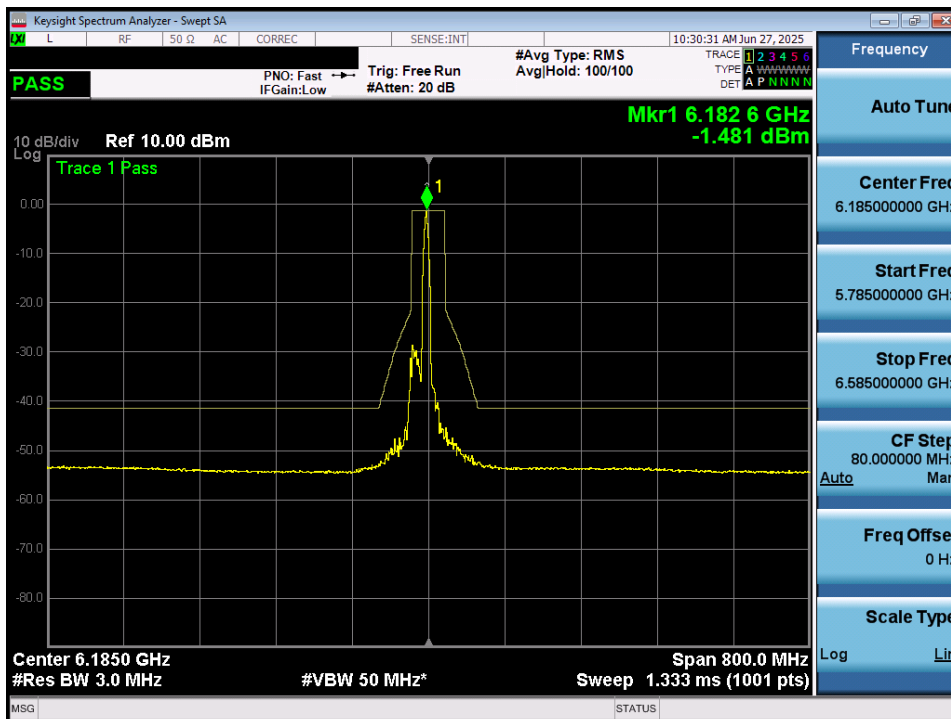
Plot 7-76. In Band Emissions Plot MIMO ANT2 (160MHz 802.11ax/be (26 Tones) (UNII Band 5) – Ch. 47) – LPI/SP
