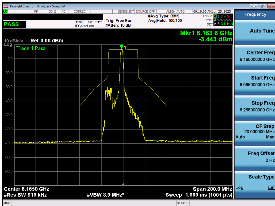
Plot 7-60. In Band Emissions Plot MIMO ANT1 (40MHz 802.11ax/be (26 Tones) (UNII Band 5) – Ch. 43) – LPI/SP
