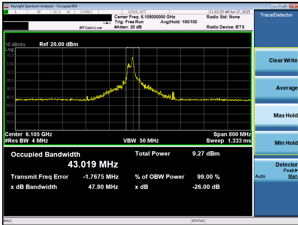
Plot 7-19. 26dB Bandwidth Plot MIMO ANT2 (320MHz 802.11ax/be (26 Tones) (UNII Band 5) – Ch. 31) – LPI/SP
