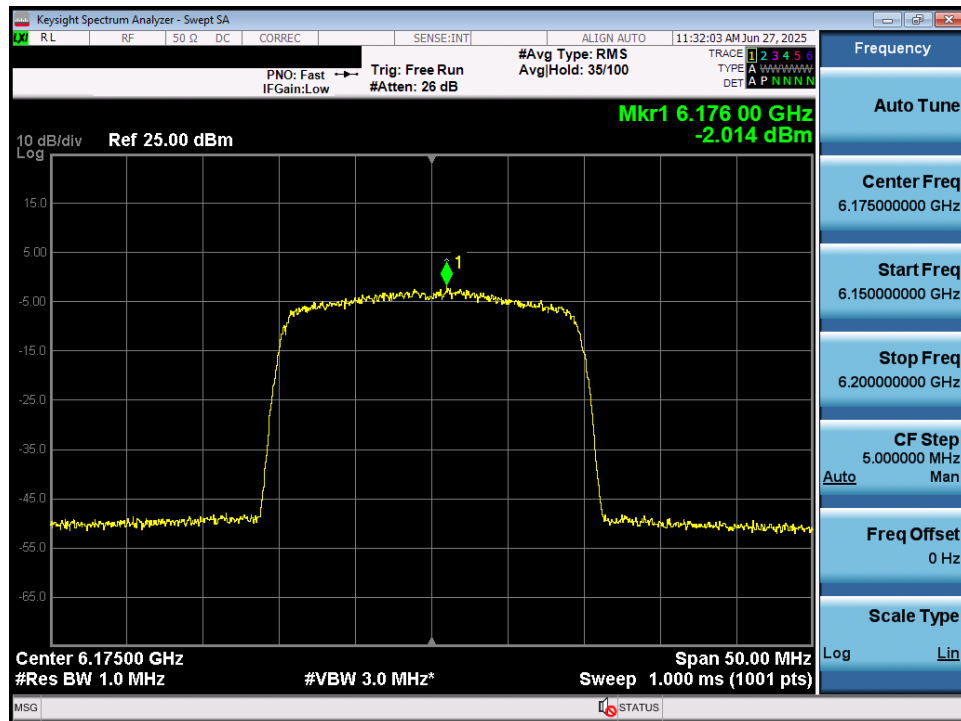
Plot 7-38. Power Spectral Density Plot MIMO ANT1 (20MHz 802.11ax/be (Full Tones) (UNII Band 5) – Ch. 45) – LPI/SP
