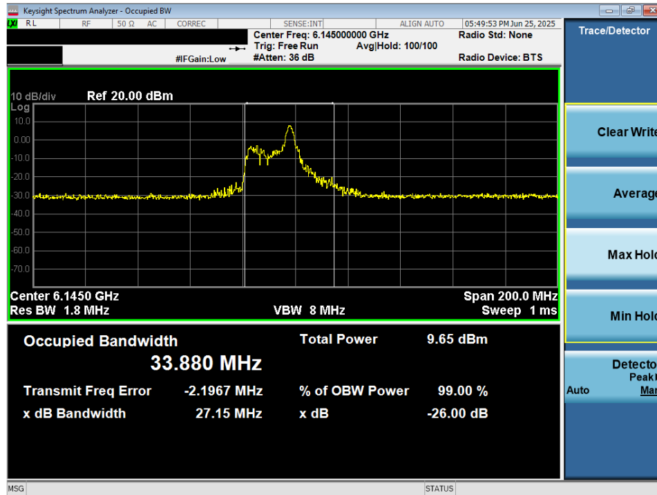
Plot 7-17. 26dB Bandwidth Plot MIMO ANT2 (80MHz 802.11ax/be (26 Tones) (UNII Band 5) – Ch. 39) – LPI/SP
