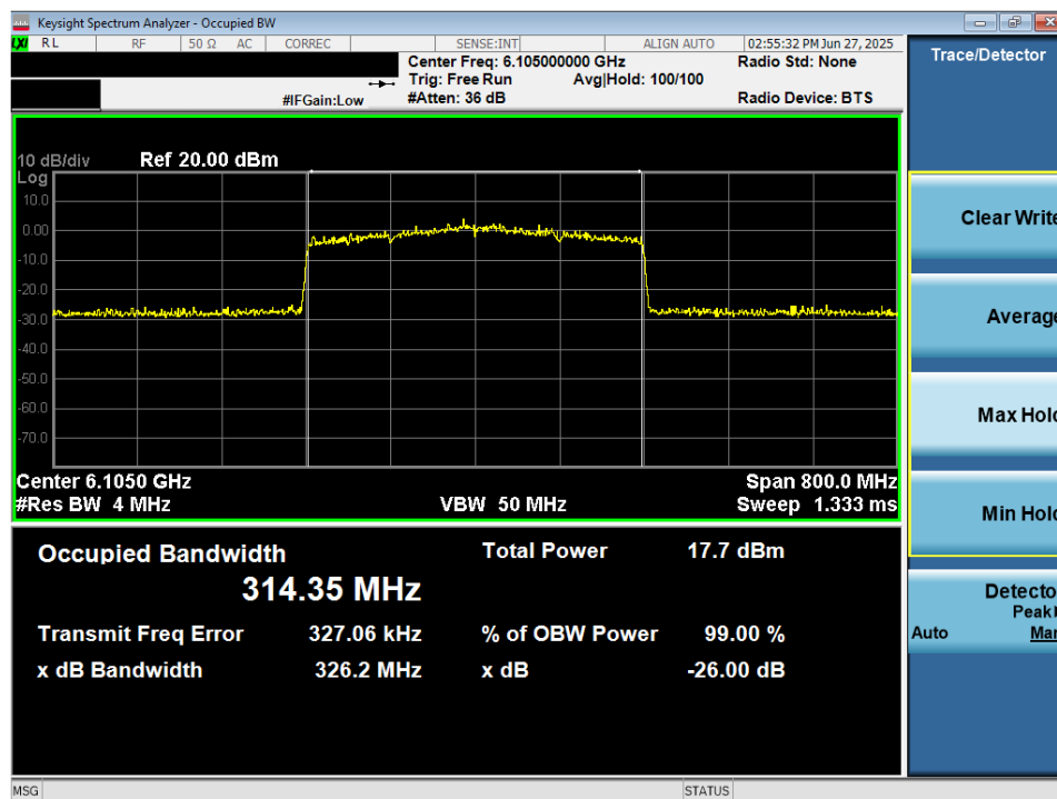
Plot 7-28. 26dB Bandwidth Plot MIMO ANT2 (320MHz 802.11ax/be (Full Tones) (UNII Band 5) – Ch. 31) - LPI/SP
