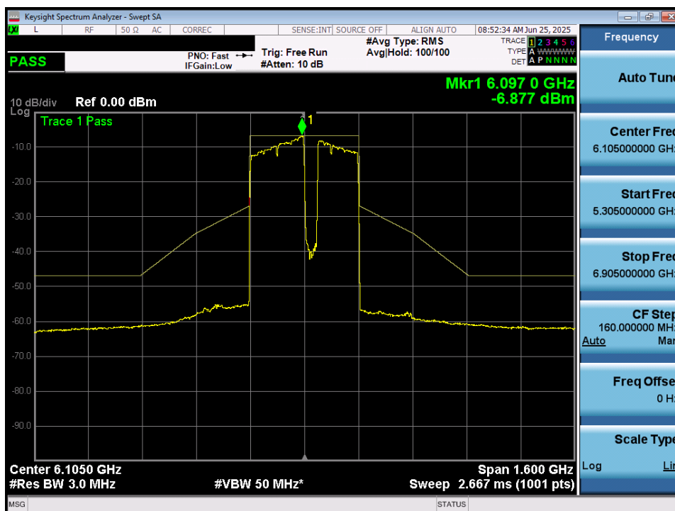
Plot 7-67. In Band Emissions Plot MIMO ANT1 (320MHz 802.11be (3*996+484 Tones) (UNII Band 5) – Ch. 31) LPI/SP
