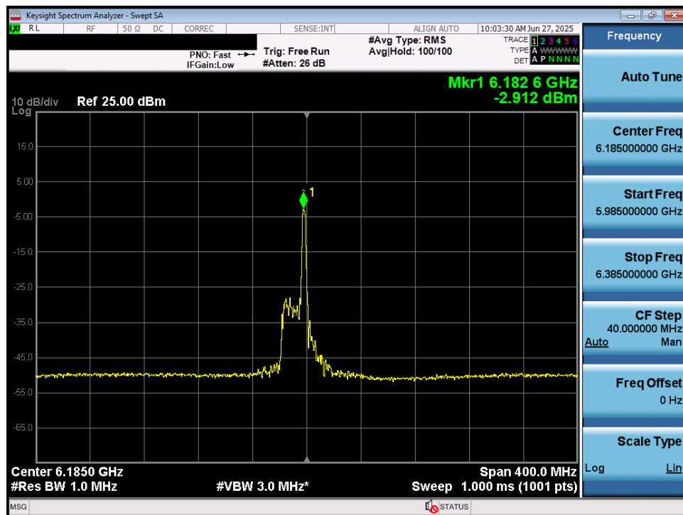
Plot 7-32. Power Spectral Density Plot MIMO ANT1 (160MHz 802.11ax/be (26 Tones) (UNII Band 5) – Ch. 47) – LPI/SP
