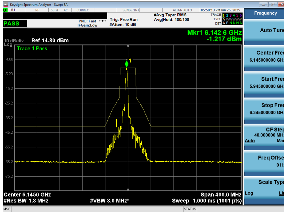
Plot 7-75. In Band Emissions Plot MIMO ANT2 (80MHz 802.11ax/be (26 Tones) (UNII Band 5) – Ch. 39) – LPI/SP
