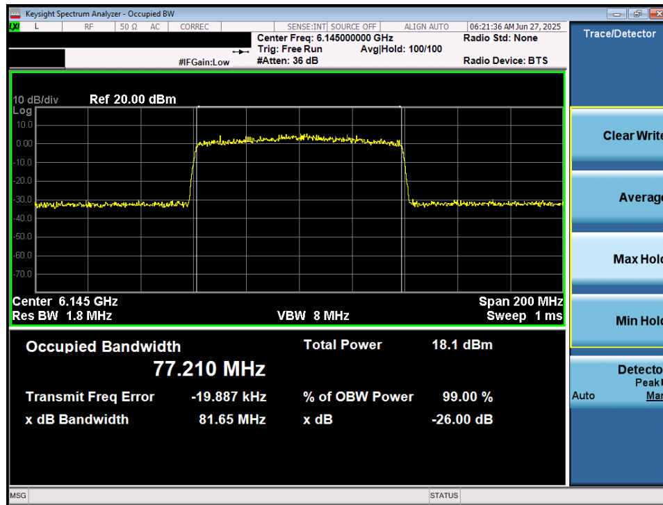
Plot 7-12. 26dB Bandwidth Plot MIMO ANT1 (80MHz 802.11ax/be (Full Tones) (UNII Band 5) – Ch. 39) - LPI/SP
