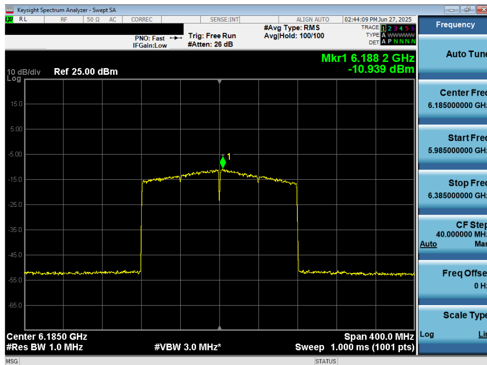
Plot 7-57. Power Spectral Density Plot MIMO ANT2 (160MHz 802.11ax/be (Full Tones) (UNII Band 5) – Ch. 47) - LPI/SP
