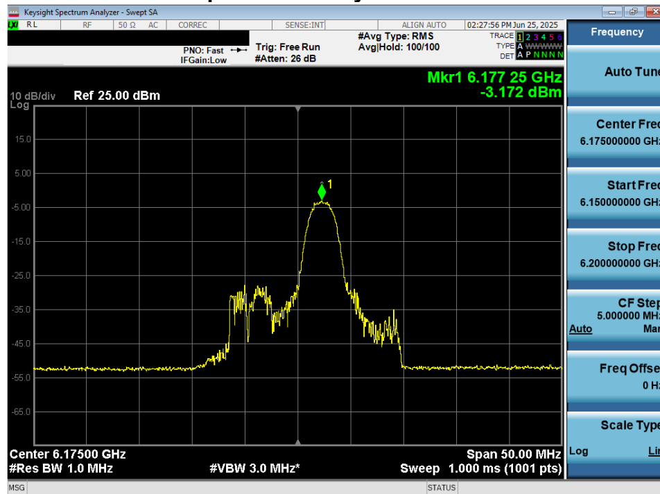
Plot 7-45. Power Spectral Density Plot MIMO ANT2 (20MHz 802.11ax/be (26 Tones) (UNII Band 5) – Ch. 45) – LPI/SP
