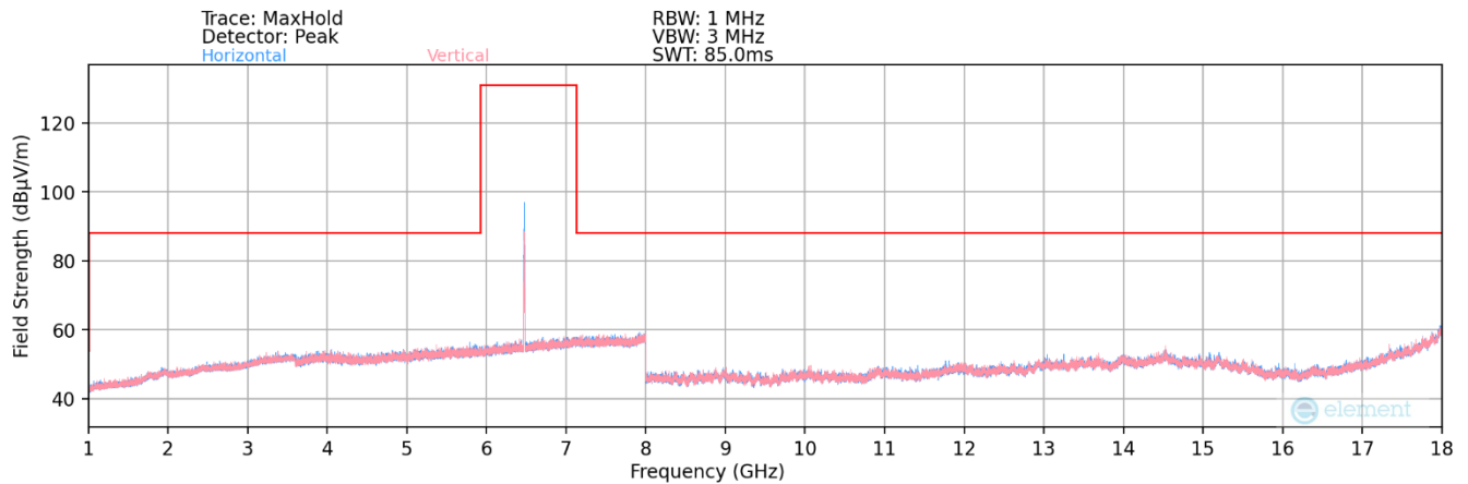
Plot 7-88. Radiated Spurious Plot 1GHz – 18GHz MIMO (802.11ax – UNII Band 6 Ch. 105)
