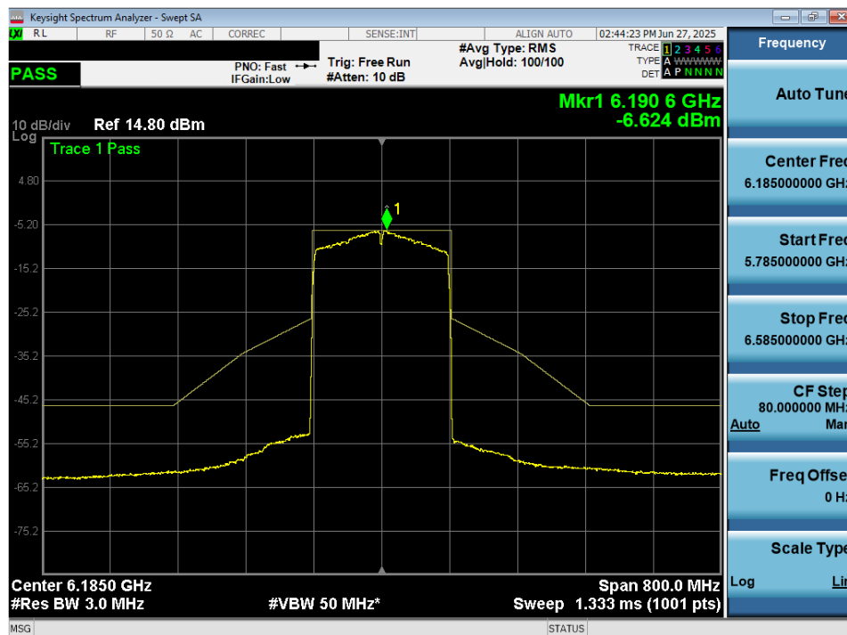
Plot 7-85. In Band Emissions Plot MIMO ANT2 (160MHz 802.11ax/be (Full Tones) (UNII Band 5) – Ch. 47) - LPI/SP
