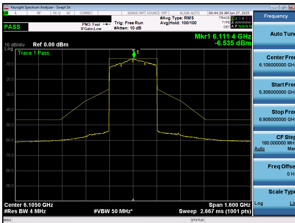
Plot 7-72. In Band Emissions Plot MIMO ANT1 (320MHz 802.11ax/be (Full Tones) (UNII Band 5) – Ch. 31) - LPI/SP
