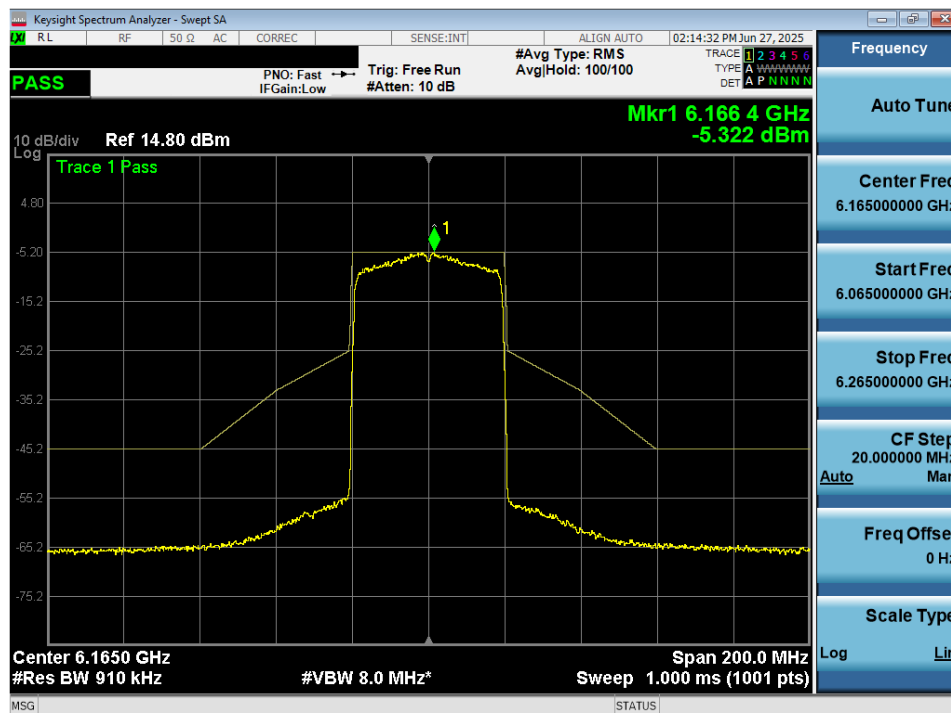
Plot 7-83. In Band Emissions Plot MIMO ANT2 (40MHz 802.11ax/be (Full Tones) (UNII Band 5) – Ch. 43) – LPI/SP
