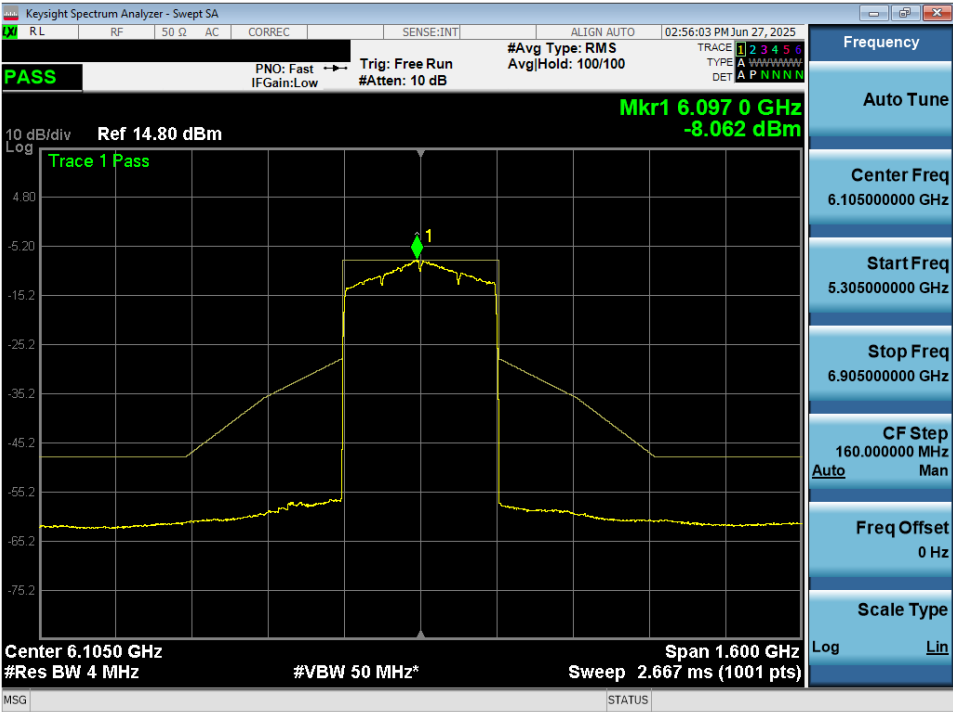
Plot 7-86. In Band Emissions Plot MIMO ANT2 (320MHz 802.11ax/be (Full Tones) (UNII Band 5) – Ch. 31) - LPI/SP
