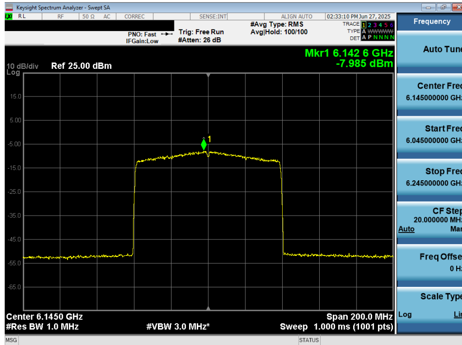
Plot 7-56. Power Spectral Density Plot MIMO ANT2 (80MHz 802.11ax/be (Full Tones) (UNII Band 5) – Ch. 39) - LPI/SP
