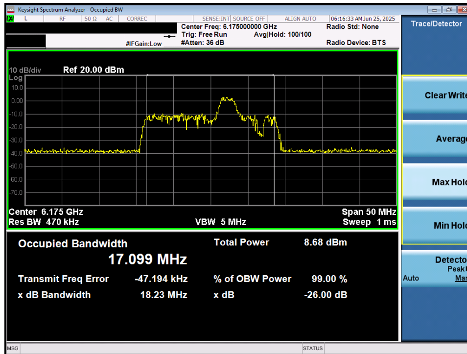
Plot 7-1. 26dB Bandwidth Plot MIMO ANT1 (20MHz 802.11ax/be (26 Tones) (UNII Band 5) – Ch. 45) – LPI/SP
