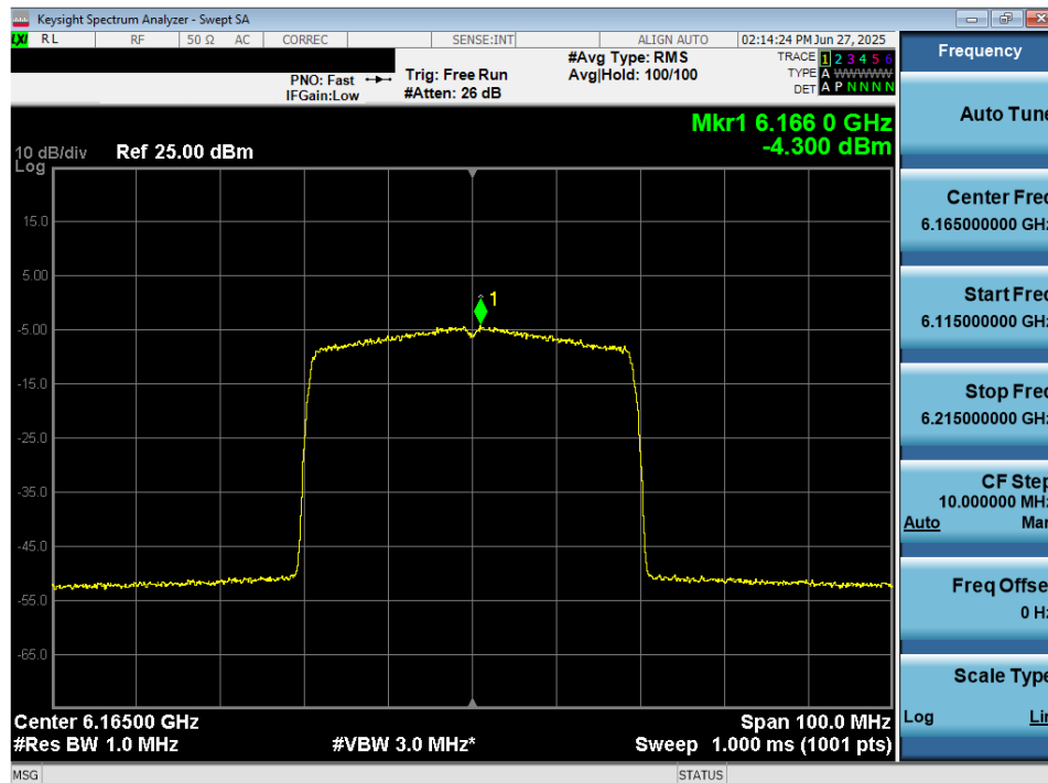
Plot 7-55. Power Spectral Density Plot MIMO ANT2 (40MHz 802.11ax/be (Full Tones) (UNII Band 5) – Ch. 43) – LPI/SP
