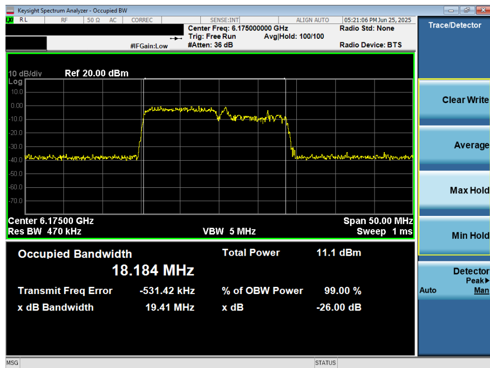
Plot 7-20. 26dB Bandwidth Plot MIMO ANT2 (20MHz 802.11be (106+26 Tones) (UNII Band 5) – Ch. 45) – LPI/SP
