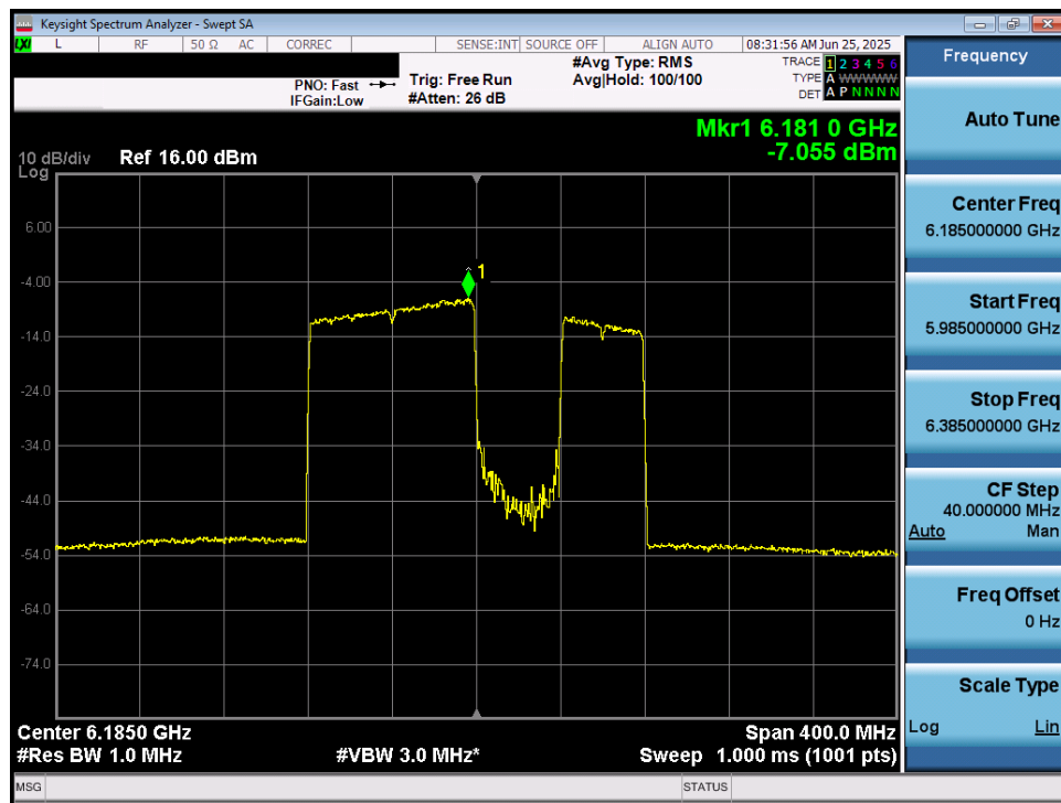
Plot 7-36. Power Spectral Density Plot MIMO ANT1 (160MHz 802.11be (996+484 Tones) (UNII Band 5) – Ch. 47) LPI/SP
