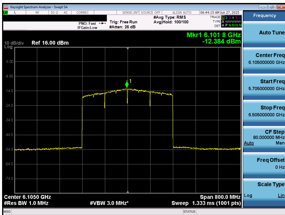
Plot 7-42. Power Spectral Density Plot MIMO ANT1 (320MHz 802.11ax/be (Full Tones) (UNII Band 5) – Ch. 31) - LPI/SP
