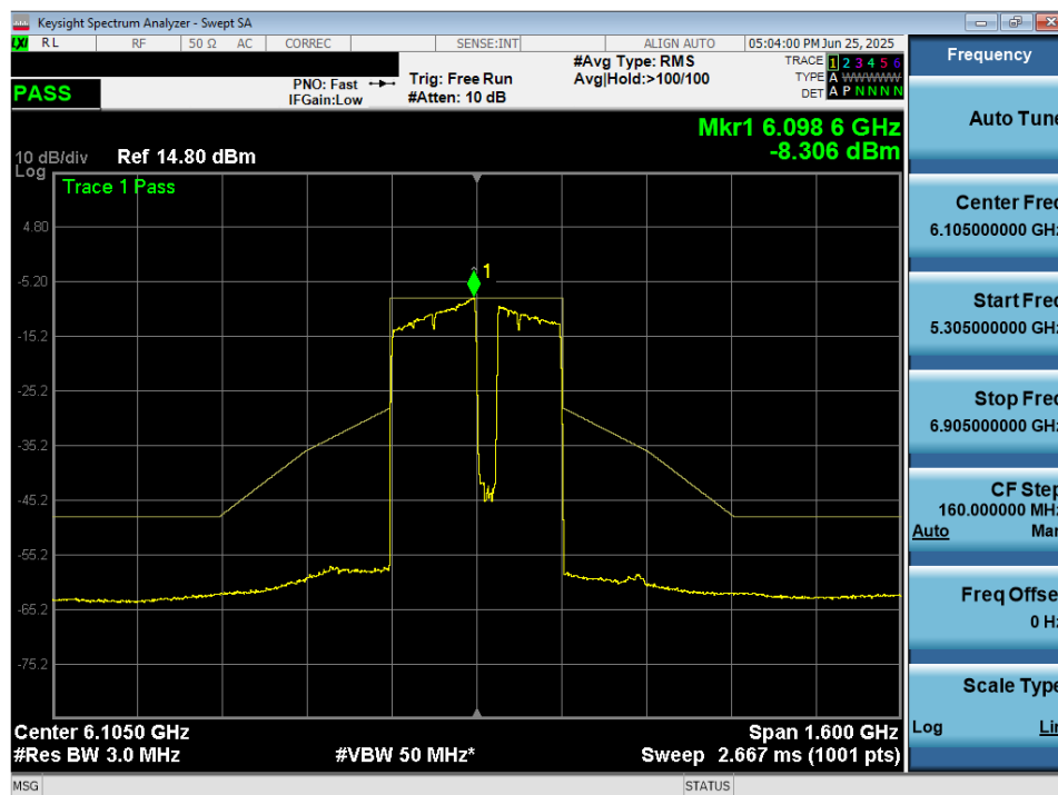
Plot 7-81. In Band Emissions Plot MIMO ANT2 (320MHz 802.11be (3*996+484 Tones) (UNII Band 5) – Ch. 31) LPI/SP
