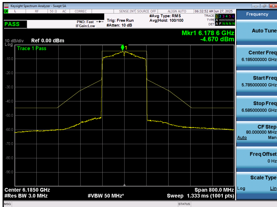
Plot 7-71. In Band Emissions Plot MIMO ANT1 (160MHz 802.11ax/be (Full Tones) (UNII Band 5) – Ch. 47) - LPI/SP
