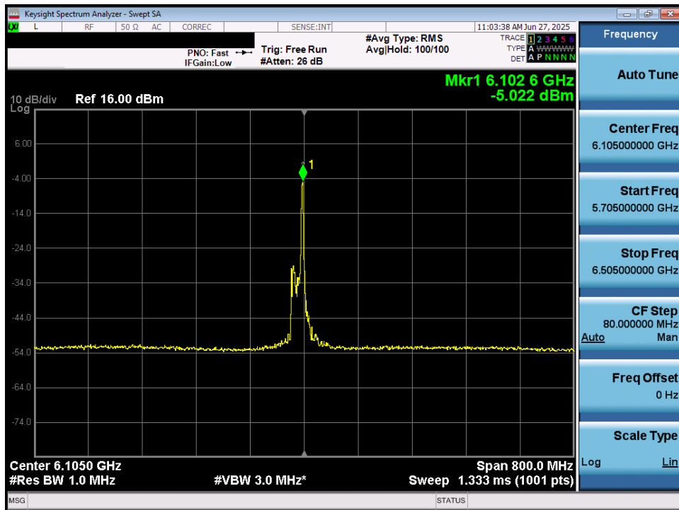
Plot 7-49. Power Spectral Density Plot MIMO ANT2 (320MHz 802.11ax/be (26 Tones) (UNII Band 5) – Ch. 31) – LPI/SP
