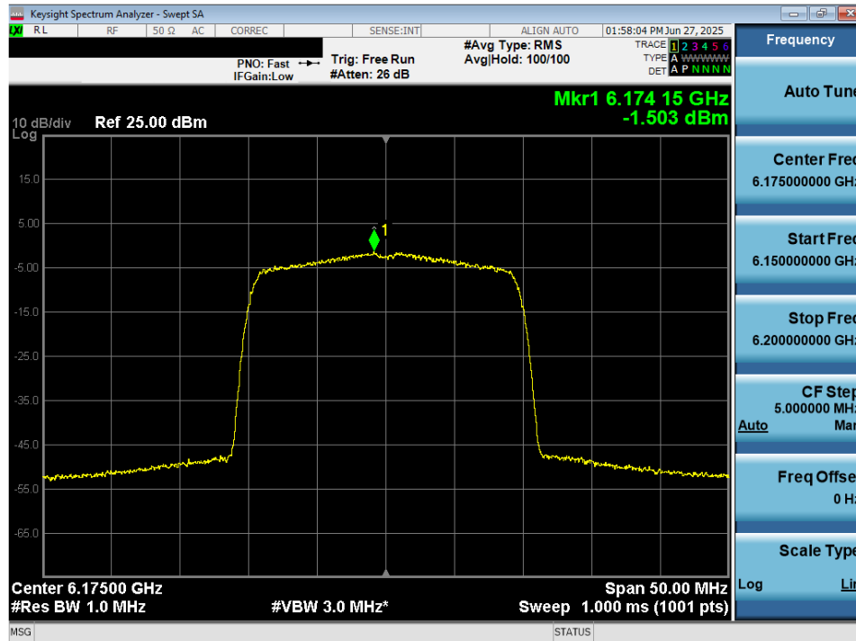
Plot 7-54. Power Spectral Density Plot MIMO ANT2 (20MHz 802.11ax/be (Full Tones) (UNII Band 5) – Ch. 45) – LPI/SP
