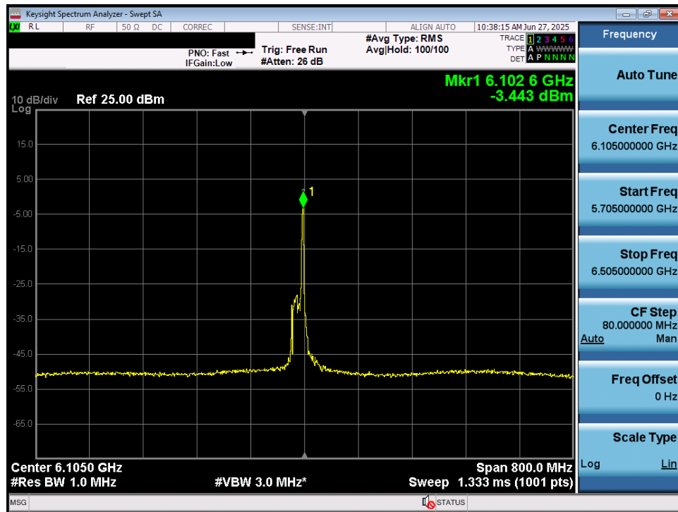
Plot 7-33. Power Spectral Density Plot MIMO ANT1 (320MHz 802.11ax/be (26 Tones) (UNII Band 5) – Ch. 31) – LPI/SP
