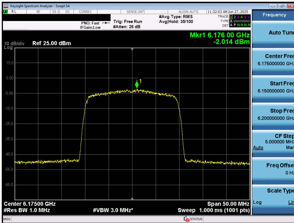
Plot 7-43. Power Spectral Density Plot MIMO ANT1 (20MHz 802.11ax/be (Full Tones) (UNII Band 5) – Ch. 45) – LPI/SP
