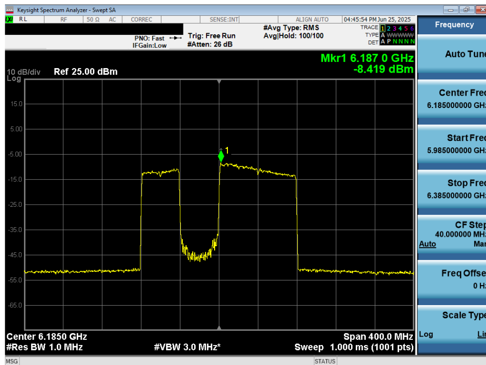
Plot 7-52. Power Spectral Density Plot MIMO ANT2 (160MHz 802.11be (996+484 Tones) (UNII Band 5) – Ch. 47) LPI/SP
