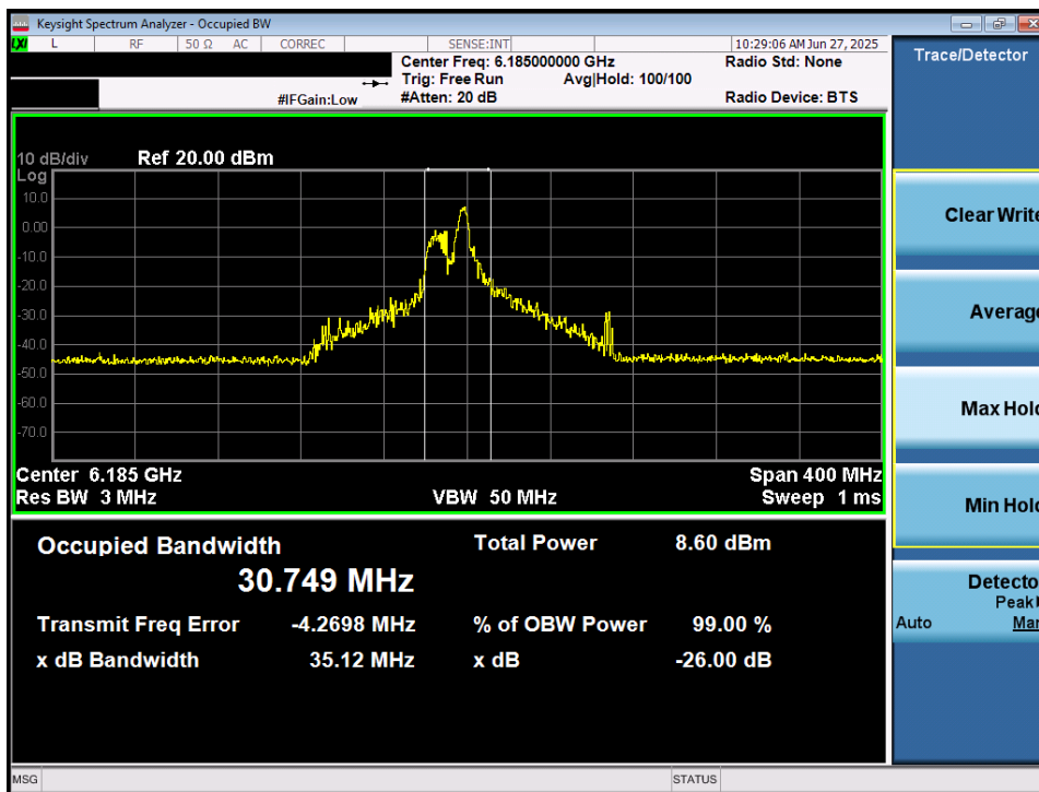
Plot 7-18. 26dB Bandwidth Plot MIMO ANT2 (160MHz 802.11ax/be (26 Tones) (UNII Band 5) – Ch. 47) – LPI/SP
