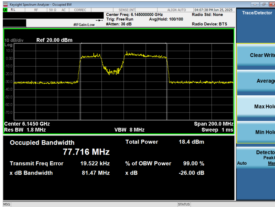
Plot 7-21. 26dB Bandwidth Plot MIMO ANT2 (80MHz 802.11be (484+242 Tones) (UNII Band 5) – Ch. 39) LPI/SP
