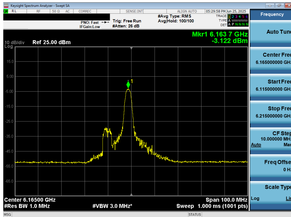
Plot 7-46. Power Spectral Density Plot MIMO ANT2 (40MHz 802.11ax/be (26 Tones) (UNII Band 5) – Ch. 43) – LPI/SP
