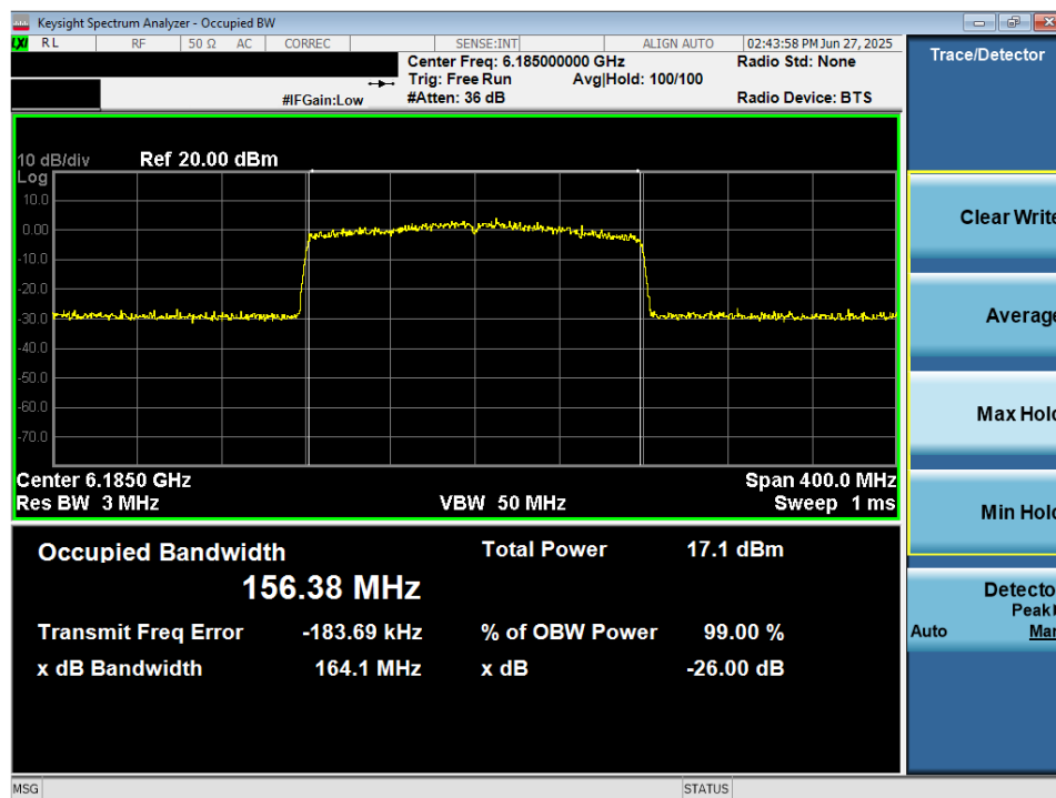
Plot 7-27. 26dB Bandwidth Plot MIMO ANT2 (160MHz 802.11ax/be (Full Tones) (UNII Band 5) – Ch. 47) - LPI/SP
