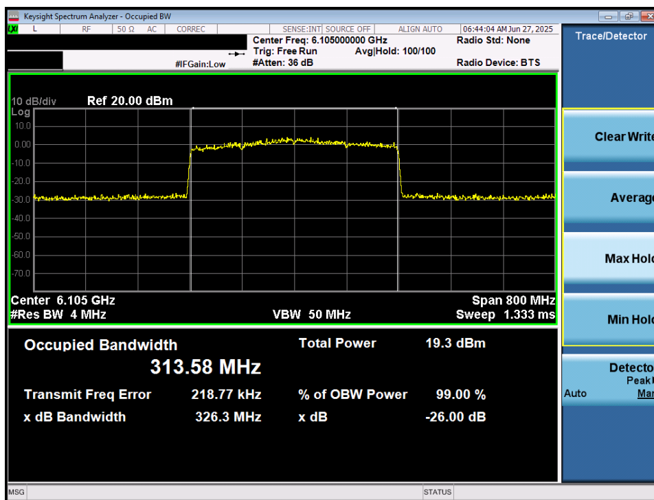
Plot 7-14. 26dB Bandwidth Plot MIMO ANT1 (320MHz 802.11ax/be (Full Tones) (UNII Band 5) – Ch. 31) - LPI/SP
