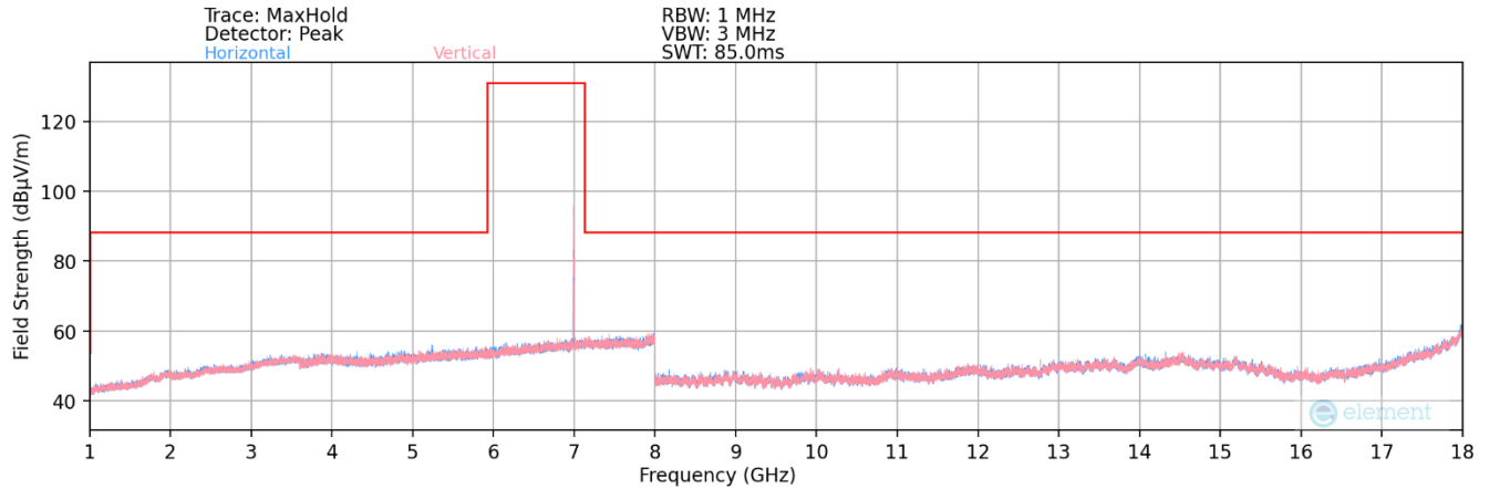
Plot 7-90. Radiated Spurious Plot 1GHz – 18GHz MIMO (802.11ax – U Band 8 Ch. 209)
