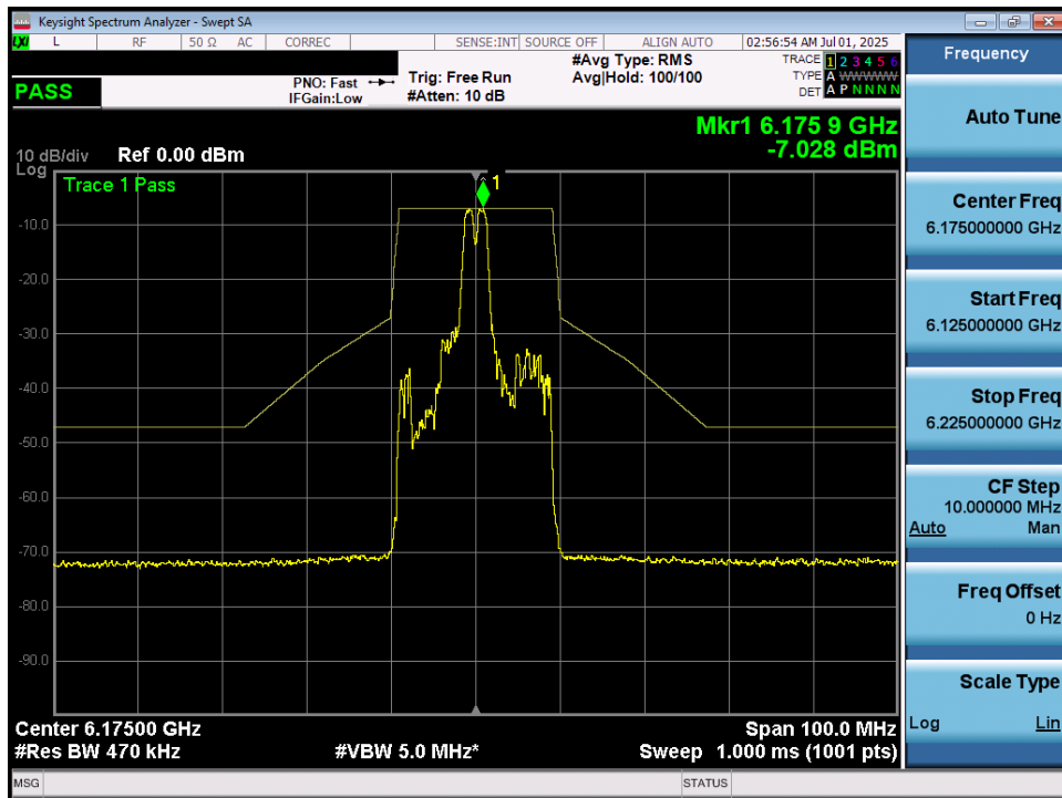
Plot 7-59. In Band Emissions Plot MIMO ANT1 (20MHz 802.11ax/be (26 Tones) (UNII Band 5) – Ch. 45) – LPI/SP
