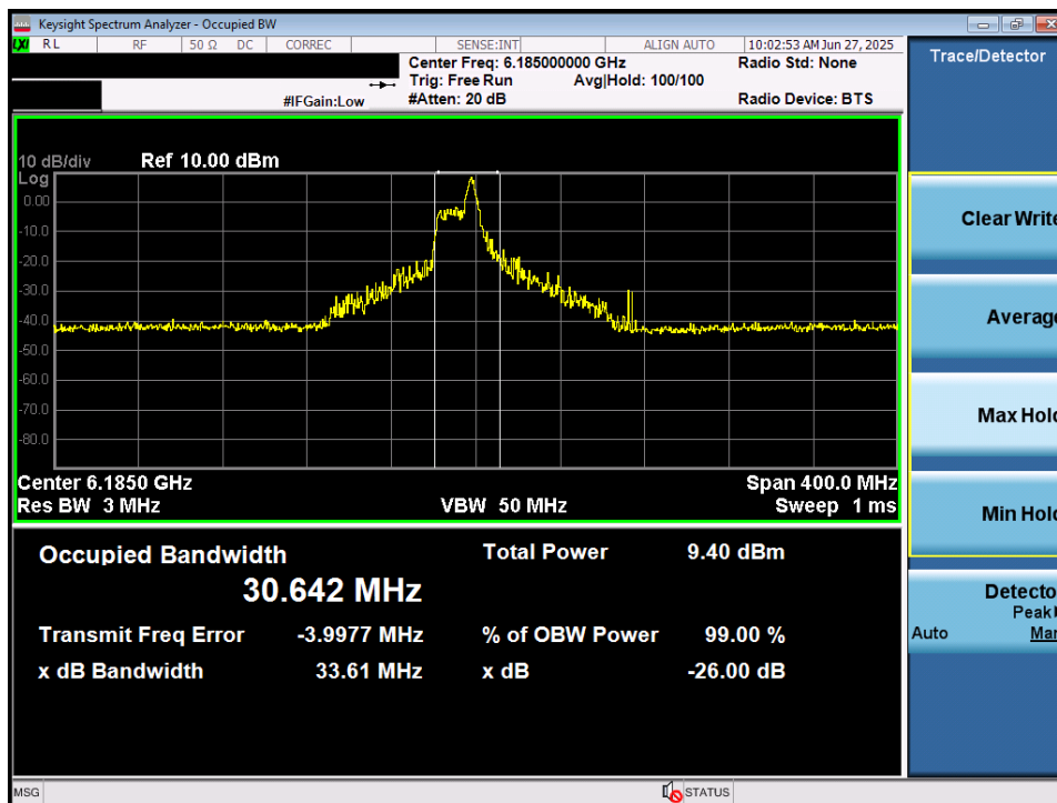
Plot 7-4. 26dB Bandwidth Plot MIMO ANT1 (160MHz 802.11ax/be (26 Tones) (UNII Band 5) – Ch. 47) – LPI/SP
