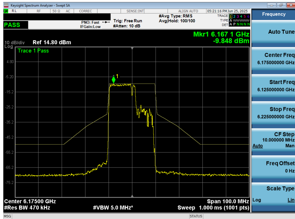
Plot 7-78. In Band Emissions Plot MIMO ANT2 (20MHz 802.11be (106+26 Tones) (UNII Band 5) – Ch. 45) - LPI/SP
