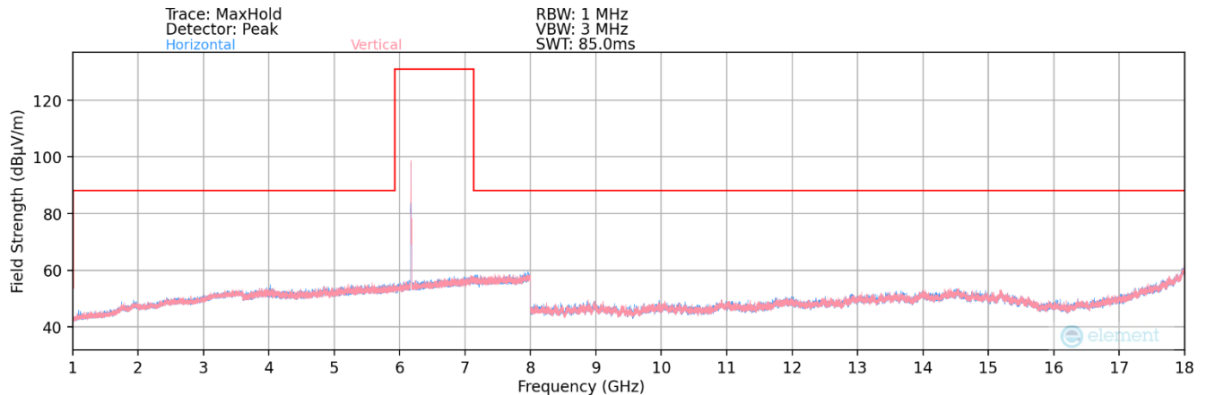
Plot 7-87. Radiated Spurious Plot 1GHz – 18GHz MIMO (802.11ax – UNII Band 5 Ch. 45)
