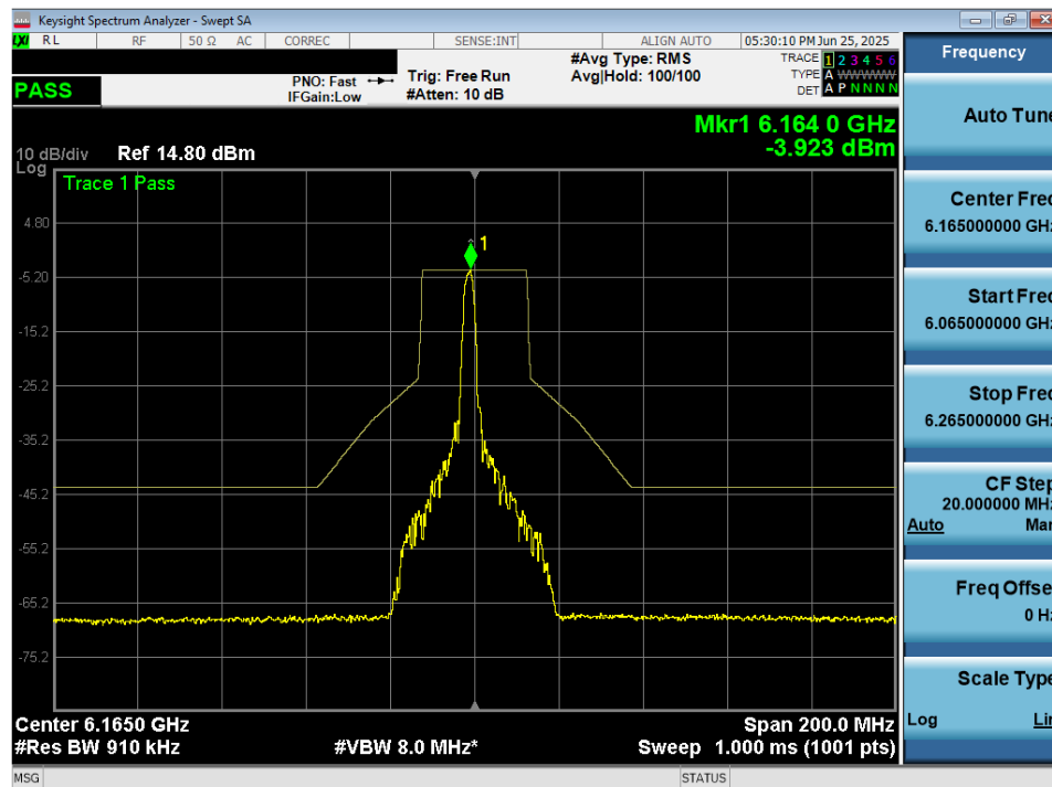
Plot 7-74. In Band Emissions Plot MIMO ANT2 (40MHz 802.11ax/be (26 Tones) (UNII Band 5) – Ch. 43) – LPI/SP
