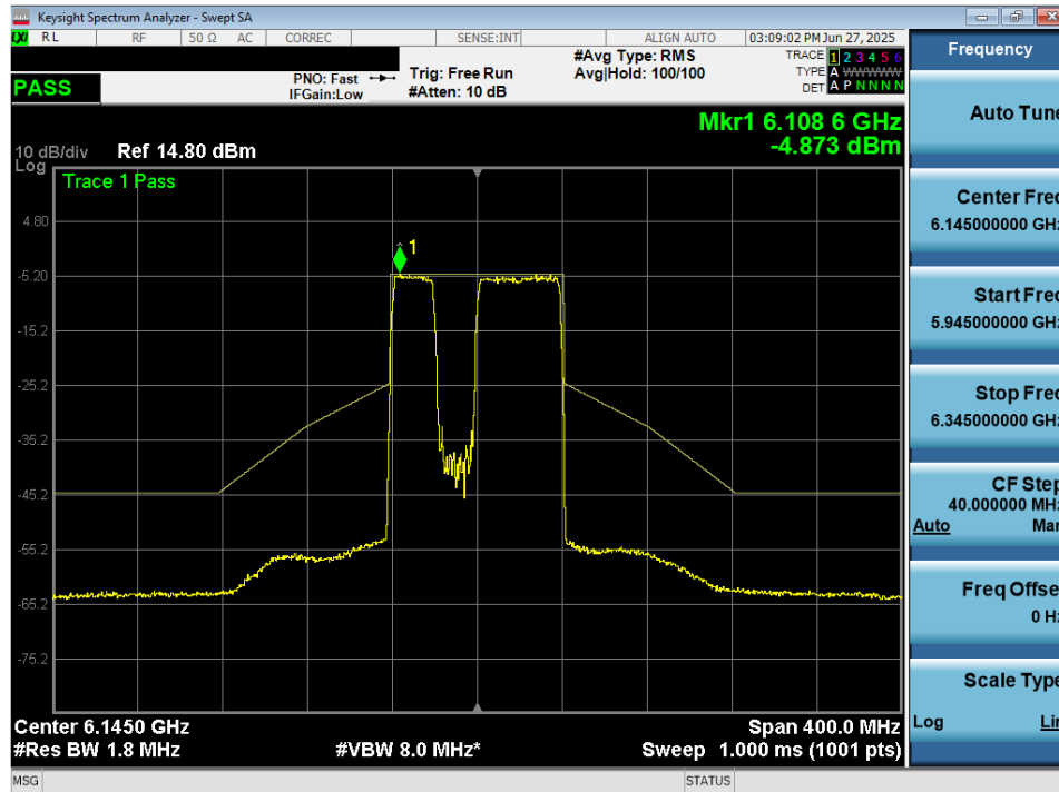
Plot 7-79. In Band Emissions Plot MIMO ANT2 (80MHz 802.11be (484+242 Tones) (UNII Band 5) – Ch. 39) LPI/SP
