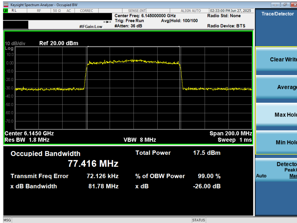
Plot 7-26. 26dB Bandwidth Plot MIMO ANT2 (80MHz 802.11ax/be (Full Tones) (UNII Band 5) – Ch. 39) - LPI/SP
