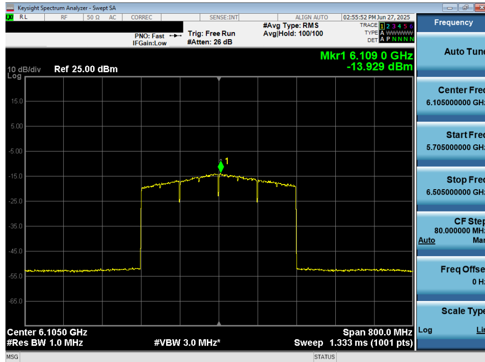
Plot 7-58. Power Spectral Density Plot MIMO ANT2 (320MHz 802.11ax/be (Full Tones) (UNII Band 5) – Ch. 31) - LPI/SP
