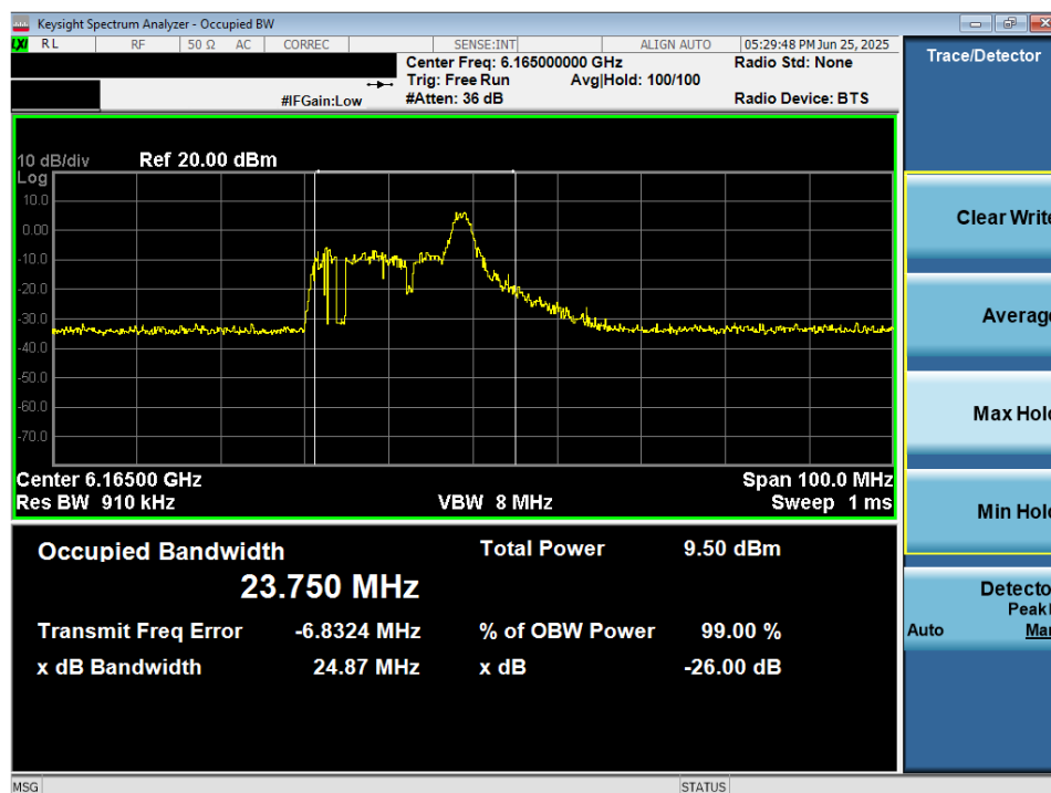
Plot 7-16. 26dB Bandwidth Plot MIMO ANT2 (40MHz 802.11ax/be (26 Tones) (UNII Band 5) – Ch. 43) – LPI/SP
