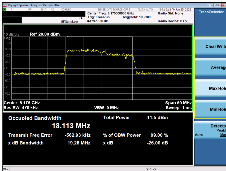
Plot 7-6. 26dB Bandwidth Plot MIMO ANT1 (20MHz 802.11be (106+26 Tones) (UNII Band 5) – Ch. 45) – LPI/SP
