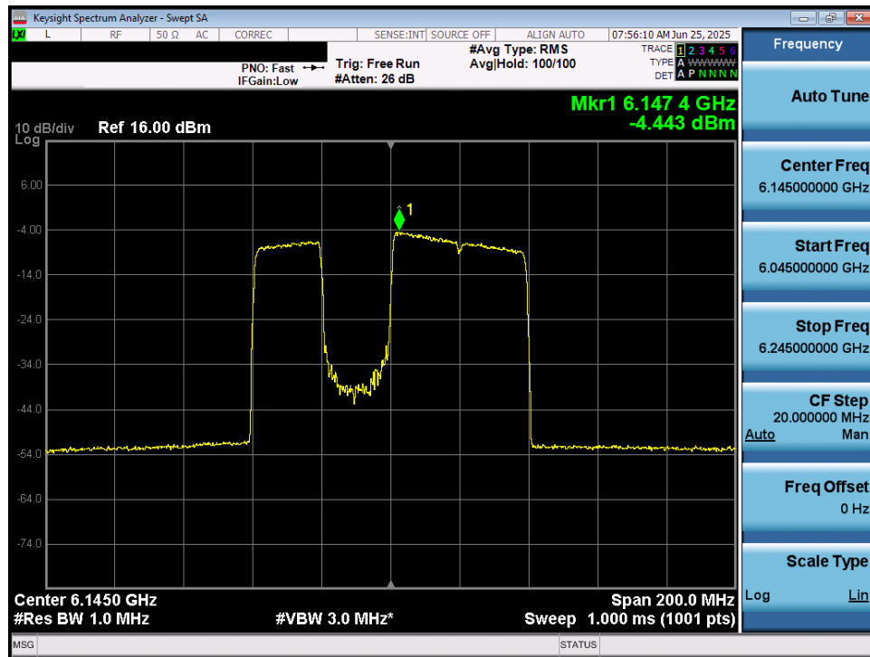
Plot 7-35. Power Spectral Density Plot MIMO ANT1 (80MHz 802.11be (484+242 Tones) (UNII Band 5) – Ch. 39) LPI/SP
