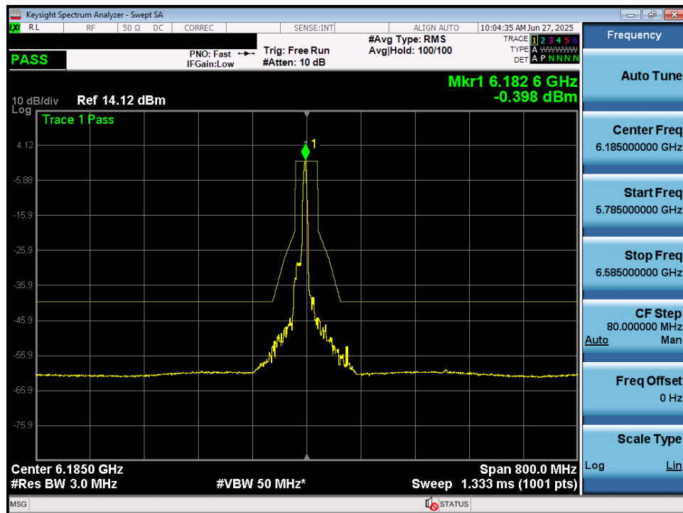
Plot 7-62. In Band Emissions Plot MIMO ANT1 (160MHz 802.11ax/be (26 Tones) (UNII Band 5) – Ch. 47) – LPI/SP
