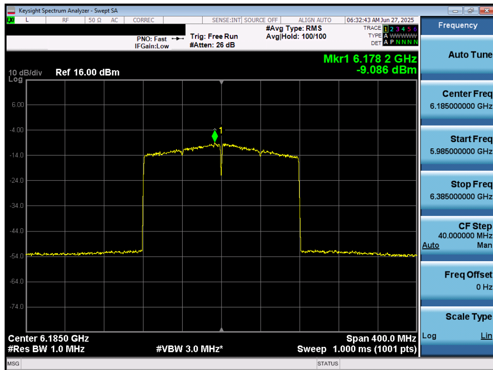
Plot 7-41. Power Spectral Density Plot MIMO ANT1 (160MHz 802.11ax/be (Full Tones) (UNII Band 5) – Ch. 47) - LPI/SP
