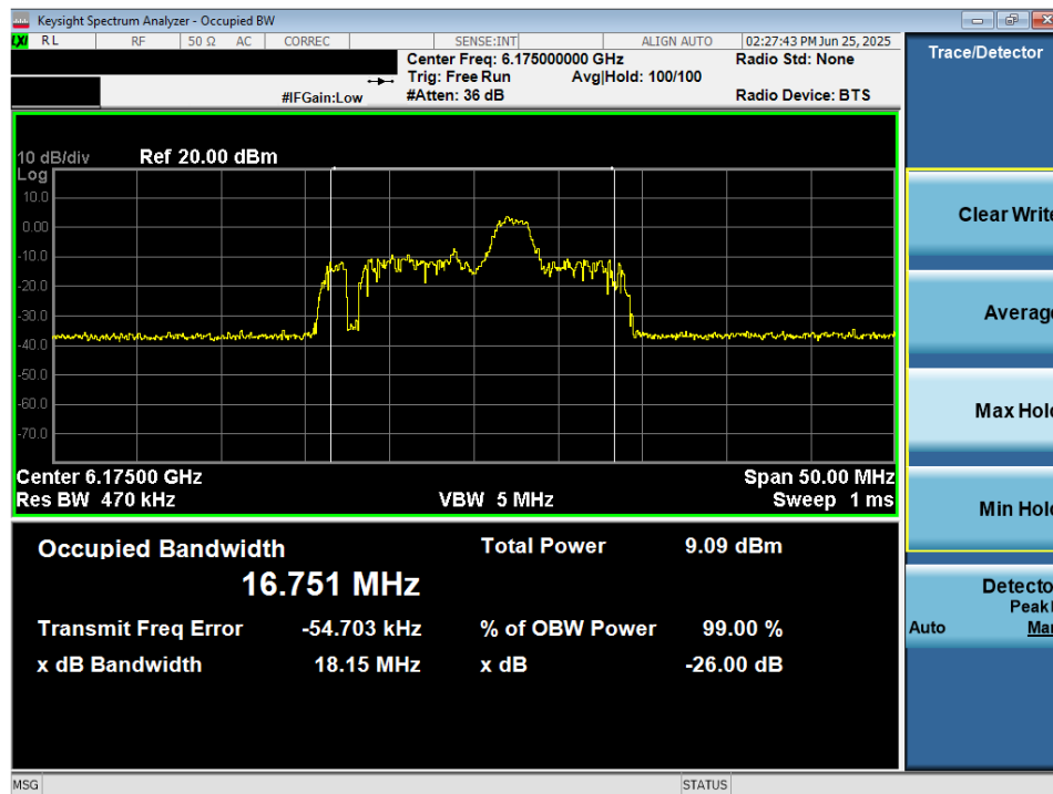
Plot 7-15. 26dB Bandwidth Plot MIMO ANT2 (20MHz 802.11ax/be (26 Tones) (UNII Band 5) – Ch. 45) – LPI/SP
