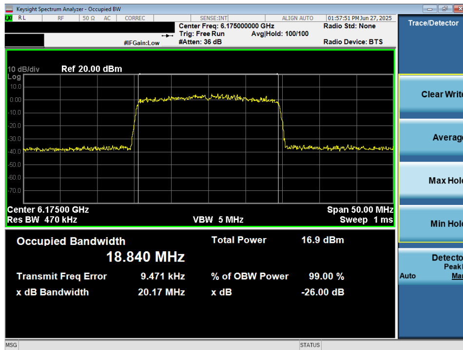
Plot 7-24. 26dB Bandwidth Plot MIMO ANT2 (20MHz 802.11ax/be (Full Tones) (UNII Band 5) – Ch. 45) – LPI/SP
