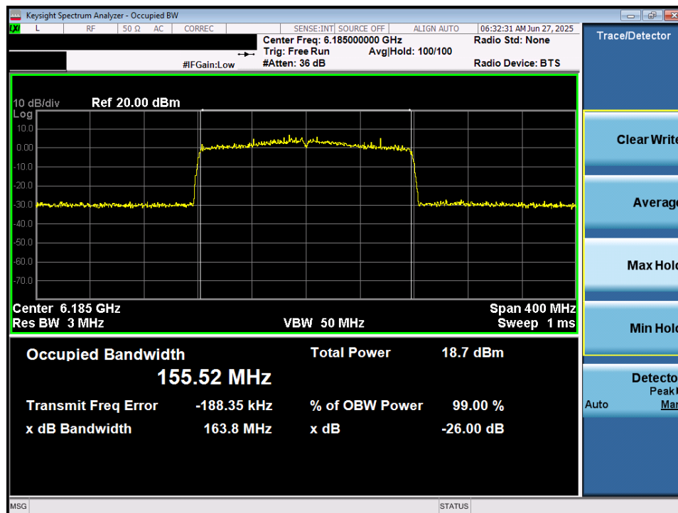
Plot 7-13. 26dB Bandwidth Plot MIMO ANT1 (160MHz 802.11ax/be (Full Tones) (UNII Band 5) – Ch. 47) - LPI/SP
