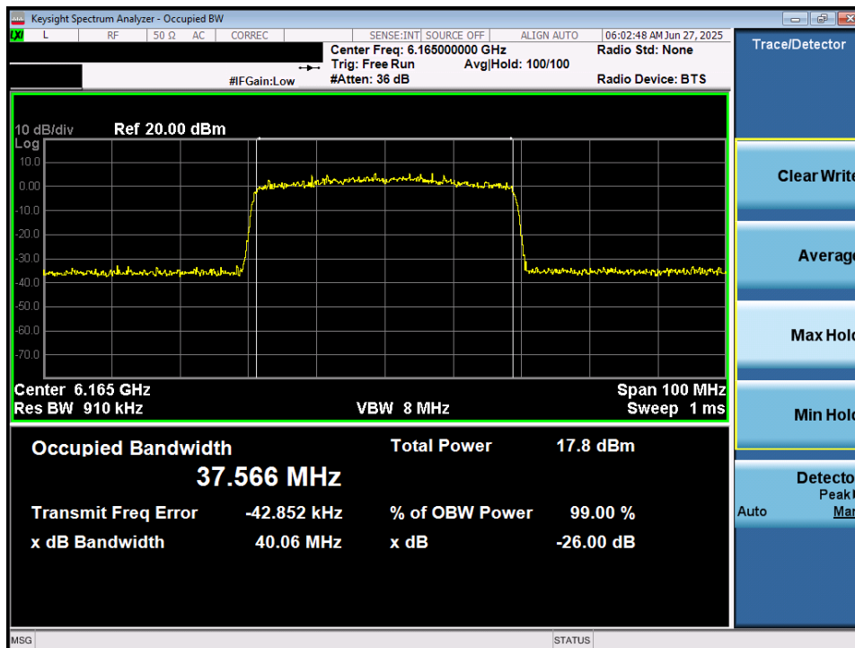
Plot 7-11. 26dB Bandwidth Plot MIMO ANT1 (40MHz 802.11ax/be (Full Tones) (UNII Band 5) – Ch. 43) – LPI/SP
