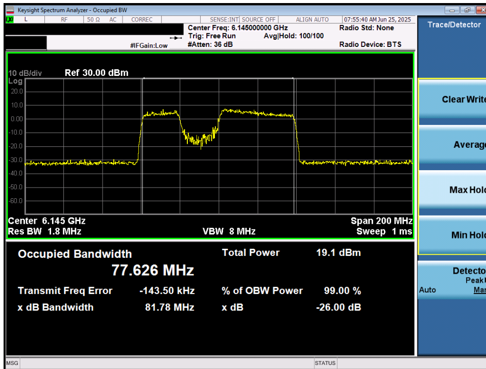
Plot 7-7. 26dB Bandwidth Plot MIMO ANT1 (80MHz 802.11be (484+242 Tones) (UNII Band 5) – Ch. 39) – LPI/SP
