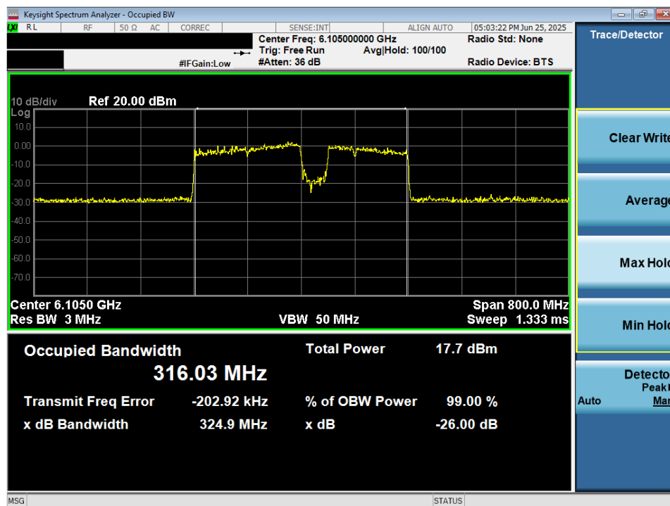
Plot 7-23. 26dB Bandwidth Plot MIMO ANT2 (320MHz 802.11be (3*996+484 Tones) (UNII Band 5) – Ch. 31) LPI/SP
