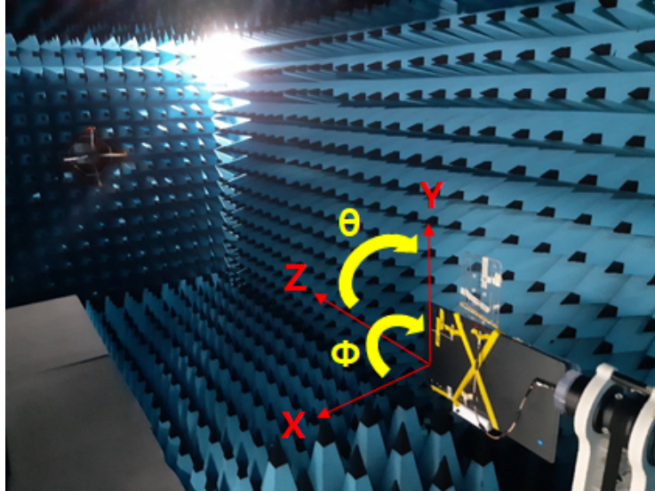
Figure 1: Geometry for SM-X930 for Radiation patterns.
