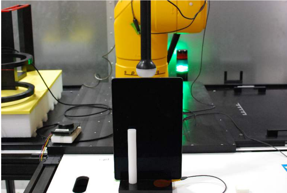
Test Setup Photo 3 Digitizer, Top Side, 0mm
