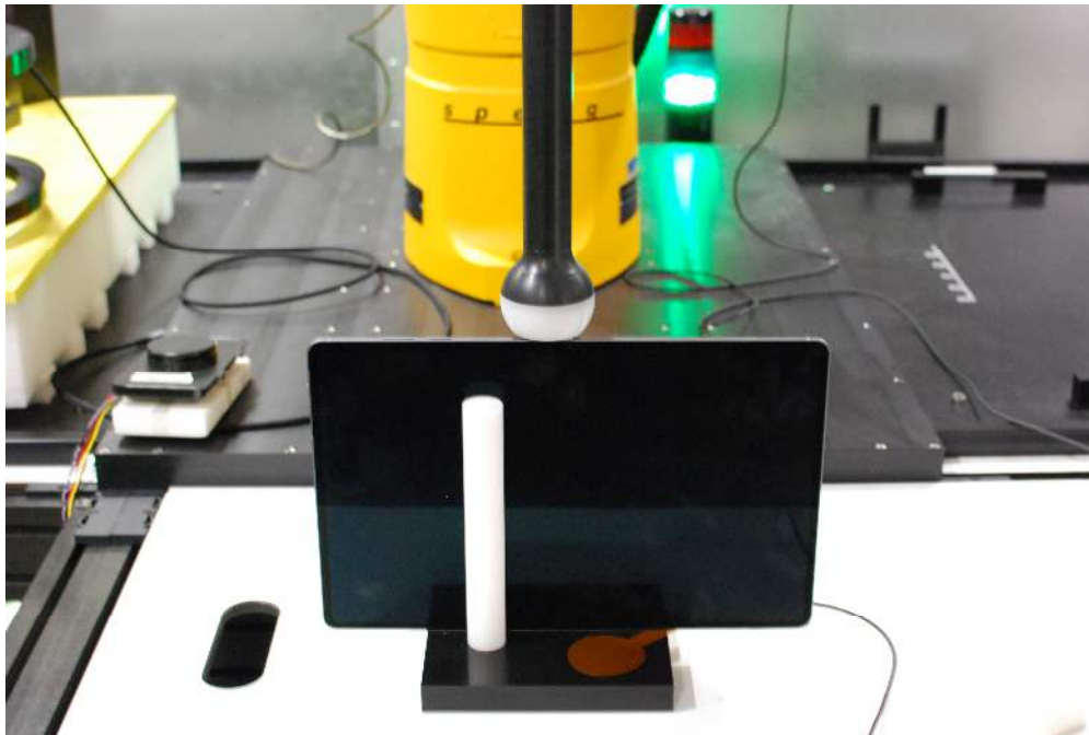
Test Setup Photo 5 Digitizer, Right Side, 0mm
