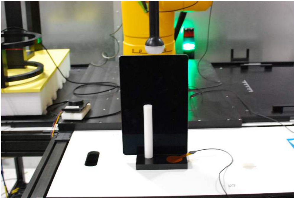
Test Setup Photo 4 Digitizer, Bottom Side, 0mm
