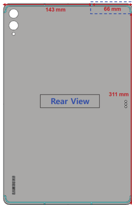
Figure I-3 DUT Dimensions
