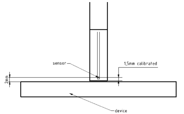
Figure I-4 EUmWVx Probe
