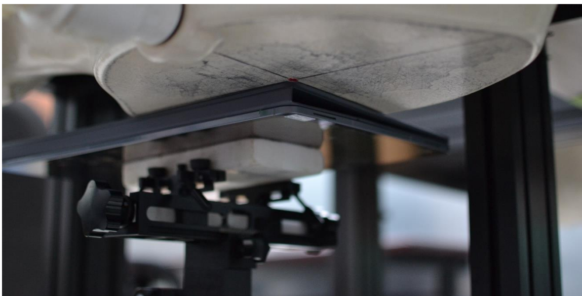
SAR Test Setup Photo 3 – Tablet with Keyboard, Back Side at 0 mm – Antenna WIFI 0
