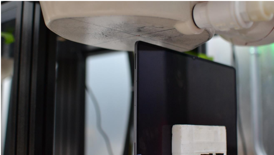
SAR Test Setup Photo 10 – Tablet, Right Edge at 8 mm
