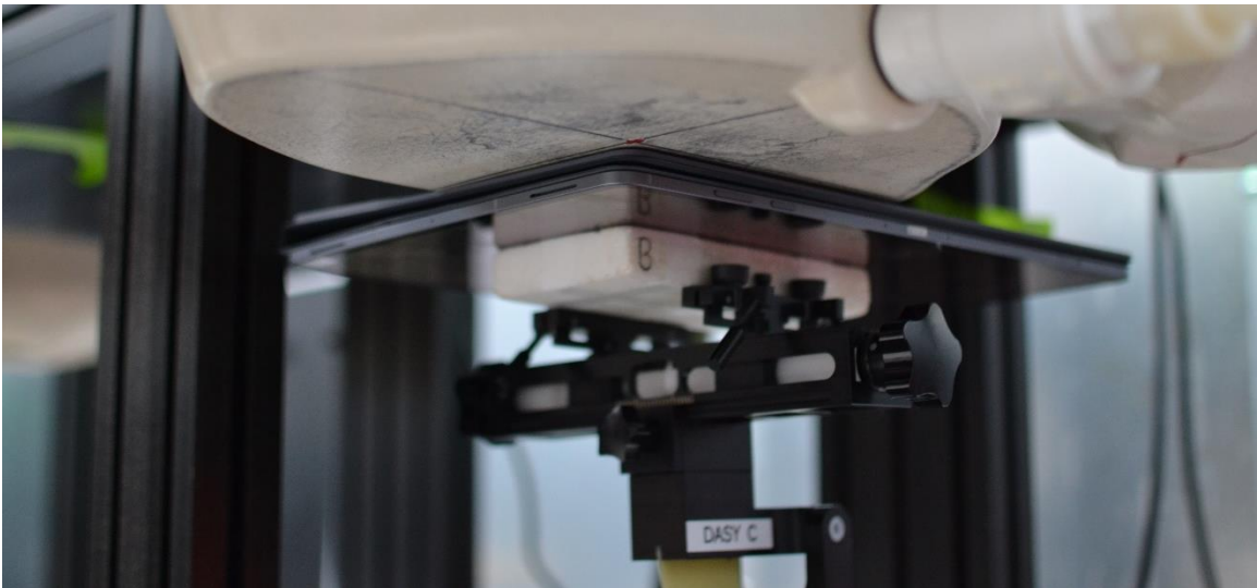
SAR Test Setup Photo 6 – Tablet with Keyboard, Back Side at 0 mm – Antenna WIFI 1
