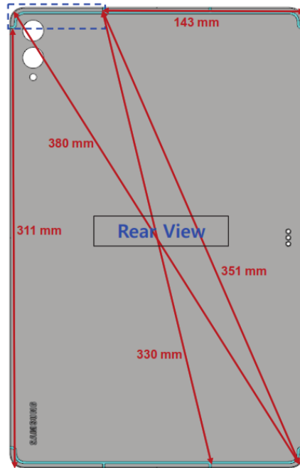
Figure I-2 DUT Dimensions
