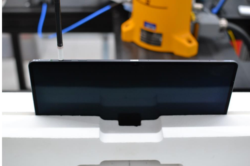
SAR Test Setup Photo 22 – Tablet, Right Edge at 2 mm – Antenna WIFI 1
