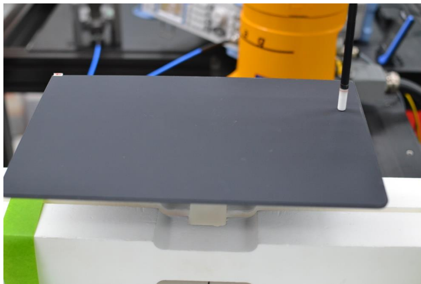
SAR Test Setup Photo 23 – Laptop with Keyboard, Bottom Edge at 2 mm
