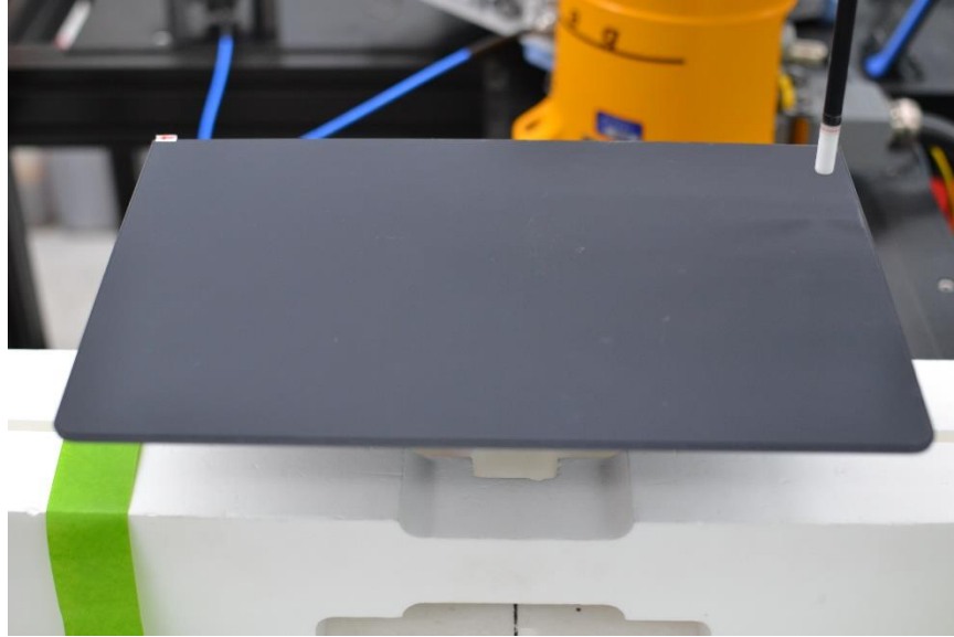
SAR Test Setup Photo 24 – Laptop with Keyboard, Bottom Edge at 9.95 mm
