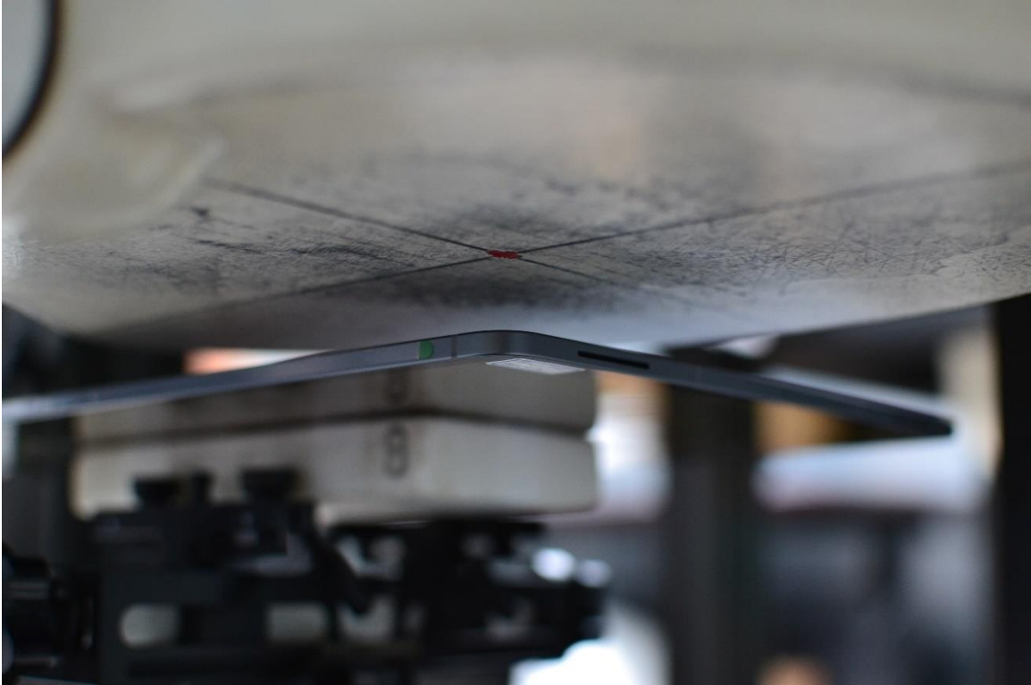
SAR Test Setup Photo 1 – Tablet, Back Side at 14 mm – Antenna WIFI 0
