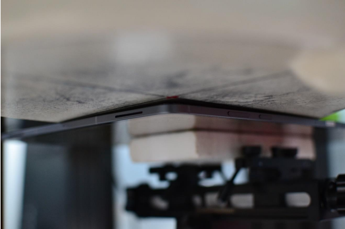
SAR Test Setup Photo 5 – Tablet, Back Side at 0 mm – Antenna WIFI 1
