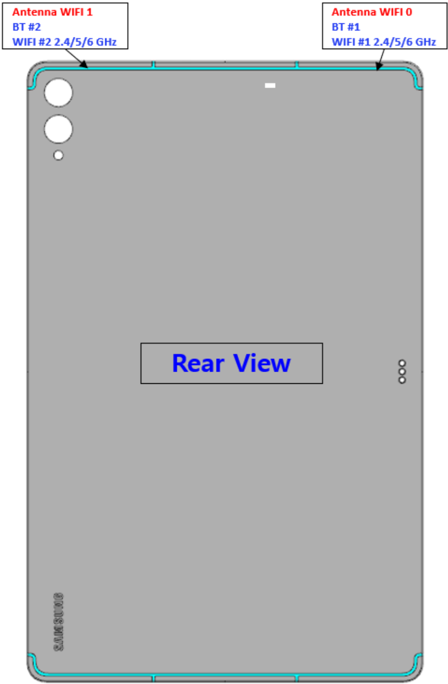
Figure I-1 DUT Antenna Locations
