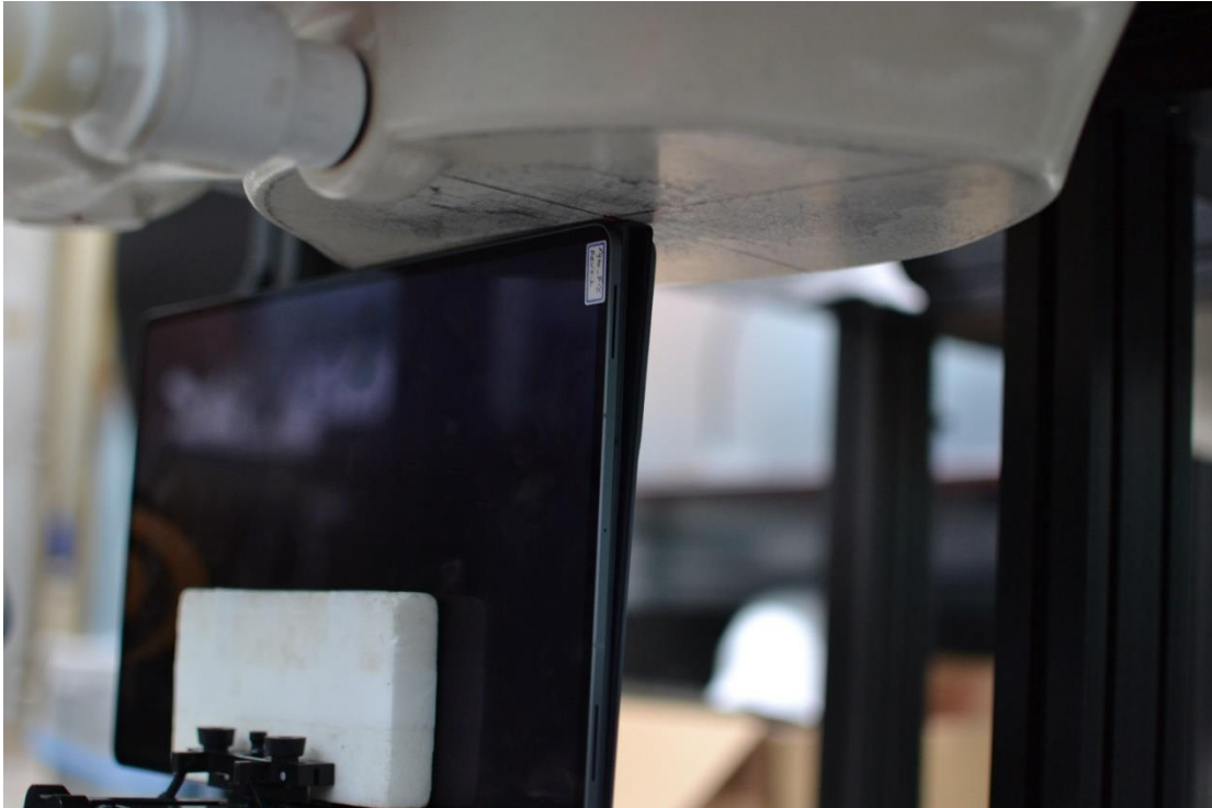
SAR Test Setup Photo 15 – Tablet with Keyboard, Left Edge at 0 mm
