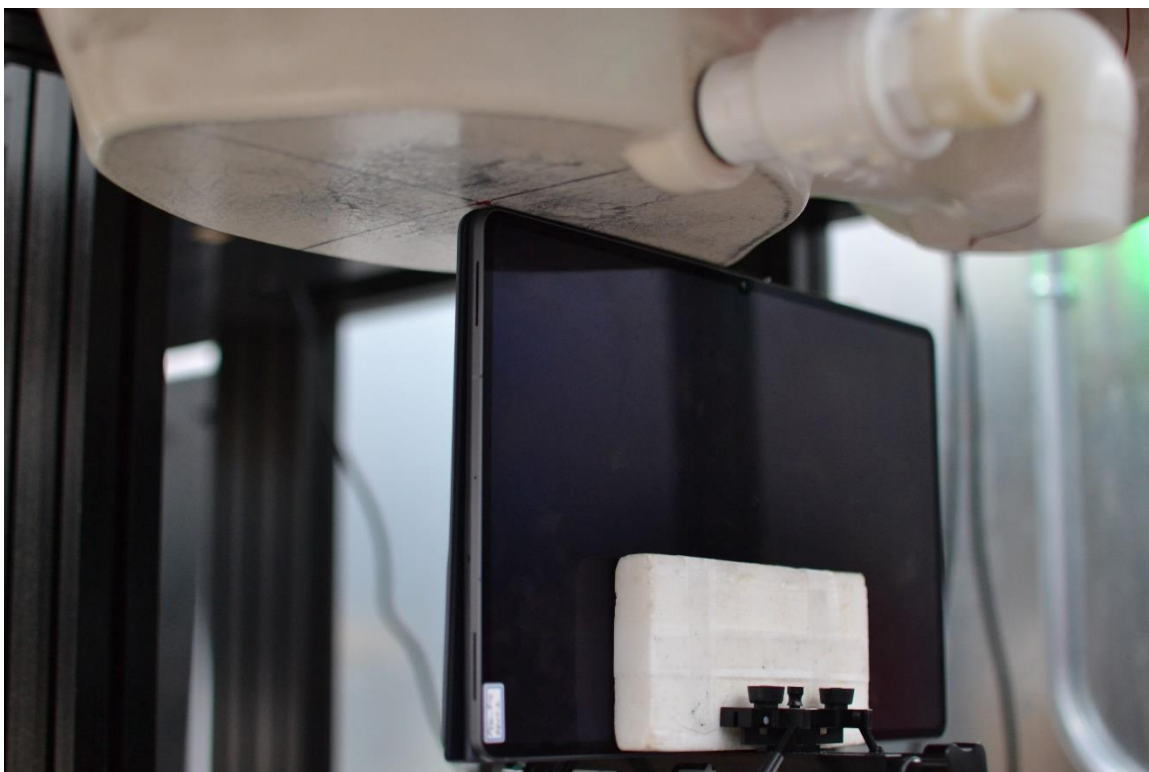
SAR Test Setup Photo 12 – Tablet with Keyboard, Right Edge at 0 mm
