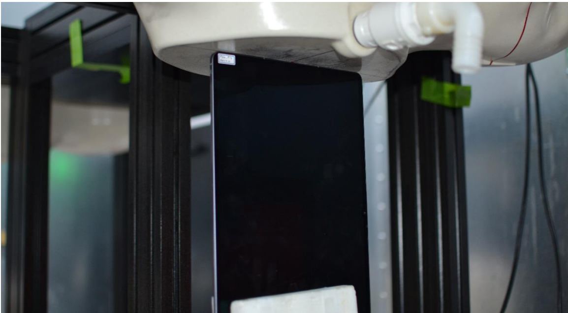
SAR Test Setup Photo 8 – Tablet, Top Edge at 0 mm
