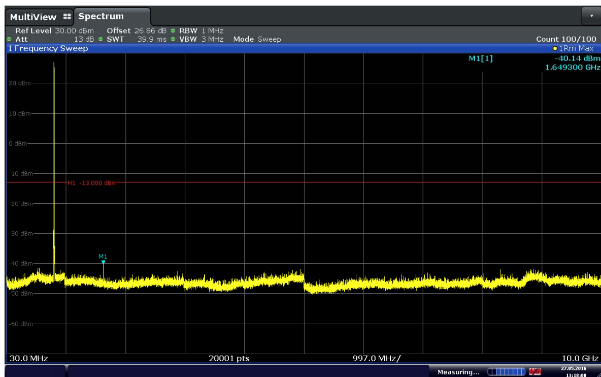
Plot 6-9. Conducted Spurious Plot (Band 5–1.4MHz–QPSK–RB Size 3–RB Offset 0–Ch.20407)
