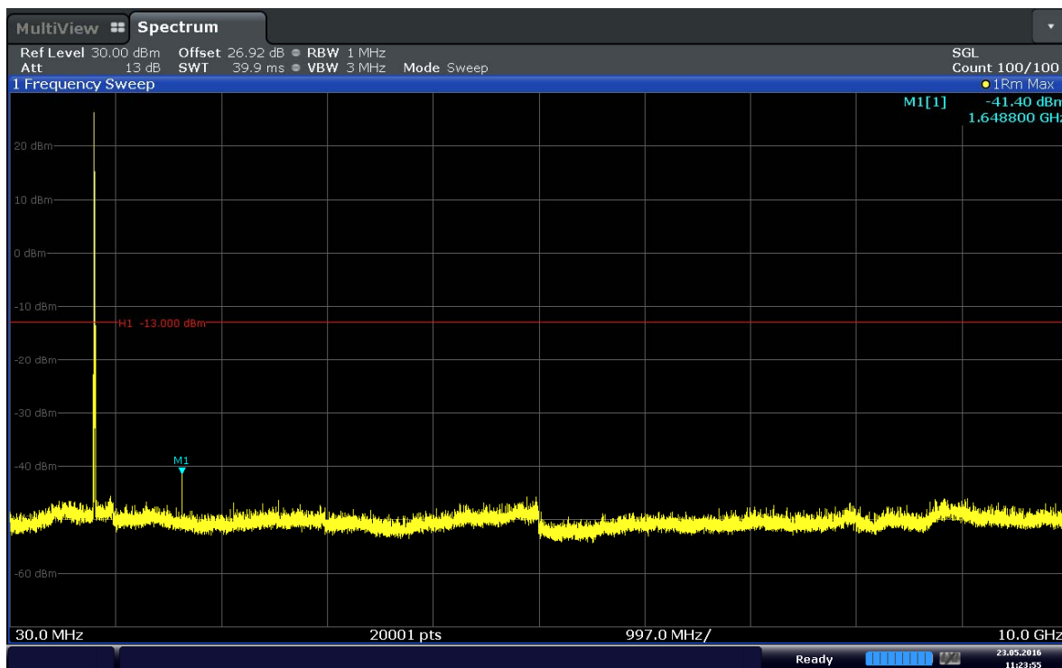
Plot 6-15. Conducted Spurious Plot (Band 5–5.0MHz–QPSK–RB Size 1–RB Offset 0– Ch.20425)
