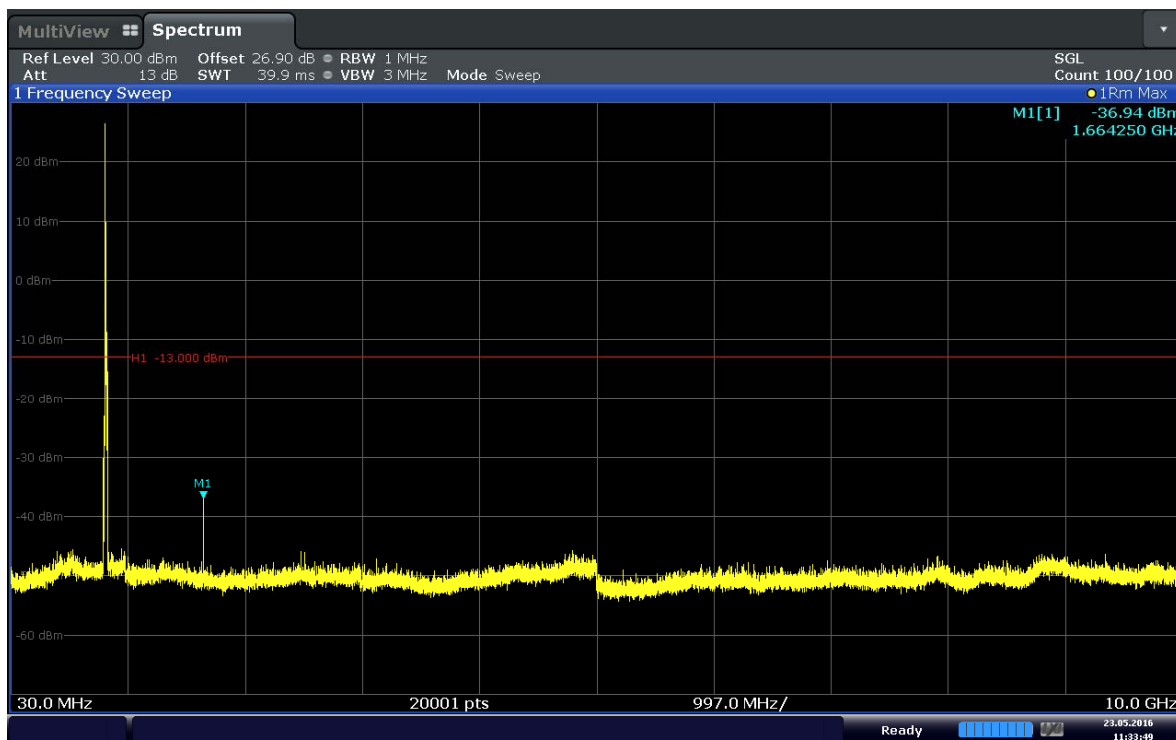
Plot 6-19. Conducted Spurious Plot (Band 5–10.0MHz–QPSK–RB Size 1–RB Offset 0– Ch.20525)
