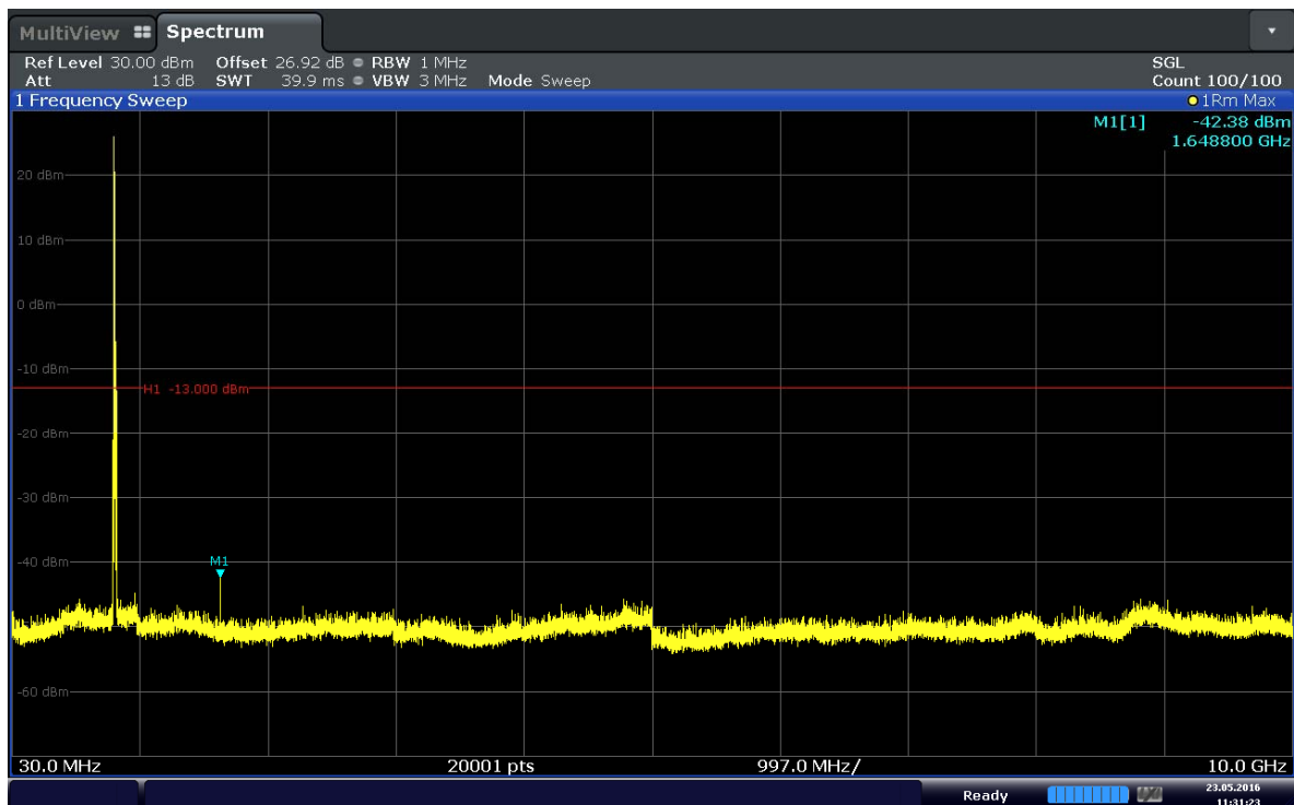
Plot 6-18. Conducted Spurious Plot (Band 5–10.0MHz–QPSK–RB Size 1–RB Offset 0– Ch.20450)
