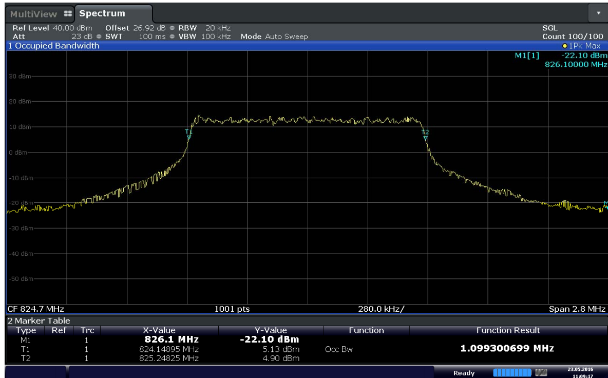
Plot 6-1. Occupied Bandwidth Plot (Band 5 – 1.4MHz QPSK - RB Size 6)
