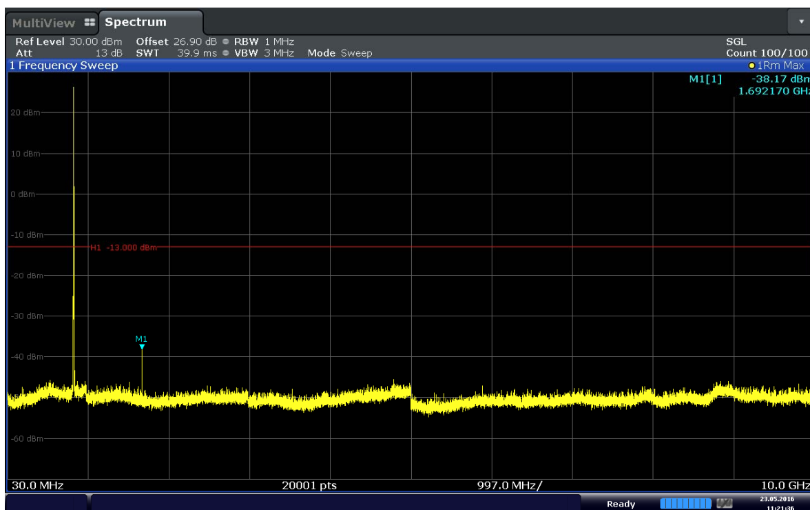
Plot 6-14. Conducted Spurious Plot (Band 5–3.0MHz–QPSK–RB Size 1–RB Offset 0– Ch.20635)
