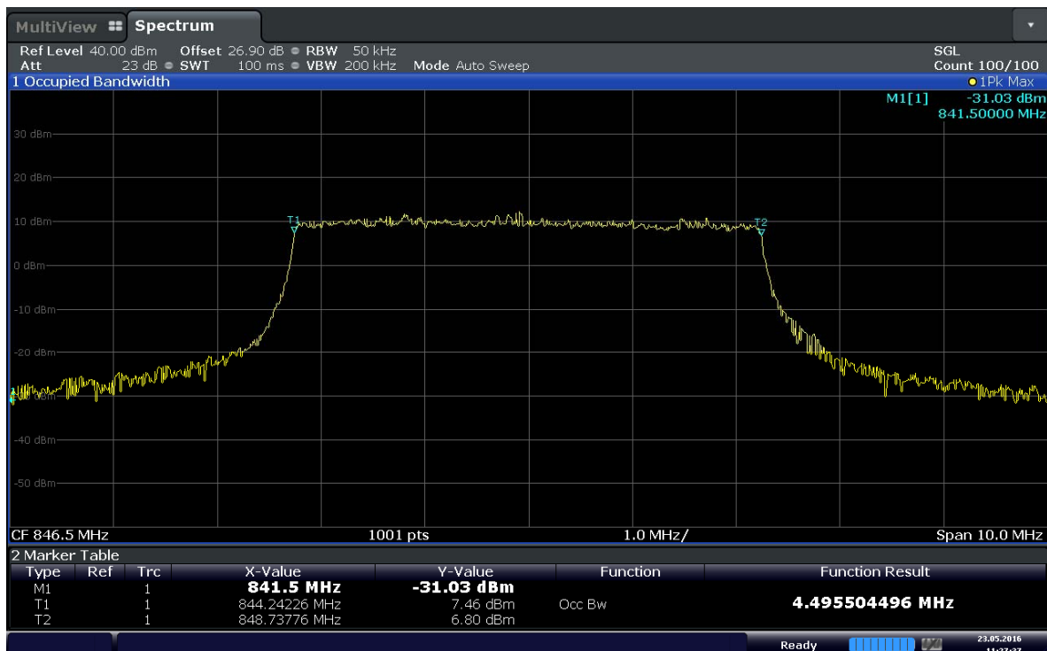
Plot 6-6. Occupied Bandwidth Plot (Band 5 - 5.0MHz 16QAM - RB Size 25)
