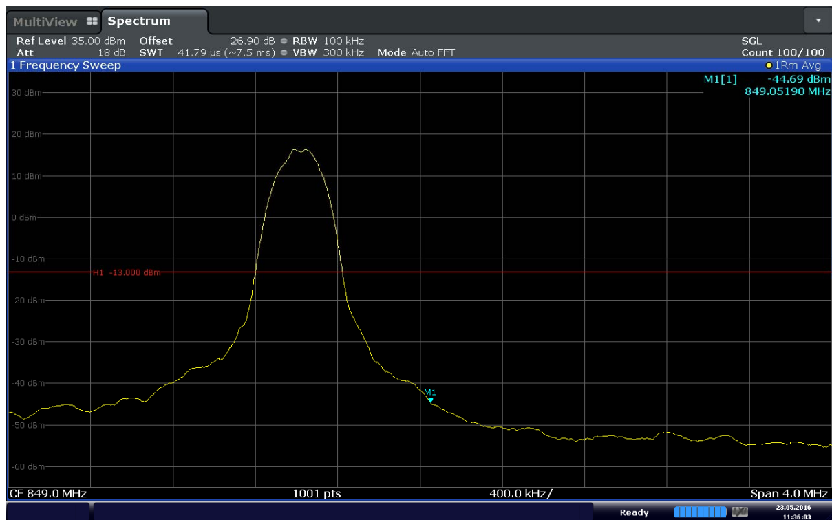
Plot 6-38. Upper Band Edge Plot (Band 5 – 10.0MHz – QPSK – RB Size 1 – RB Offset 50)
