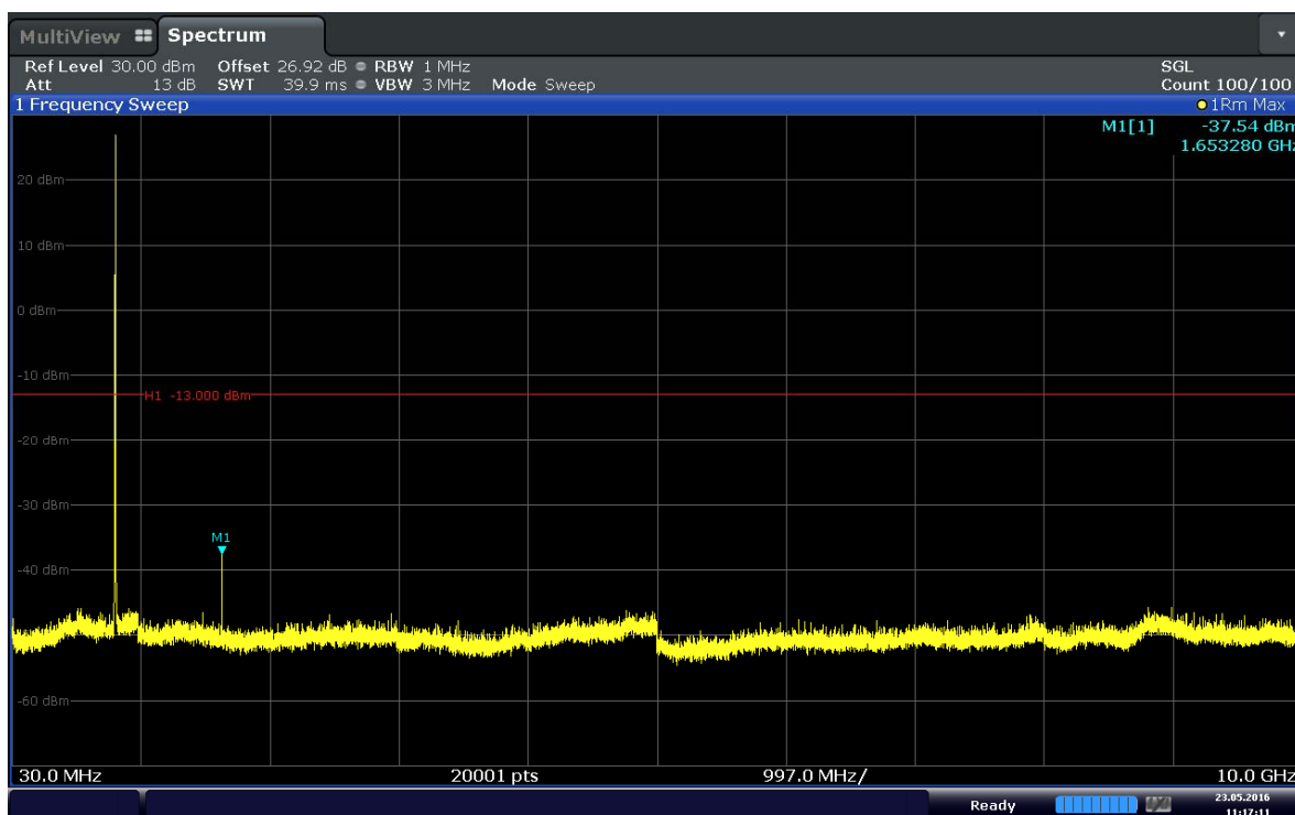
Plot 6-12. Conducted Spurious Plot (Band 5-3.0MHz-QPSK-RB Size 1-RB Offset 14- Ch.20415)
