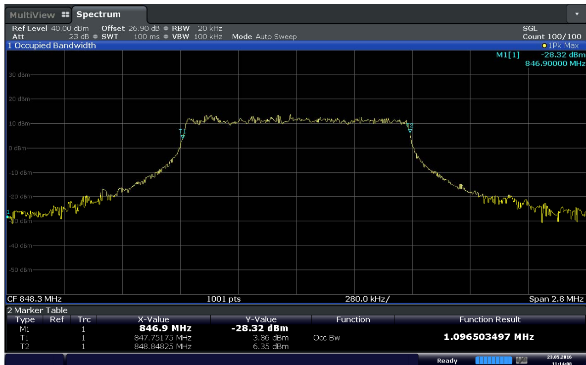
Plot 6-2. Occupied Bandwidth Plot (Band 5 – 1.4MHz 16QAM - RB Size 6)
