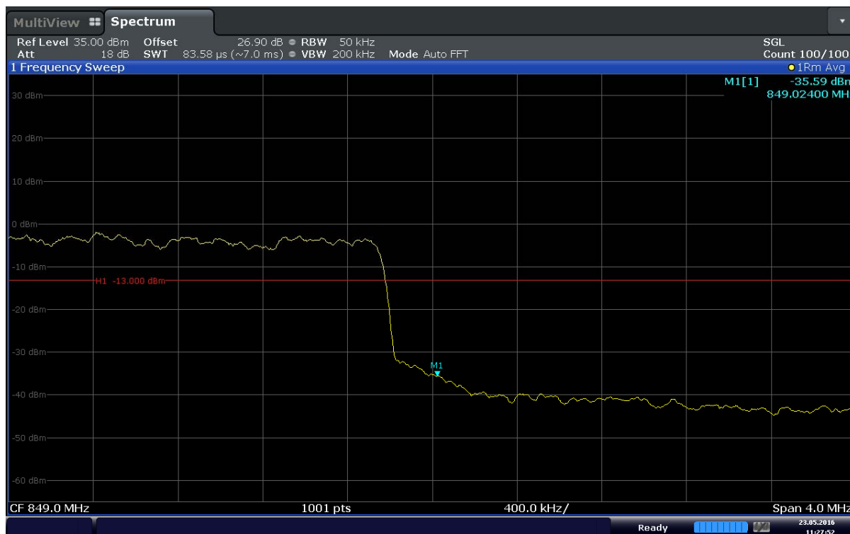
Plot 6-31. Upper Band Edge Plot (Band 5 – 5.0MHz – QPSK – RB Size 25)
