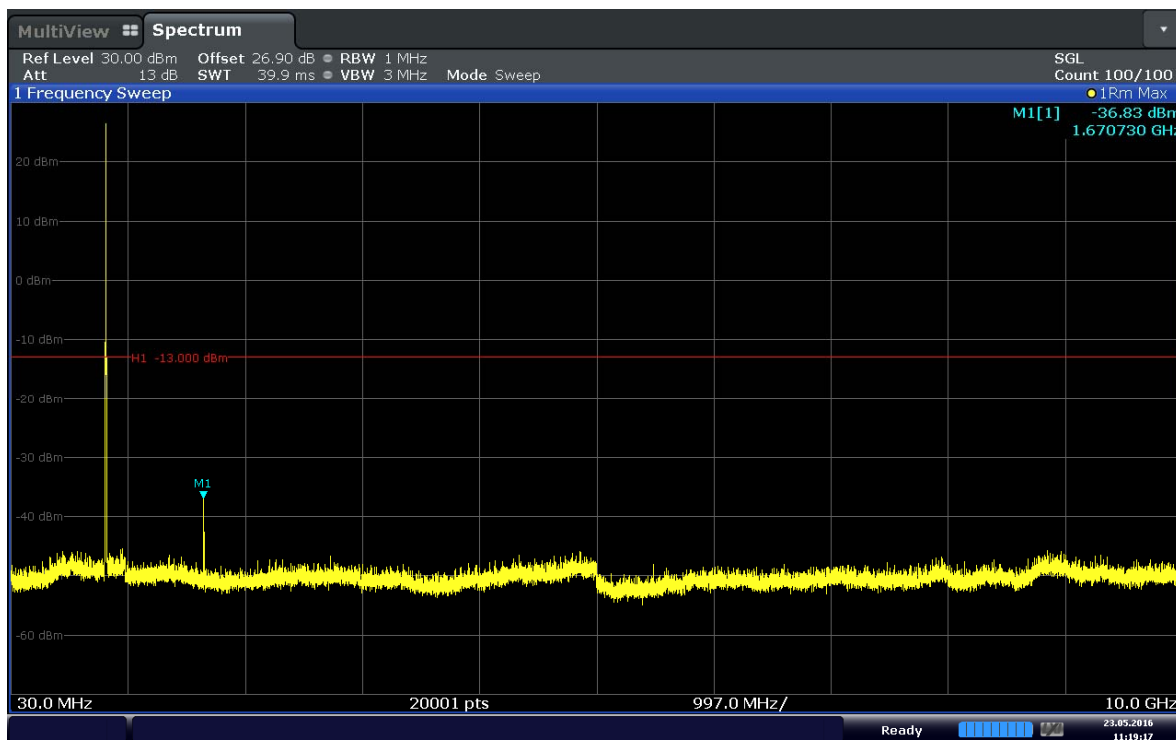
Plot 6-13. Conducted Spurious Plot (Band 5–3.0MHz–QPSK–RB Size 1–RB Offset 0– Ch.20525)
