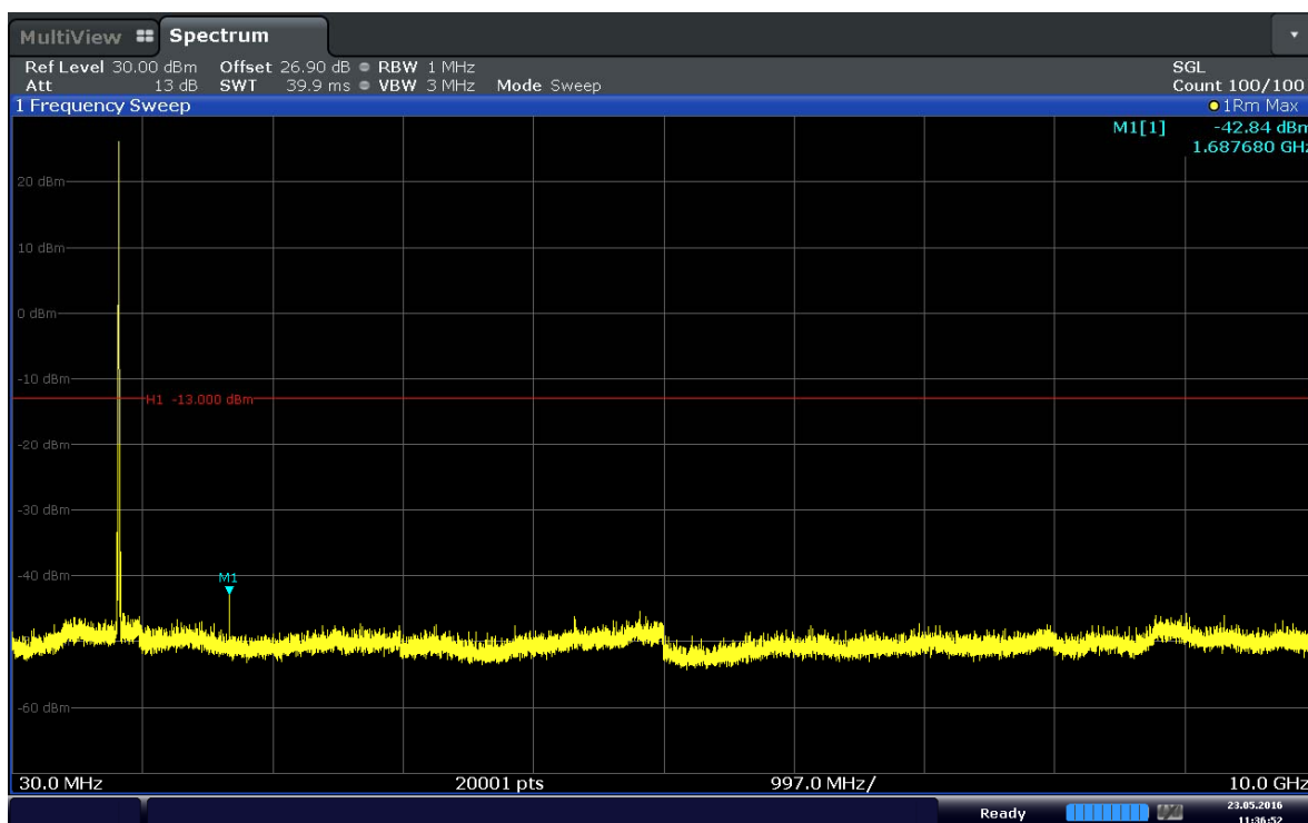
Plot 6-20. Conducted Spurious Plot (Band 5–10.0MHz–QPSK–RB Size 1–RB Offset 24– Ch.20600)
