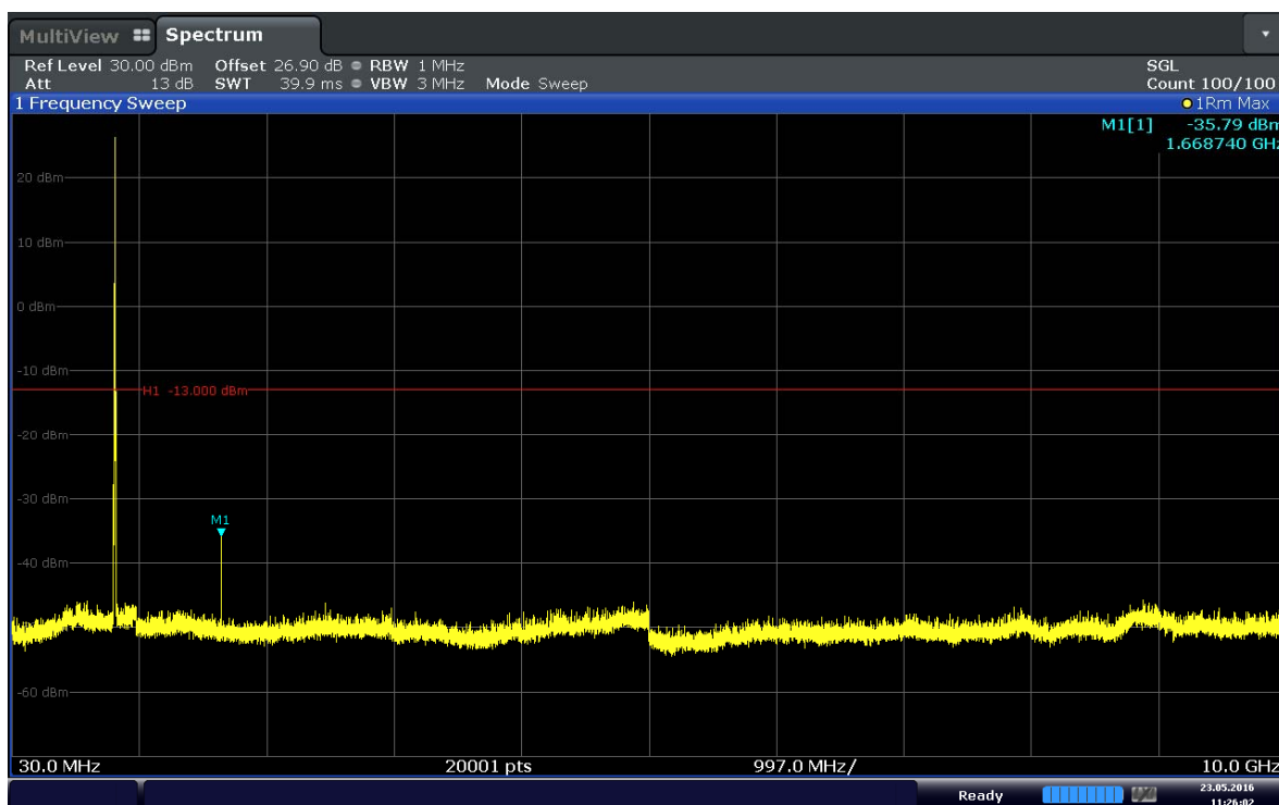
Plot 6-16. Conducted Spurious Plot (Band 5–5.0MHz–QPSK–RB Size 1–RB Offset 0– Ch.20525)
