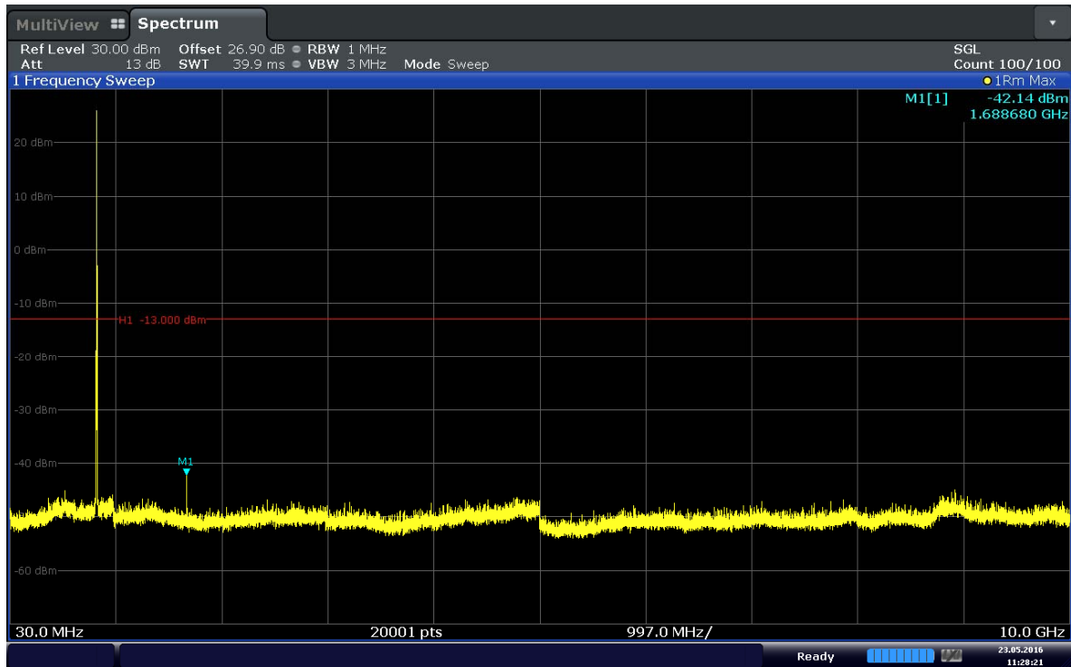
Plot 6-17. Conducted Spurious Plot (Band 5–5.0MHz–QPSK–RB Size 1–RB Offset0– Ch.20625)
