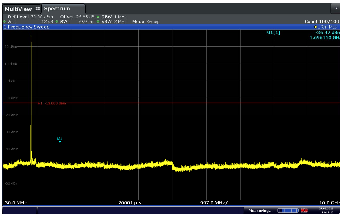
Plot 6-11. Conducted Spurious Plot (Band 5-1.4MHz-QPSK-RB Size 1-RB Offset 5- Ch.20643)
