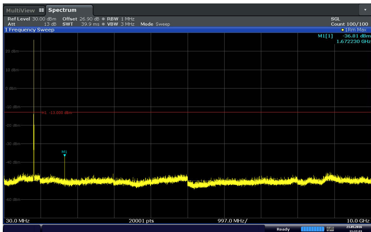
Plot 6-10. Conducted Spurious Plot (Band 5–1.4MHz–QPSK–RB Size 1–RB Offset 0–Ch.20525)
