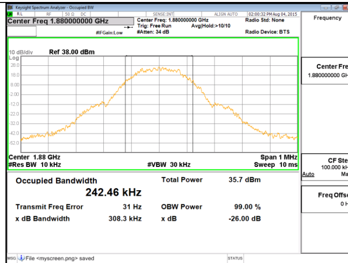
GSM1900 GPRS Mid channel
