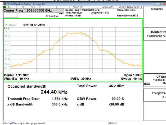
GSM1900 GPRS High channel
