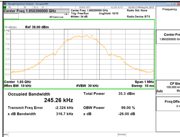
GSM1900 GPRS Low channel
