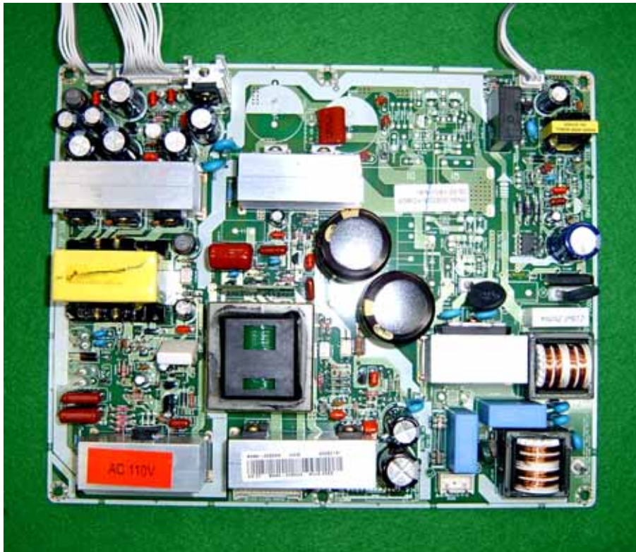
SMPS board top view
