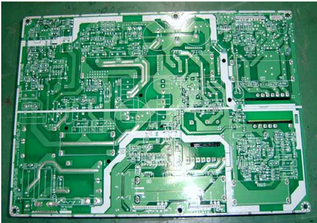
SMPS board top view
