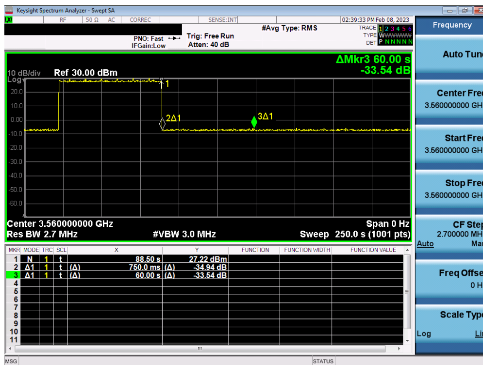
Plot 21. Conducted Measurement - RF transmission stops (WINNF.FT.C.RLQ.1) – NR
