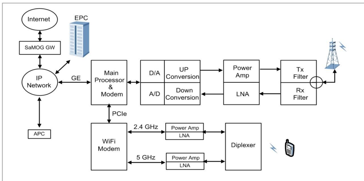
Figure 10. SOL230 Traffic Flow (WiFi)
