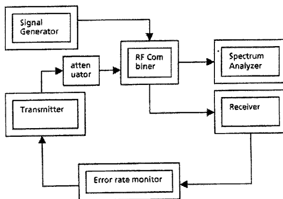
Figure 1 - Block diagram processing gain test setup
