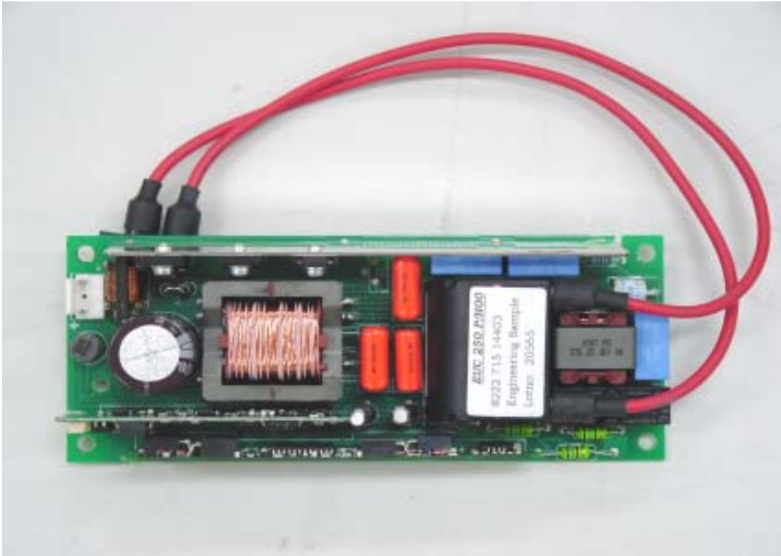
Ballast board top view
