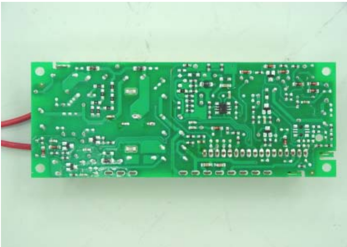
Ballast board bottom view
