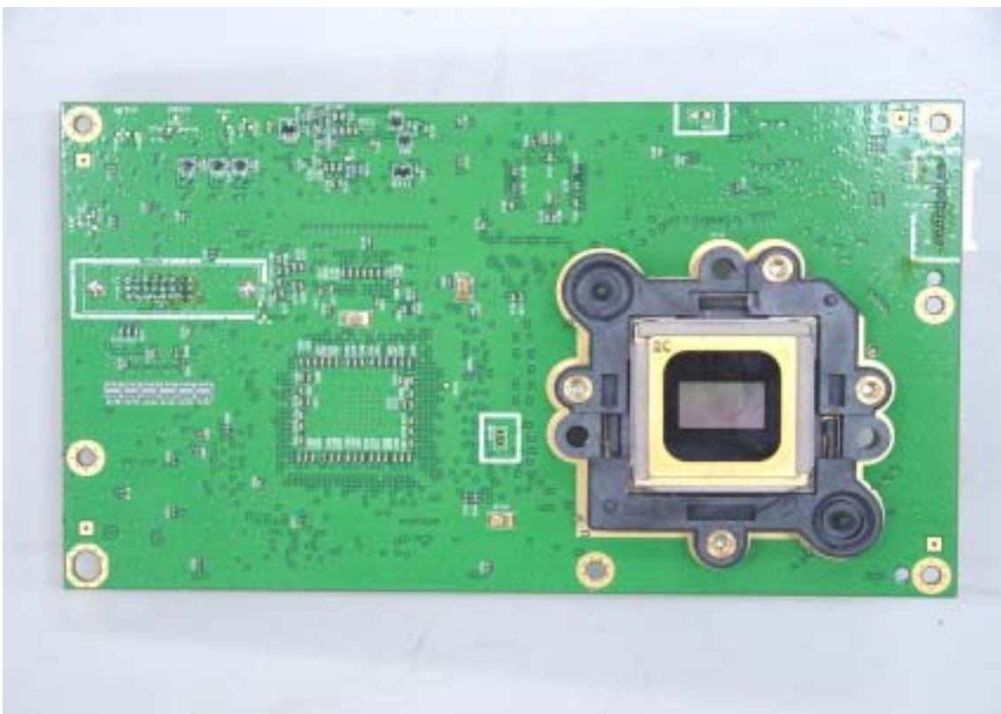
DVD board bottom view
