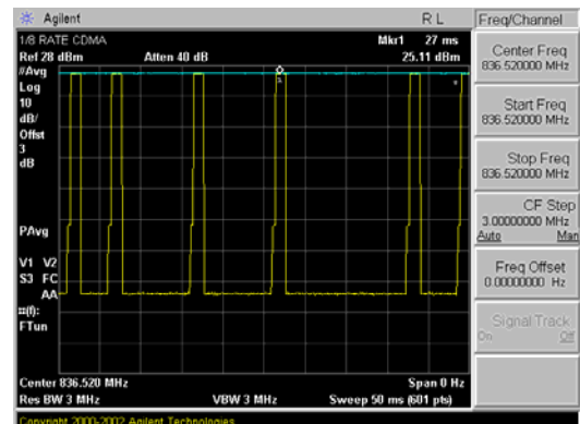
Figure 26 Zero-Span Plots
