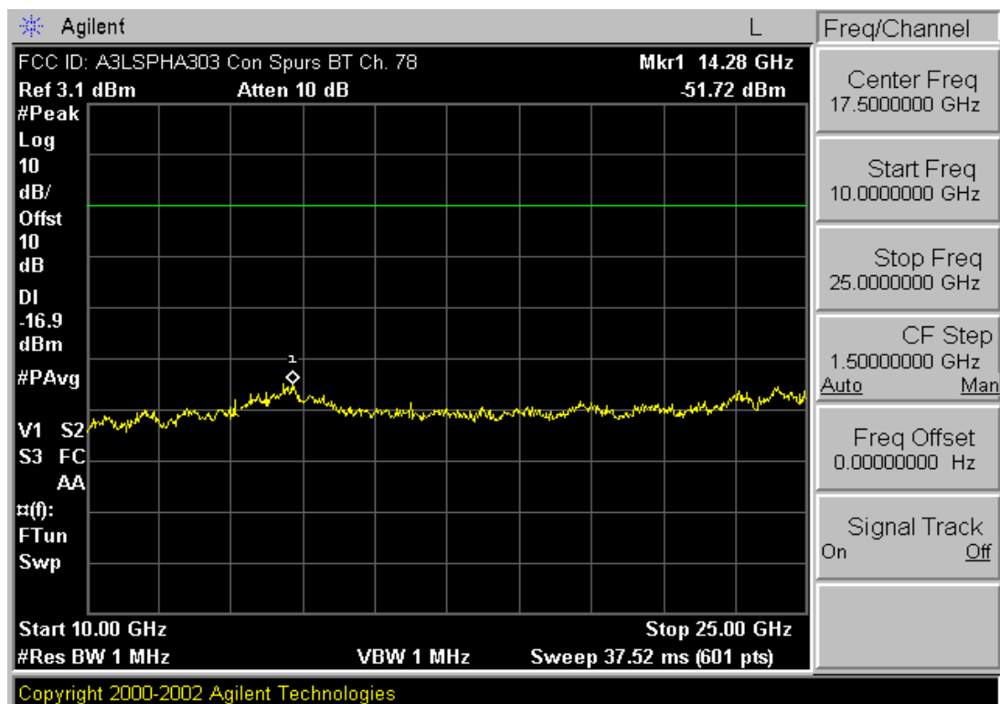
Plot 6-17. Conducted Spurious Plot (Bluetooth – Ch. 78)
