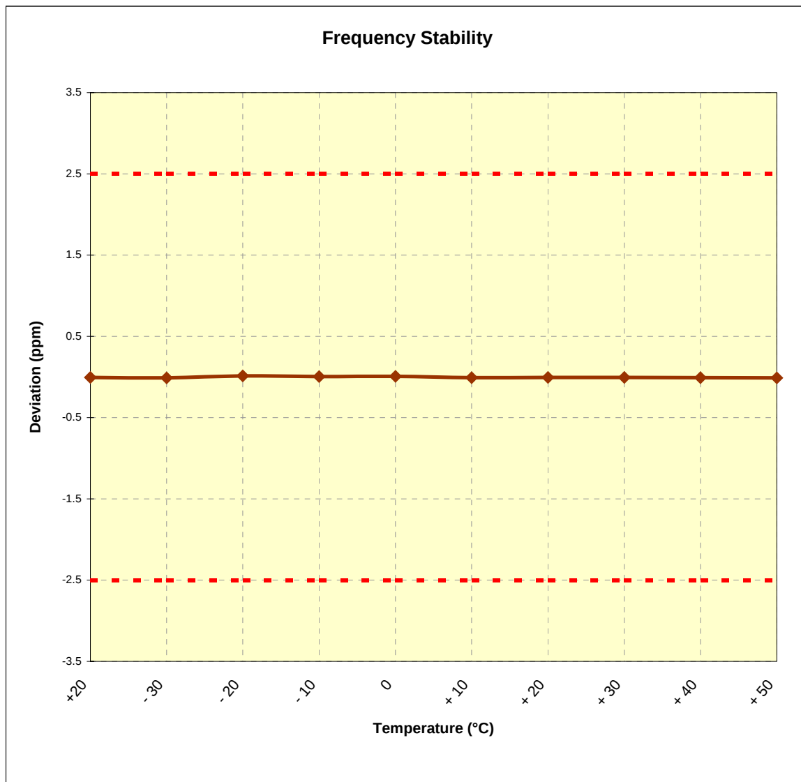
Figure 6-2. Frequency Stability Graph (PCS CDMA Mode – Ch. 600)
