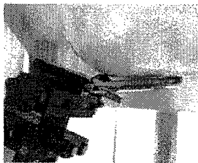
Figure 8.4 Left Head SAR Test Setup -- Cheek / Touch Position--
