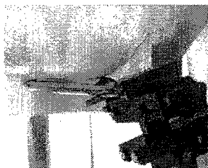
Figure 8.6 Right Head SAR Test Setup -- Cheek / Touch Position--
