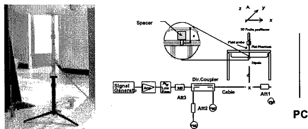
Figure 7.1 Dipole Validation Test Setup
