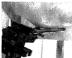
Figure 8.8 Left Head SAR Test Setup -- Cheek / Touch Position--
