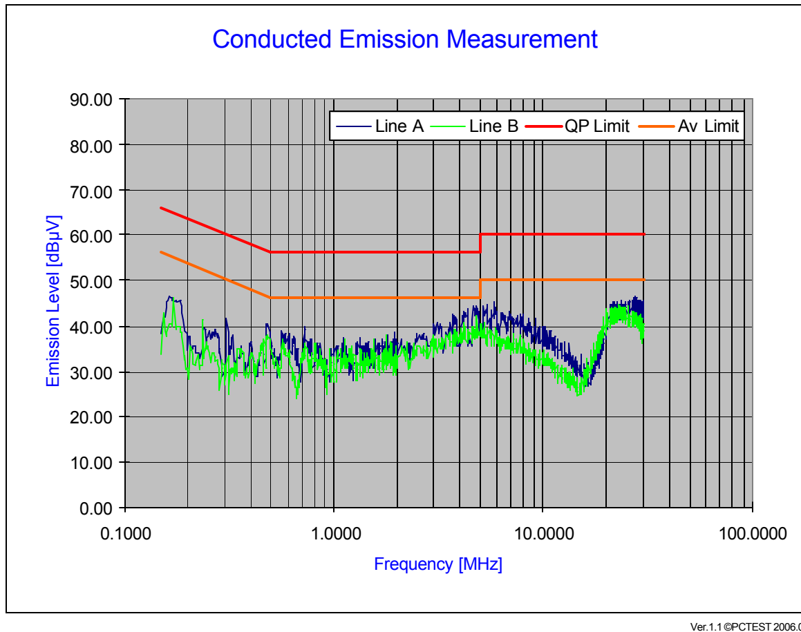
Plot 6-24. Line Conducted Plot with Bluetooth
