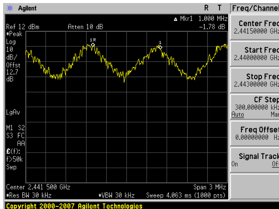
Plot 6-14. Channel Spacing Plot (Bluetooth)
