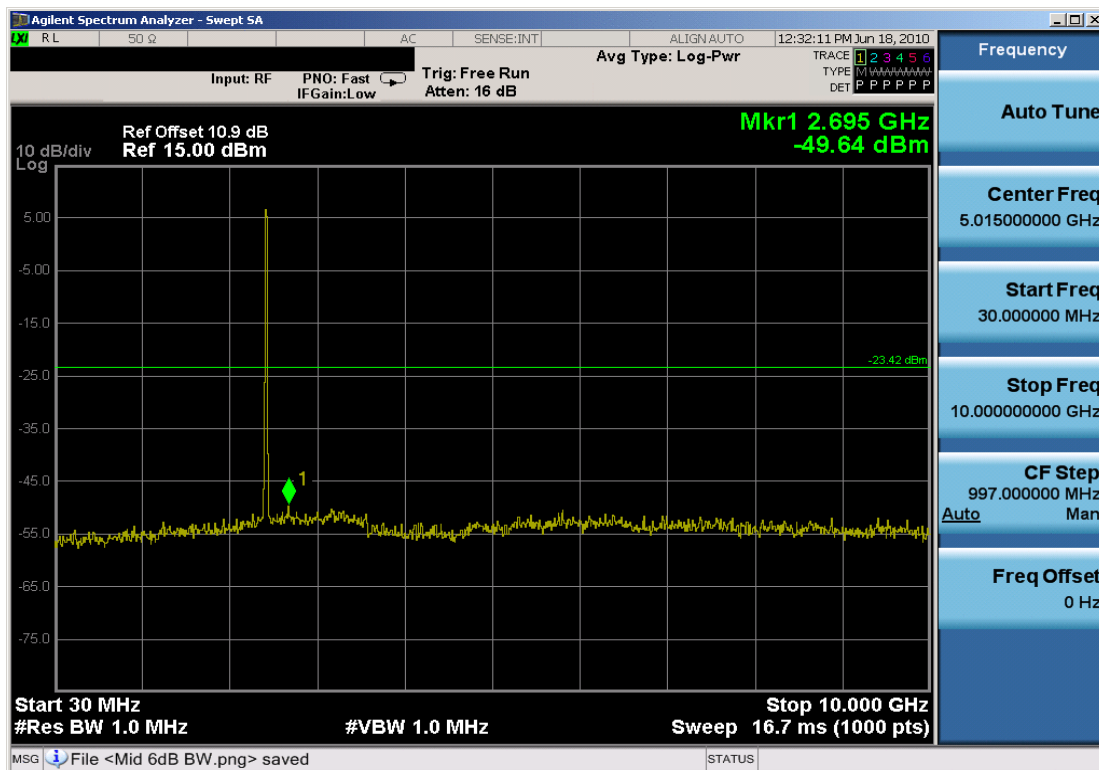
Plot 6-27. Conducted Spurious Plot (802.11b – Ch. 6, 1 Mbps)
