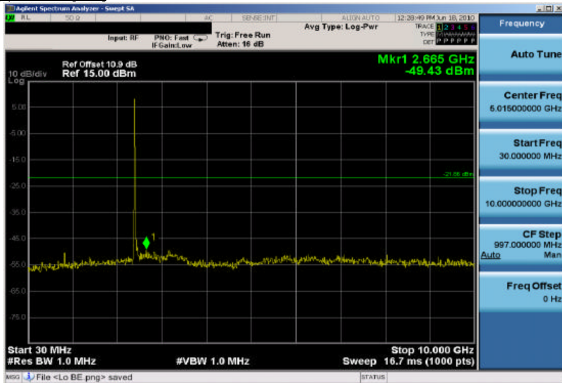
Plot 6-25. Conducted Spurious Plot (802.11b – Ch. 1, 1 Mbps)
