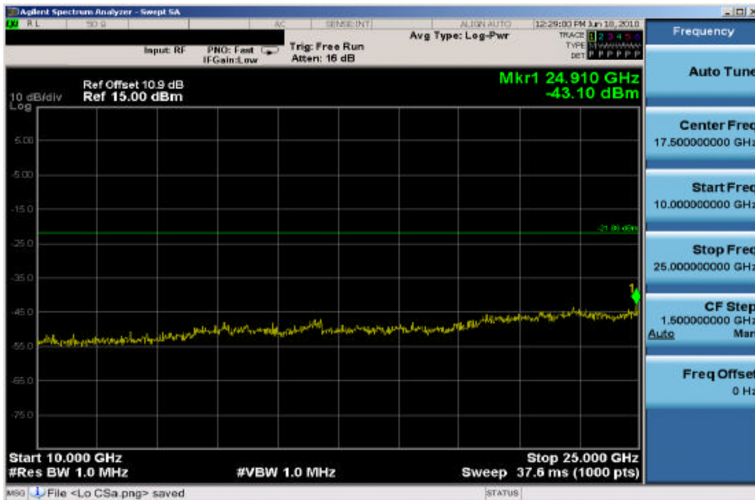
Plot 6-26. Conducted Spurious Plot (802.11b – Ch. 1, 1 Mbps)
