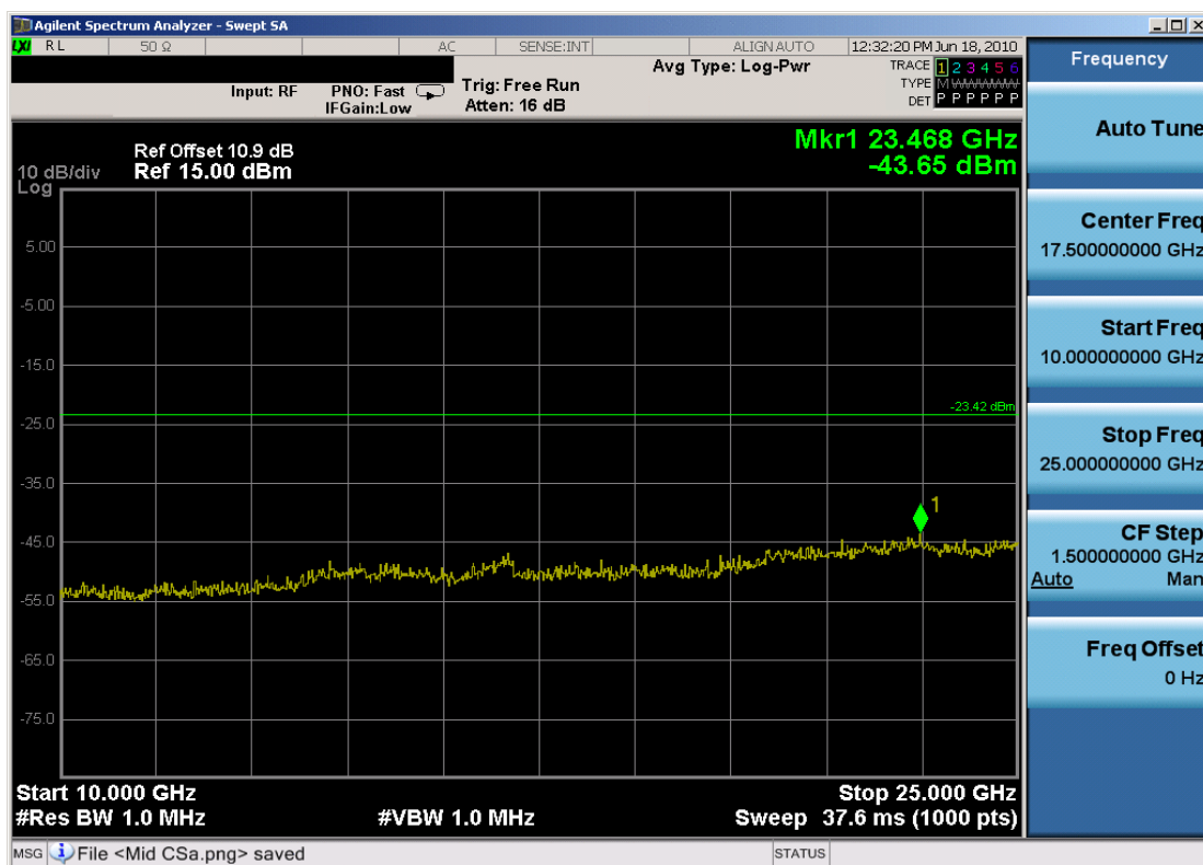
Plot 6-28. Conducted Spurious Plot (802.11b – Ch. 6, 1 Mbps)
