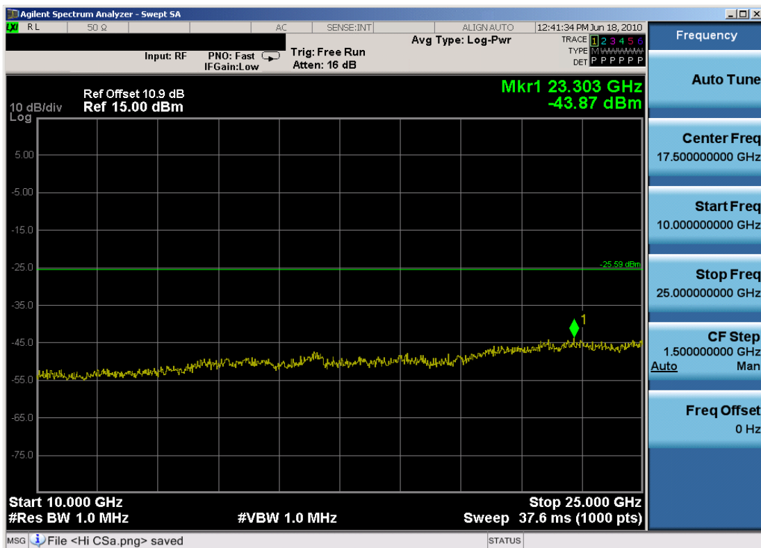
Plot 6-30. Conducted Spurious Plot (802.11b – Ch. 11, 1 Mbps)
