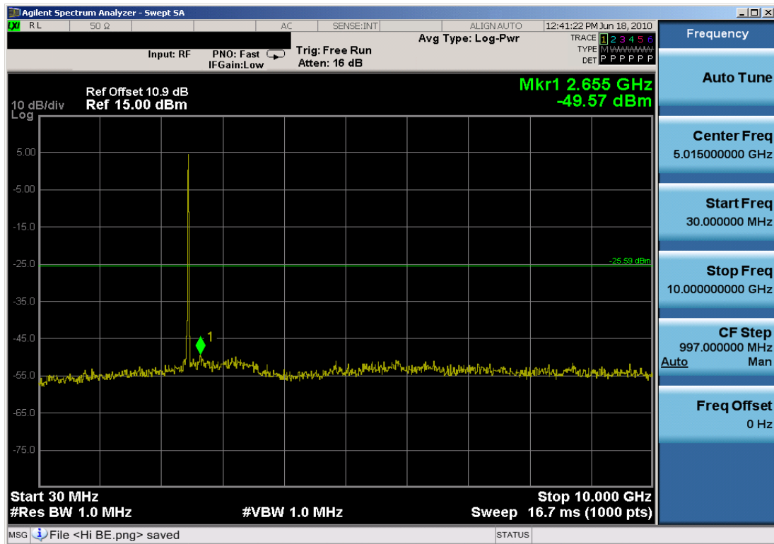
Plot 6-29. Conducted Spurious Plot (802.11b – Ch. 11, 1 Mbps)
