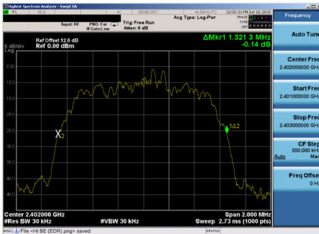
Plot 6-1. 20dB Bandwidth Plot (Bluetooth 2.1 with Enhanced Data Rates – Ch. 0)
