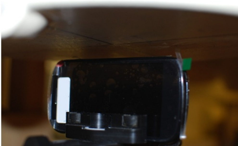
Figure 24-9 SAR Test Setup Photo – Right Edge at 1.0cm
