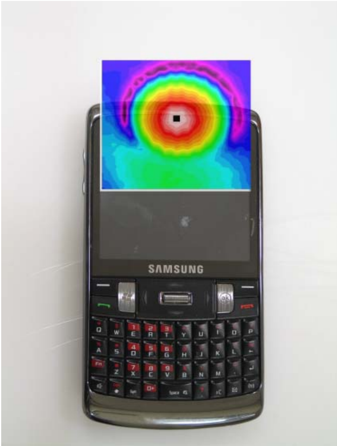
Scan overlay with actual device for CDMA (Axial)
