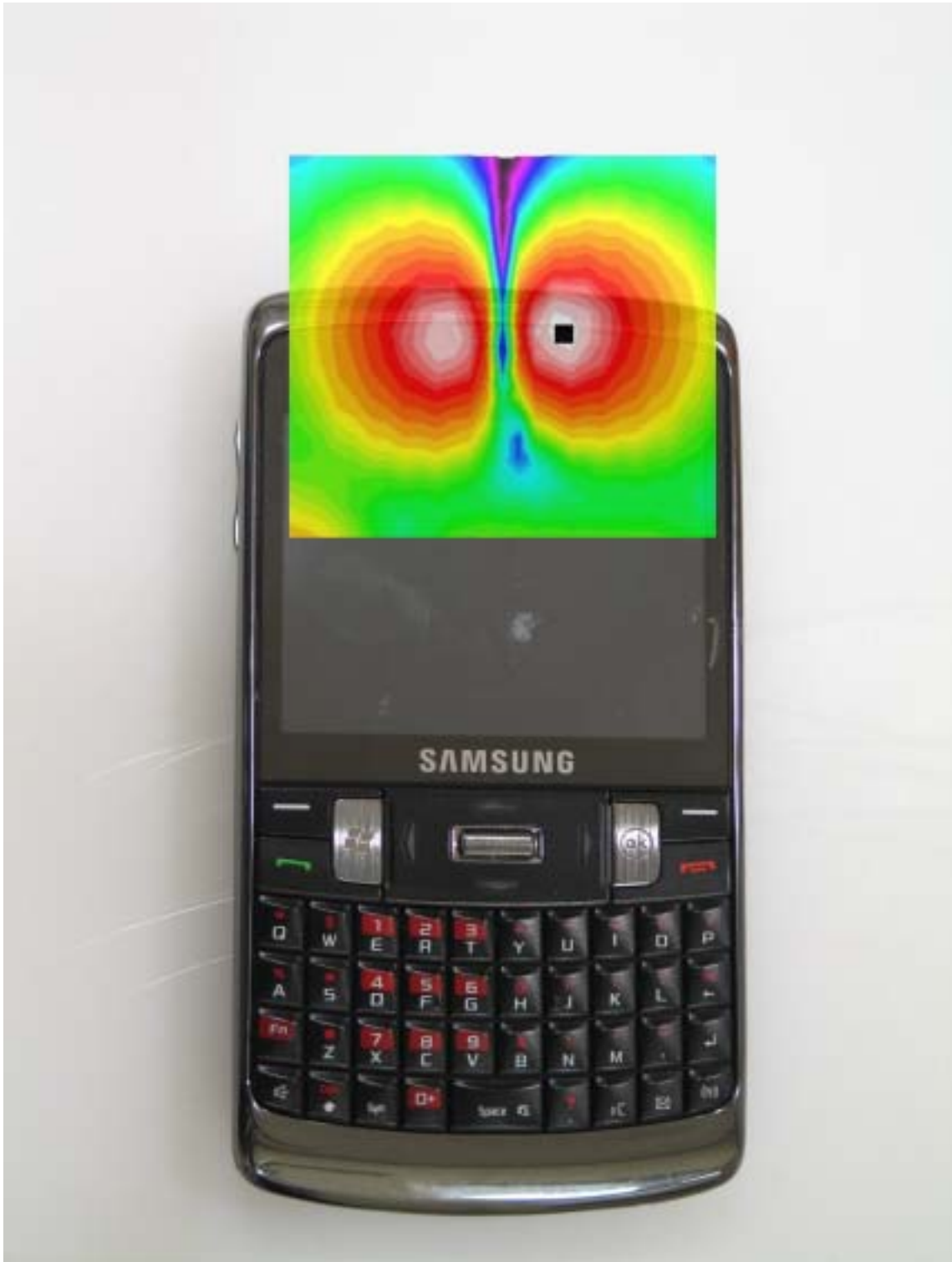
Scan overlay with actual device for GSM (Radial Transverse)
